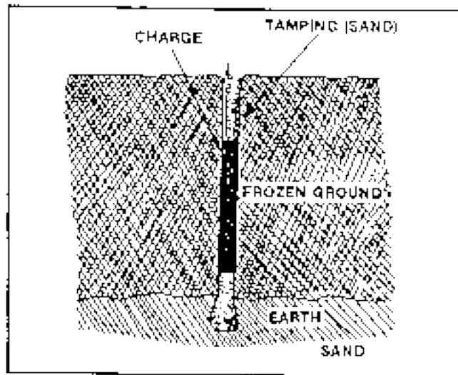
Figure B-10. Preparation of Hole Made by Shaped Charge
