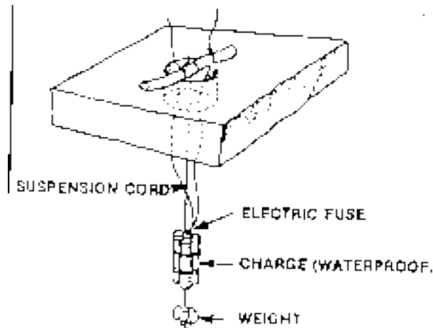
Figure B-15. Example of Suspended Charge for Demolishing Ice
