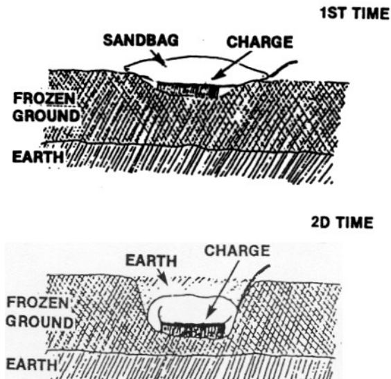
Figure B-9: Use of Pressure Charge
