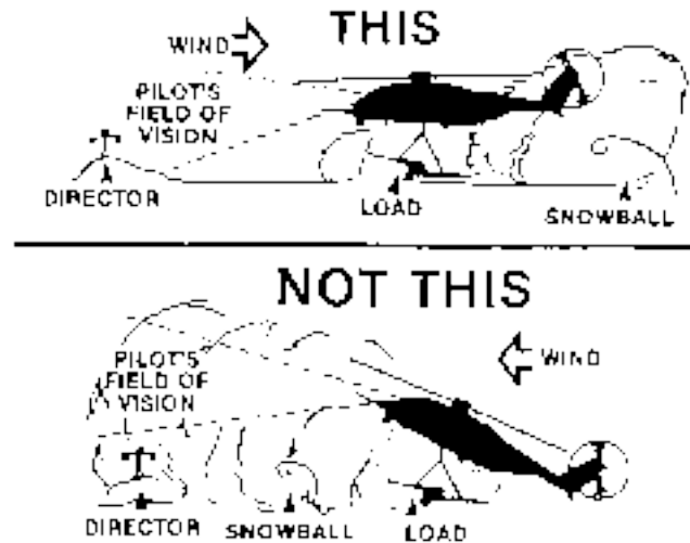
Figure 4007-1: Downwind Approach
