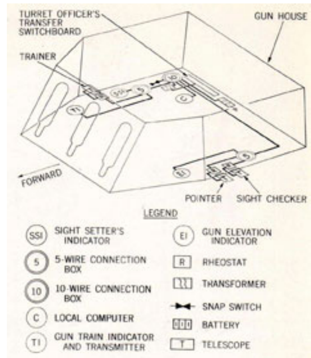
Figure 59. Instrument Illumination Circuit Schematic
