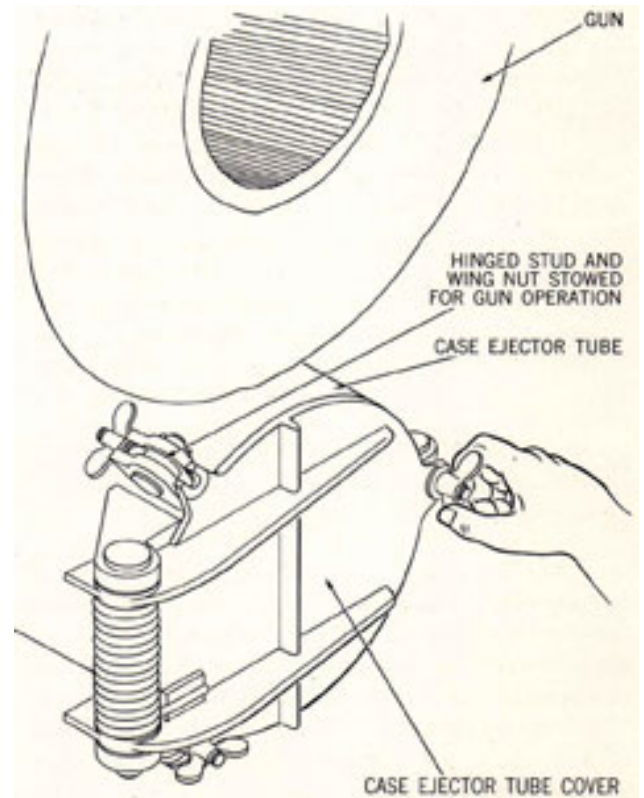
Figure 81. Securing Case Ejector Tube Cover for Action
