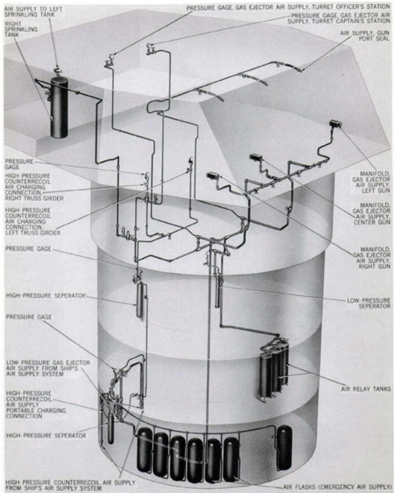
Figure 60. Gas Ejector and Counterrecoil Air Supply Pipe System. General Arrangement
