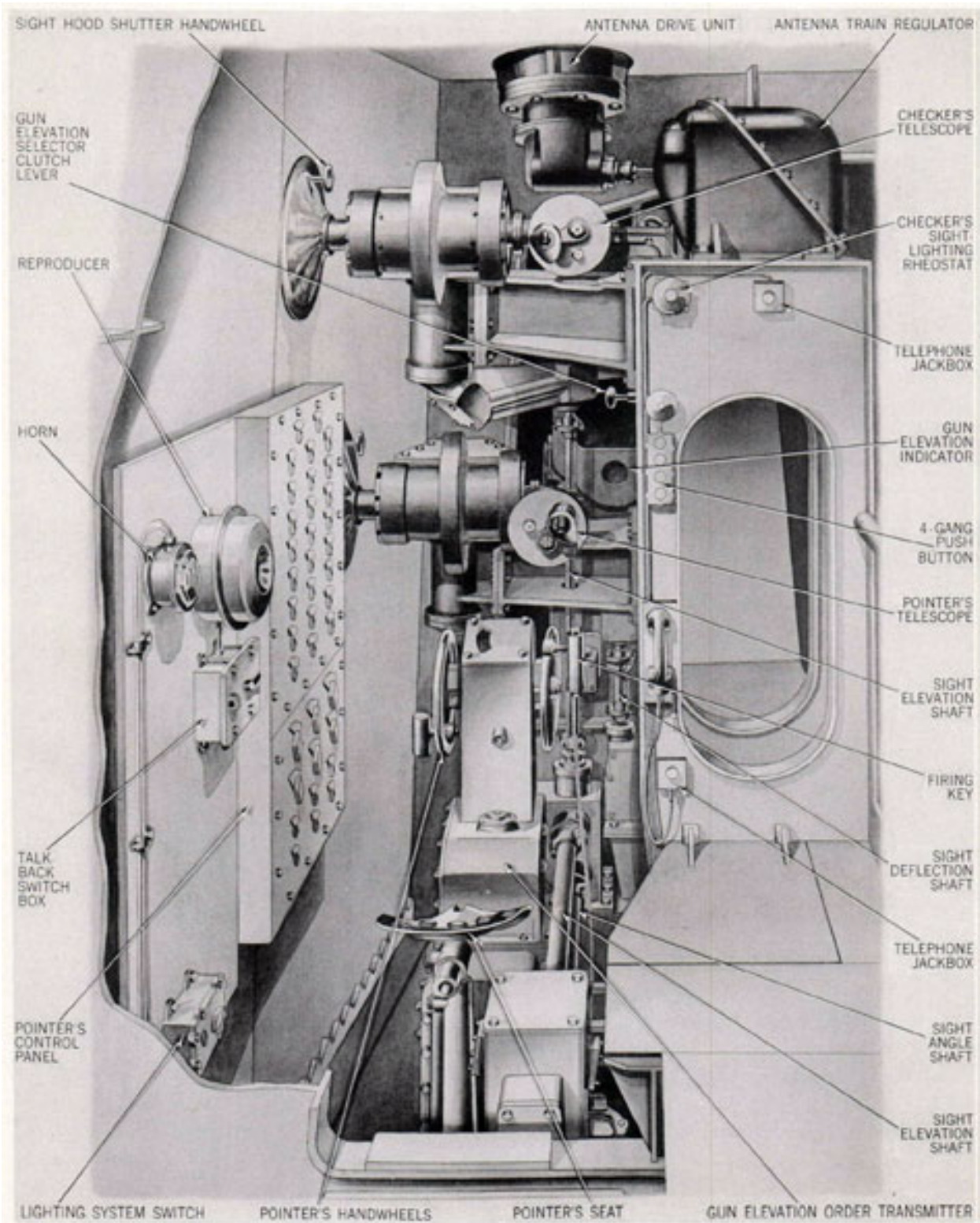
Figure 34. Pointer's and Checker's Stations General Arrangement
