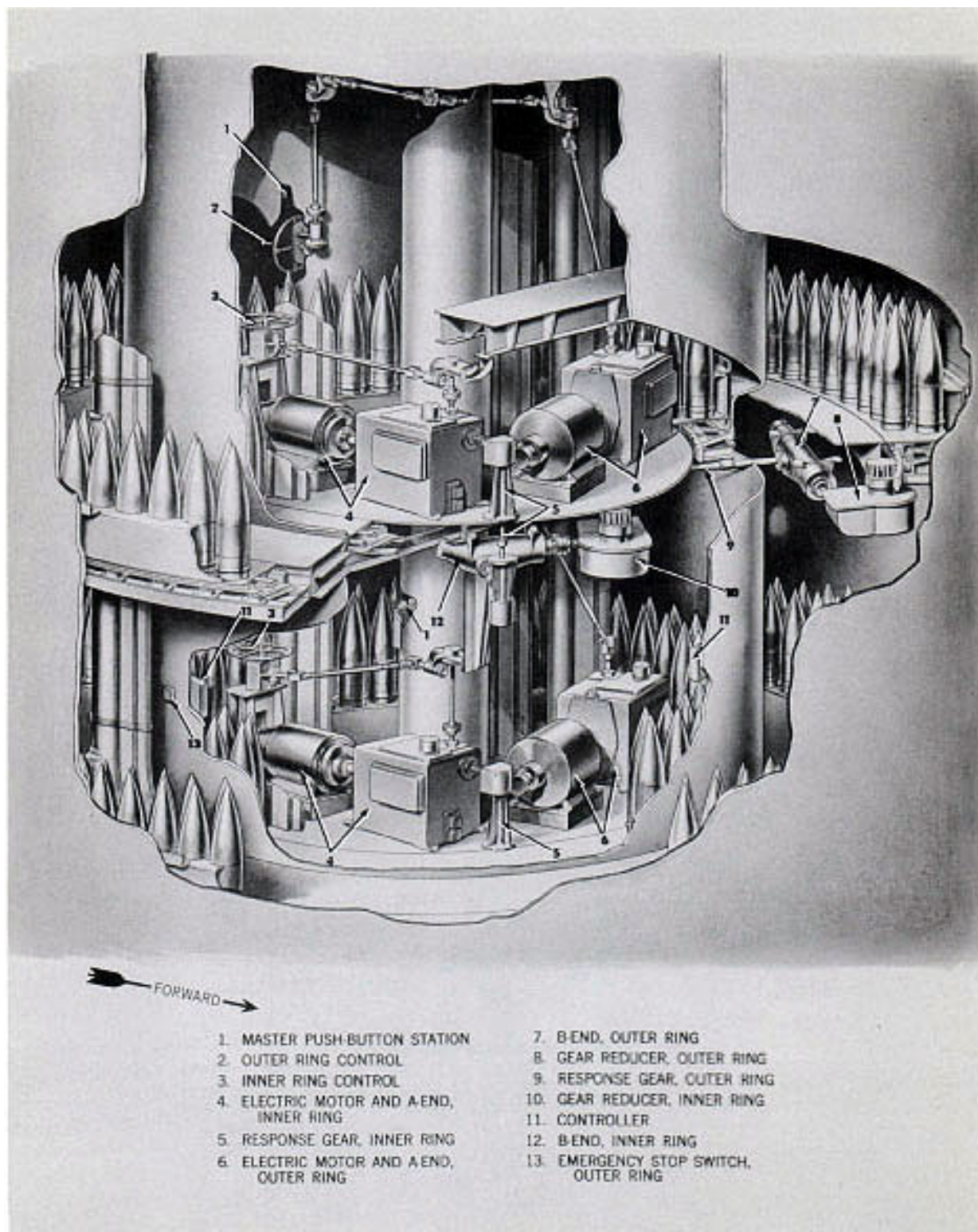
Figure 39. Projectile Ring. General Arrangement, Upper and Lower Projectile
