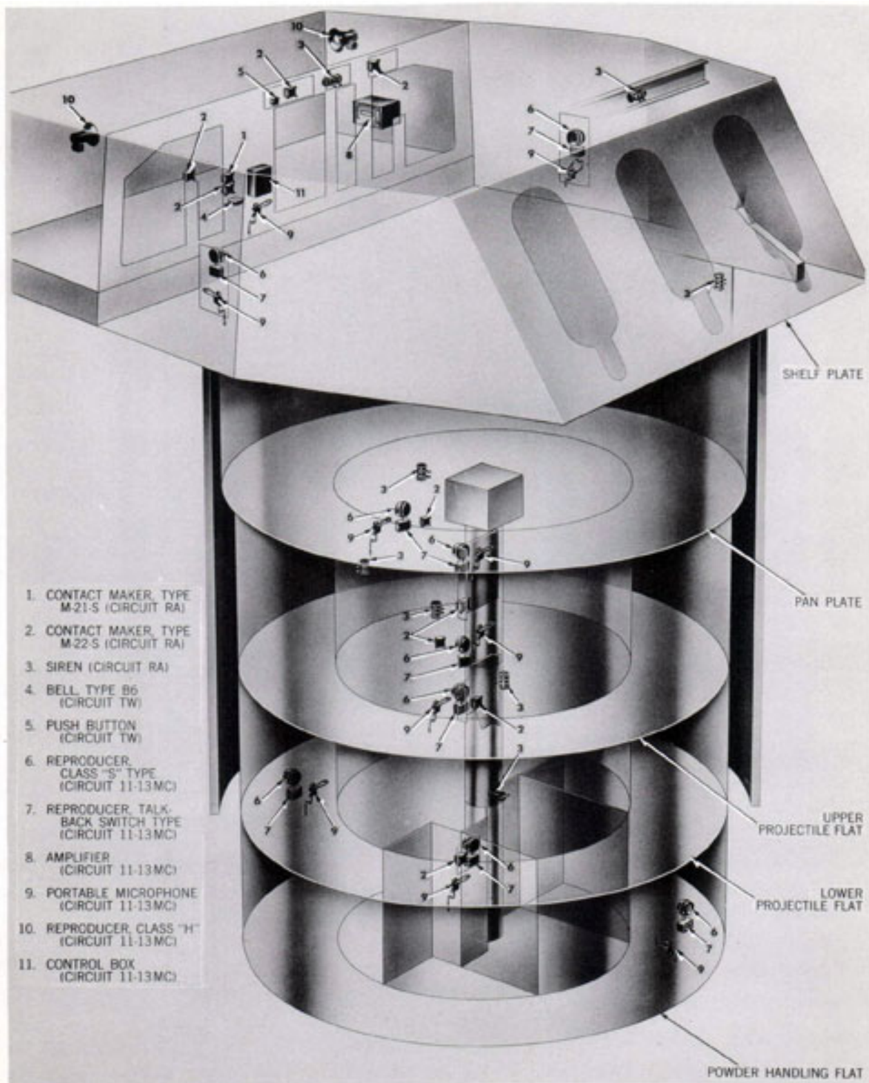
Figure 57. Turret Interior Communications System. General Arrangement
