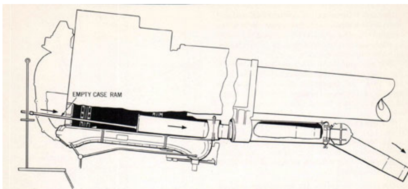
Figure 101. Use of Empty-Case Ram
