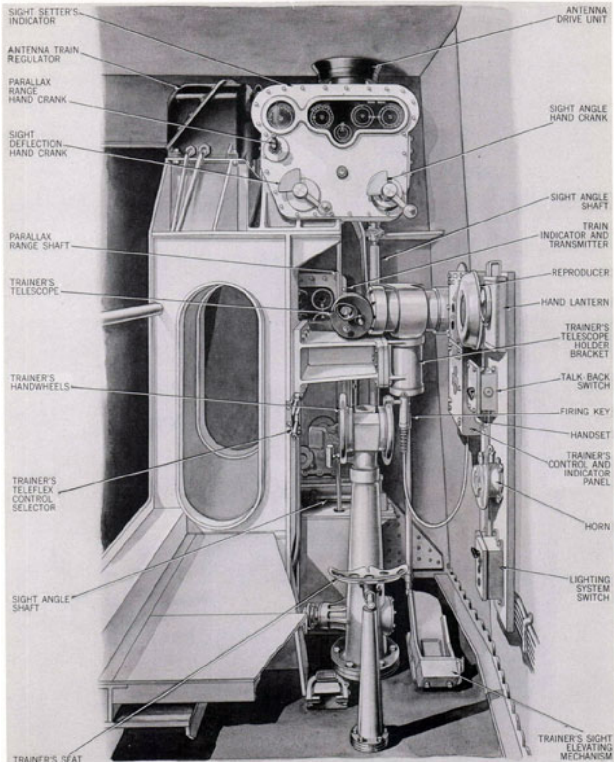
Figure 31. Trainer's and Sight Setter's Station General Arrangement
