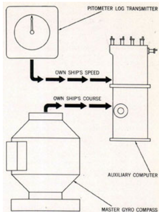
Figure 97. Auxiliary Computer Operation Automatic Inputs
