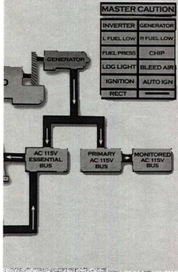
RAFT Electrical System
