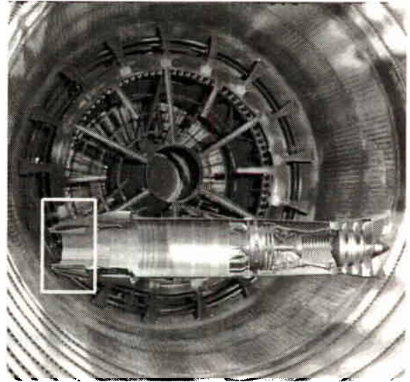
Figure 3.2-31 Variable Exhaust Nozzle
