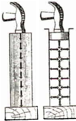
Figure 3.6-1 Force
