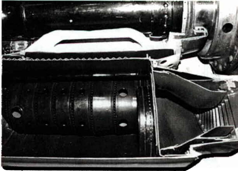
Figure 3.2-18 Can – Annular Type Combustion Chamber
