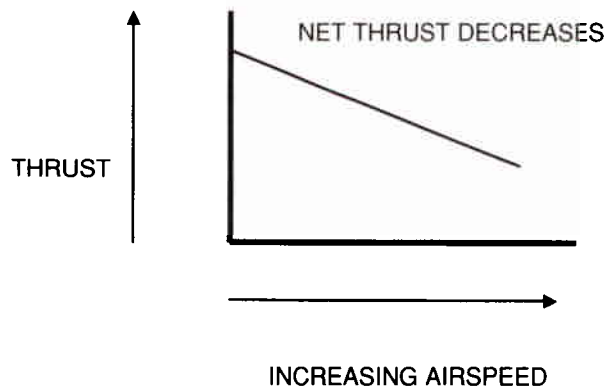
Figure 3.1-12 Airspeed Effect on Thrust
