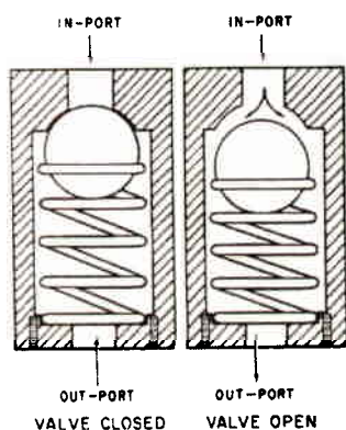
Figure 3.6-7 Check Valve
