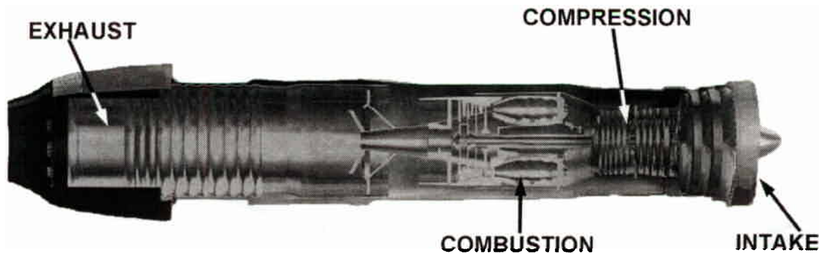
Figure 3.1-4 Brayton Cycle
