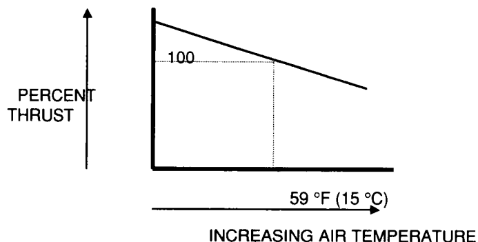
Figure 3.1-9 Temperature Effect on Thrust
