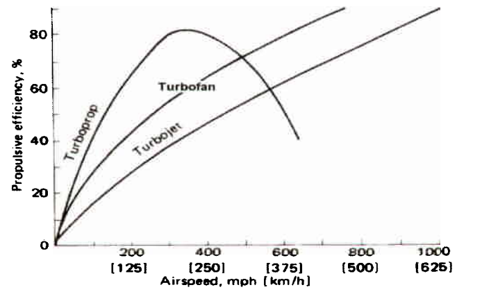
Figure 3.4-2 Engine Efficiency
