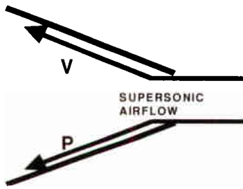
Figure 3.1-1a Supersonic Nozzle
