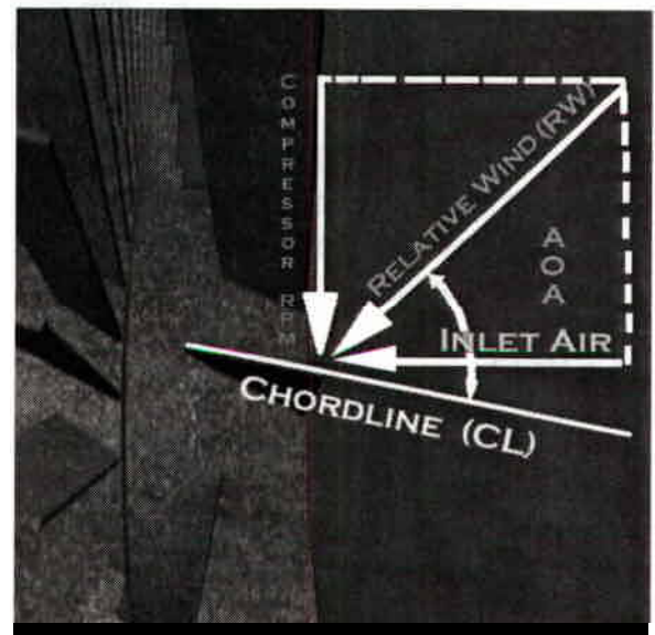
Figure 3.3-1 Angle of Attack
