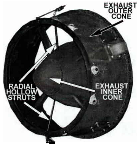
Figure 3.2-23 Exhaust Section
