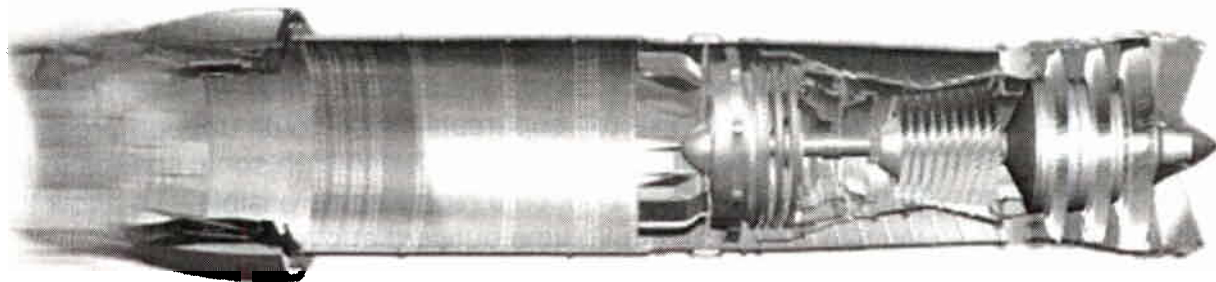
Figure 3.2-26 Gas Generator with Afterburner Unit
