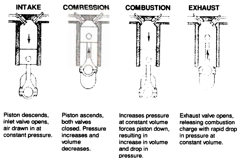
Figure 3.1-5 Otto Cycle
