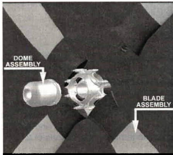
Figure 3.5-3 Propeller Assembly
