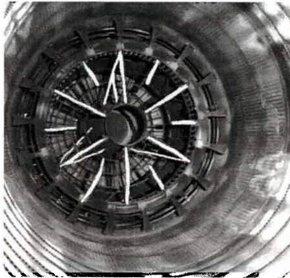
Figure 3.2-29 Flame Holder
