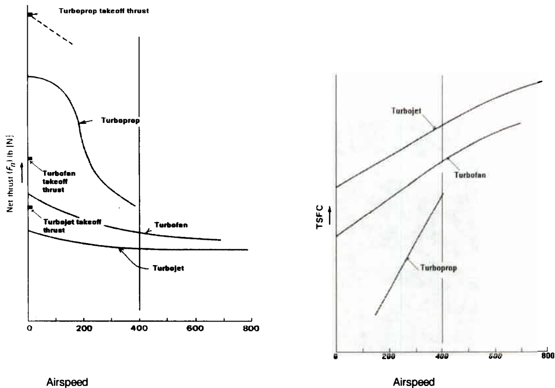
Figure 3.5-7 Thrust Comparison Graph
