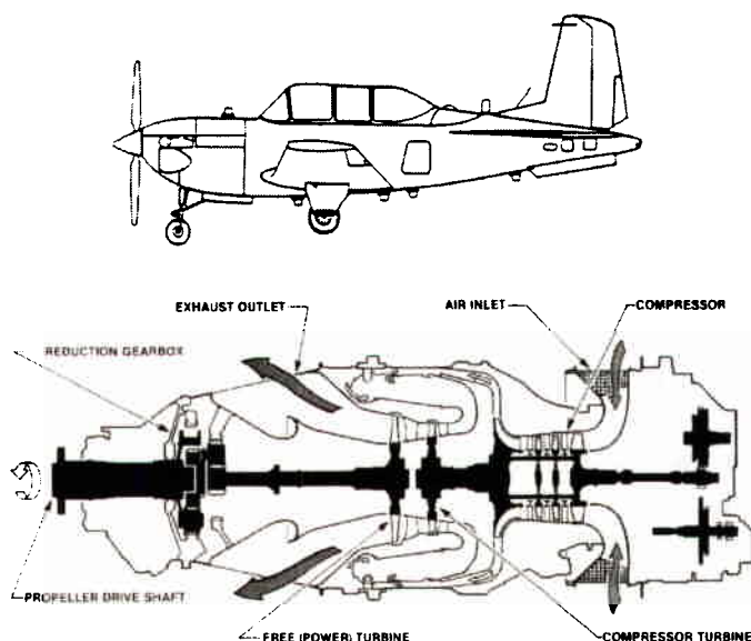
Figure 3.5-6 PT-6 Engine, T-34C
