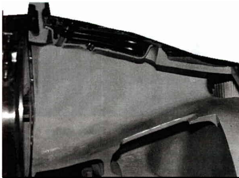
Figure 3.2-14 Diffuser
