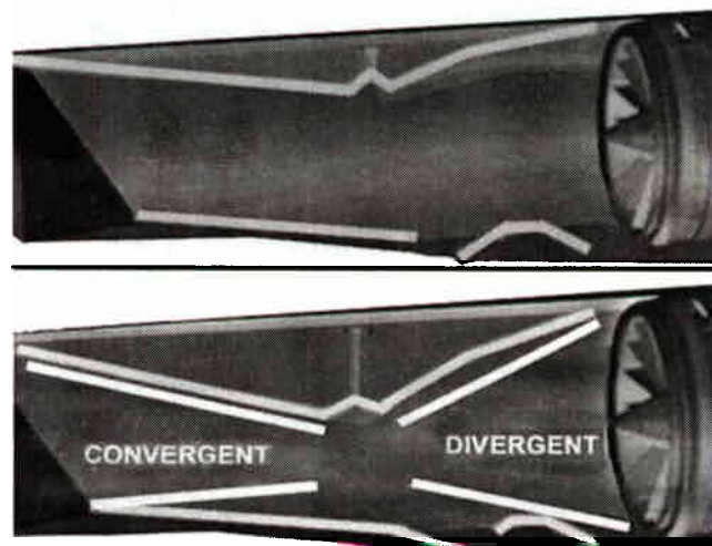
Figure 3.2-7 Variable Geometry Inlet Duct
