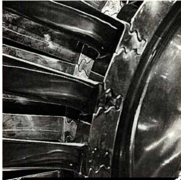
Figure 3.2-22 Fir Tree
