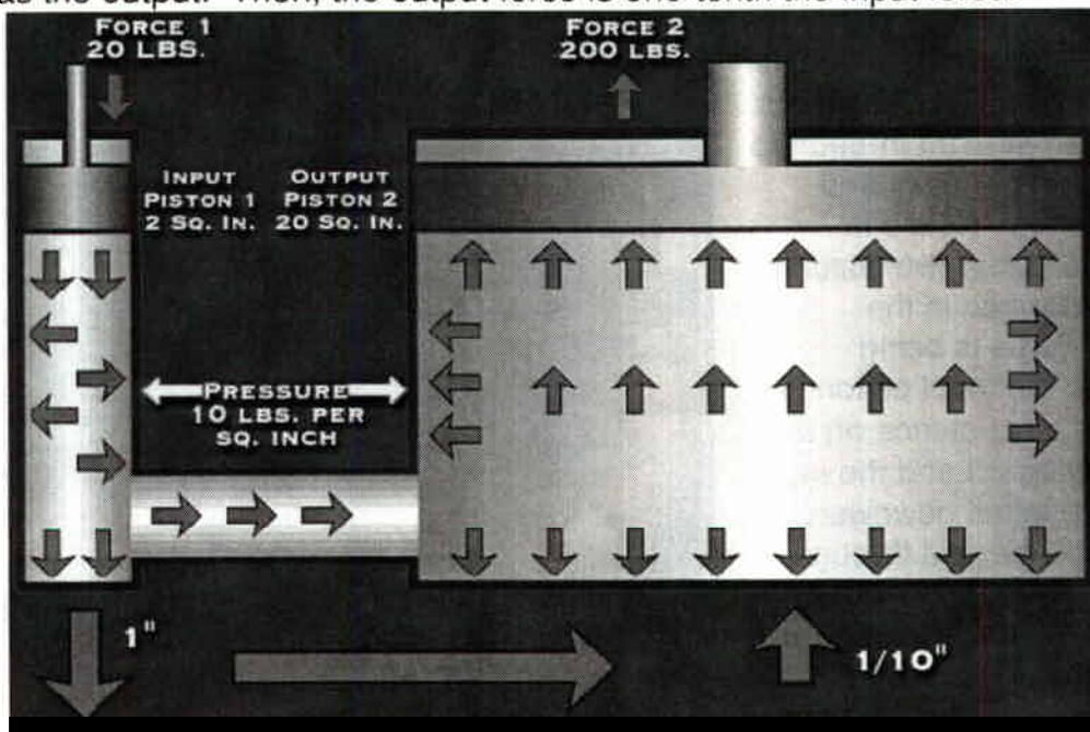
Figure 3.6-3 Hydraulic Example
