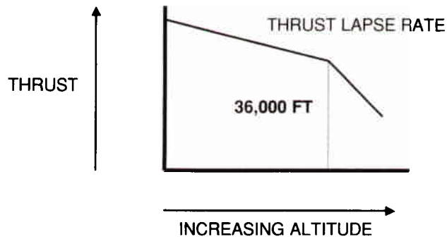
Figure 3.1-11 Altitude Effect on Thrust
