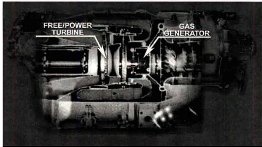
Figure 3.5-9 Turboshaft Engine
