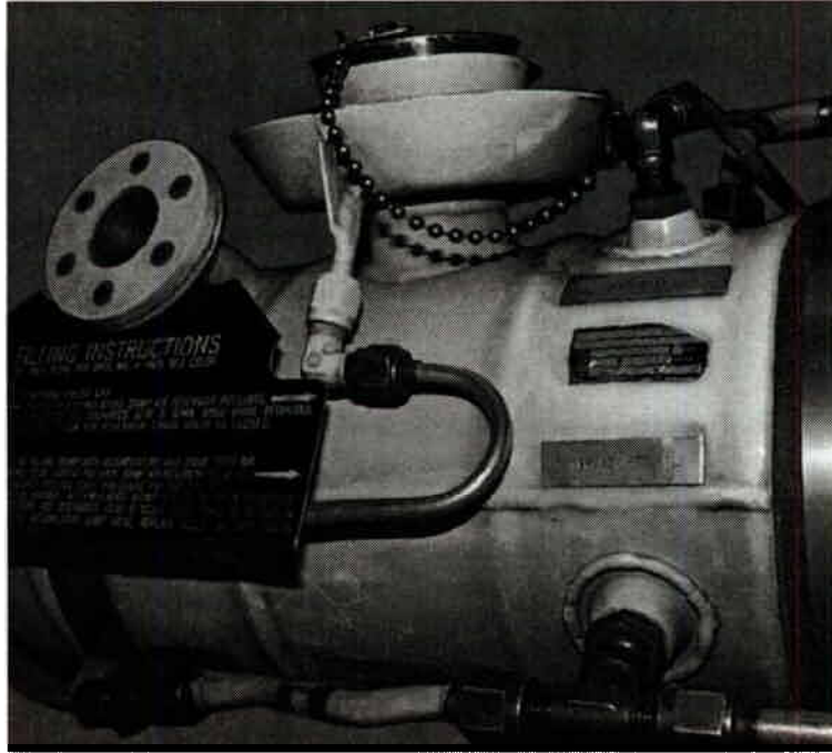
Figure 3.6-5 Pressurized Reservoir
