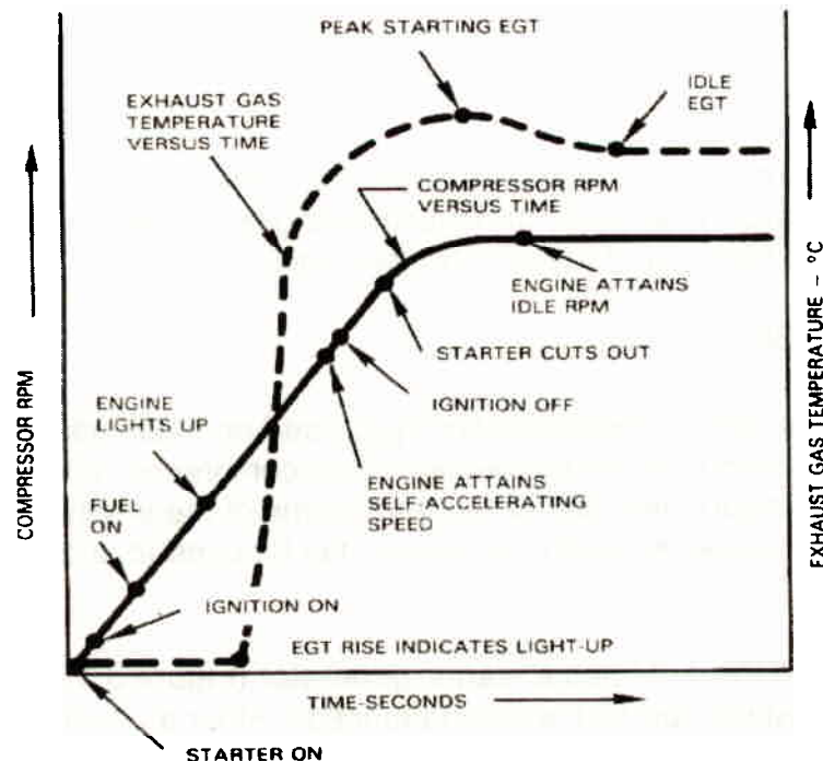
Figure 3.10-4 Starting Cycle
