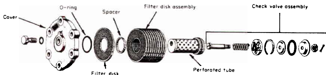
Figure 3.9-6 Oil Filter
