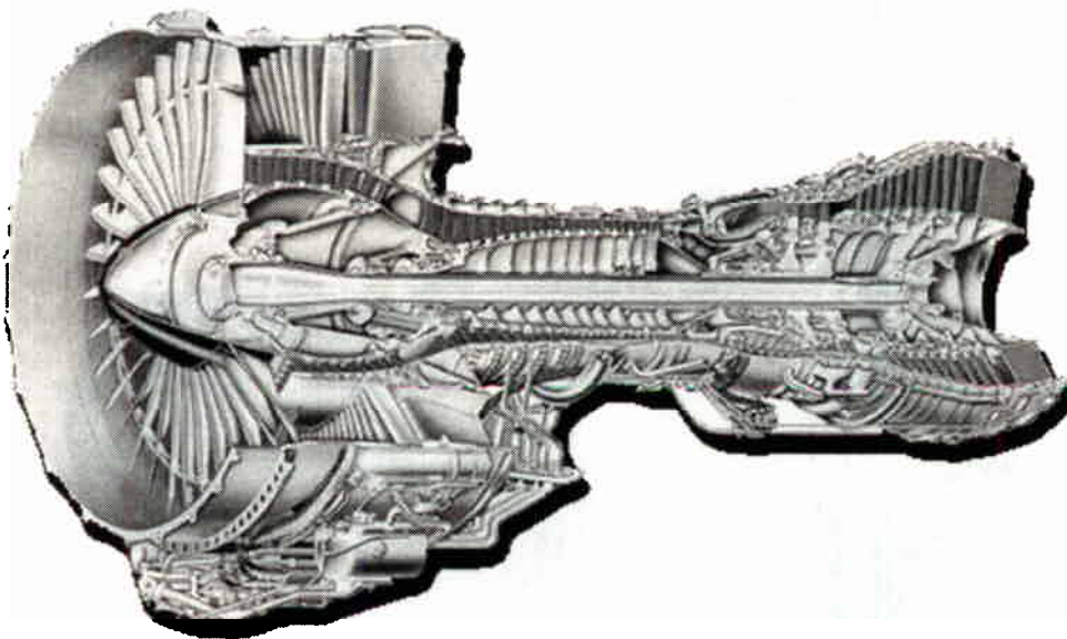
Figure 3.4-4 Free or Power Turbine
