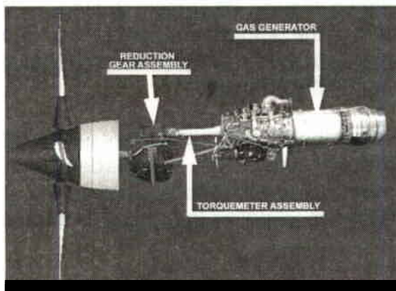
Figure 3.5-1 Turboprop Engine Assembly
