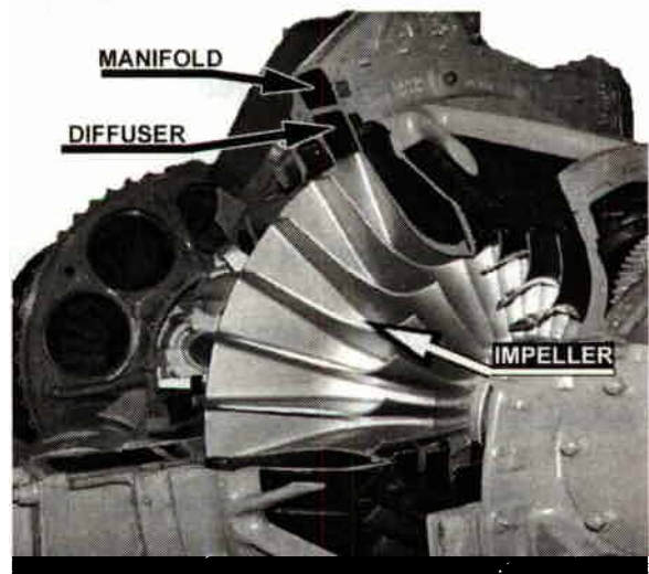
Figure 3.2-8 Centrifugal Compressor
