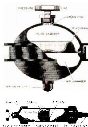
Figure 3.6-8 Accumulators
