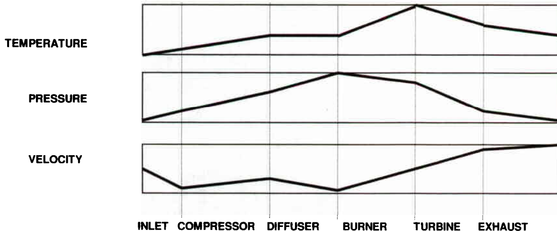
Figure 3.1-6 Temperature / Pressure / Velocity
