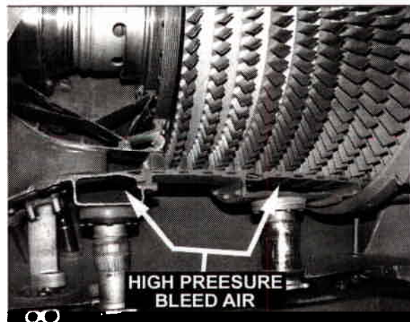
Figure 3.10-1 Bleed Air
