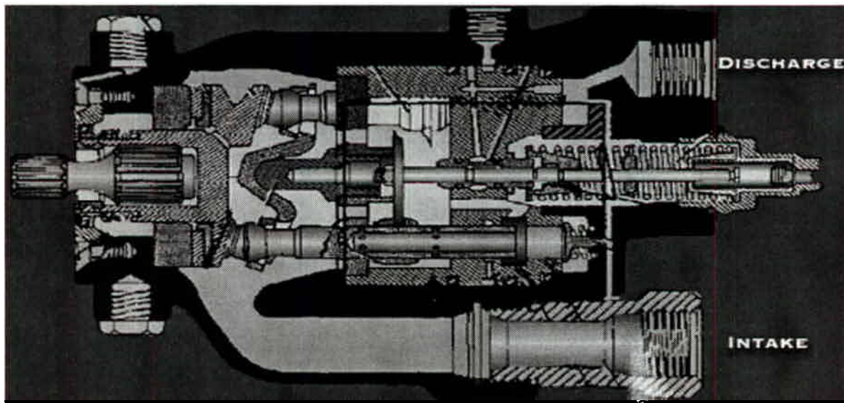
Figure 3.6-6 Pump
