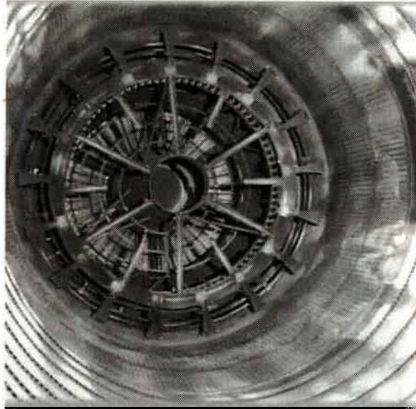
Figure 3.2-27 Afterburner Assembly
