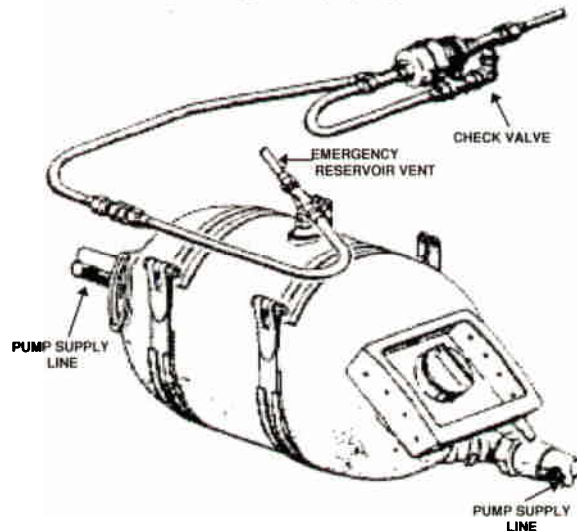
Figure 3.6-4 Nonpressurized Reservoir
