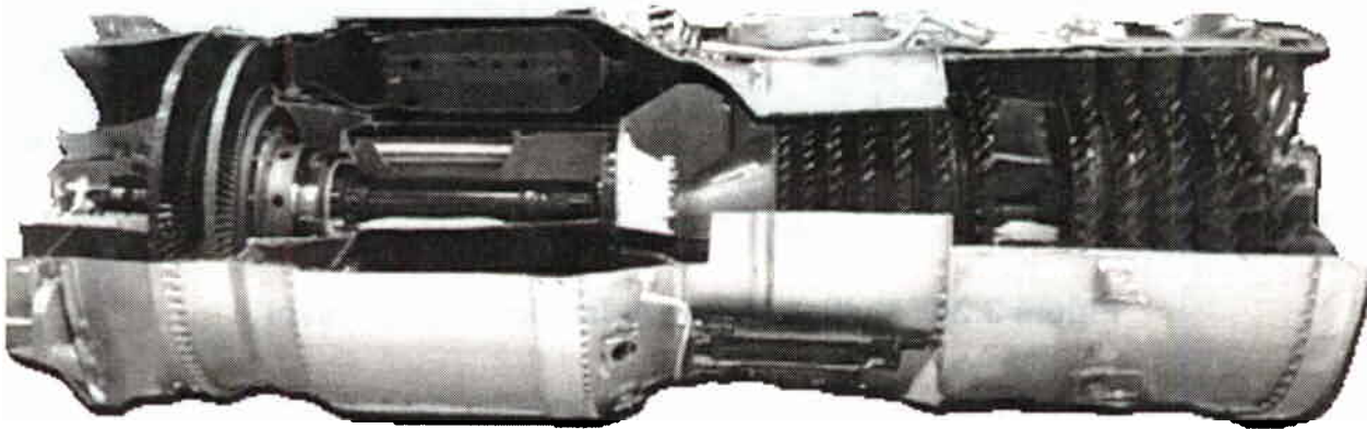
Figure 3.2-10 Dual Axial Flow Compressor
