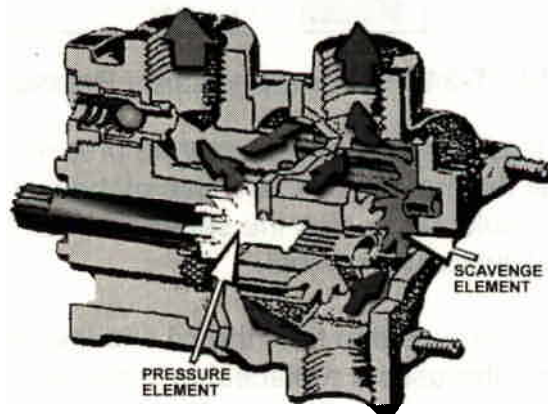
Figure 3.9-4 Gear Type Pump
