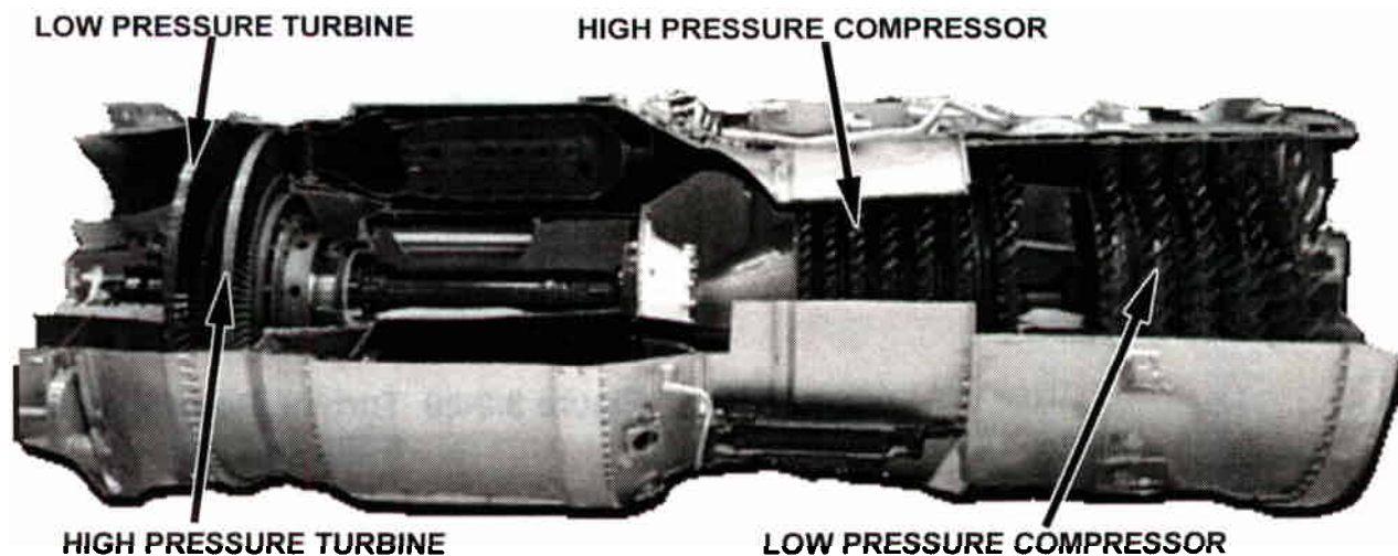
Figure 3.2-21 Dual Turbine
