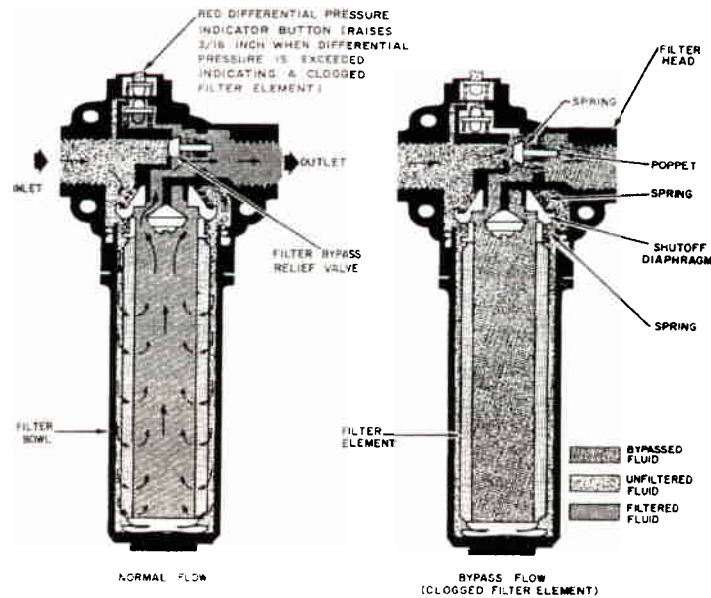
Figure 3.6-9 Hydraulic Filter
