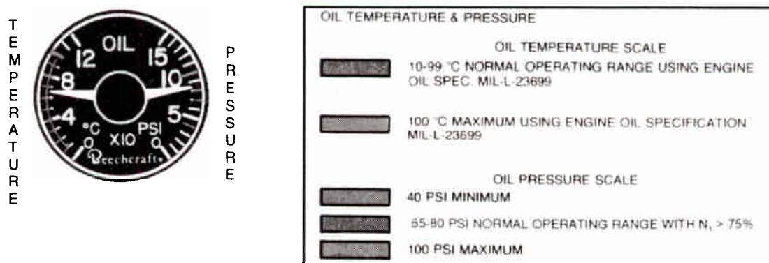
Figure 3.9-5 T-34C Oil Temperature / Pressure Gauge
