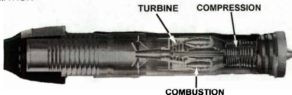
Figure 3.2-1 Gas Generator
