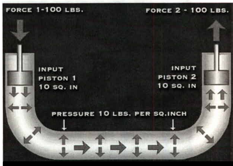
Figure 3.6-2 Pascal's Law
