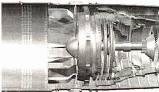
Figure 3.2-19 Turbine Section
