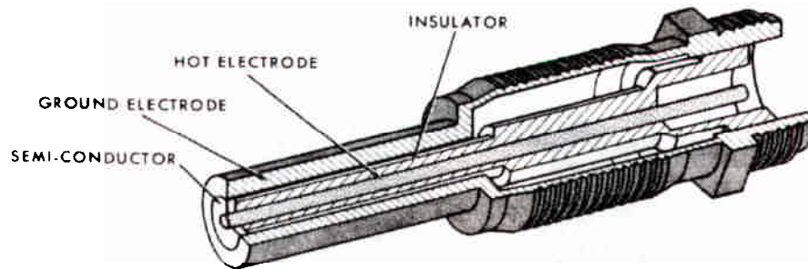
Figure 3.10-8 Typical Ignitor Plug
