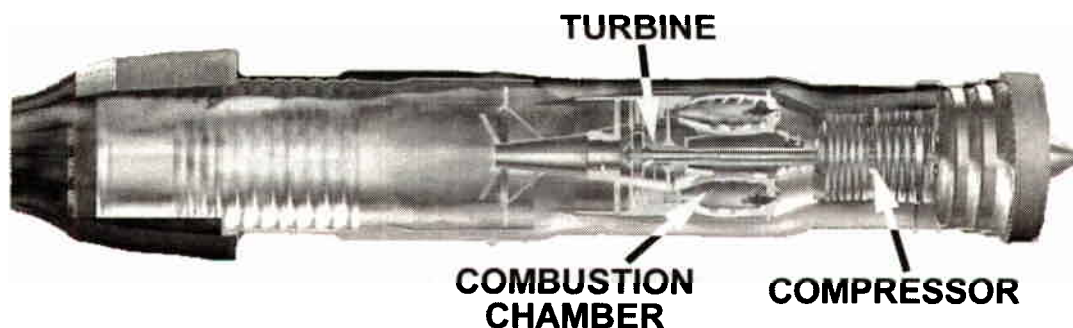
Figure 3.1-3 Gas Generator
