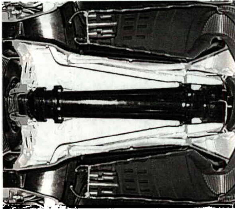
Figure 3.2-17 Annular Type Combustion Chamber
