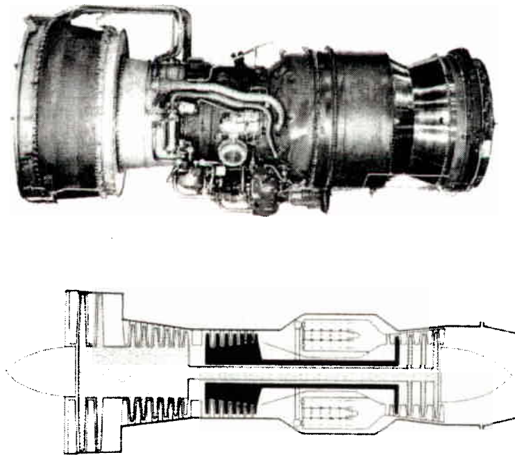
Figure 3.4-5 Turbofan
