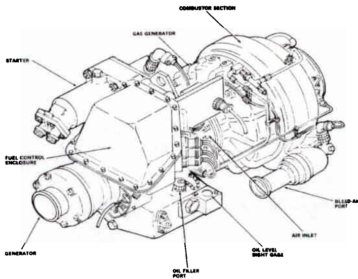
Figure 3.7-7 SH-60B Auxiliary Power Unit
