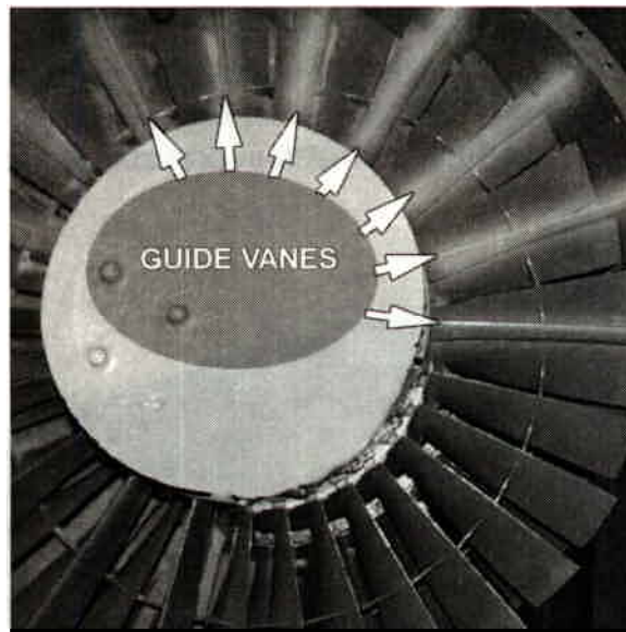
Figure 3.2-12 Inlet Guide Vanes
