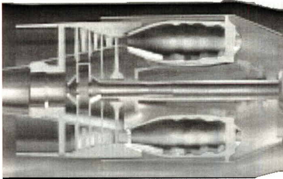
Figure 3.2-15 Burner Section
