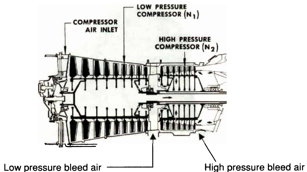
Figure 3.10-2 Low and High Pressure Bleed Air Locations
