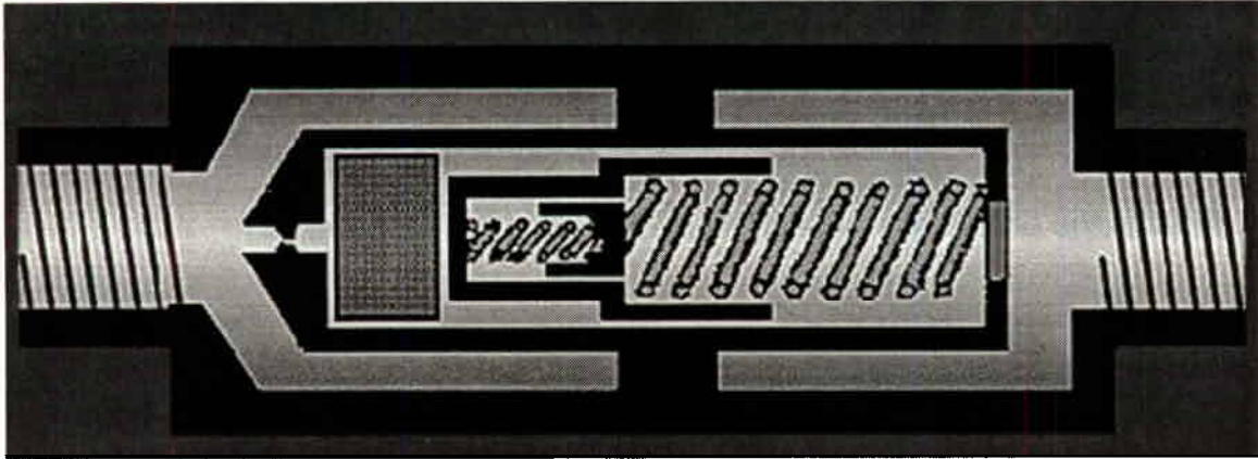
Figure 3.6-10 Hydraulic Fuse
