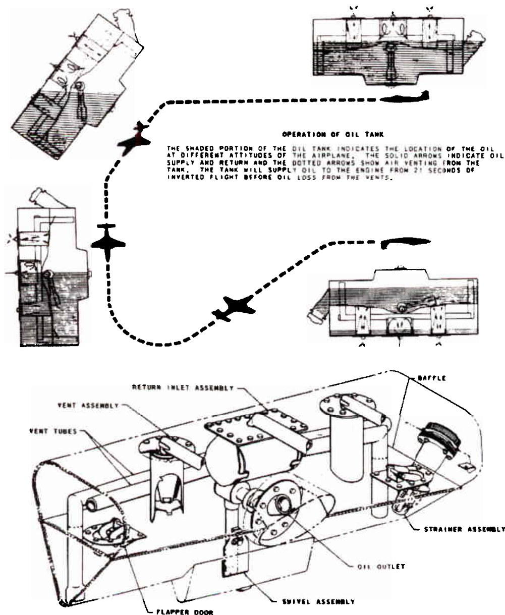
Figure 3.9-3 Swivel Assembly
