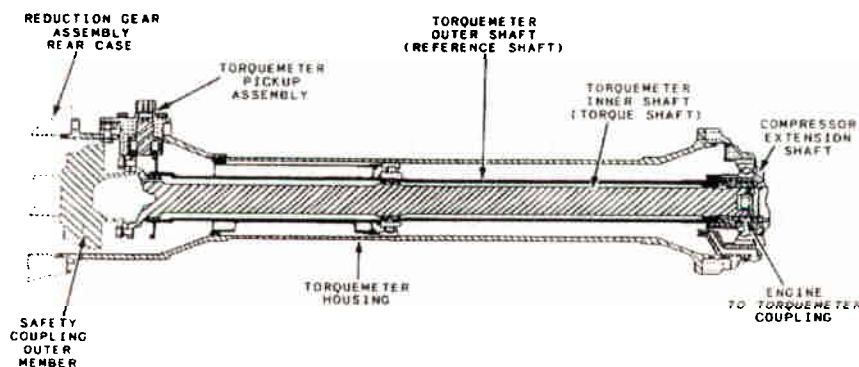
Figure 3.5-5 Torquemeter Assembly
