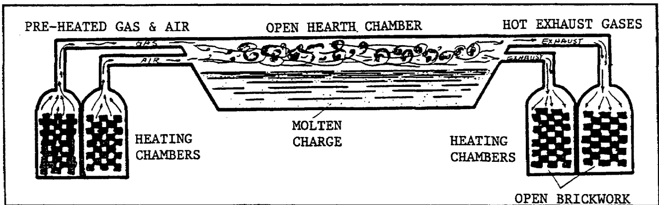
Figure 2-65. Open-Hearth Layout.
