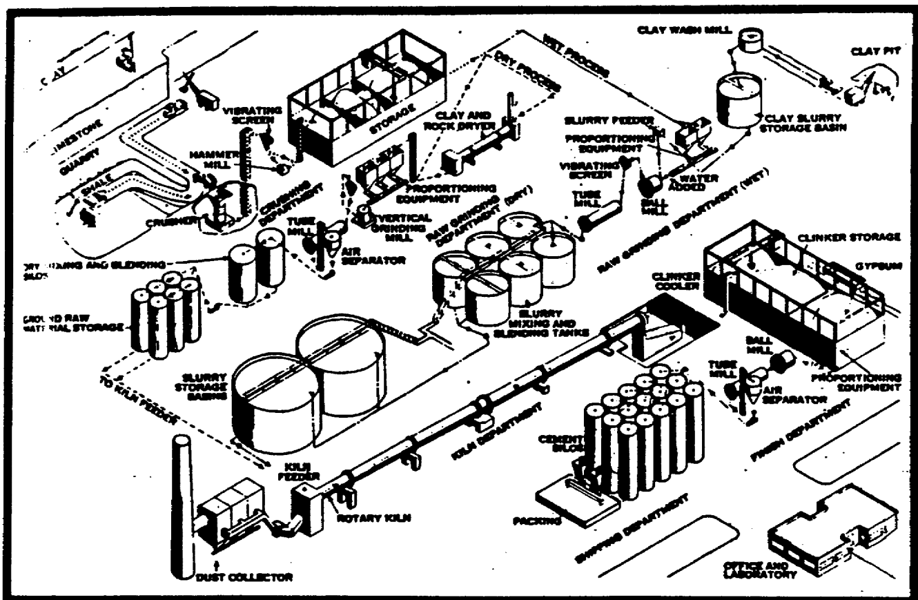
Figure 2-73. Wet Cement Production.
