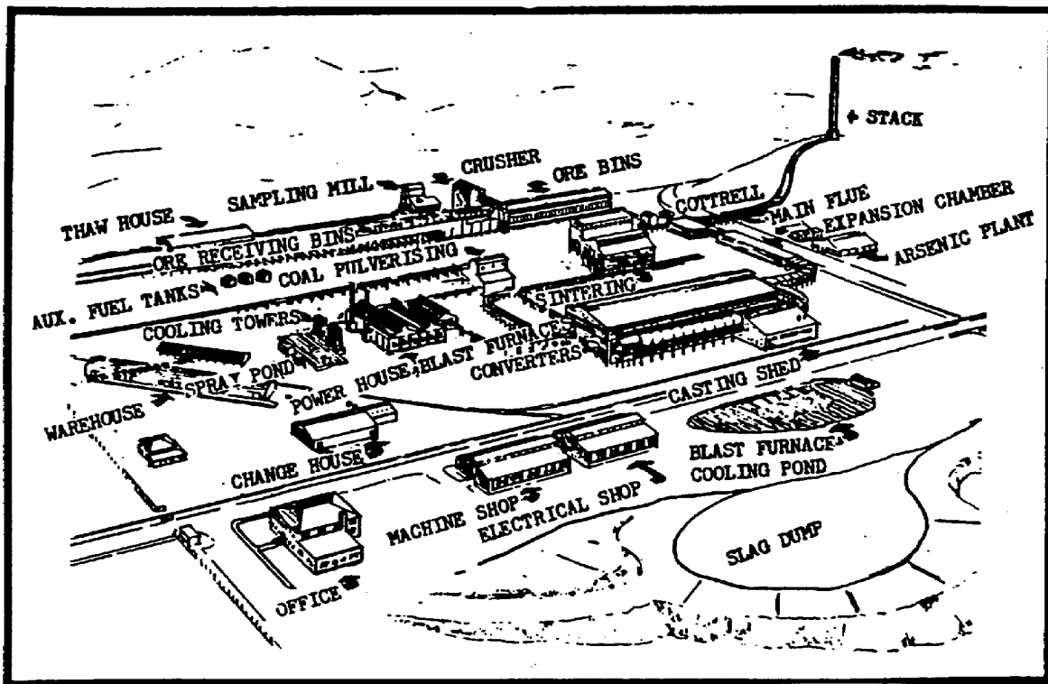
Figure 2-70. Copper Smelter.
