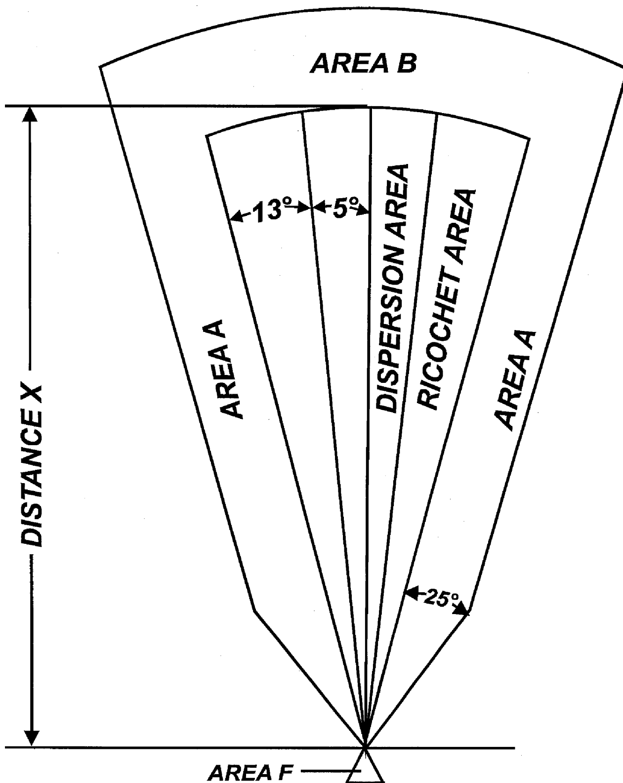
Figure 8-1. SDZ for firing rocket launchers
