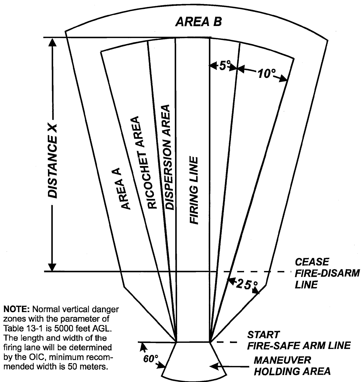
Figure 13-1. SDZ for firing aerial rocketry at ground targets
