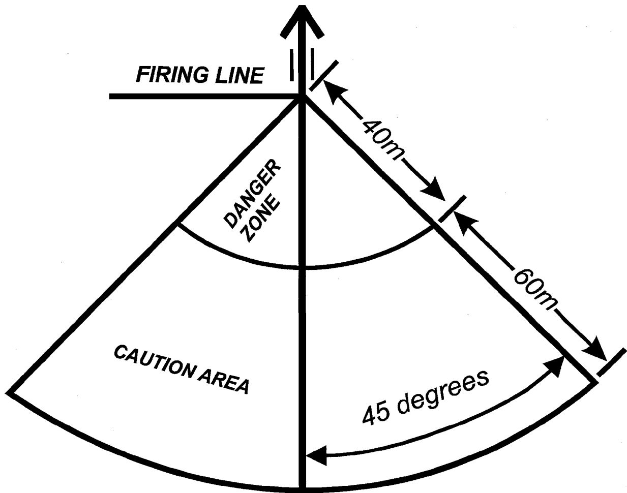
Figure 8-3. SDZ, area F for firing RAAWS
