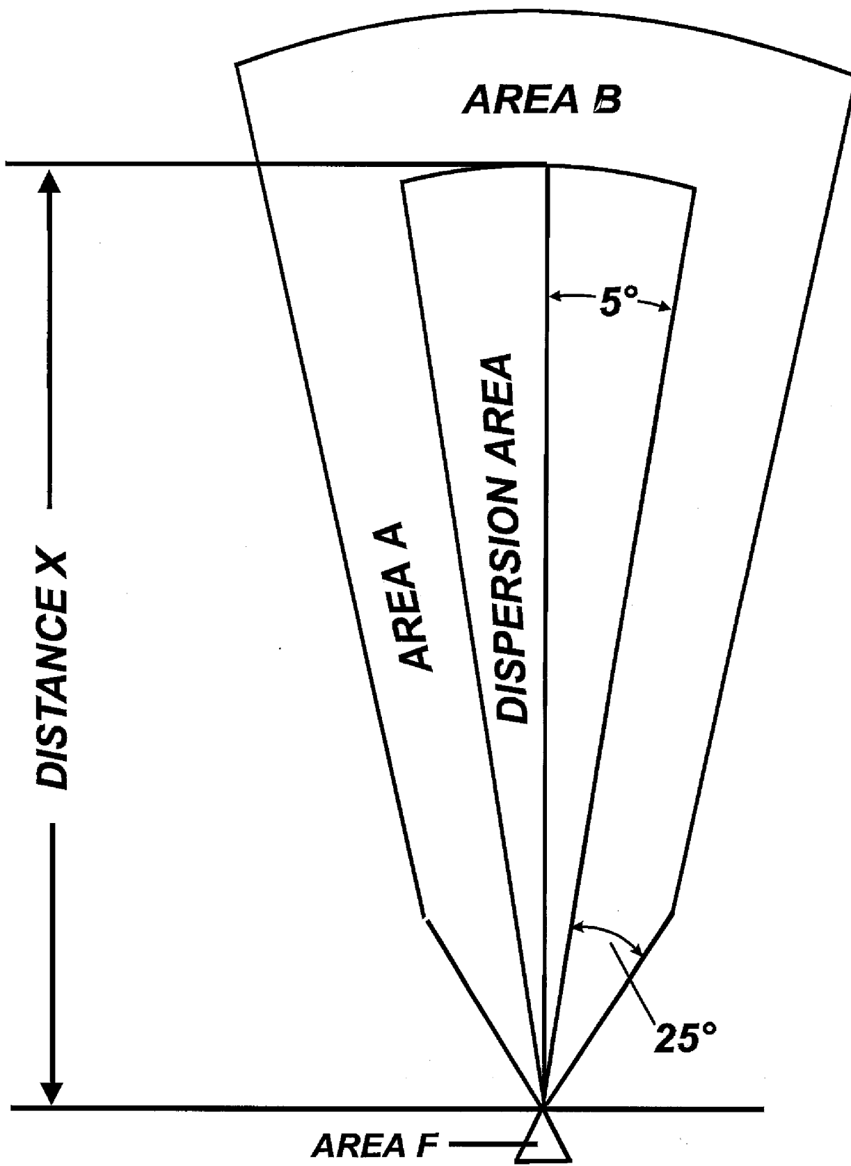
Figure 9-1. SDZ for firing recoilless rifles firing at quadrant elevation of 15° or more
