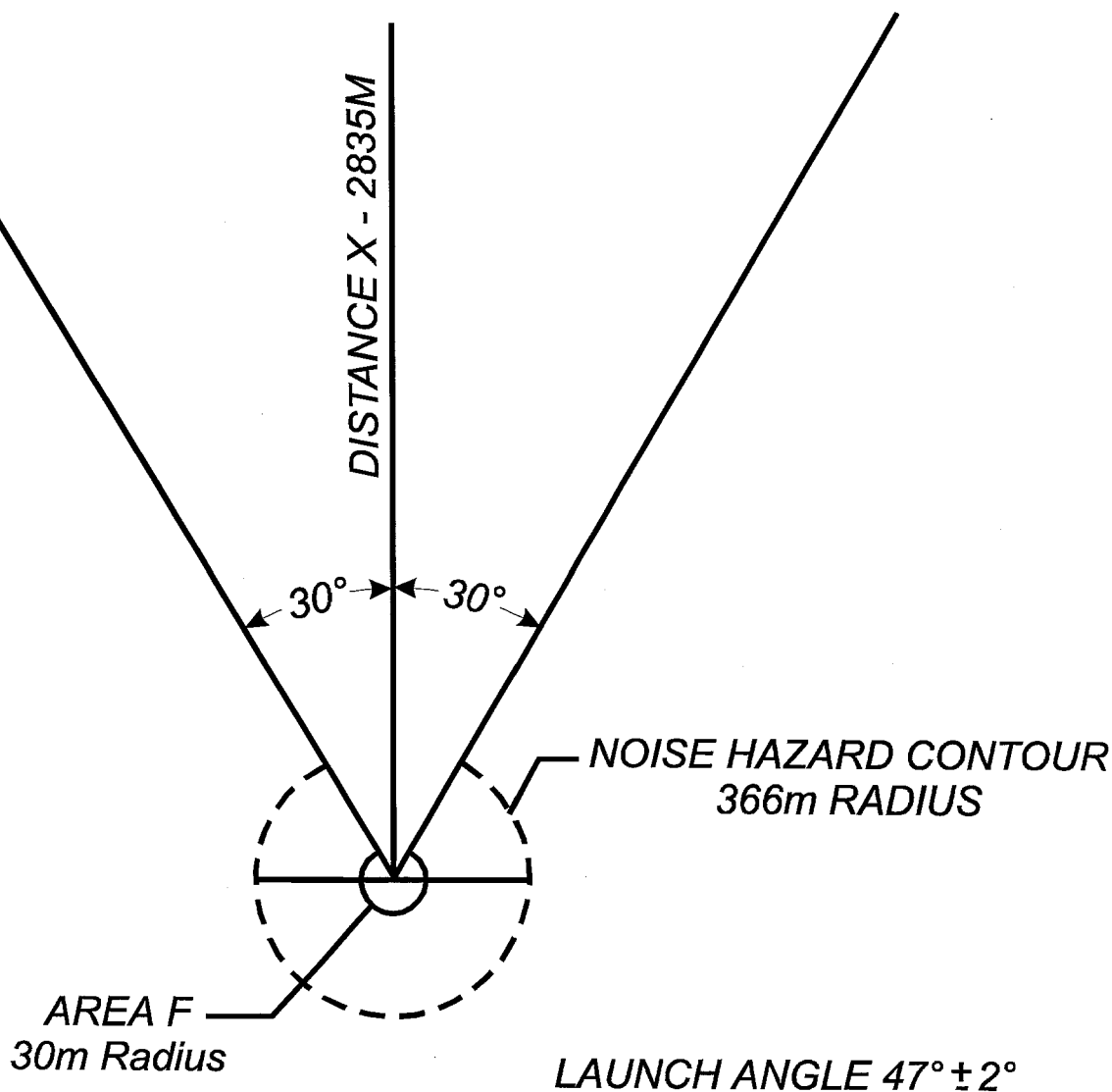
Figure 17-3. SDZ for firing mine-clearing line charge with the M68 inert charge
