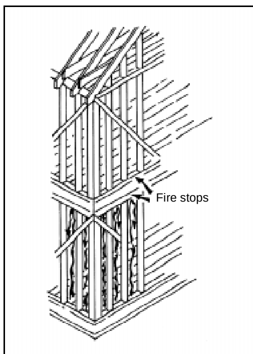
Figure 8-3. Fire stops
