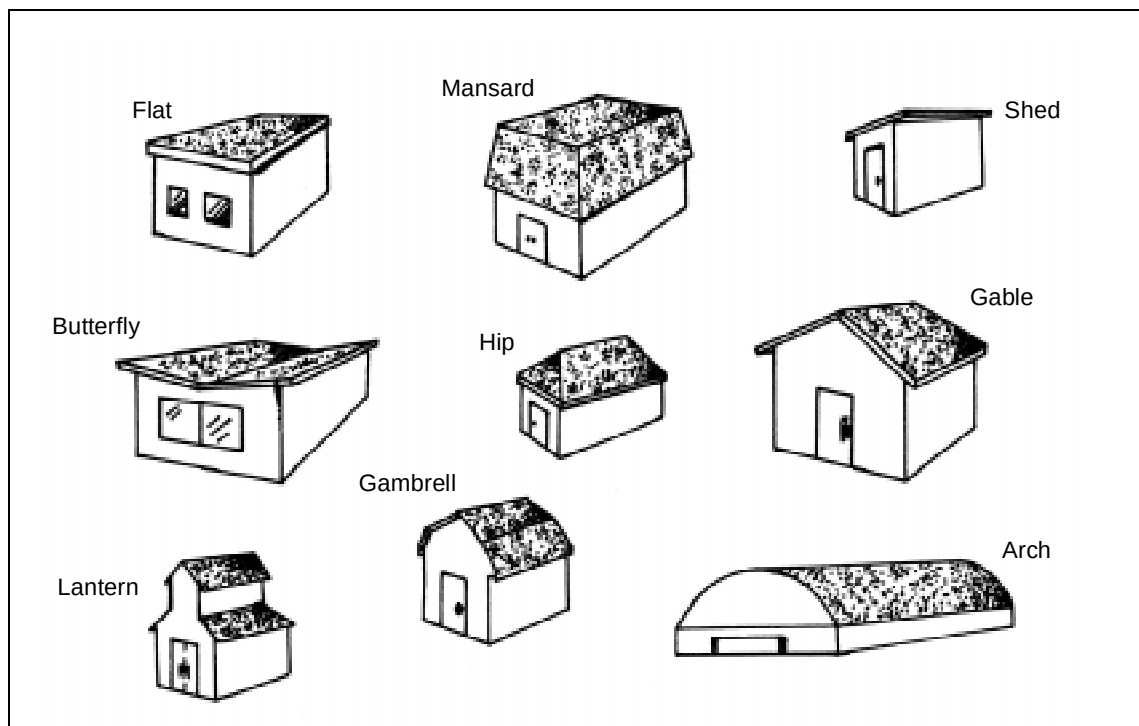
Figure 8-4. Roof types
