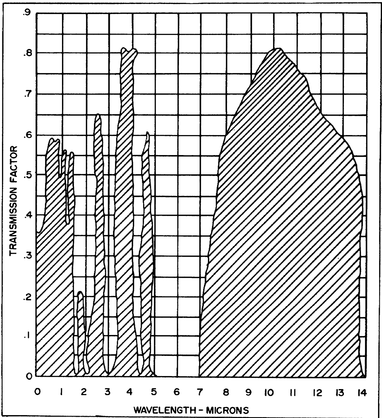
Figure 1-3. Atmospheric Windows.
