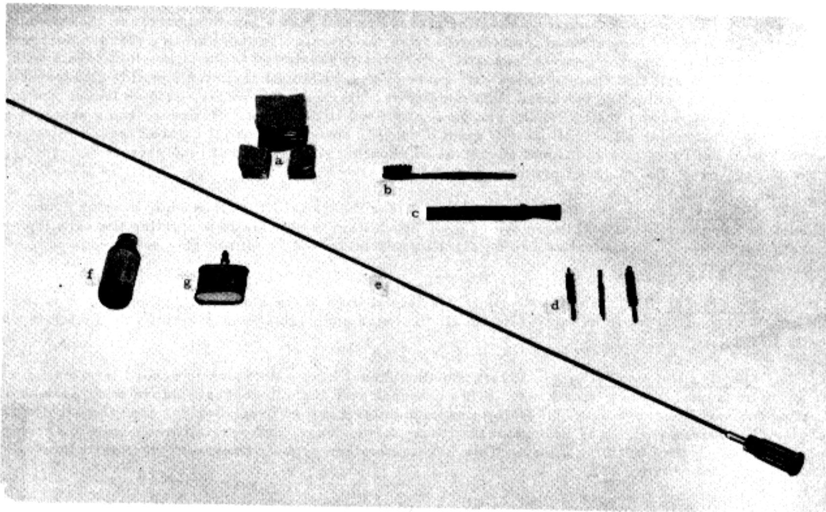
Figure 12. Cleaning equipment.
