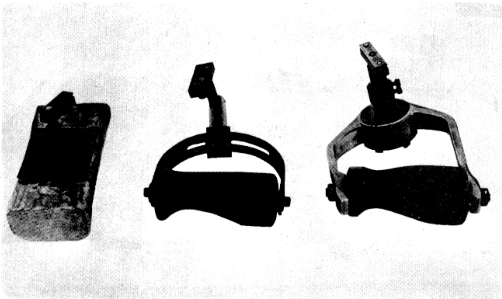
Figure 7. Palm rests.
