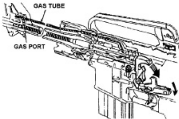
Figure 2-6. Firing.
