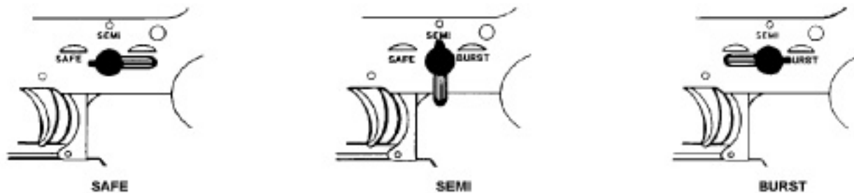
Figure 2-3. Selector Lever.
