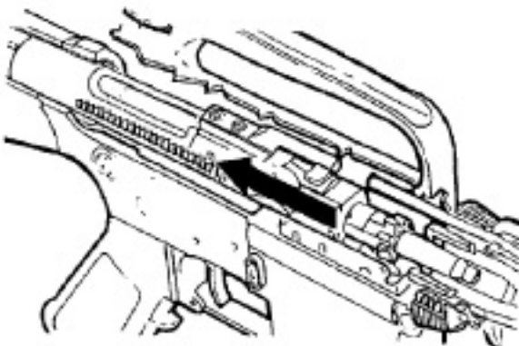
Figure 2-8. Extracting.
