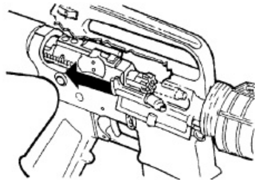
Figure 2-9. Ejecting.
