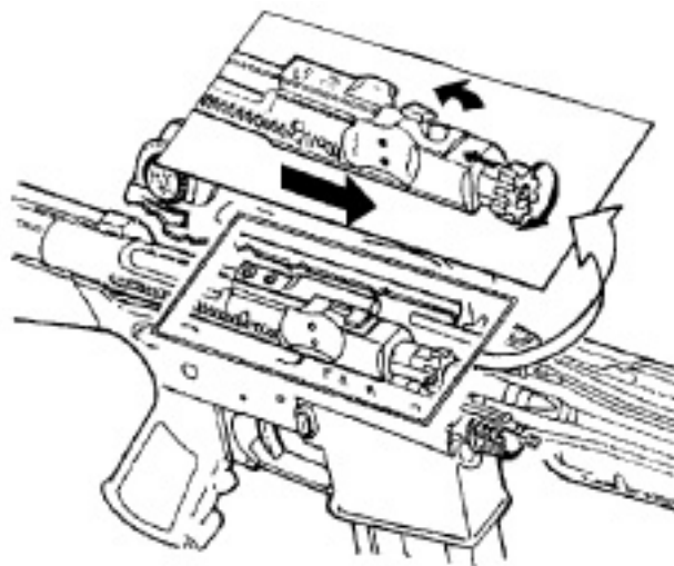
Figure 2-13. Locking.
