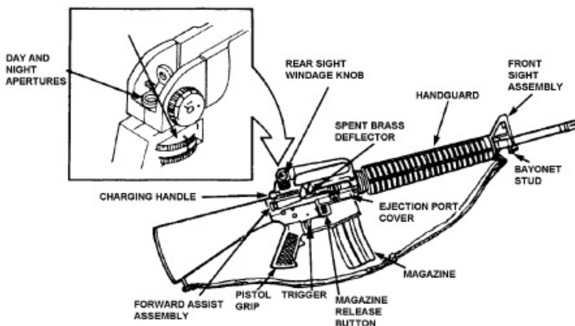
Figure 2-1. M16A2 Service Rifle (Right Side View).
