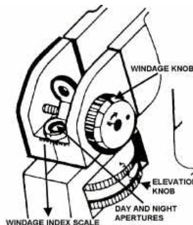
Figure 9-4. Rear Sight.
