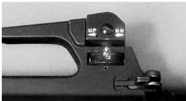
Figure 9-7. Rear Sight Elevation Knob Set for 800 Yards/Meters.
