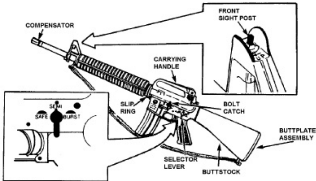
Figure 2-2. M16A2 Service Rifle (Left Side View).
