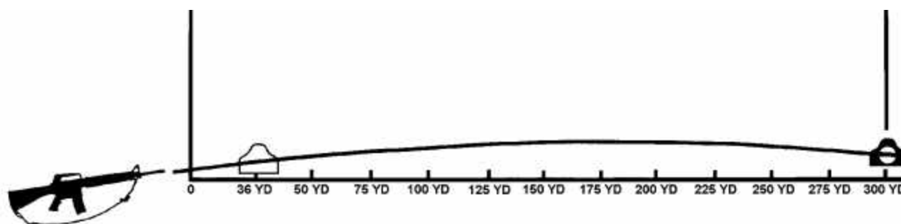
Figure 9-13. Bullet Crossing the Line of Sight Twice.
