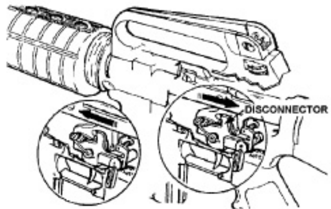
Figure 2-10. Cocking.
