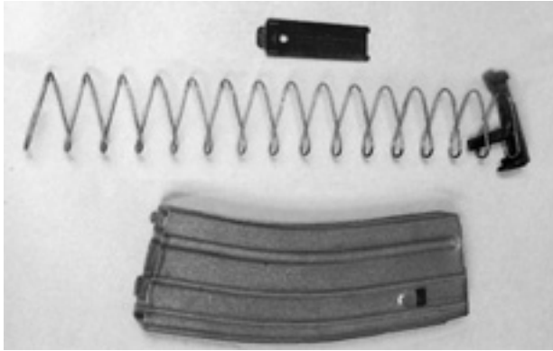
Figure 2-19. Magazine Disassembled.
