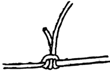
Figure A-18. Example of branch line connection, using a girth hitch with an extra
