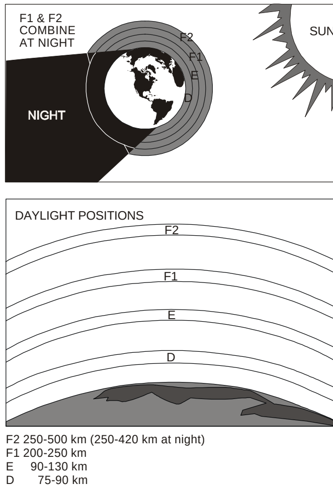
Figure 1-5. Ionospheric Structure.
