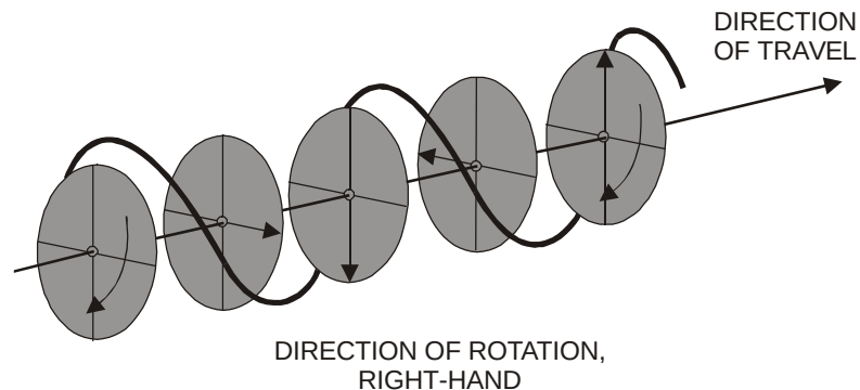
Figure 2-5. Circular Polarization.
