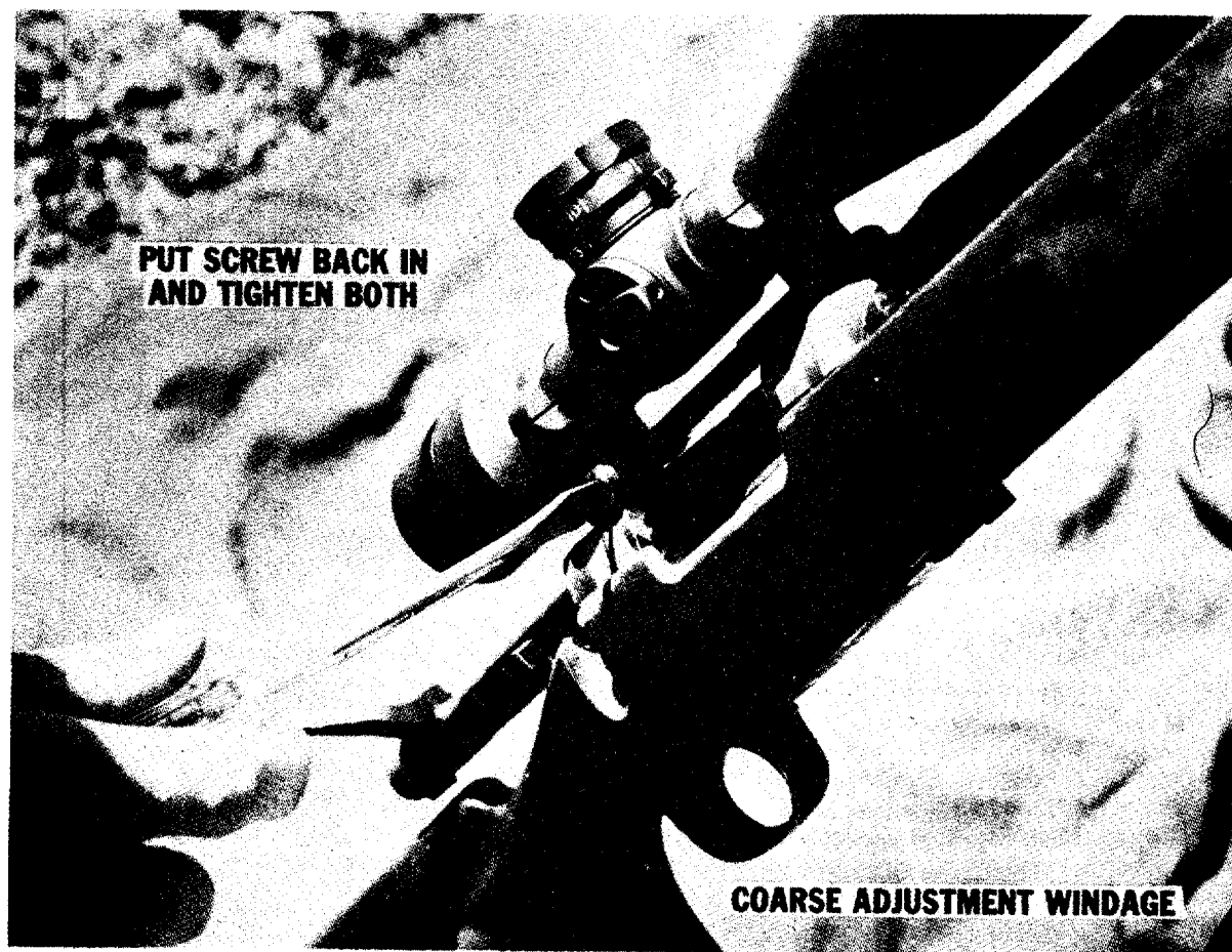
Figure 3-14. Course Adjustment with Scope Base for Zeroing.
