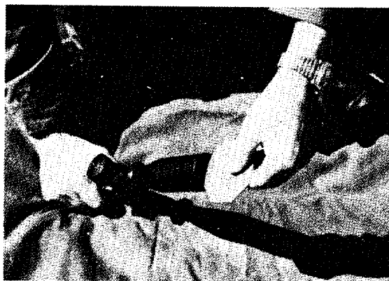
Figure 2-6. Adjusting Parallax With "Spanner."
