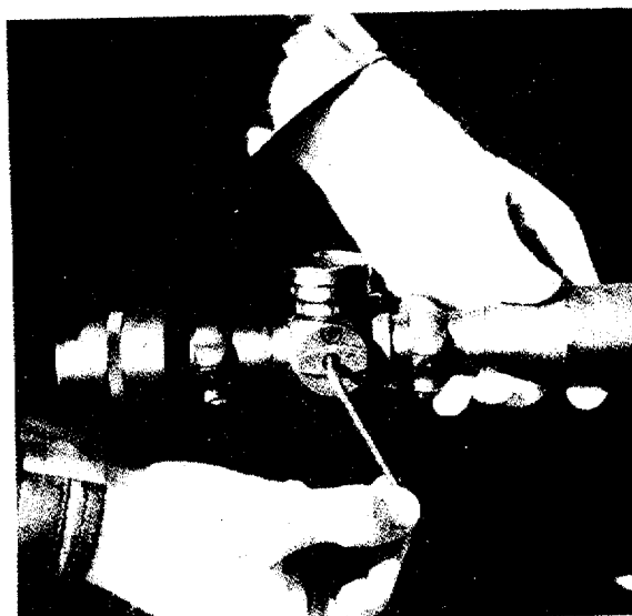
Figure 3-18. Zeroing with Allen Wrench Windage Control (View 2).
