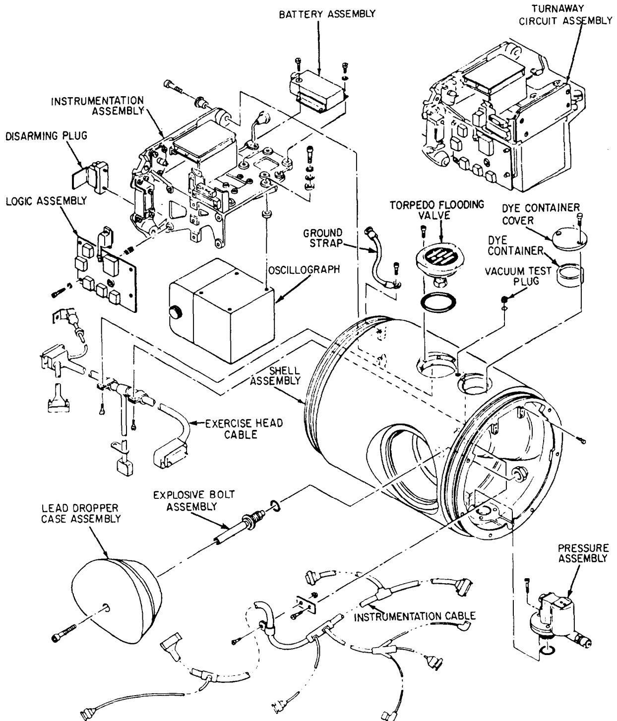
Figure 2-16.-Mk 85 Mod 4 exercise head.
