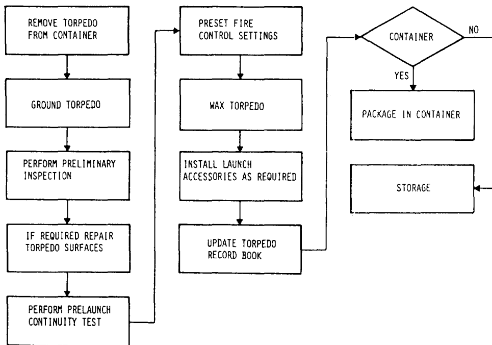
Figure 2-34.-Inspection flow diagram of fleet return torpedoes.
