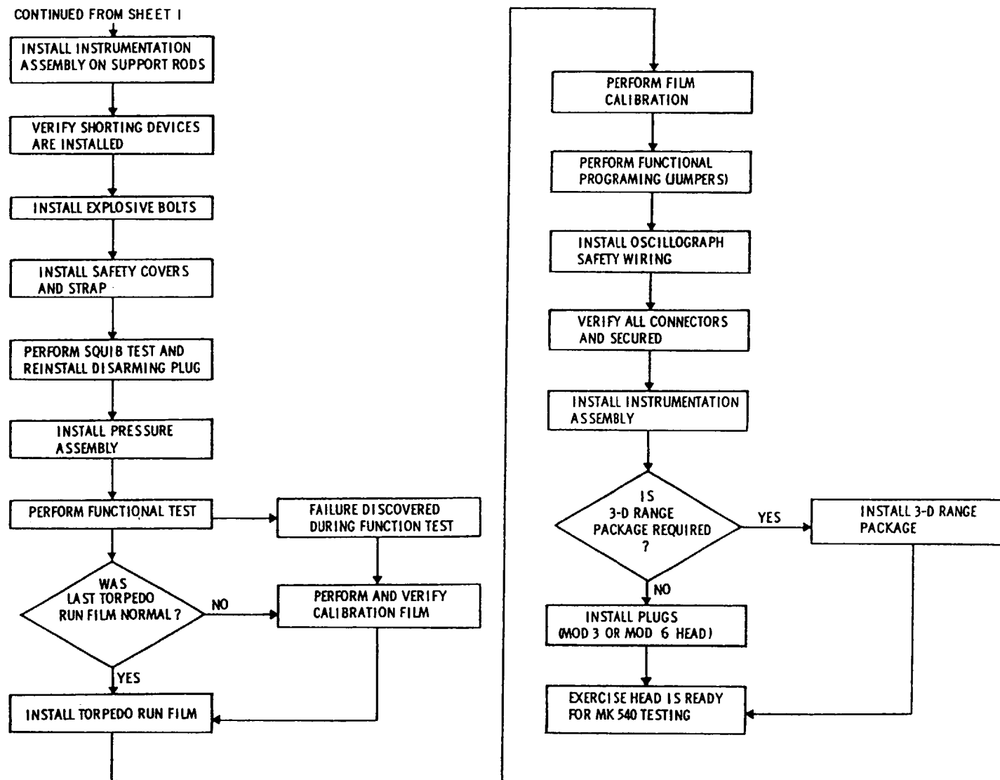
Figure 2-18.—Maintenance flow diagram for the exercise head—Continued.
