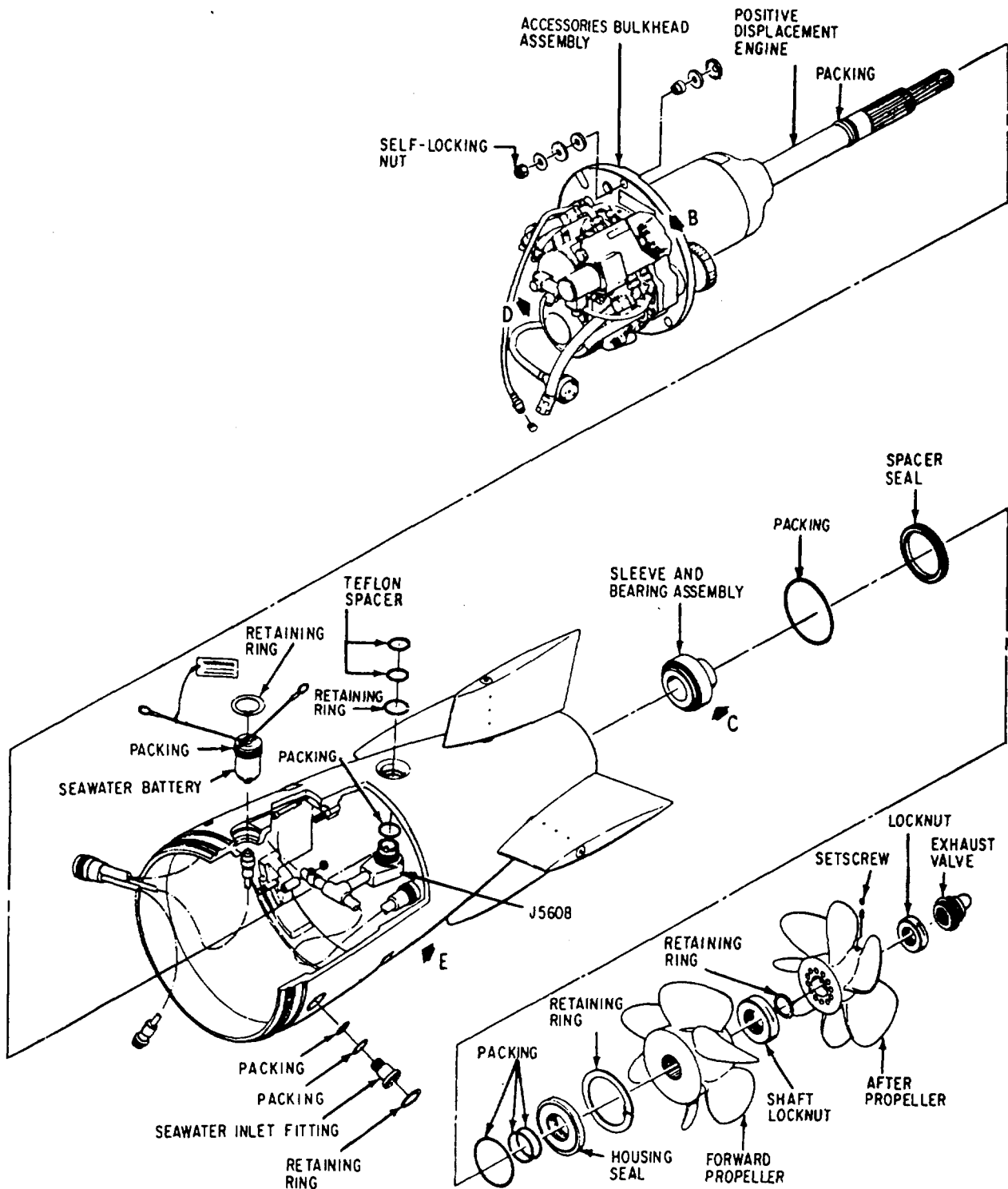
Figure 2-28.-Afterbody components.
