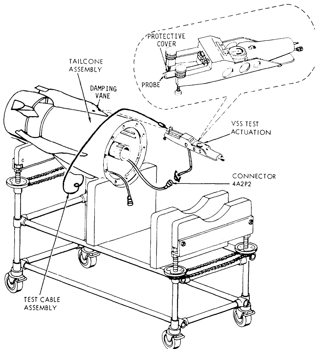
Figure 3-19-Velocity sensor switch test.
