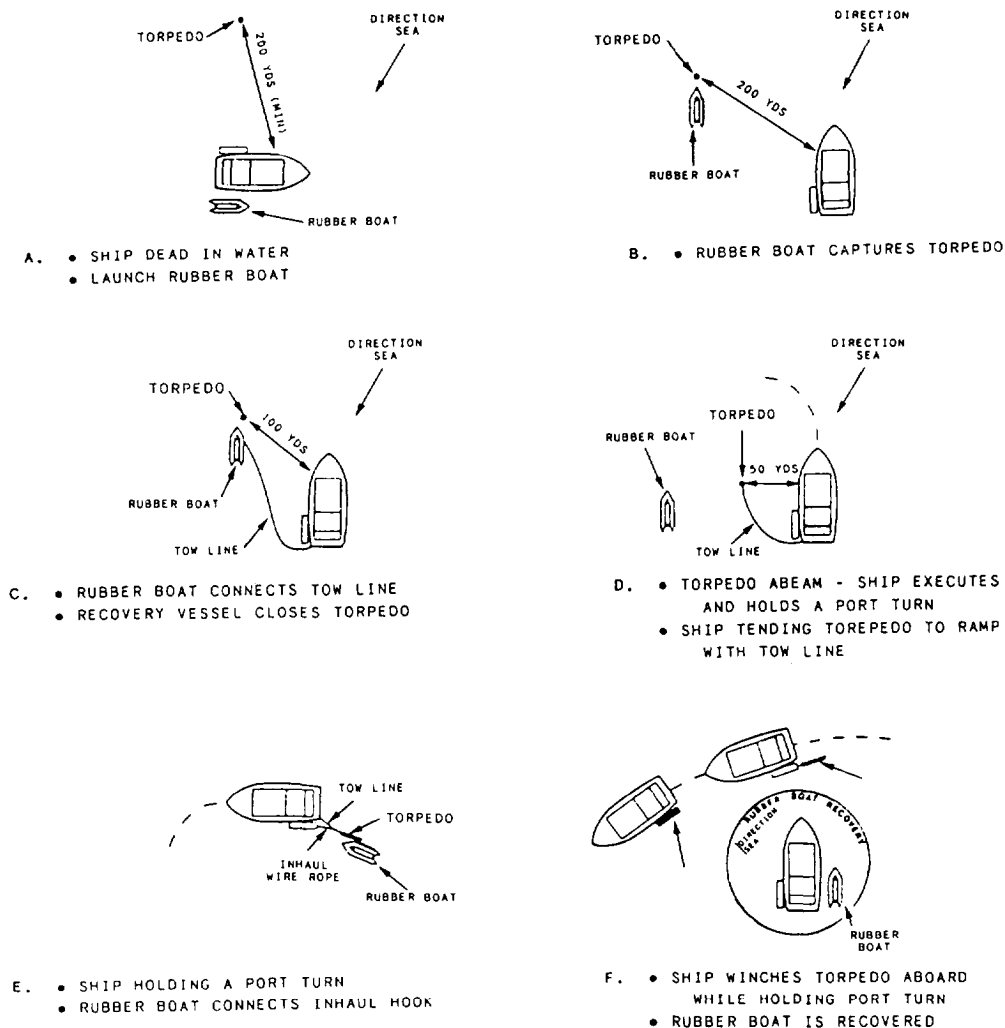
Figure 1-43.-Portable ramp recovery (diagram).
