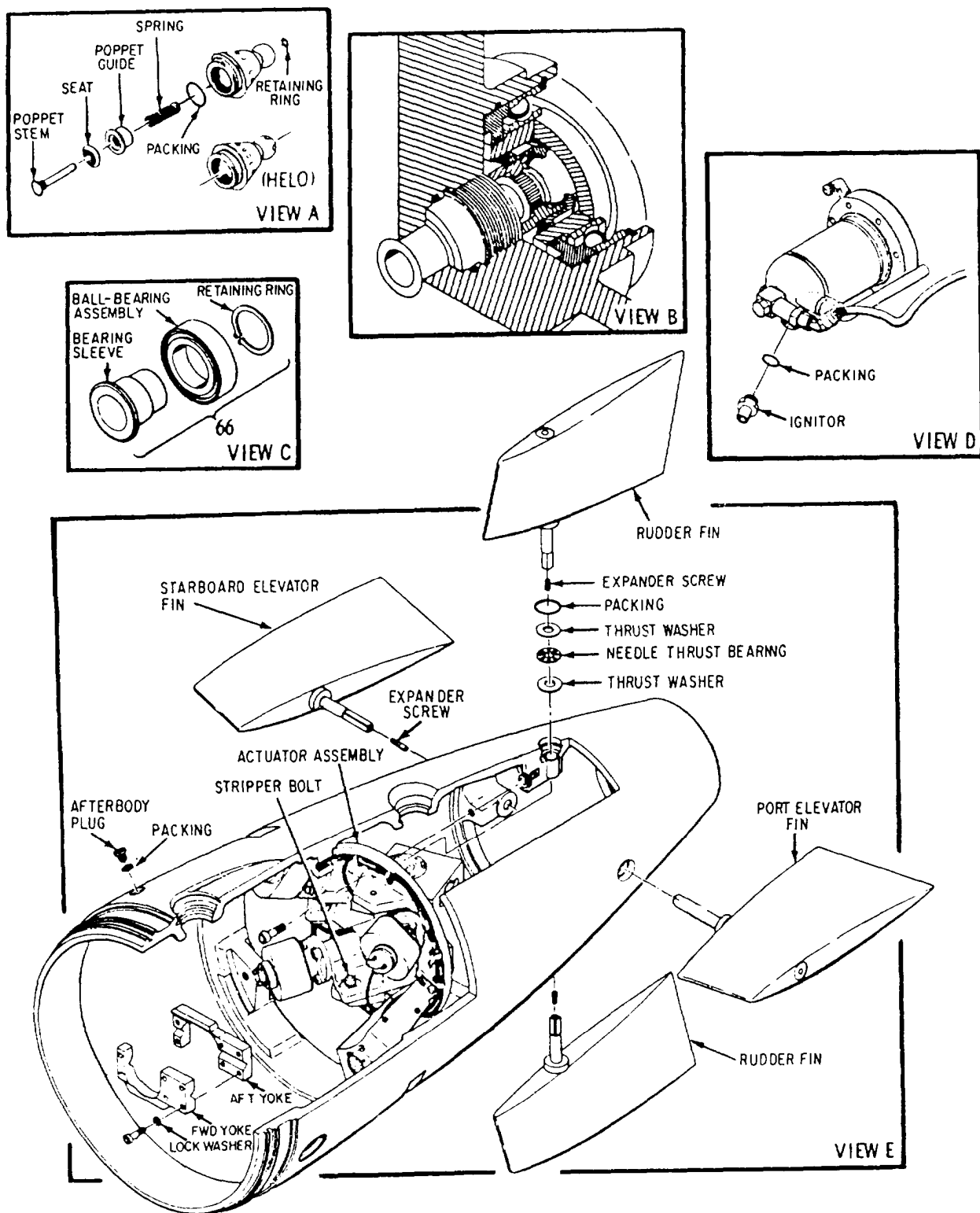
Figure 2-27.-Afterbody components.
