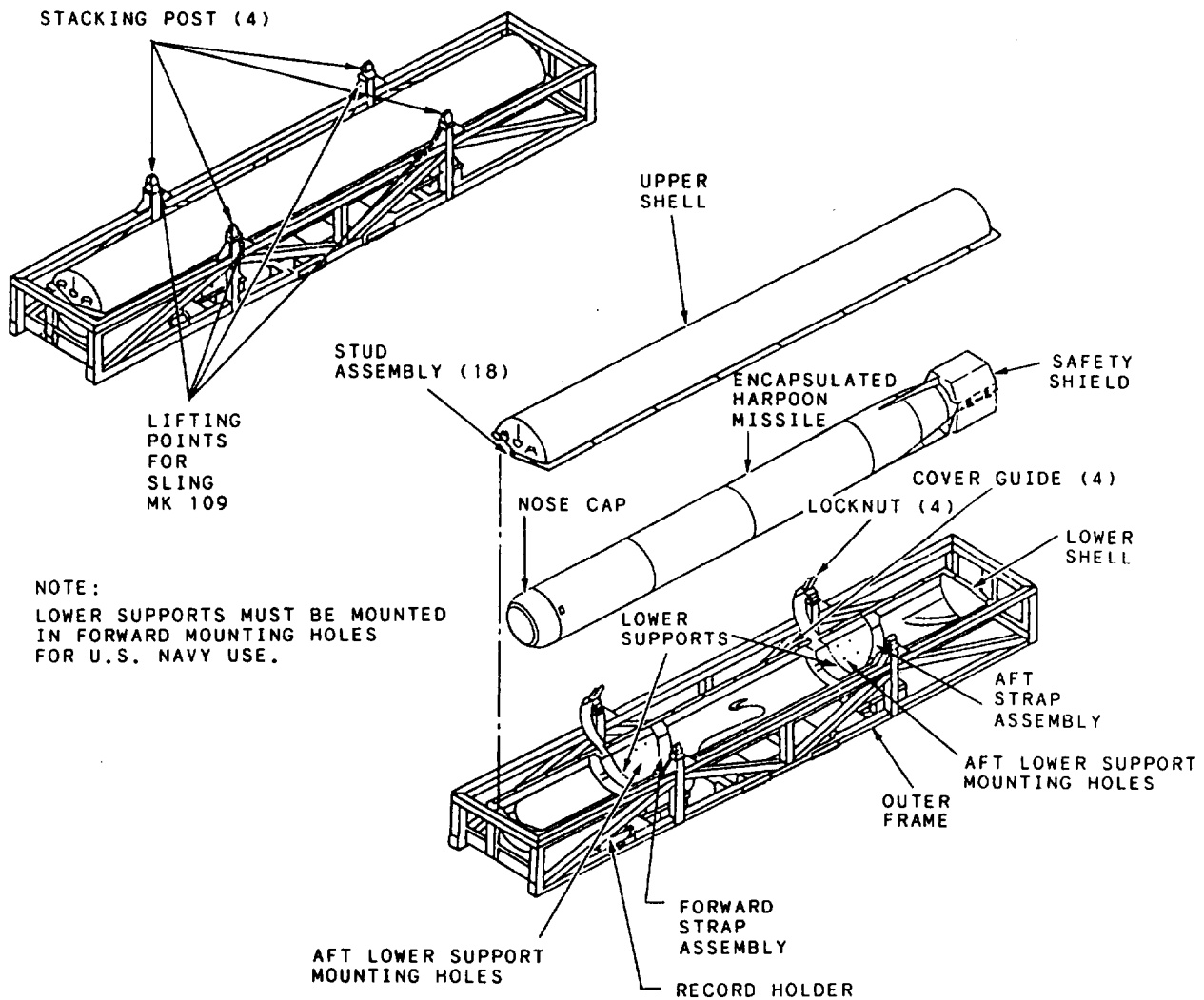
Figure 1-7.-Encapsulated Harpoon missile shipping container.
