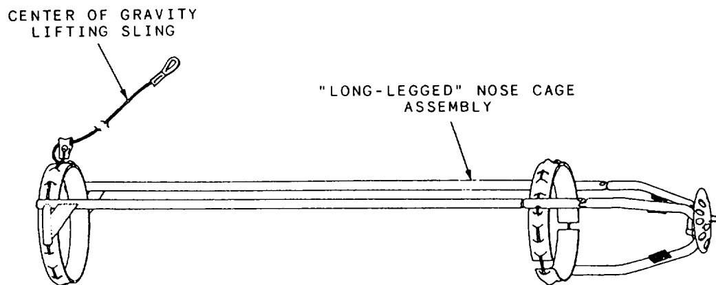
Figure 1-37.-Nose cage (Torpedo Mk 48, long-legged).
