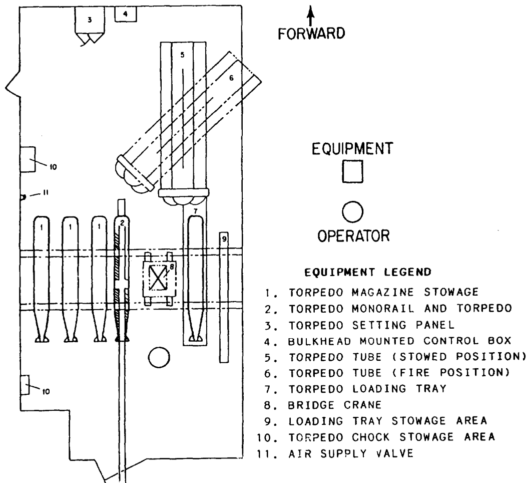
Figure 1-23.-Starboard torpedo room layout.
