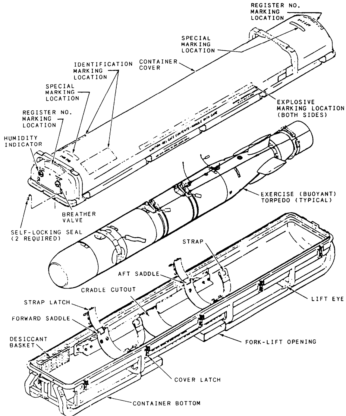
Figure 1-1.-Mk 46 torpedo container Mk 535 Mod 0.
