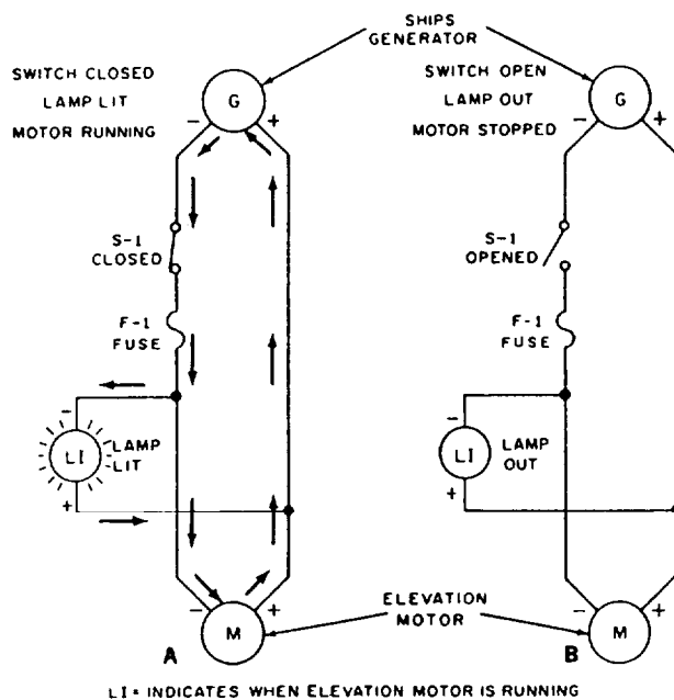
Figure 5-9.-Indicator lights.
