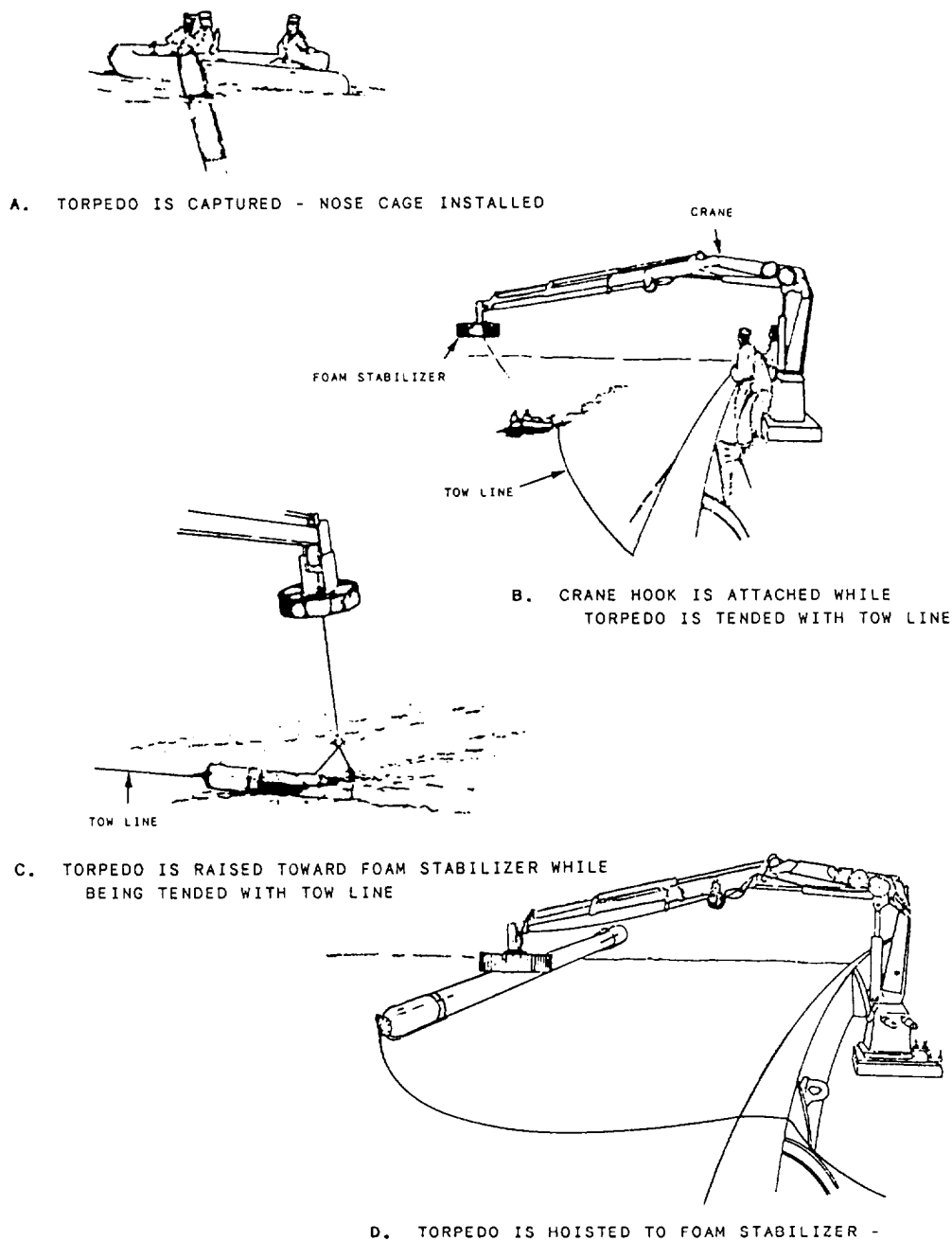
Figure 1-45.-Over-the-side recovery sequence.
