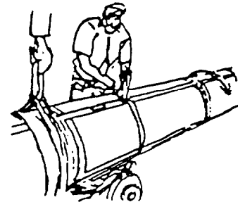
6. SECURING AEROSKID LASHING STRAPS
