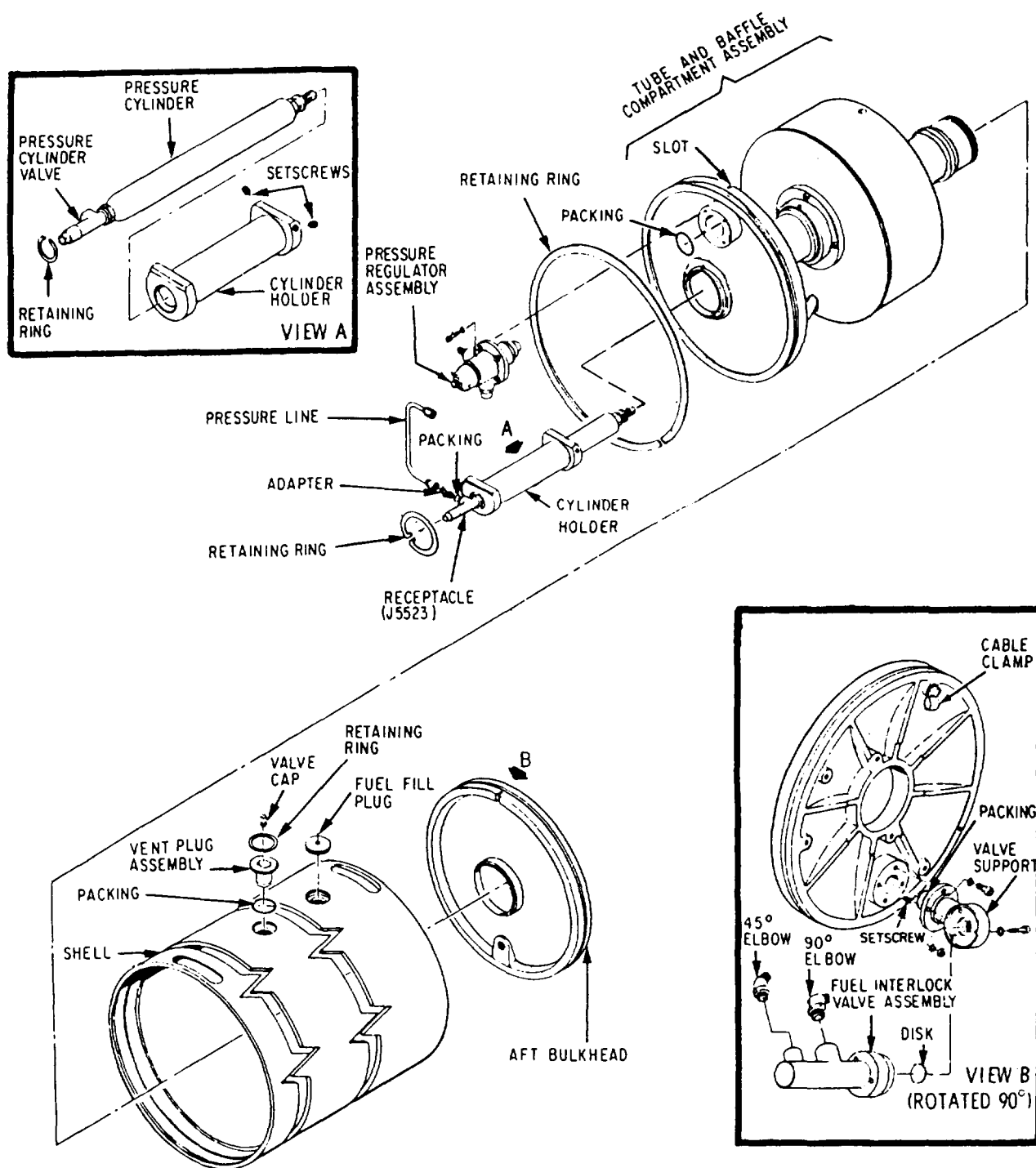
Figure 2-21.-Short fuel tank.
