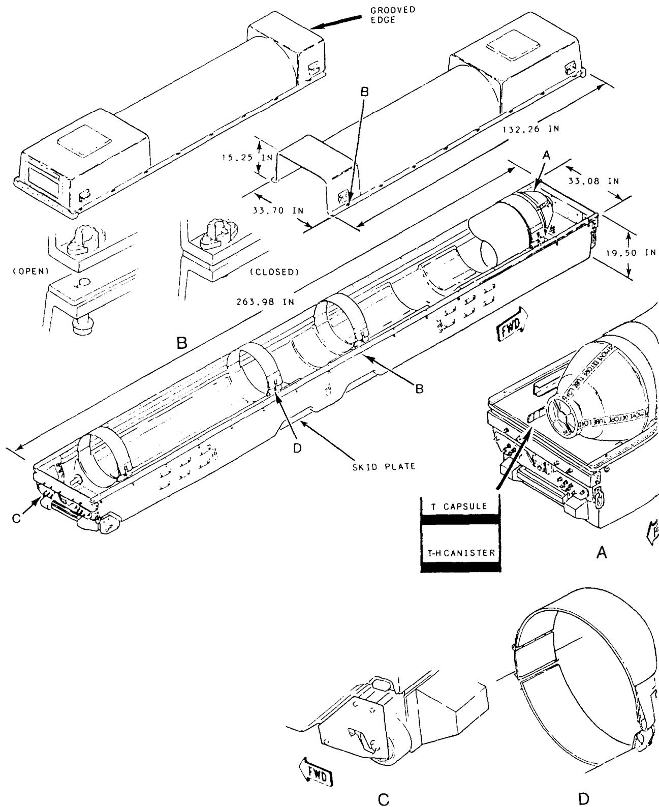
Figure 1-6.-Tomahawk AUR Shipping Container CNU-308/E.
