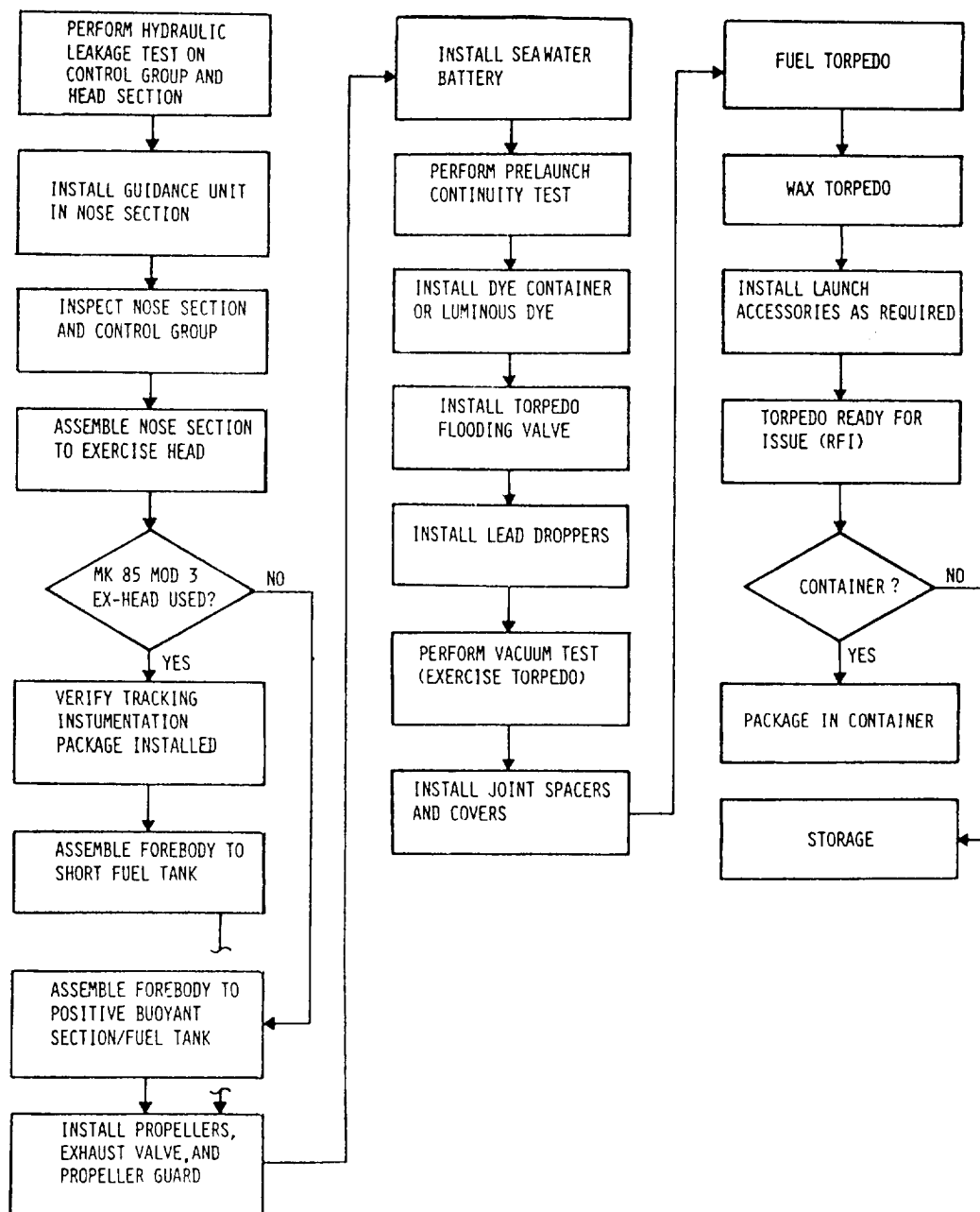
Figure 2-31.-Maintenance actions required after a torpedo (exercise) system test with the Mk 540 test set.
