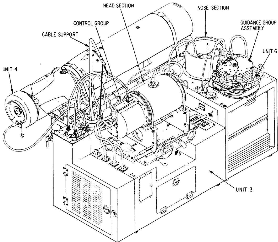
Figure 2-30.-Guidance and control test fixture, unit 3.
