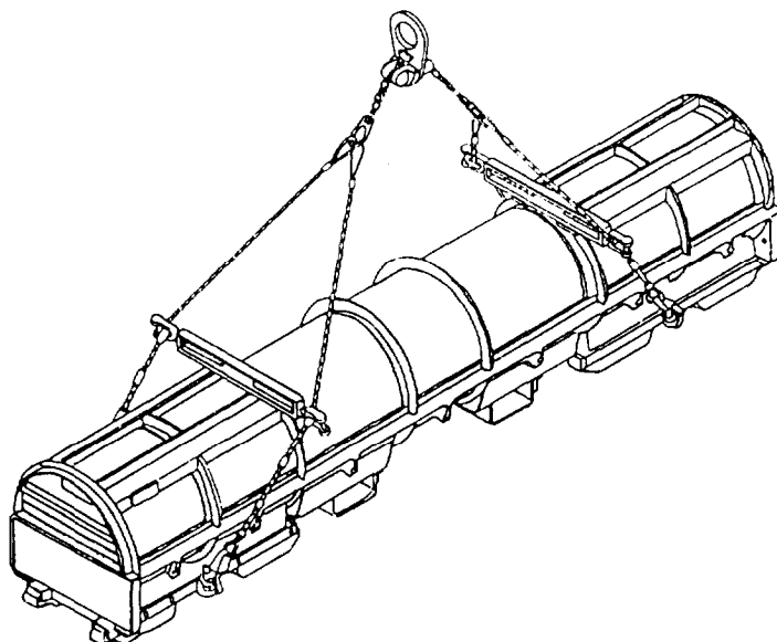
Figure 1-15.-Slings for lifting containers.
