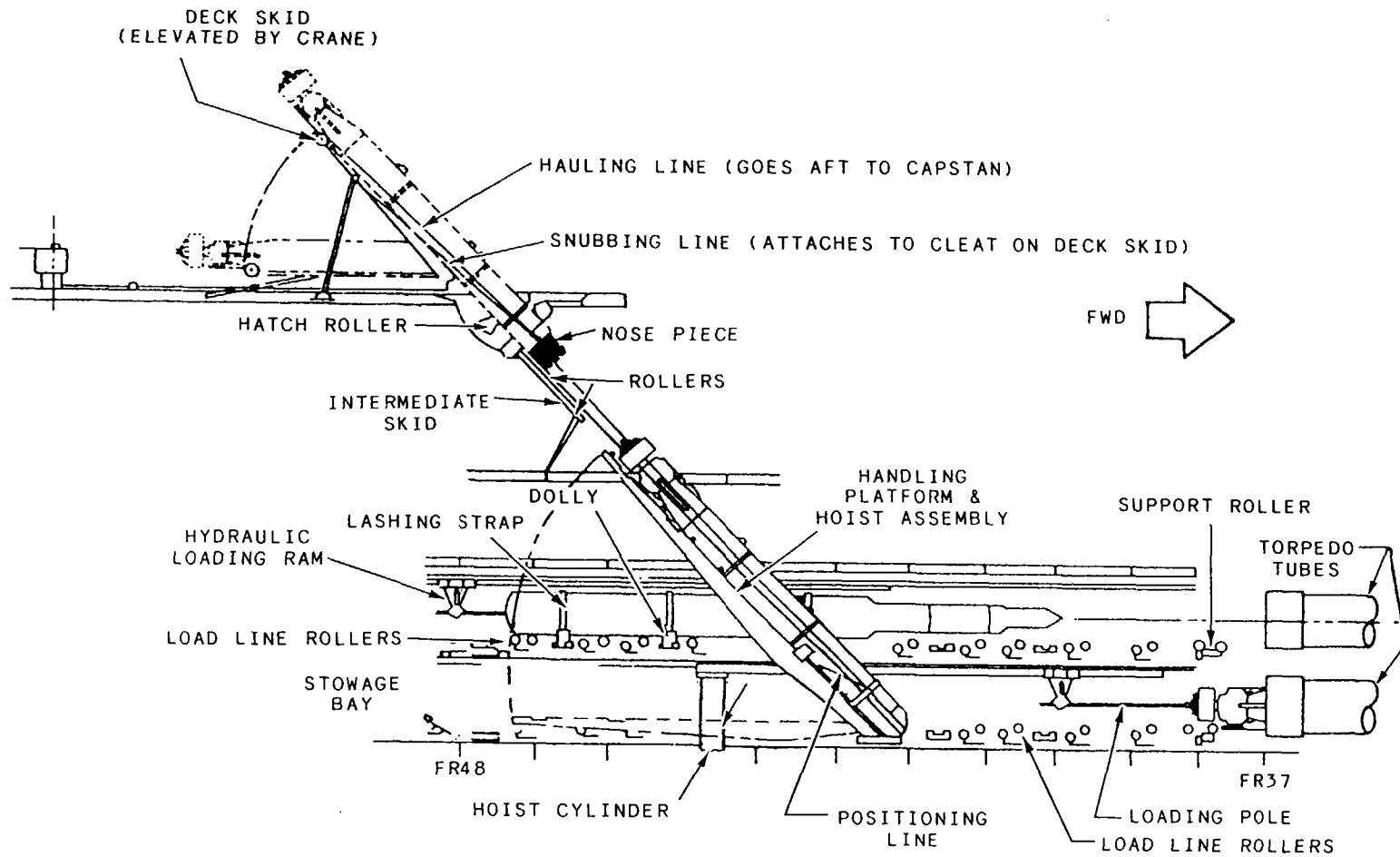
Figure 1-20.—SSN 637-class torpedo room.
