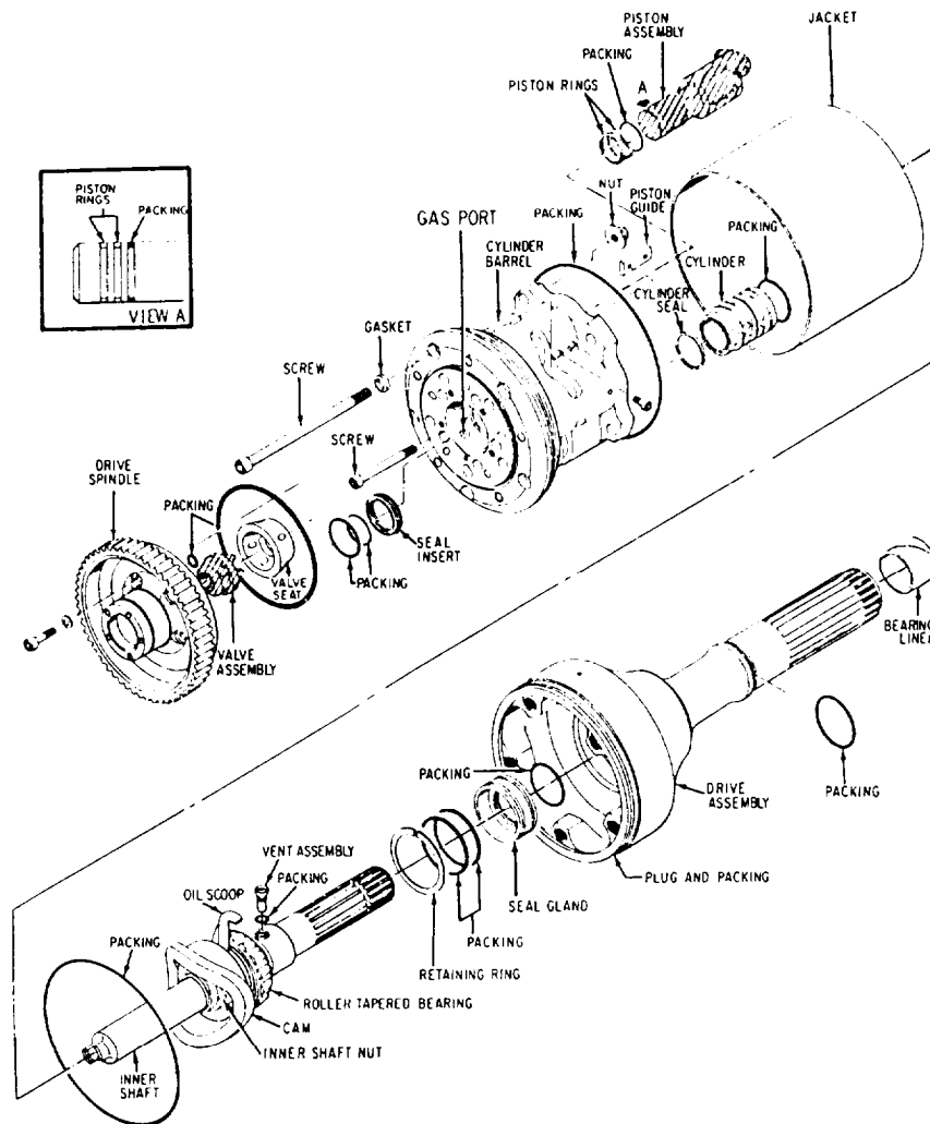
Figure 2-29.-Positive displacement engine.
