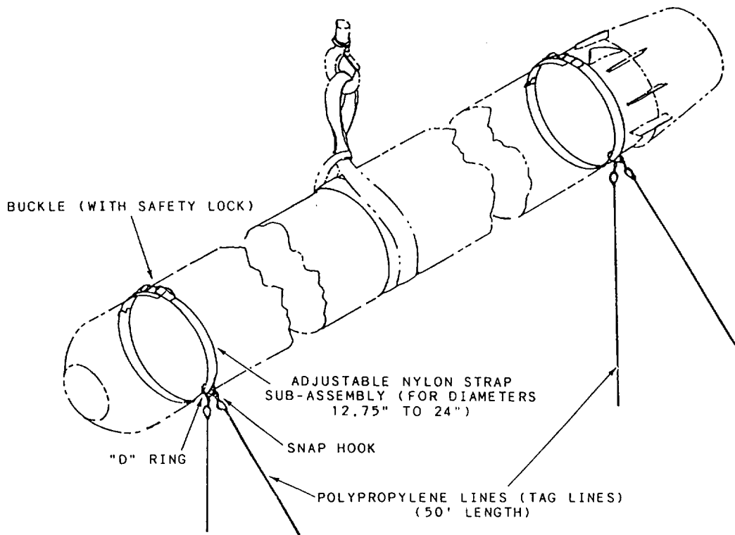
Figure 1-16.-Tagline Mk 1 Mod 0.
