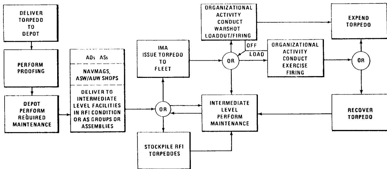
Figure 2-1-Typical torpedo maintenance cycle.
