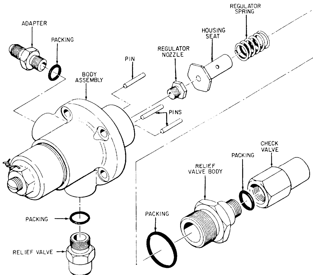
Figure 2-23.-Pressure regulator assembly (exploded view).
