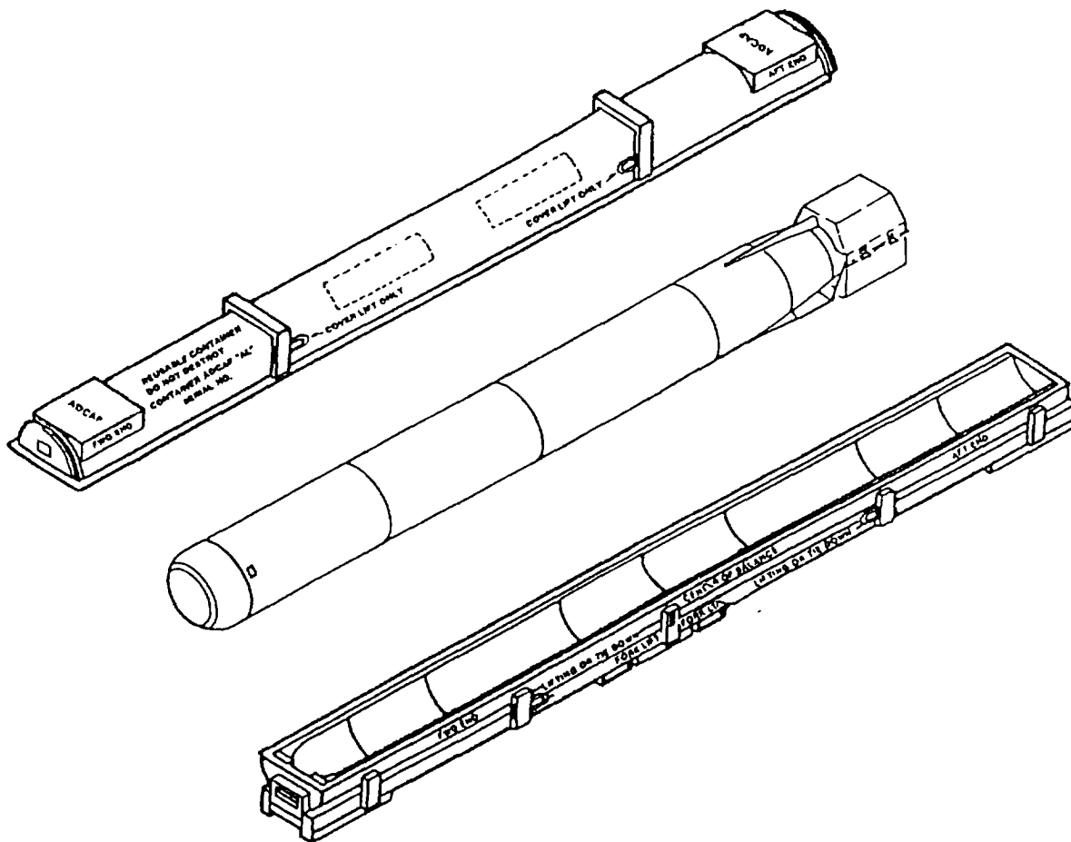
Figure 1-2.-Mk 48 torpedo shipping container Mk 481 Mod 1.
