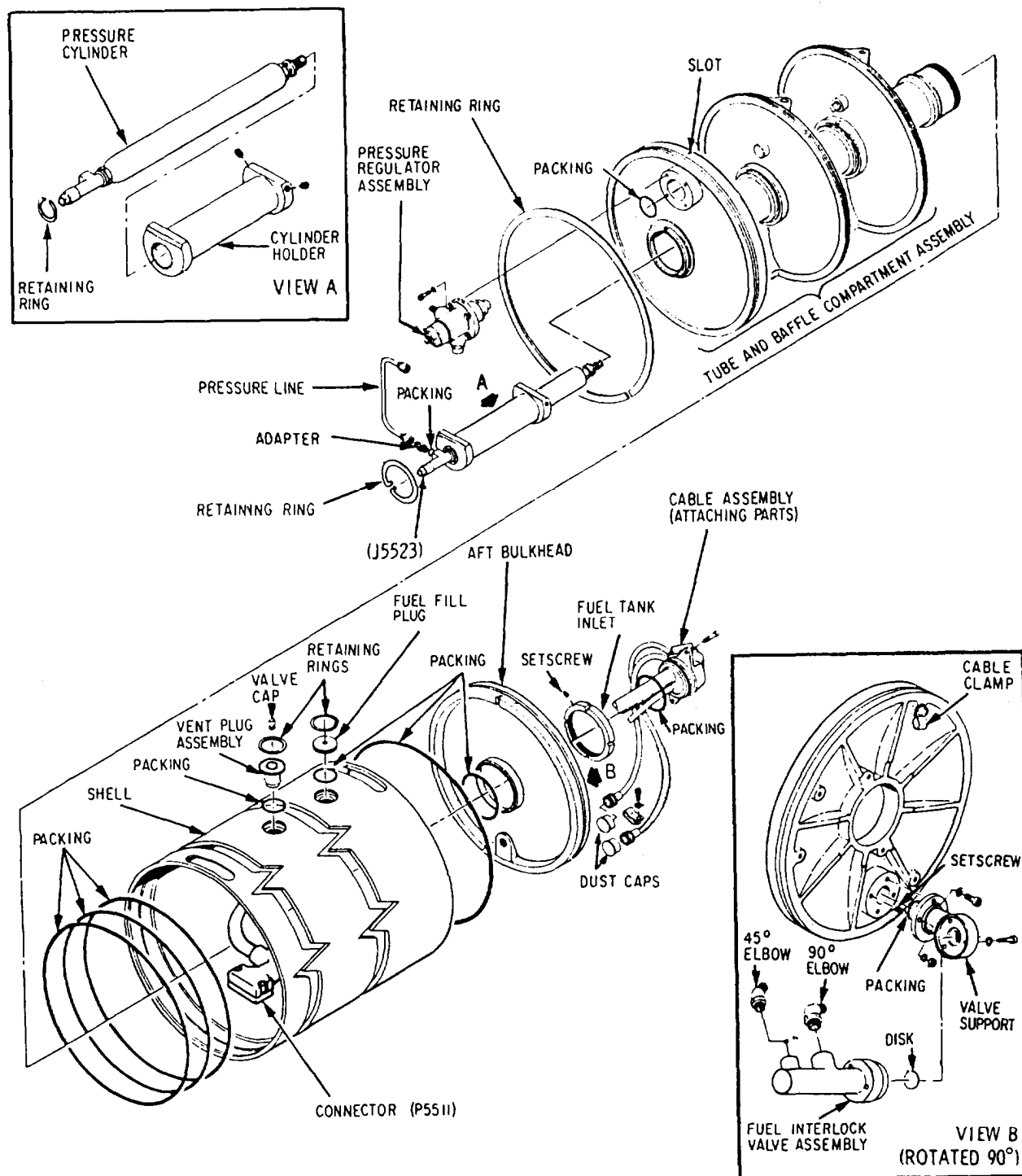
Figure 2-22.-Short fuel tank (disassembled for tenth-run turnaround maintenance).
