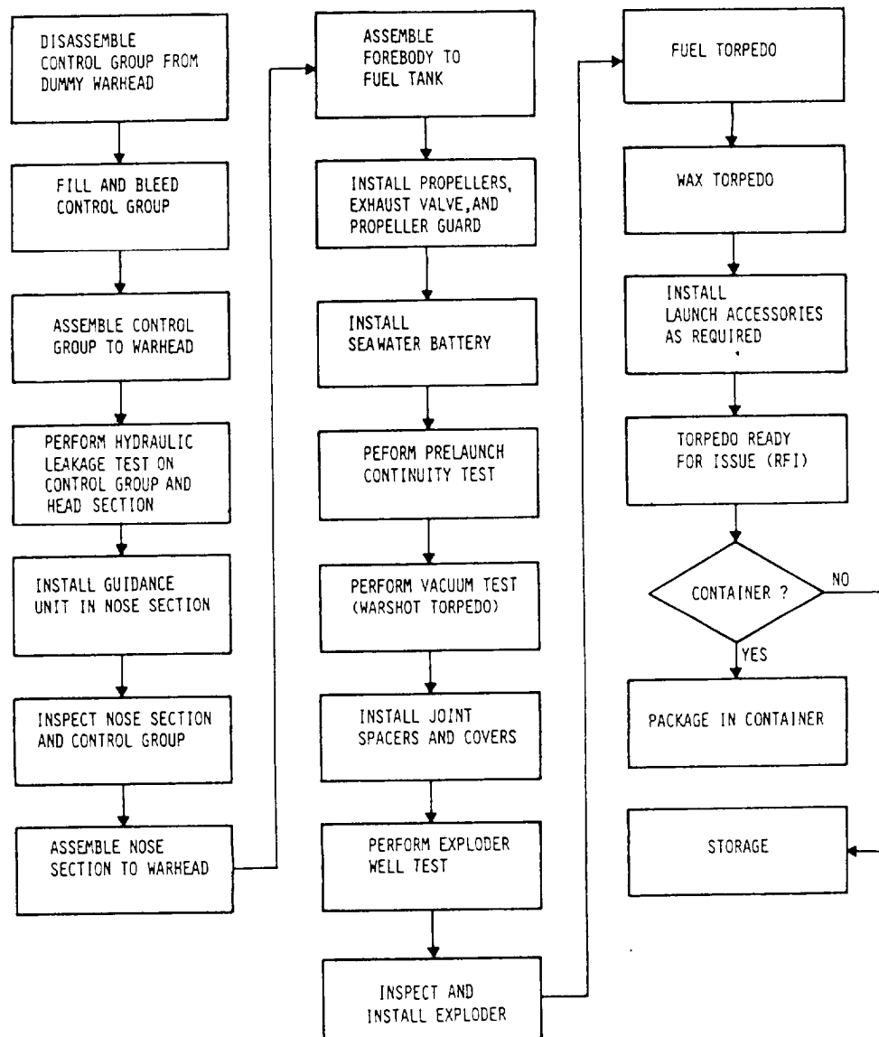
Figure 2-32.-Maintenance actions required after a torpedo (warshot) system test with the Mk 540 test set.
