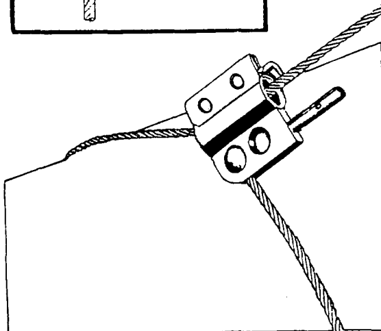
Figure 1-27.-Snare locked on a weapon.
