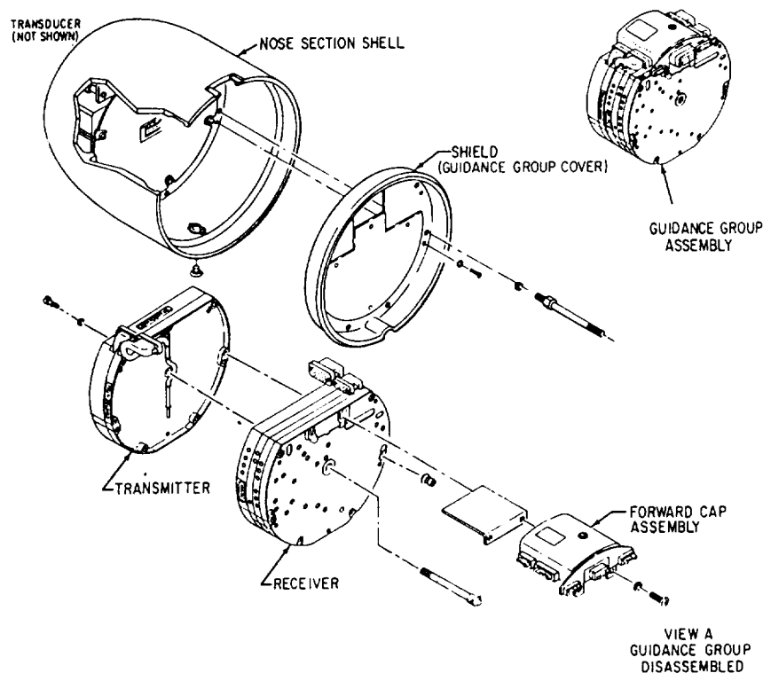
Figure 2-14.-Nose section.
