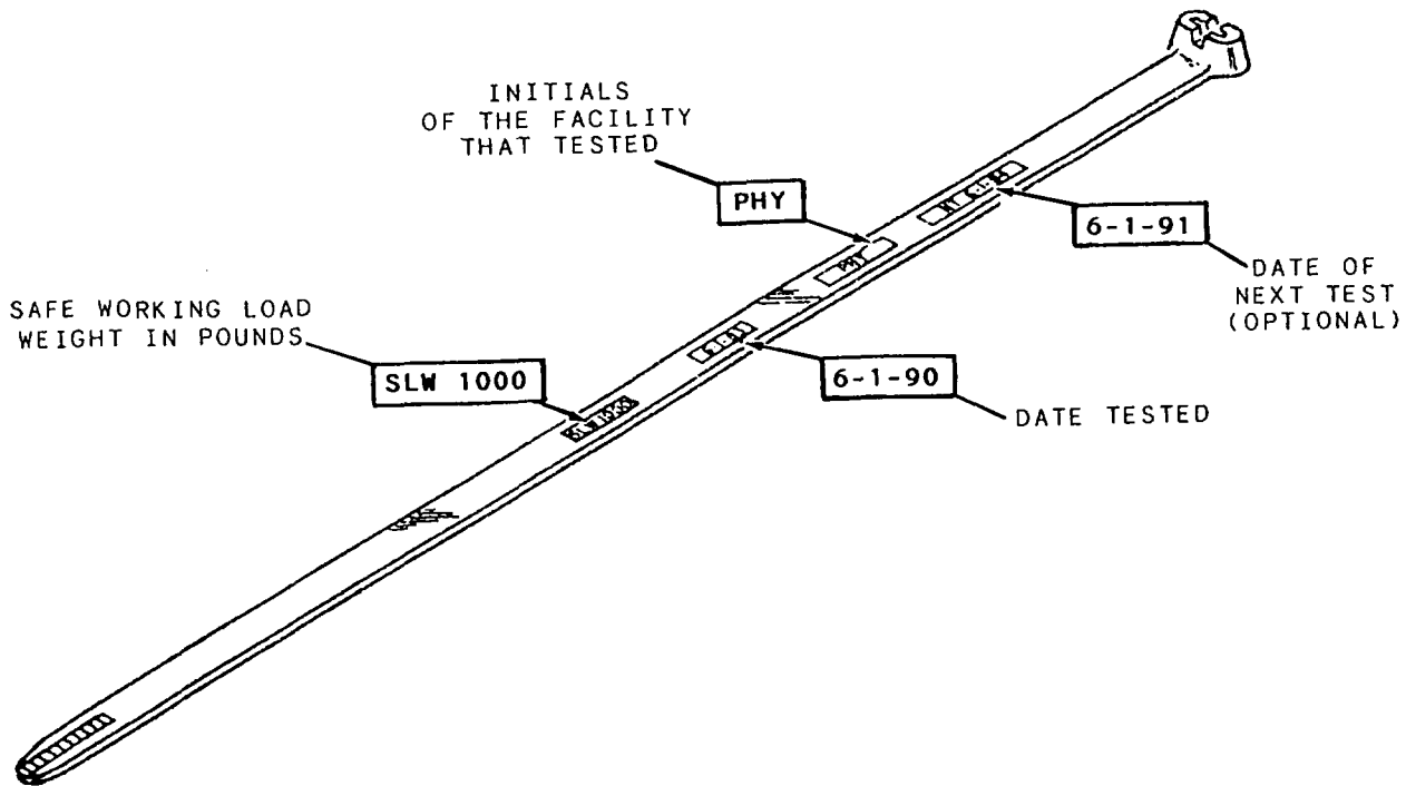
Figure 1-25.-Periodic load test record strap.
