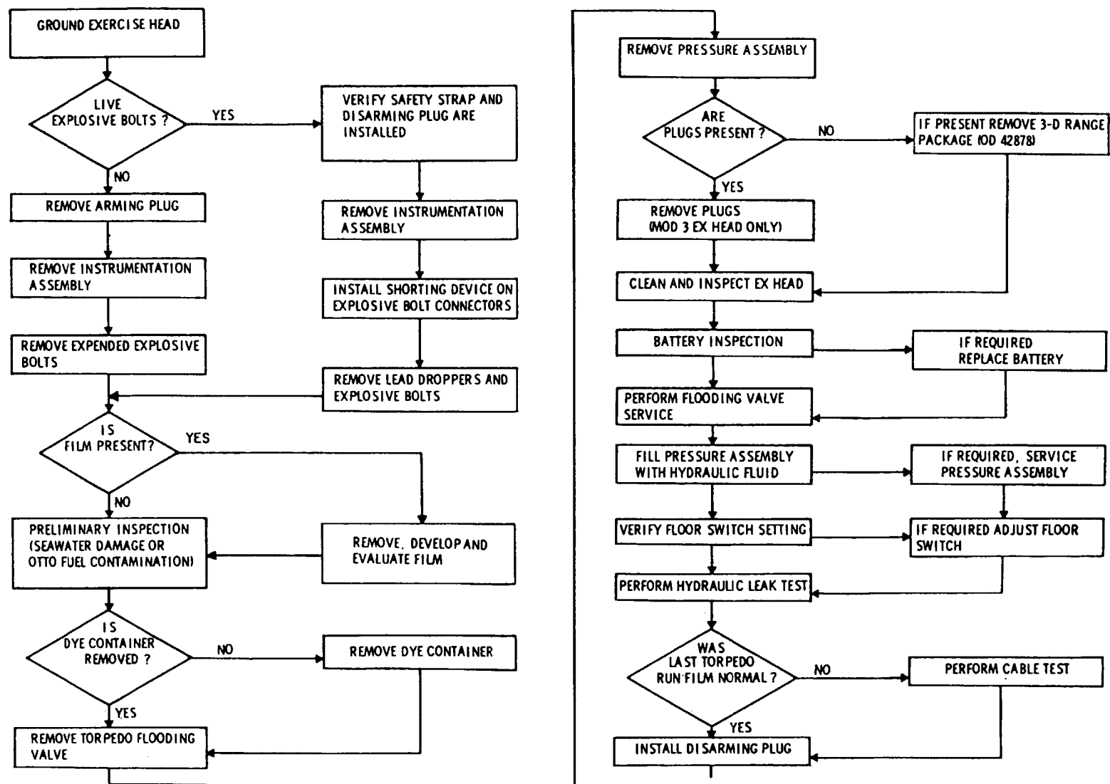
Figure 2-18.—Maintenance flow diagram for the exercise head.
