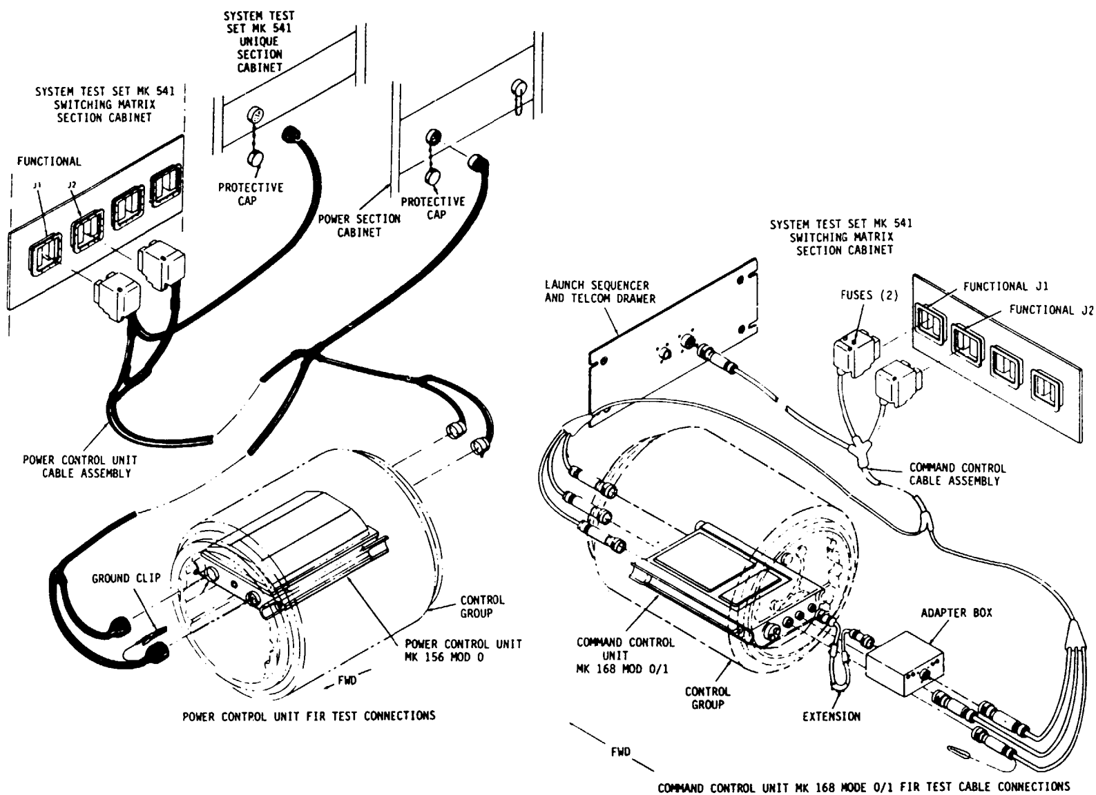
Figure 3-13.—Power control unit and command control unit; FIR test setup.
