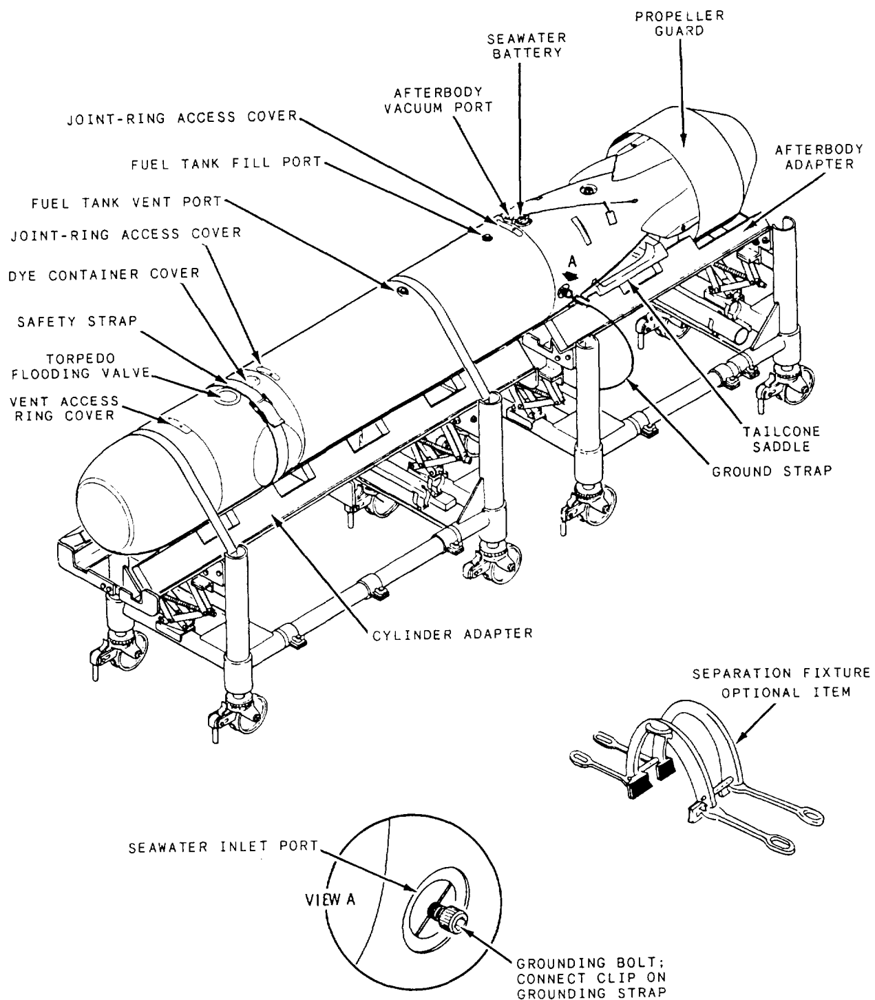
Figure 2-11.-Mk 46 torpedo (exercise) on universal dollies.
