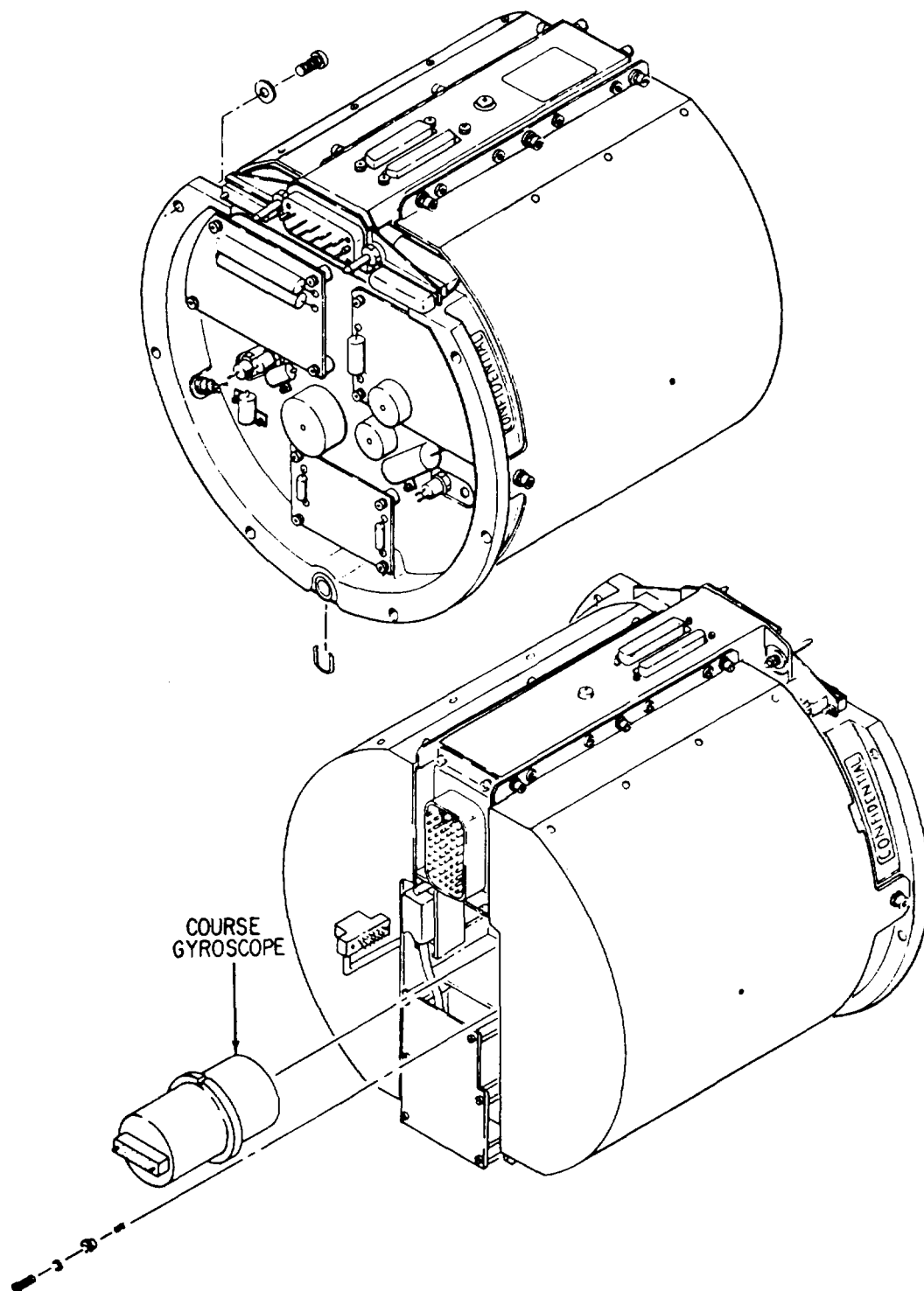
Figure 2-19.-Control group.
