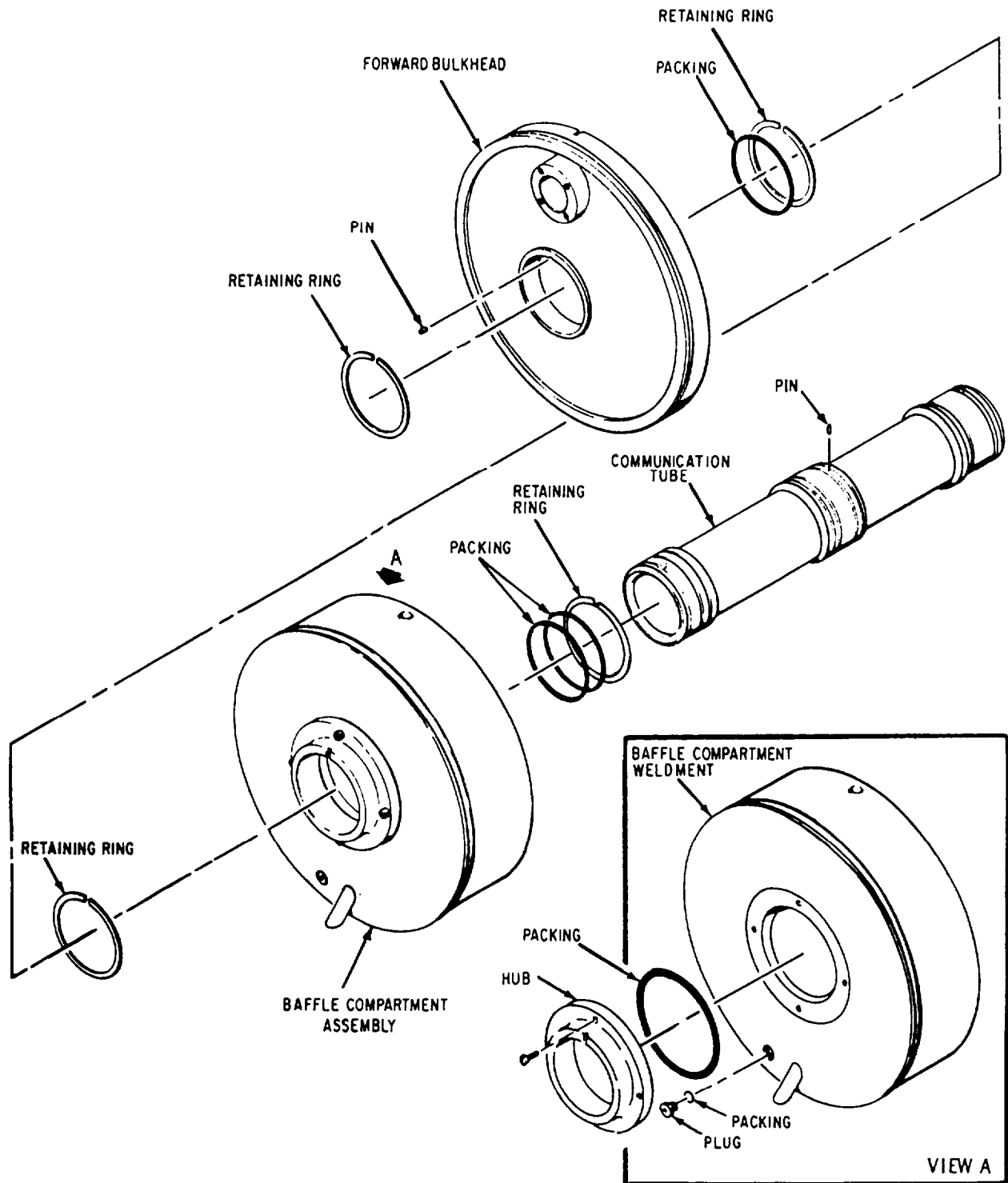
Figure 2-25.-Short fuel tank tube and baffle compartment assembly.
