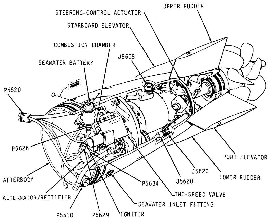
Figure 2-26.-Afterbody component locations.
