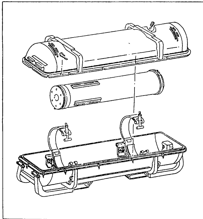
Figure 1-4.-Rocket motor Mk 37 container Mk 178.
