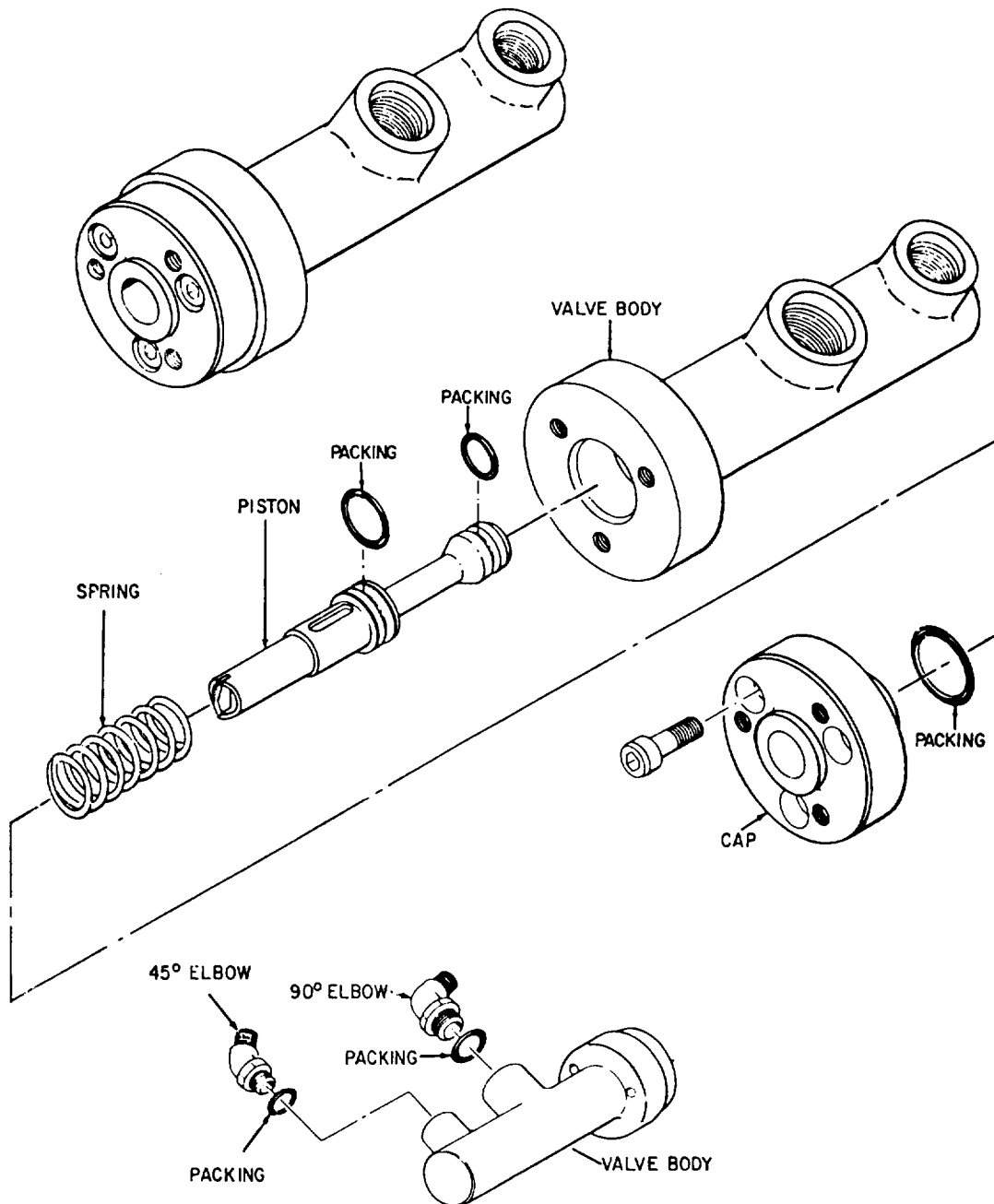
Figure 2-24.-Fuel interlock valve assembly.
