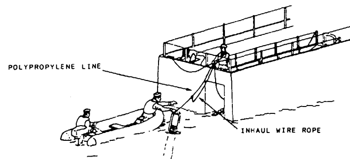
D. THE INHAUL HOOK IS PASSED DOWN THE POLYPROPYLENE LINE
