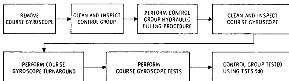
Figure 2-20.-Control group turnaround diagram.
