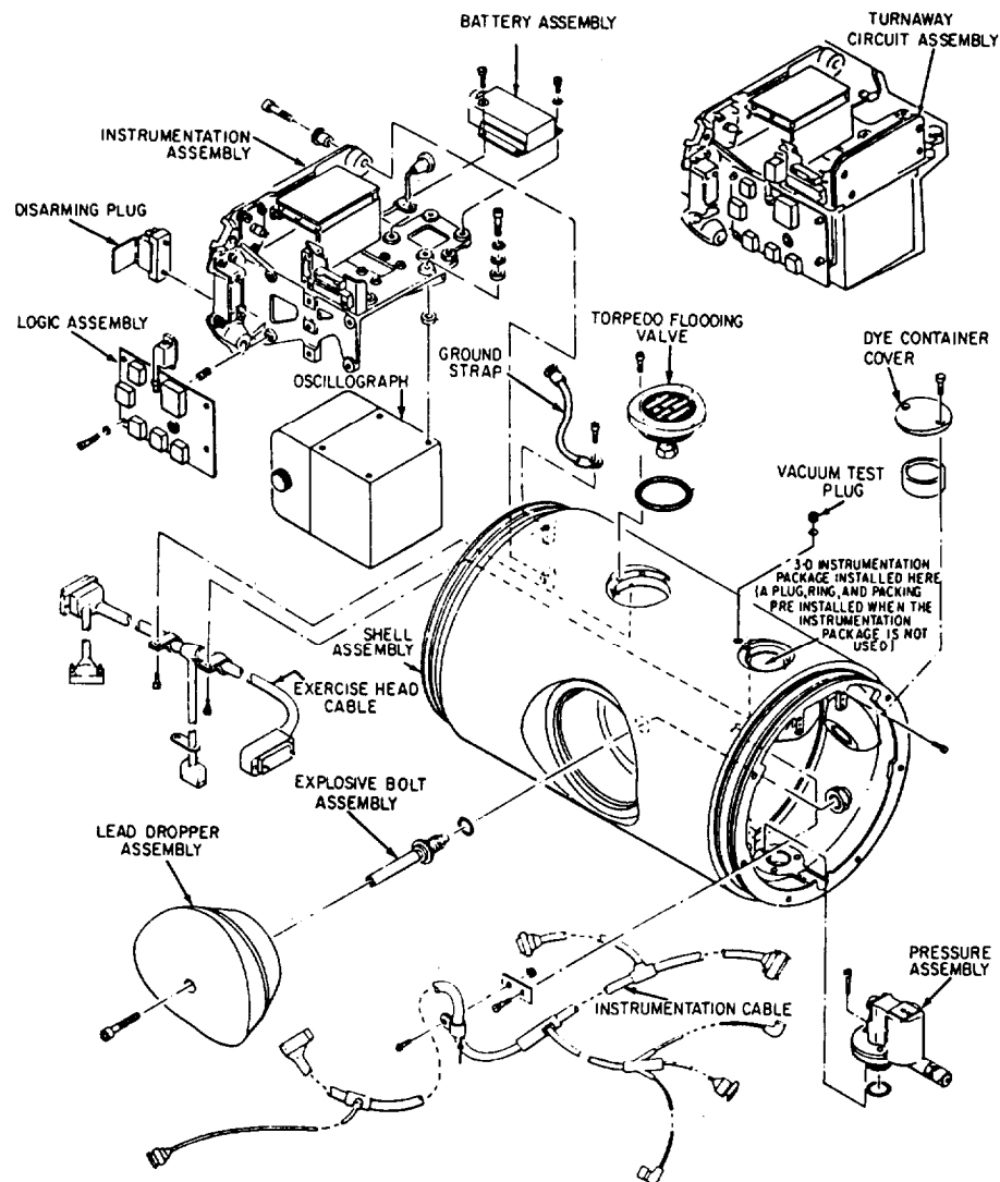
Figure 2-15.-Mk 85 Mod 3 exercise head.
