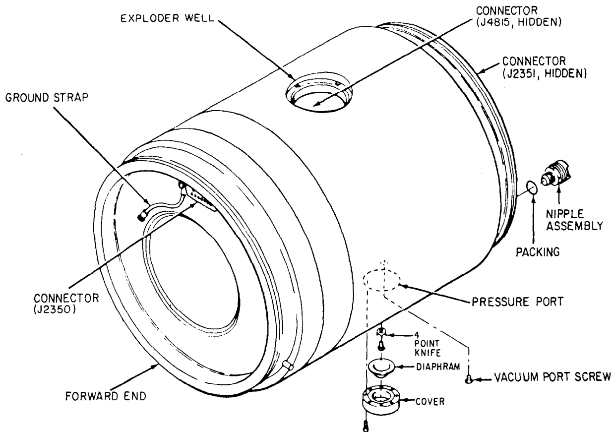
Figure 2-33.-Mk 103 warhead.
