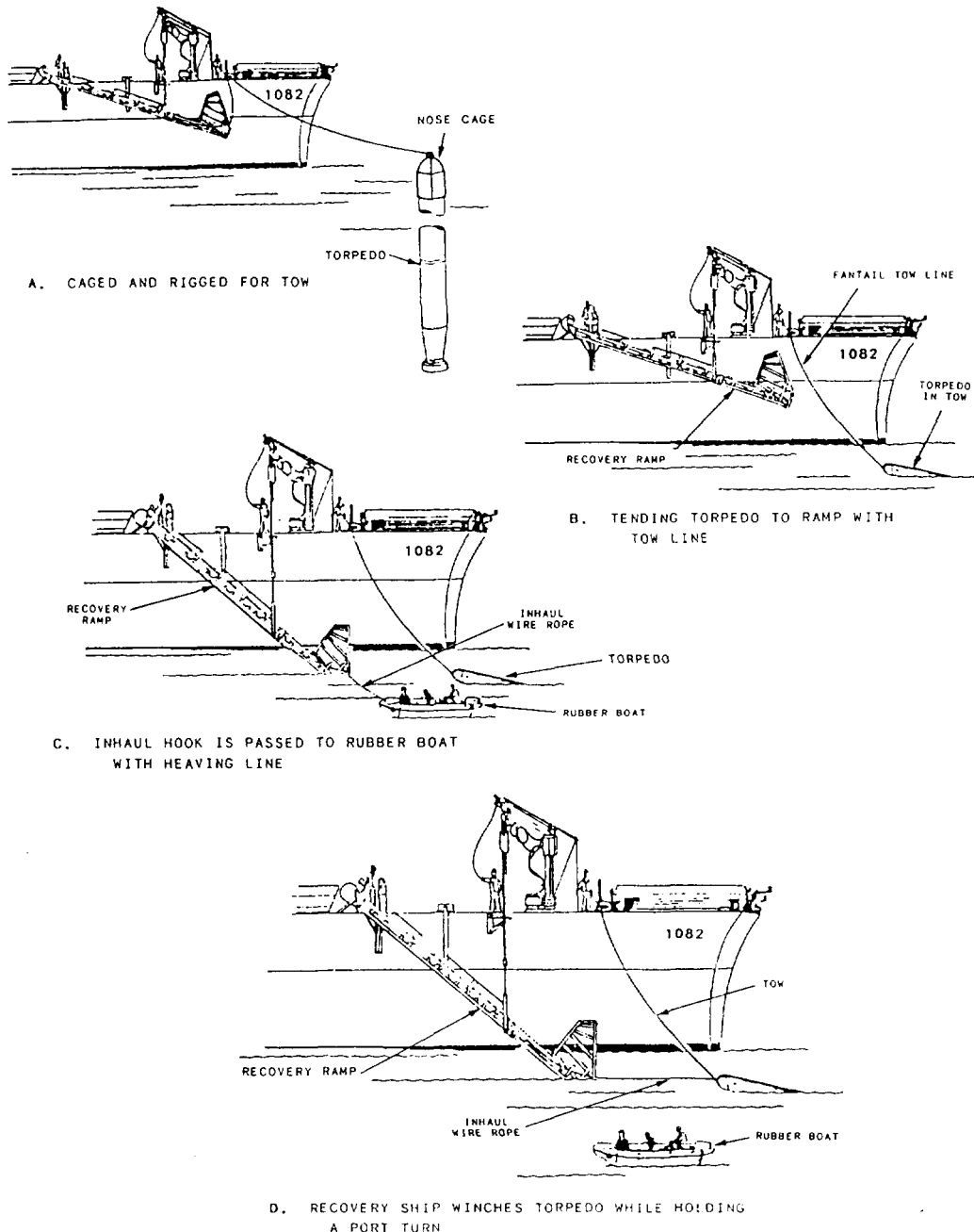
Figure 1-44.-Portable ramp recovery (pictorial).
