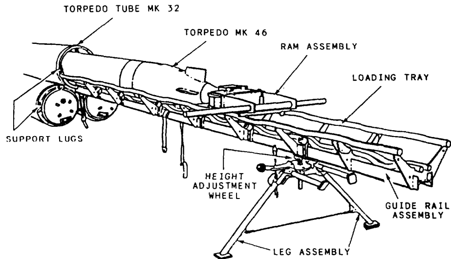
Figure 1-22.-Torpedo loading tray Mk 2.
