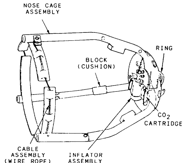
Figure 1-36.-Nose cage (Torpedo Mk 48 STD).
