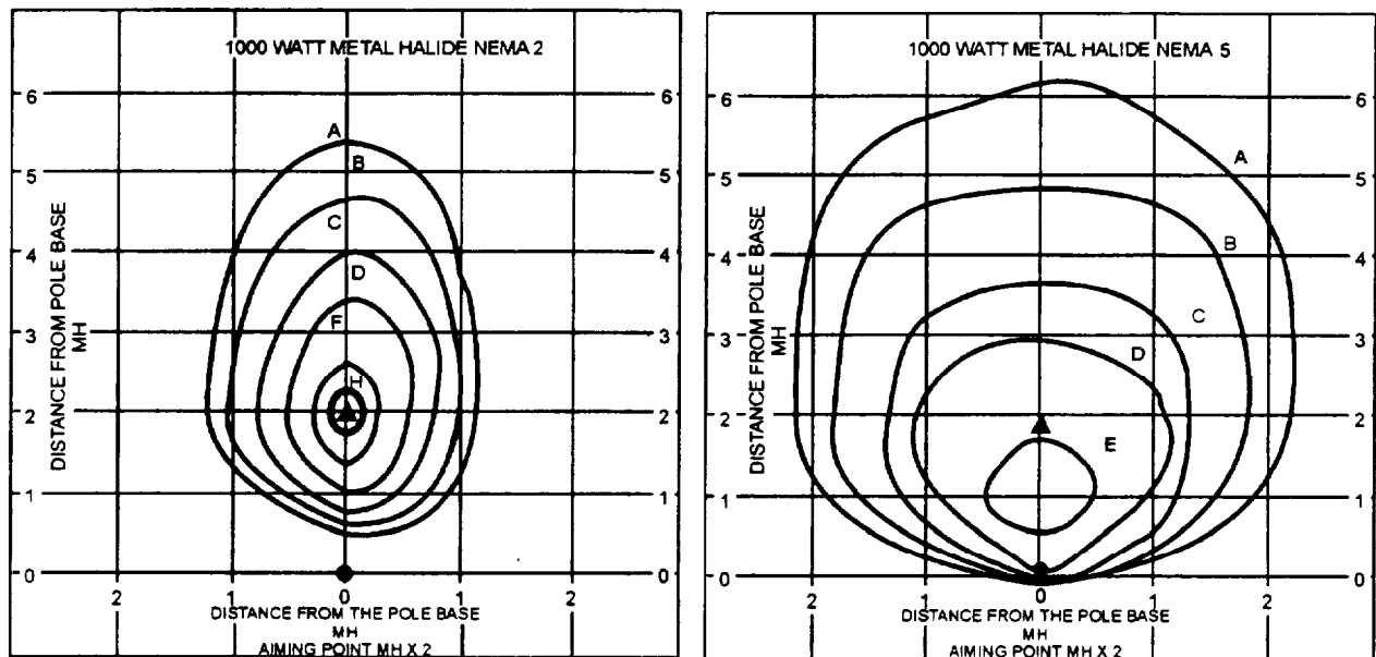
Figure 6-26.—Isofootcandle diagrams.
