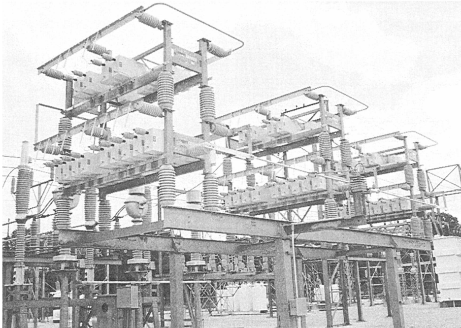
Figure 4-29.—Capacitors, open-rack installation.
