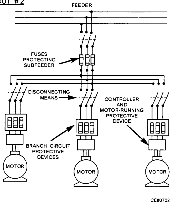
Figure 7-2.—Branch-circuit layout #2.
