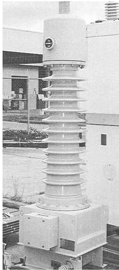
Figure 4-28.—Coupling capacitor.
