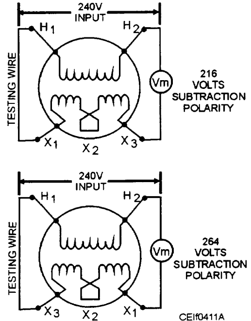
Figure 4-11.—Polarity tests.
