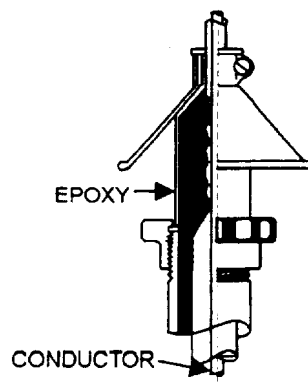
Figure 4-45.—Diagram of a modern single-phase cable end termination kit.
