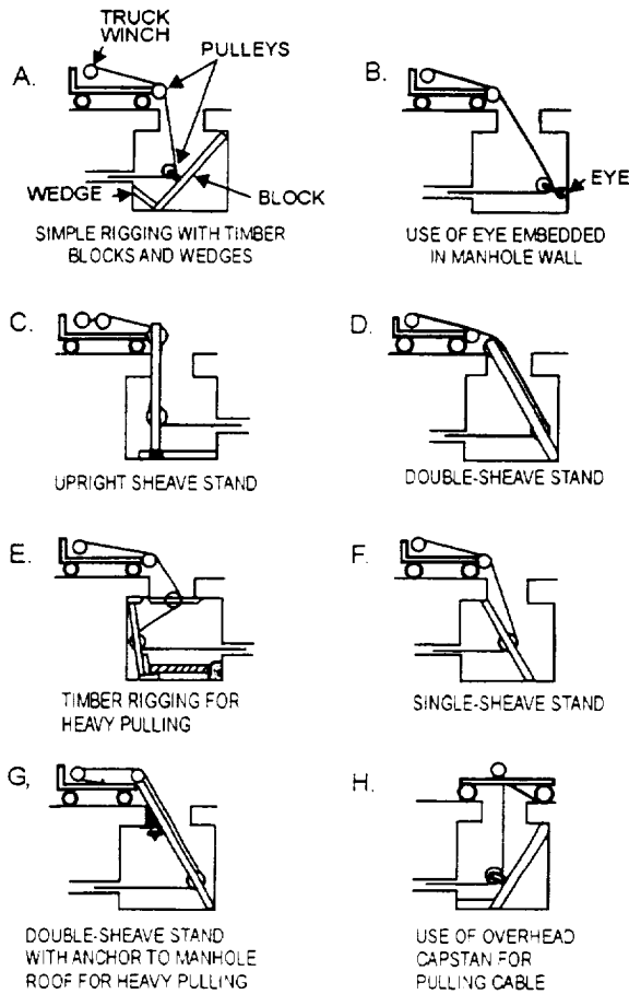
Figure 4-47.—Manhole rigging for pulling cables.
