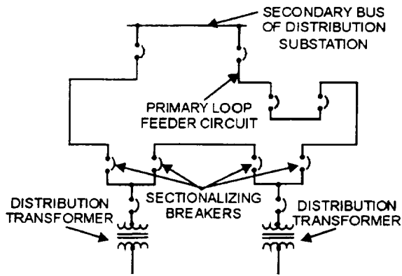
Figure 4-2.—Loop, or ring, distribution system.
