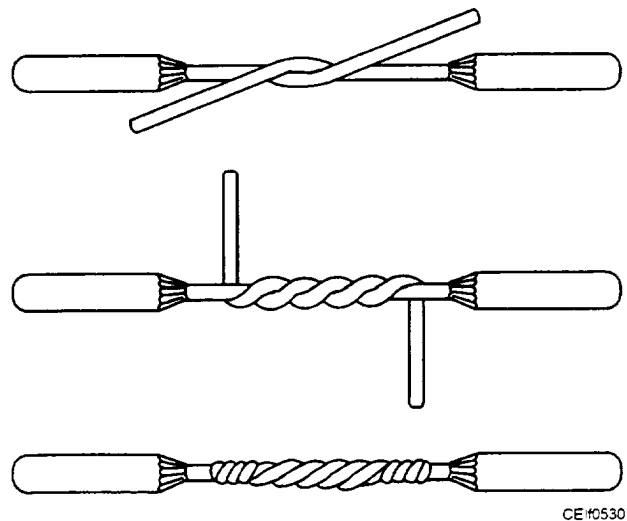
Figure 5-30.—Western Union splice used where substantial strain may be placed on the connection.
