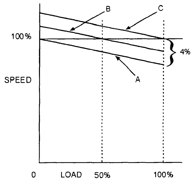
Figure 3-4.—Speed-droop governor curve.
