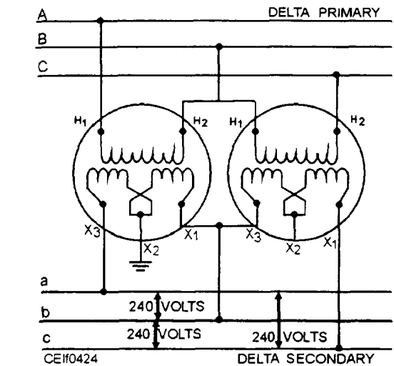
Figure 4-24.—Two single-phase transformers connected open-delta.
