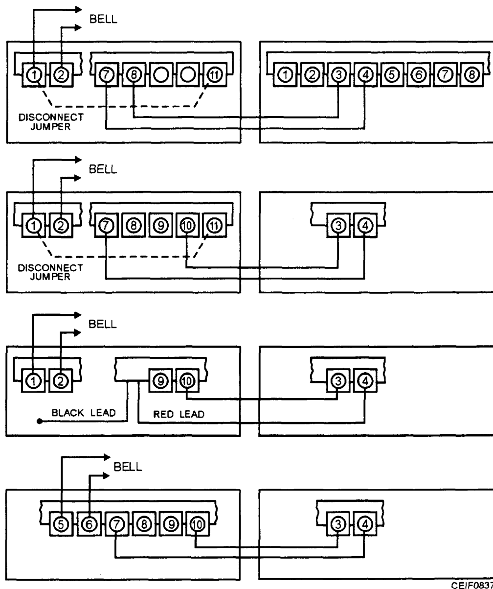
Figure 8-37.—Preferred connections for a typical telephone dialer.
