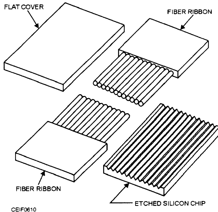
Figure 6-10.—Ribbon splice on etched silicon chip.
