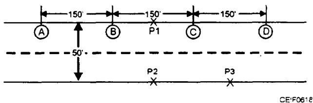
Figure 6-18.—Streetlight layout.
