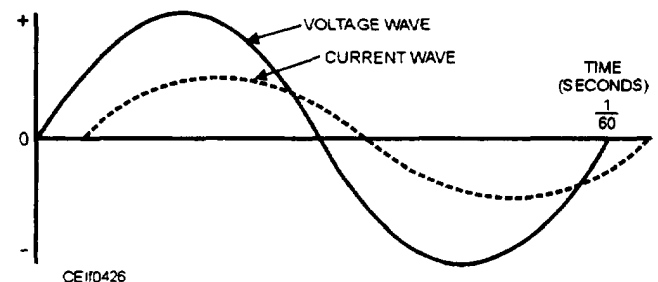
Figure 4-26.—Current wave lagging behind the voltage wave, usual condition in transmission and distribution systems.
