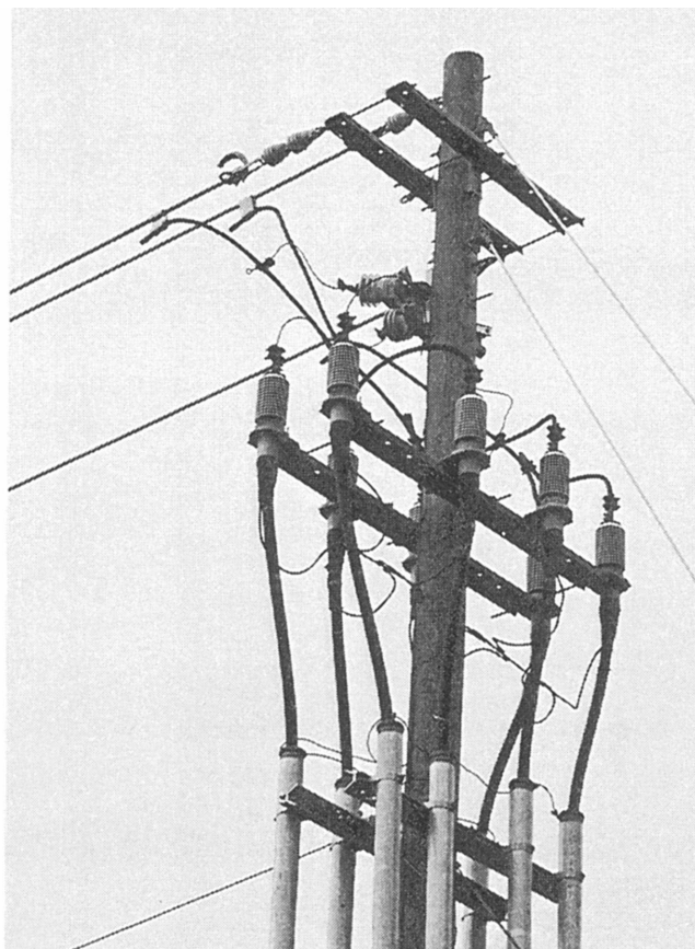
Figure 4-46.—Riser pole for underground distribution circuit.
