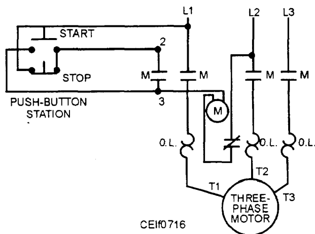
Figure 7-16.—Three-wire control circuit.
