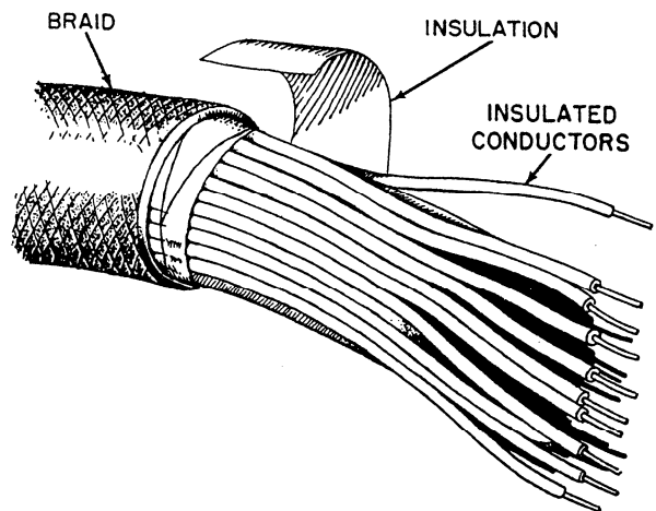
Figure 5-10.—Multiconductor cable.
