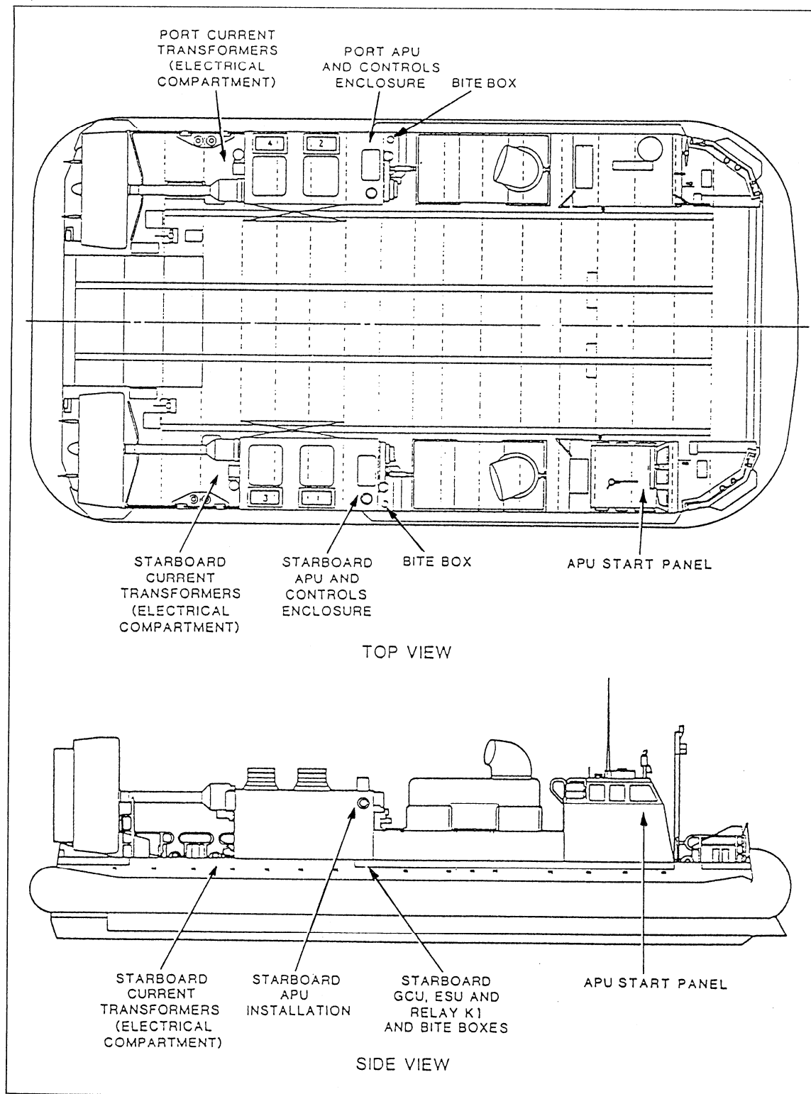
Figure 7-16.—Auxiliary powerunit (APU) locations.
