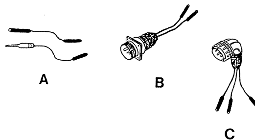
Figure 5-12.—Fabricated pin testers.
