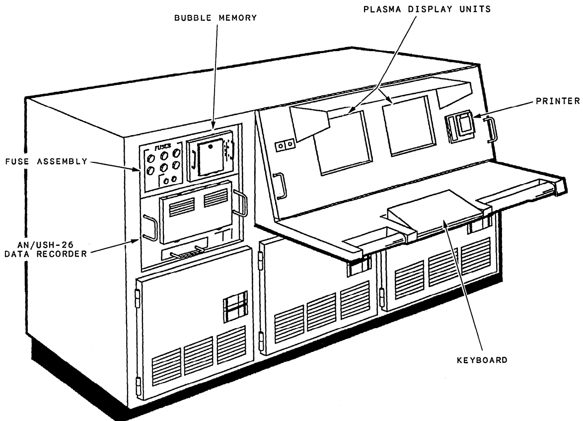
Figure 3-11.—Overall view of the EOOW/LU.
