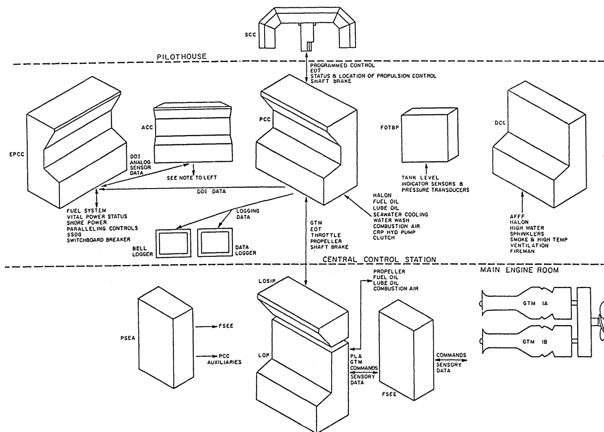
Figure 3-2.—Engineering plant control system.
