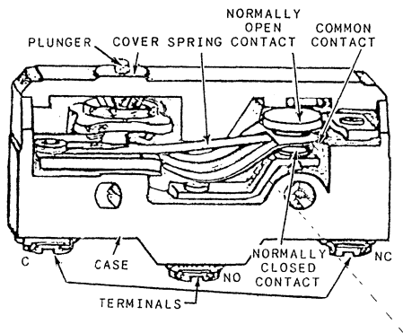
Figure 5-5.—Microswitch.
