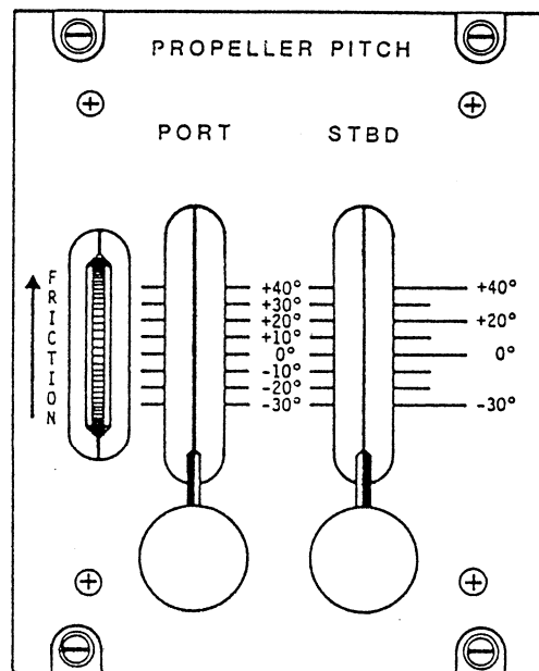
Figure 7-9.—Propeller pitch control levers.
