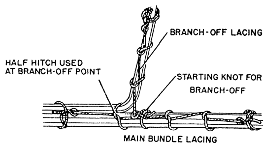
Figure 5-15.—Lacing a branch-off.
