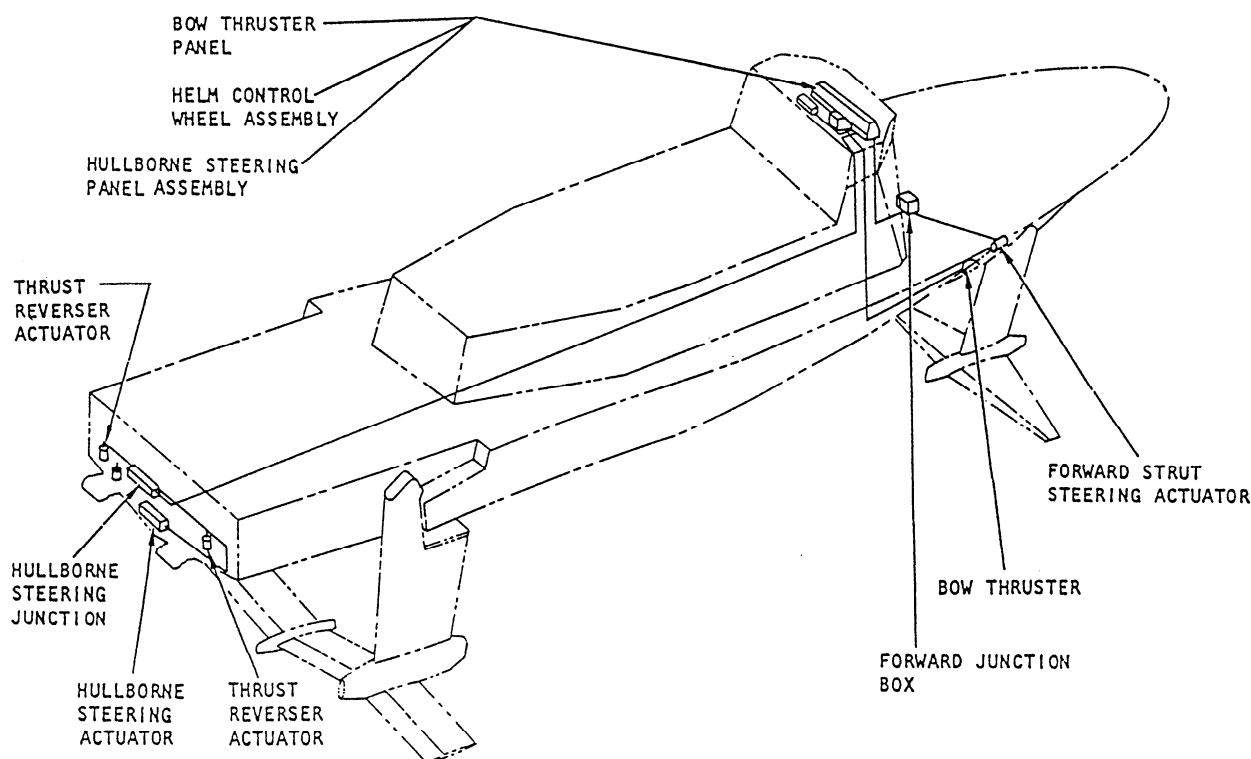
Figure 7-28.—Hullborne steering system equipment.
