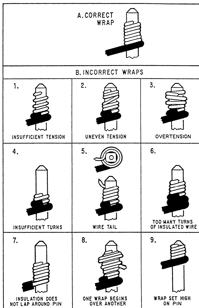
Figure 5-18.—Correct and incorrect wire wraps.
