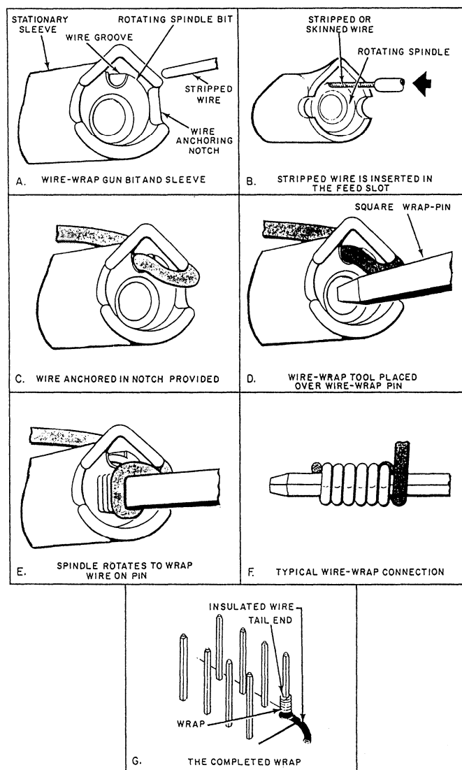
Figure 5-17.—Basic wire-wrap procedure.
