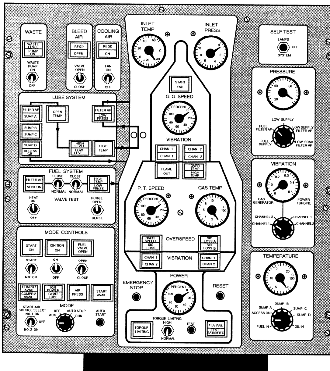
Figure 7-23.—Foilborne engine control system (FECS) panel at the EOS.
