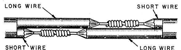
Figure 5-11.—Staggering splices.
