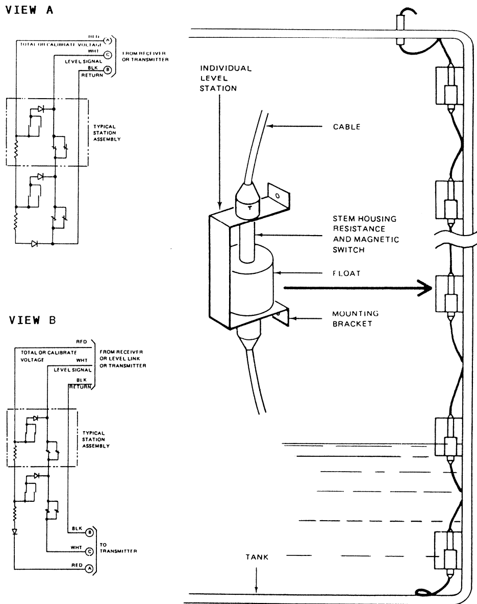
Figure 6-13.—Link transmitter float assembly.
