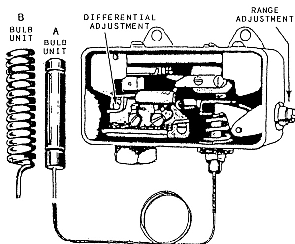
Figure 6-8.—Temperature switch with two types of sensing elements. A. Bulb unit. B. Helix unit.
