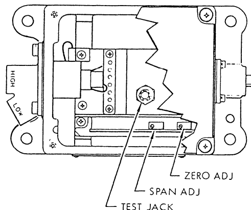
Figure 6-4.—Transducer construction.
