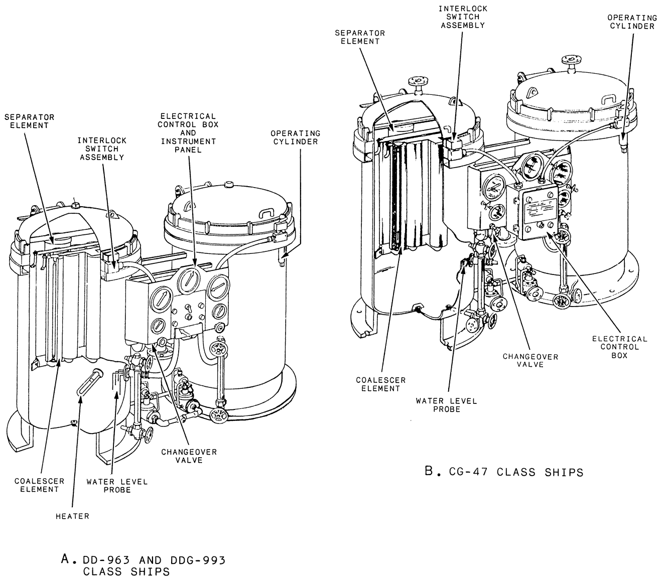
Figure 4-2.—Fuel oil filter/coalescers.
