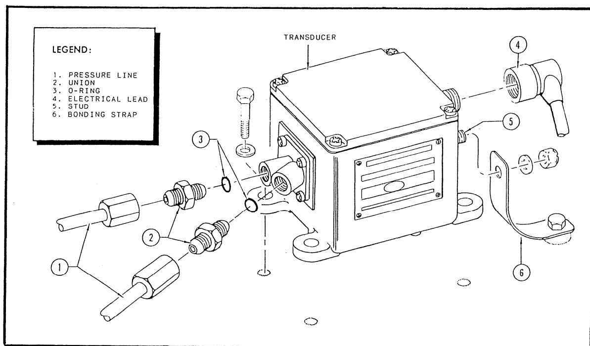
Figure 6-7.—Pressure transducer.
