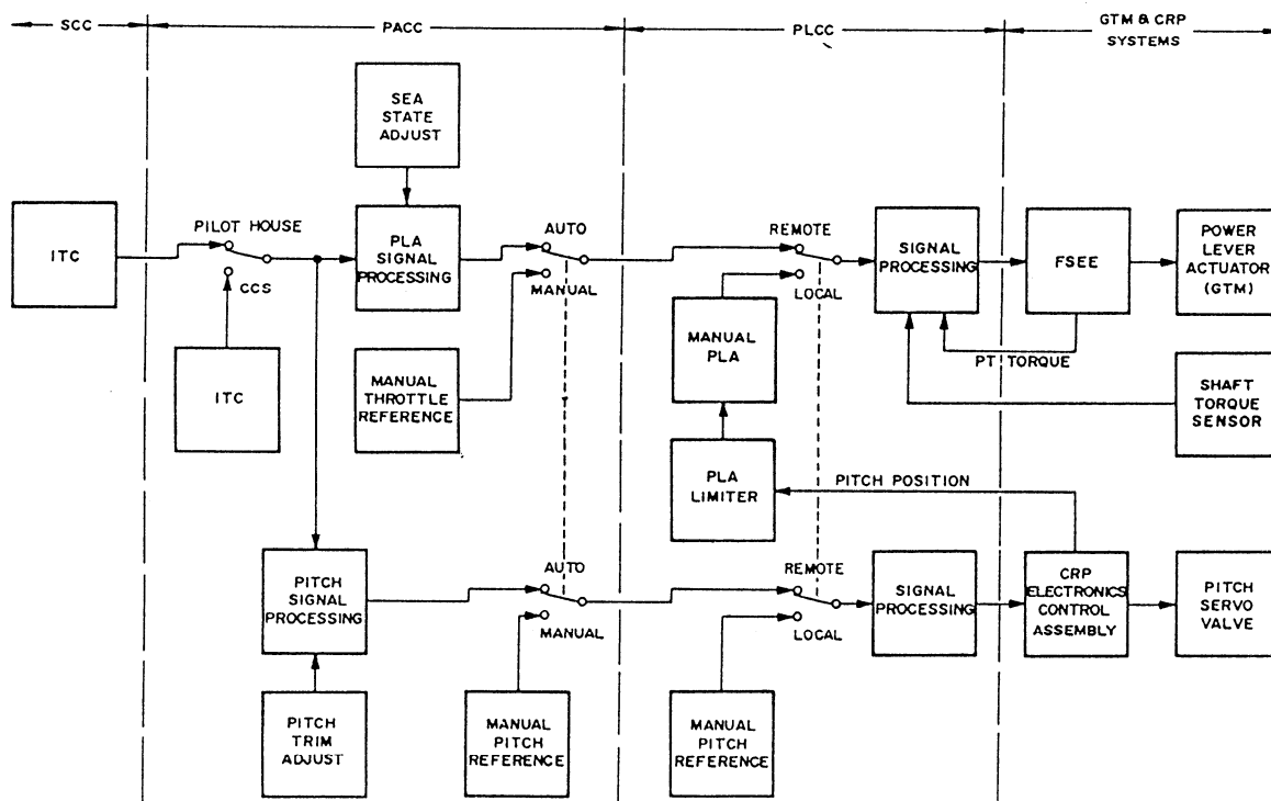
Figure 3-5.—Throttle and pitch control block diagram.
