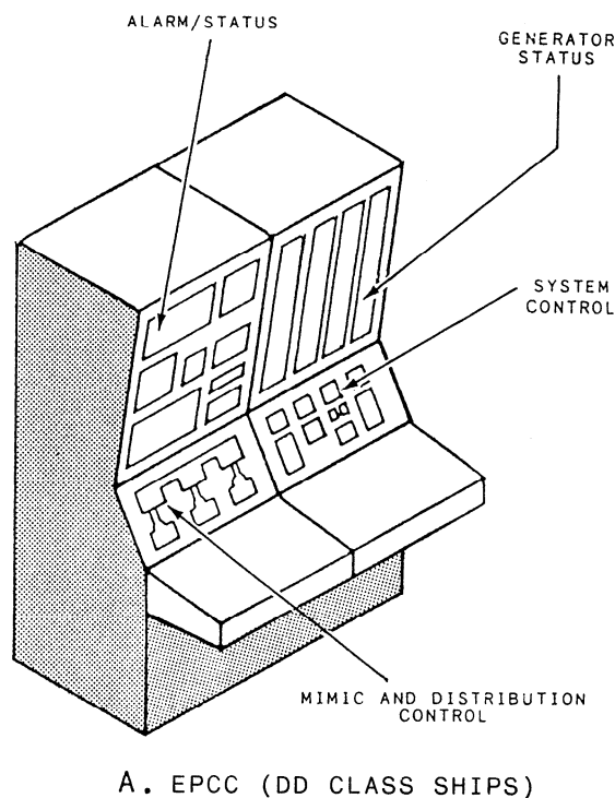
Figure 3-6.—EPCC layout.
