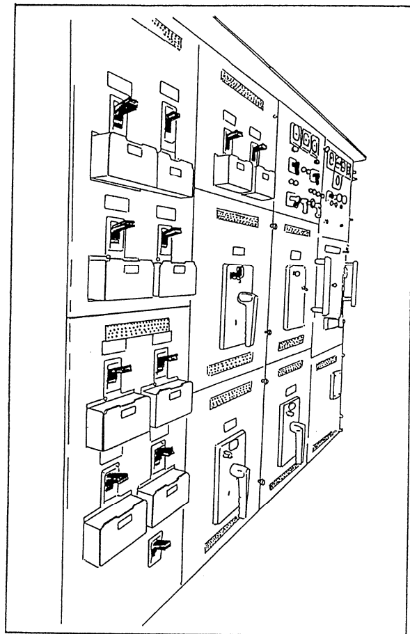
Figure 5-29.—Dead front of a ship's service switchboard.
