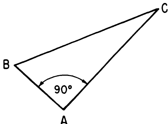
Figure 19-3.—Using the Pythagorean Theorem.
