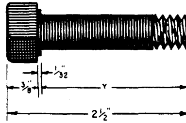
Figure 4-6.—Finding unknown dimensions by subtracting fractions.
