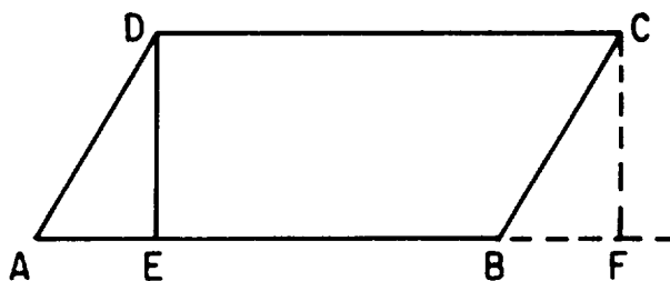
Figure 17-14.—A parallelogram.
