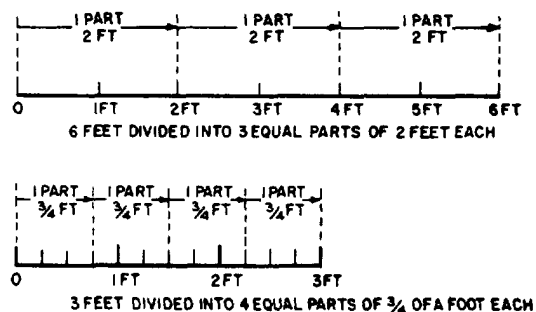
Figure 4-3.—Partitive fractions
