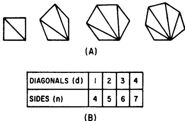
Figure 14-3.—Diagonals of plane figures.
