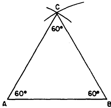
Figure 18-7.—Constructing 60^\circ angles.
