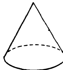
Figure 18-17.—Right circular cone.
