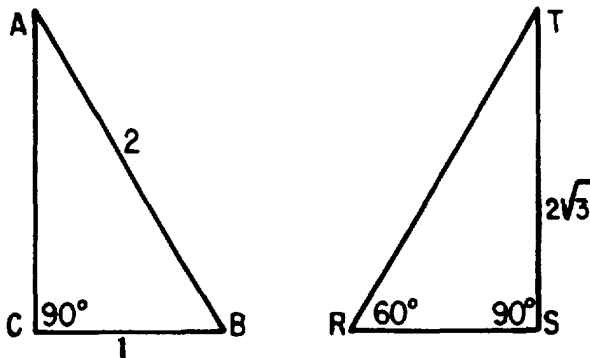
Figure 19-11.—Finding parts of 30^\circ - 60^\circ - 90^\circ triangles.
