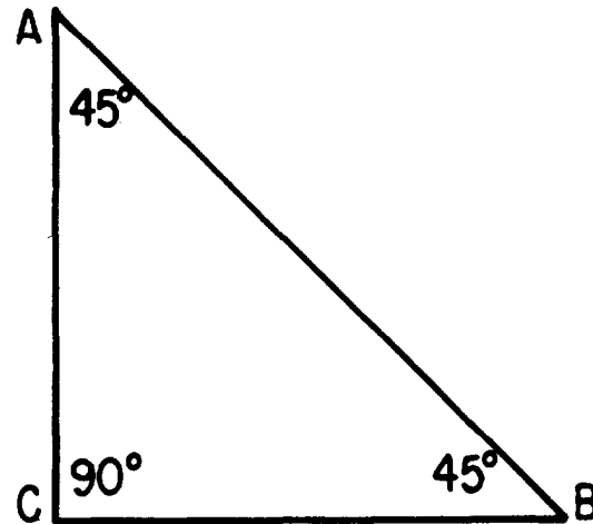
Figure 19-12.—A 45^\circ - 90^\circ triangle.
