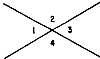
Figure 17-6.—Vertical angles.
