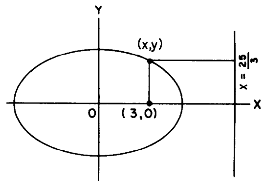
Figure 2-4.—Ellipse.
