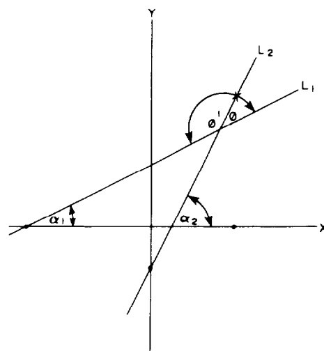
Figure 1-7.—Angle between two lines.
