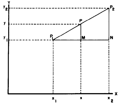
Figure 1-3.—Division of a line segment.
