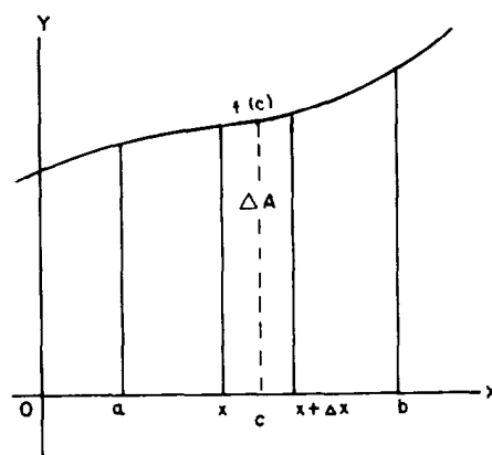
Figure 6-5.—Increments of area at f(c) .
