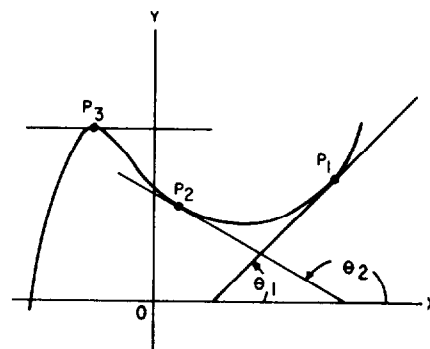
Figure 3-3.—Curve with tangent lines.
