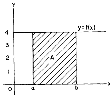
Figure 6-1.—Area of a rectangle.
