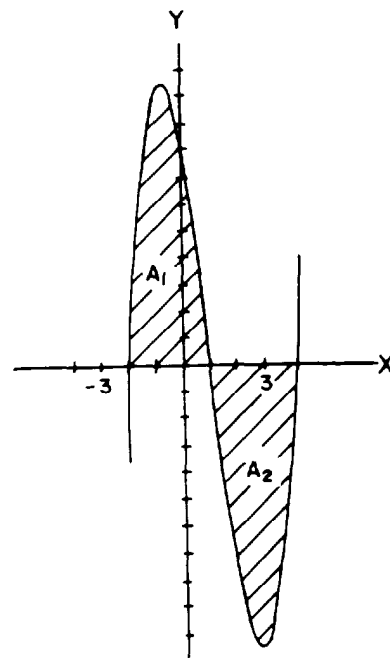
Figure 6-14.—Positive and negative value areas.
