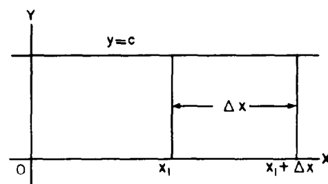
Figure 5-1.—Graph of y = c , where c is a constant.
