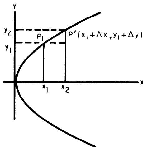
Figure 3-4.—Parabola.
