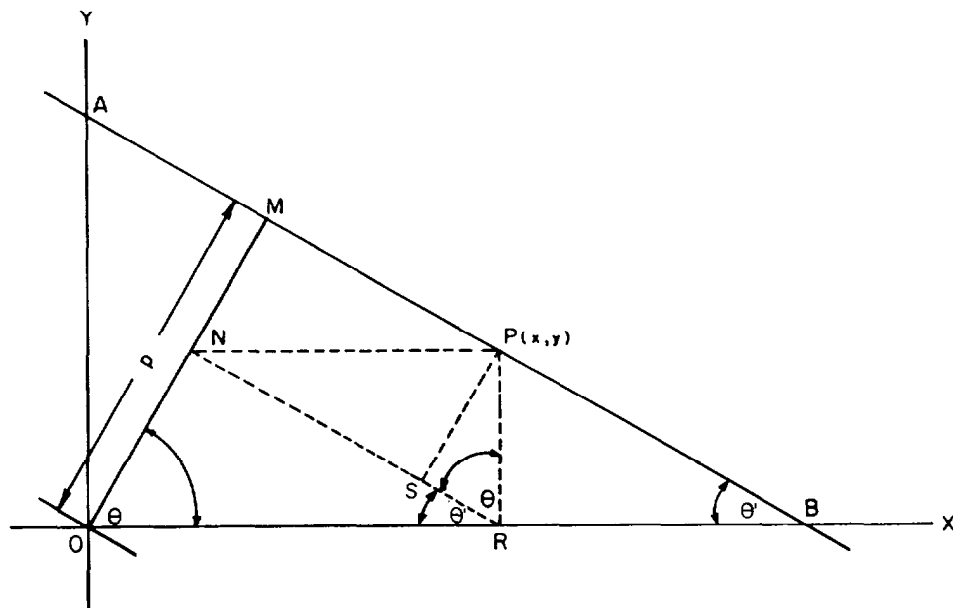
Figure 1-9.—Normal form.
