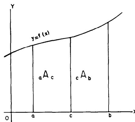
Figure 6-4.—Designation of limits.
