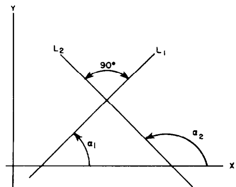
Figure 1-5.—Slopes of perpendicular lines.
