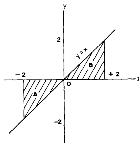
Figure 6-13.—Negative and positive value areas.
