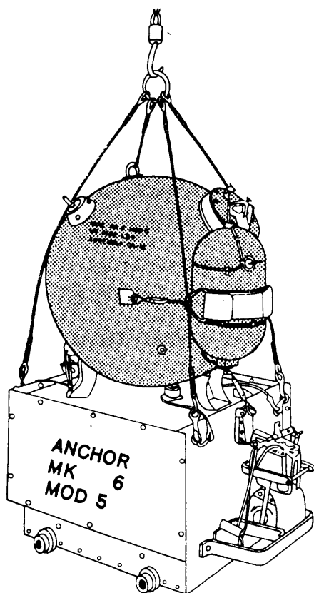
Figure 1-2.—Mk 6 mine.
