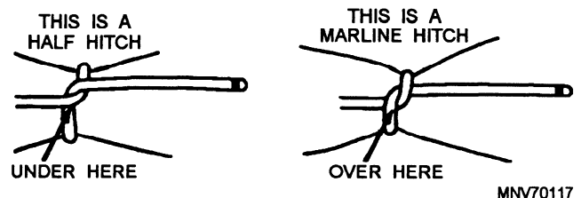
Figure 4-21.—Difference between a marline hitch and a half hitch.
