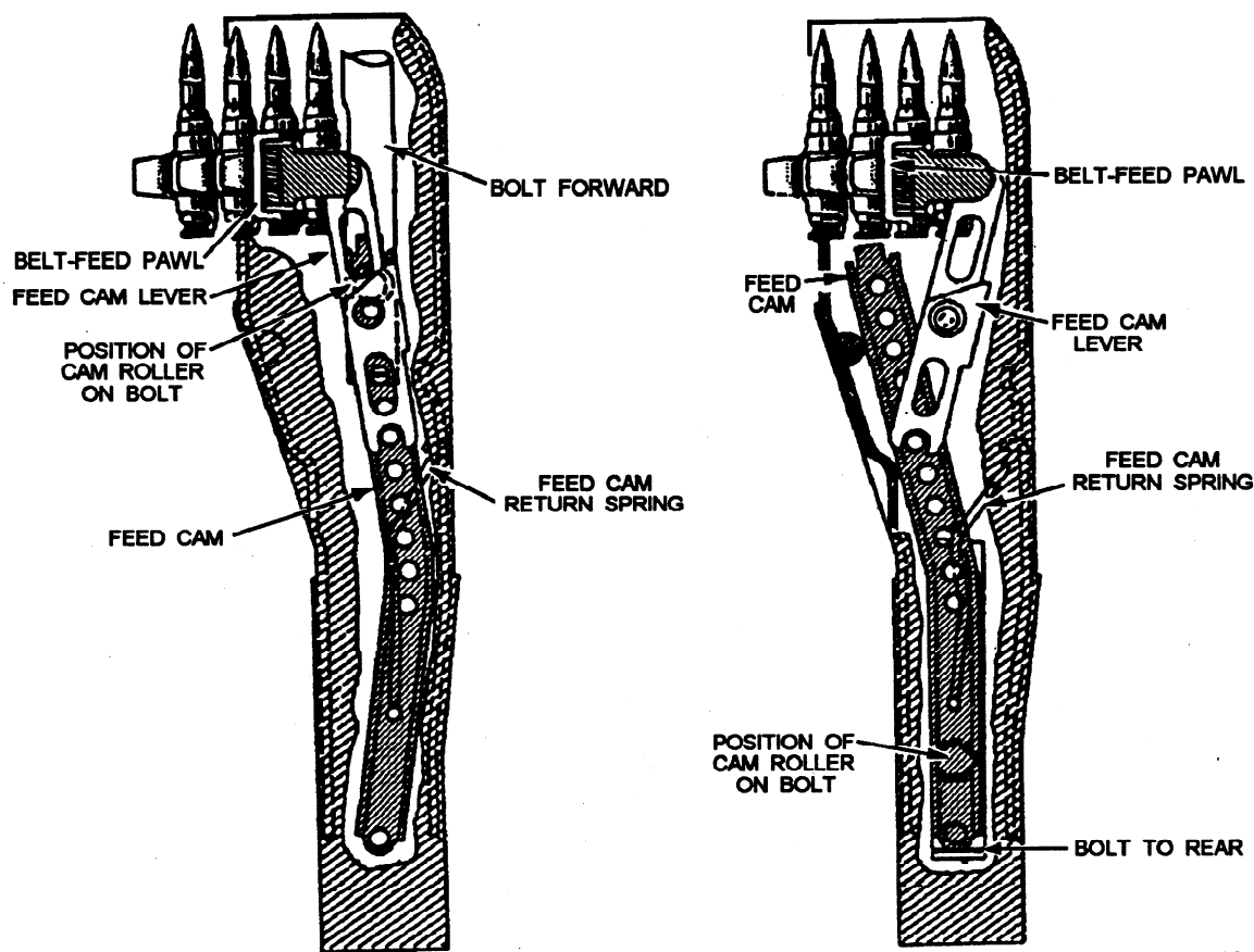
Figure 2-47.—Feeding.
