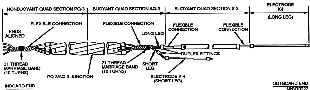
Figure 10-1.—Magnetic quadrad tail assembly.
