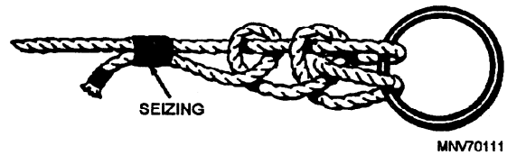
Figure 4-15.—Fisherman's bend.
