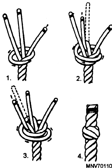
Figure 4-14.—Tying a double Matthew Walker.
