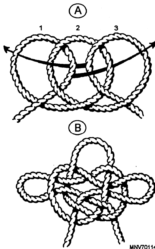
Figure 4-18.—Masthead knot.
