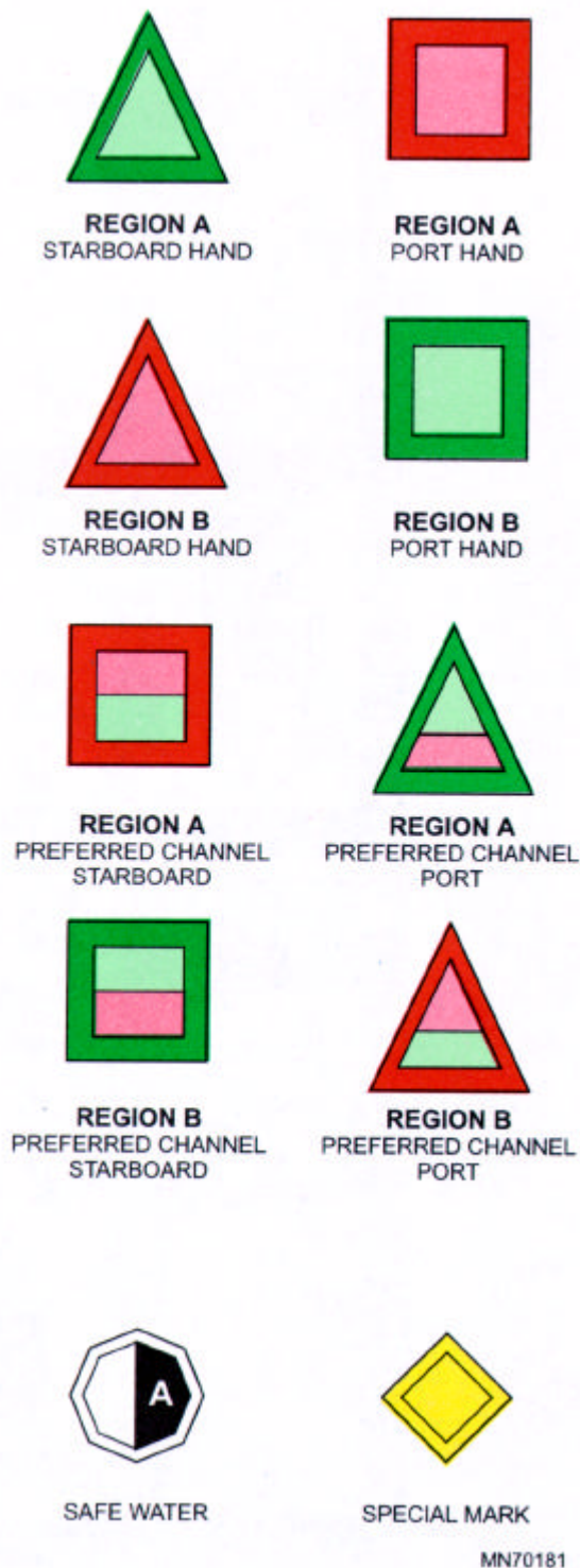
Figure 6-27.—IALA Maritime Buoyage System, lateral daymark
