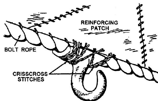
Figure 5-19.—Awning hooks.
