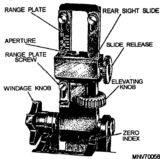
Figure 2-45.—M60 rear sight.
