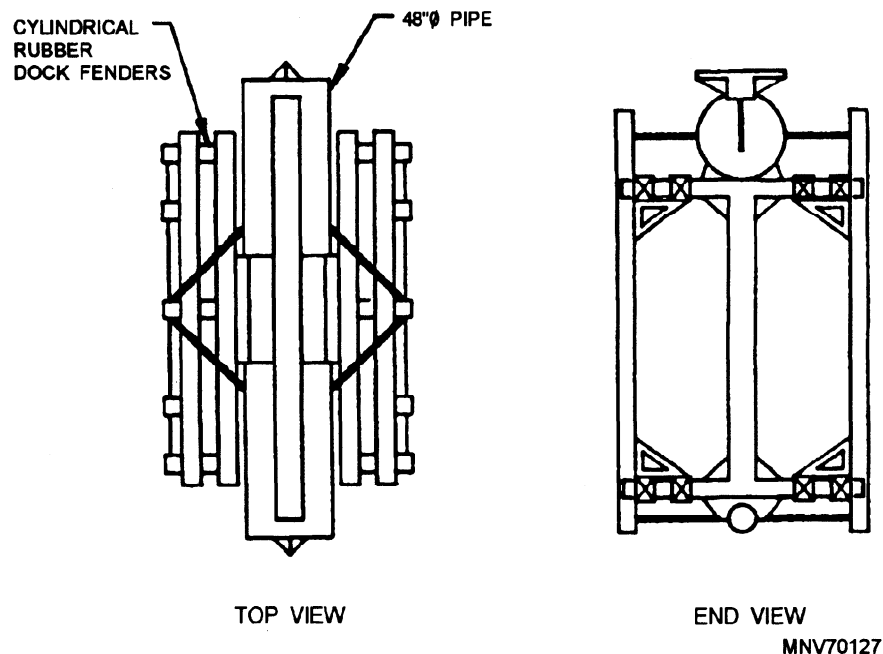
Figure 5-3.—Camels.
