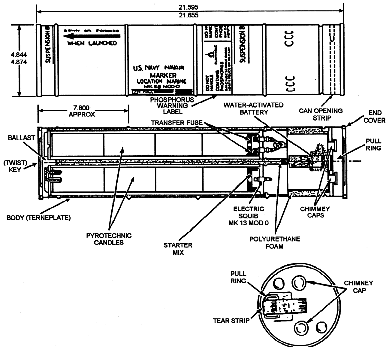
Figure 3-1.—The Mk 58 Mod 0 marine location marker.
