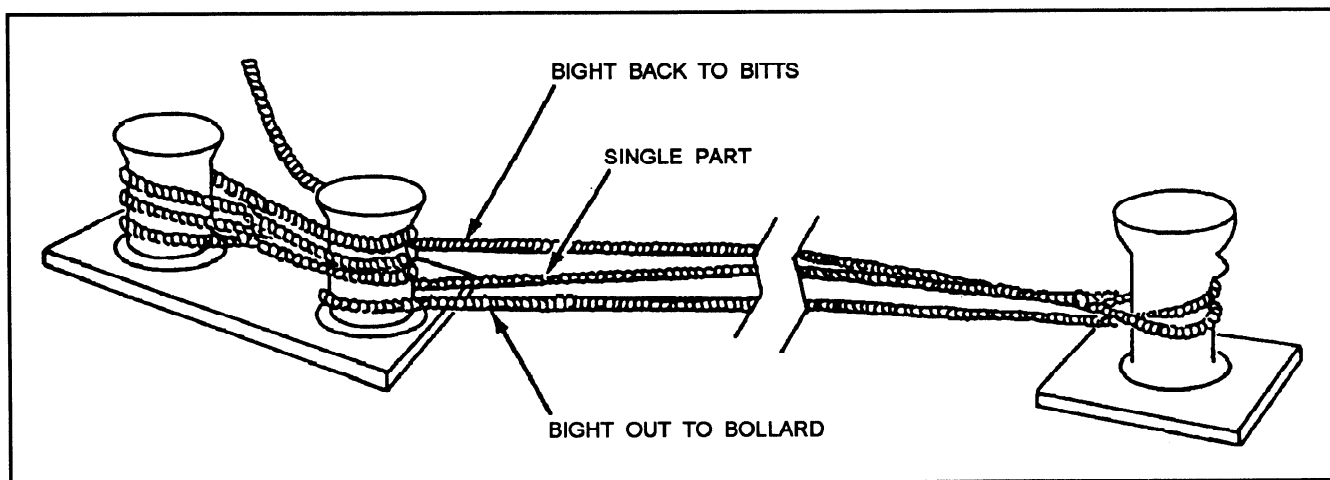
Figure 4-11.—Correct method of doubling up.
