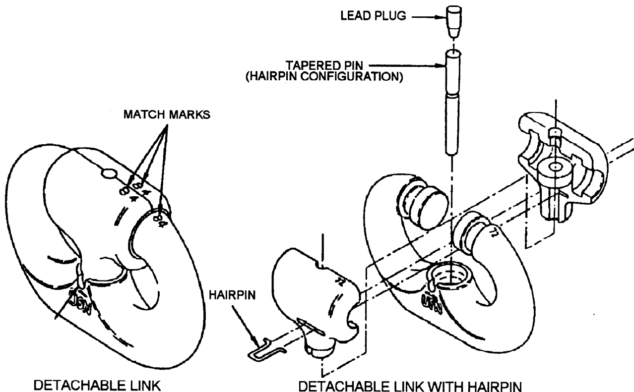
Figure 7-2.—Detachable link.
