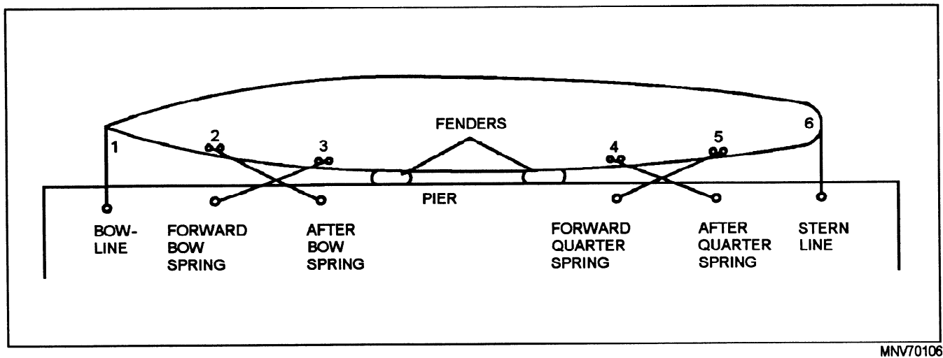
Figure 4-10.—Mooring lines of a ship.
