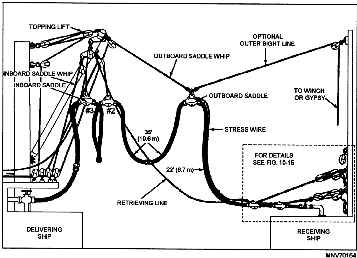
Figure 5-30.—Close-in rig.
