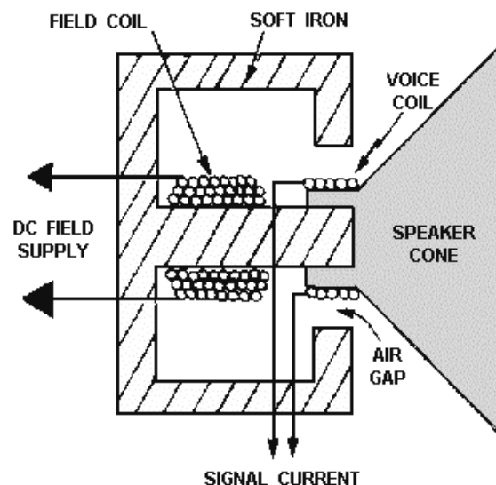
Figure 2-31.—Electromagnetic speaker.
