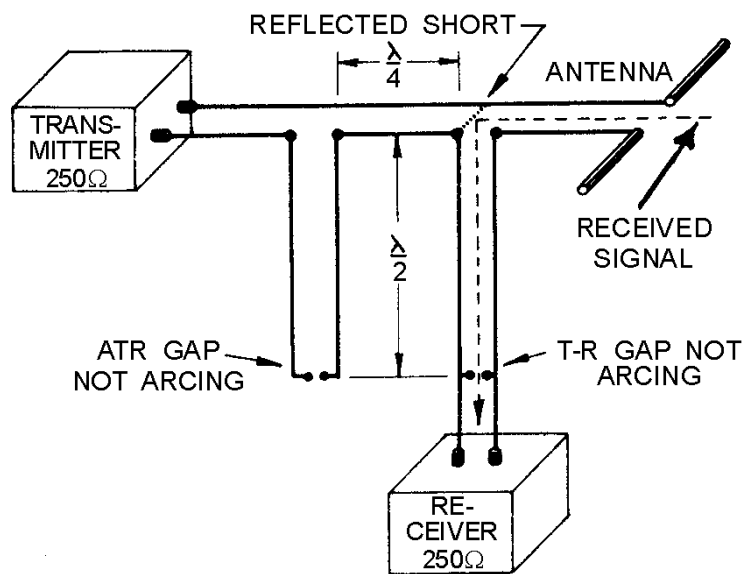
Figure 2-19.—Series-connected duplexer during reception.
