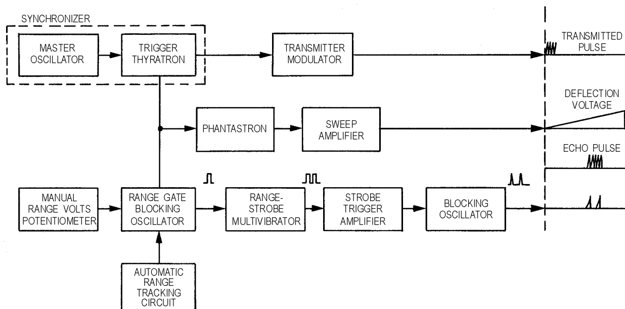
Figure 3-11.—Range-gate generator.
