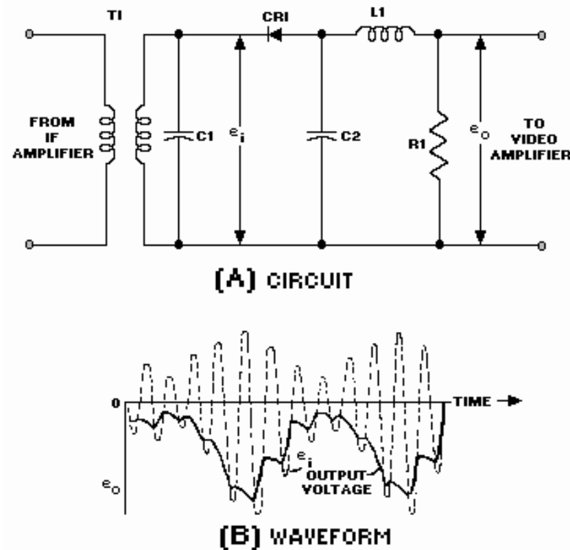
Figure 2-28.—Diode detector.
