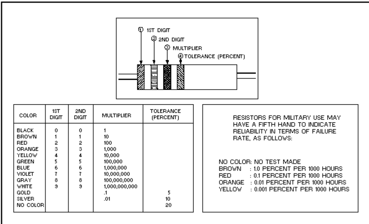
Figure 1-18.—Resistor color code.
