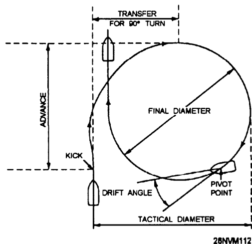
Figure 11-5. Turning circle.
