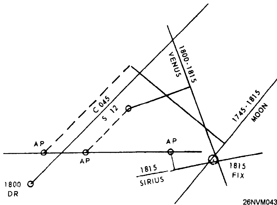
Figure 9-14. A fix from several LOPs.
