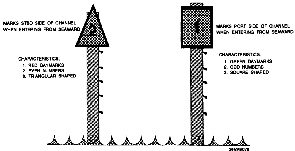
Figure 4-7. Daymarks.
