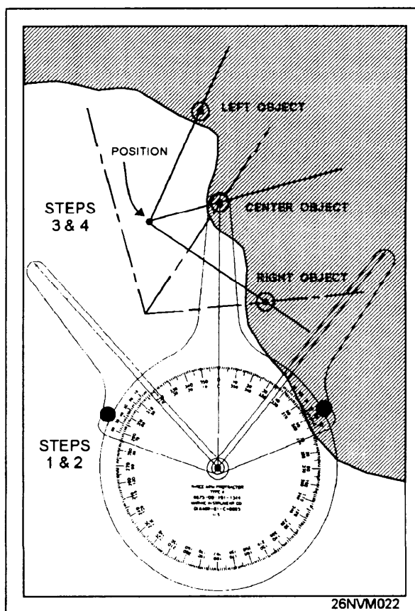
Figure 8-24. Aligning the three-arm protractor.
