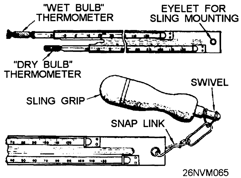
Figure 10-12. Sling psychrometer.
