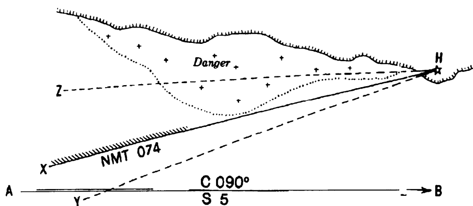
Figure 12-6. Example of a danger bearing.
