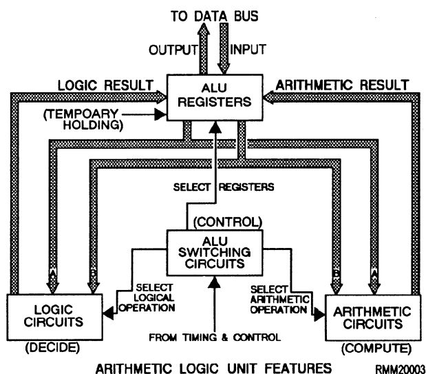
Figure 1-2.—Representative block diagram of an ALU.
