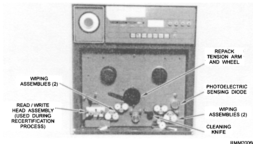
Figure 2-12.—Tape cleaner/certifier.
