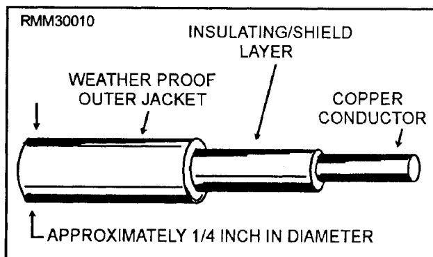
Figure 1-10.—Coaxial cable,
