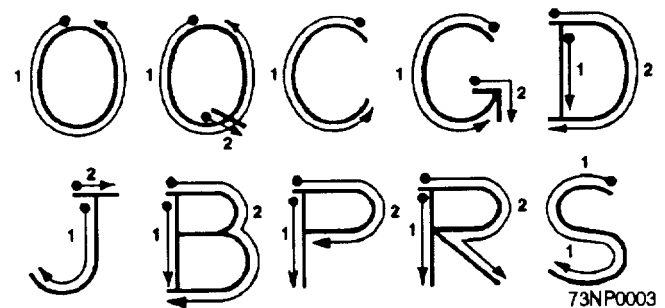
Figure 1-3.—Circular lettering.
