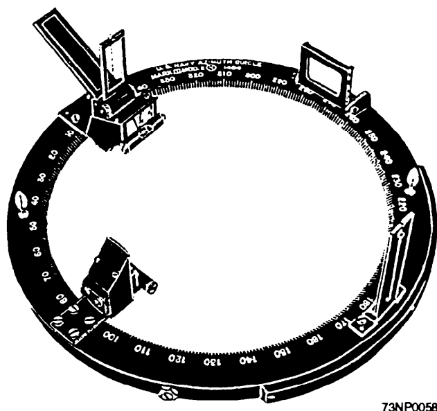
Figure 9-1.—Azimuth circle.
