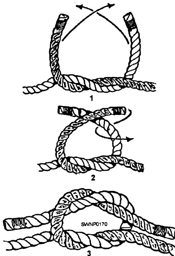
Figure 4-11.—Square knot.
