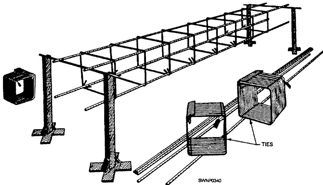
Figure 7-25.—Column assembly.
