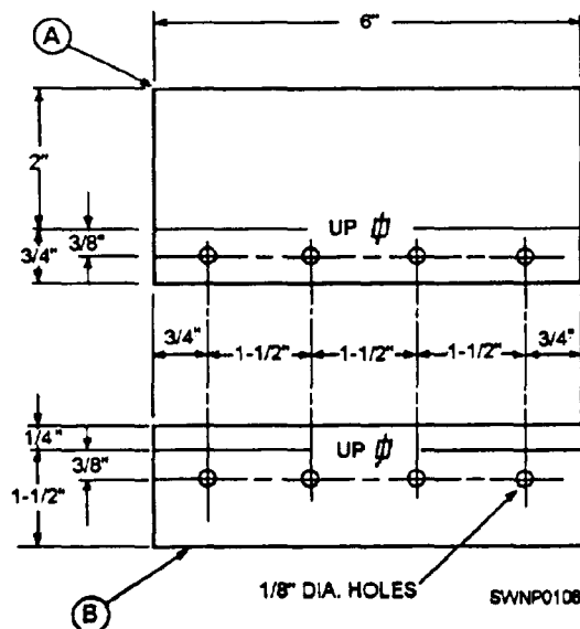
Figure 2-91.—Riveted seam for tapped and riveted corner seam.
