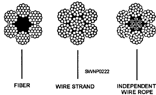
Figure 5-3.—Core construction.
