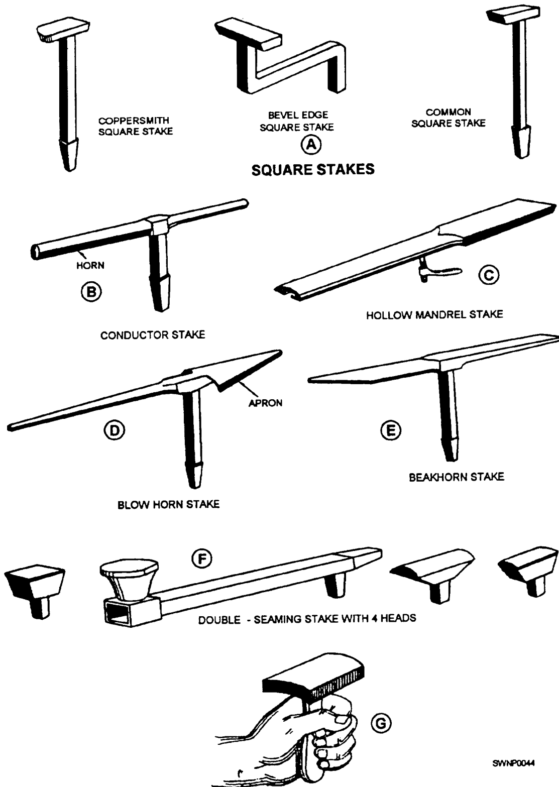
Figure 2-27.—Metal stakes
