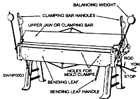
Figure 2-36.—Cornice brake.
