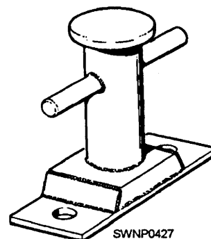
Figure 10-17.—B1 all-purpose bitt.
