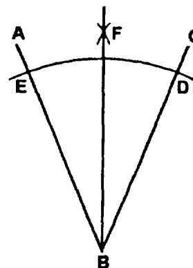
Figure 2-11.—Bisecting an arc.
