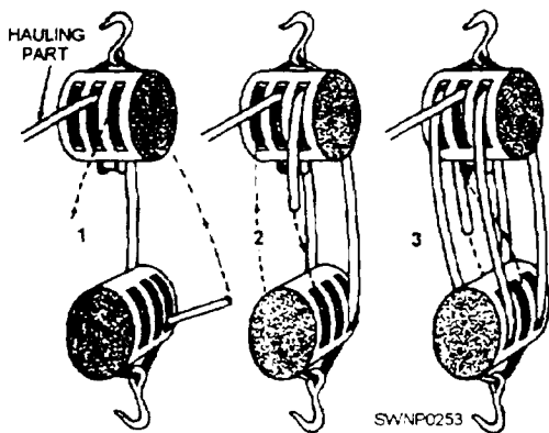
Figure 6-6.—Reeving two 3-sheave blocks.
