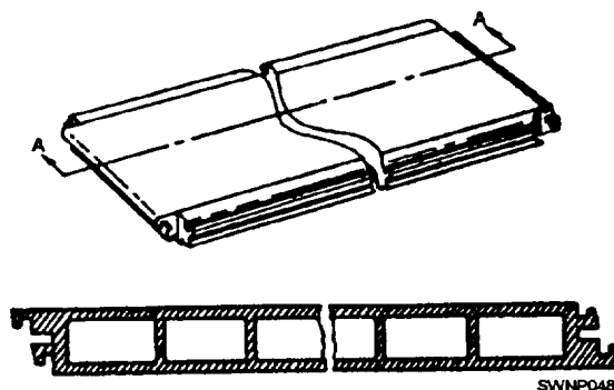
Figure 11-37.—Heavy-duty mat.
