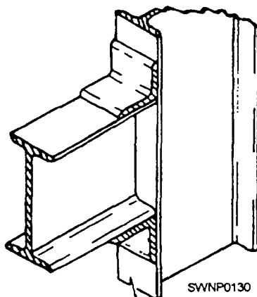
Figure 3-37.—Seated connection.
