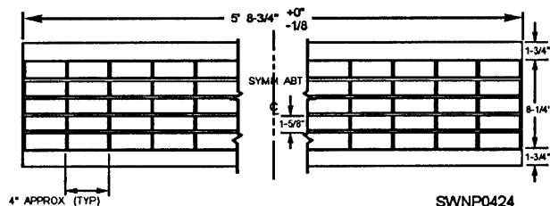
Figure 10-14.—DC6 deck closure.
