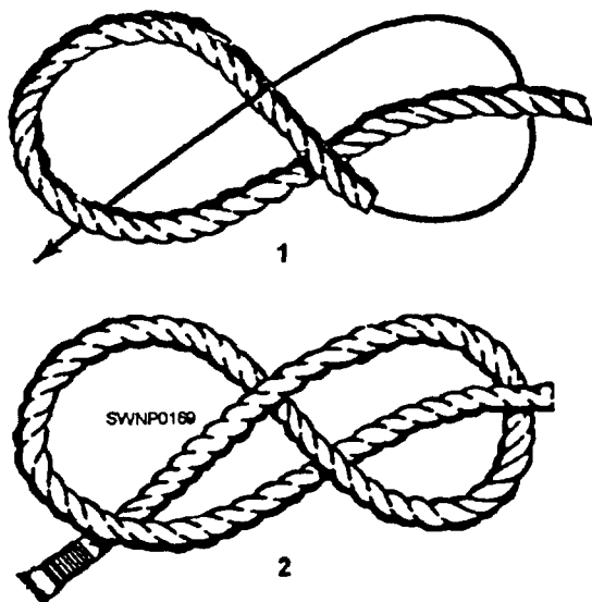
Figure 4-10.—Figure-eight knot
