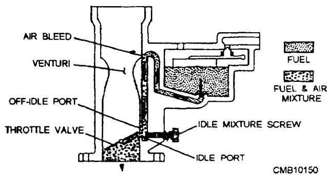
Figure 4-21.—Idle system.
