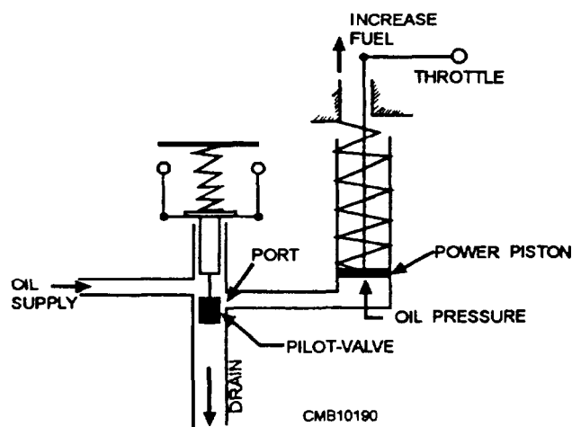
Figure 5-7.—Hydraulic governor.
