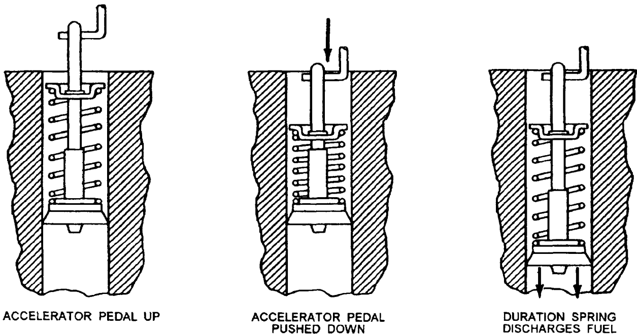
Figure 4-24.—Duration spring.
