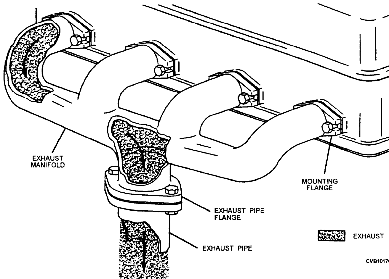
Figure 4-47.—Exhaust manifold.
