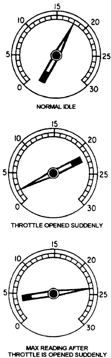
Figure 3-77.—Approximate vacuum gauge readings on a normal operating engine.
