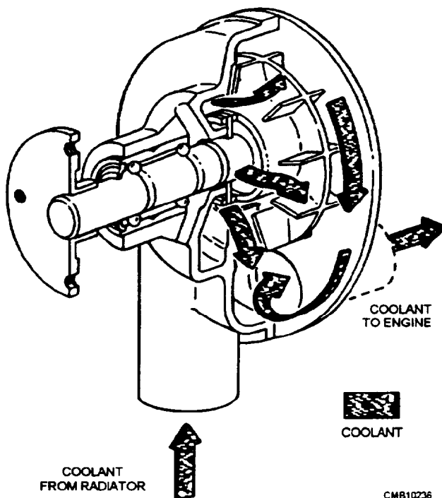
Figure 6-8.—Water pump operation.
