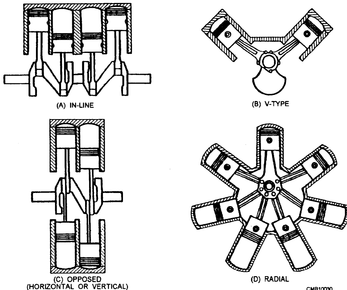
Figure 2-10.—Typical cylinder arrangements
