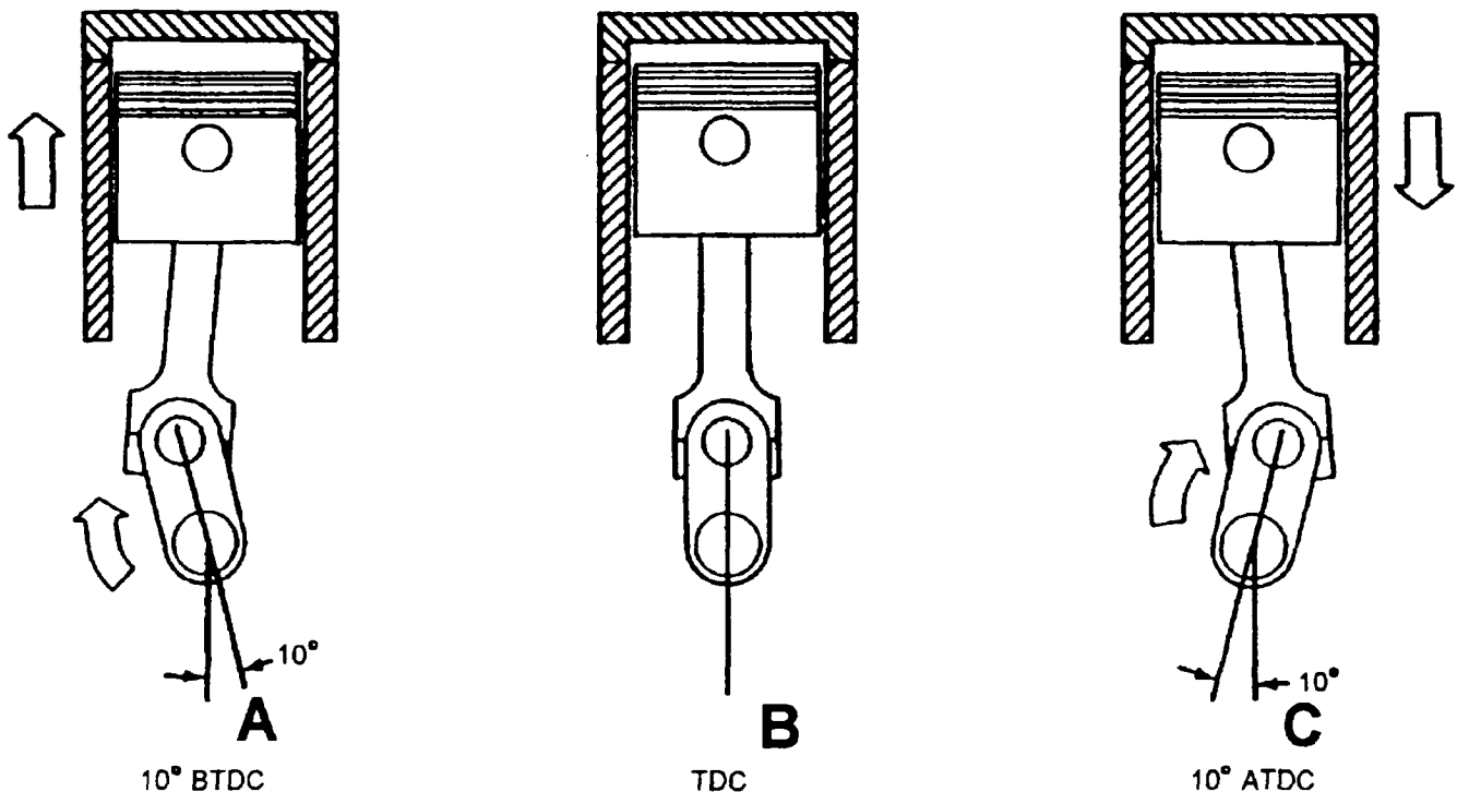
Figure 2-31.—Ignition timing.
