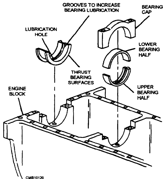
Figure 3-69.—Crankshaft main bearings.
