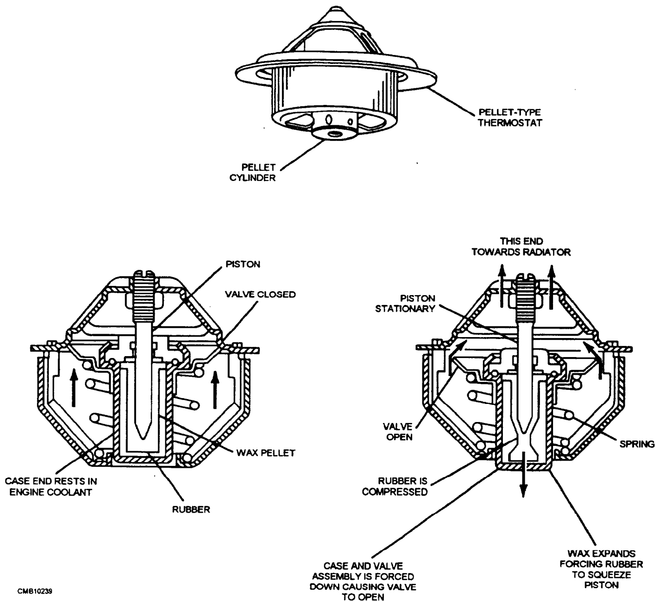
Figure 6-11.—Pellet-type thermostat.
