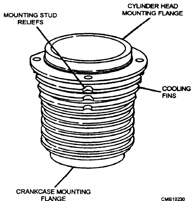
Figure 6-2.—Air-cooled cylinder.
