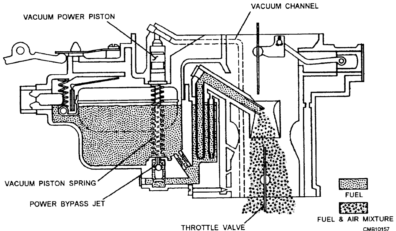
Figure 4-28.—Vacuum power jet.
