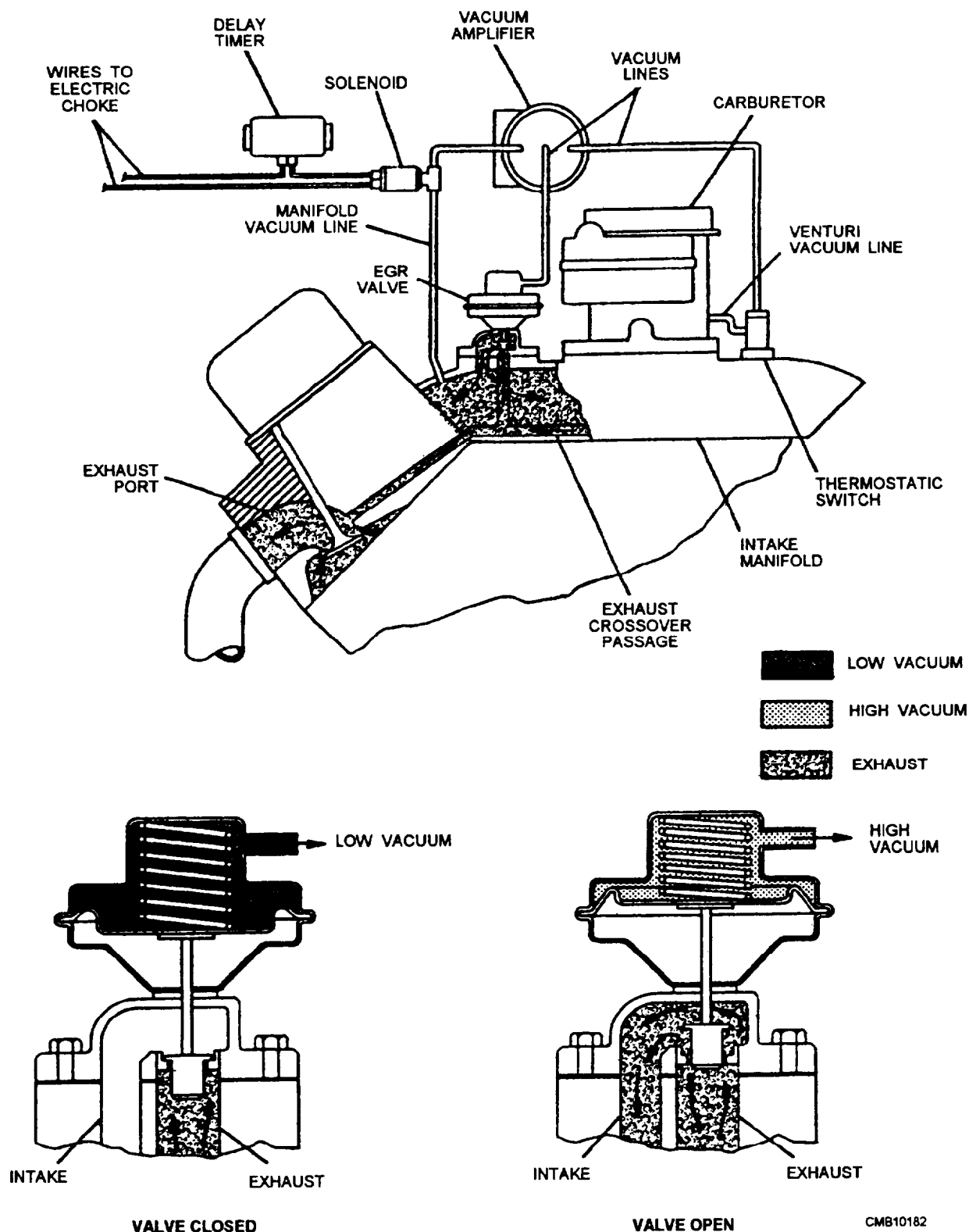
Figure 4-53.—EGR system.
