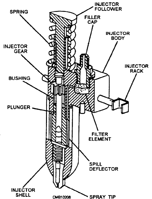
Figure 5-25.—Unit injector.
