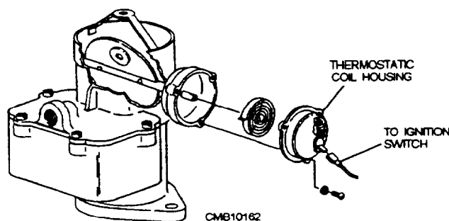
Figure 4-33.—Electric choke.
