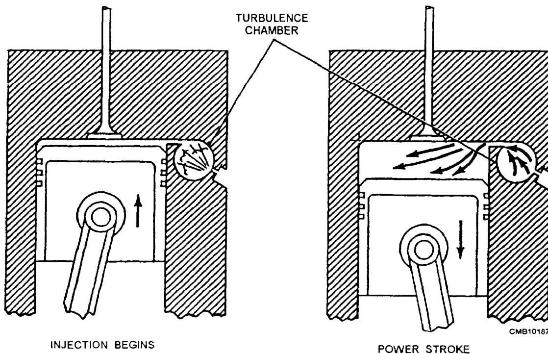
Figure 5-4.—Turbulence chamber.
