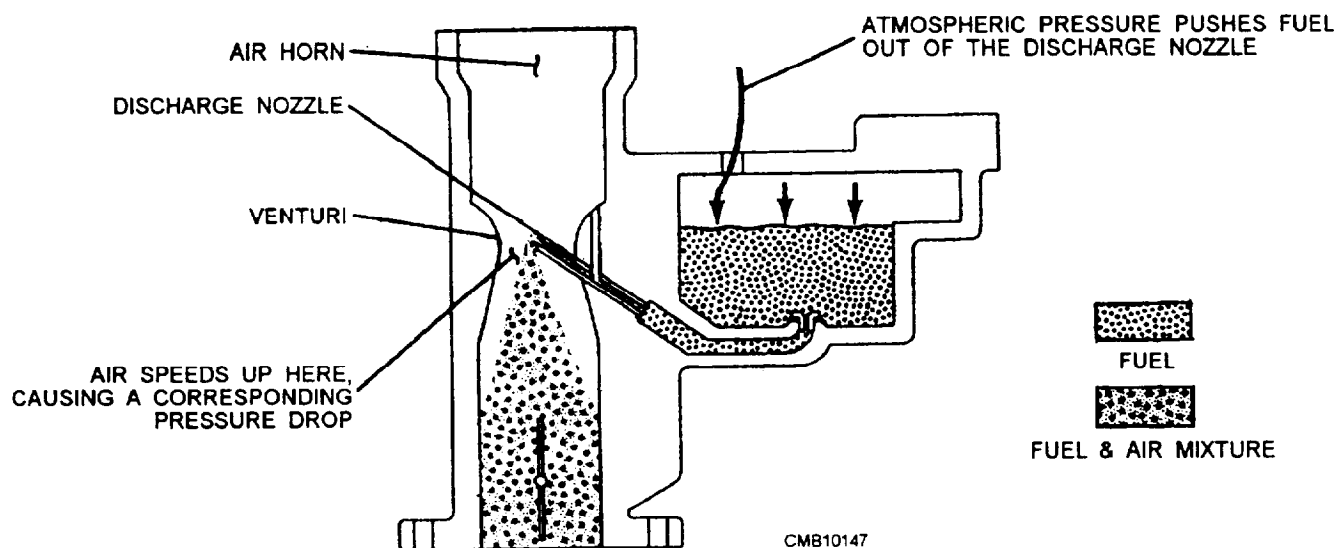
Figure 4-18.—Venturi effect.
