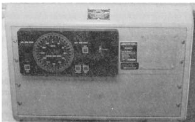
Figure 2-25.—ID-2447/U wind speed and direction indicator.
