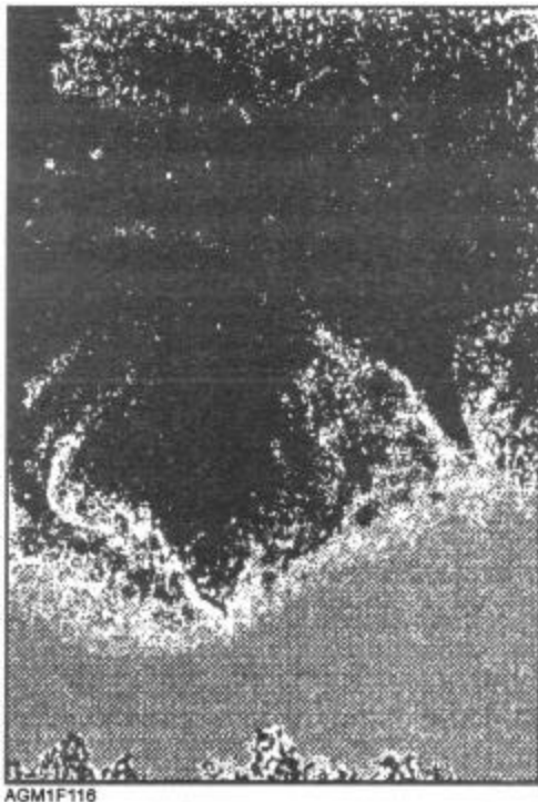
Figure 1-16.—Funnel clouds.
