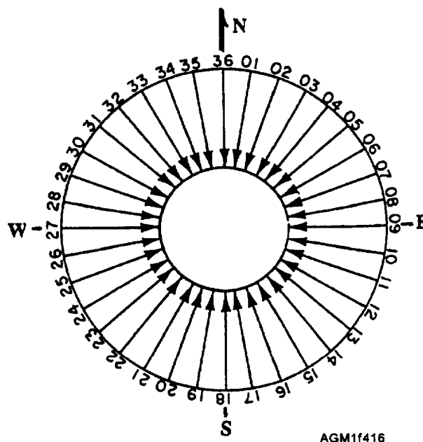
Figure 4-16.—Wind direction in true degrees indicated by the orientation of the wind shaft from the station circle or station location.
