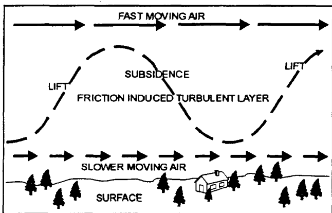
Figure 1-4.—Turbulent lift.
