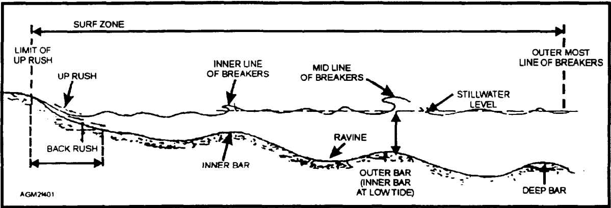
Figure 4-1.—Nearshore profile.
