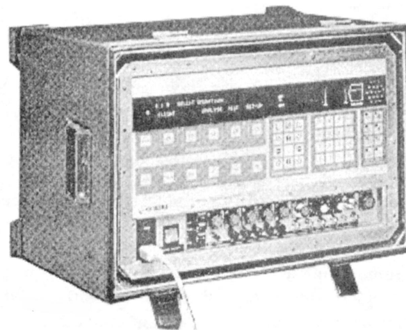
Figure 1-2.— AN/UMQ-12 MRS data receiver/processor and case.
