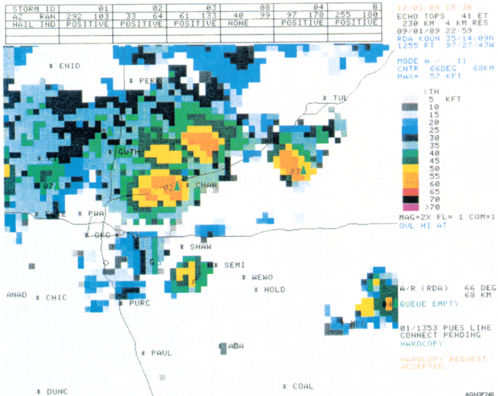
Figure 2-40.—Echo Tops (ET) product.
