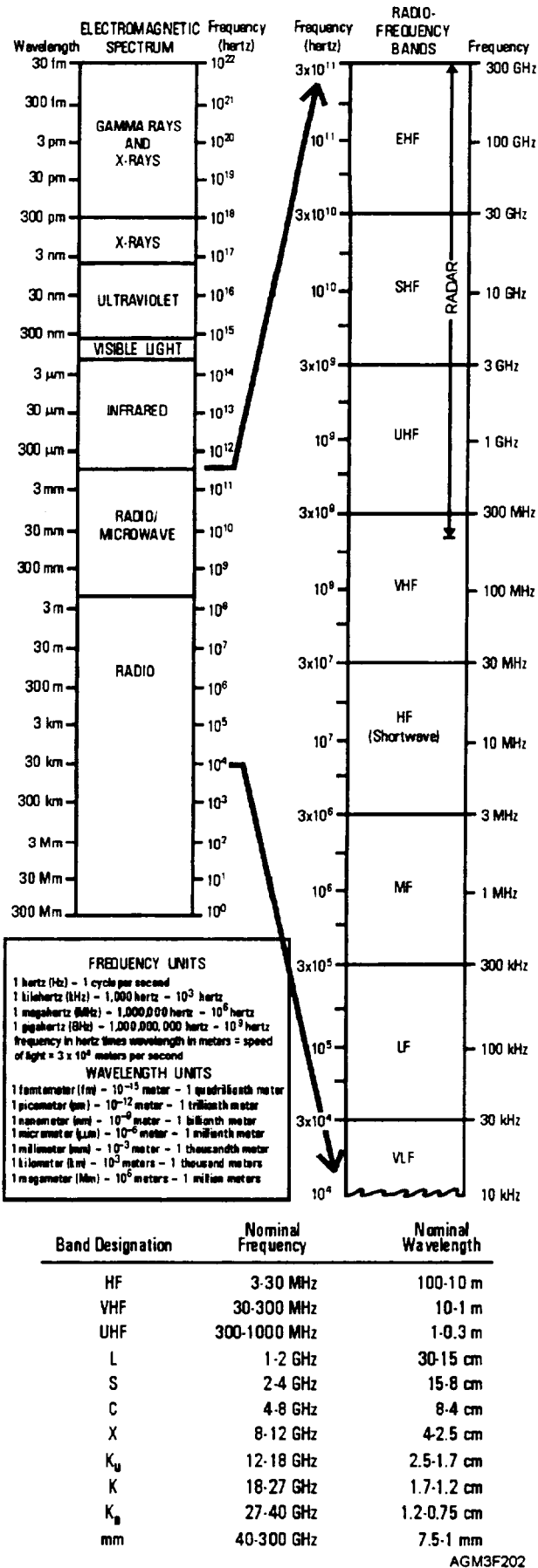
Figure 2-2.—The electromagnetic spectrum.
