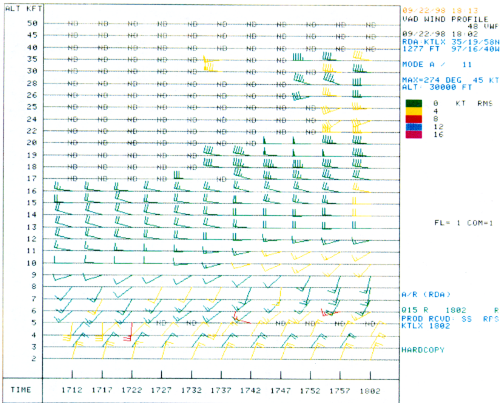
Figure 2-39.—VAD Wind Profile (VWP) product.
