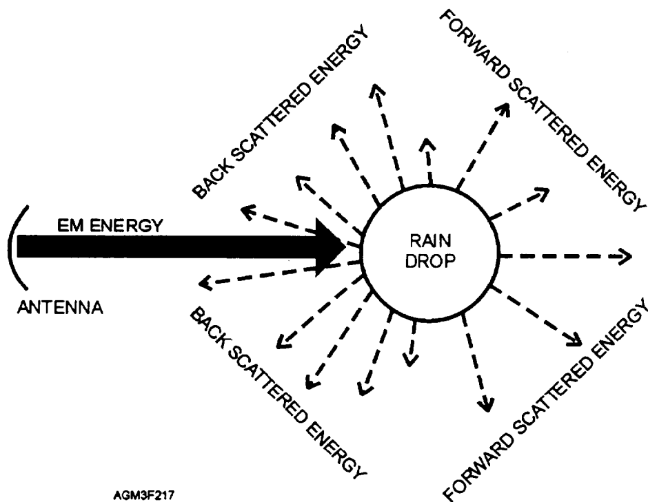
Figure 2-17.—Scattering of radar energy.
