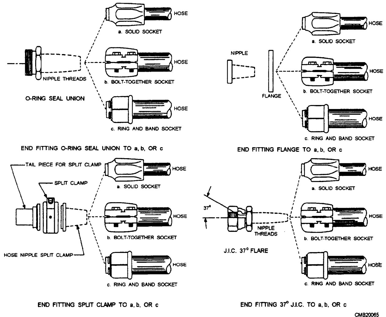
Figure 3-43.—End fittings and hose fittings.
