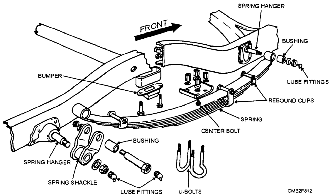
Figure 8-12.—Multileaf spring.
