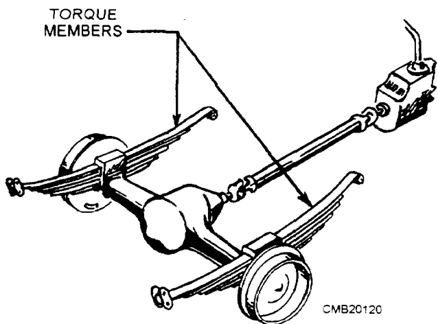
Figure 5-2.—Hotchkiss drive.
