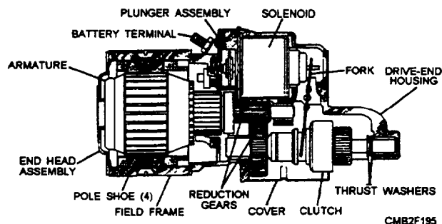
Figure 2-42.—Gear reduction starter.
