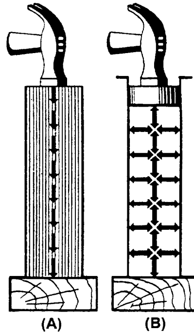
Figure 3-2.—Transmission of force: (A) Solid; (B) Fluid.
