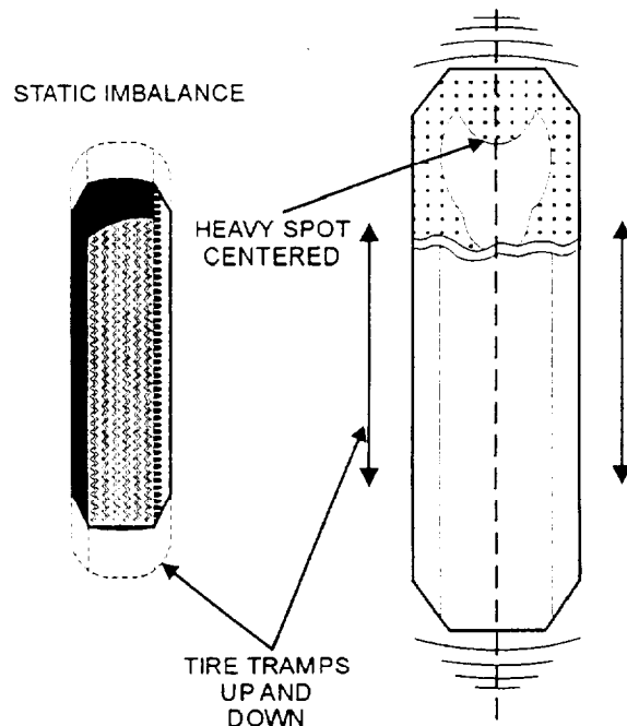
Figure 8-43.—Static imbalance.
