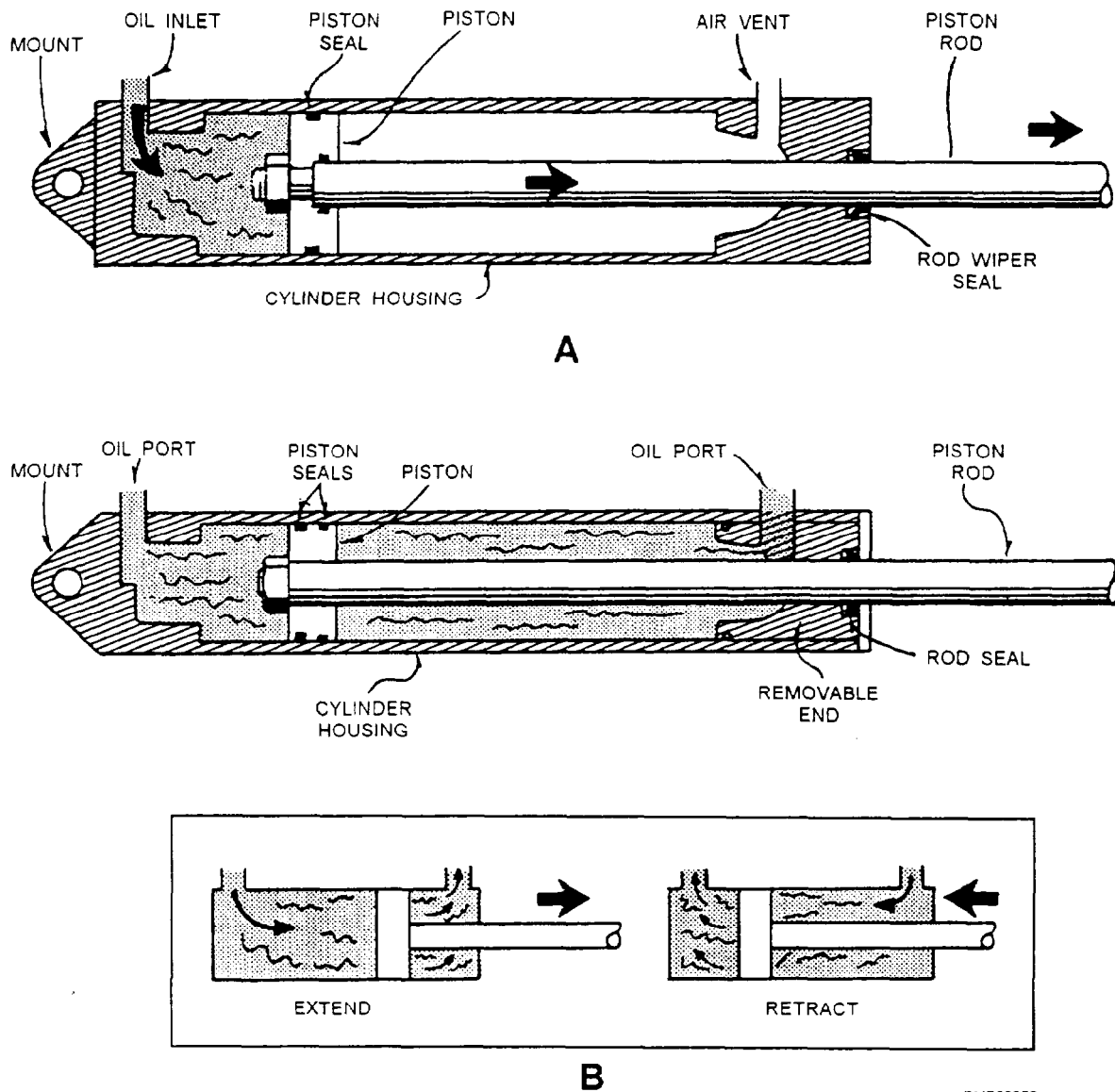
Figure 3-30.—(A) Single- and (B) double-acting piston-type cylinders.
