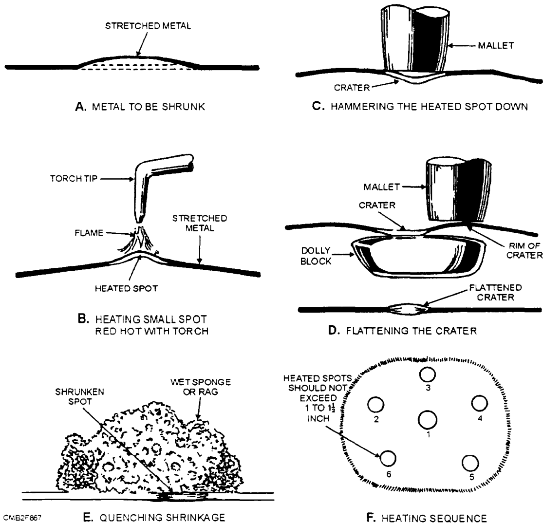
Figure 8-67.—Metal shrinking process and sequence used for large areas.
