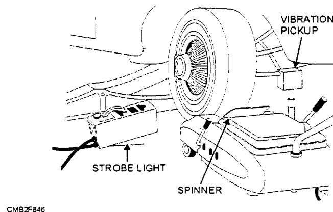
Figure 8-46.—On-the-vehicle balancer.
