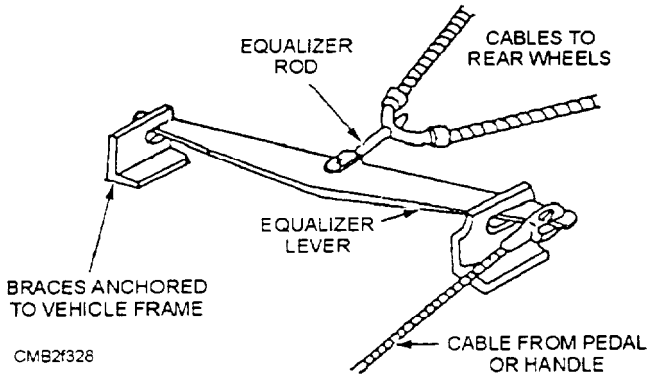
Figure 7-27.—Equalizer linkage.
