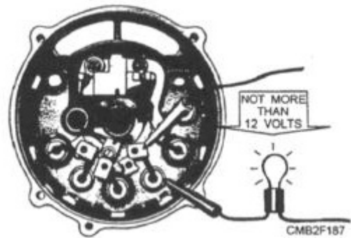
Figure 2-34.—Testing diodes with a test lamp.
