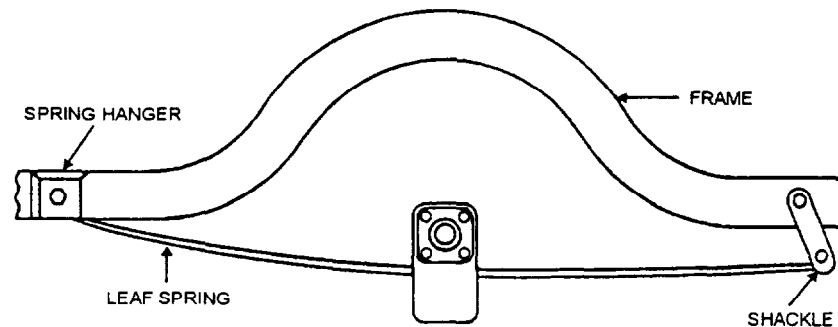
A. SINGLE LEAF SPRING
