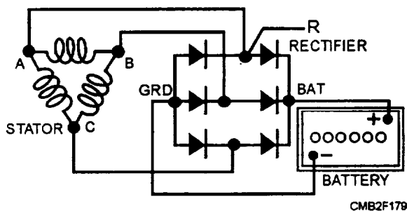
Figure 2-26.—Electrical diagram indicating a delta-type stator.
