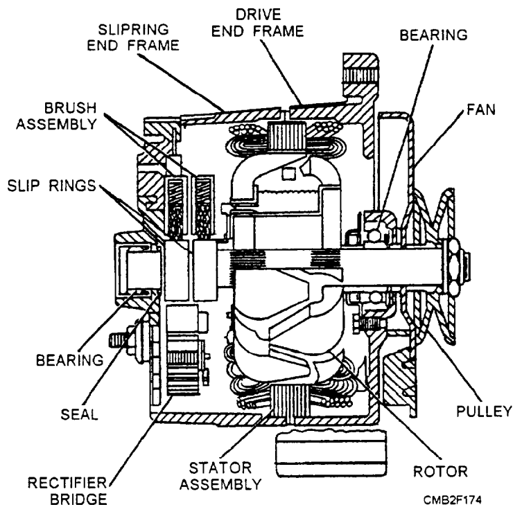
Figure 2-21.—Typical alternator.
