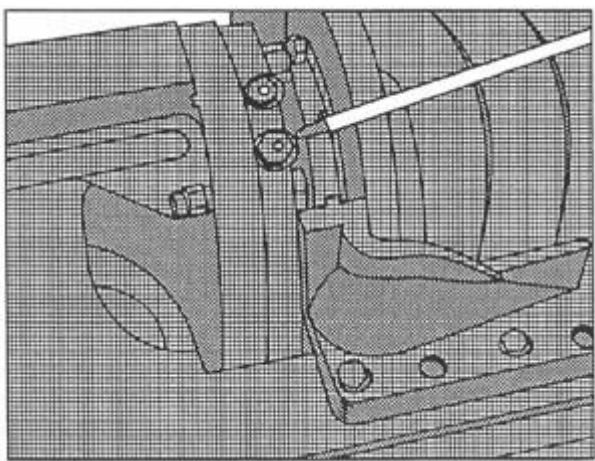
Figure 6-27.—Hydraulic track adjuster.
