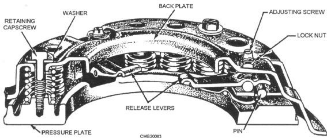
Figure 4-6.—Coil spring pressure plate.
