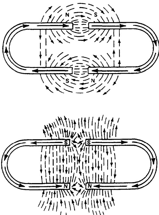
Figure 1-18.—Electromagnetism.
