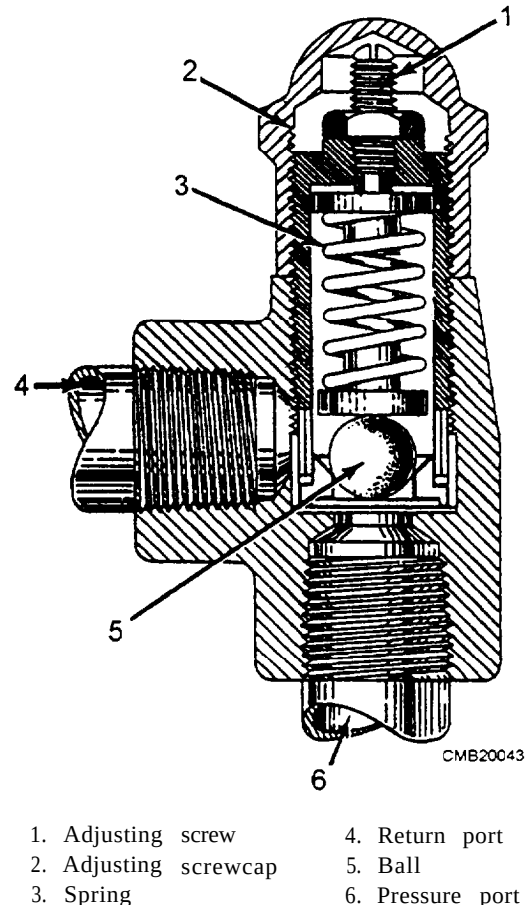
Figure 3-21.—Typical relief valve.
