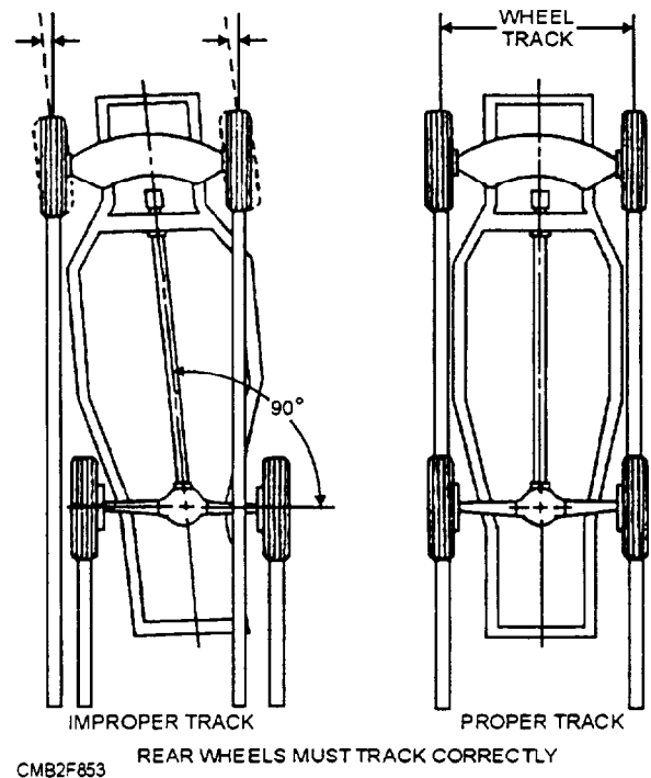
Figure 8-53.—Tracking.
