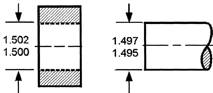
Figure 3-39. —The basic hole system.
