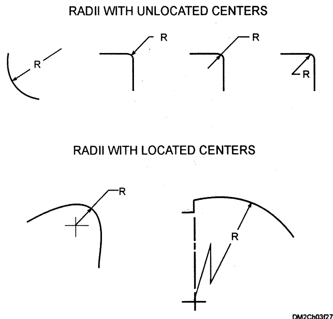
Figure 3-27. —Dimensioning radii.
