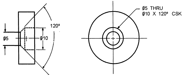
COUNTERSUNK HOLES
