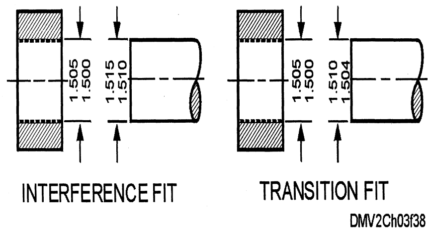
Figure 3-38. —The difference between: A. An interference fit, and B. A transition fit.
