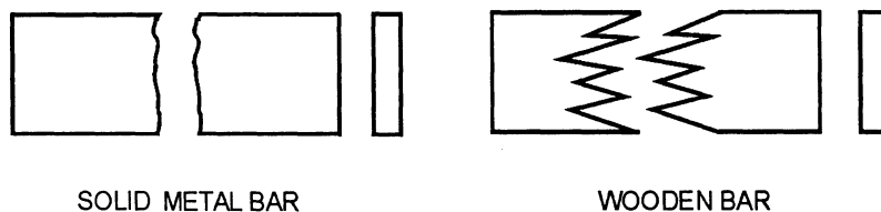
Figure 3-18. —Conventional breaks.
