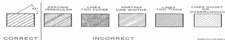
Figure 3-64. —Correct and incorrect section linings.
