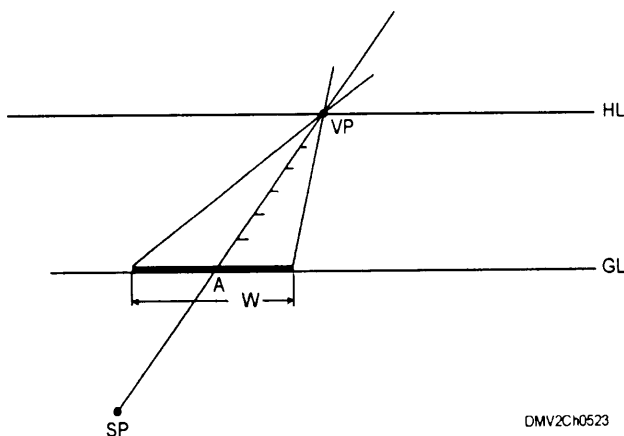
Figure 5-23. —Projecting horizontal points.
