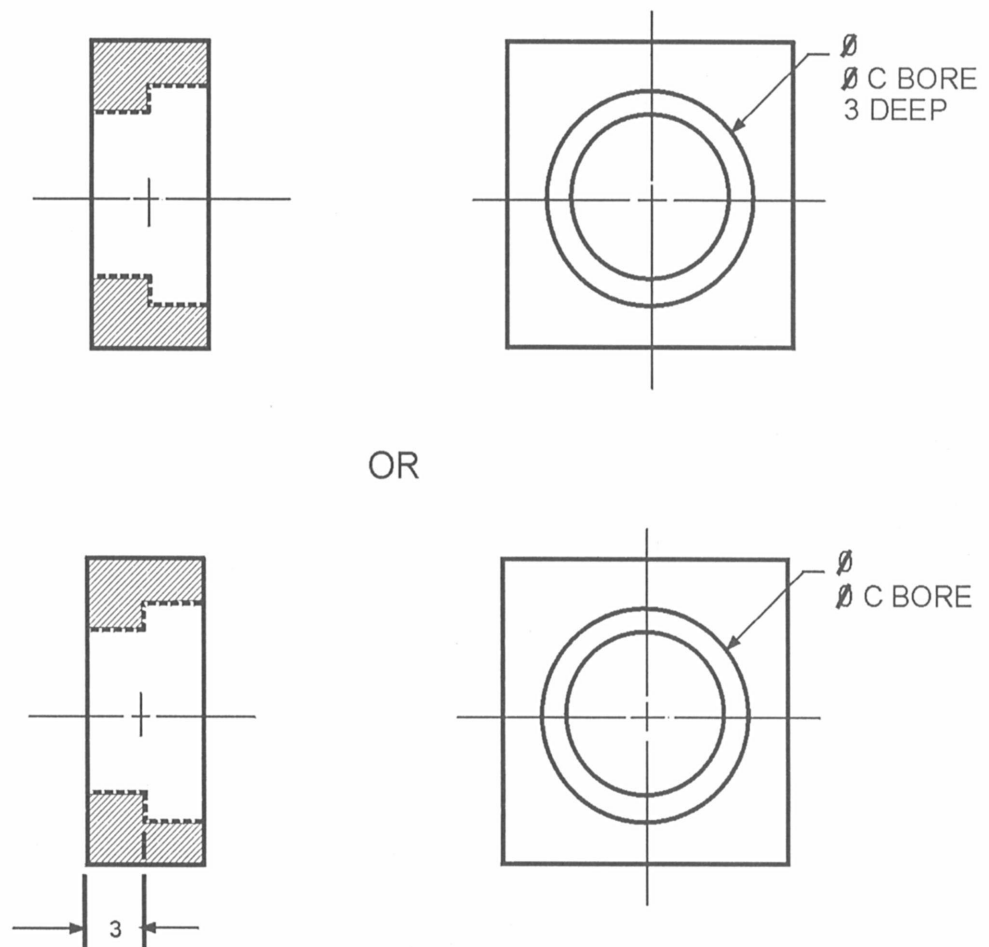
Figure 3-32. —Counterbore dimensions.
