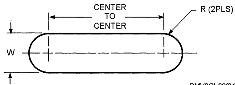
Figure 3-31. —Dimensioning slotted holes.
