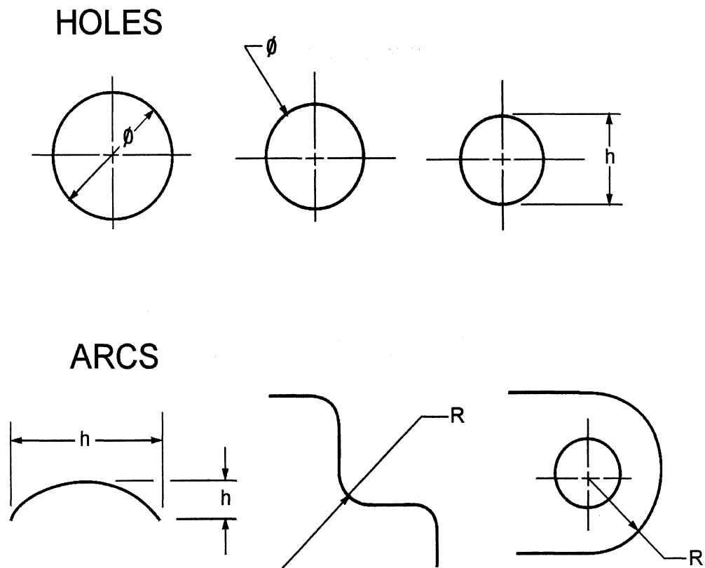
Figure 3-15. —Dimensioning arcs and circles.
