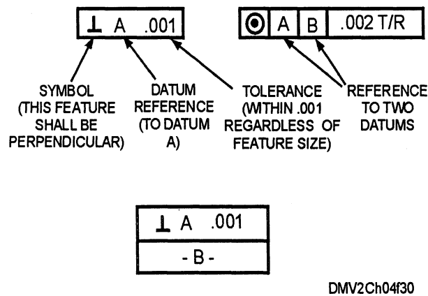
Figure 4-30. —Feature control frame indicating a datum reference.
