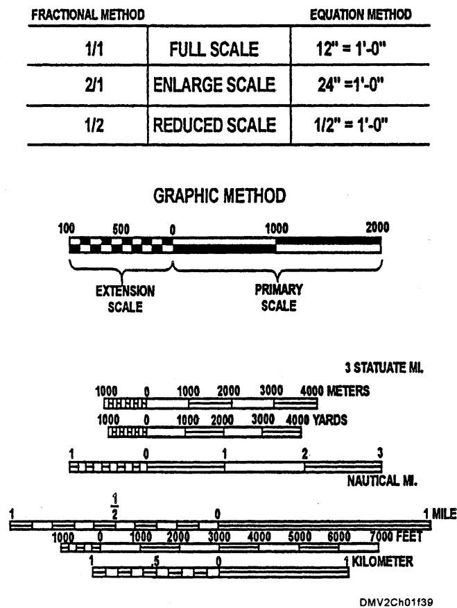
Figure 1-39.—Indicating scale.
