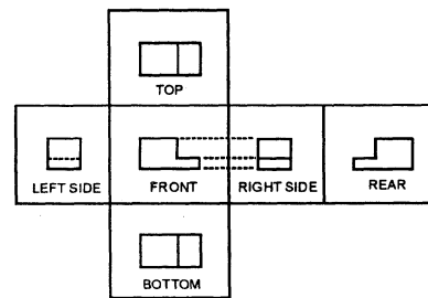
Figure 3-41. —View arrangement.
