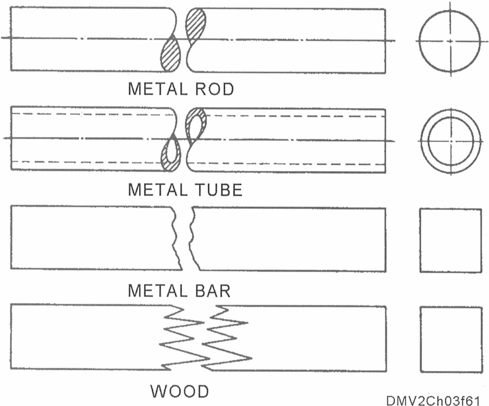
Figure 3-61. —Conventional break lines.
