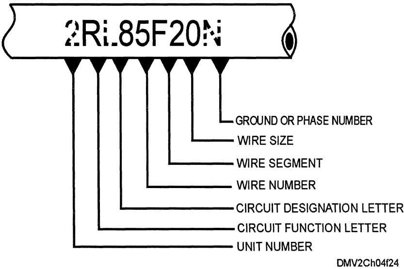
Figure 4-24. —Aircraft wire identification.
