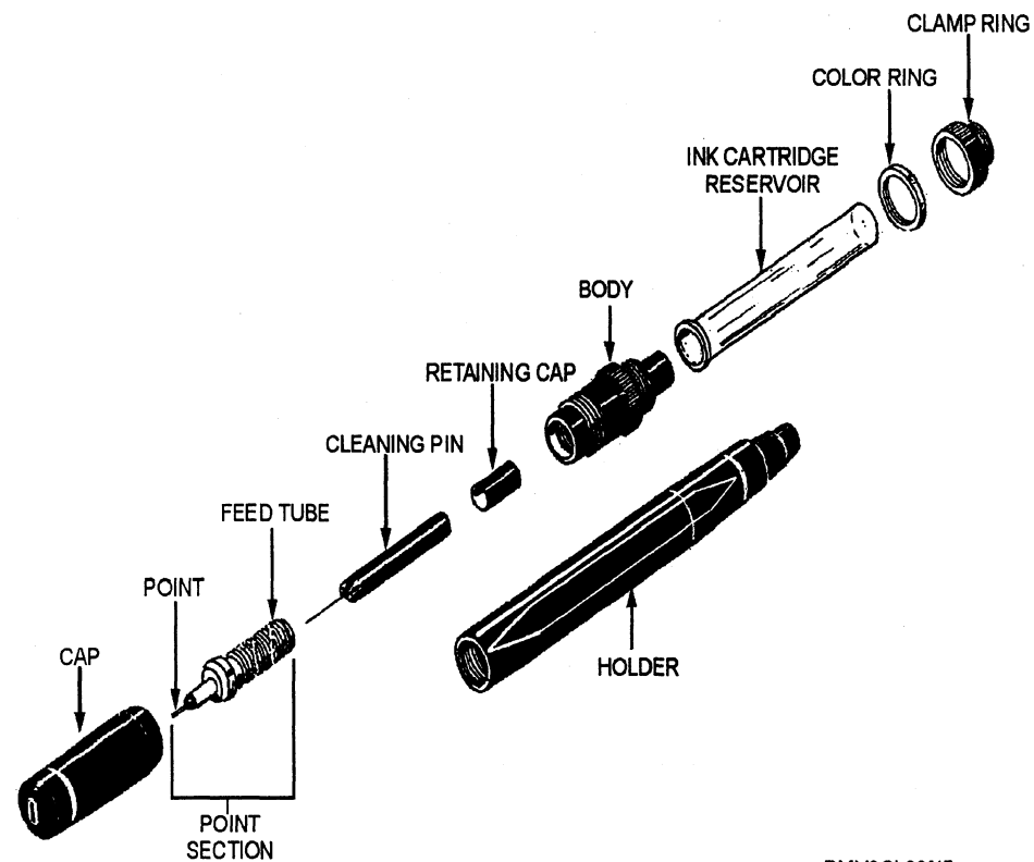
Figure 3-45. —An exploded view in isometric projection.
