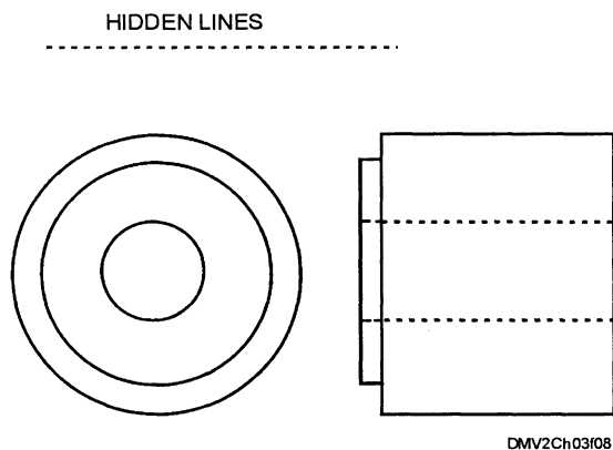
Figure 3-8. —Hidden lines.
