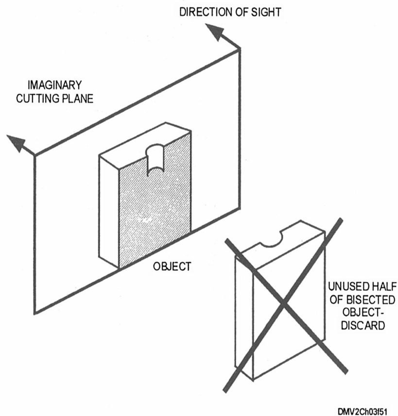
Figure 3-51. —Sectional views.
