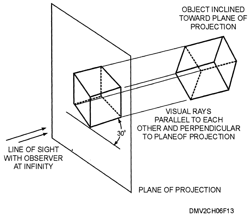
Figure 6-13. —An axonometric projection.
