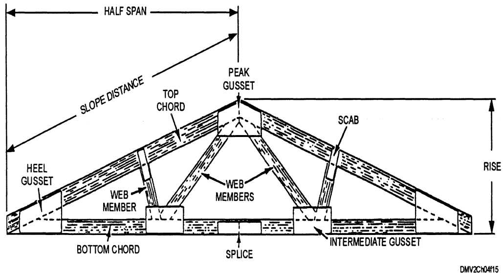
Figure 4-15. —Truss nomenclature.
