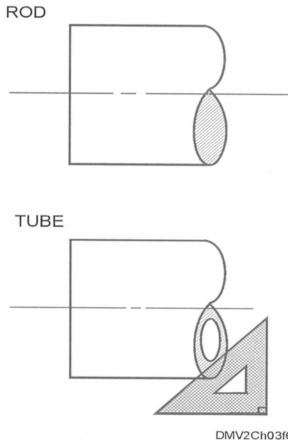
Figure 3-60. —Conventional breaks in rods and tubing.
