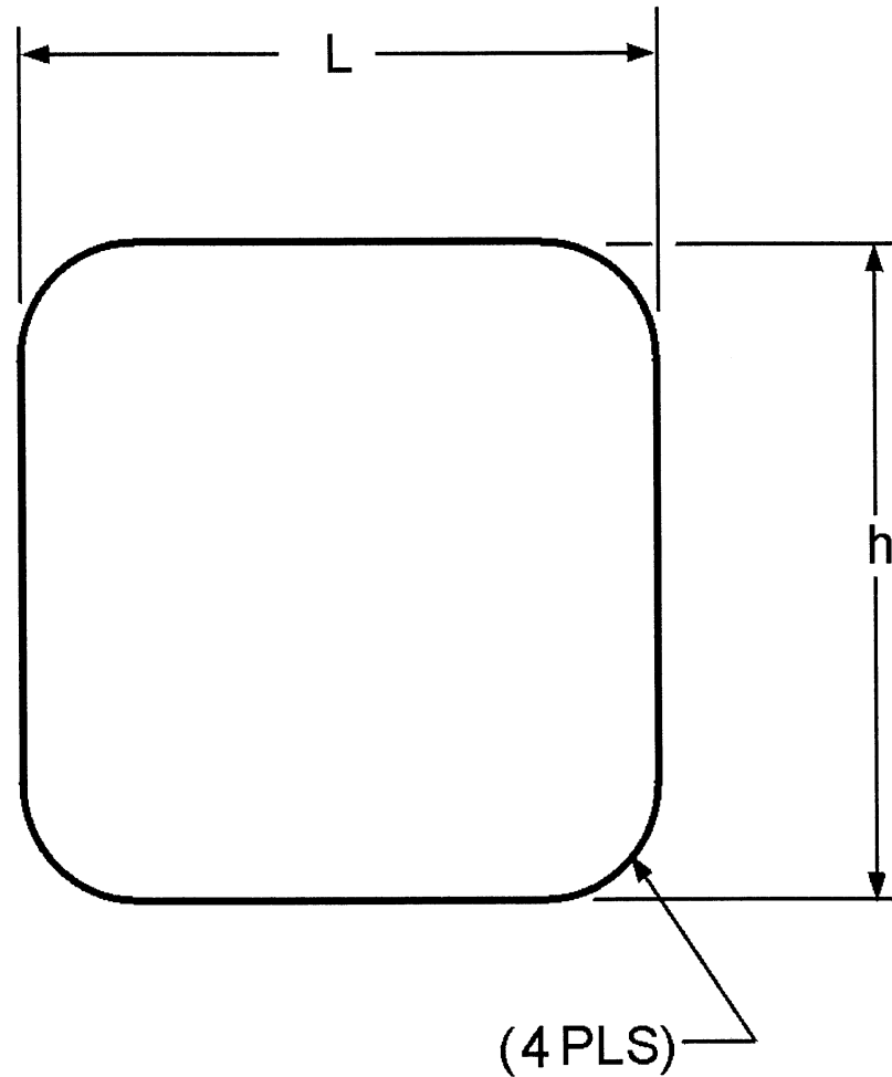
DMV2Ch03f29 Figure 3-29. —Dimensioning rounded corners.
