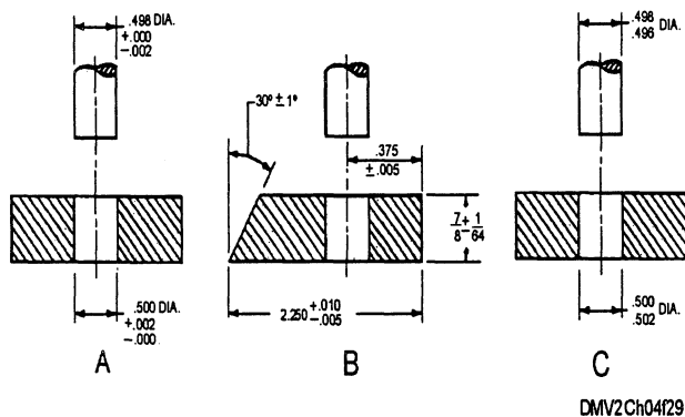
Figure 4-29. —Methods of indicating tolerance.
