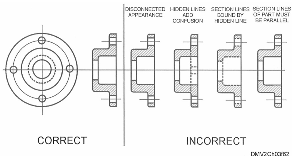
Figure 3-62. —Correct and incorrect lines in a sectional view.
