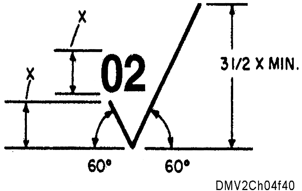
Figure 4-40. —Proportions for a basic finish mark.
