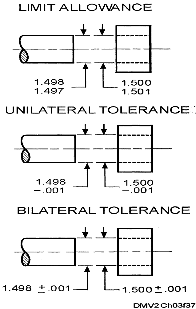
Figure 3-37. —Indicating tolerance.
