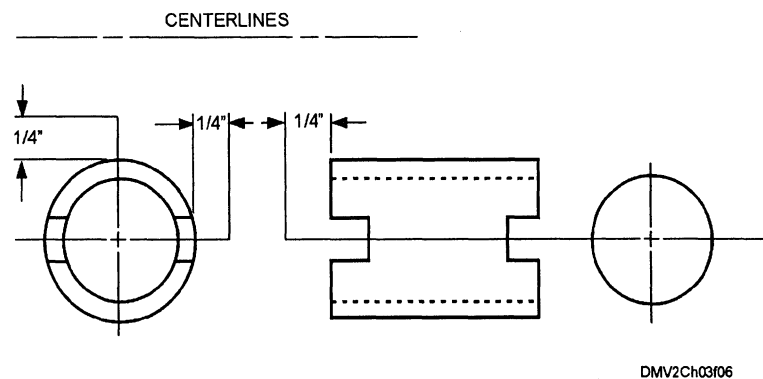
Figure 3-6.—Centerlines.
