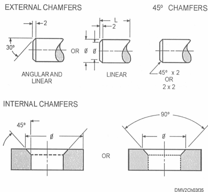
Figure 3-35. —Dimensioning chamfers.
