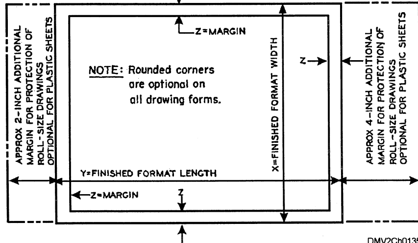
Figure 1-35.—Drawing sheet sizes and associated margin widths.
