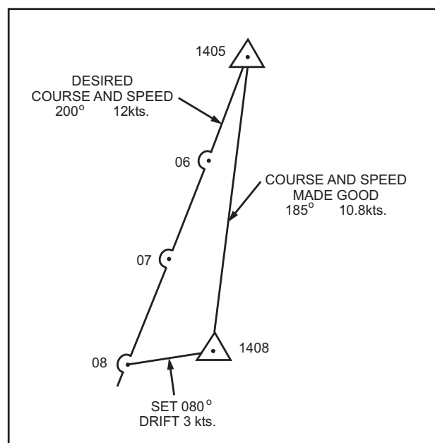
Figure 12-27.—Determining set and drift.
