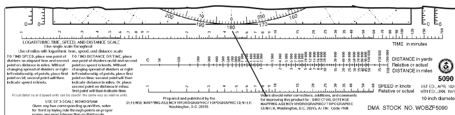
Figure 11-6.—Maneuvering board nomogram.
