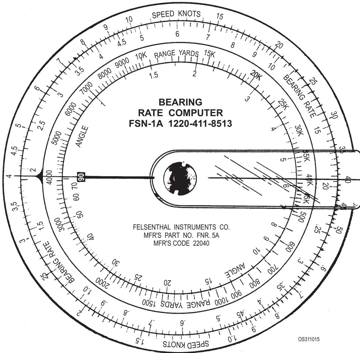
Figure 10-15.—Bearing Rate Computer (bearing slide rule [BRSR]).
