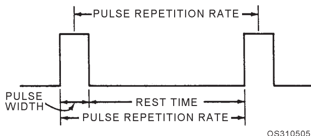
Figure 5-5.—Radar pulse relationships
