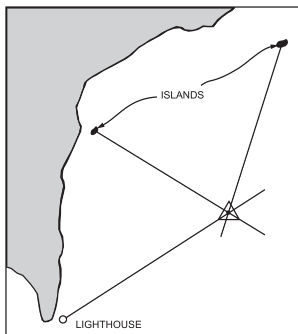
Figure 12-22.—Three-bearing fix.
