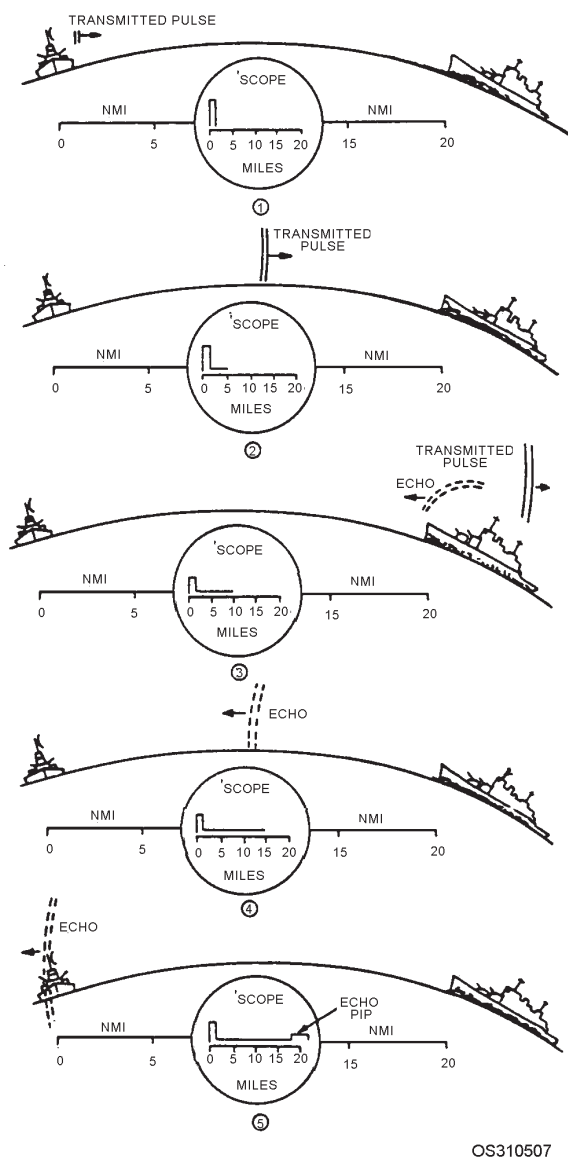
Figure 5-7.—Radar range determination.
