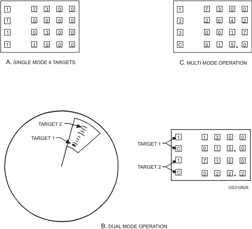
Figure 8-29.—Examples of intra-target data indicator displays.
