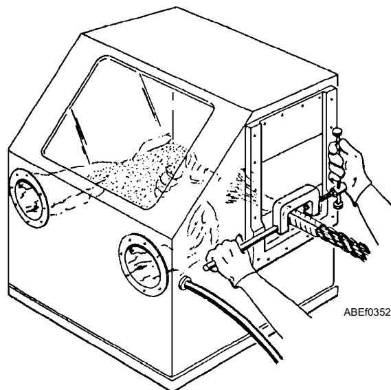
Figure 3-52.—Rotating the cable in the grit blast cabinet.
