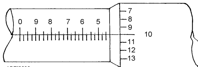
Figure 2-30.—Depth micrometer sleeve and thimble scales.
