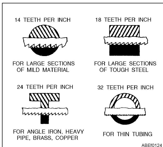
Figure 1-14.—Selecting the proper hacksaw blade.
