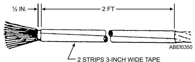
Figure 3-50.—Adhesive cloth tape applied to wire rope.
