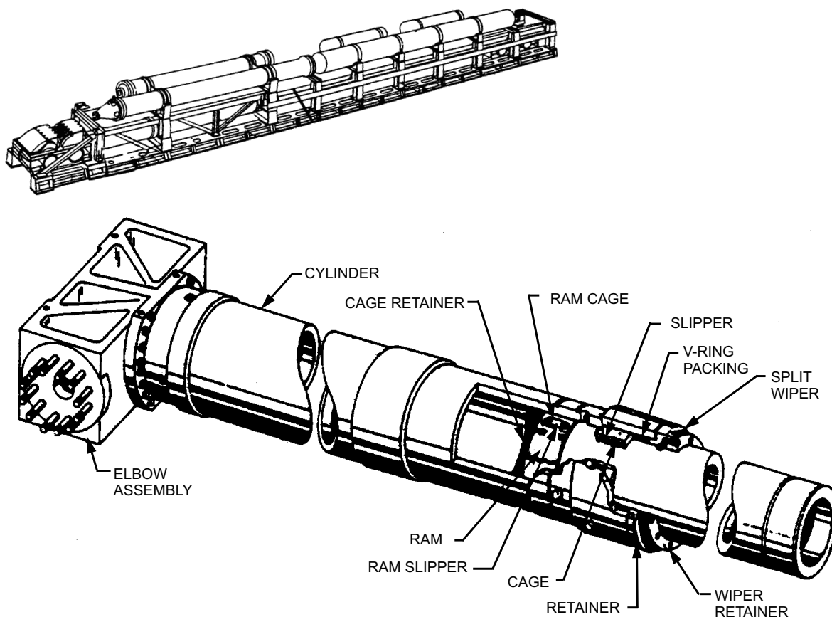
Figure 3-15.—Cylinder and ram assembly.
