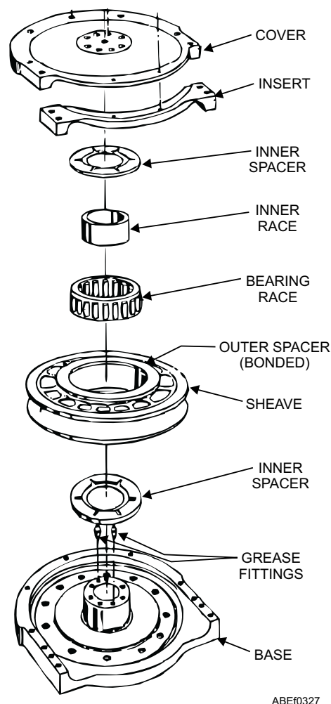
Figure 3-27.—Typical sheave assembly.
