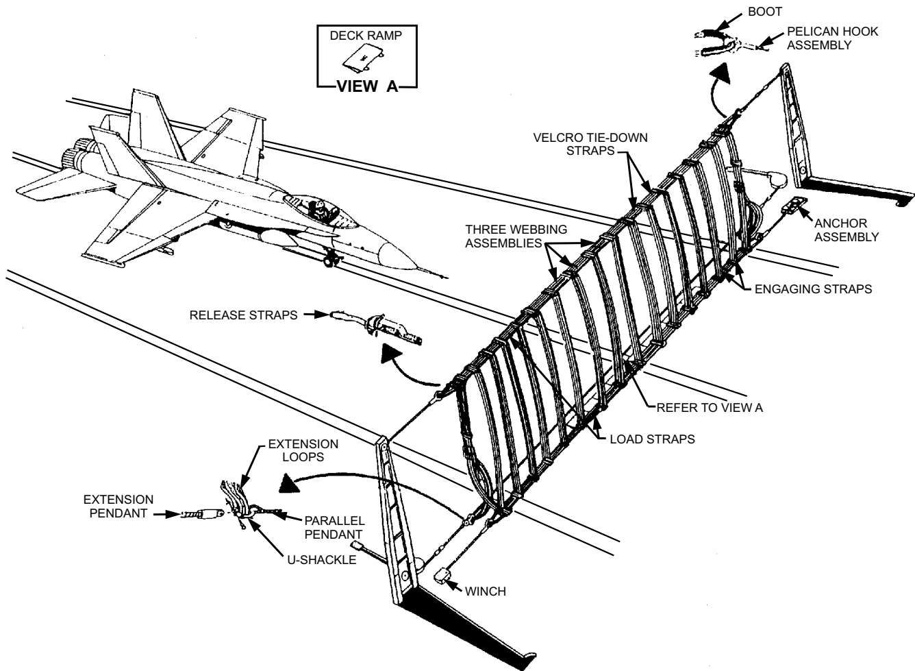
Figure 3-37.—Emergency arrestment.
