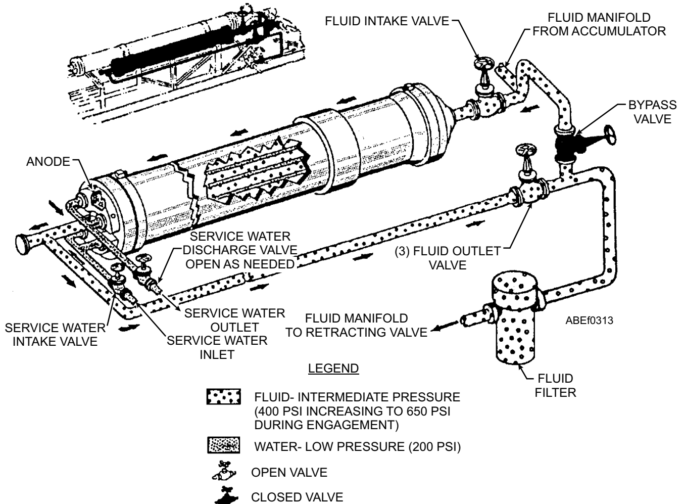
Figure 3-13.—Fluid cooler assembly.
