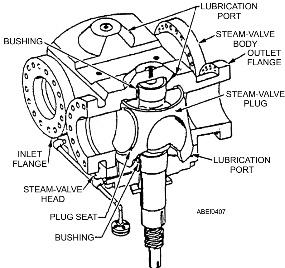
Figure 4-6.—Launching valve steam valve.
