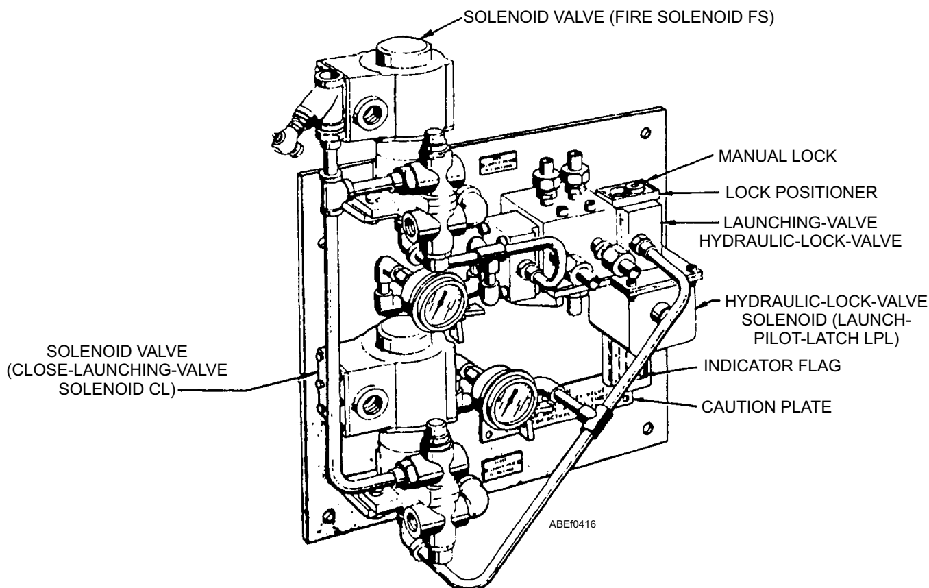
Figure 4-15.—Launch-valve hydraulic-lock-valve panel.
