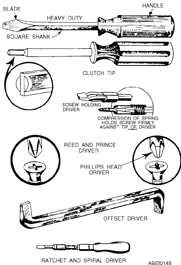
Figure 1-71.—Types of screwdrivers.
