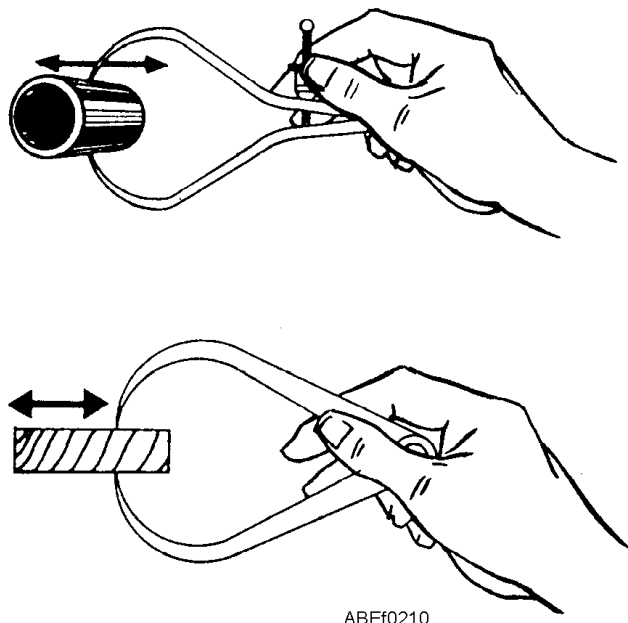
Figure 2-10.—Using an outside caliper.
