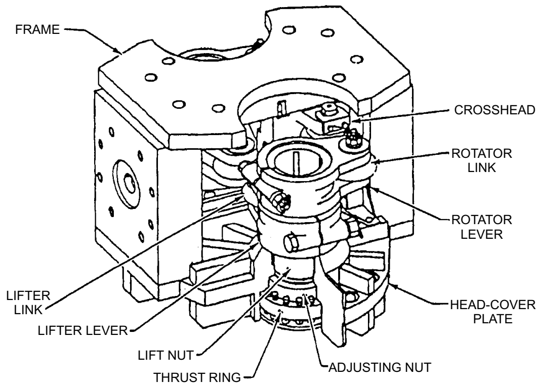
Figure 4-7.—Launch valve operation control assembly.
