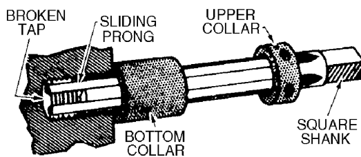
A. STRAIGHT TAP EXTRACTOR
