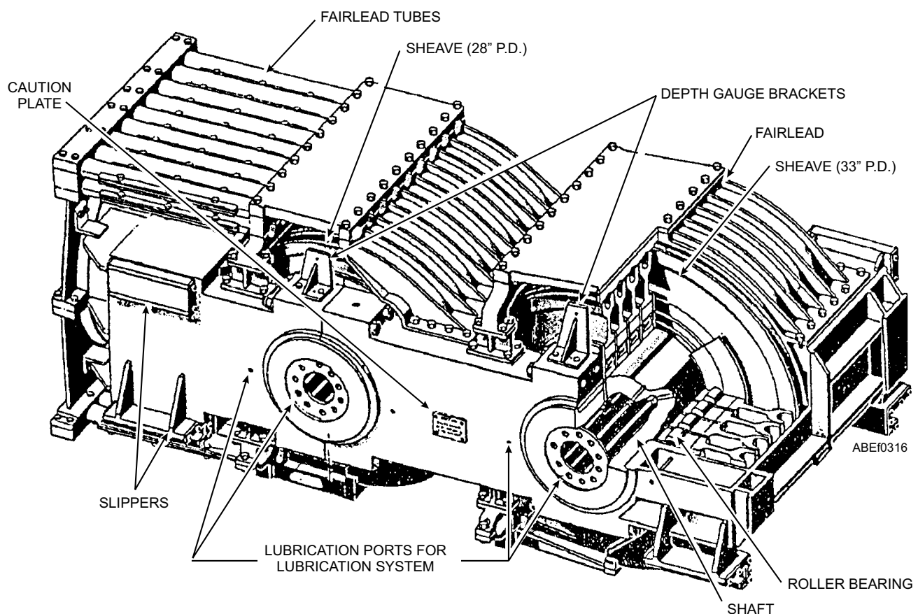
Figure 3-16.—Crosshead assembly.
