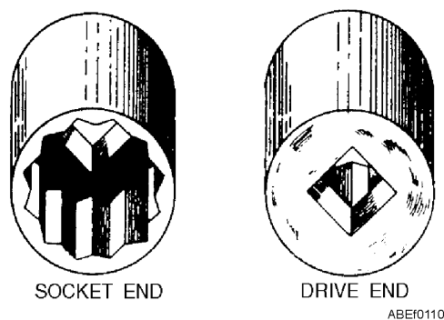
Figure 1-33.—12-point sockets.
