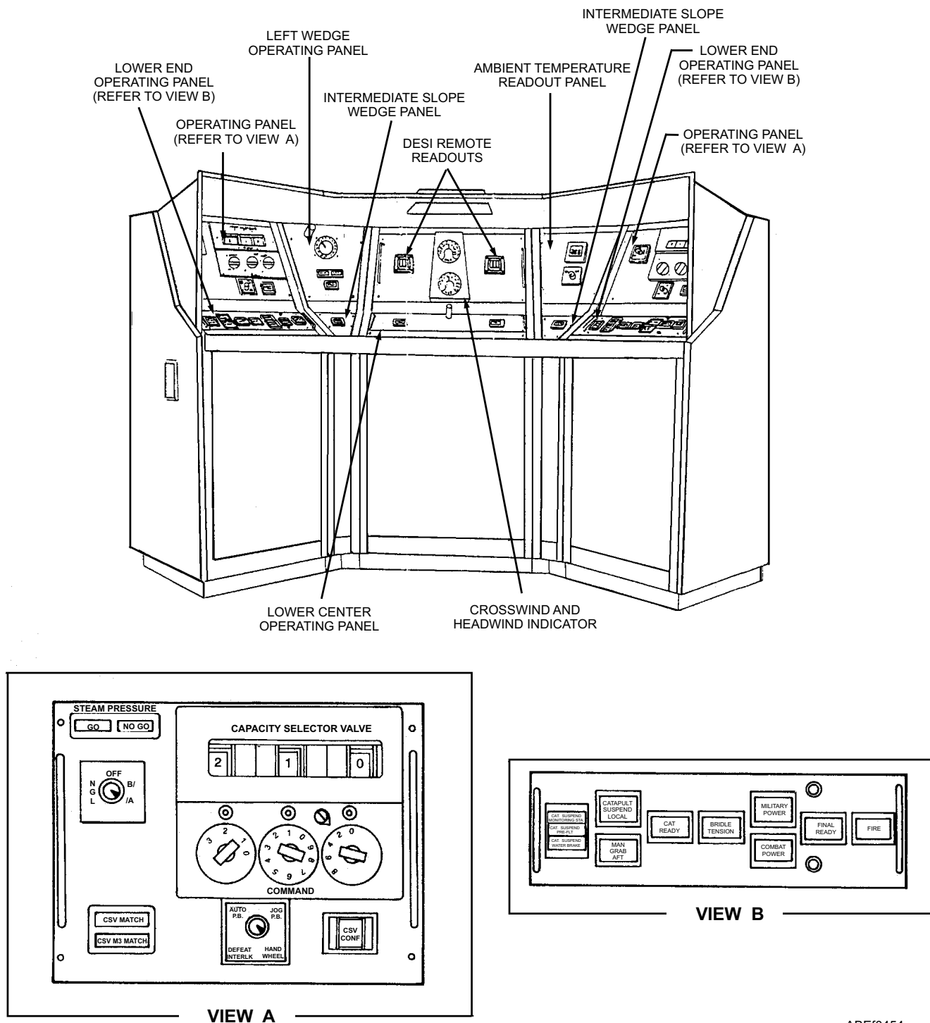
Figure 4-53.—Catapult-officer control console.
