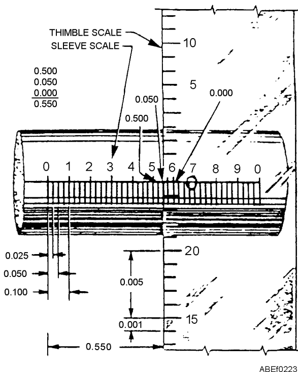
Figure 2-23.—Sleeve and thimble scales of a micrometer.
