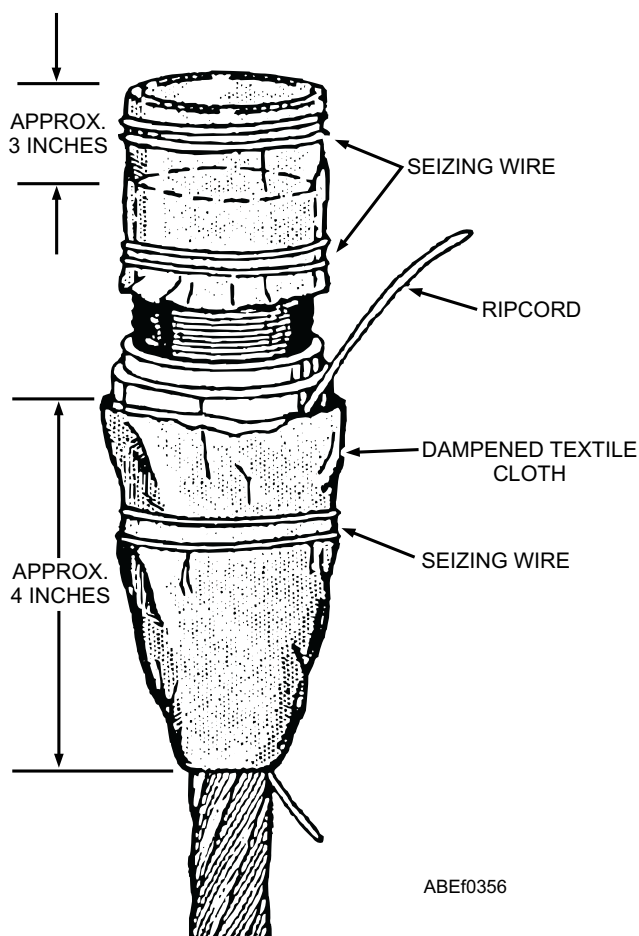
Figure 3-56.—Textile cloth applied to the terminal.
