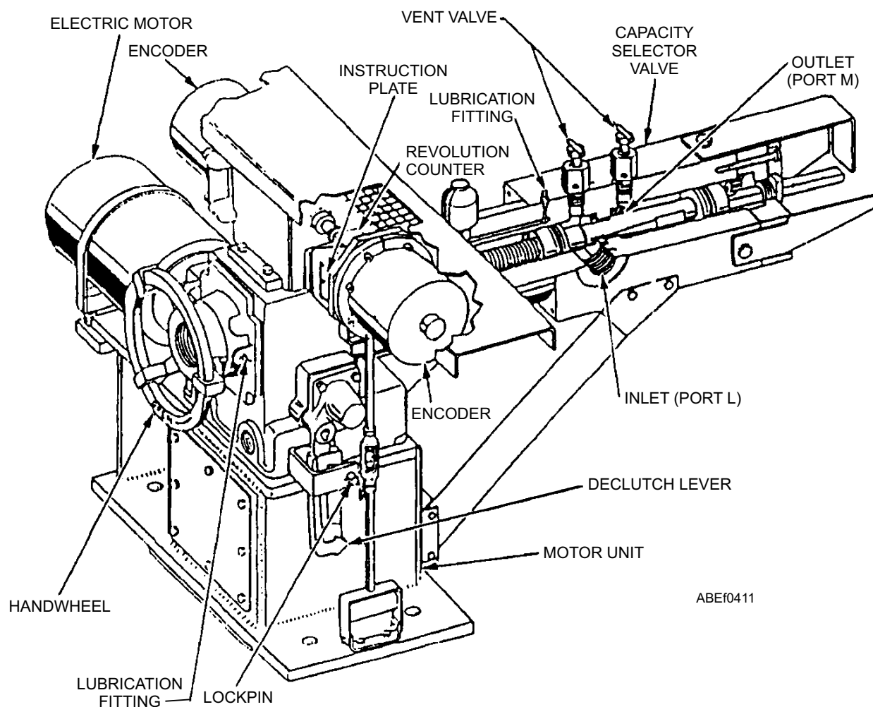
Figure 4-10.—Capacity selector valve assembly.
