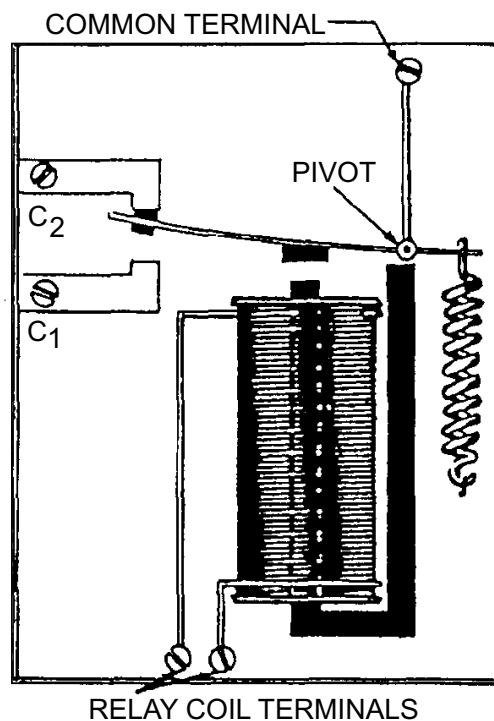
Figure 4-52.—Relay construction.
