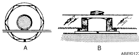
Figure 1-17.—Removing a frozen nut with a hacksaw.
