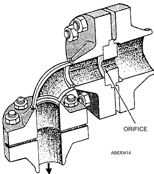
Figure 4-13.—Pressure-breaking orifice elbow.
