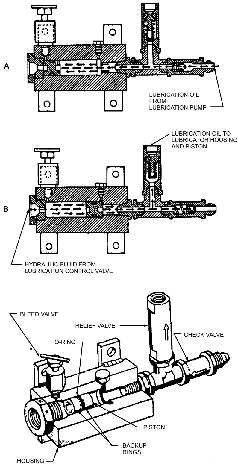
Figure 4-36.—Metering pump.
