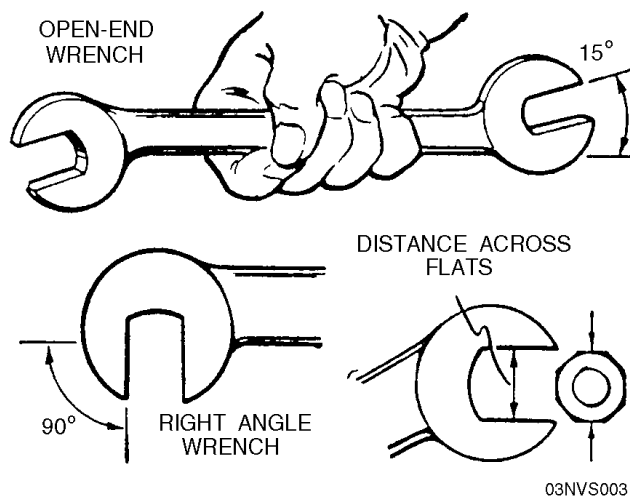
Figure 1-26.—Open-end wrenches.
