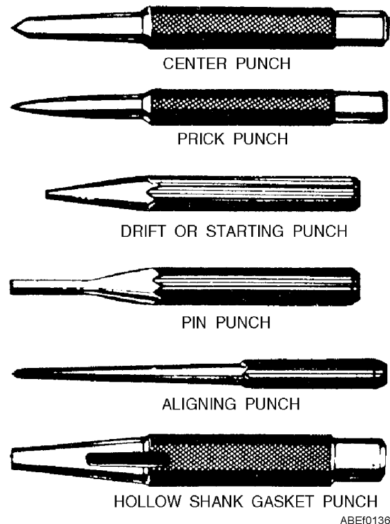
Figure 1-50.—Punches.
