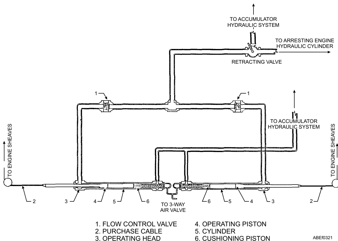
Figure 3-21.—Cable anchor damper fluid flow (arrestment).
