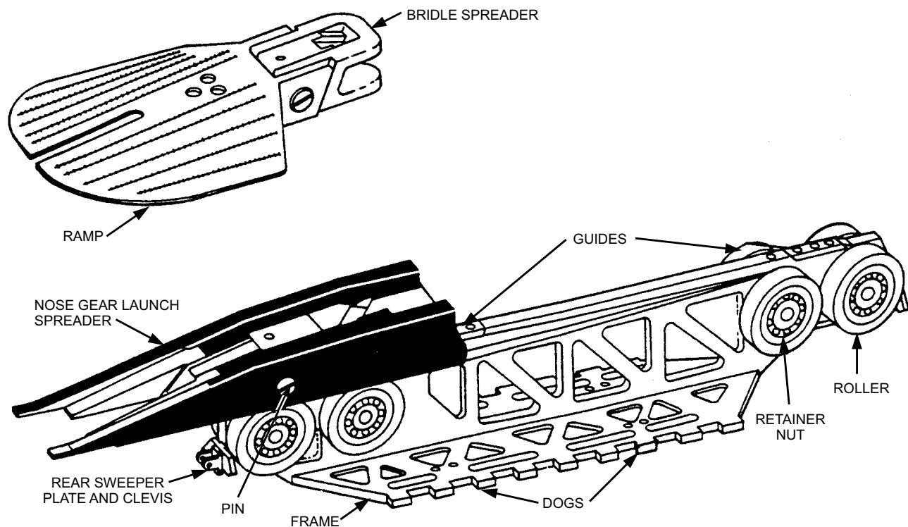
Figure 4-26.—Shuttle assembly.
