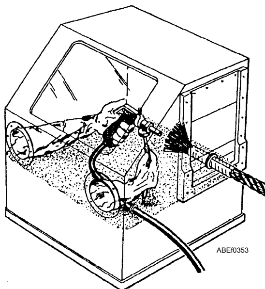
Figure 3-53.—Blasting inner wires.
