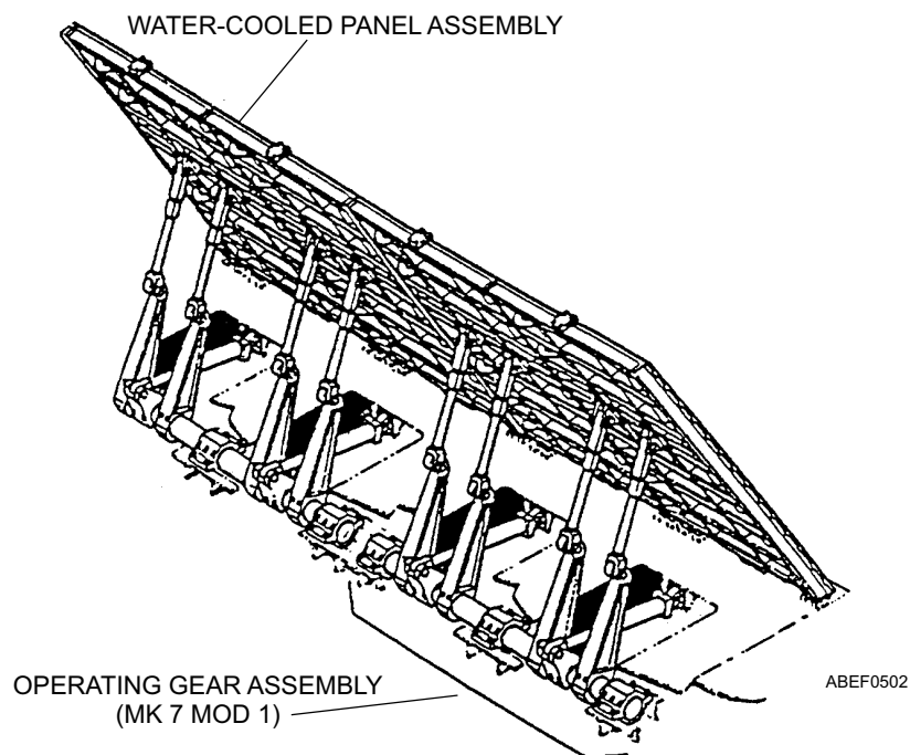
Figure 5-2.—Jet blast deflector assembly.
