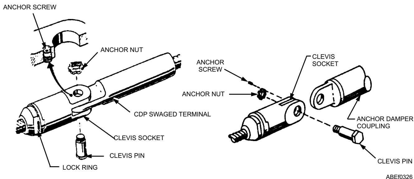
Figure 3-26.—Purchase cable attachments.
