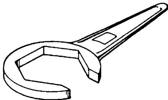
Figure 1-29.—Nonadjustable union nut wrench.
