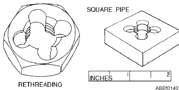
Figure 1-54.—Types of solid dies.
