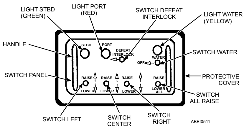
Figure 5-11.—Chestpack portable control assembly.
