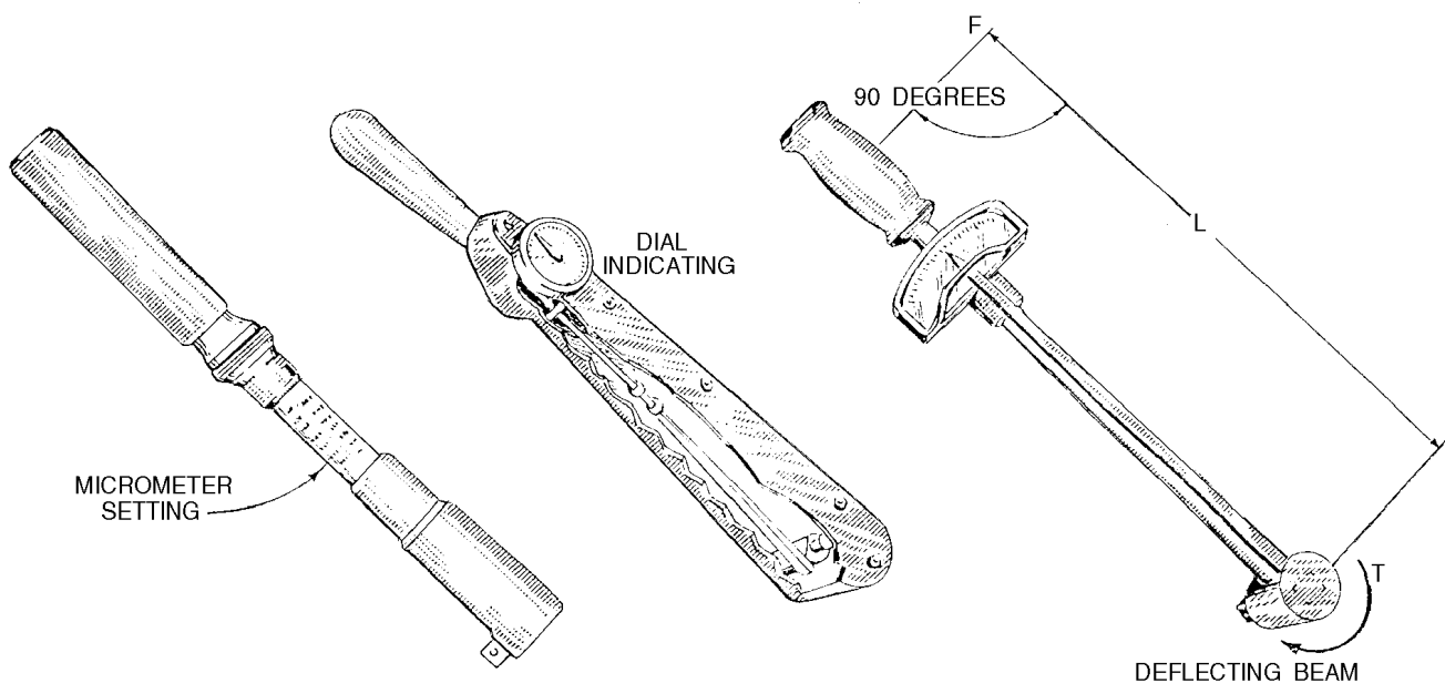
Figure 1-34.—Torque wrenches.
