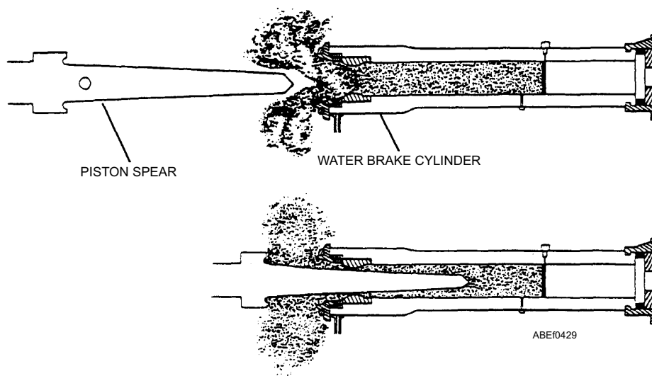
Figure 4-28.—Water brakes.
