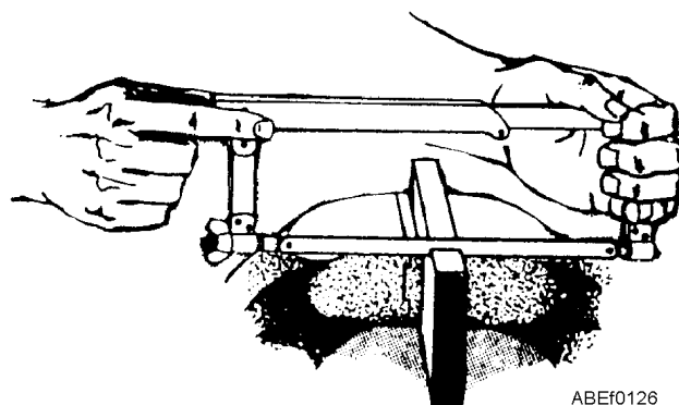
Figure 1-16.—Proper way to hold a hacksaw.
