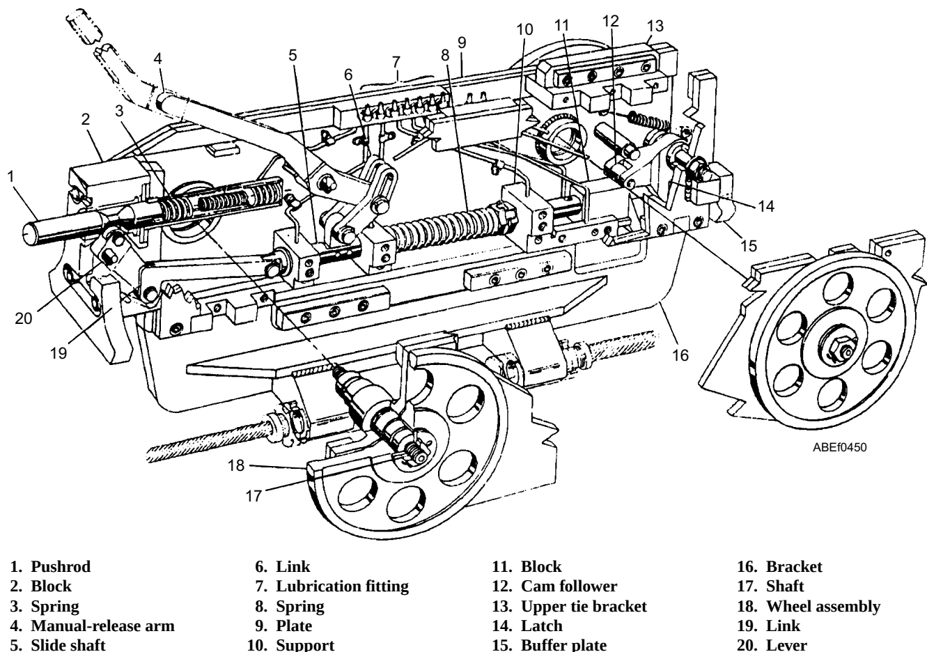
Figure 4-49.—Grab.
