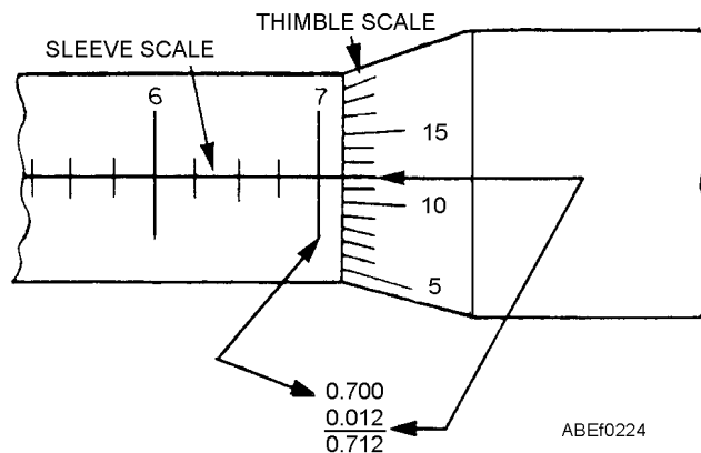
Figure 2-24.—Enlarged micrometer scale.
