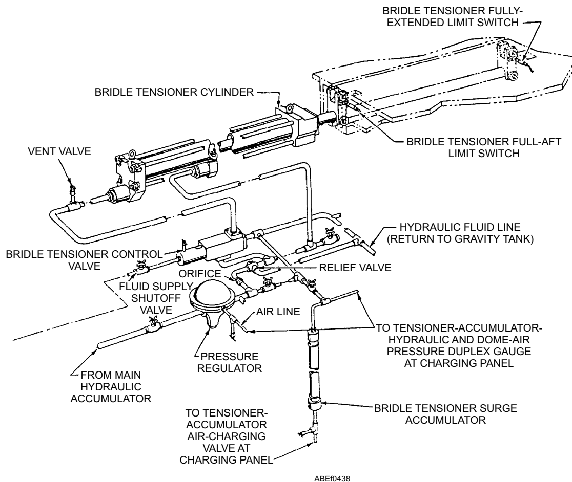
Figure 4-37.—Bridle tensioning system.
