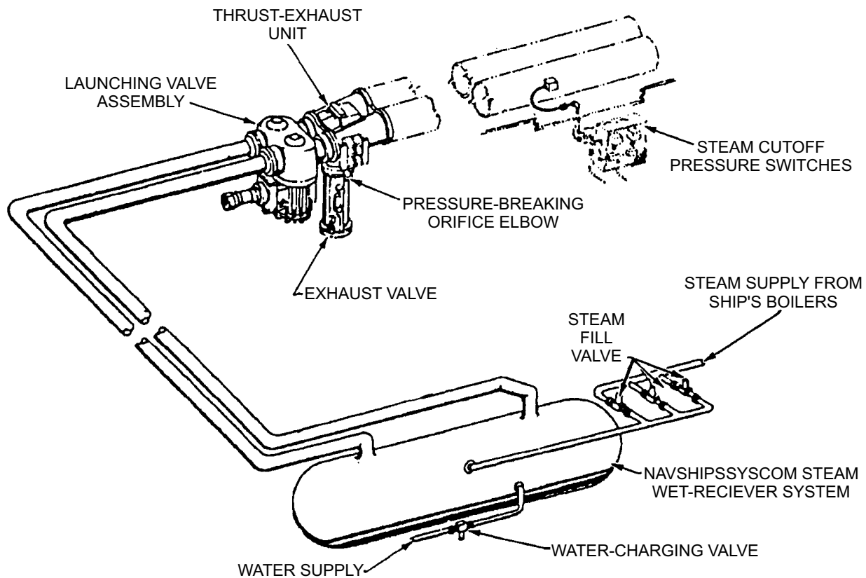
Figure 4-1.—Steam system.
