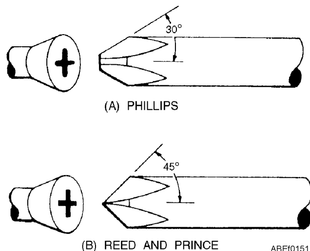
Figure 1-74.—Matching cross-slot screws and screwdrivers.
