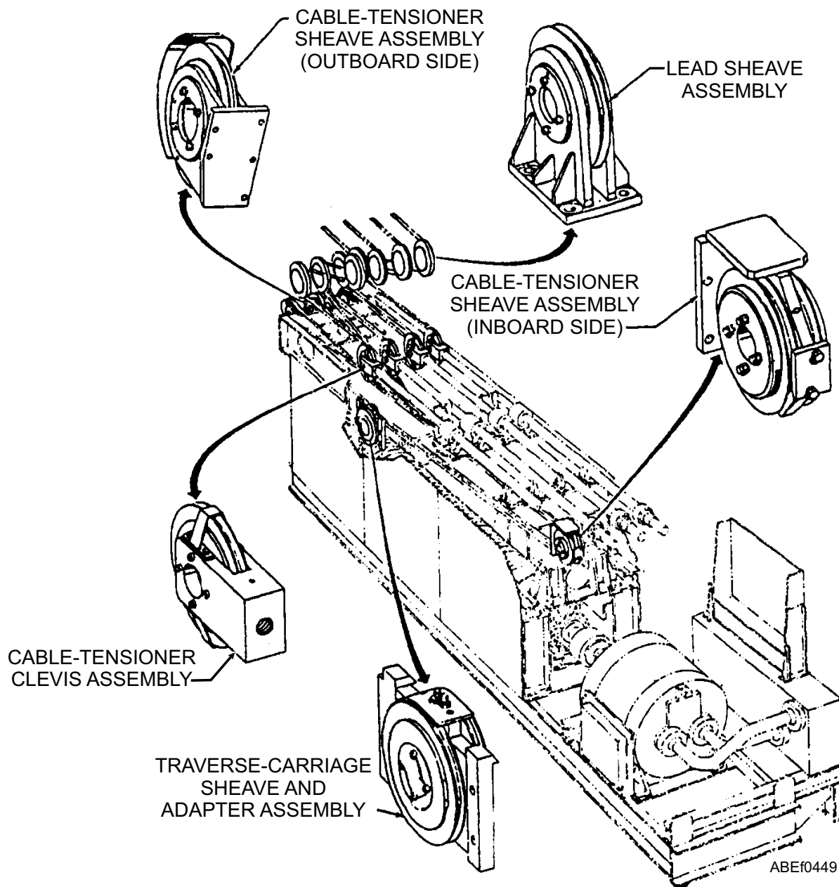
Figure 4-48.—Sheaves.
