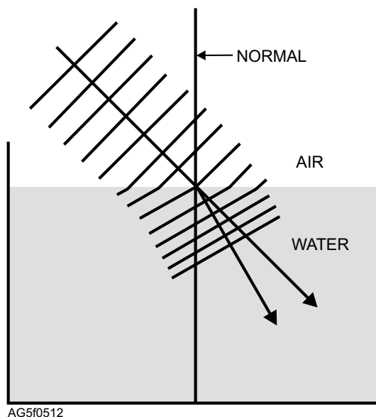
Figure 5-12.—Wave front diagram illustrating refraction of light at an air-water boundary. Ray is entering a more dense substance.
