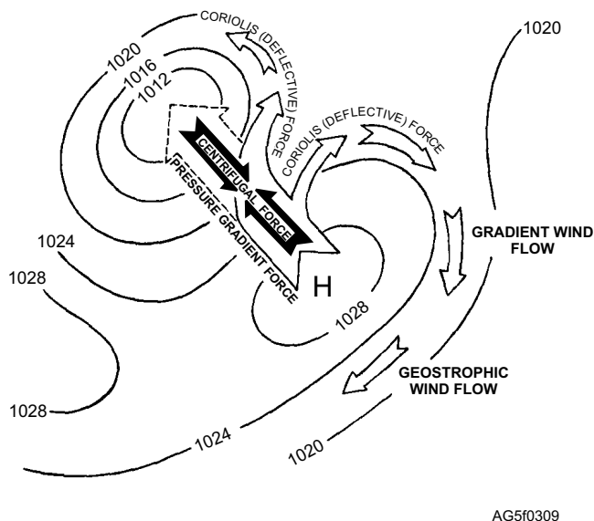
Figure 3-9.—Examples of circulation around high and low pressure systems.
