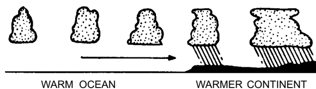
Figure 4-18.—mT (Gulf of Mexico or Atlantic) air in summer moving northward over a warm continental surface.
