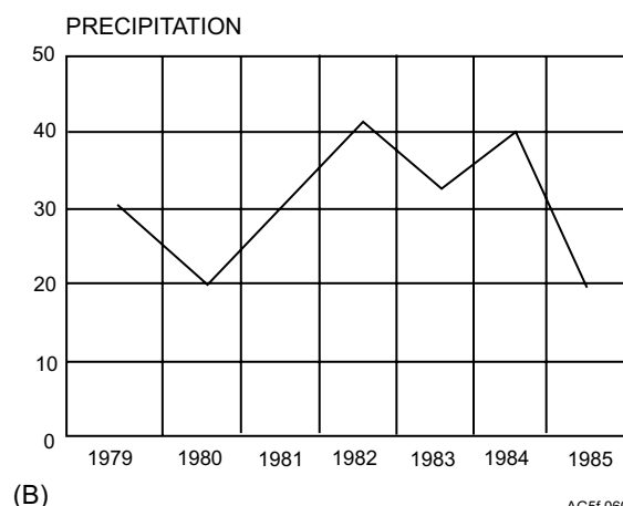
Figure 6-5.—A comparison of the bar and line graph method of showing the variable annual precipitation in a time series. (A) Bar graph; (B) Line graphs.
