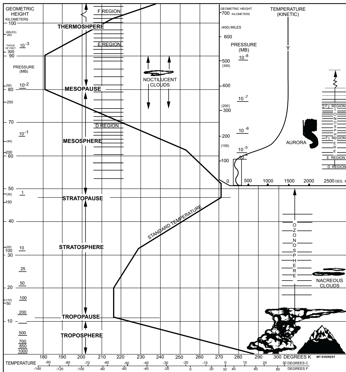
Figure 1-9.—Earth's Atmosphere.
