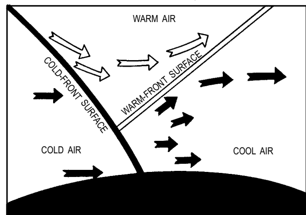
COLD TYPE OCCLUSION
