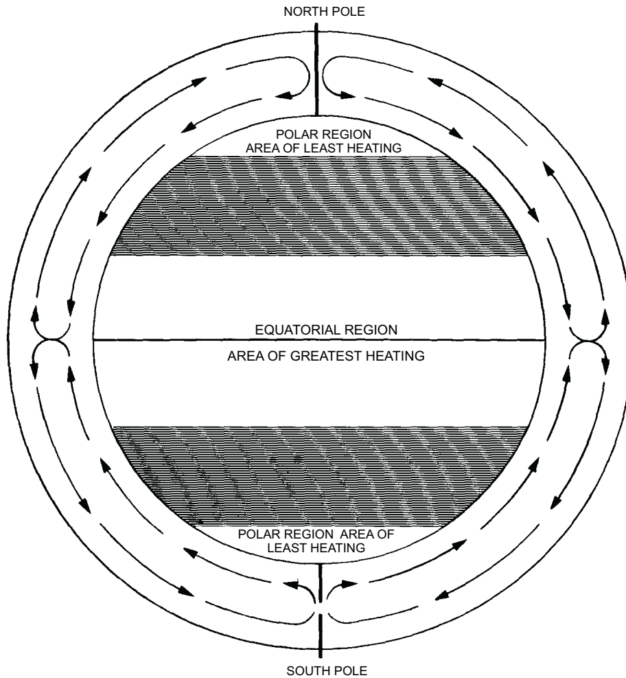
Figure 3-1.—Simple circulation.
