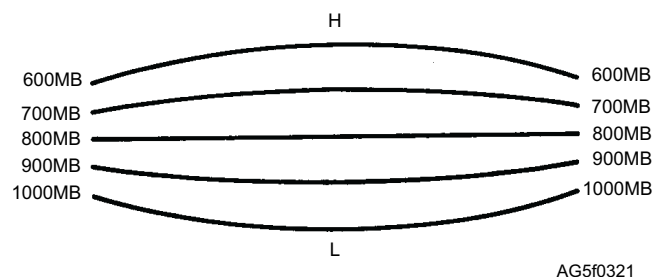
Figure 3-21.—Warm core low.
