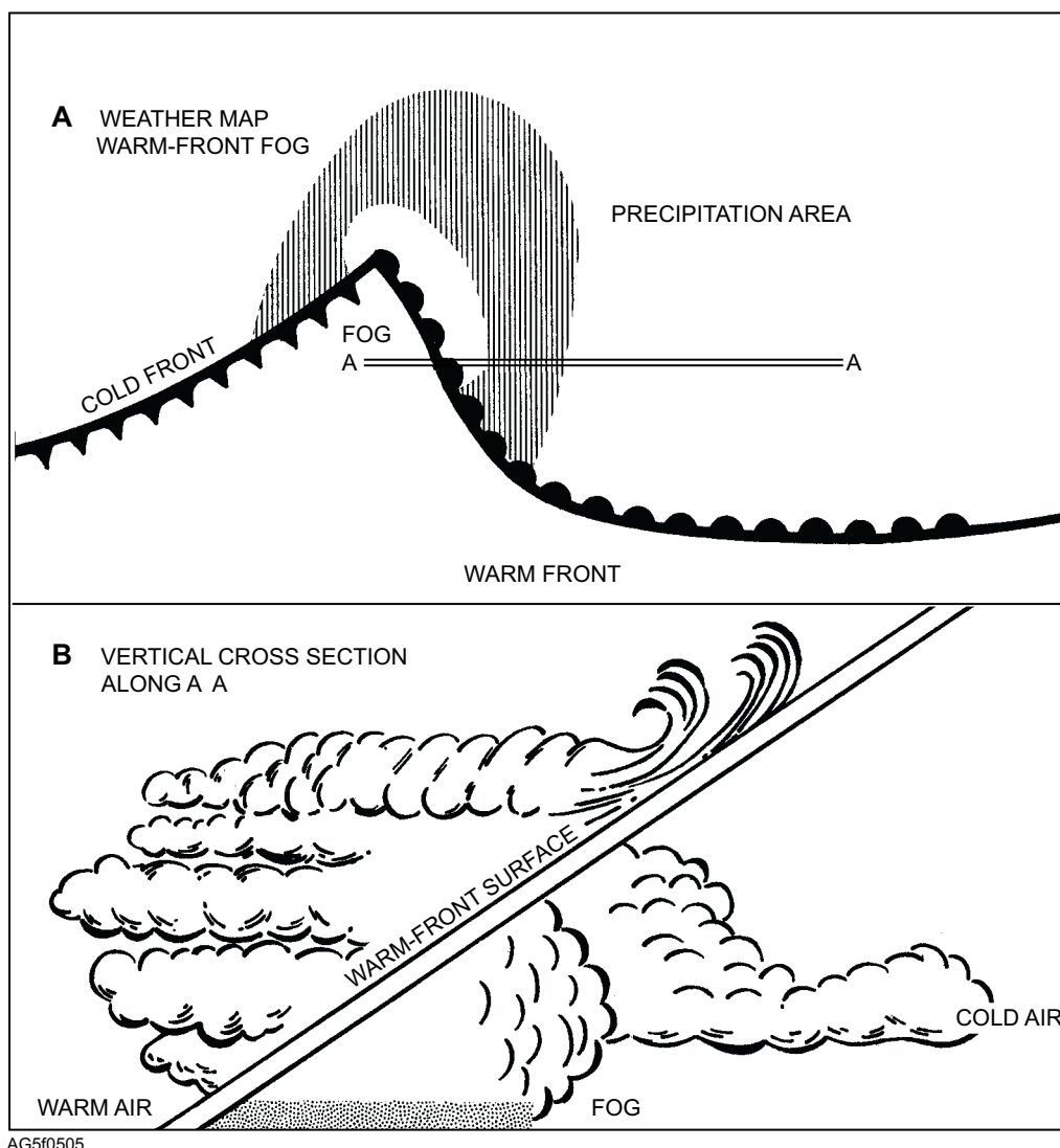
Figure 5-5.—Warm-front fog.
