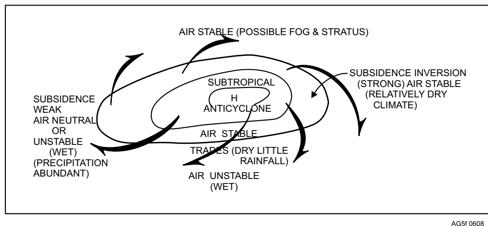
Figure 6-8.—Weather, winds, and stability conditions around the subtropical high.
