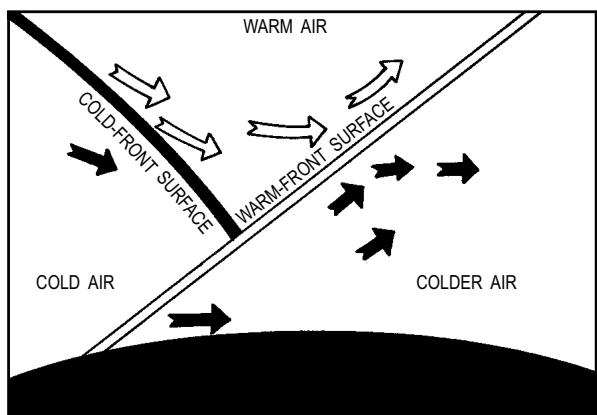
Figure 4-40.—Vertical cross-section of a warm type of occlusion. AG5f0440
