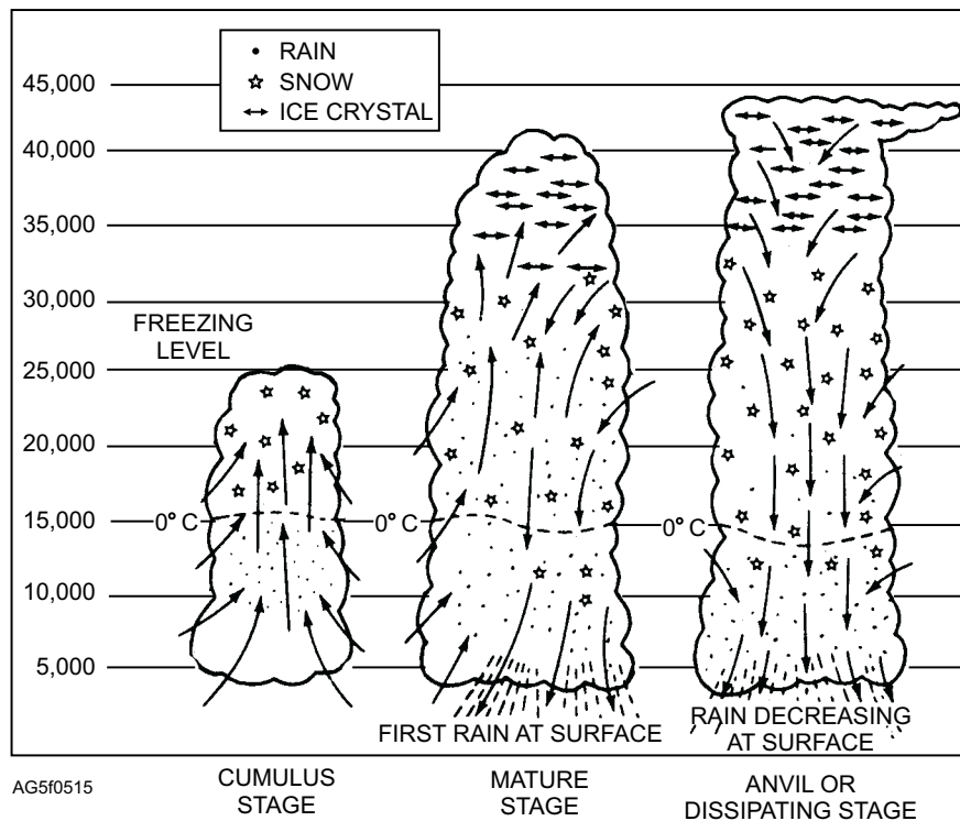
Figure 5-15.—Life cycle of a thunderstorm cell.
