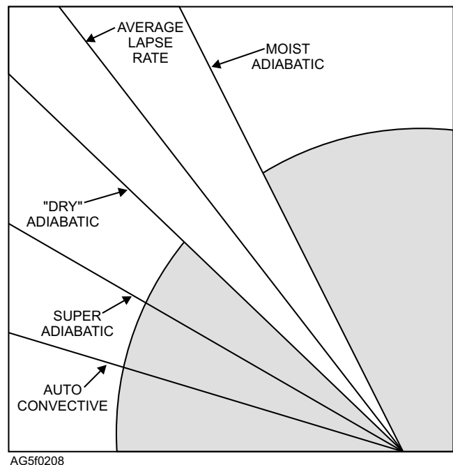
Figure 2-8.—Adiabatic lapse rates.
