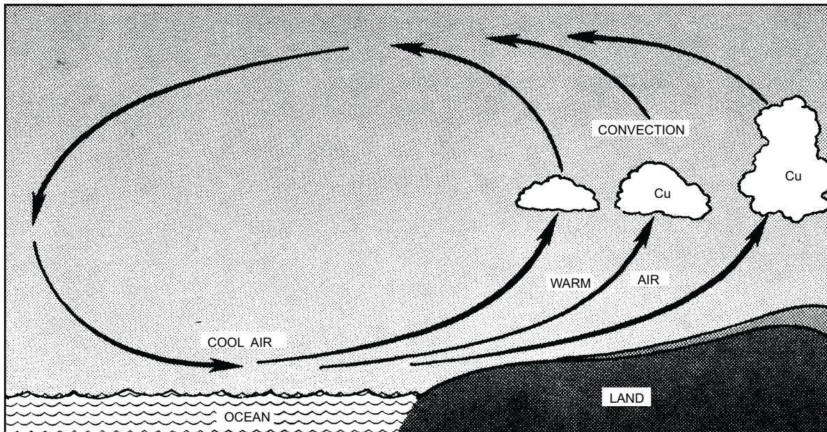
SEA BREEZE
