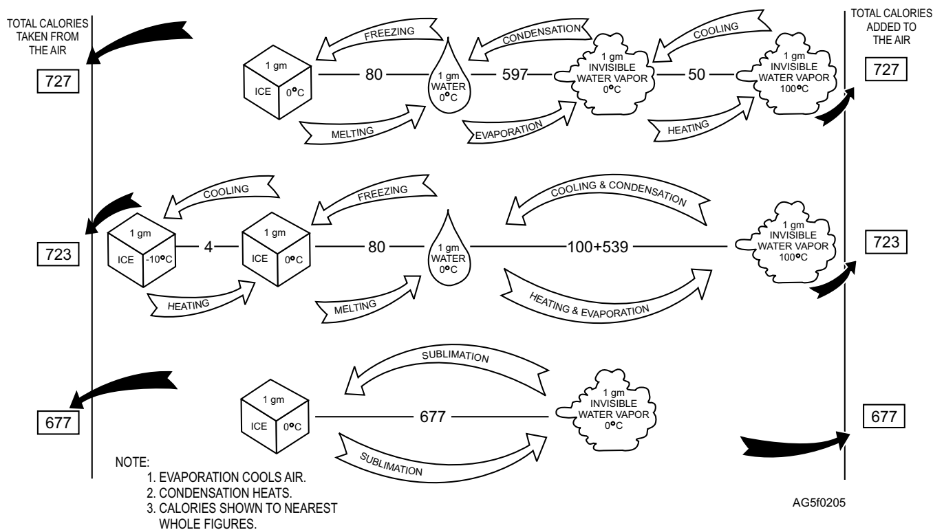
Figure 2-5.—Thermal history of 1 gram of ice during changes of state.
