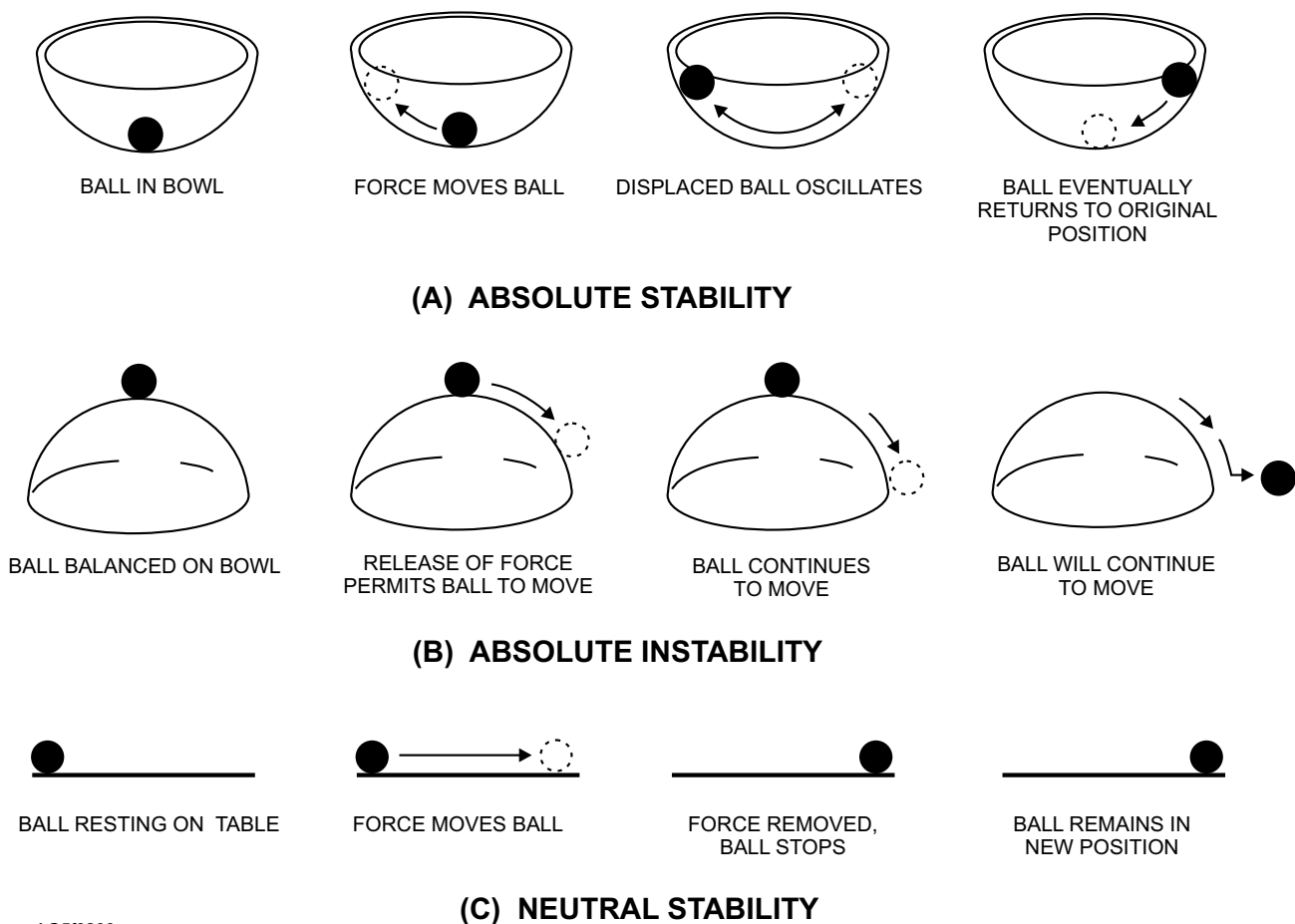
Figure 2-9.—Analogy depiction of stability.
