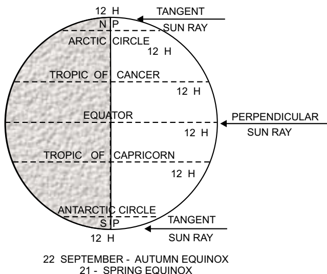
Figure 6-3.—Latitude differences in amount of insolation.
