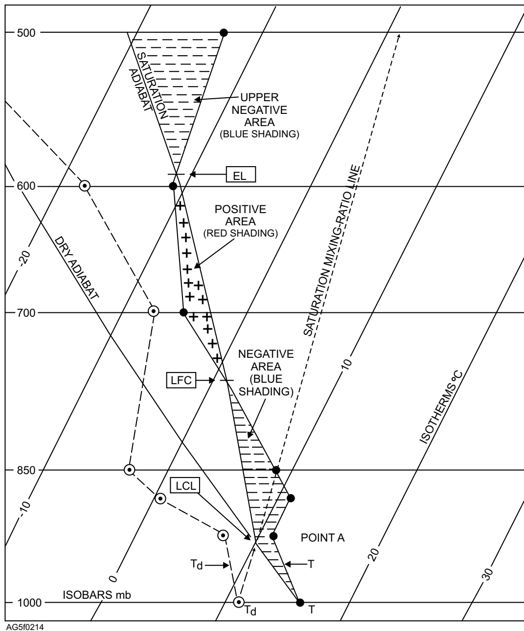
Figure 2-14.—Example of positive and negative energy areas (mechanical lifting).
