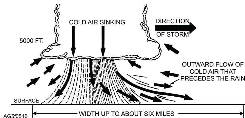
Figure 5-16.—Downdraft beneath a thunderstorm cell in the mature stage. Arrows represent wind flow. Dashed lines indicate rainfall.
