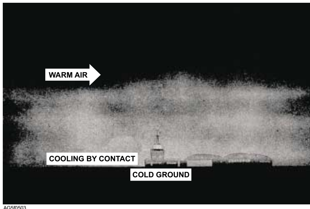
Figure 5-3.—Advection fog.
