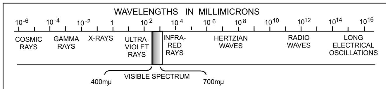
Figure 1-5.—Electromagnetic spectrum.
