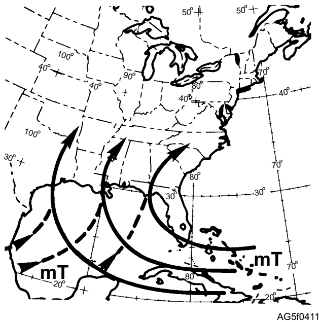
Figure 4-11.—Trajectories of mT air over the Atlantic in winter.
