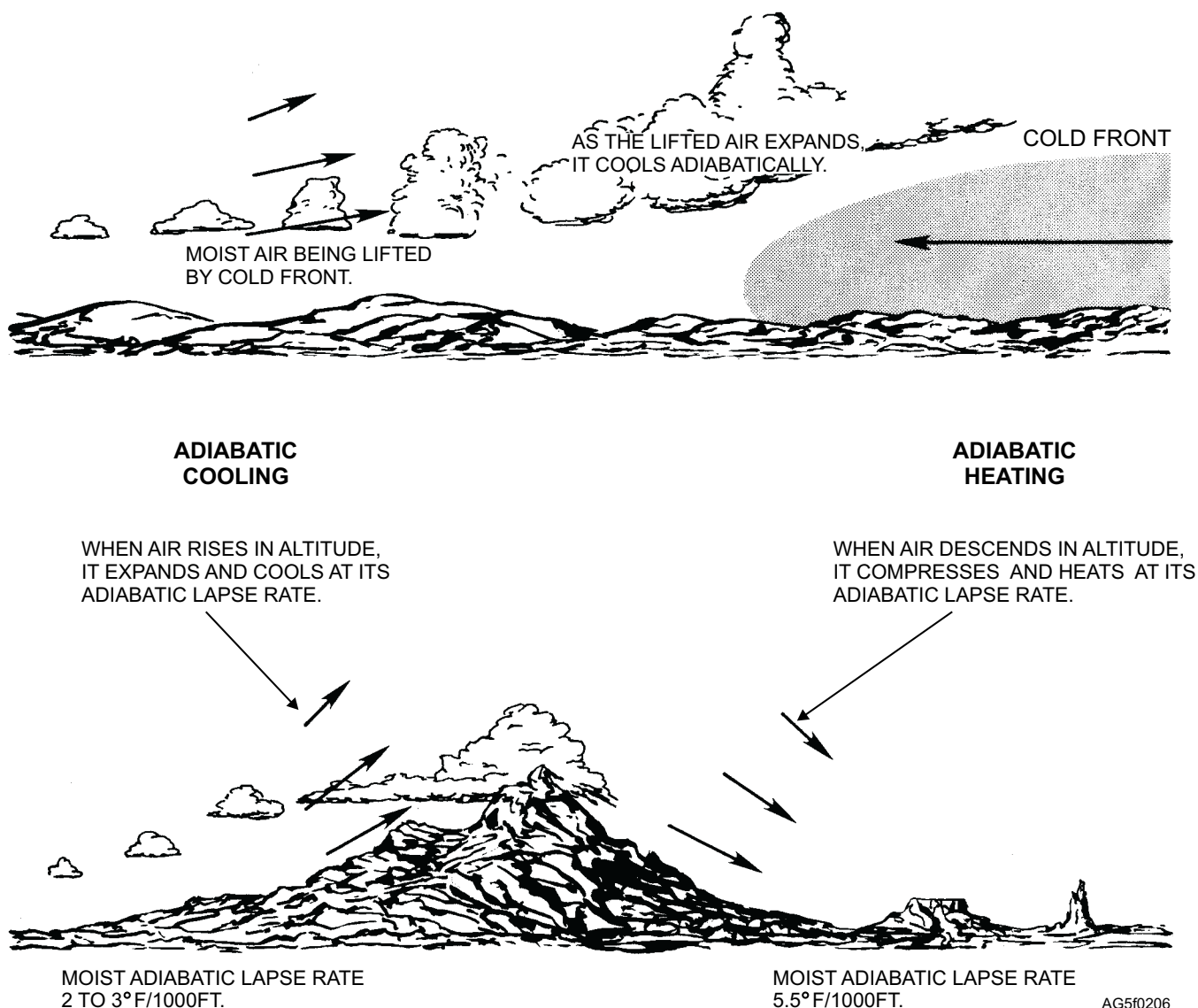
Figure 2-6.—Adiabatic cooling and heating process.
