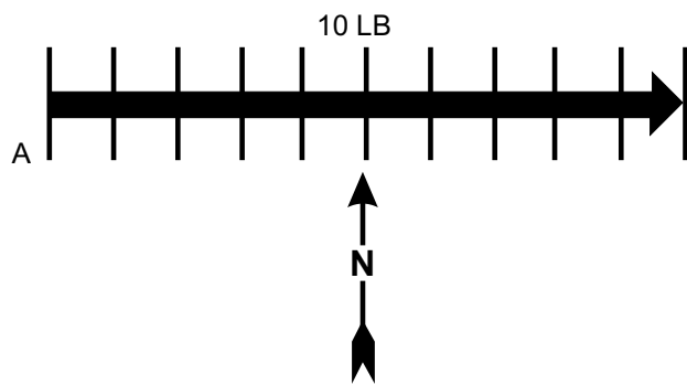
Figure 2-1.—Example of a vector.
