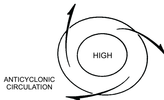
Figure 3-15.—Anticyclone.
