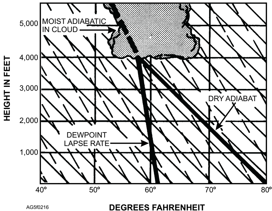
Figure 2-16.—Determine of cloud's base when the dew point and temperature are known.
