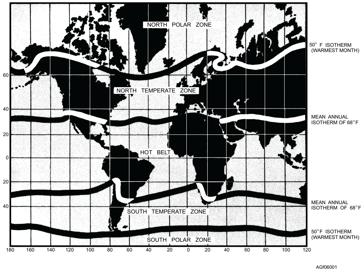
Figure 6-1.—Temperature zones.
