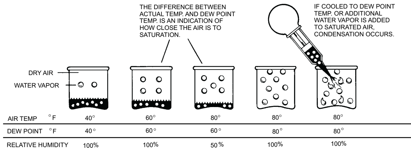
Figure 1-12.—Relative humidity and dew point.
