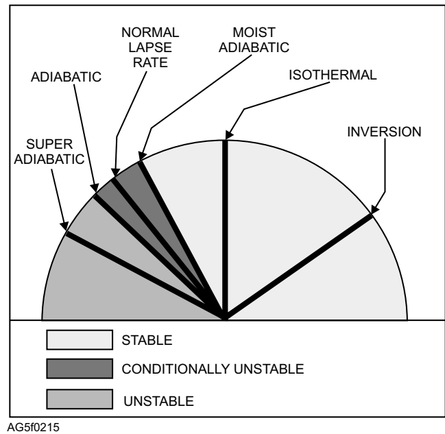
Figure 2-15.—Degrees of stability in relation to temperature changes with height.
