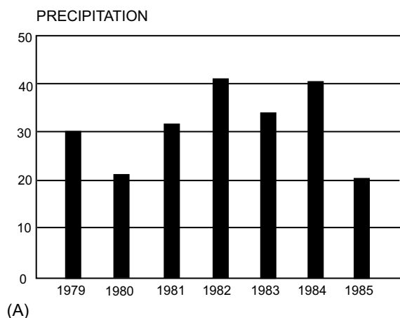
Figure 6-5.—A comparison of the bar and line graph method of showing the variable annual precipitation in a time series. (A) Bar graph; (B) Line graphs.
