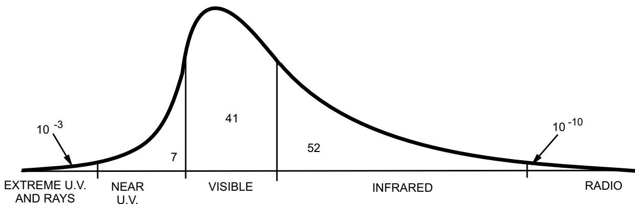
SCHEMATIC DIAGRAM OF THE DISTRIBUTION OF ENERGY IN THE SOLAR SPECTRUM. (NOT TO SCALE). THE NUMBERS ARE PERCENTAGES OF THE SOLAR CONSTANT. THE FIGURE FOR THE RADIO ENERGY IS FOR THE OBSERVED BAND FROM 15 TO 30,000 MHZ.
