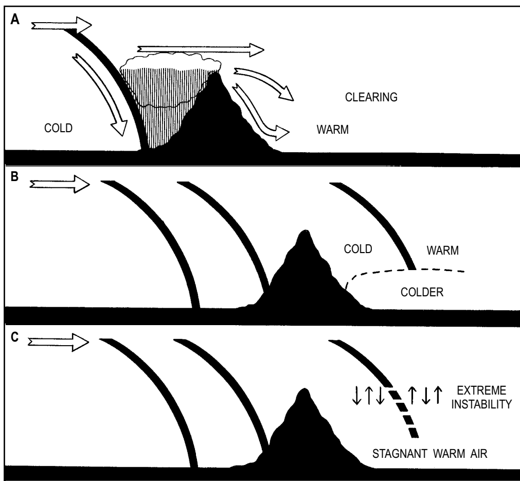
Figure 4-44.—Orographic effects on a cold front.
