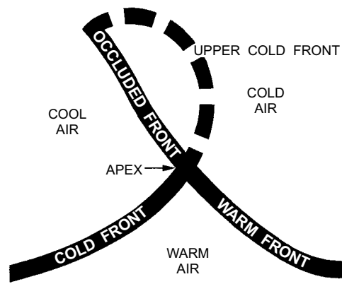
B. WARM TYPE OF OCCLUSION
