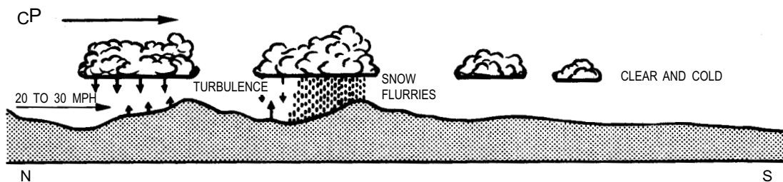
Figure 4-6.—cP air moving southward.
