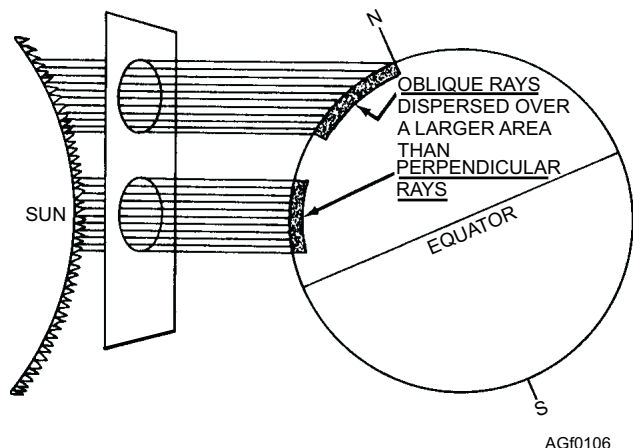
Figure 1-6.—Dispersion of insolation.
