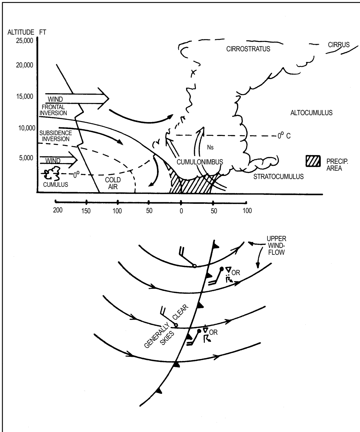
Figure 4-32.—Typical vertical structure of a fast-moving cold front with upper windflow across the front.
