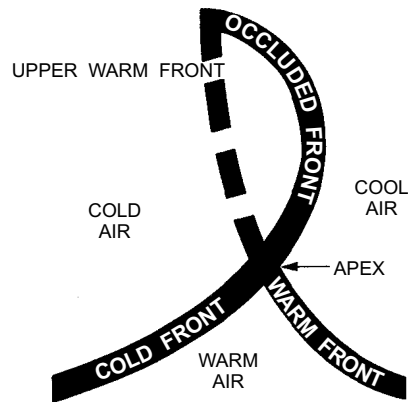
A. COLD TYPE OF OCCLUSION
