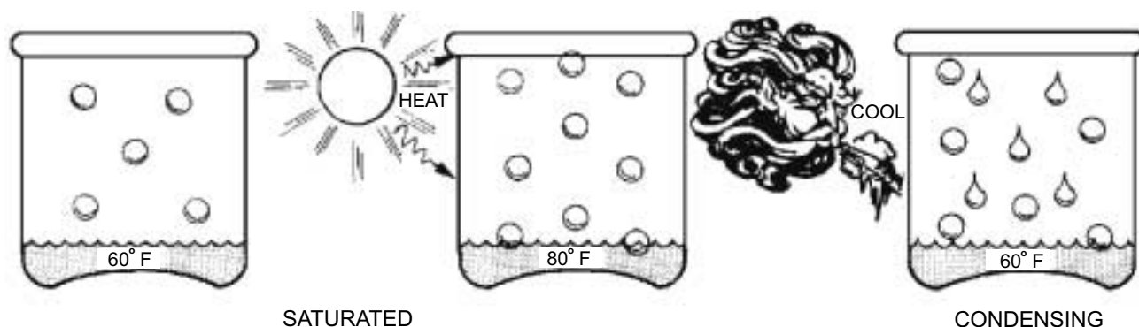
Figure 1-10.—Saturation of air depends on its temperature.
