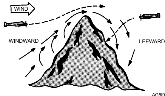
Figure 3-30.—Effect of windflow over mountains.
