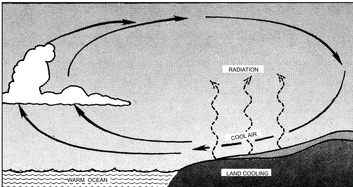
LAND BREEZE
