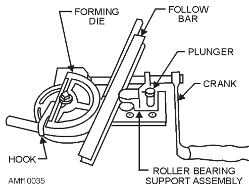
Figure 10-35.—Mechanically operated tube bender.
