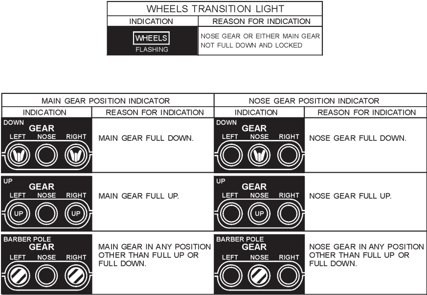
Figure 13-3.—Landing gear warning and position indicator.
