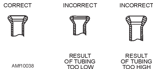
Figure 10-38.—Tube position and resulting flare.
