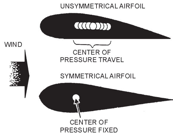
Figure 17-1.—Center of pressure.
