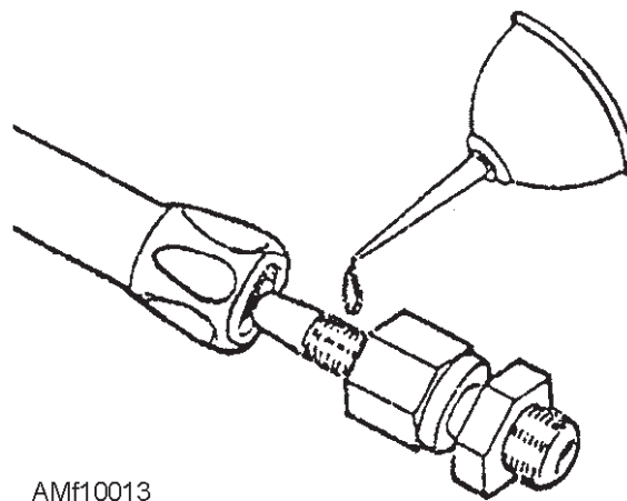
Figure 10-13.—Assembly lubrication.
