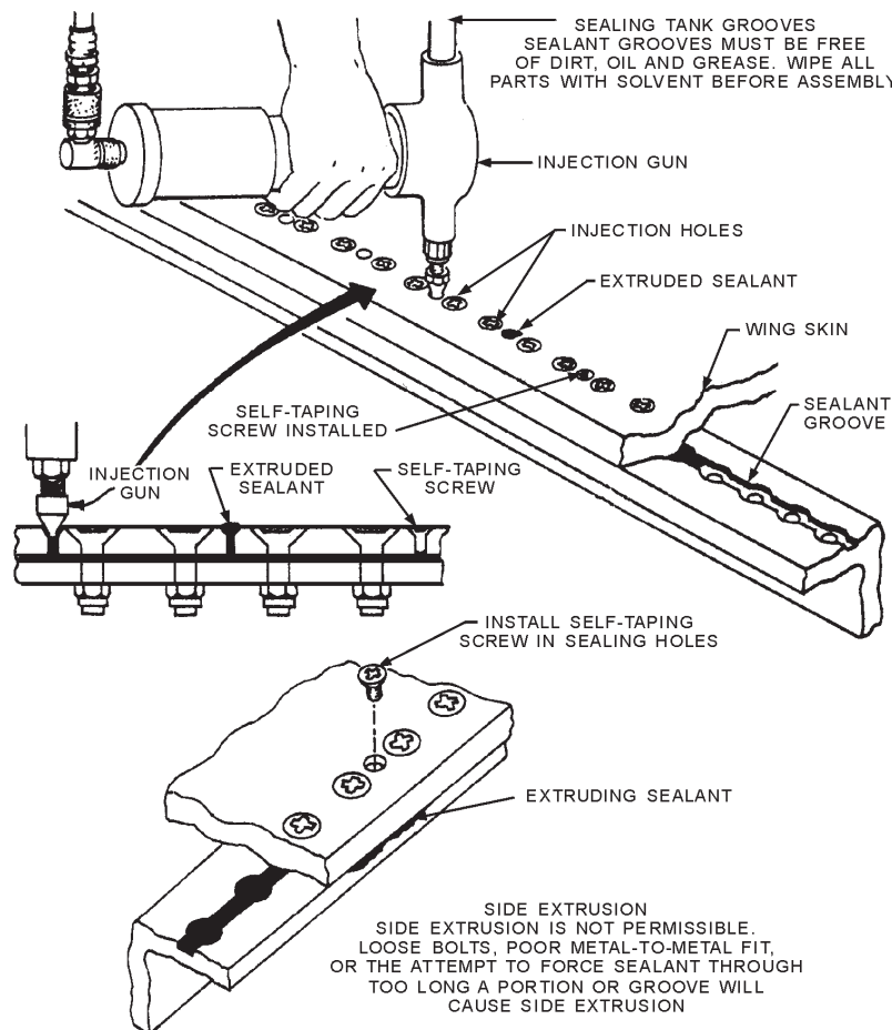
Figure 4-77.—Injection of sealing compound.
