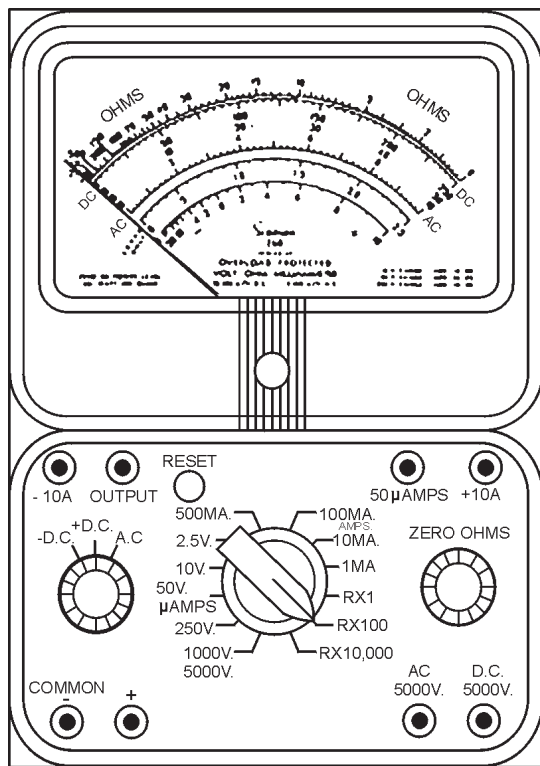
Figure 1-10.—A typical multimeter.
