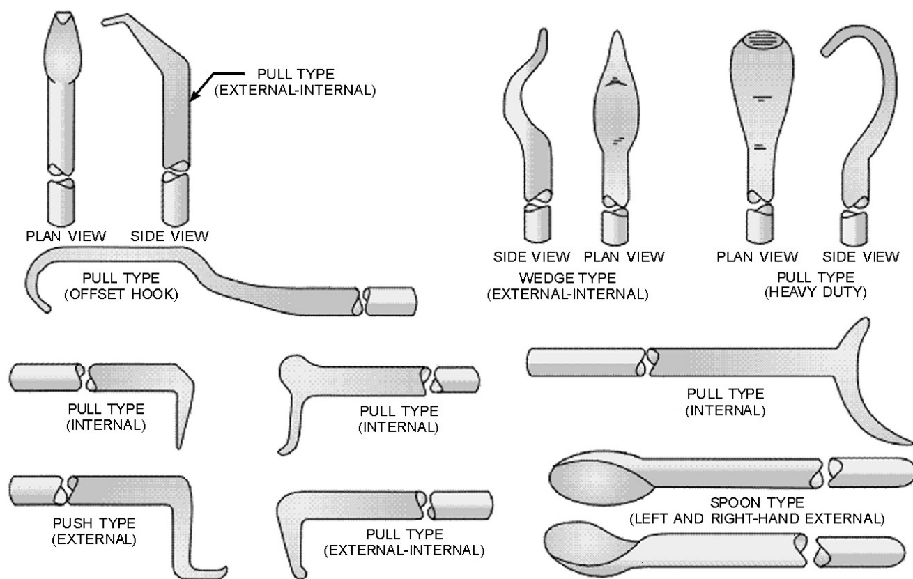
Figure 8-14.—Typical O-ring installation and removal tools.
