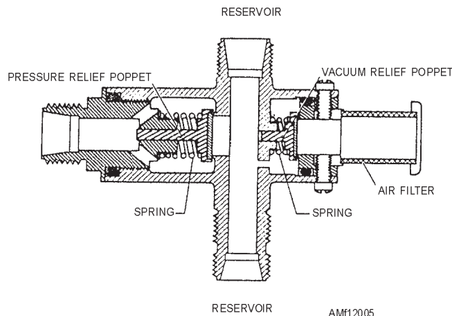
Figure 12-5.—Pressure and vacuum relief valve.
