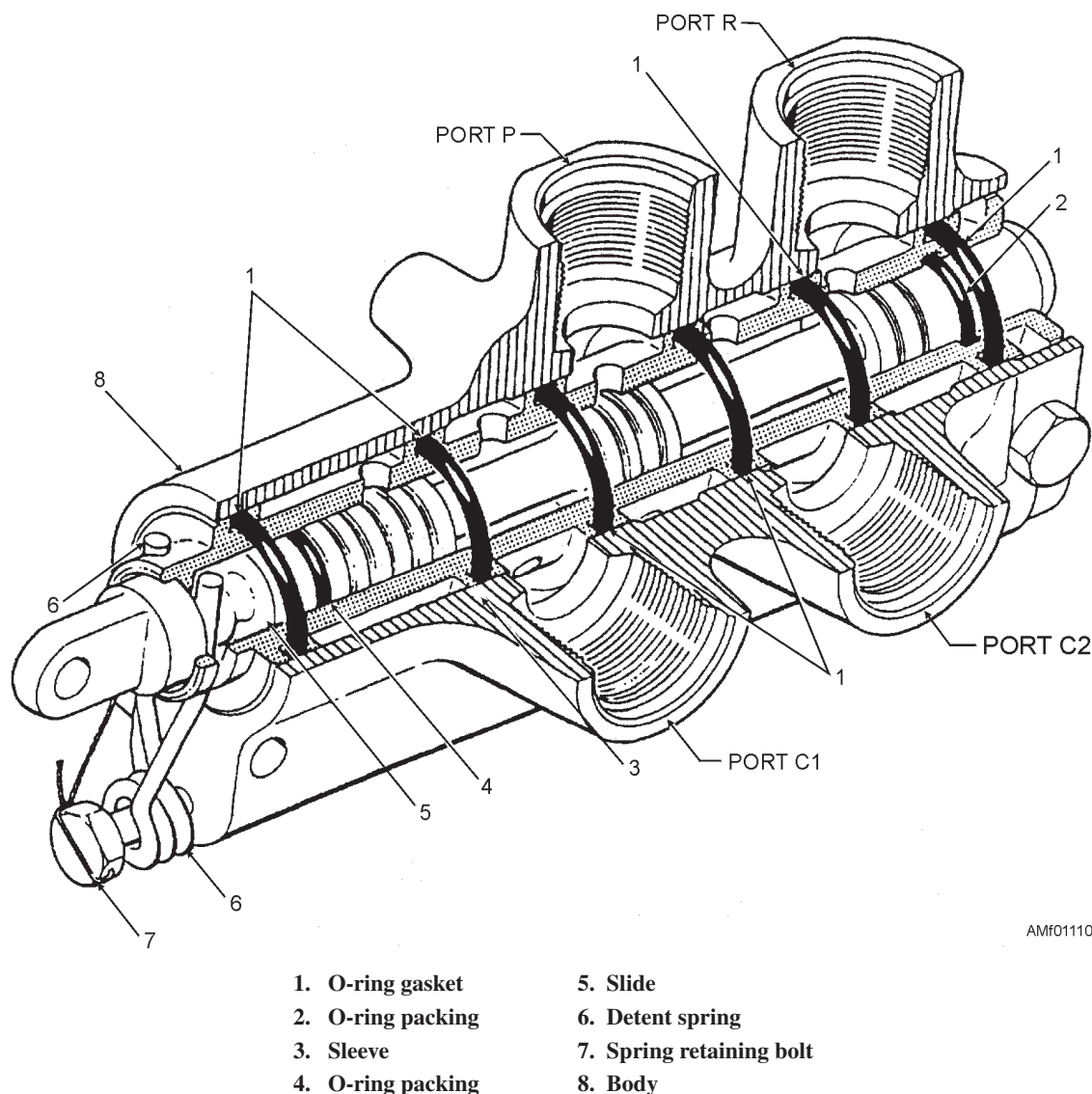
Figure 11-10.—Slide-type selector valve.
