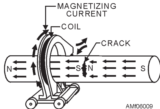
Figure 6-9.—Coil creates a longitudinal field to show crack in a part.
