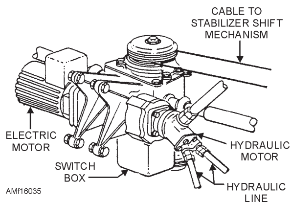
Figure 16-35.—Flap drive gearbox.
