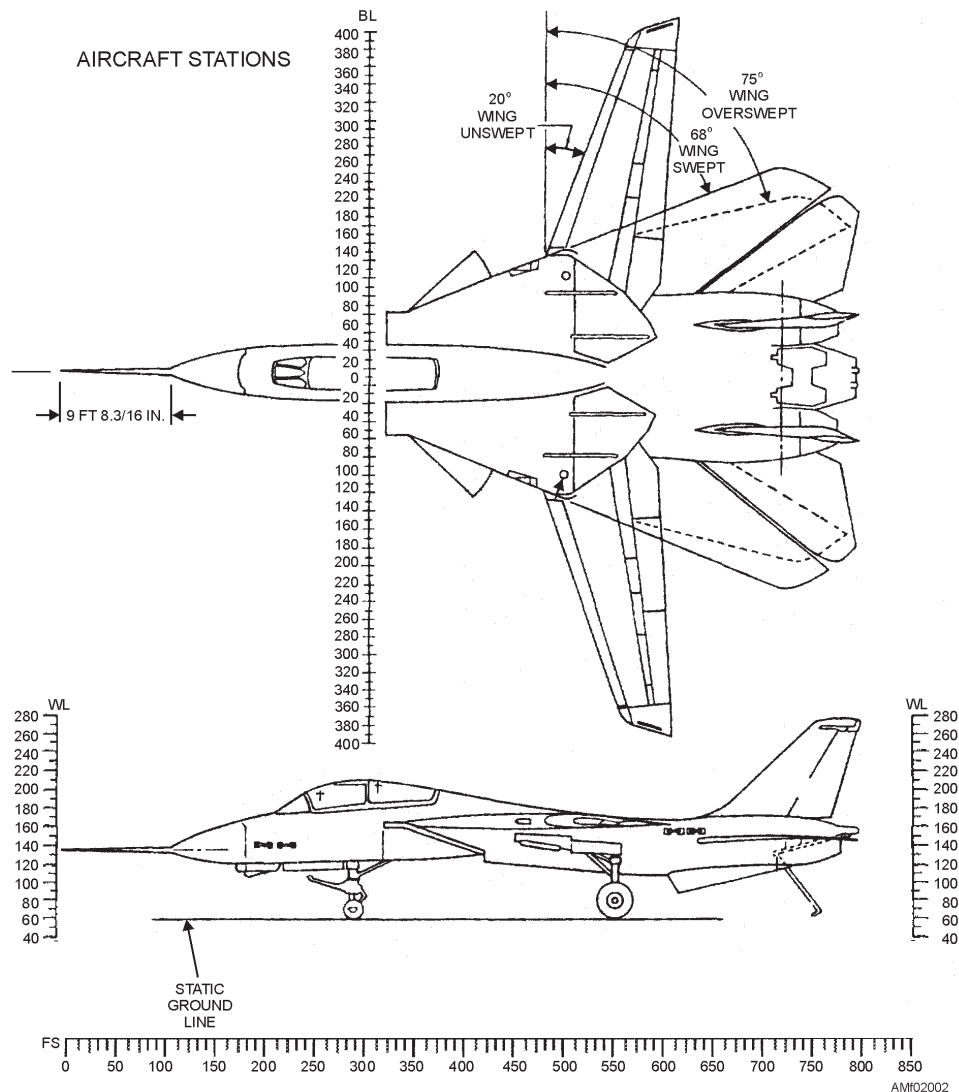
Figure 2-2.—Typical fuselage station diagram.
