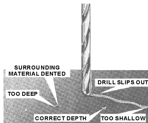
Figure 4-59.—Drilling holed for rivets.
