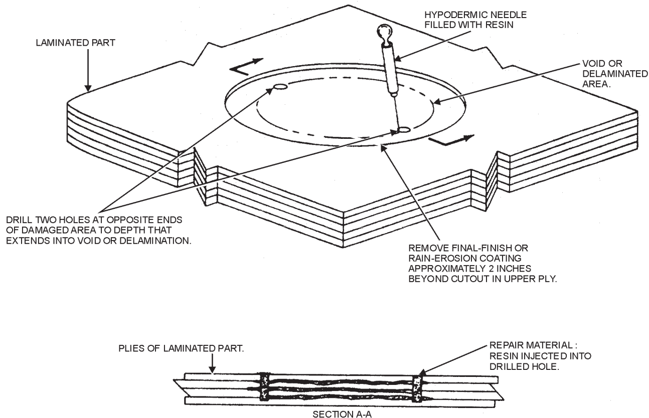
Figure 5-10.—Delaminated ply repair.
