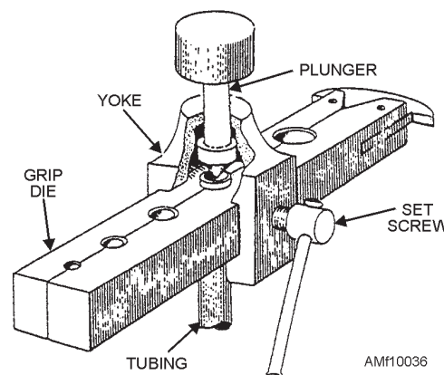
Figure 10-36.—Tube flaring tool (single-flare).
