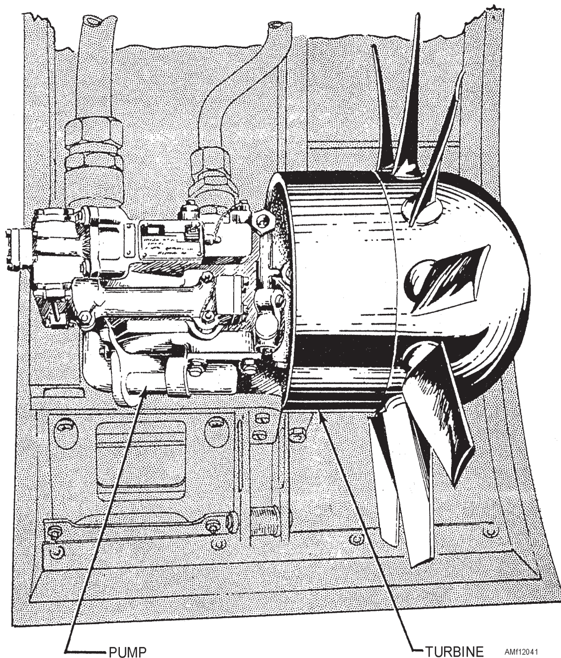
Figure 12-41.—Ram air turbine hydraulic pump assembly.
