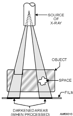
Figure 6-10.—Diagram of radiographic exposure.
