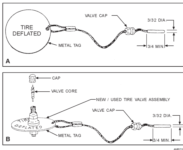
Figure 7-5.—(A) Deflated tire flag, (B) Storage of valve core and cap using alternate deflated tire flag.
