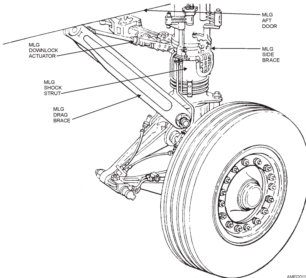
Figure 2-11.—Main landing gear.
