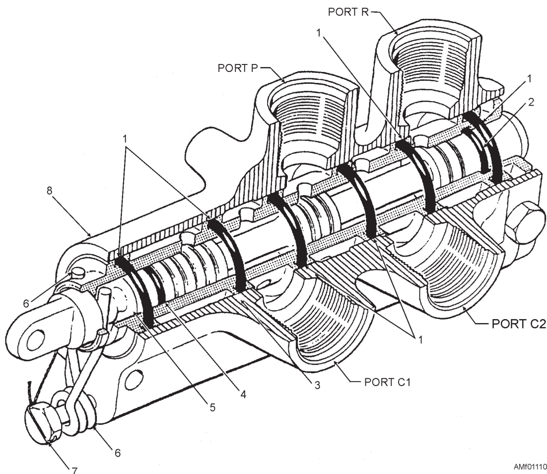
Figure 11-9.—Working view of a poppet-type selector valve.
