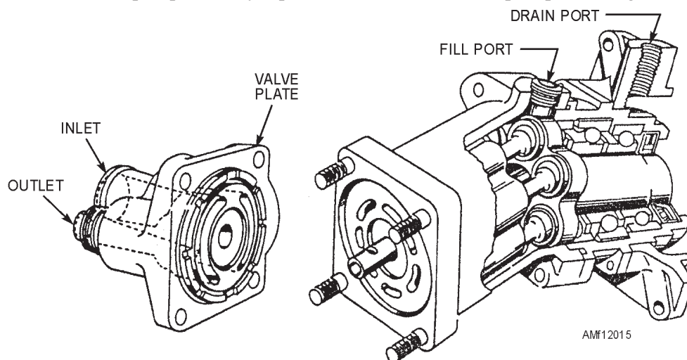
Figure 12-15.—Partial cutaway view of piston-type pump.
