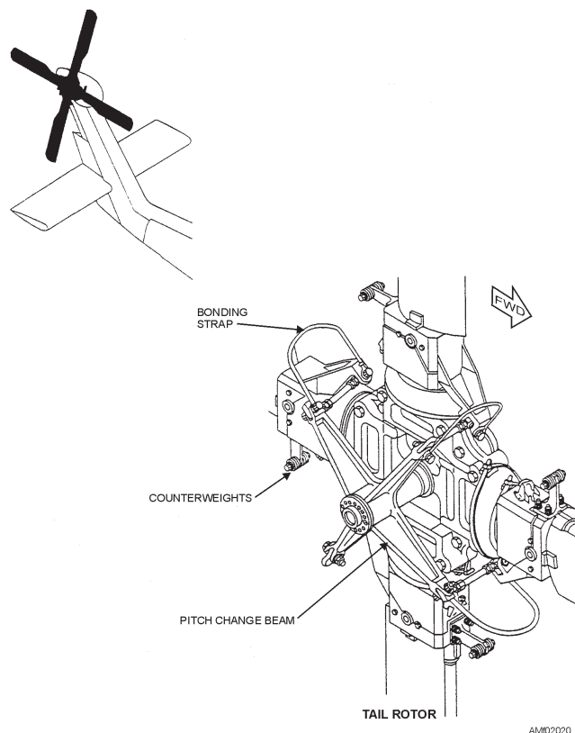
Figure 2-20.—H-60 tail rotor.
