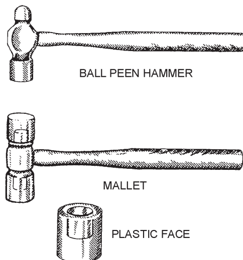
Figure 4-1.—Hammers.
