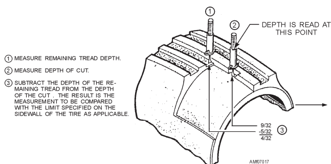
Figure 7-17.—Method of measuring depth of cuts, cracks, and holes.
