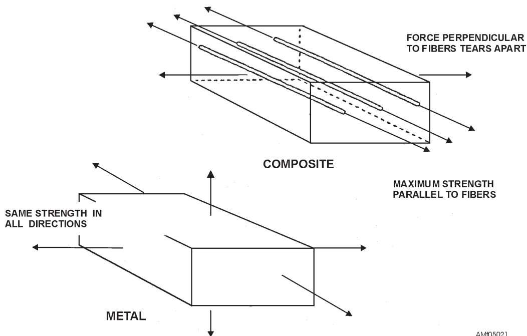
Figure 5-21.—Design properties comparison.
