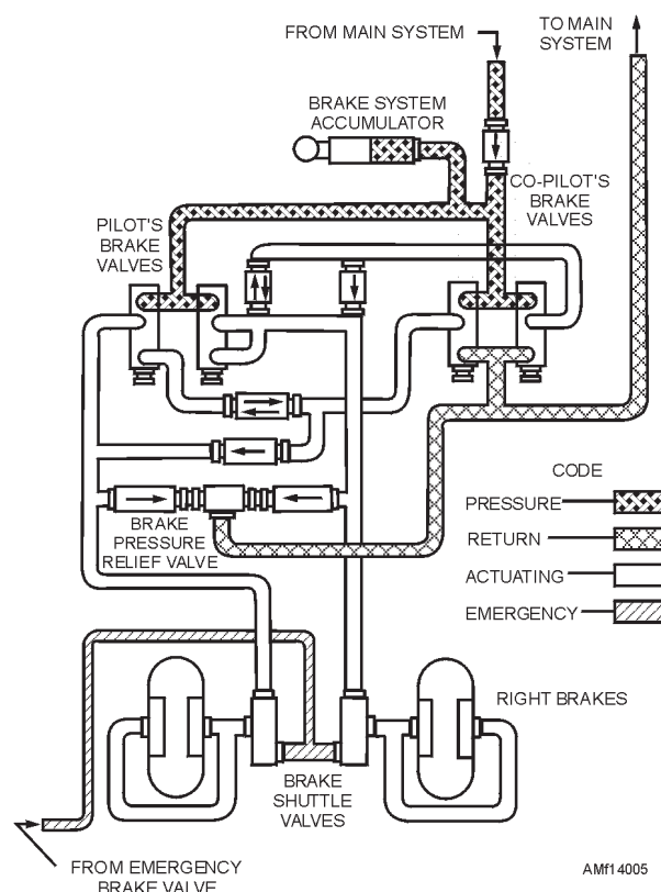
Figure 14-5.—Typical power brake control valve system.
