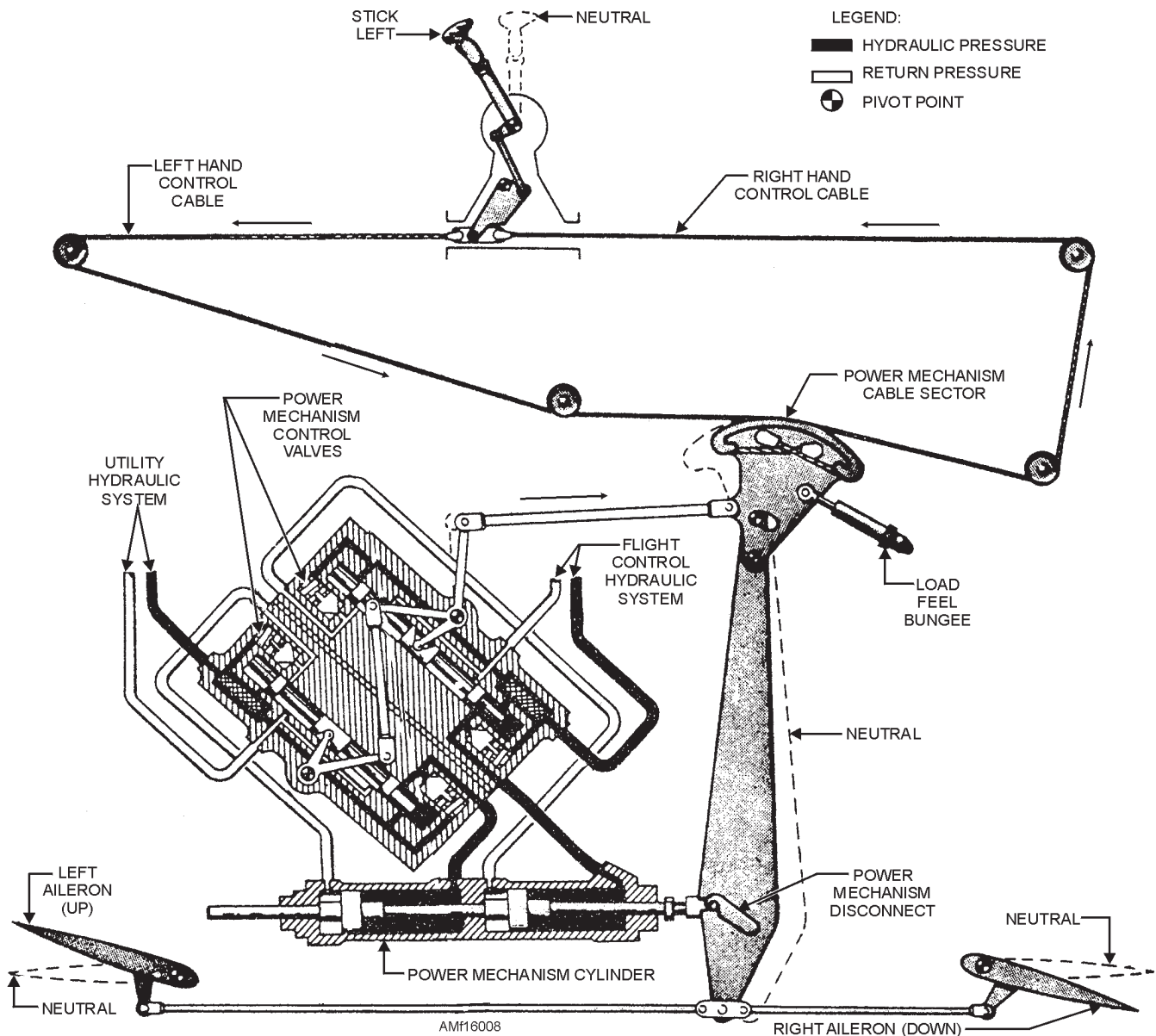
Figure 16-8.—Hydraulically powered aileron control system.
