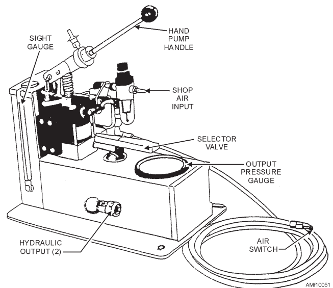
Figure 10-51.—D10004 Permaswage hydraulic power supply.
