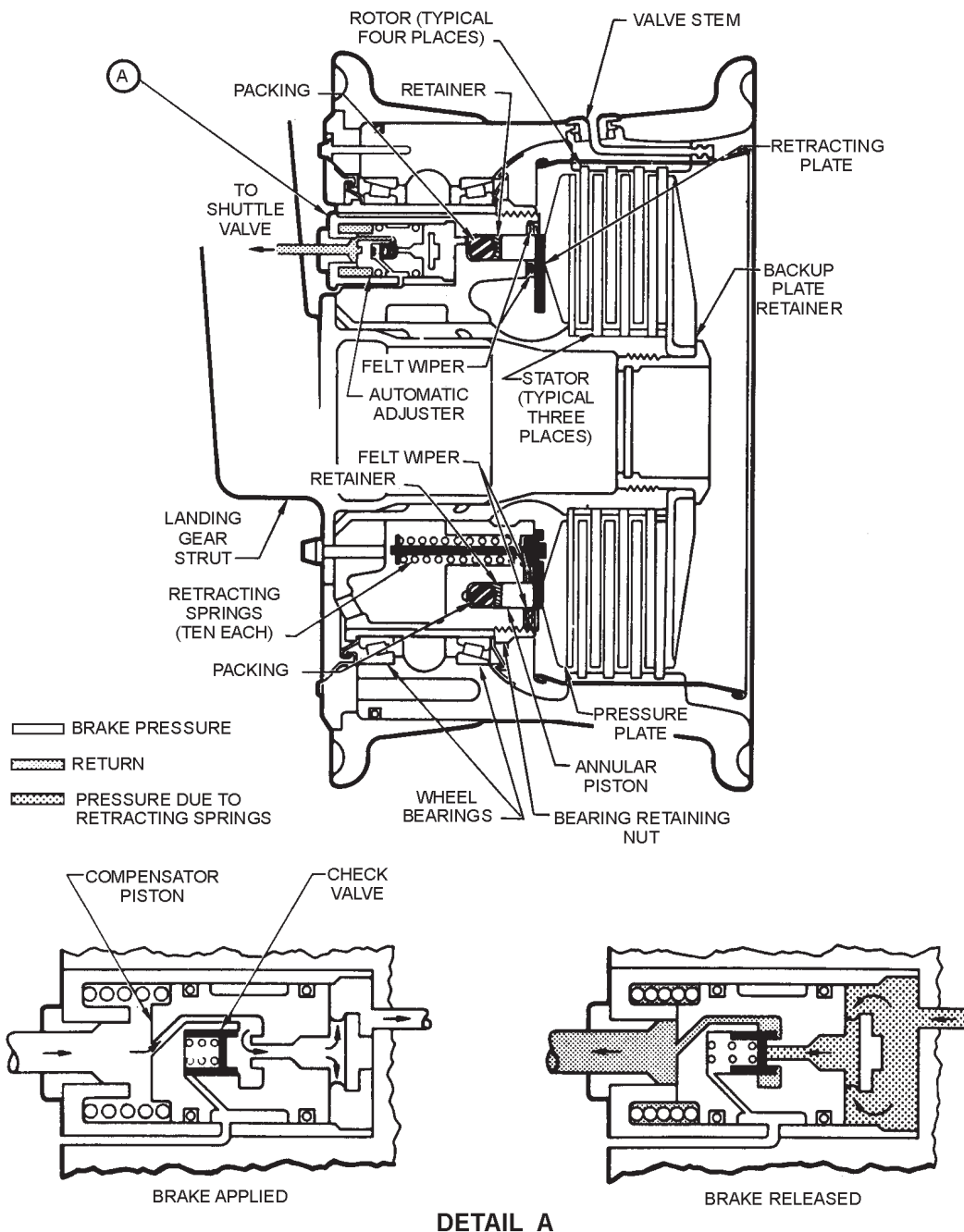
Figure 14-12.—Cross-sectional view of multiple disc brake.
