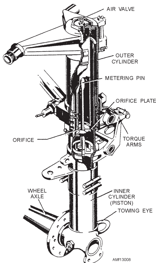
Figure 13-8.—Landing gear shock strut (metering pin type).
