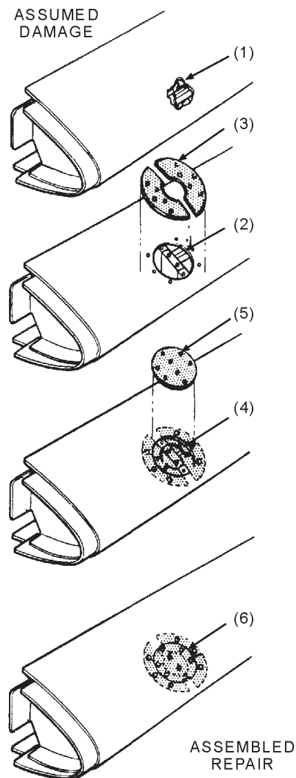
Figure 4-62.—Flush patch over internal structure.
