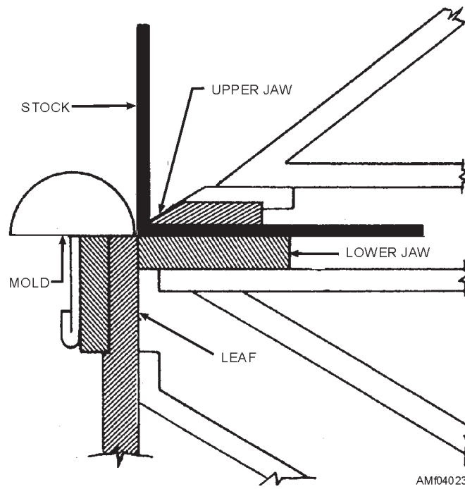
Figure 4-23.—Cornice brake with mold and stock.
