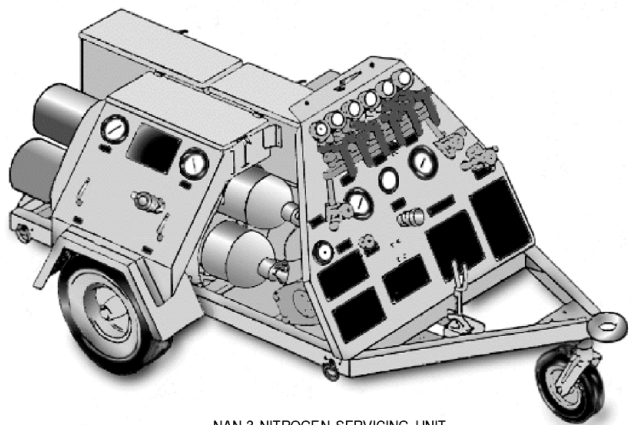
NAN-3 NITROGEN SERVICING UNIT
