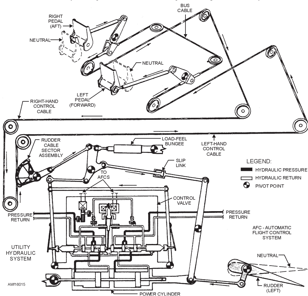
Figure 16-15.—Rudder control system.
