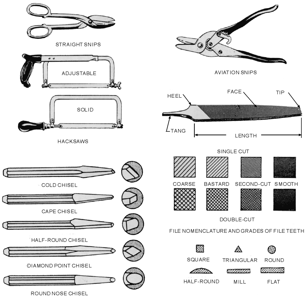
Figure 4-8.—Types of cutting tools.
