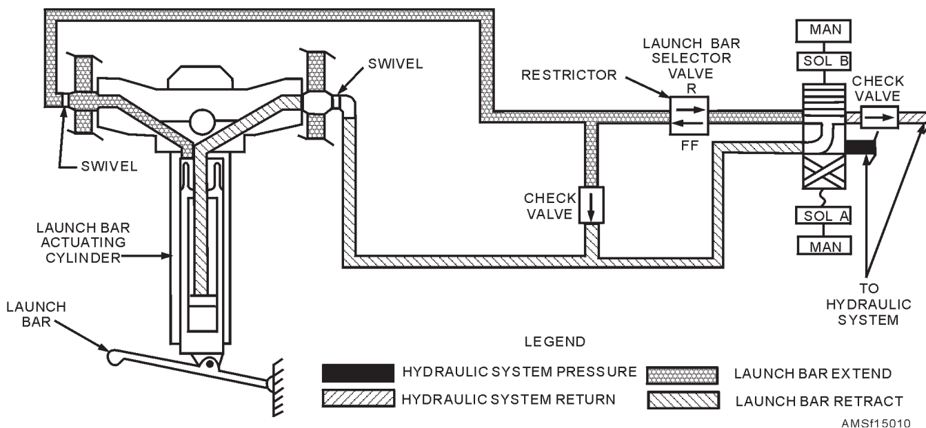
Figure 15-10.—Catapult system hydraulic schematic.
