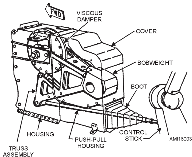
Figure 16-3.—Elevator forward bobweight and damper assembly.
