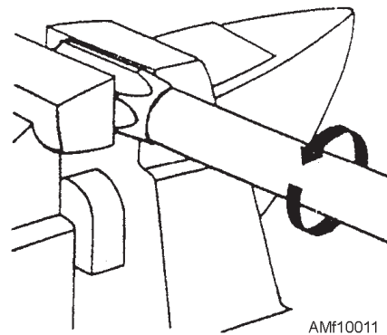
Figure 10-11.—Hose insertion.
