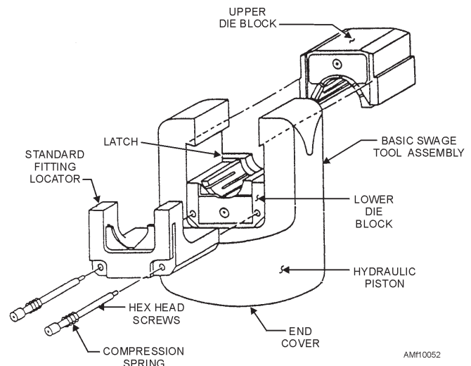
Figure 10-52.—Basic swage tool assembly.
