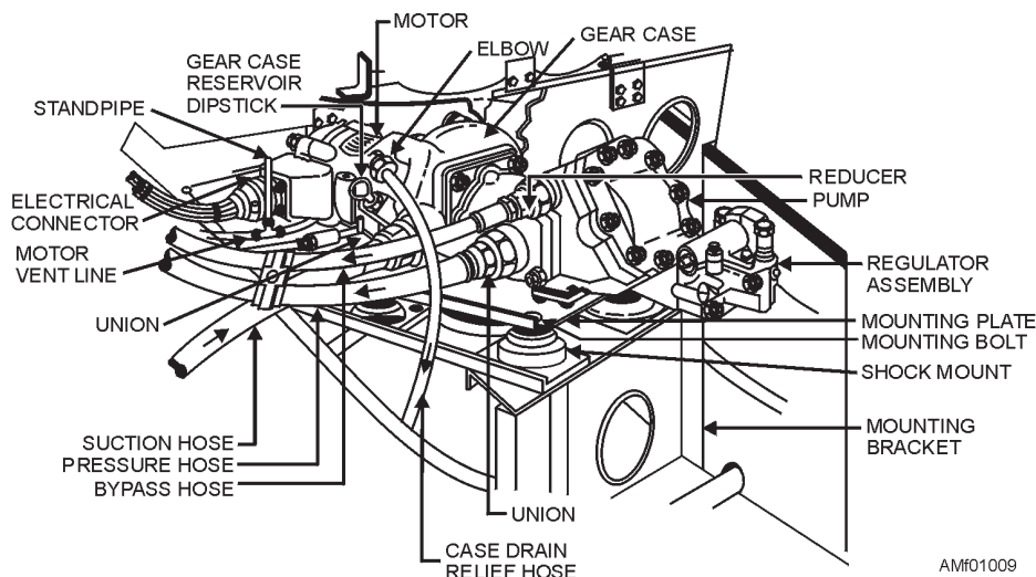
Figure 1-9.—Installation diagram of a motor-driven hydraulic pump.
