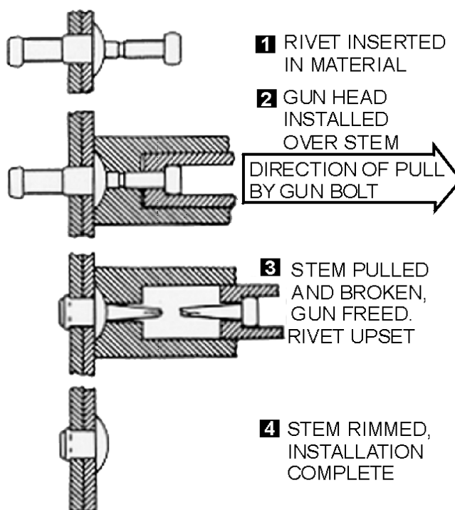
Figure 3-4.—Self-plugging rivet (friction lock).
