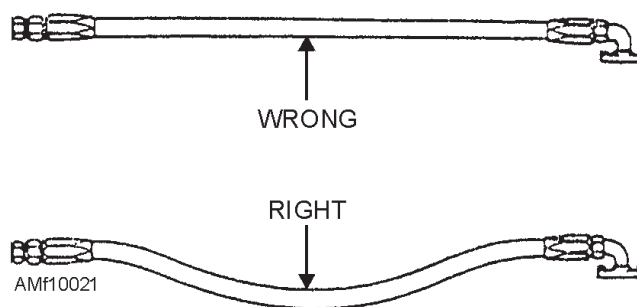
Figure 10-21.—Hose slack.
