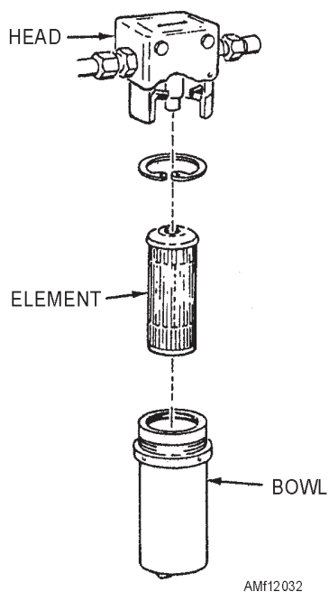
Figure 12-32.—Hydraulic filter assembly.
