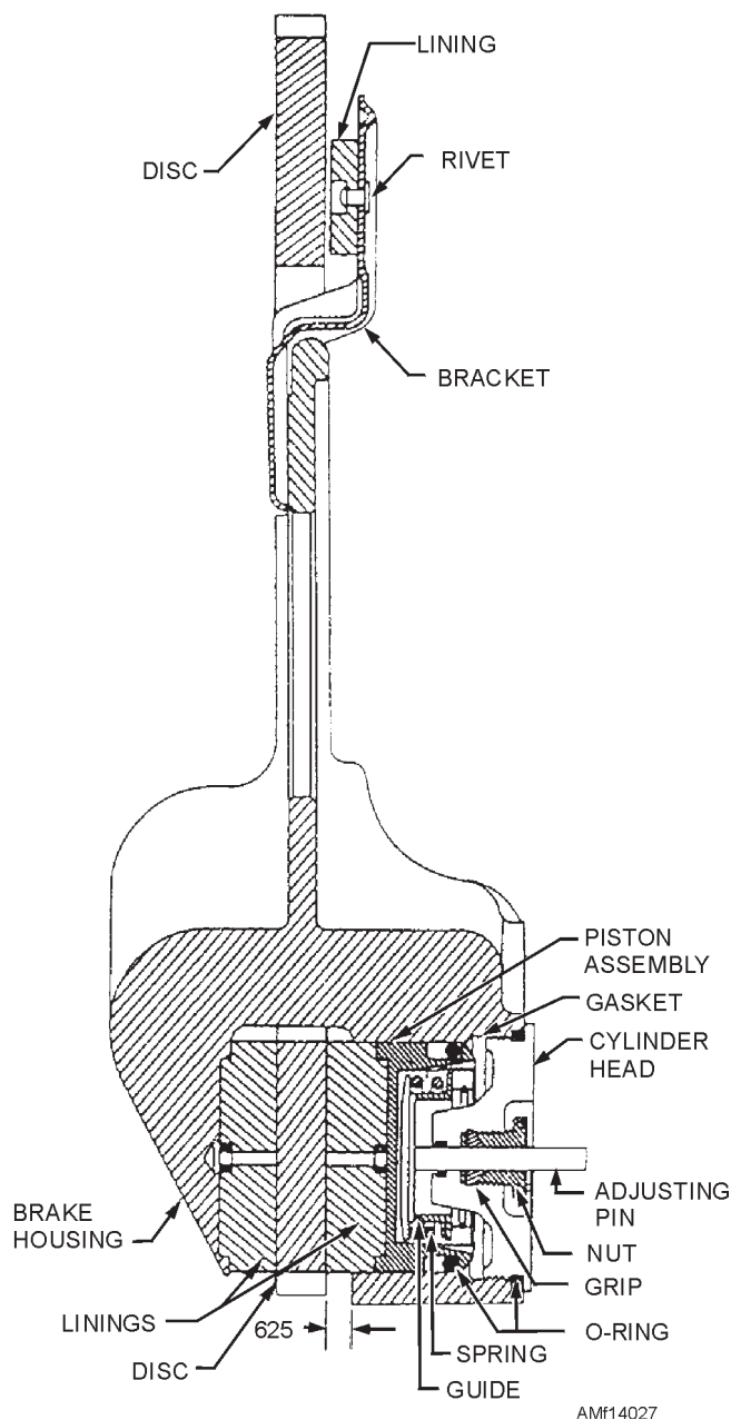
Figure 14-27.—Cross-sectional view of a single disc brake assembly with captured torquing-type automatic adjuster.
