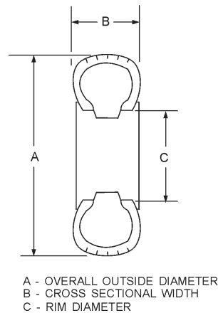
Figure 7-12.—Size designation of tires.
