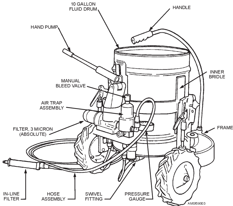
Figure 9-3.—Model 310 fluid service cart.
