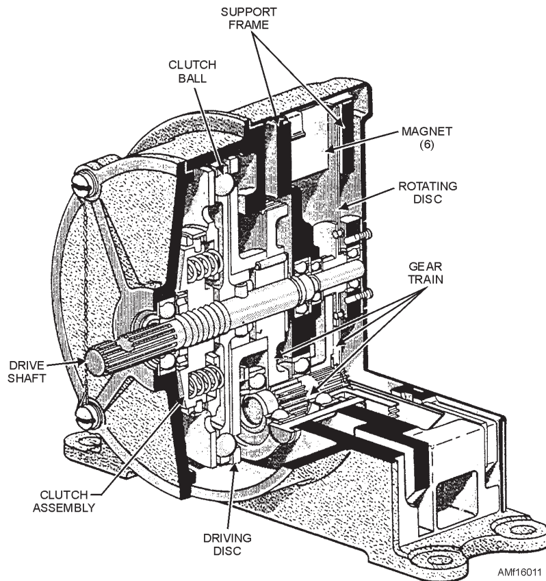
Figure 16-11.—Eddy current damper.
