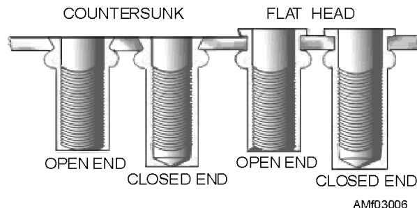
Figure 3-6.—Sectional view of rivnut showing head and end designs.
