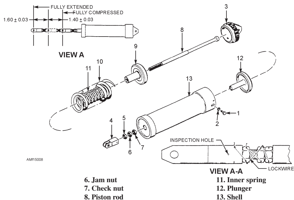
Figure 15-7.—Arresting gear assembly.
