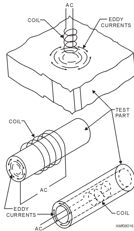
Figure 6-16.—Generation of eddy currents in various part configurations.
