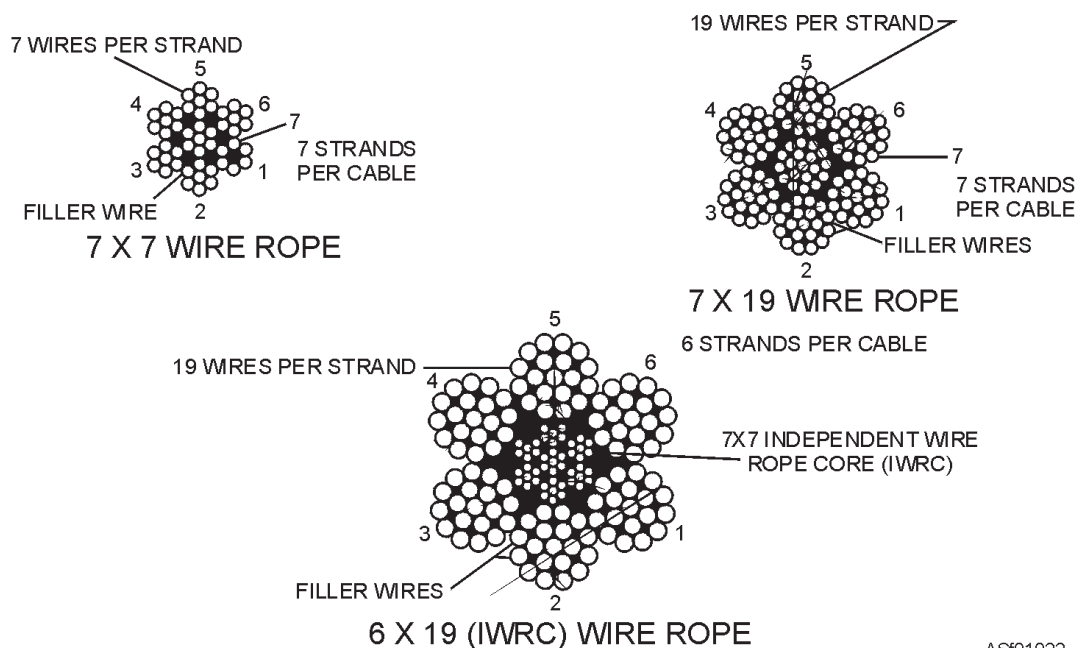
Figure 1-22.—Cross sections of wire rope.
