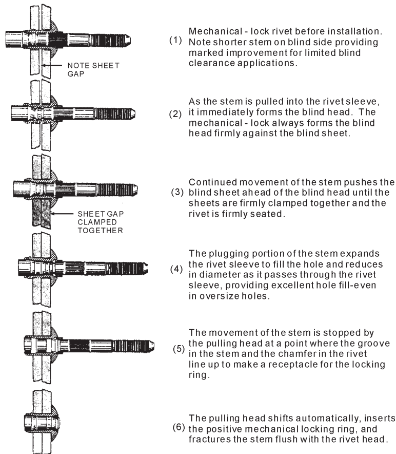
Figure 4-53.—Self-plugging rivet (mechanical lock).
