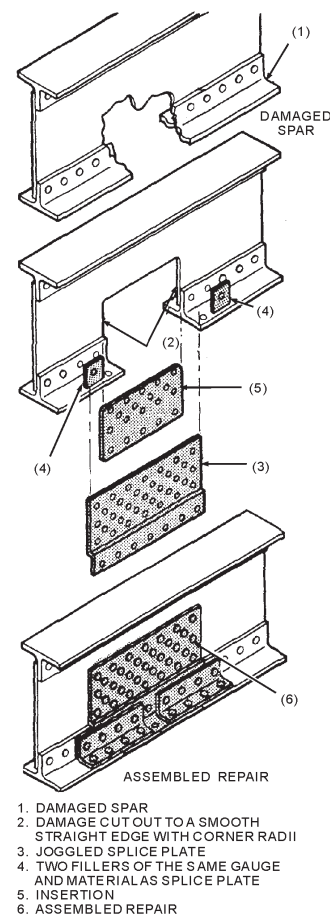
Figure 4-69.—Spar repair by insertion.
