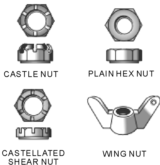
Figure 3-17.—Nuts.
