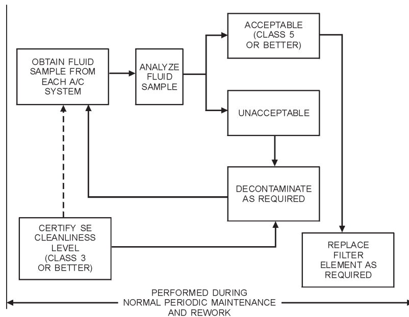
Figure 8-1.—Periodic fluid surveillance requirements.
