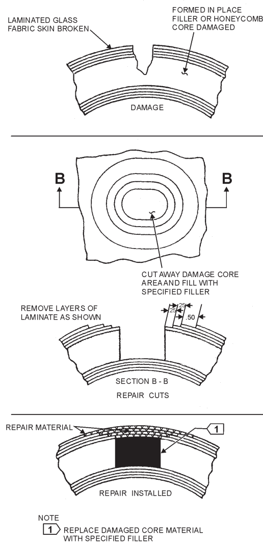
Figure 5-12.—Foam-type core repair.
