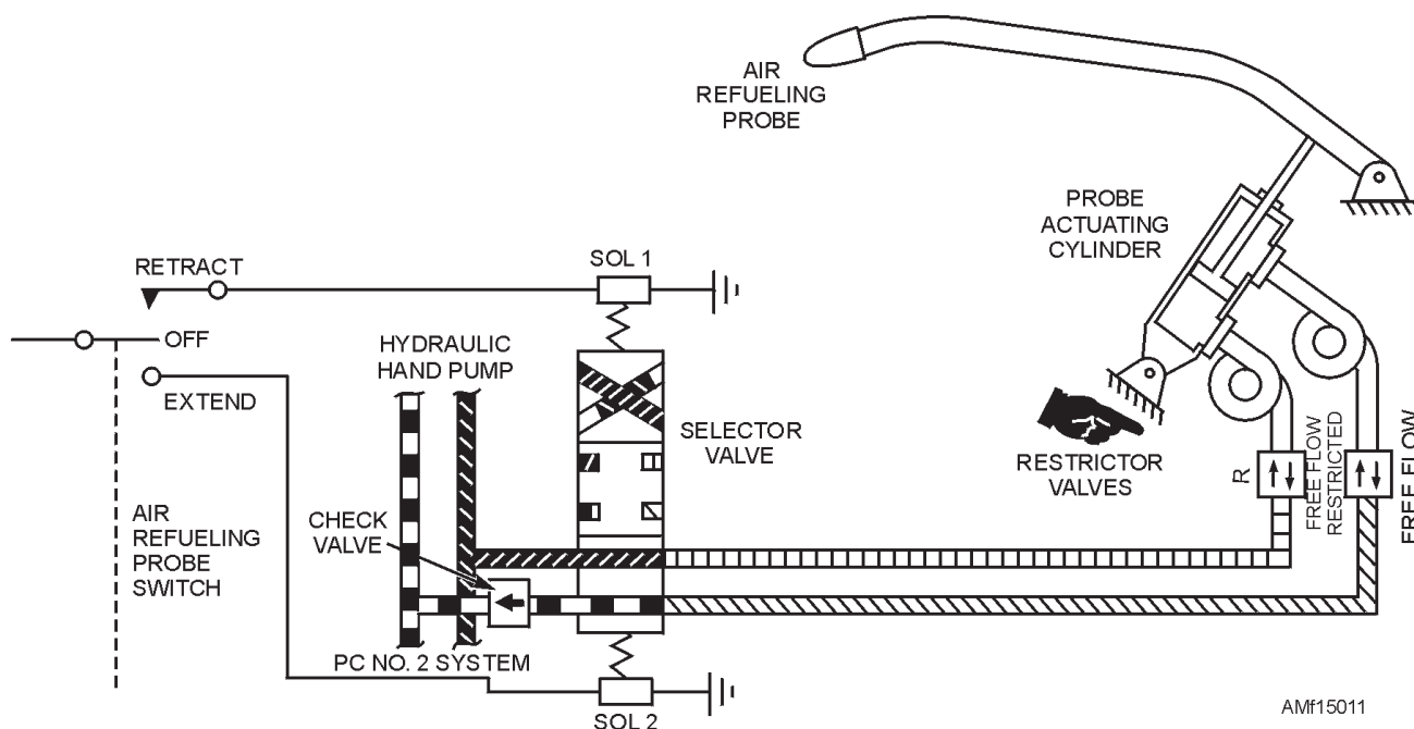
Figure 15-11.—Air refueling probe hydraulic system.
