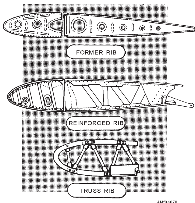
Figure 4-70.—Types of ribs.
