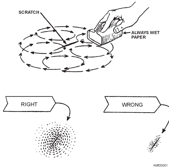
Figure 5-1.—Proper method of sanding plastic.
