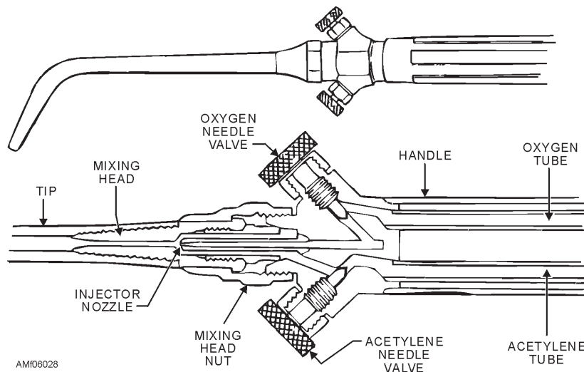
Figure 6-28.—Mixing head for injector-type welding torch.
