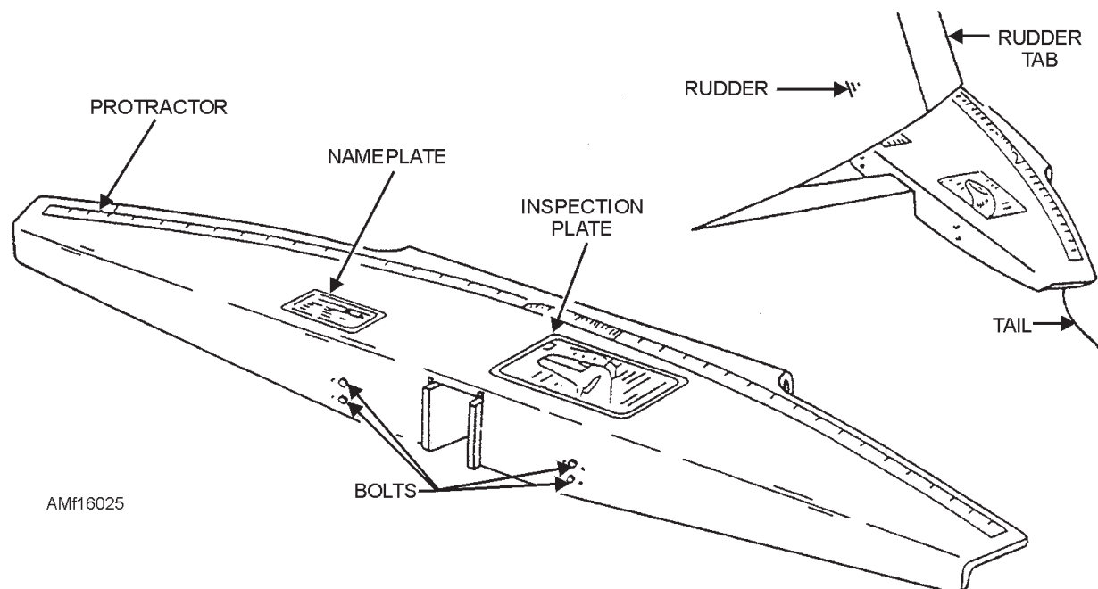
Figure 16-25.—Typical throwboard used for rigging rudder and rudder tab controls.
