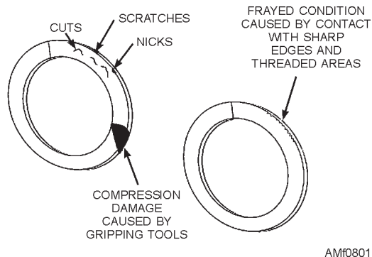
Figure 8-17.—Teflon® backup ring damages caused by improper handling.
