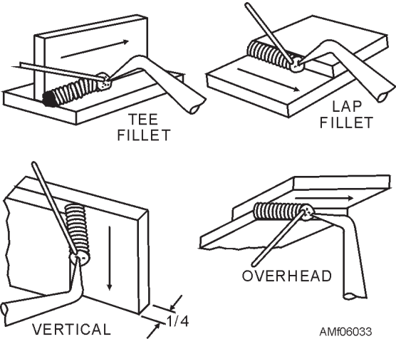
Figure 6-33.—Backhand welding.
