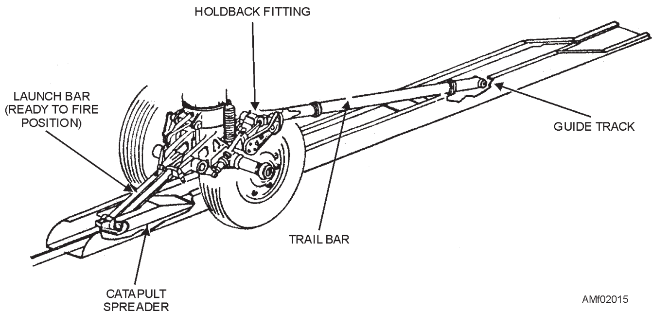
Figure 2-15.—Nose gear launch equipment.
