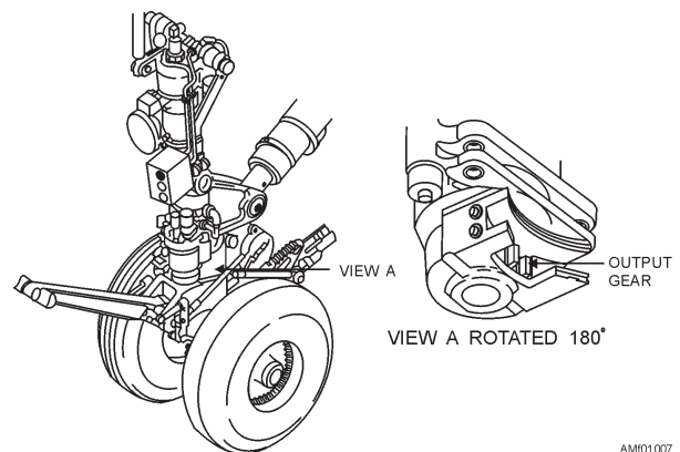
Figure 1-7.—Pictorial drawing with exploded view.
