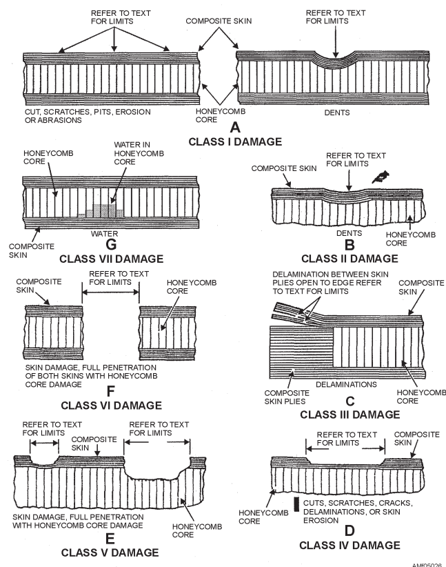
Figure 5-26.—Example of repairable damage on composite material.
