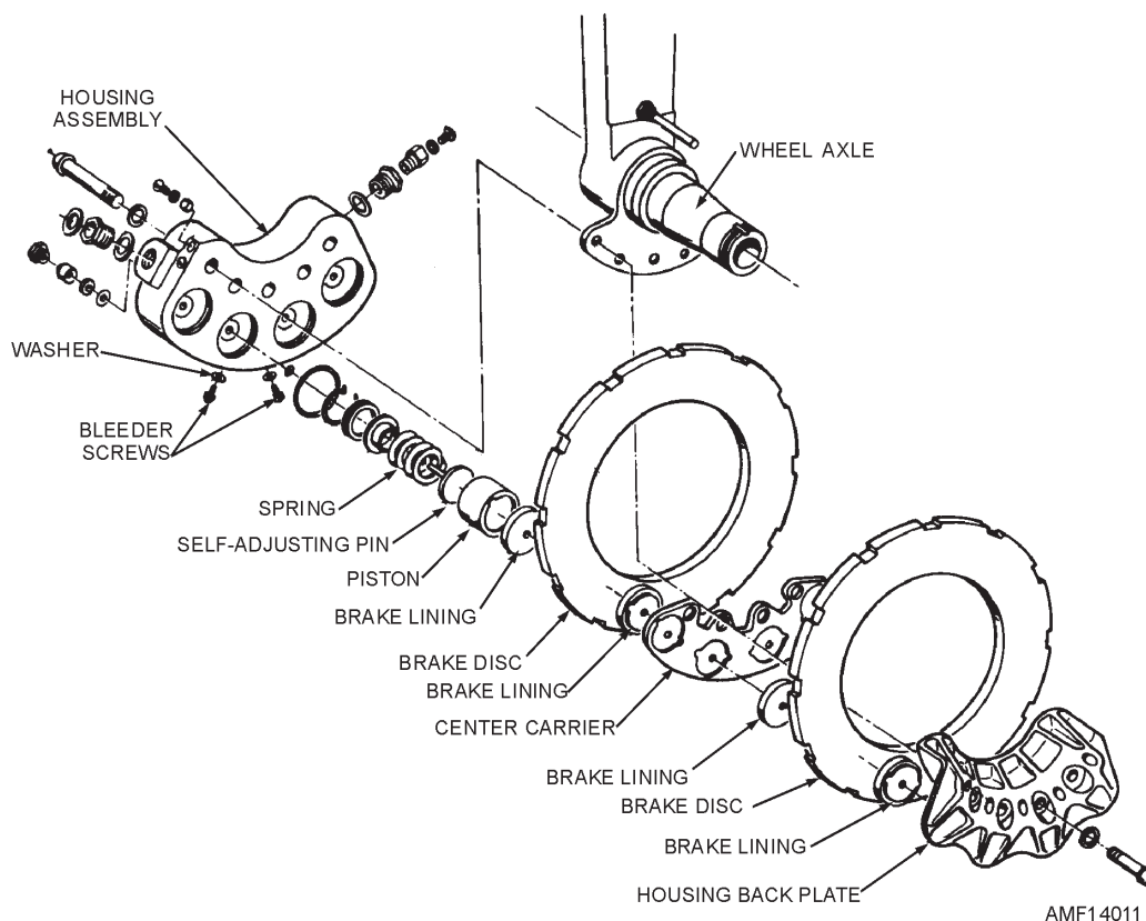
Figure 14-11.—Dual disc brake.
