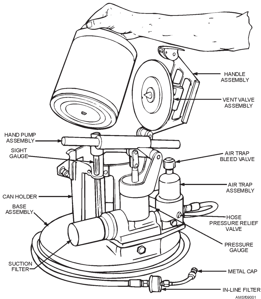
Figure 9-1.—Insertion of can into Hydraulic Servicing Unit H-250-1.
