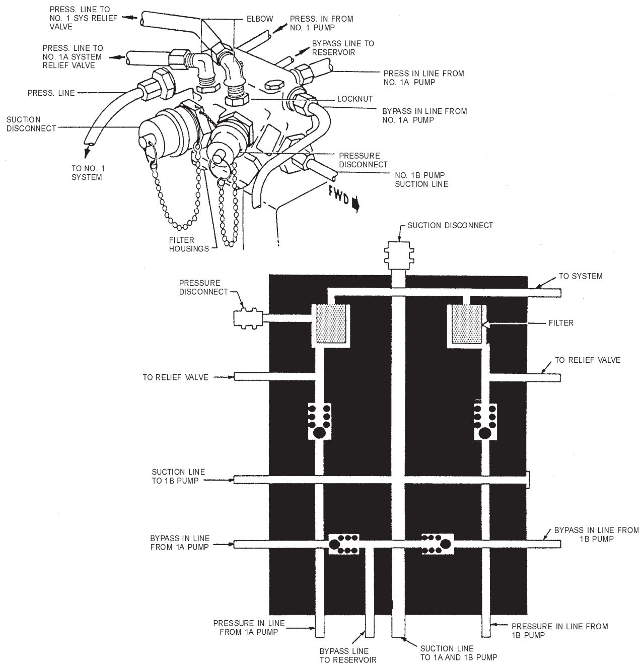
Figure 12-30.—Hydraulic manifold assembly.
