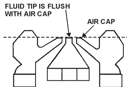
Figure 5-34.—Suction and pressure fluid tips and air caps.
