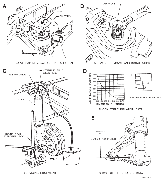
Figure 13-15.—Servicing a landing gear strut.
