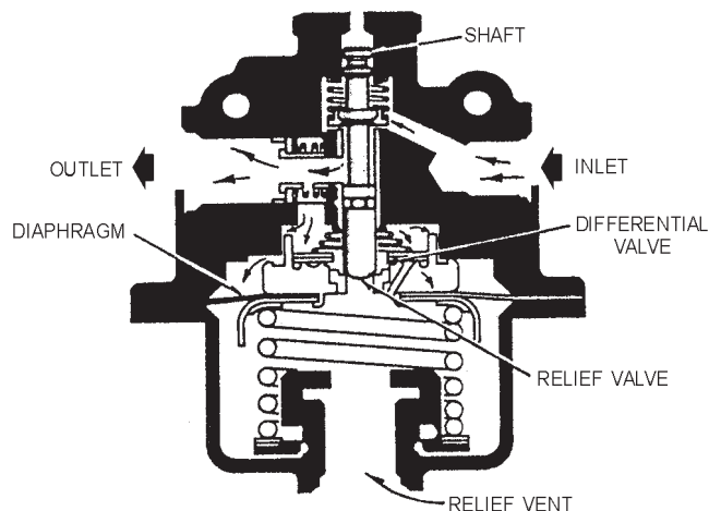
Figure 12-9.—Air pressure regulator.
