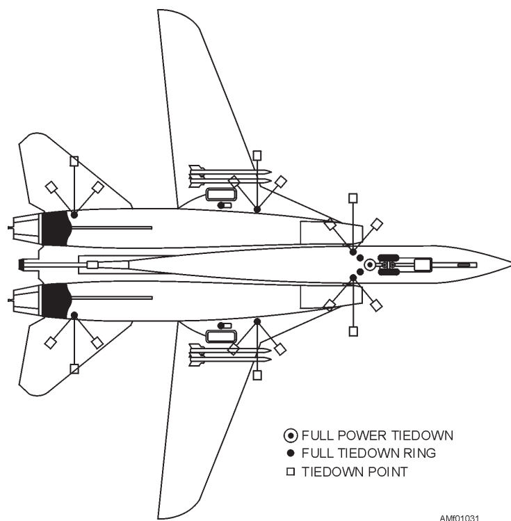
Figure 1-31.—Carrier tie-downs for aircraft jacking.
