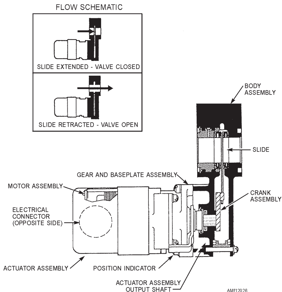
Figure 12-26.—Motor operated shutoff valve.
