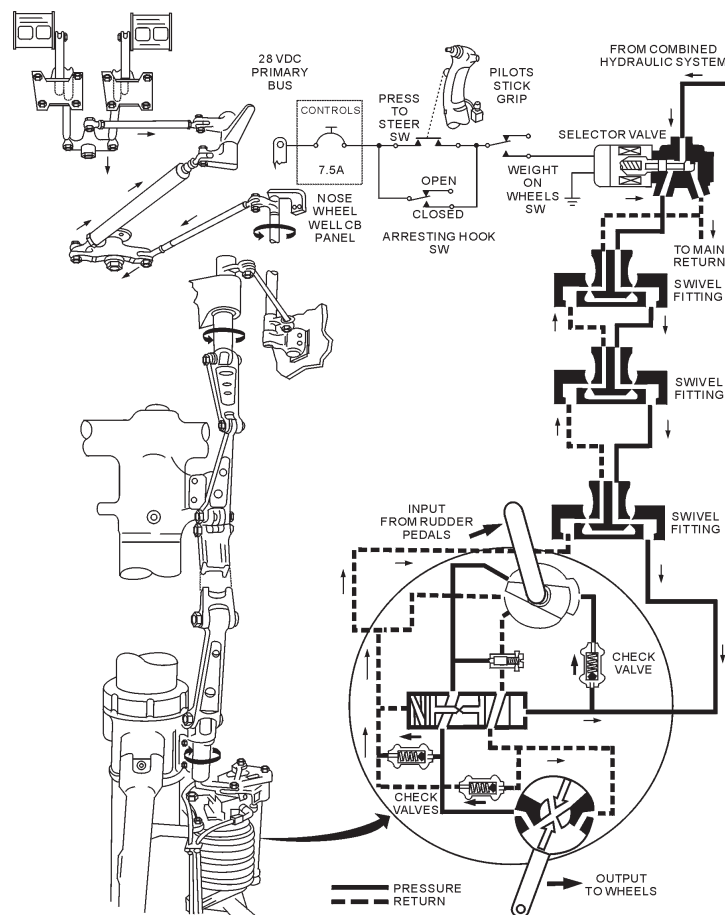
Figure 15-4.—Nosewheel steering system.
