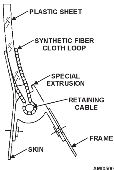
Figure 5-7.—Typical loop edge attachment.
