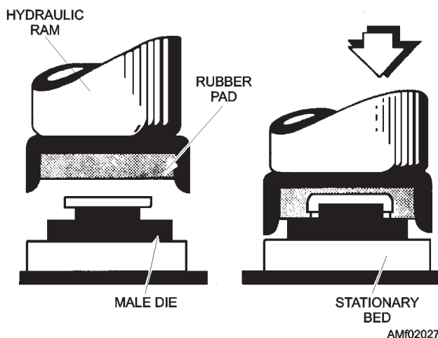
Figure 2-27.—Guerin process.
