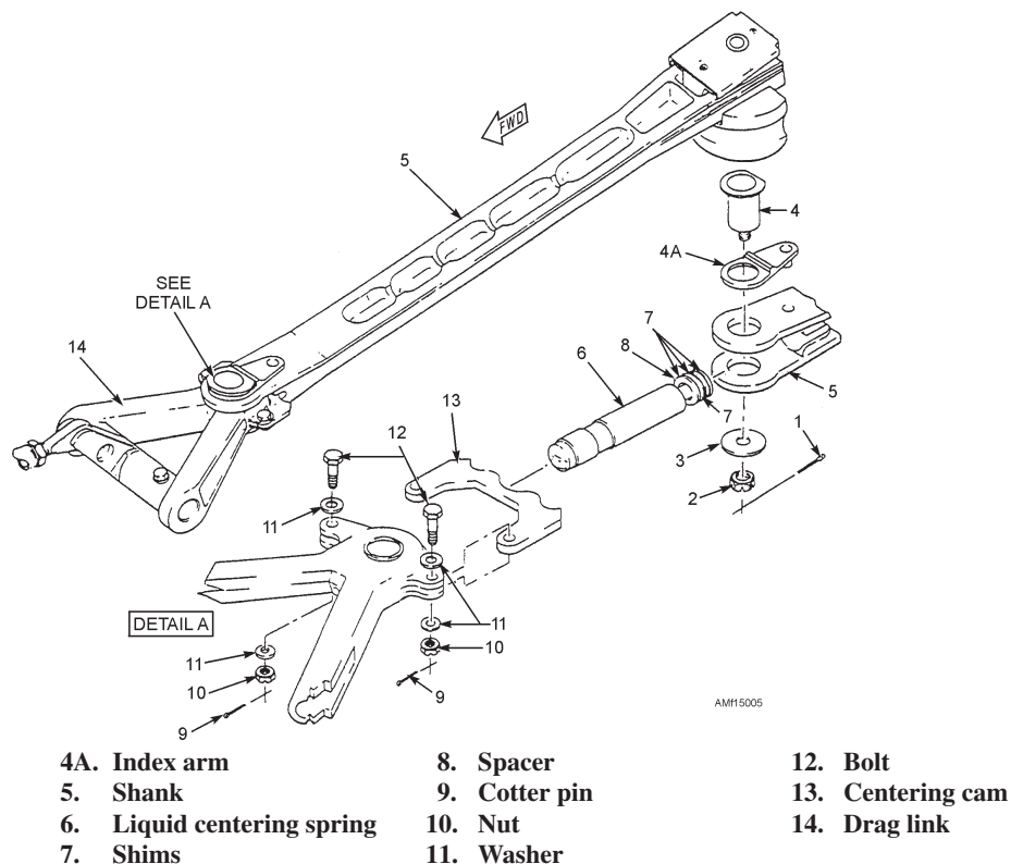
Figure 15-5.—Arresting gear mechanism.
