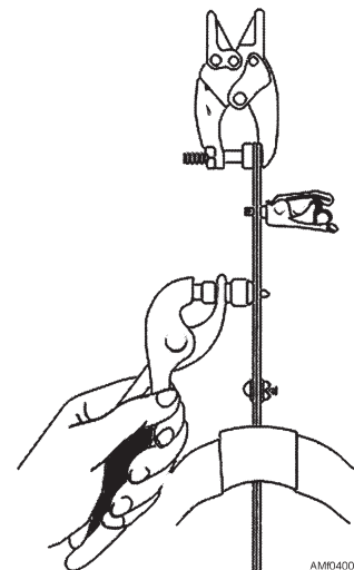
Figure 4-6.—Skin fasteners.
