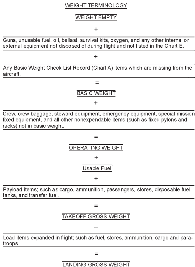
Figure 1-16.—Weight terminology.
