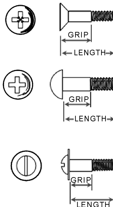
Figure 3-21.—Structural screws.
