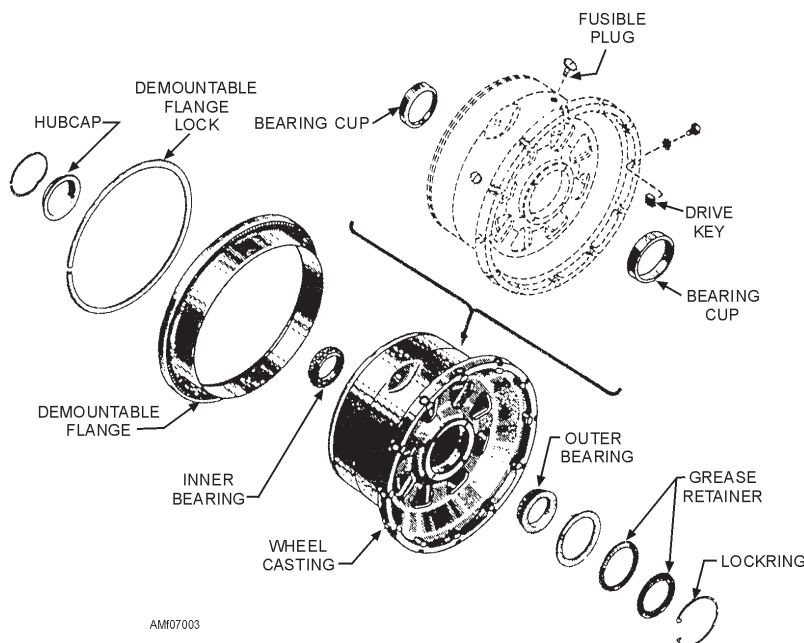
Figure 7-3.—Typical wheel assembly.
