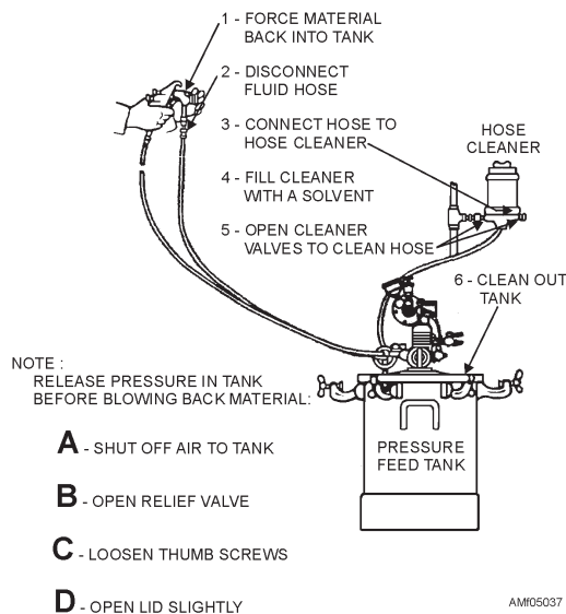
Figure 5-37.—Cleaning pressure-feed spray gun.
