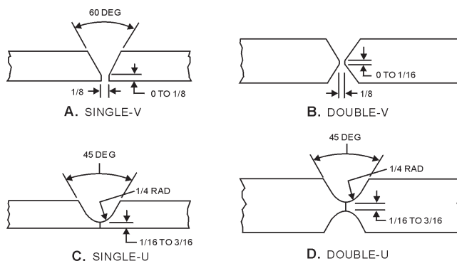
Figure 6-37.—Butt joints in heavy sections.
