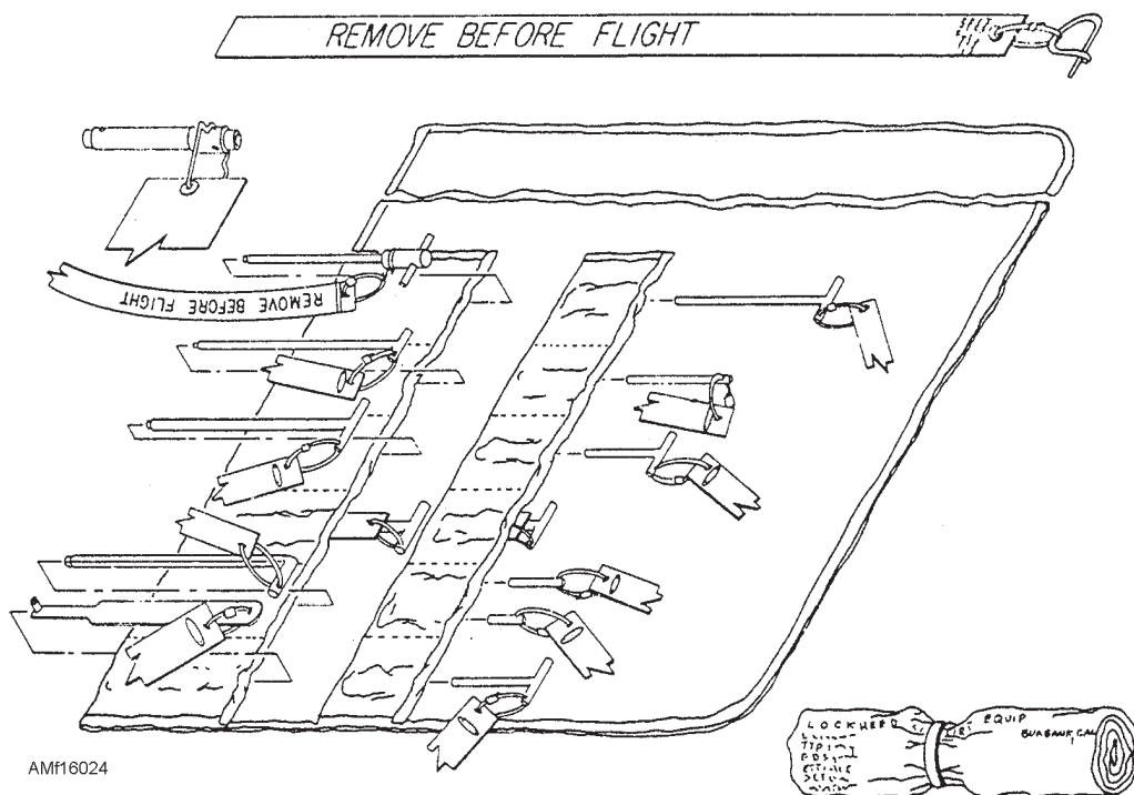
Figure 16-24.—Rigging pin set.
