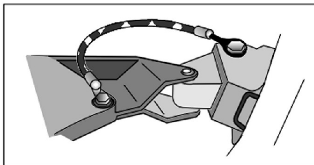
Figure 3-41.—Typical bonding link installation.
