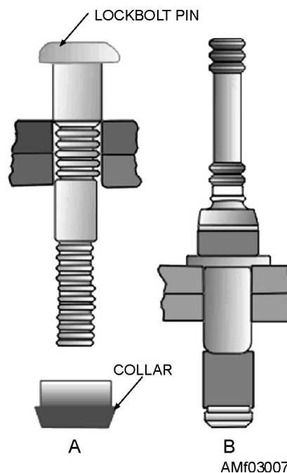
Figure 3-7.—Lock bolts.
