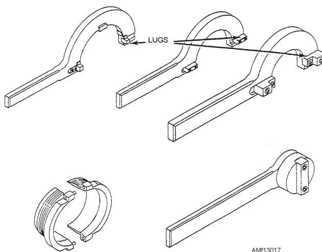
Figure 13-17.—Landing gear shock strut tools.
