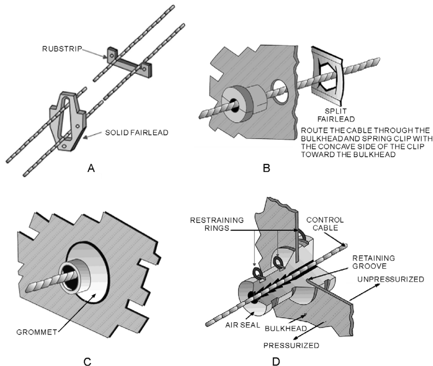
Figure 3-37.—Typical cable guides.
