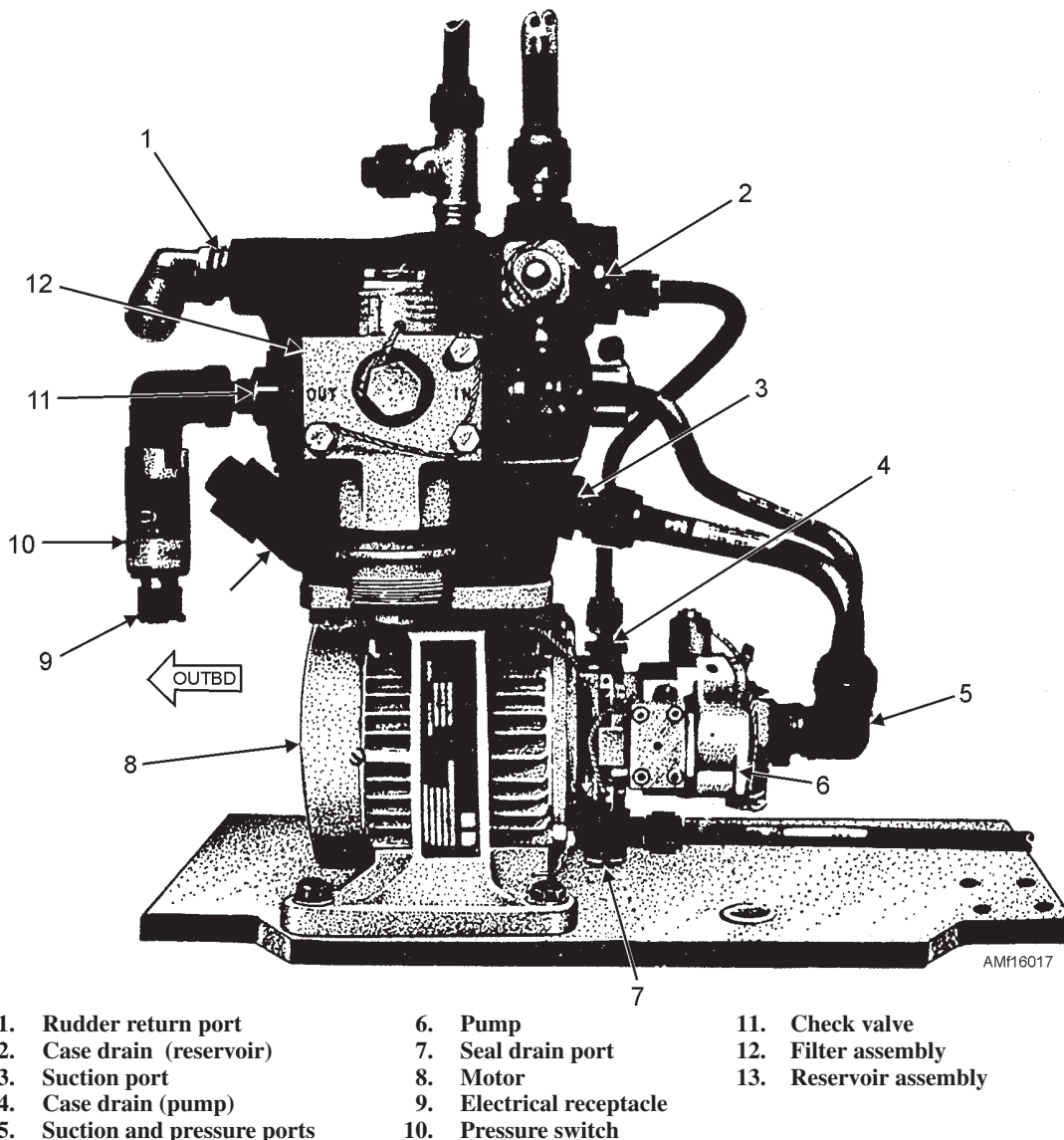
Figure 16-17.—Backup flight control hydraulic system.
