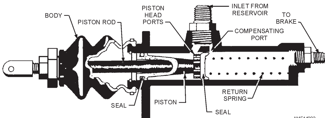
Figure 14-2.—Goodyear master brake cylinder.
