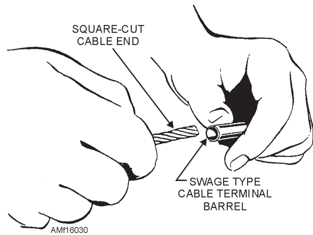
Figure 16-30.—Inserting cable in swage terminal.
