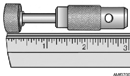
Figure 7-4.—Safe-core valve tool.
