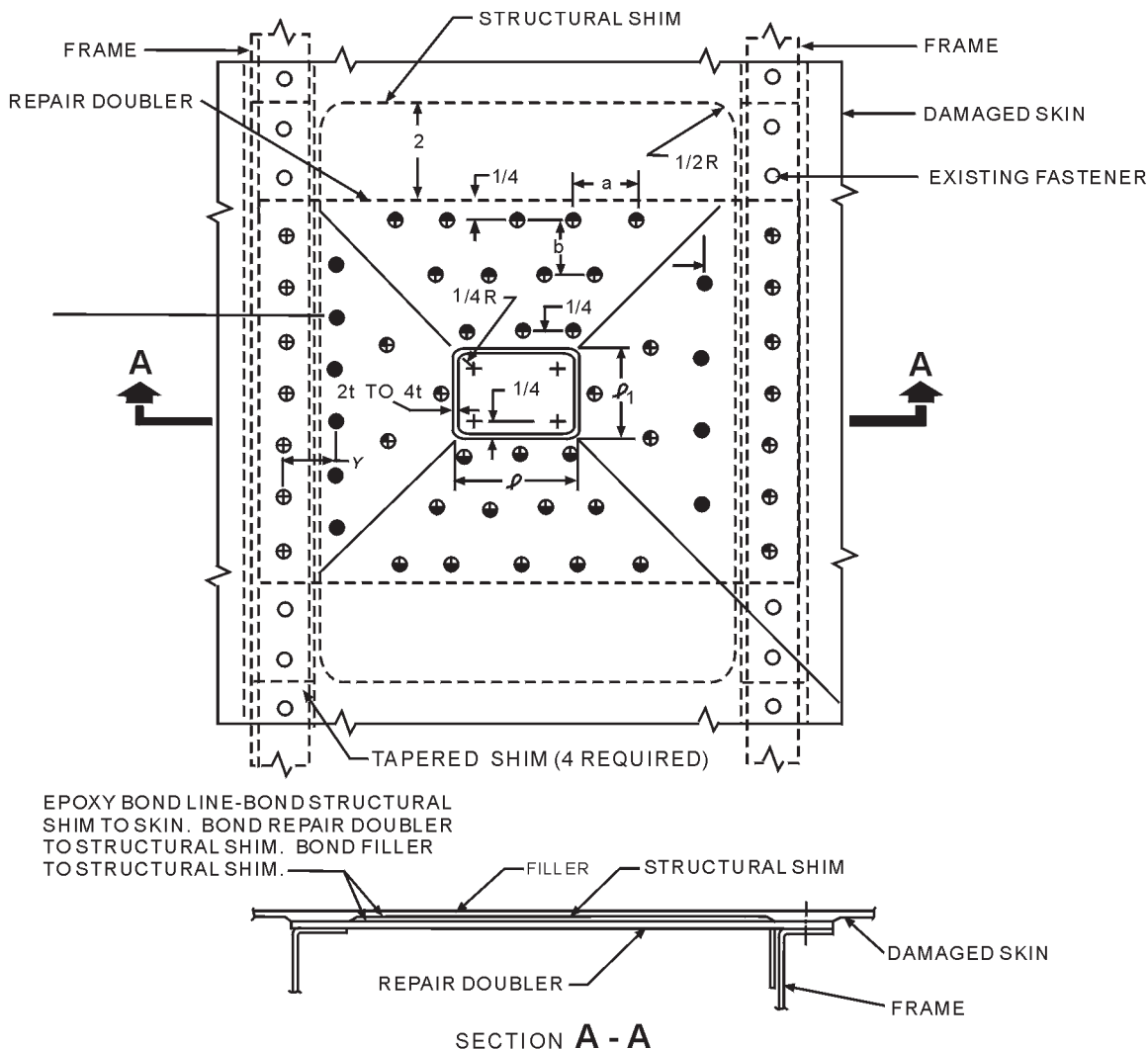
Figure 4-63.—Chem-Milled skin repair (fuselage pressurized).
