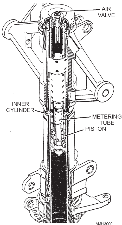
Figure 13-9.—Landing gear shock strut (metering tube type).
