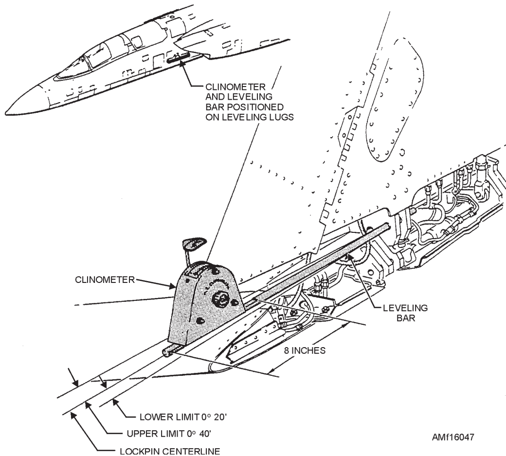
Figure 16-47.—Alignment data—wing twist check.
