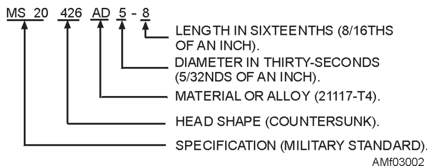
Figure 3-2.—Rivet coding example.
