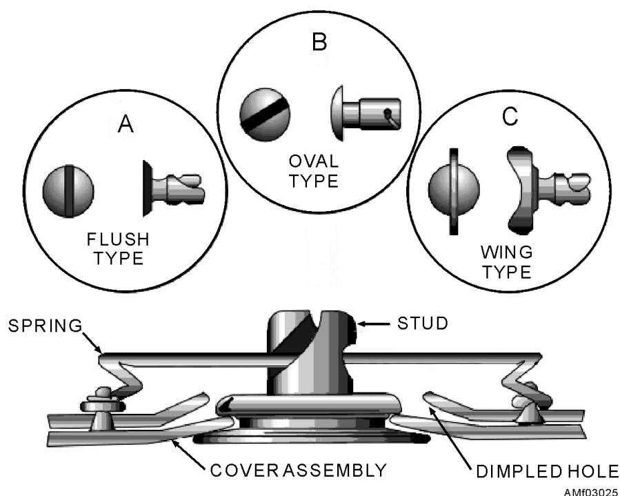
Figure 3-25.—Dzus fastener.
