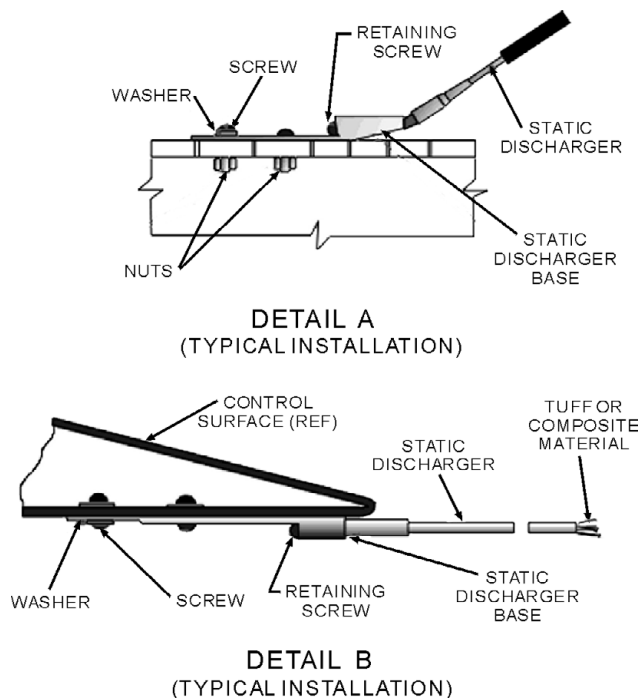
Figure 3-42.—Typical static dischargers.
