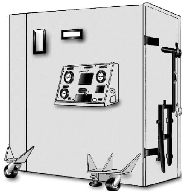
Figure 7-24.—Inflation safety cage with aircraft tire inflator/monitor attached.
