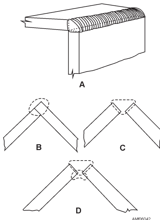
Figure 6-42.—Corner joints for sheets and plates.
