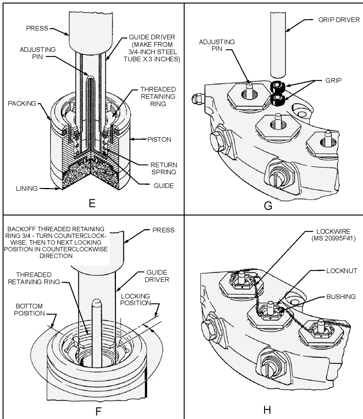
Figure 14-31.—Seal replacement and piston return adjustment—Continued.
