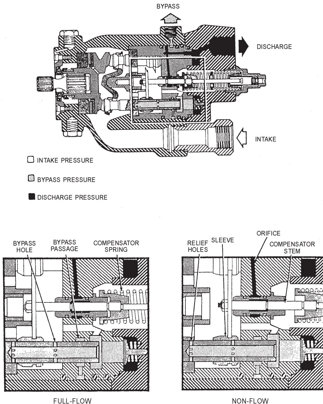
Figure 12-20.—Fluid flow.
