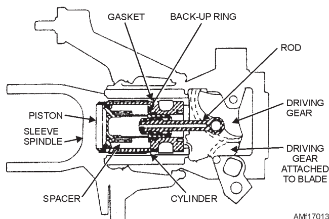
Figure 17-13.—Blade fold cylinder.
