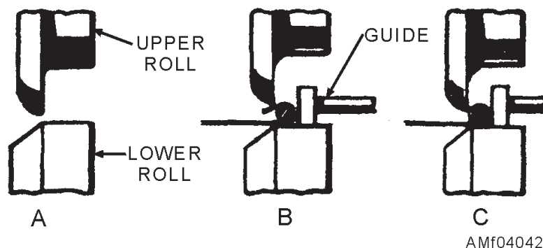
Figure 4-42.—Wiring operation.
