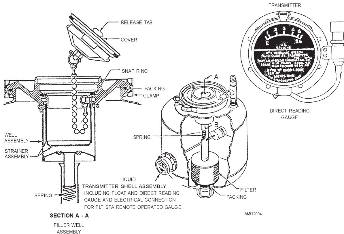
Figure 12-4.—Nonpressurized reservoir.
