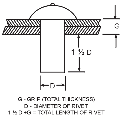
Figure 4-43.—Rivet length.
