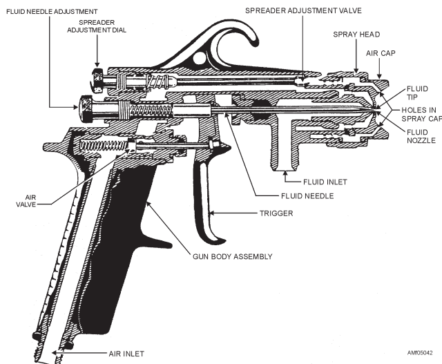
Figure 5-42.—Sectional view of typical spray gun.
