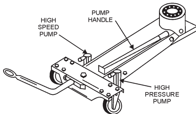
Figure 1-28.—T-Bar axle jack.
