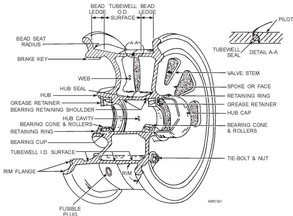
Figure 7-1.—Typical divided (split) wheel assembly.
