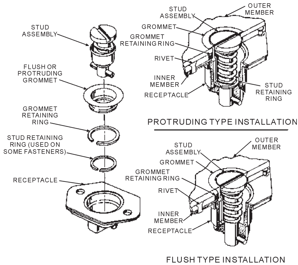
Figure 3-23.—Camloc 4002 series fastener.
