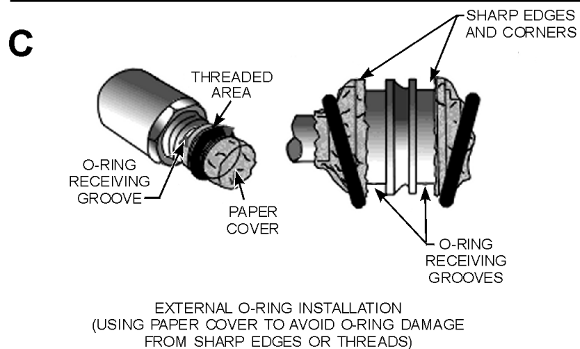
Figure 8-16.—O-ring installation.
