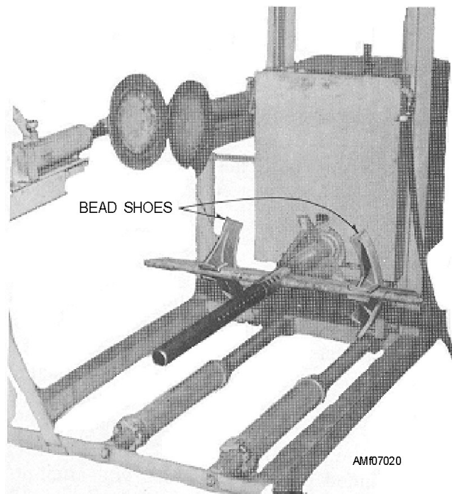
Figure 7-20.—Shaft arranged to hold tire bead while removing lockring.
