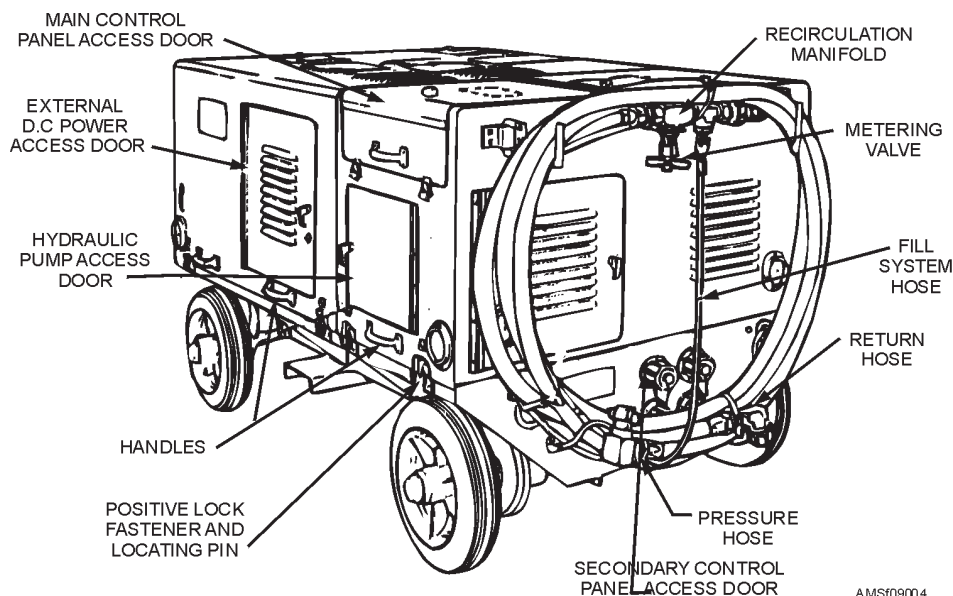
Figure 9-4.—A/M27T-5 portable hydraulic power supply, rear and right-hand side view.
