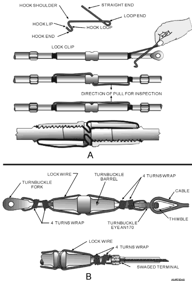
Figure 3-48.—Safetying turnbuckles: (A) Clip-locking method (preferred); (B) wire-wrapped method.
