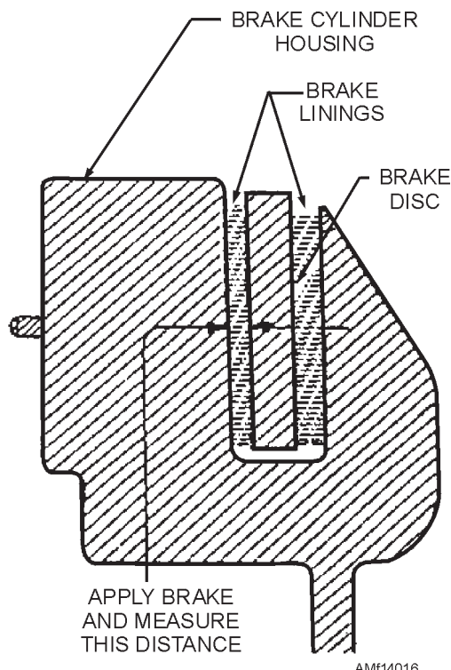
Figure 14-16.—Checking lining wear (Method No. 1).
