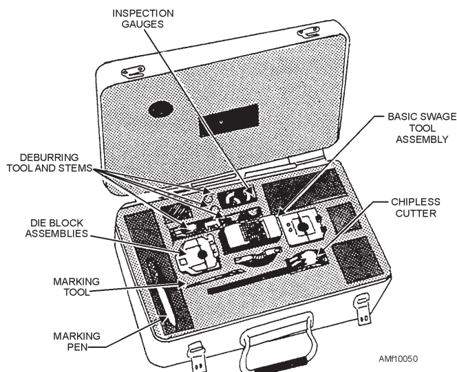
Figure 10-50.—Permaswage Tool Kit D10031-812S.
