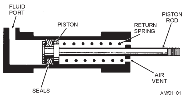
Figure 11-1.—Single-acting, spring-loaded, piston-type, actuating cylinder.
