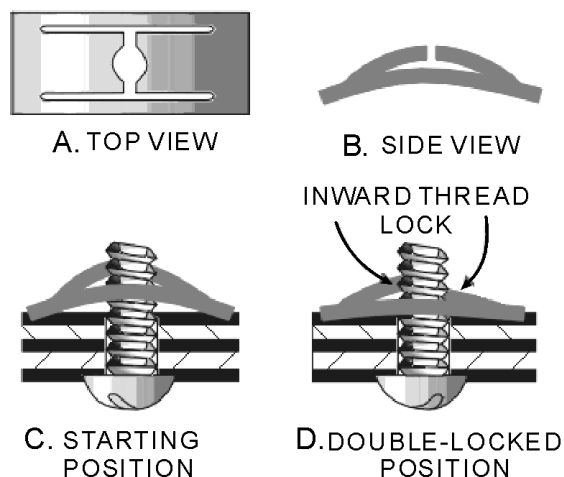
Figure 3-19.—Sheet spring nut.
