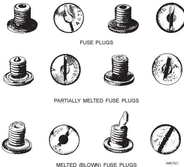
Figure 7-7.—Fuse plugs.
