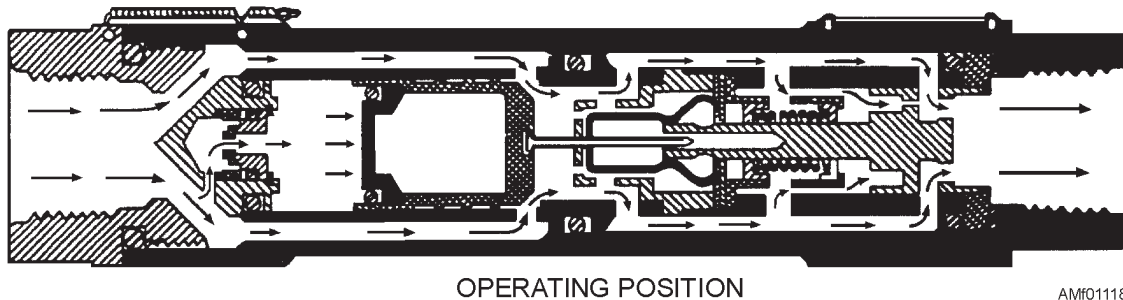
Figure 11-18.—Fuse, operational view.
