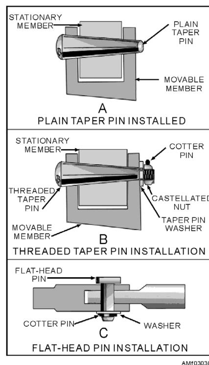
Figure 3-30.—Types of aircraft pins.
