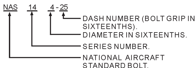
Figure 3-16.—NAS bolt part number breakdown.
