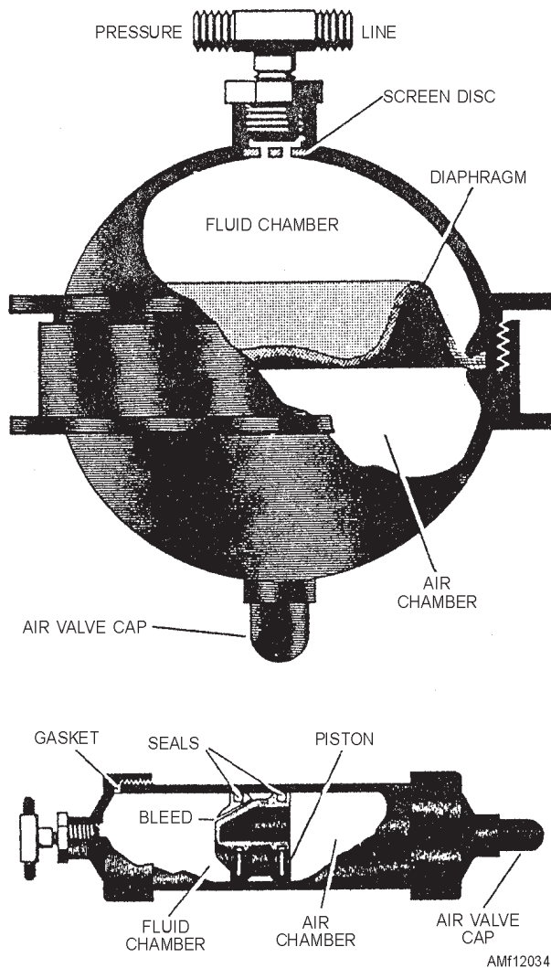
Figure 12-34.—Pressure accumulator, spherical and cylindrical types.
