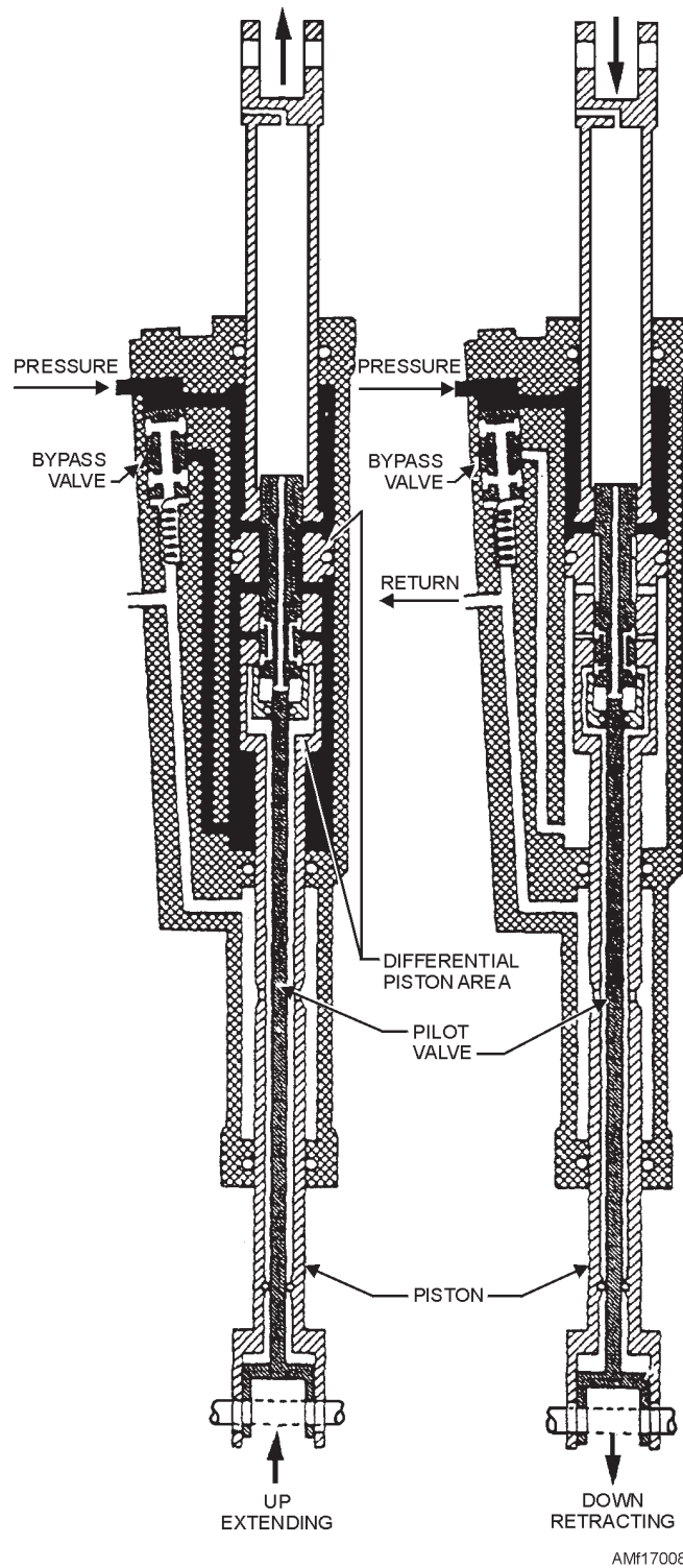
Figure 17-8.—Primary servo cylinder.
