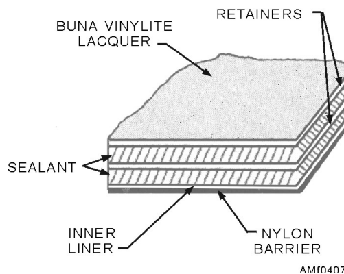
Figure 4-74.—Self-sealing fuel cell (standard construction).
