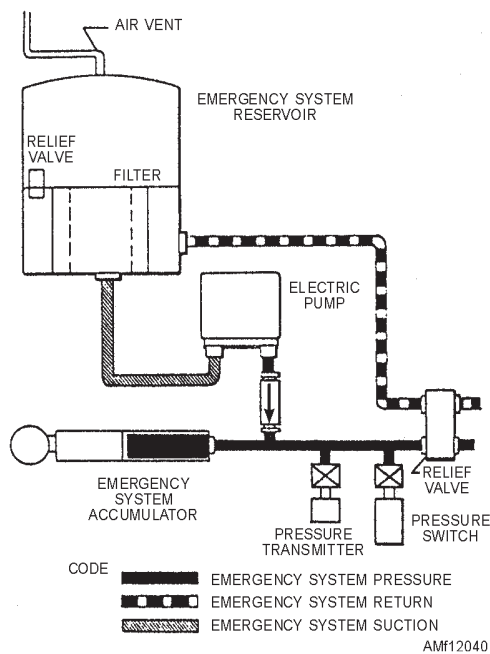
Figure 12-40.—Schematic diagram of typical emergency power system (electric-motor driven).
