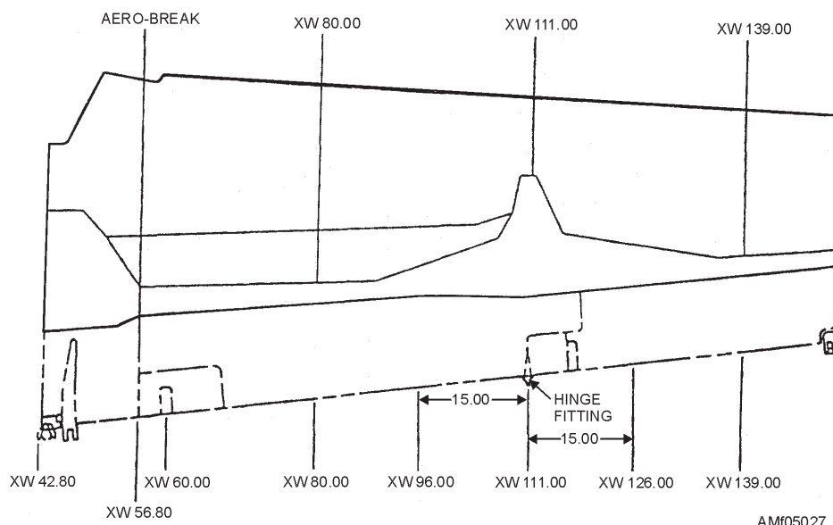
Figure 5-27.—Repair zones.
