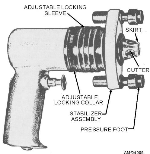
Figure 4-9.—Rivet-head shaver.
