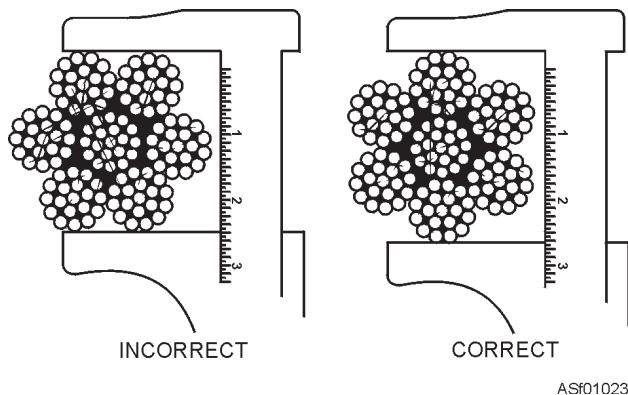
Figure 1-23.—Measuring the diameter of a wire rope.
