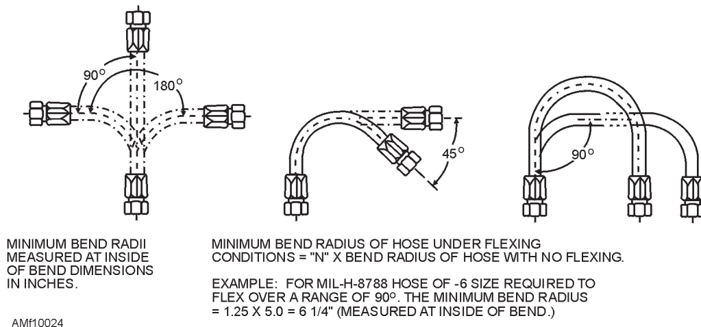
Figure 10-24.—"N" factor for flexing bends.
