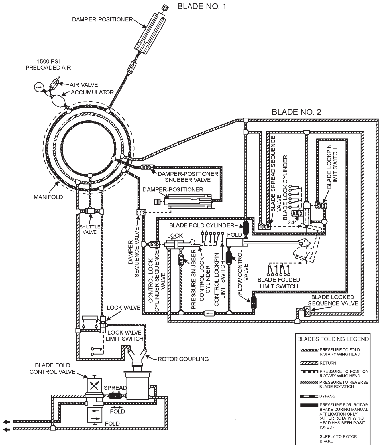
Figure 17-12.—Automatic blade folding system schematic—Continued.
