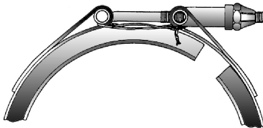
Figure 3-29.—Safetying a V-band coupling.
