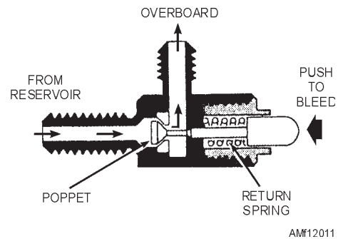
Figure 12-11.—Air bleeder valve.
