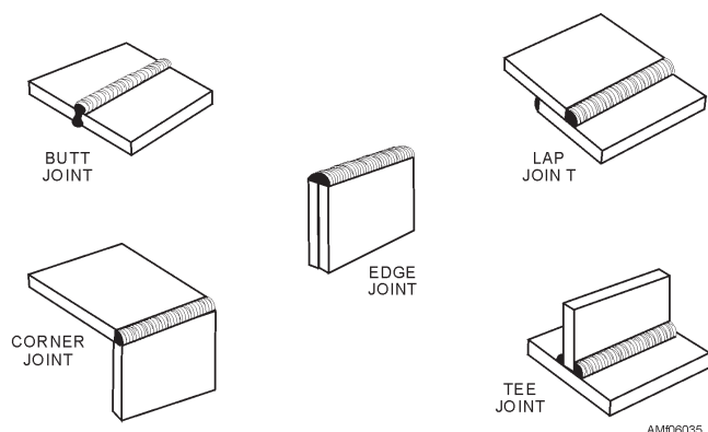
Figure 6-35.—Types of welded joints.
