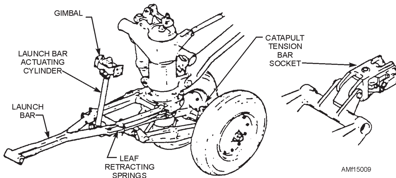
Figure 15-9.—Catapult system.
