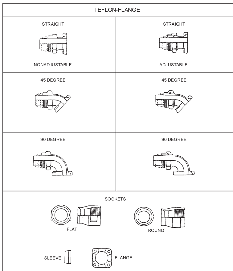
Figure 10-4.—Teflon® hose fittings—(Continued).
