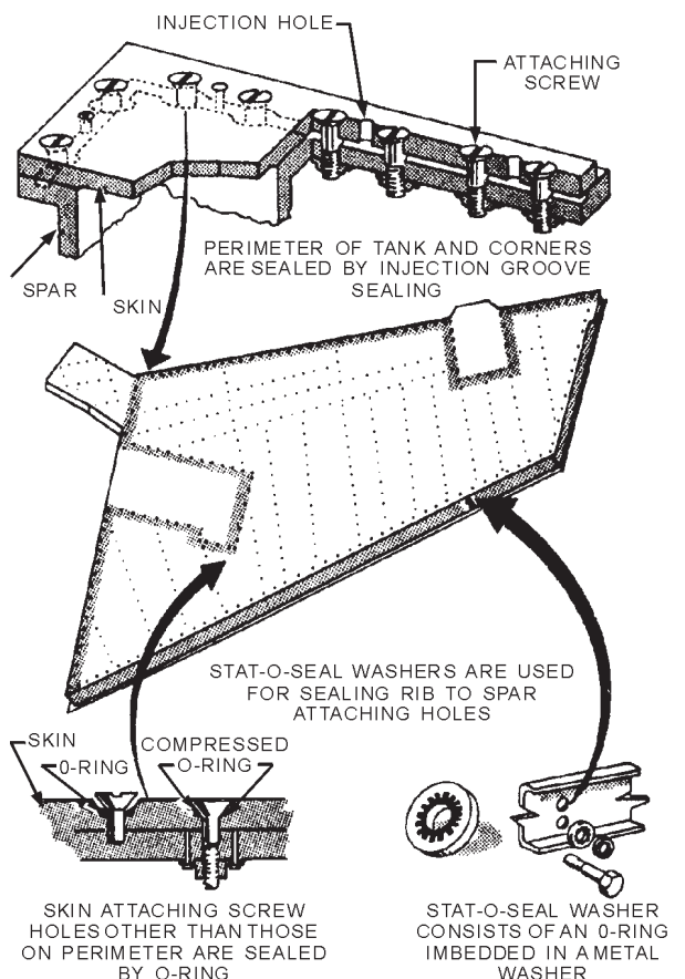
Figure 4-76.—Sealing integral fuel cell screws and bolts.
