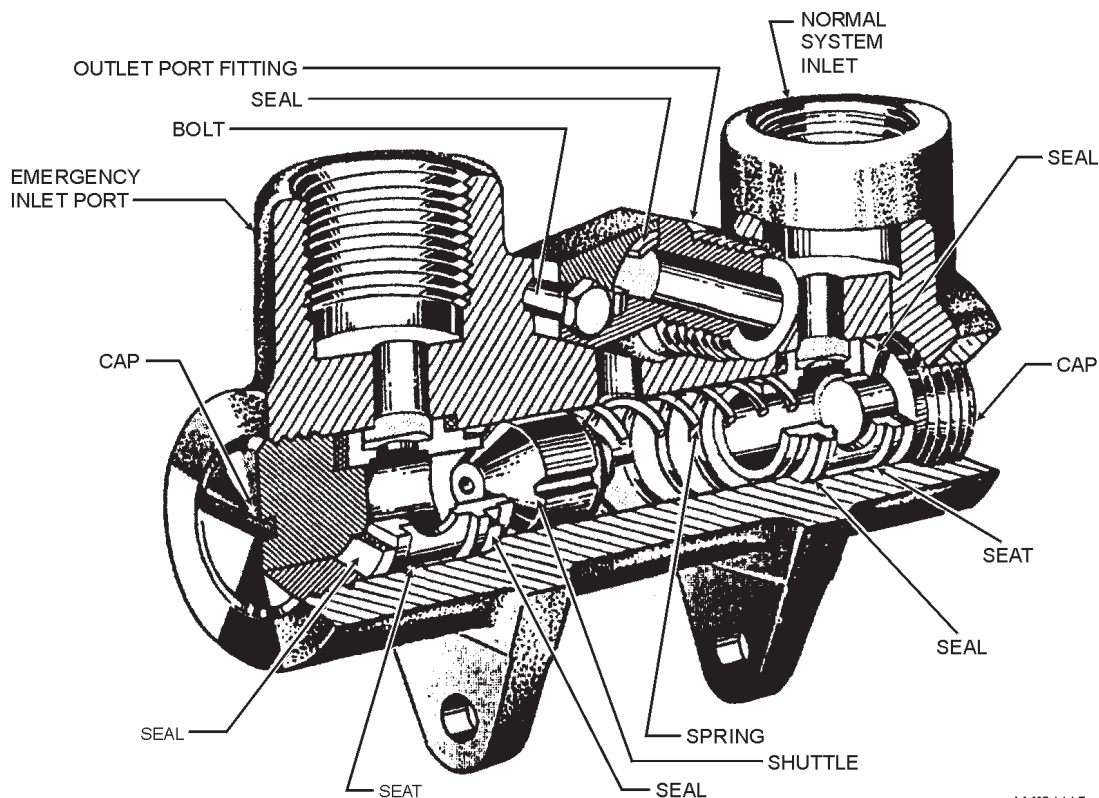
Figure 11-15.—Shuttle valve.
