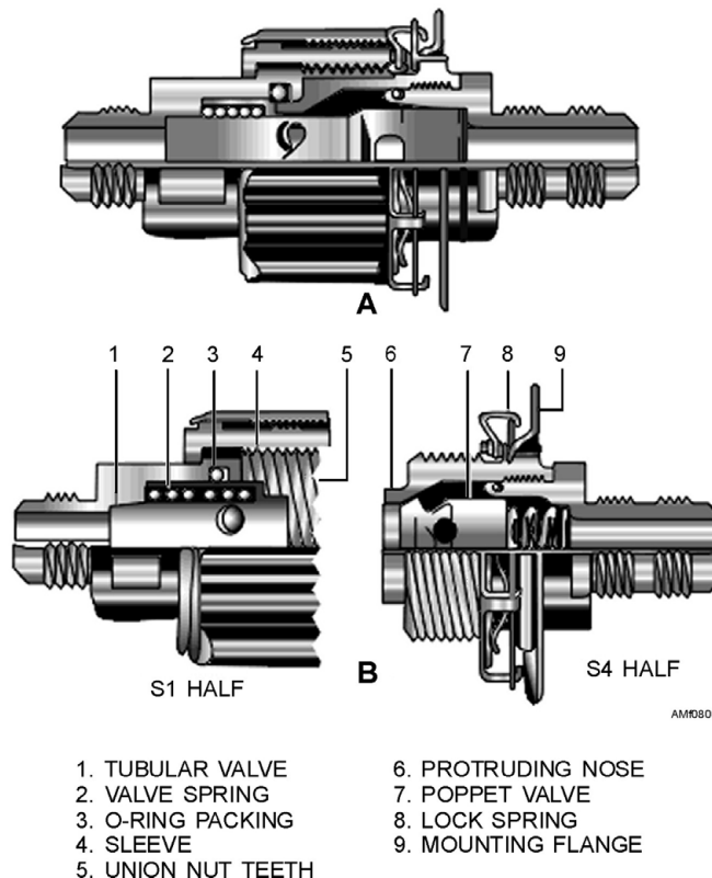
Figure 8-8.—Series 145 and 155 quick-disconnect couplings.
