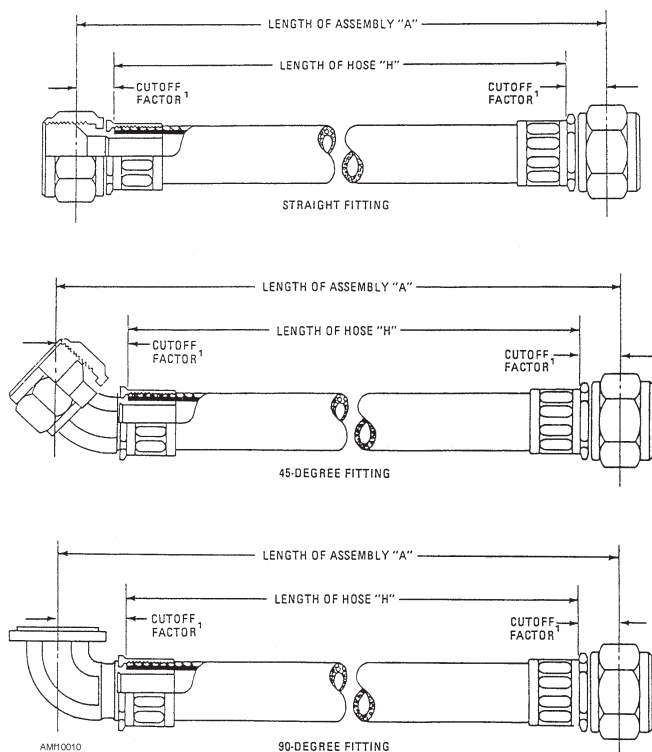
Figure 10-10.—Determining hose assembly length.
