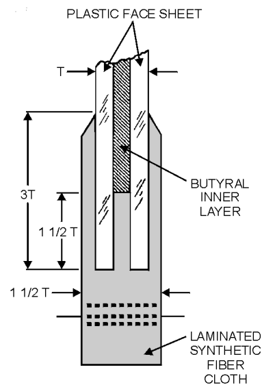
Figure 5-5.—Approved edge attachment for laminated plastic.
