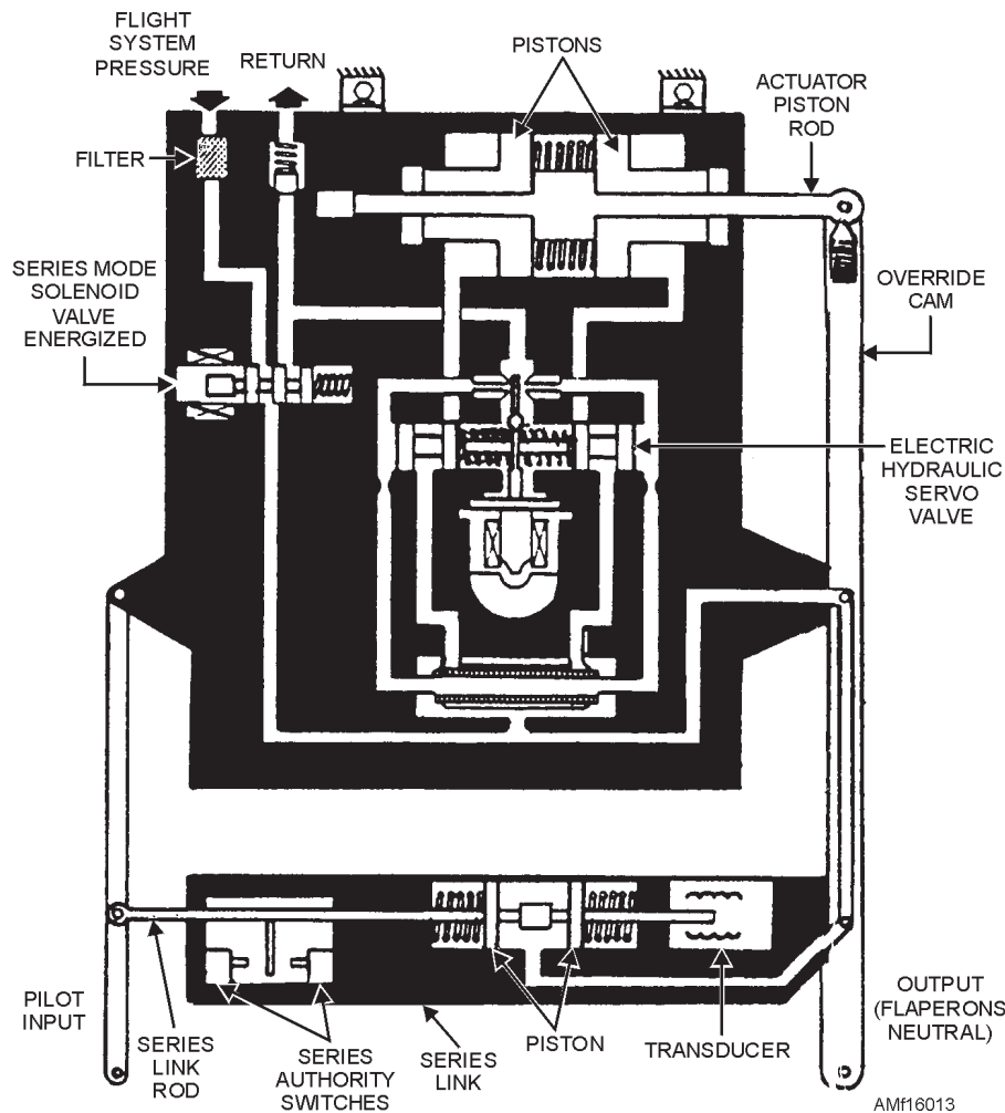
Figure 16-13.—Flaperon autopilot actuator.
