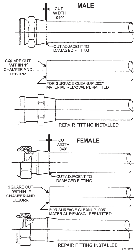
Figure 10-55.—Male and female repair fitting installation.
