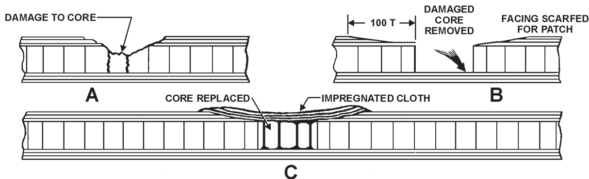
Figure 5-11.—Honeycomb-type core repair.
