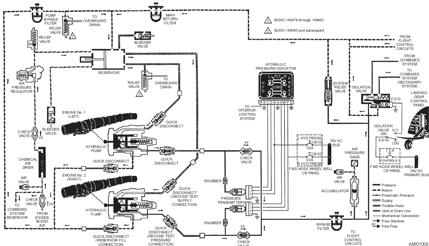
Figure 1-8.—Hydraulic system schematic.
