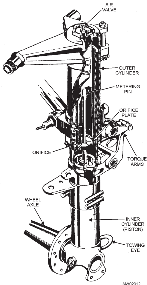
Figure 2-12.—Shock strut showing internal construction.
