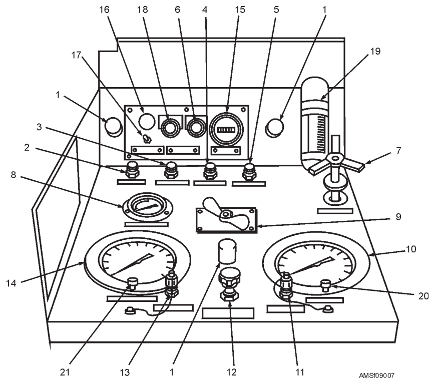
Figure 9-6.—Portable electric motor-driven hydraulic power supply (A/M27T-7).
