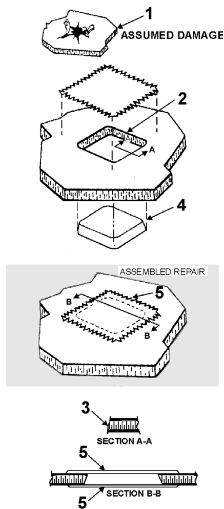
Figure 5-17.—Balsa wood repair with filler plug and fabric patch.
