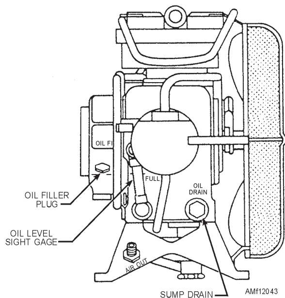
Figure 12-43.—Air compressor.
