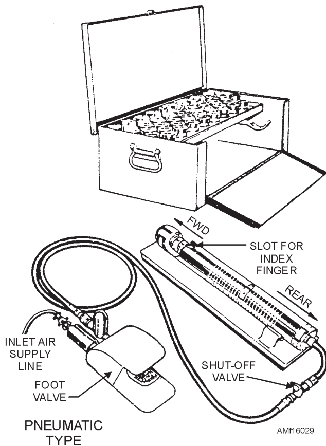
Figure 16-29.—Hand-swaging tools—mechanical and pneumatic.
