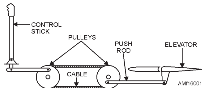
Figure 16-1.—Mechanical (unboosted) flight control system.
