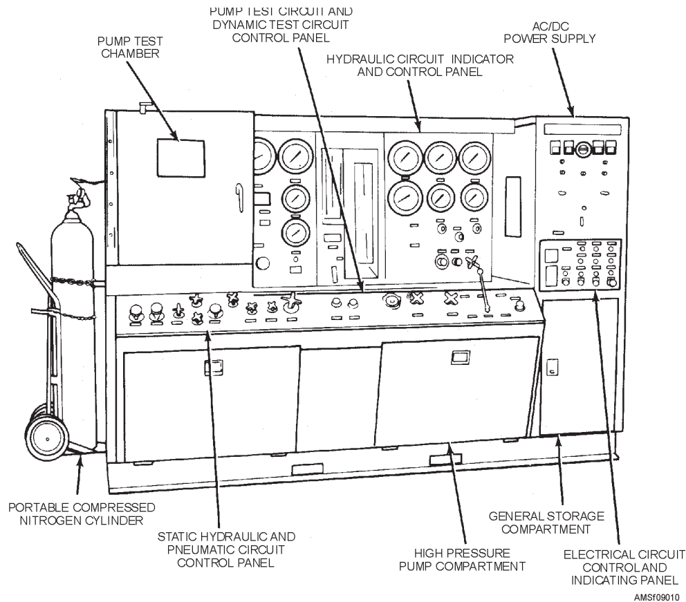
Figure 9-10.—Model HCT-10 hydraulic and pneumatic component test stand.
