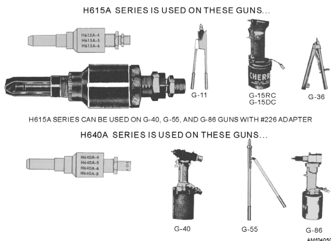
Figure 4-50.—Cherrylock guns.
