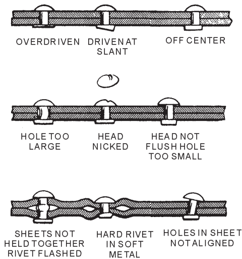
Figure 4-47.—Incorrectly driven rivets.
