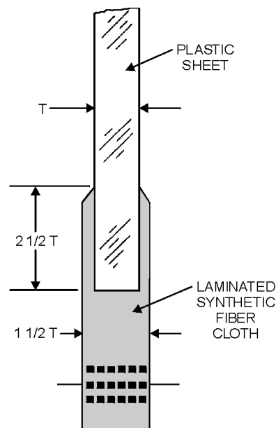
Figure 5-4.—Approved edge attachment for solid plastic.
