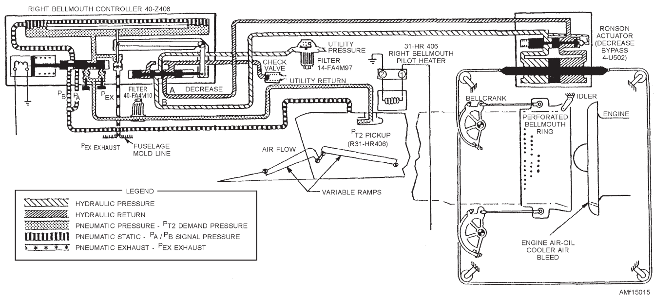
Figure 15-15.—Variable bellmouth system.
