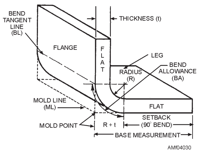
Figure 4-30.—Bend allowance terms.
