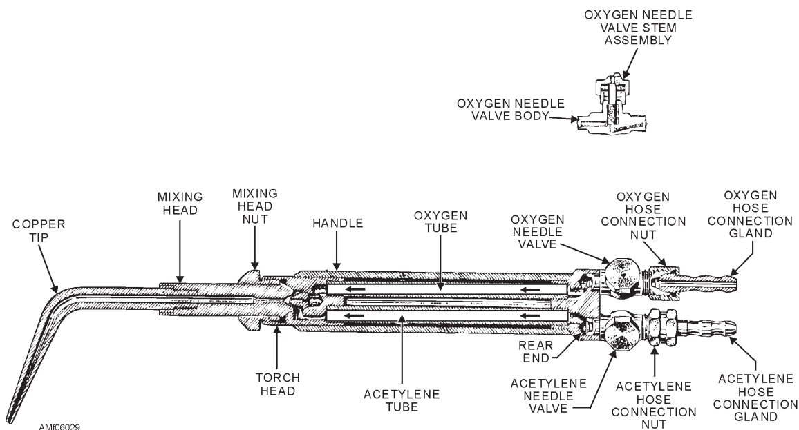
Figure 6-29.—Equal pressure welding torch.
