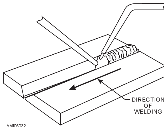
Figure 6-32.—Forehand welding.
