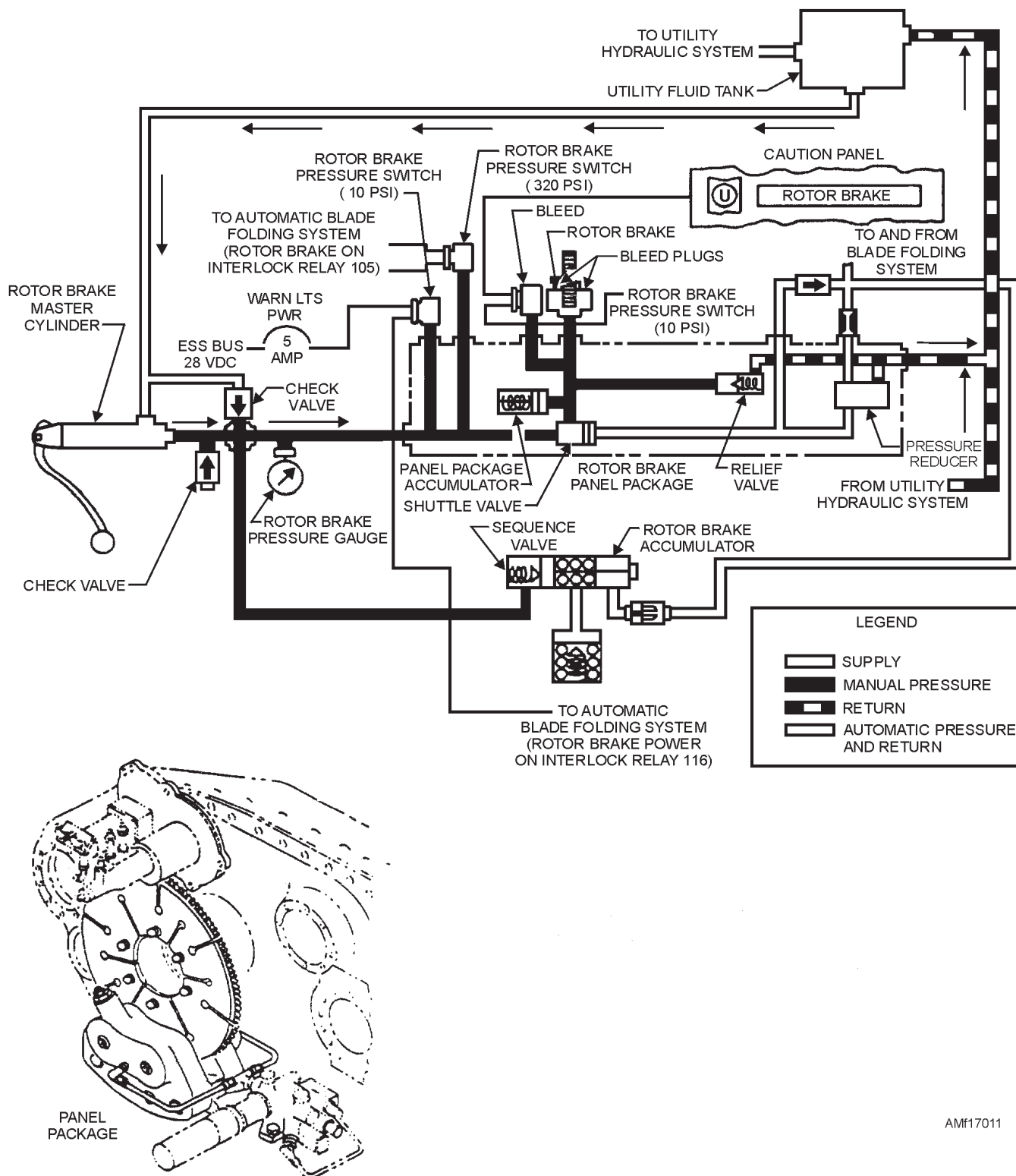
Figure 17-11.—Rotor brake and system schematic.
