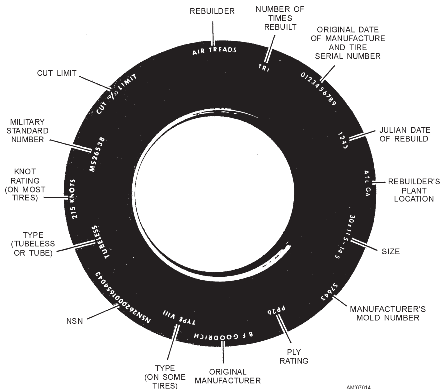
Figure 7-14.—Rebuilt tire identification markings.
