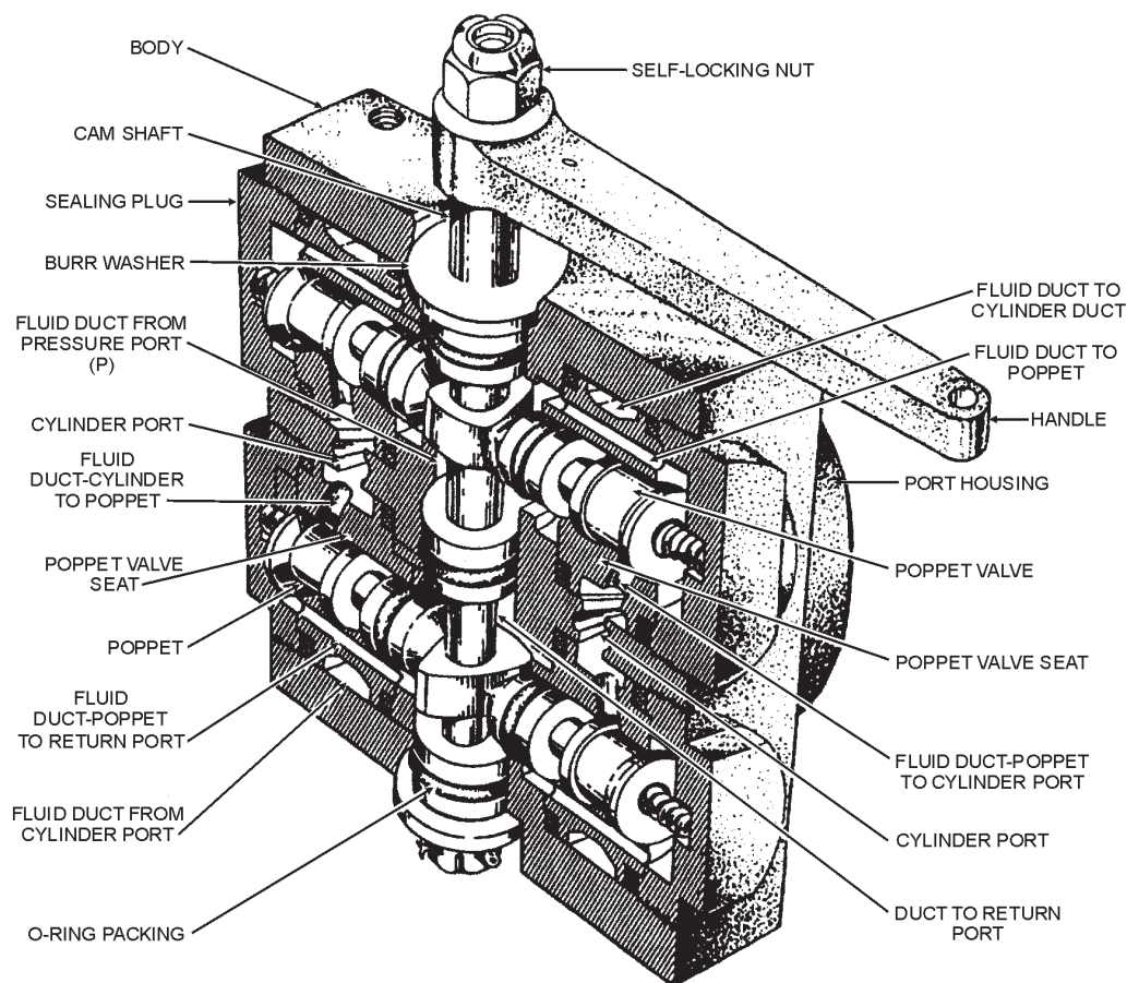
Figure 11-8.—Cutaway view of selector valve body.
