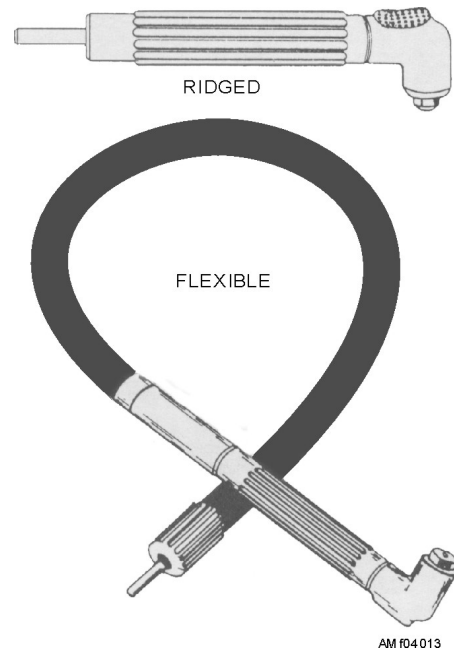
Figure 4-13.—Angle-drive drills.
