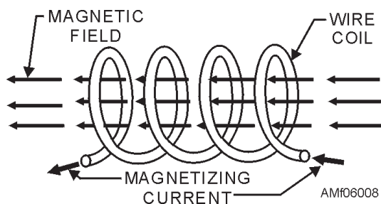
Figure 6-8.—Magnetic field in a part placed in a coil.
