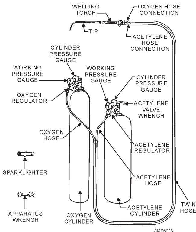
Figure 6-23.—Portable oxyacetylene welding and cutting equipment.
