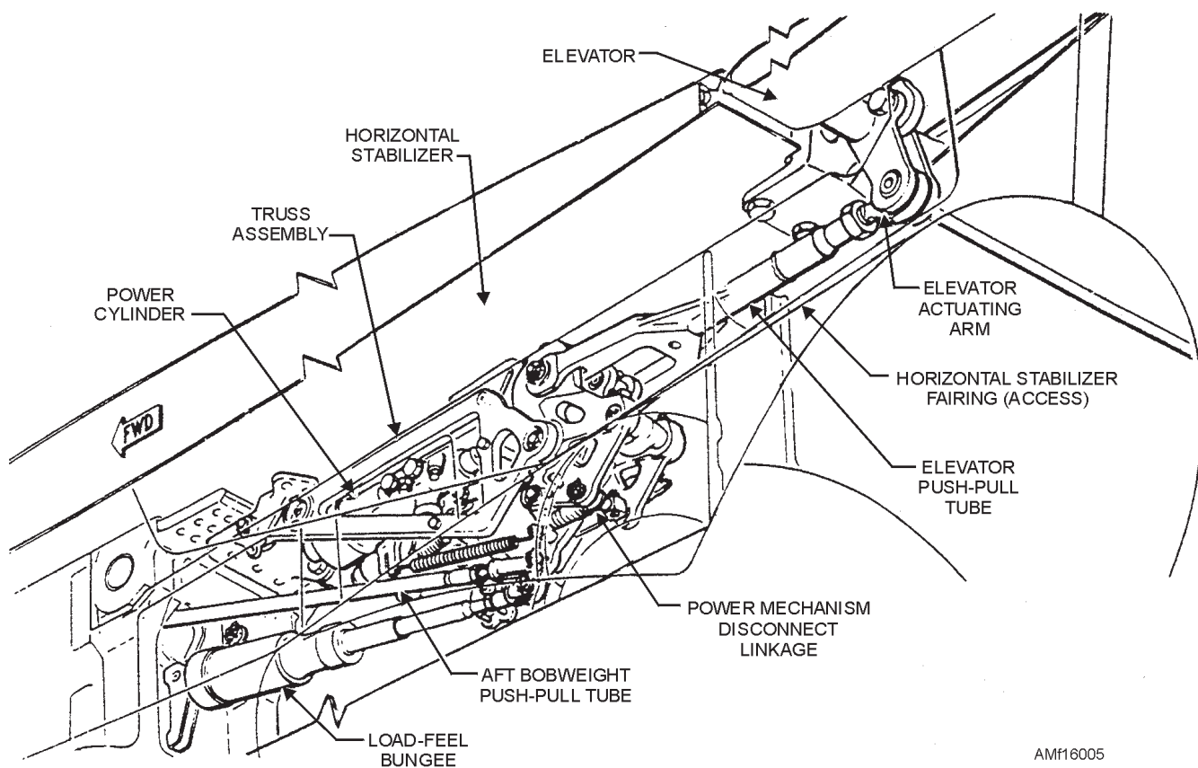
Figure 16-5.—Elevator power mechanism.
