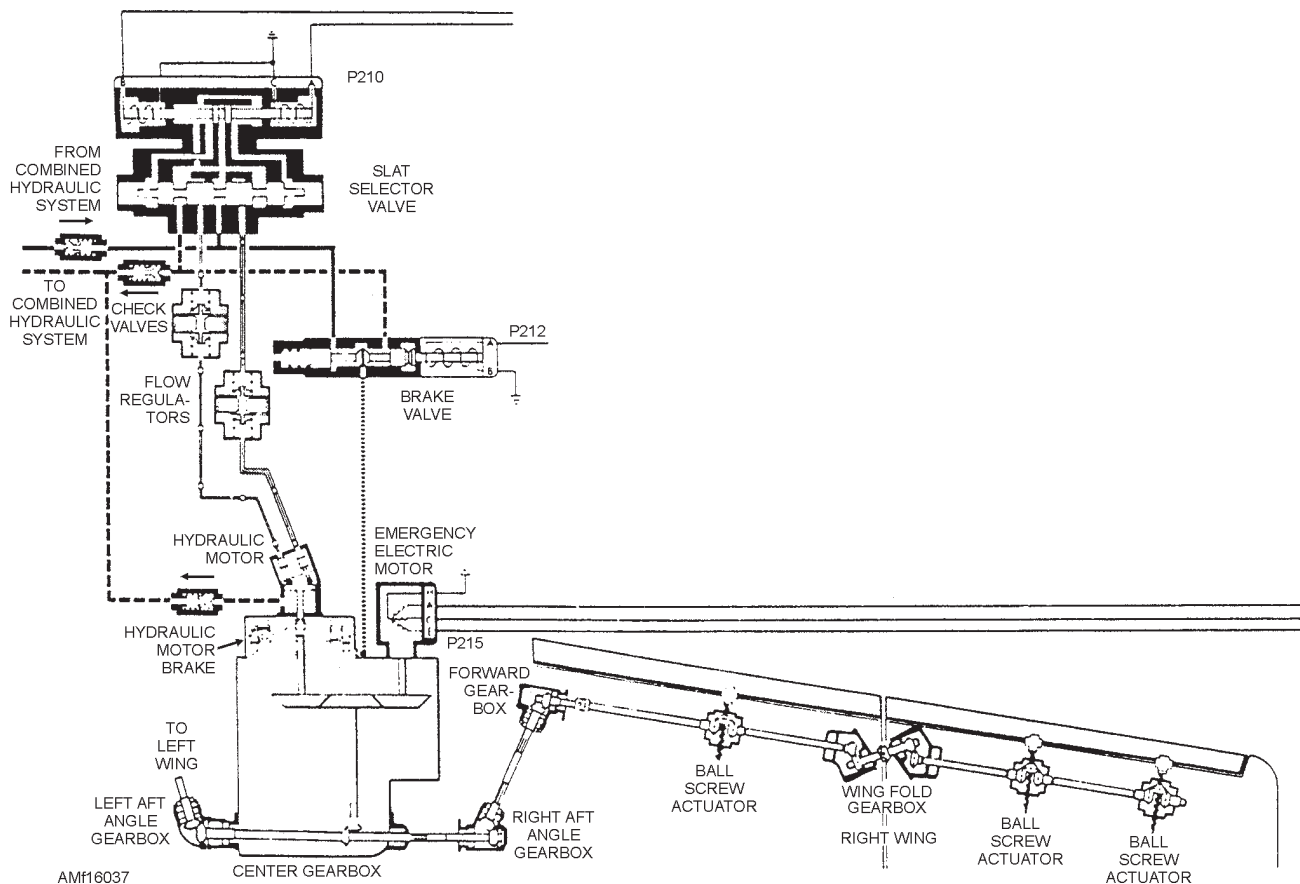
Figure 16-37.—Slat drive system.
