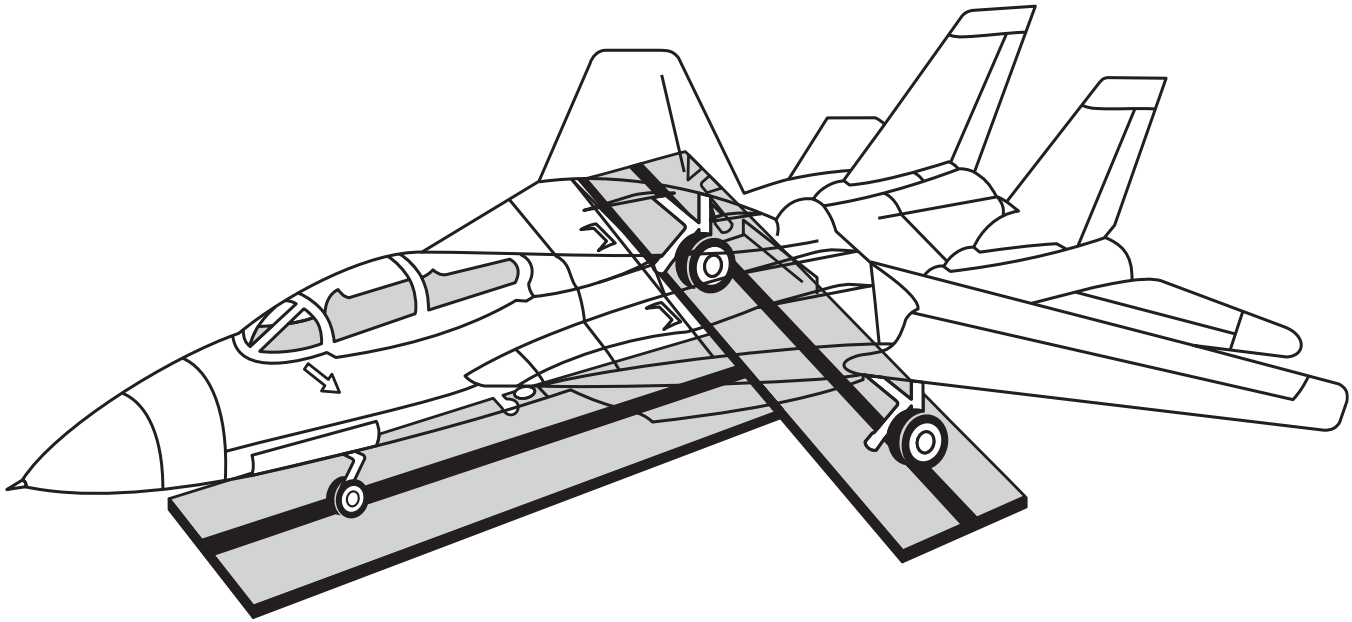
Figure 1-18.—Stationary pit-type scales.
