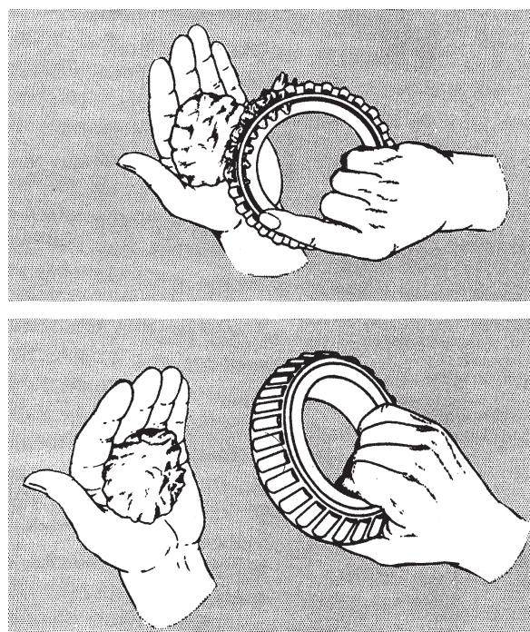
Figure 7-9.—Hand repacking of wheel bearings.
