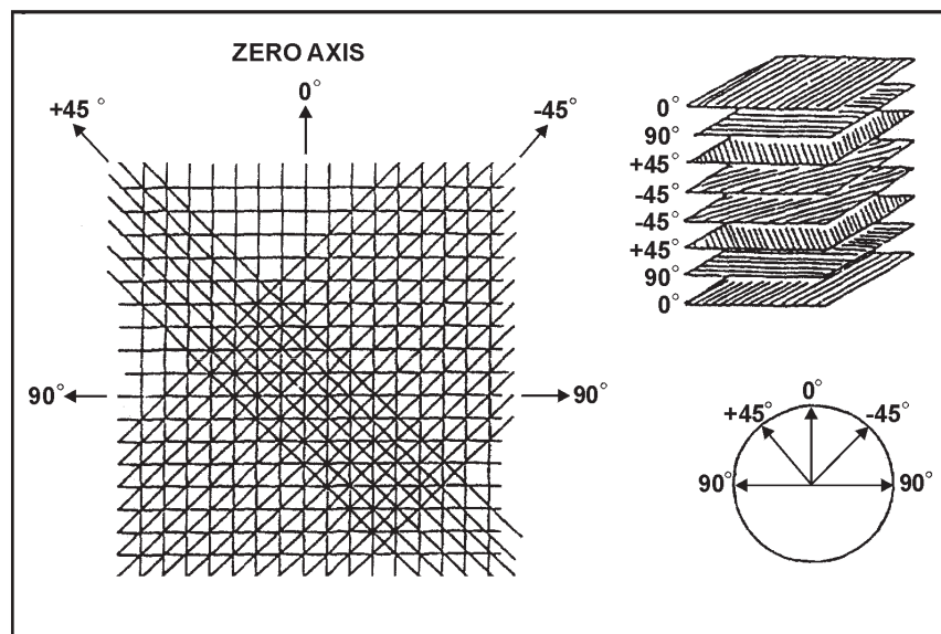
Figure 5-24.—Standard ply orientation clock.
