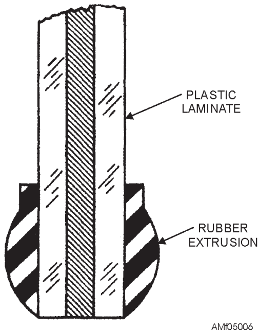
Figure 5-6.—Typical sighting dome attachment.
