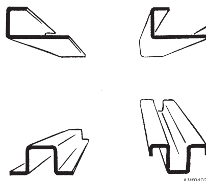
Figure 4-37.—Types of bends on a bar folder.
