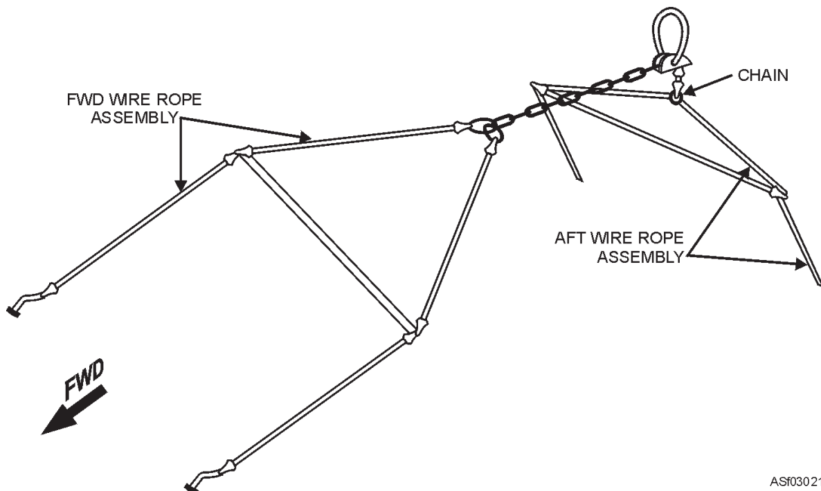
Figure 1-21.—Combination wire rope and chain sling.
