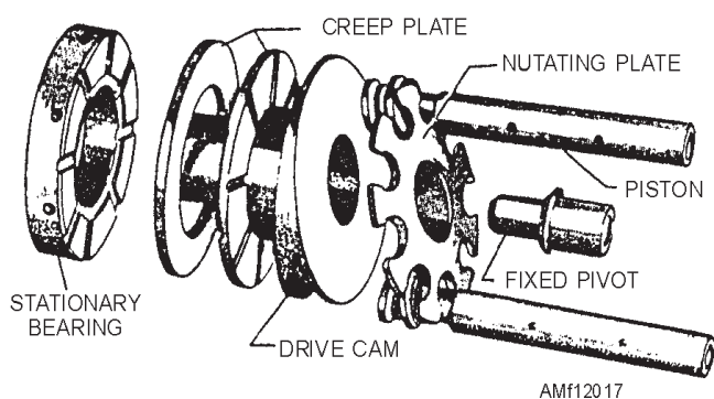
Figure 12-17.—Mechanical drive.
