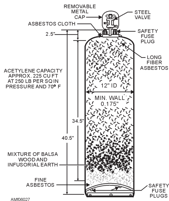
Figure 6-27.—Acetylene cylinder.
