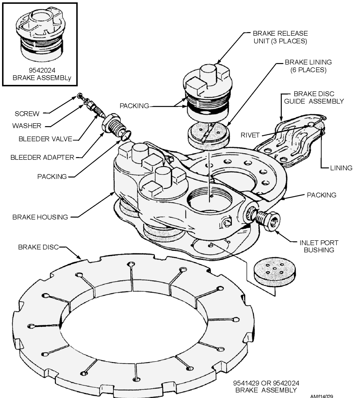
Figure 14-29.—Single disc brake—repair and parts replacement diagram.
