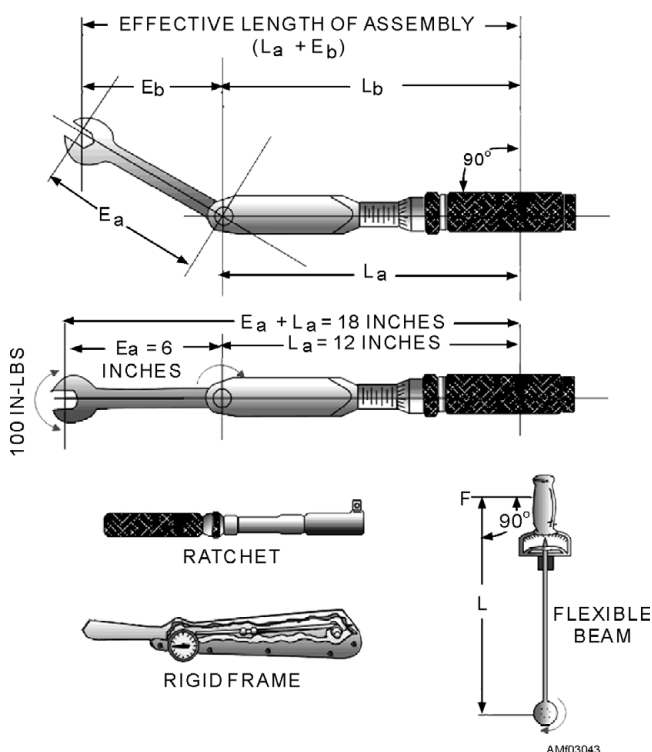
Figure 3-43.—Torque wrenches.
