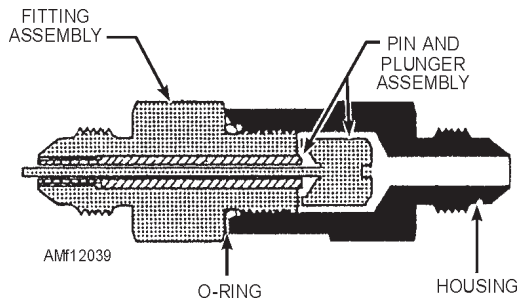
Figure 12-39.—Gauge and pressure transmitter snubber.
