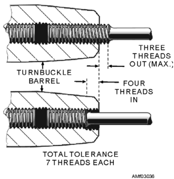
Figure 3-36.—Turnbuckle tolerances.
