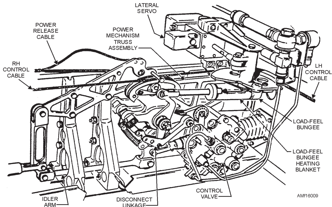
Figure 16-9.—Aileron power mechanism.
