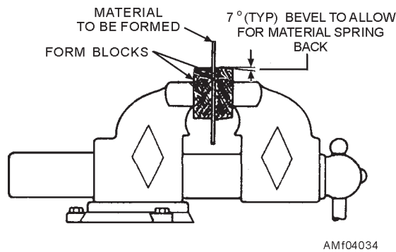
Figure 4-34.—Preparation for straight bend by hand.
