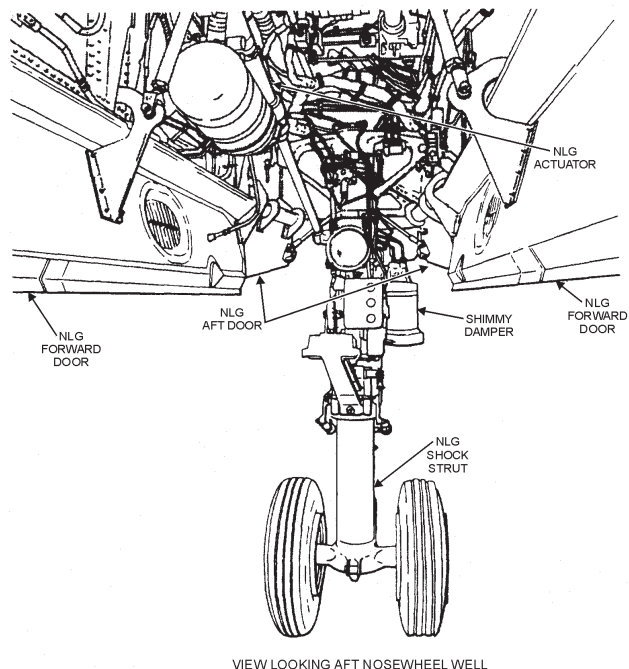
Figure 2-13.—Nose gear assembly.
