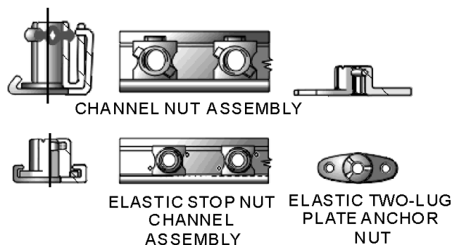
Figure 3-18.—Self-locking plate nuts.
