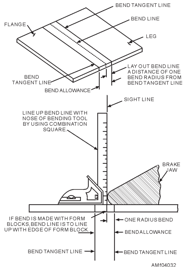
Figure 4-32.—Locating bend lines in a brake.
