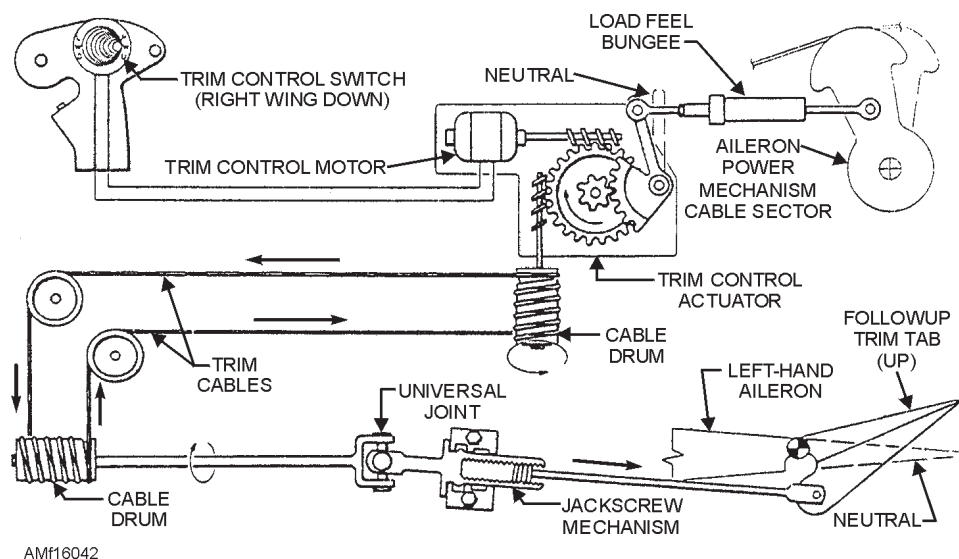
Figure 16-42.—Aileron trim control system.
