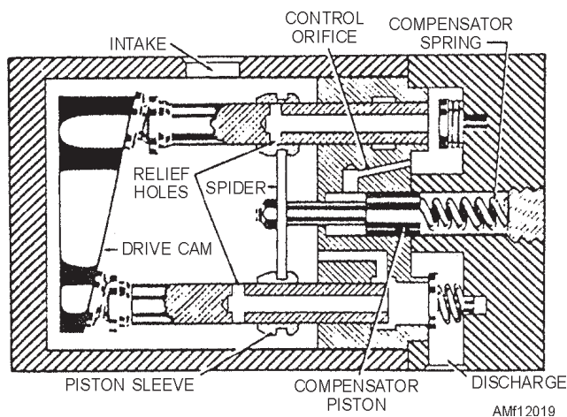
Figure 12-19.—Pressure control mechanism.
