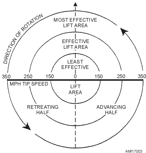
Figure 17-3.—Symmetry of lift.
