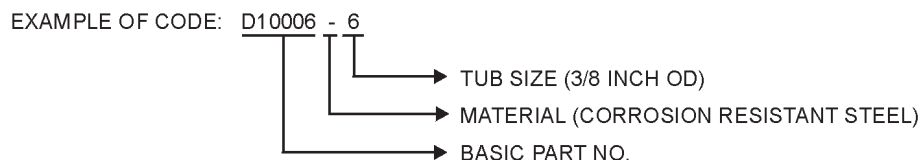
Figure 10-27.—Typical style of Permaswage fittings.
