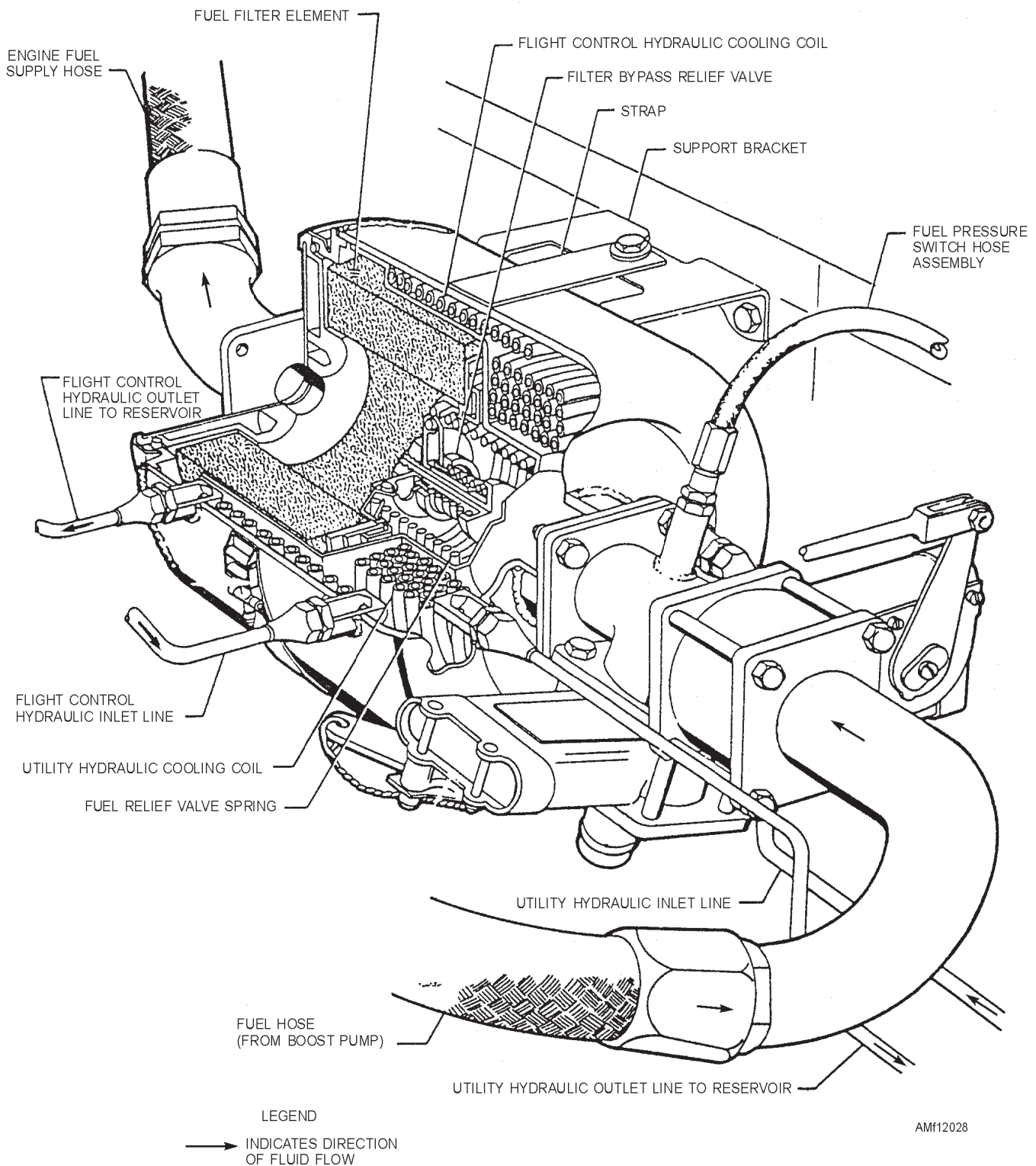
Figure 12-28.—Hydraulic fluid cooler.
