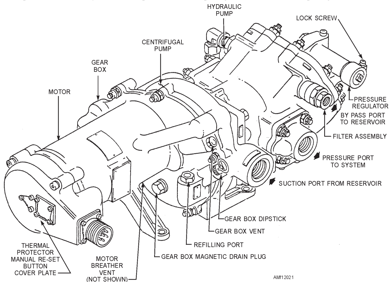
Figure 12-21.—Motor-driven variable displacement piston pump.
