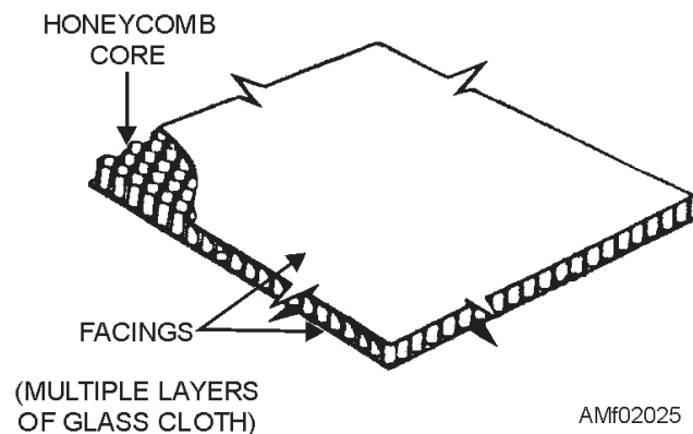
Figure 2-25.—Reinforced plastic.
