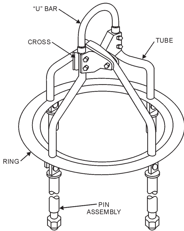
Figure 1-20.—Typical steel/aluminum sling.
