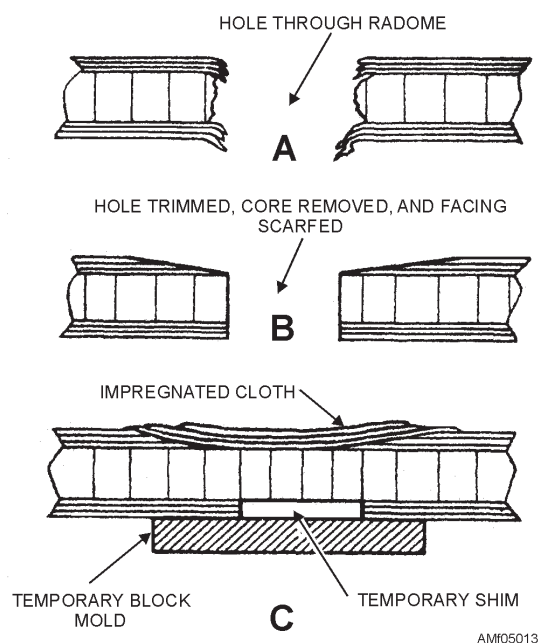
Figure 5-13.—Scarfed repair method.
