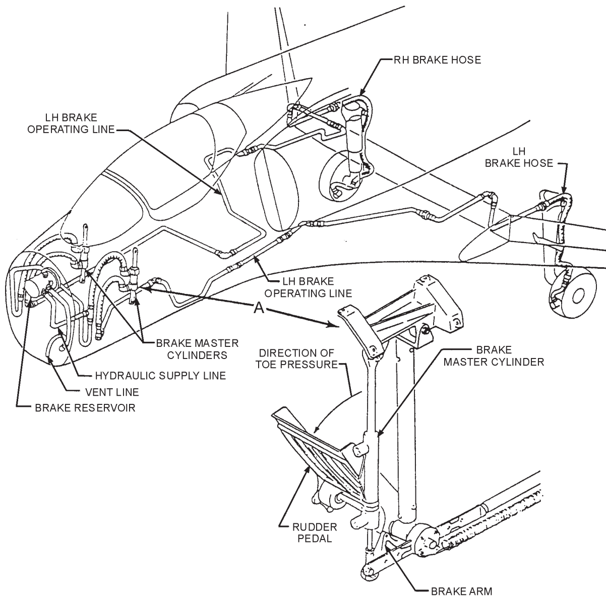
Figure 14-1.—Typical independent-type brake system.
