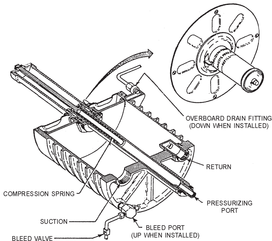
Figure 12-12.—Typical fluid-pressurized reservoir.
