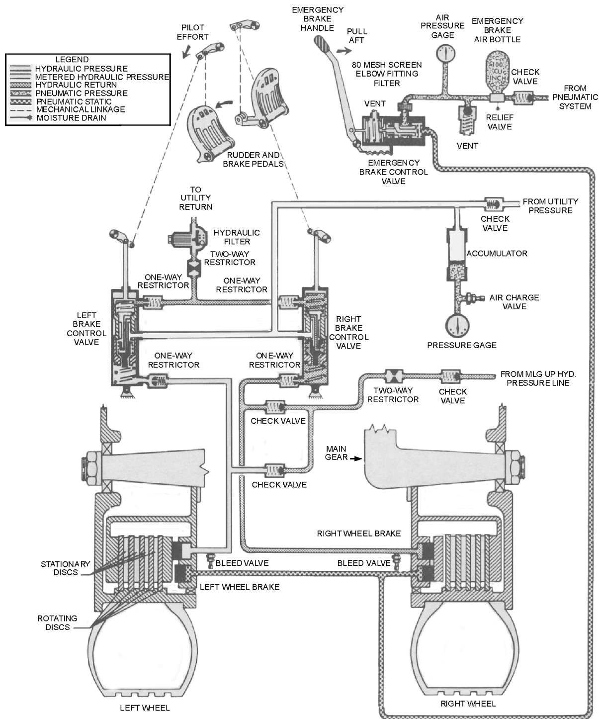
Figure 14-14.—Power/manual brake systems—schematic.
