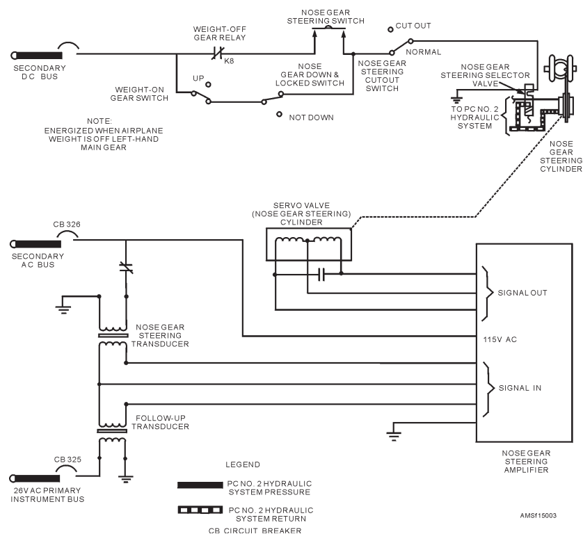
Figure 15-3.—Nose gear steering system diagram.
