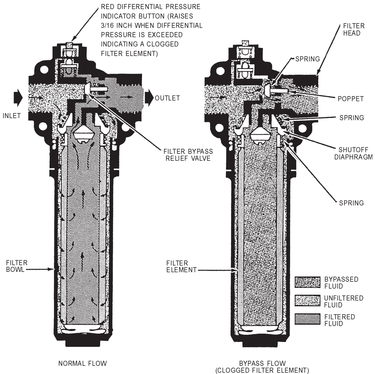
Figure 12-33.—Hydraulic filter assembly incorporating differential pressure indicator.
