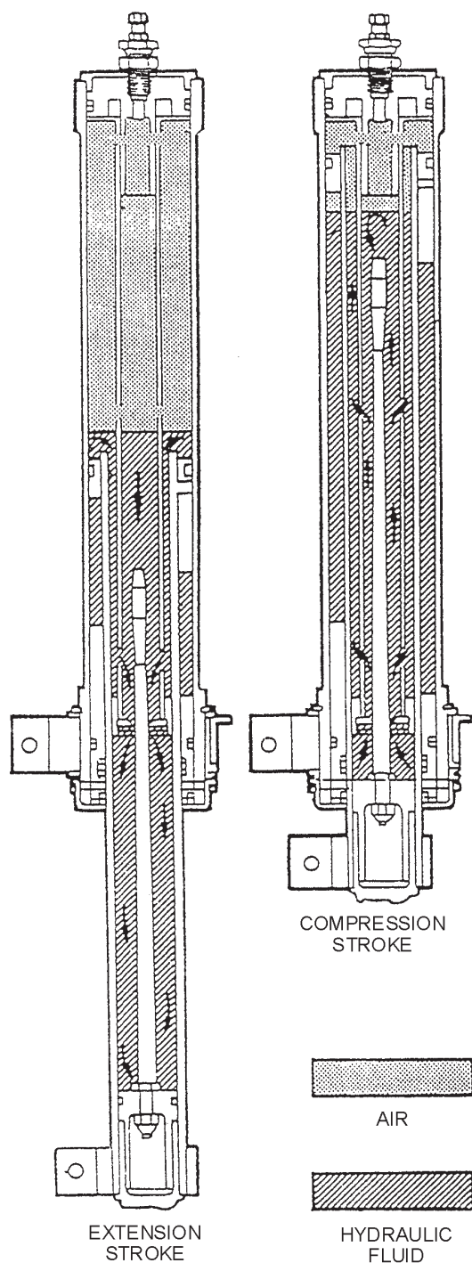
Figure 13-11.—Shock strut operation.
