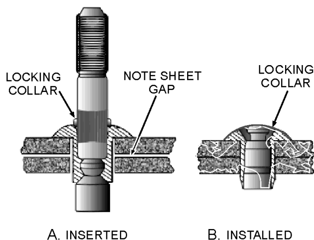
Figure 3-3.—Self-plugging rivet (mechanical lock).
