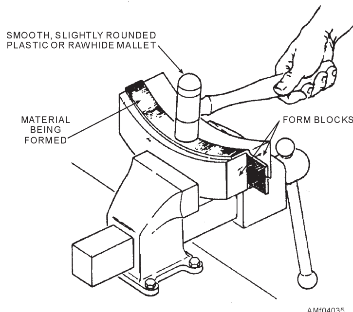
Figure 4-35.—Forming concave hand bend.
