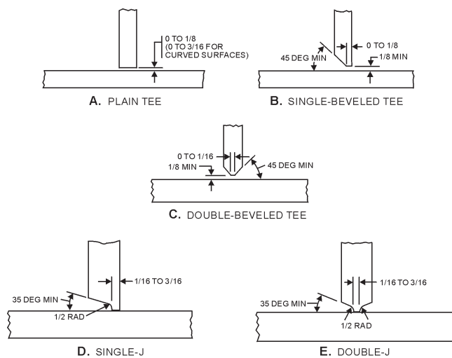
Figure 6-39.—Edge preparations for tee joint.
