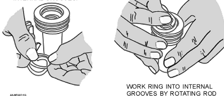
Figure 8-19.—Installation of Teflon® backup rings (internal).
