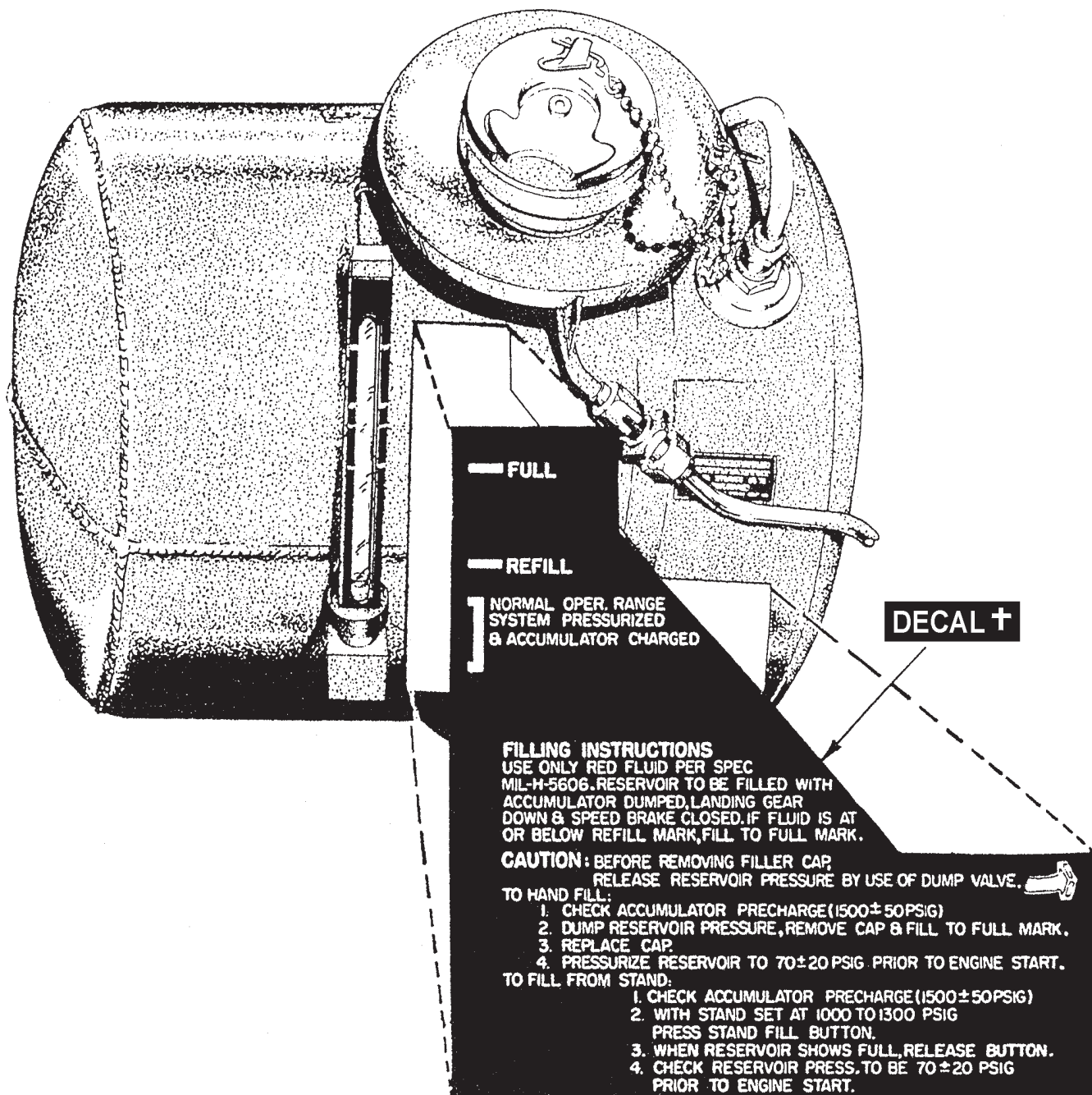
Figure 12-3.—Hydraulic reservoir instruction plate.
