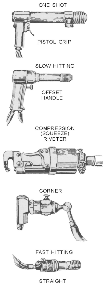
Figure 4-11.—Various types of rivet guns.
