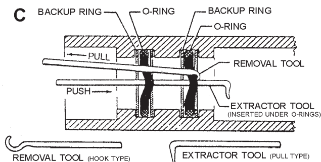
DUAL INTERNAL O-RING REMOVAL (USING PUSH TYPE EXTRACTOR AND HOOK TYPE REMOVAL TOOLS)
