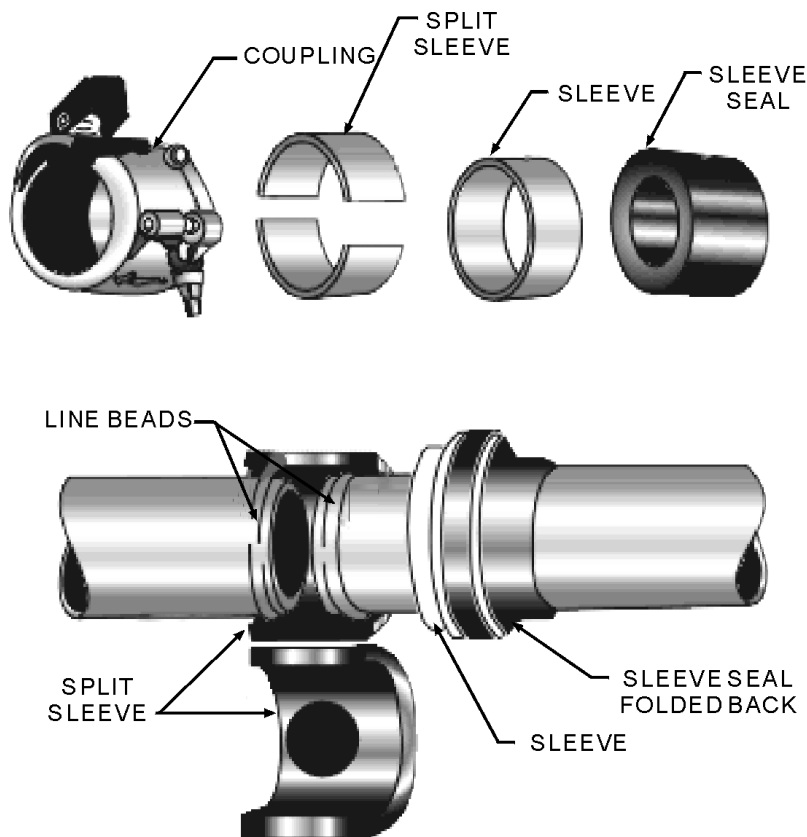
Figure 3-27.—Flexible line coupling.
