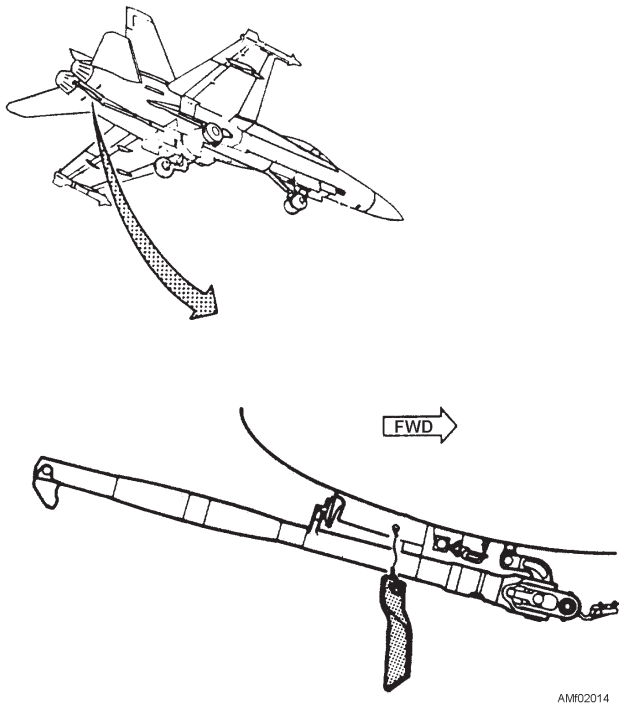
Figure 2-14.—Arresting gear installation.
