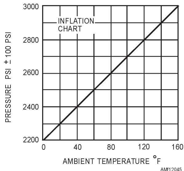
Figure 12-45.—Pneumatic storage cylinder inflation chart
