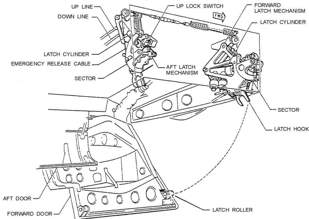
Figure 13-5.—Main gear door latch mechanisms.
