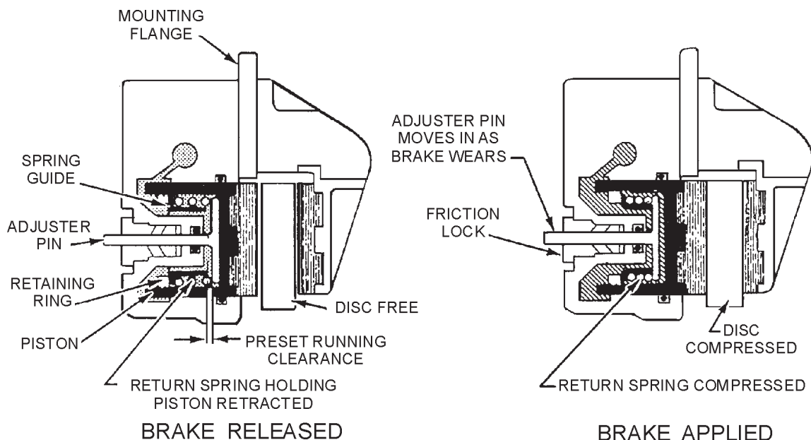
Figure 14-26.—Brake self-adjustment feature—single disc brake.
