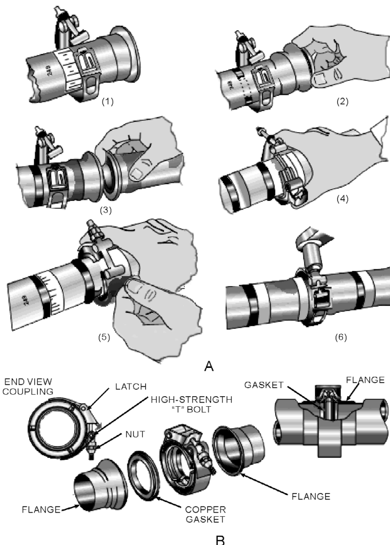
Figure 3-28.—Installation of rigid line couplings.
