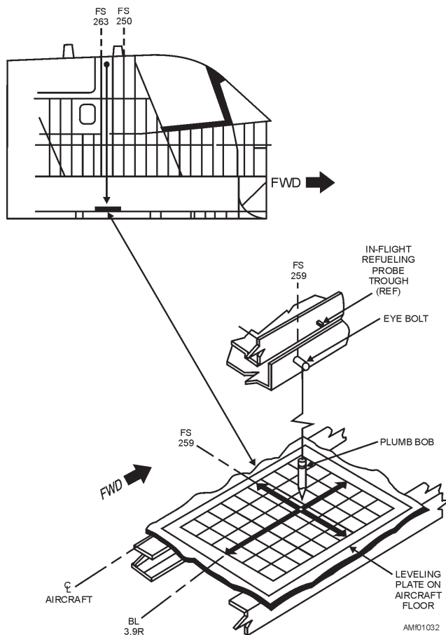
Figure 1-32.—Aircraft leveling.
