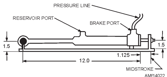
Figure 14-22.—Piston, valve, and brake chamber proof test setup diagram
