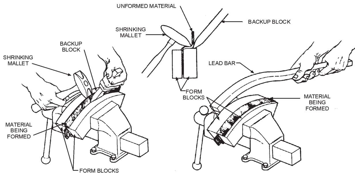
Figure 4-36.—Forming convex hand bends.
