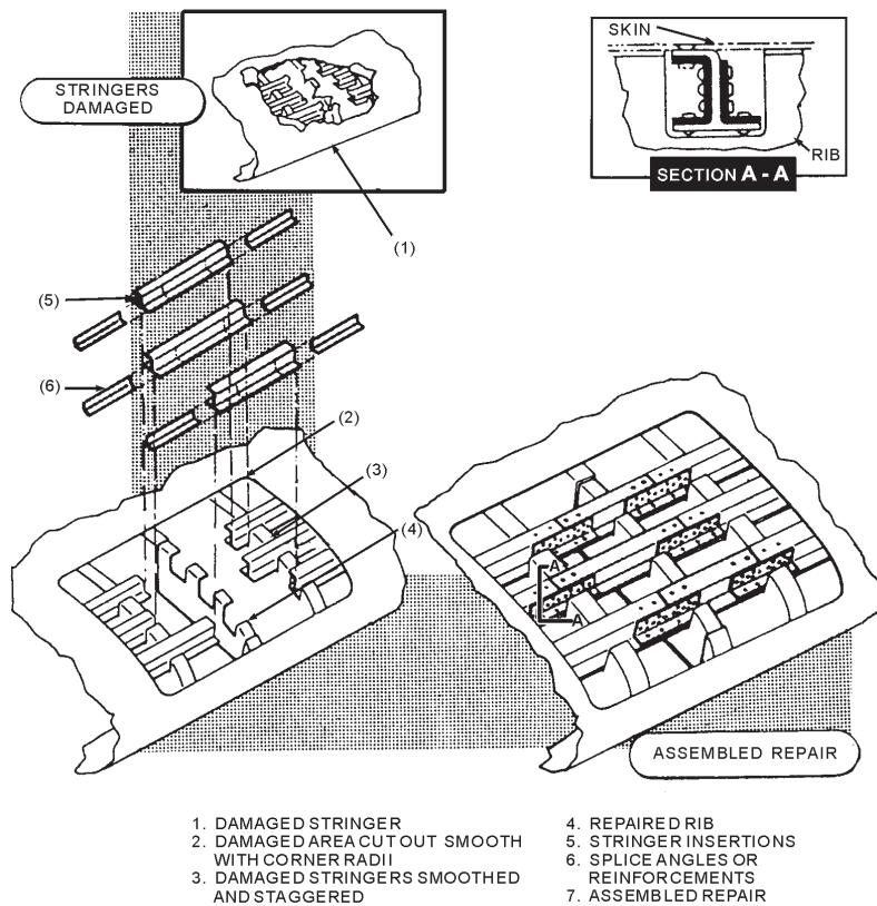
Figure 4-68.—Stringer repair by insertion.
