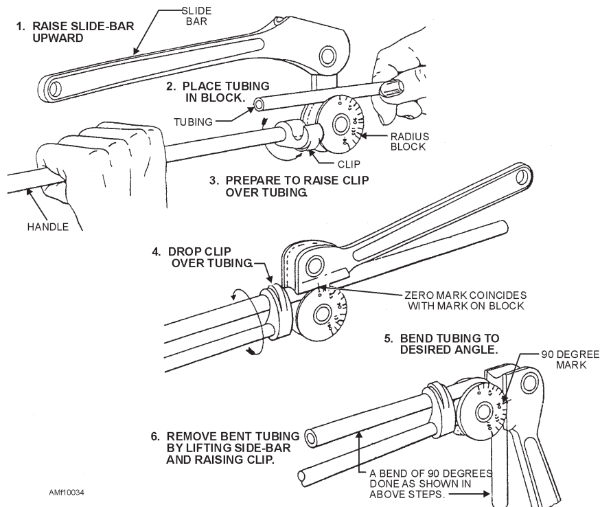
Figure 10-34.—Bending tubing with hand-operated tube bender.
