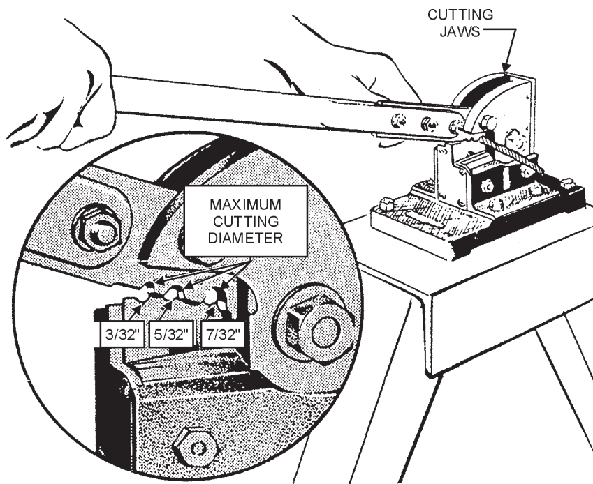
Figure 16-28.—Cable-cutting machine.
