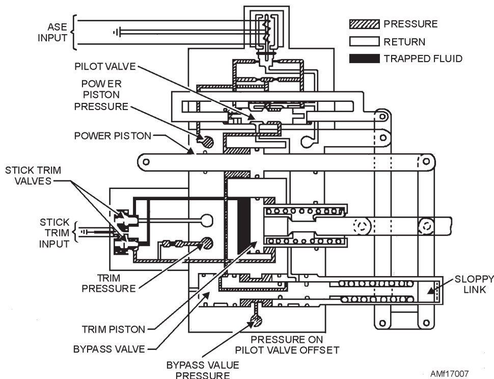
Figure 17-7.—Auxiliary servo cylinder.
