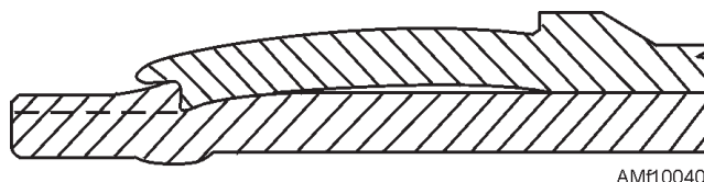
Figure 10-40.—Preset sleeve.
