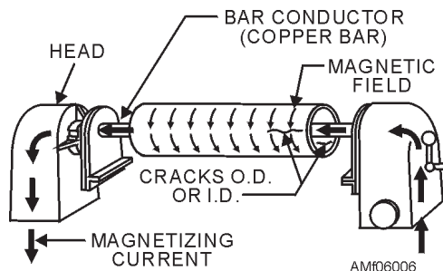
Figure 6-6.—Using a central conductor to circularly magnetize a cylinder.
