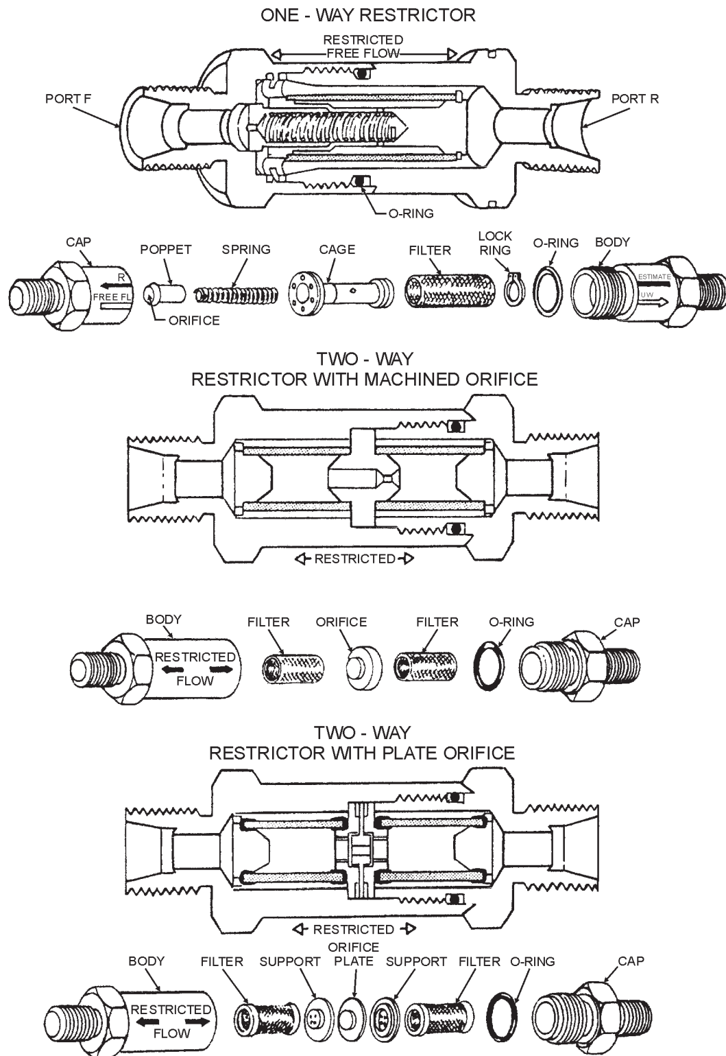
Figure 11-16.—Restrictors.
