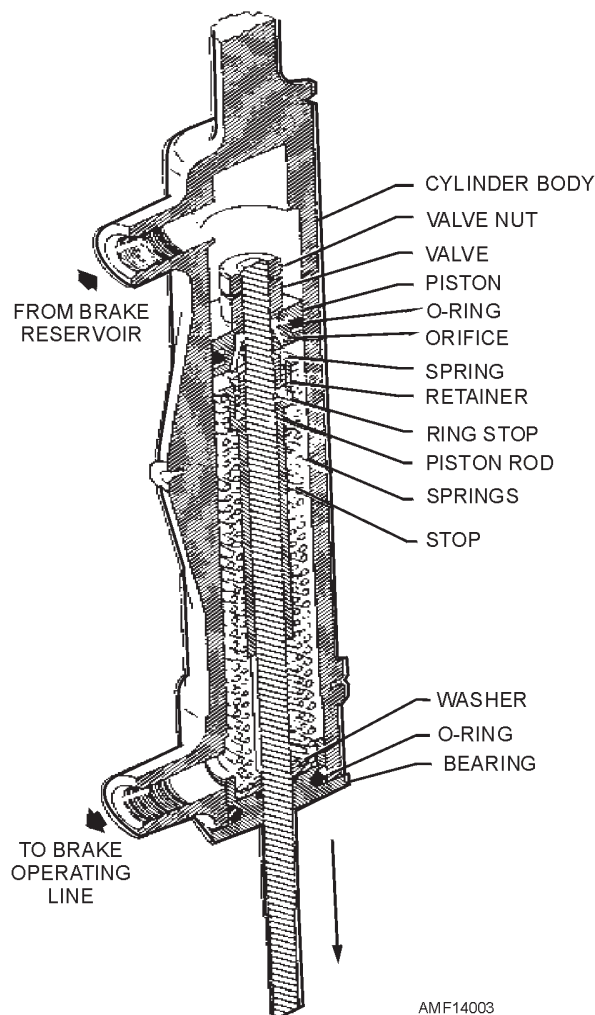
Figure 14-3.—Gladden master brake cylinder.
