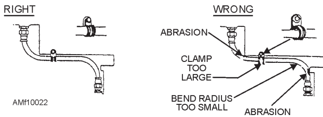
Figure 10-22.—Hose clamp mounting.
