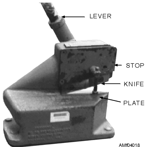
Figure 4-18.—Throatless shears.
