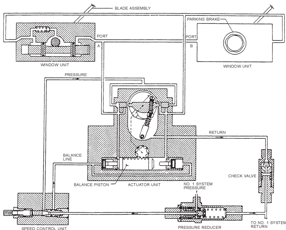
Figure 15-17.—Windshield wiper schematic.
