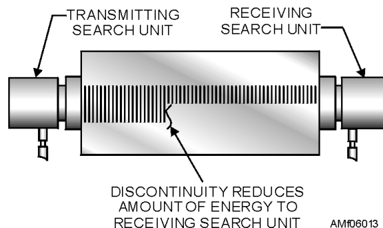
Figure 6-13.—Through-transmission inspection.
