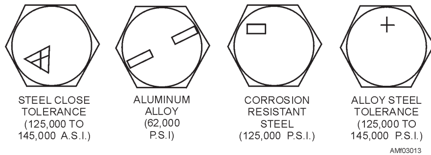
Figure 3-13.—Bolt head markings.
