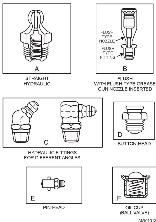
Figure 1-13.—Types of lubrication fittings.
