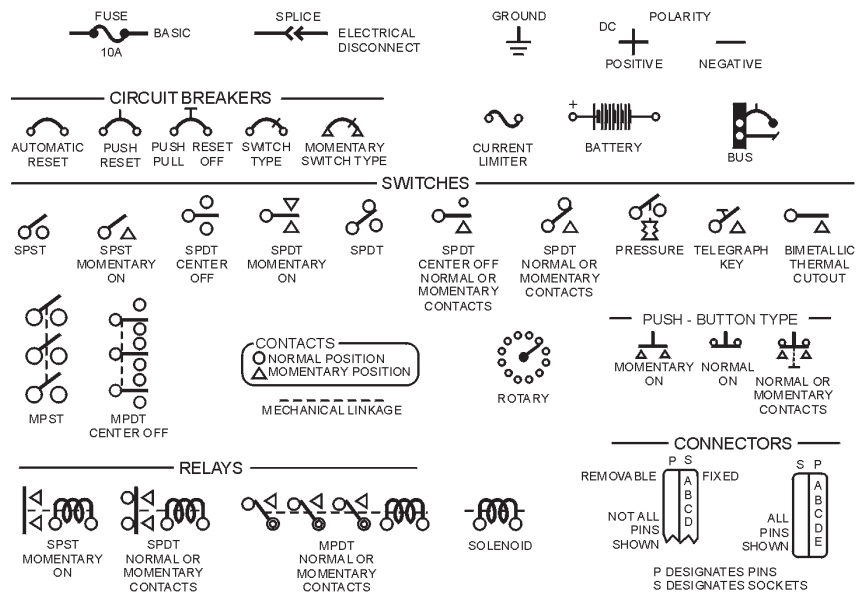
Figure 1-4.—Electrical symbols.
