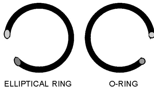
Figure 8-11.—Hydraulic seals.
