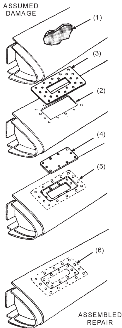
Figure 4-61.—Flush rectangular patch.
