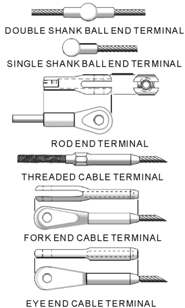
Figure 3-33.—Types of cable terminal fittings.
