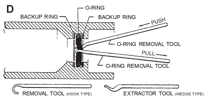
INTERNAL O-RING REMOVAL (USING WEDGE TYPE EXTRACTOR AND HOOK TYPE REMOVAL TOOLS)
