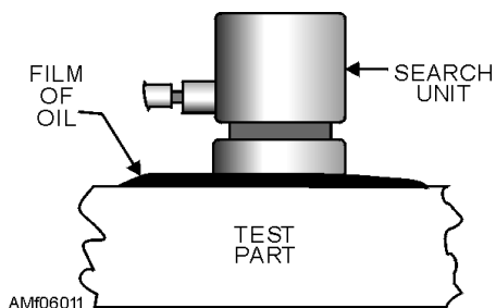
Figure 6-11.—Coupling of search unit to test part for transmission of ultrasonic energy.
