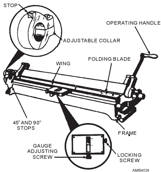
Figure 4-24.—Bar folder.
