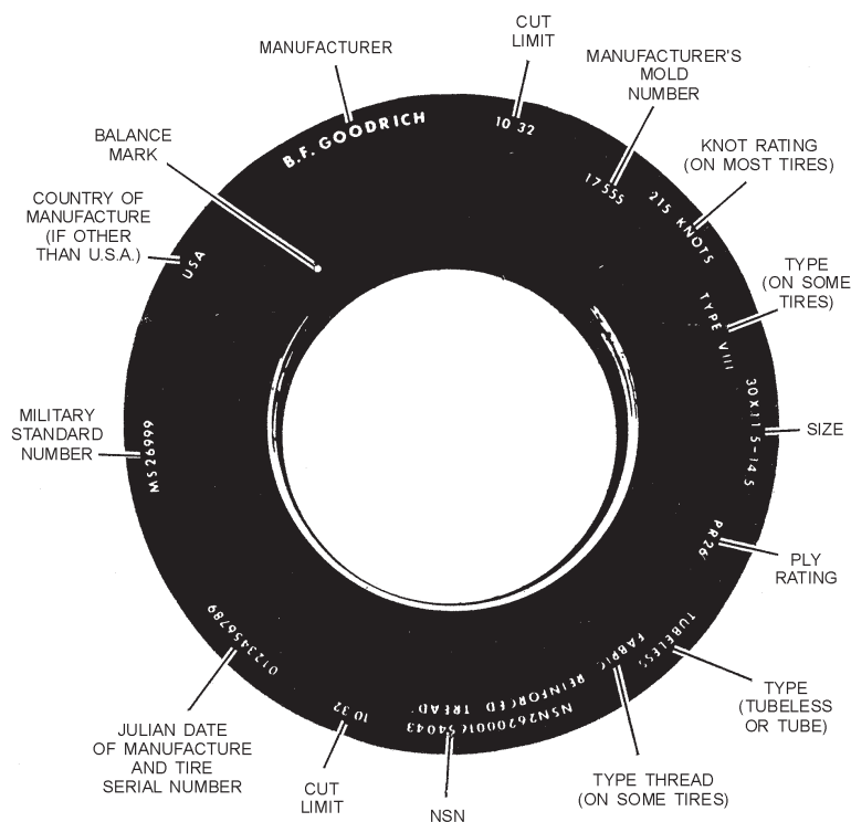
Figure 7-13.—New tire identification markings.
