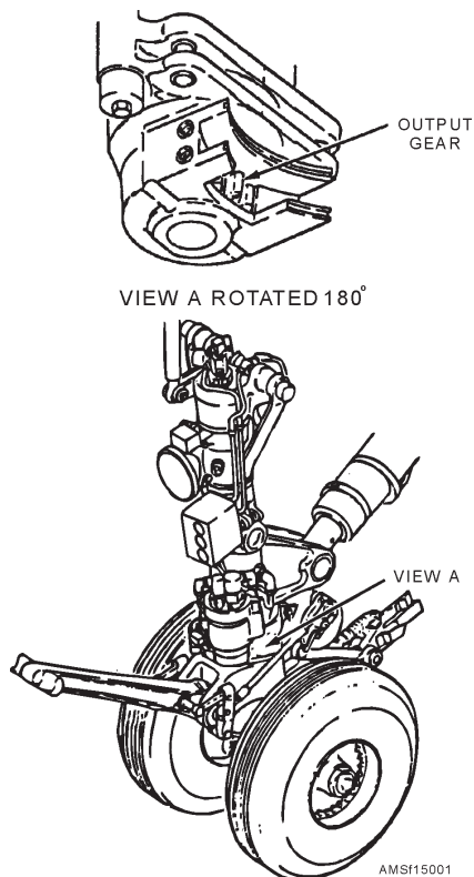
Figure 15-1.—Nosewheel steering power unit.
