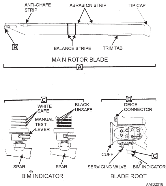
Figure 2-18.—H-60 main rotor blade pressurization system.
