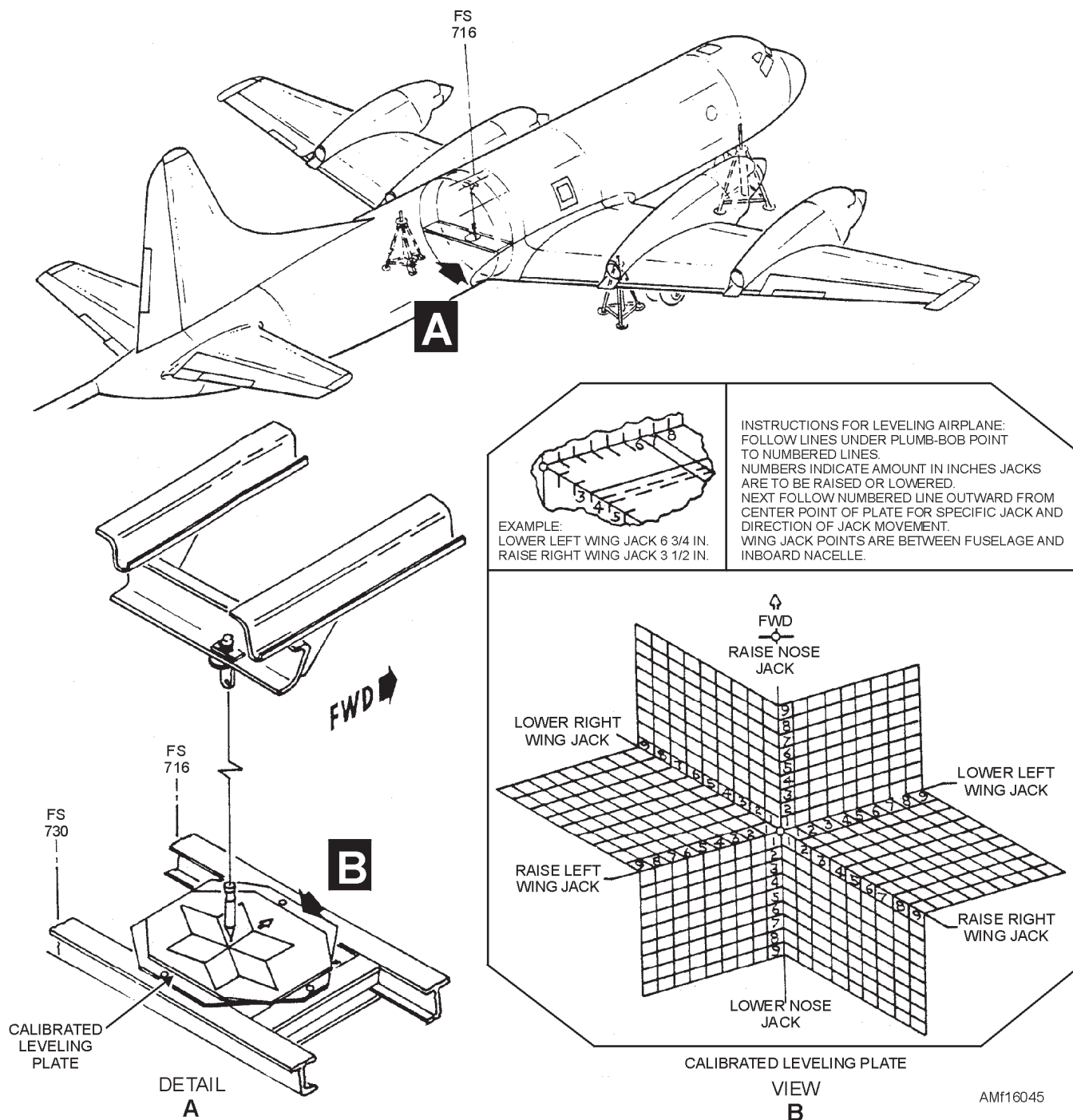
Figure 16-45.—Plumb bob and datum plate leveling.
