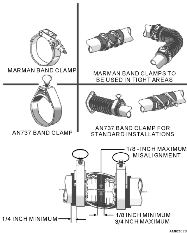
Figure 3-26.—Flexible line connectors.
