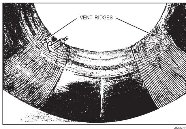
Figure 7-29.—Inner tube vent ridges.
