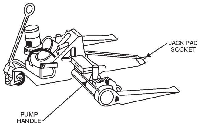
Figure 1-29.—Outrigger axle jack.
