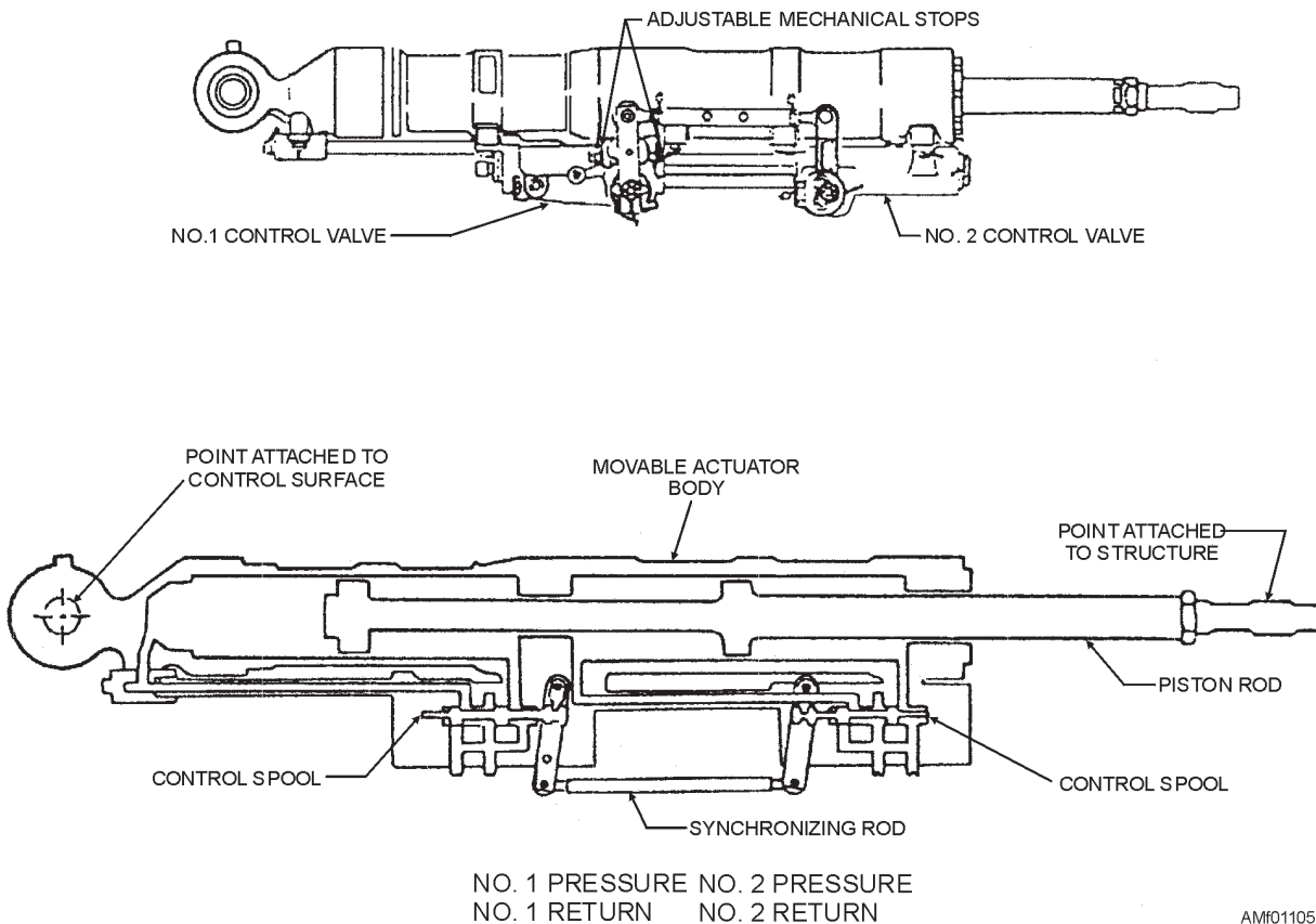
Figure 11-5.—Control surface actuating cylinder.
