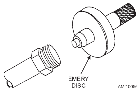
Figure 10-56.—Dynatube fitting resurfacing tool.
