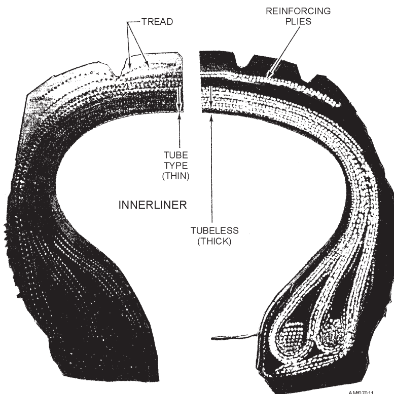
Figure 7-11.—Sectional view of two aircraft tires showing different construction details.
