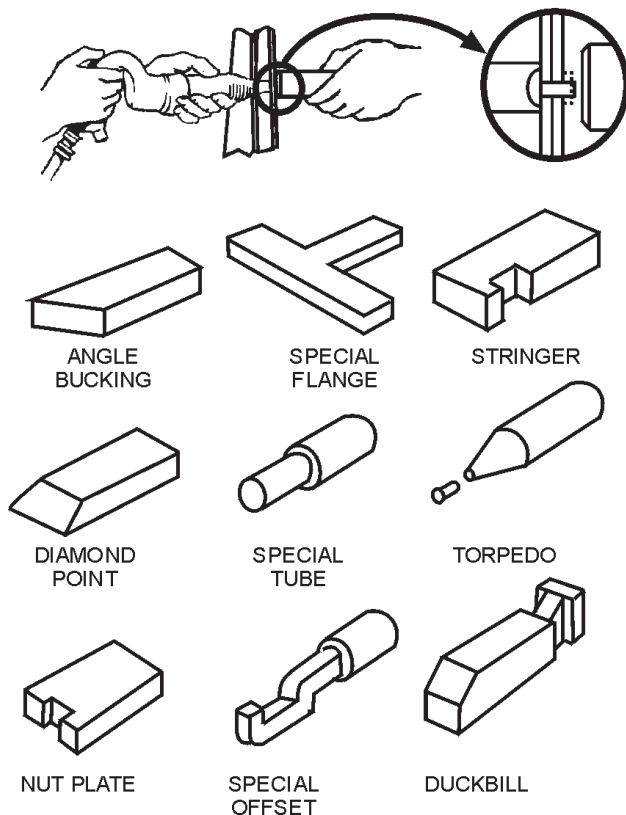
Figure 4-4.—Bucking bars.
