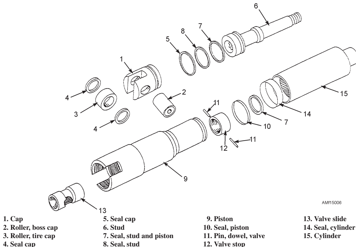
Figure 15-6.—Liquid spring shock assembly.
