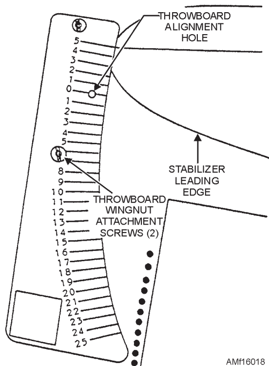
Figure 16-18.—Stabilizer throwboard installation.
