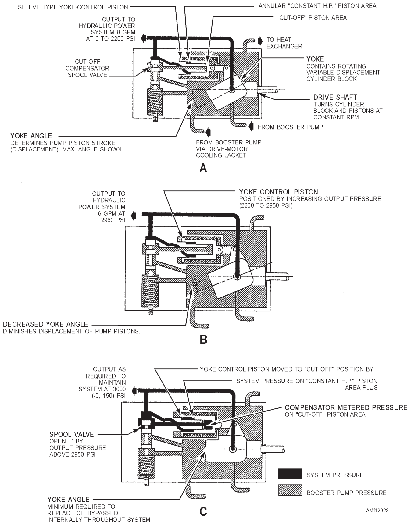
Figure 12-23.—Pump compensation. (A) full flow position; (B) reduced flow; (C) minimum flow.
