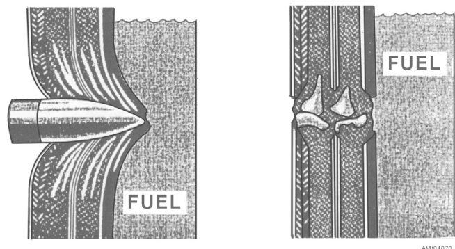
Figure 4-73.—Bullet-sealing action.
