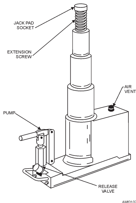
Figure 1-26.—Hand carried axle jack.
