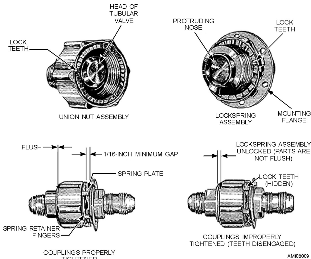
Figure 8-9.—Quick disconnects properly and improperly connected.
