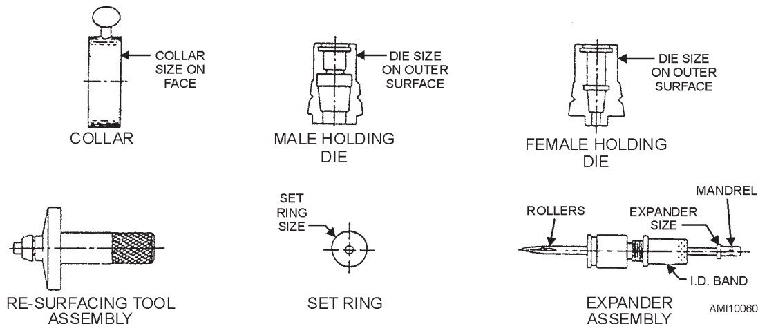
Figure 10-60.—Swaging and repair tool kit.
