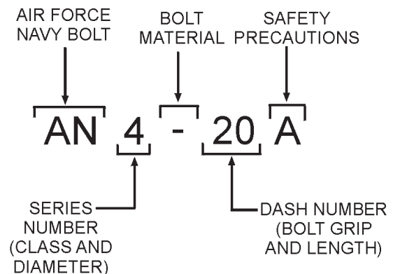
Figure 3-14.—AN bolt part number breakdown.
