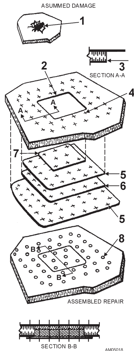
Figure 5-18.—Balsa wood repair with flush patch.
