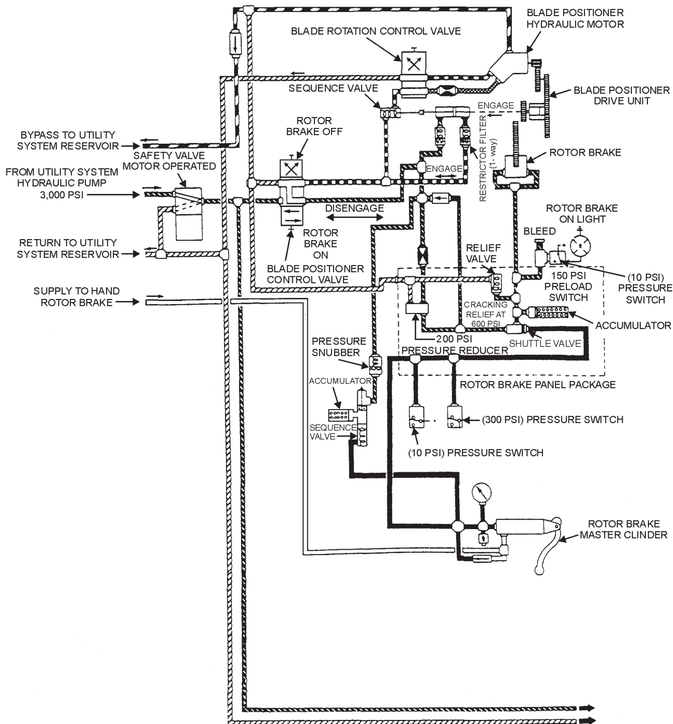
Figure 17-12.—Automatic blade folding system schematic.
