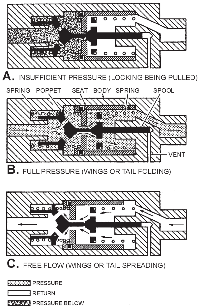
Figure 11-14.—View of priority valve.
