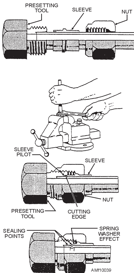
Figure 10-39.—Presetting flareless-tube assembly.
