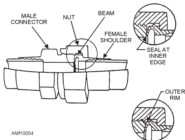
Figure 10-54.—Dynatube fitting.
