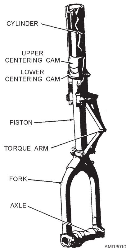
Figure 13-10.—Nose gear shock strut.
