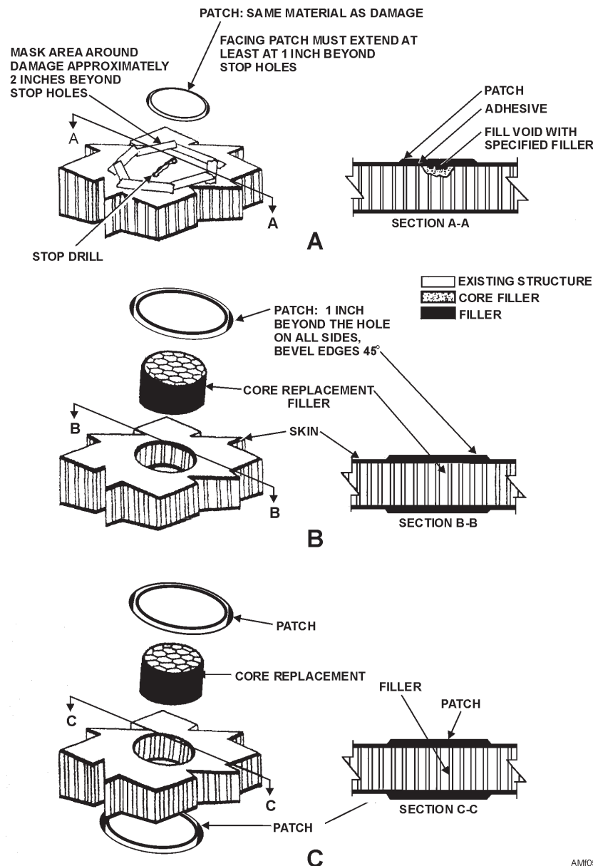
Figure 5-16.—Sandwich construction puncture repair (honeycomb core).
