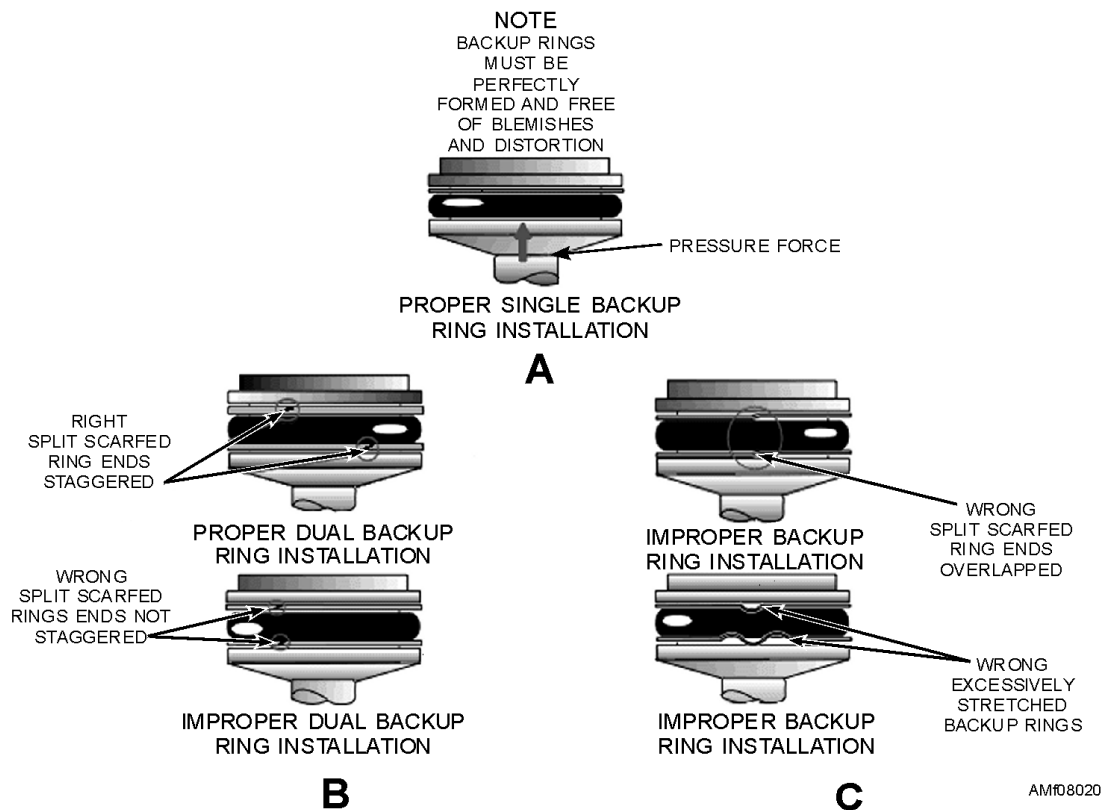
Figure 8-20.—Teflon® backup ring installation (external).
