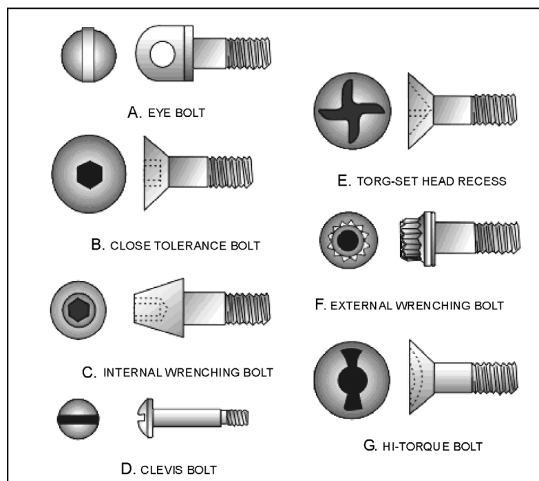
Figure 3-12.—Bolt Heads.
