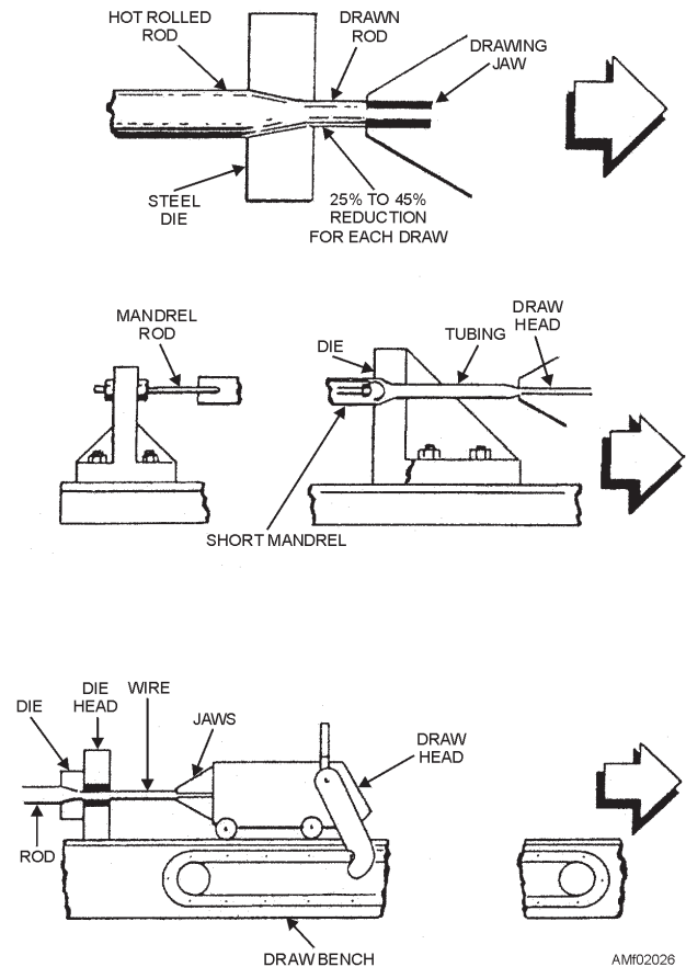
Figure 2-26.—Cold drawing operation for rods, tubing, and wire.
