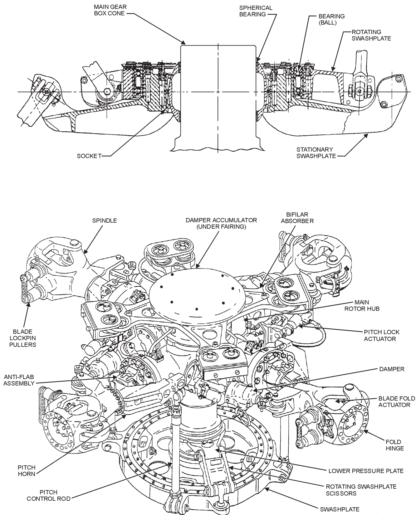
Figure 17-9.—Swashplate—cross-sectional and installed view.
