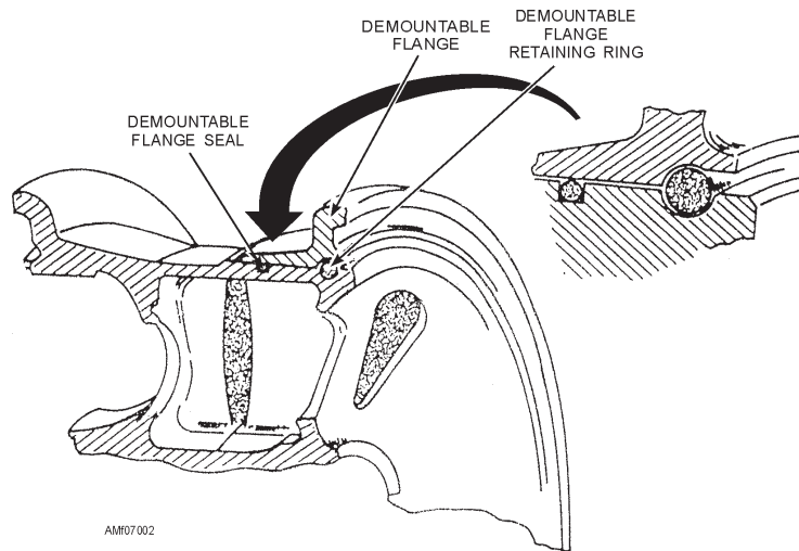
Figure 7-2.—Demountable flange wheel.
