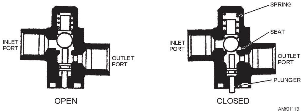
Figure 11-13.—Typical sequence valve.
