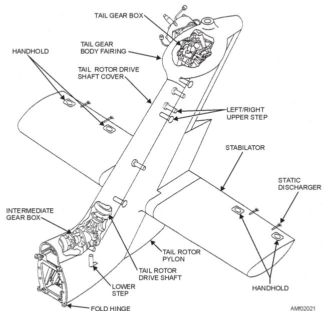
Figure 2-21.—H-60 tail pylon.
