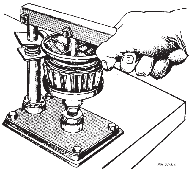
Figure 7-8.—Pressure repacking of wheel bearings.
