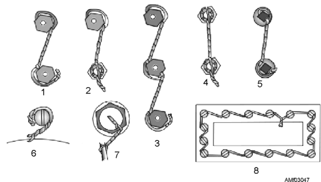
Figure 3-47.—Safety wiring methods.
