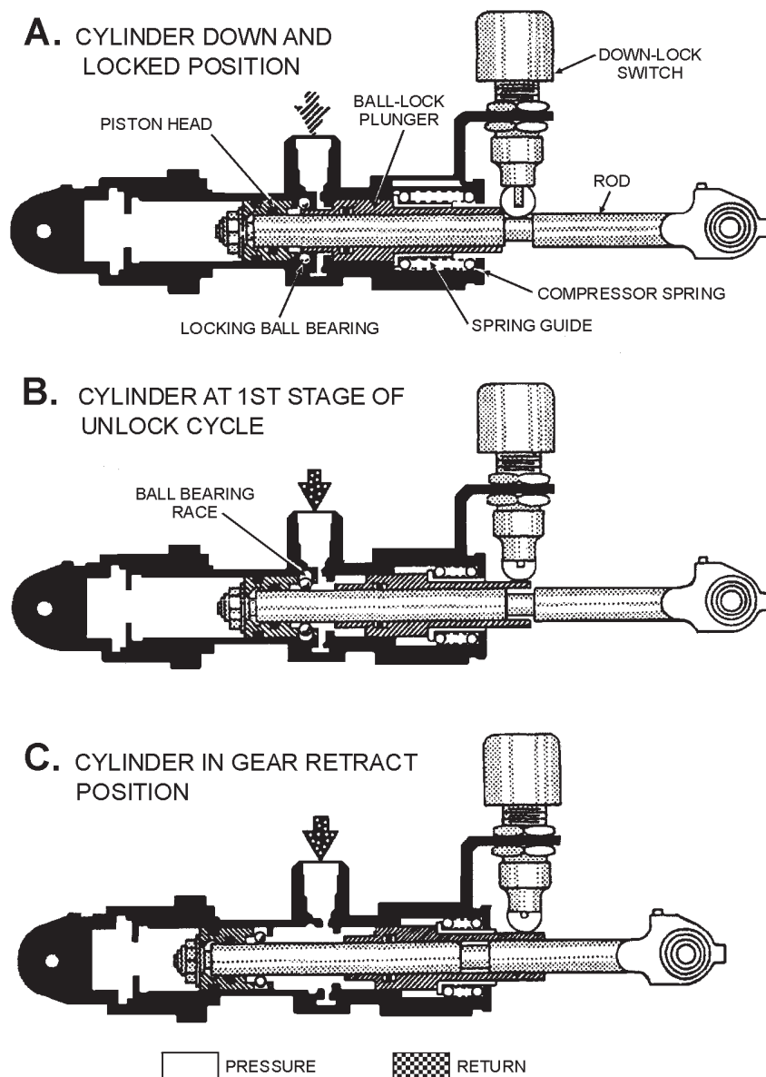
Figure 11-3.—Cutaway of a single-action, ball-lock actuating cylinder.
