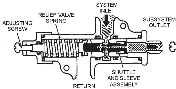
Figure 11-17.—Pressure-reducing valve operational schematic.
