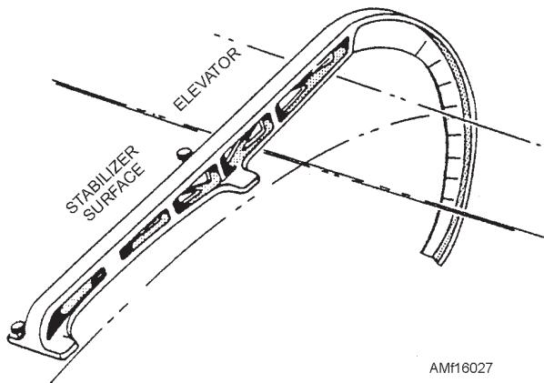
Figure 16-27.—Elevator rigging fixture.
