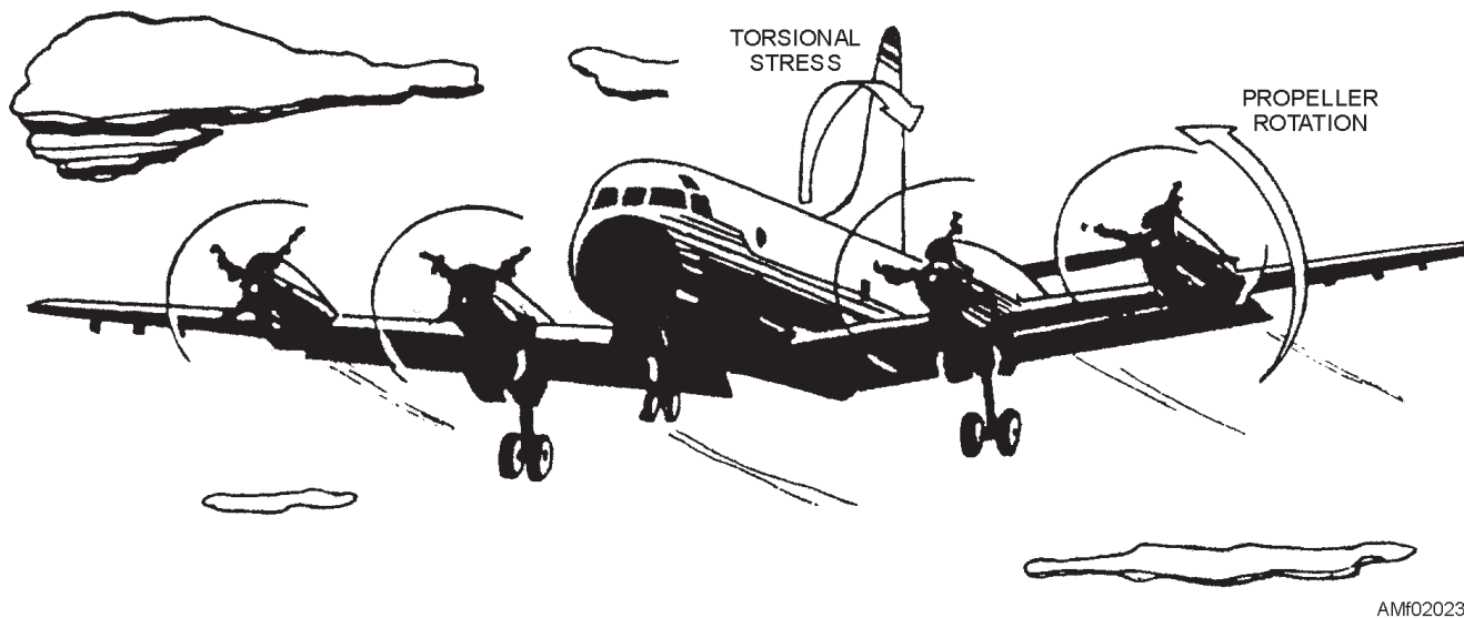
Figure 2-23.—Engine torque creates torsional stress in aircraft fuselages.
