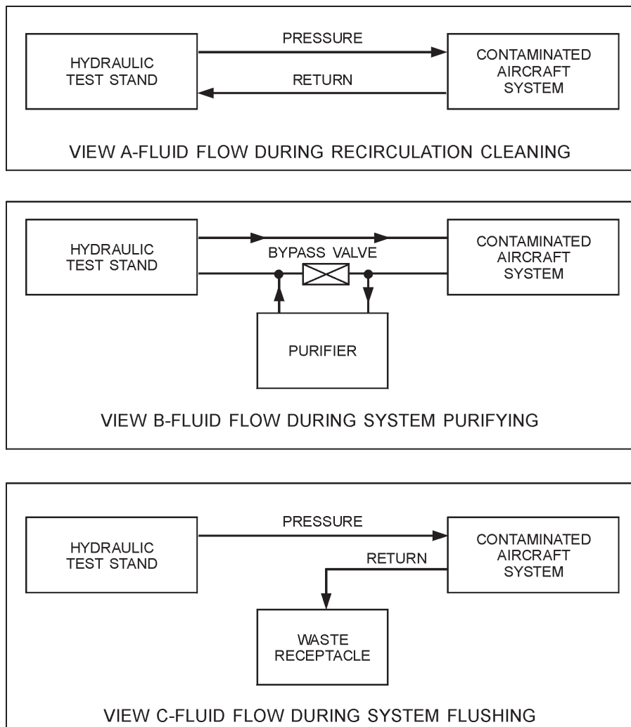
Figure 8-6.—Fluid flow during decontamination.
