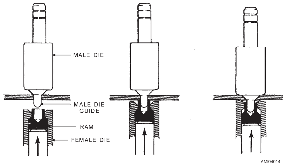
Figure 4-14.—Dimple countersinking.
