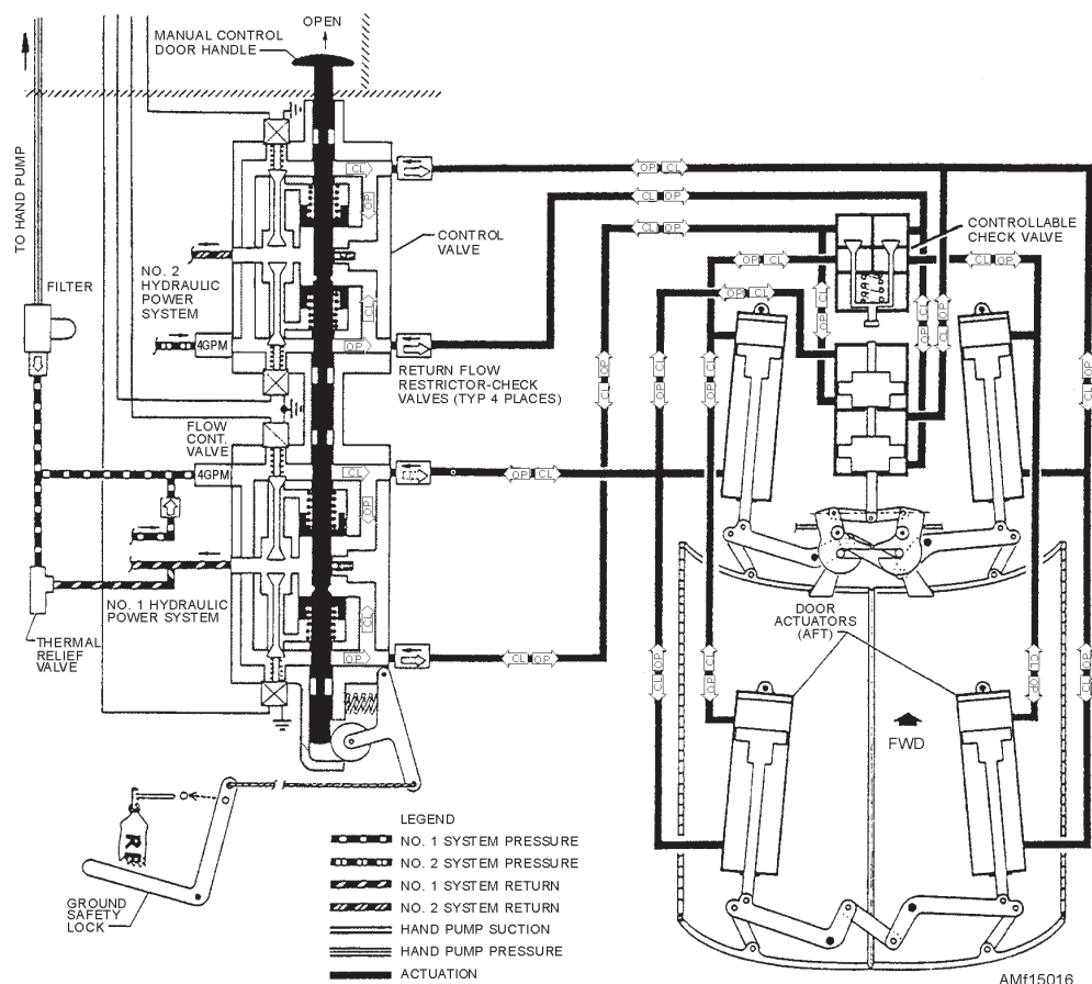
Figure 15-16.—Bomb bay door hydraulic schematic.
