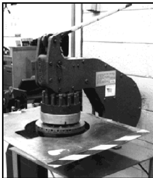
Figure 4-20.—Hand-operated turret punch.
