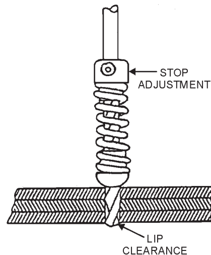
Figure 5-28.—Drill stop.
