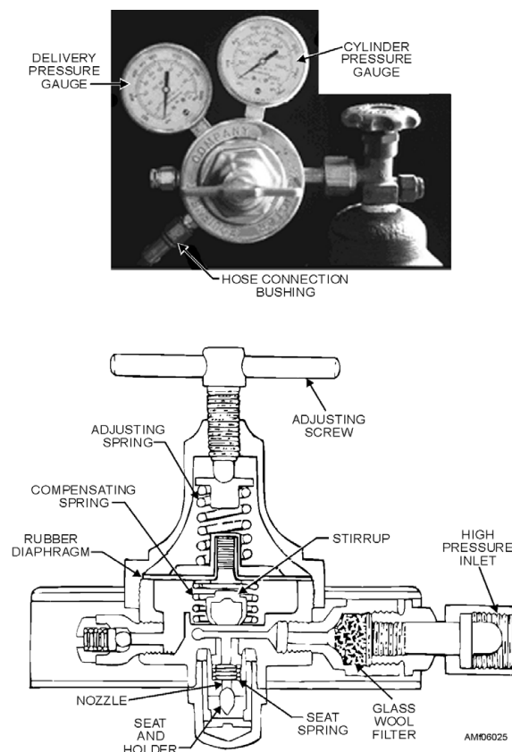
Figure 6-25.—Single-stage oxygen regulator.
