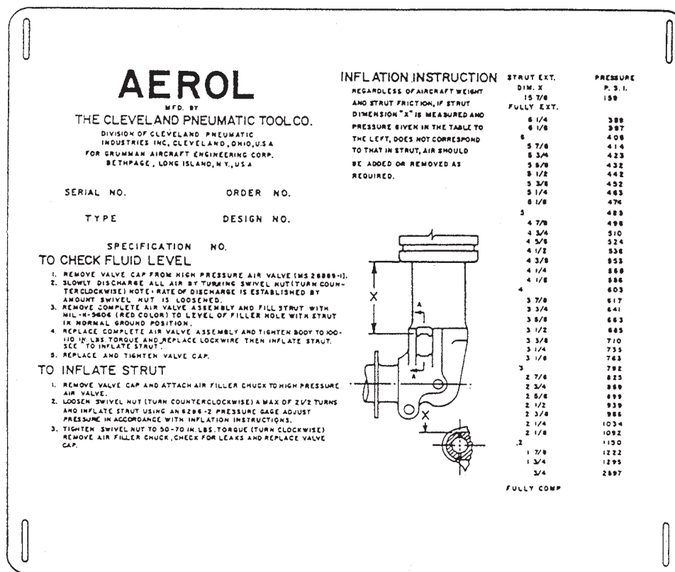
Figure 13-16.—Landing gear strut servicing instruction plate.
