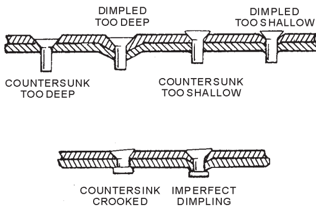
Figure 4-45.—Incorrect countersinking.
