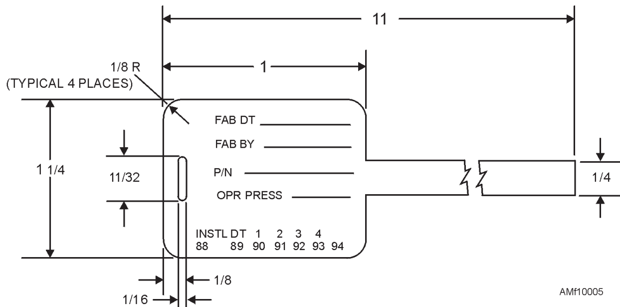
Figure 10-5.—Hose assembly identification tags.
