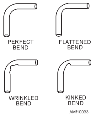
Figure 10-33.—Tubing bends.
