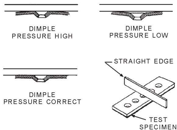
Figure 4-16.—Checking dimple equipment air pressure.
