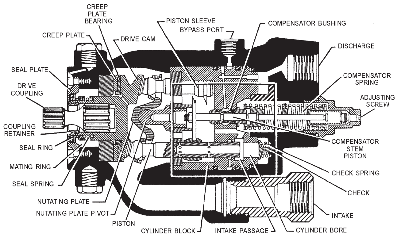
Figure 12-16.—Internal features of the Stratopower pump.
