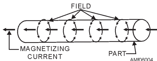
Figure 6-4.—Magnetic field in part used as a conductor.
