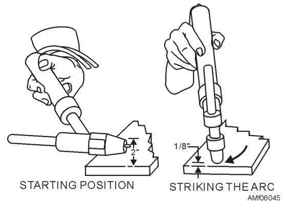
Figure 6-45.—Starting the arc.
