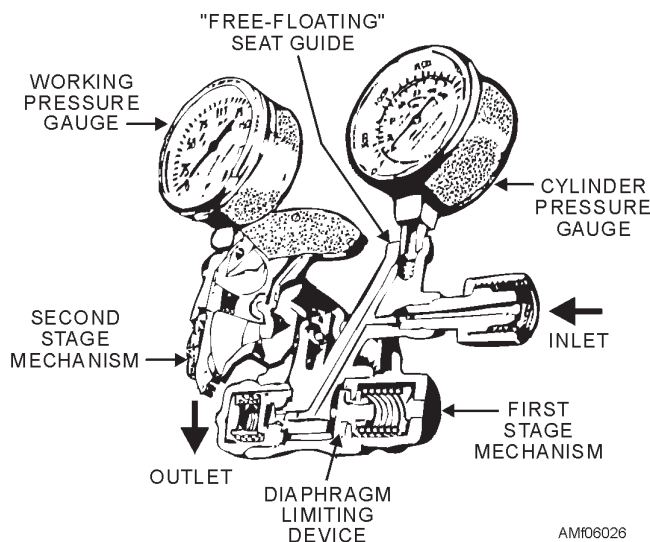
Figure 6-26.—Two-stage regulator.
