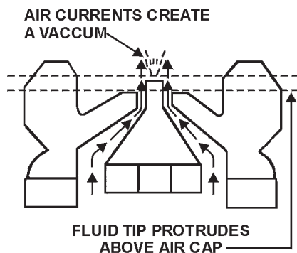
Figure 5-34.—Suction and pressure fluid tips and air caps.
