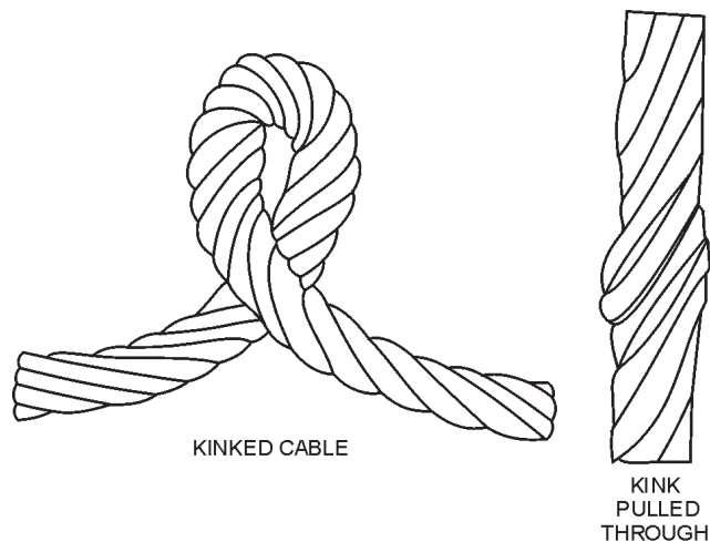
Figure 1-25.—Cable damage resulting from a pulled-through kink.
