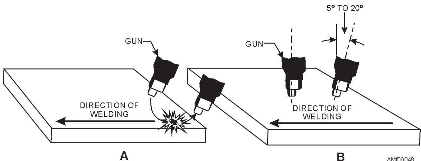
Figure 6-48.—Gas metal-arc welding. (A) striking the arc; (B) gun angle.
