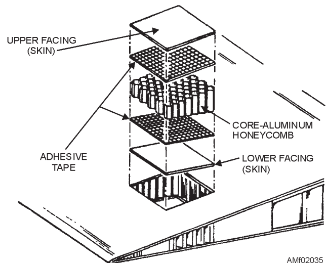
Figure 2-35.—Sandwich construction.
