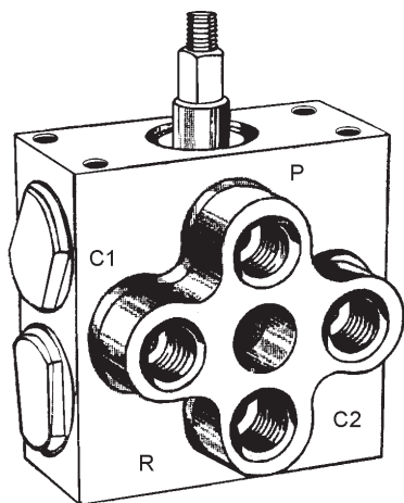
Figure 11-7.—Poppet-type selector valve.
