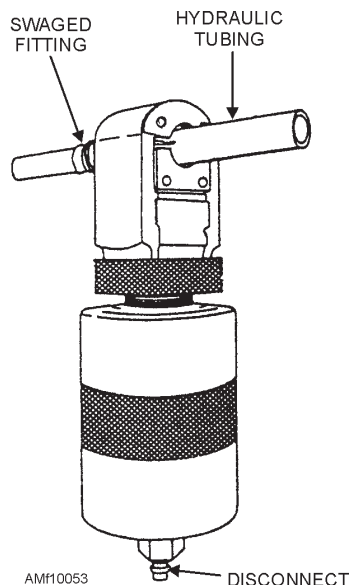
Figure 10-53.—Series D12200 kit swage tool operation.
