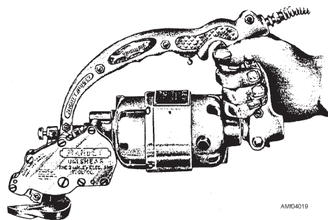
Figure 4-19.—18-gauge Unishear.
