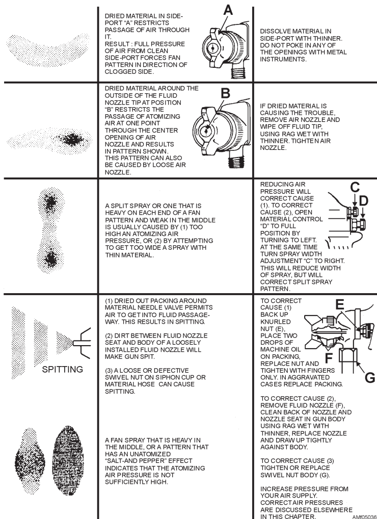
Figure 5-36.—Faulty spray patterns and how to correct them.
