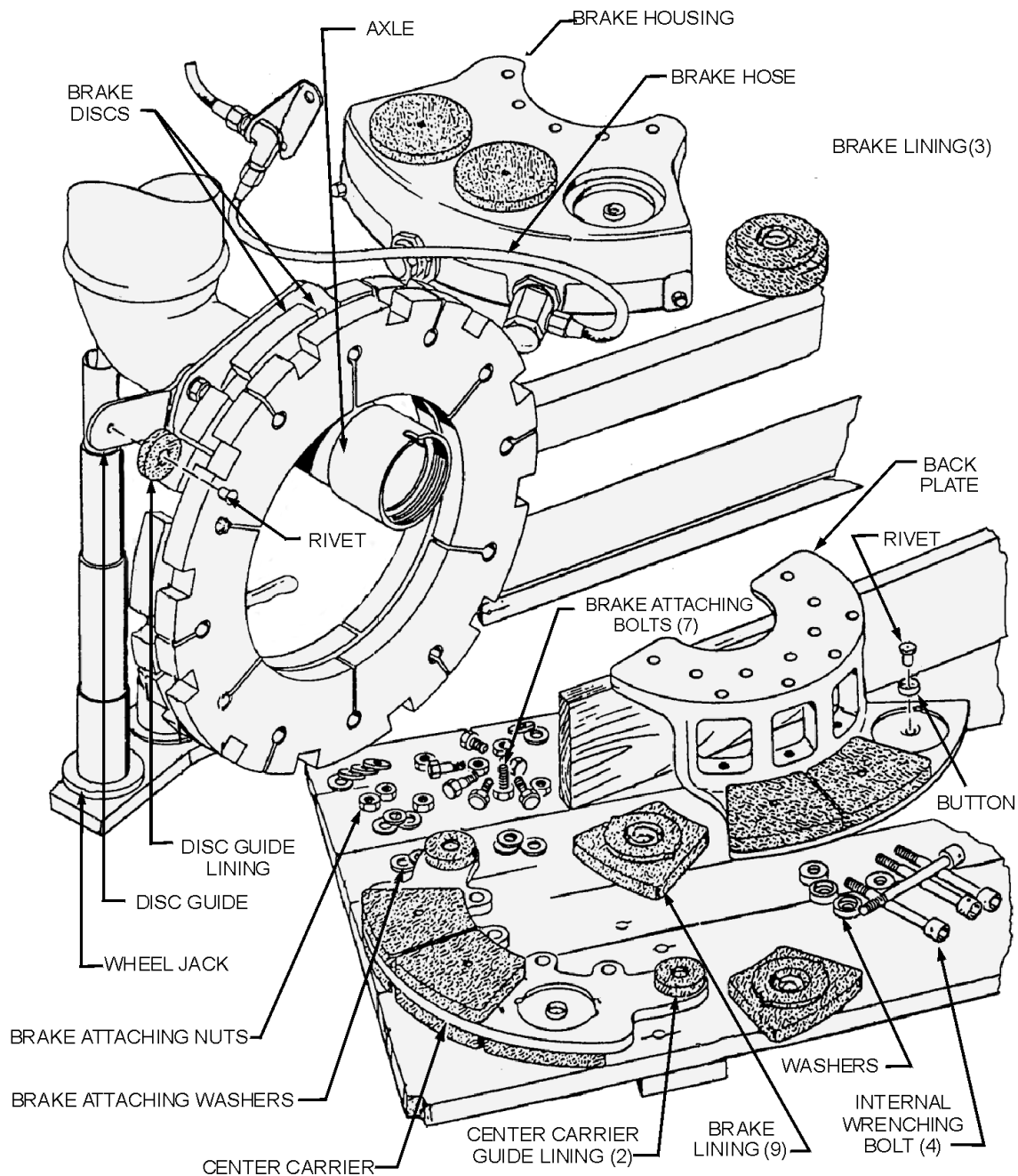
9541299 BRAKE ASSEMBLY
