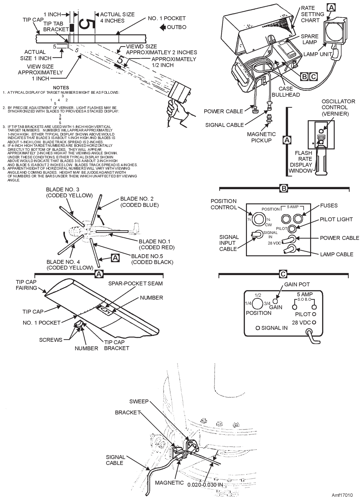
Figure 17-10.—Blade tracking—Strobex.
