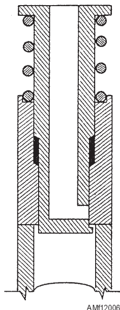
Figure 12-6.—Manual air bleed valve.
