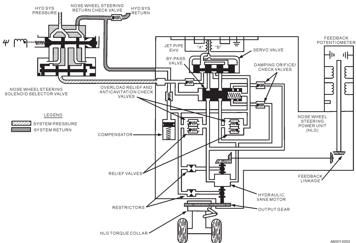
Figure 15-2.—Nosewheel steering system schematic.
