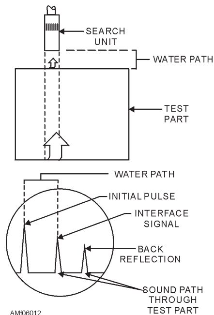
Figure 6-12.—Immersion method.
