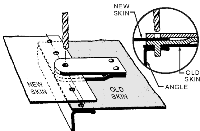
Figure 4-66.—Using a hole finder.
