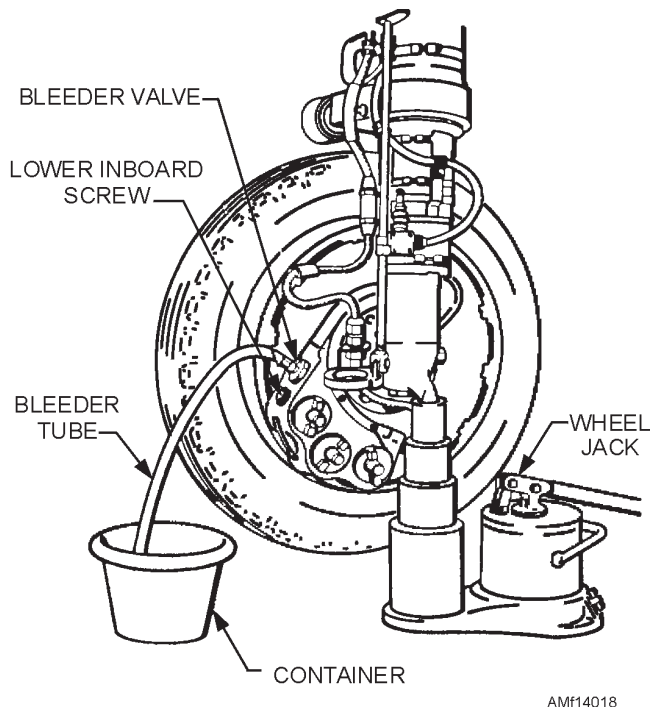
Figure 14-18.—Bleeding brake system (top-down method).
