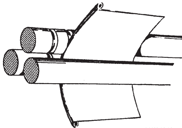
Figure 4-40.—Rolling a wired edge.
