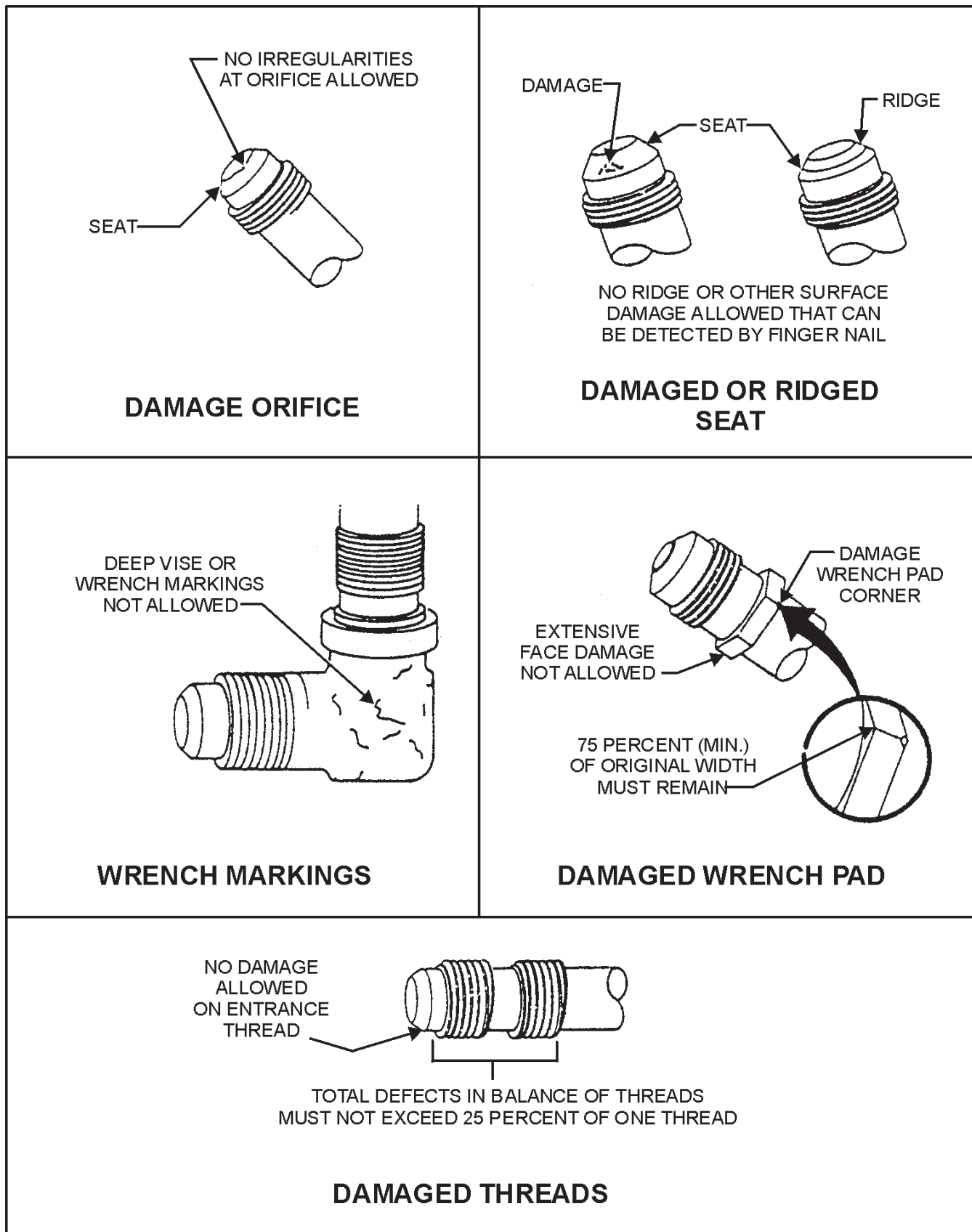
Figure 10-44.—Damaged fittings.
