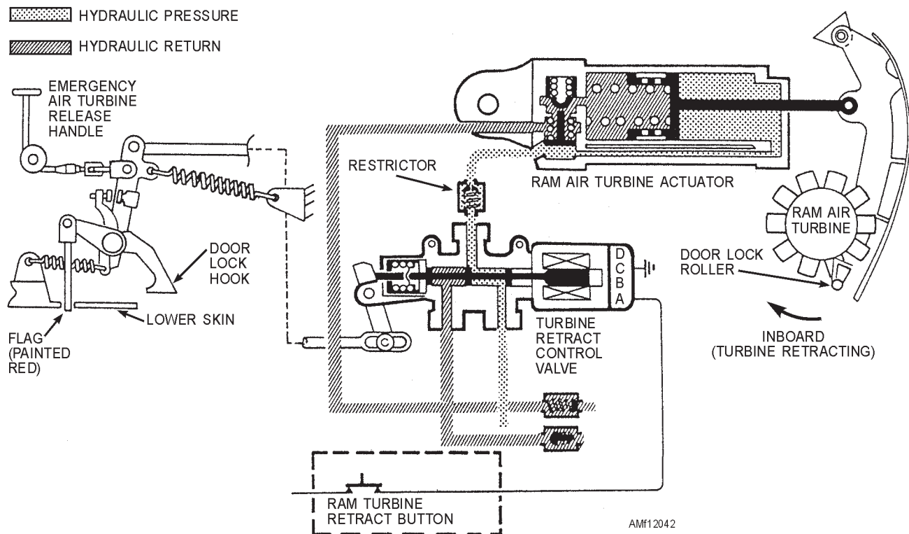
Figure 12-42.—Ram air turbine-control system schematic.
