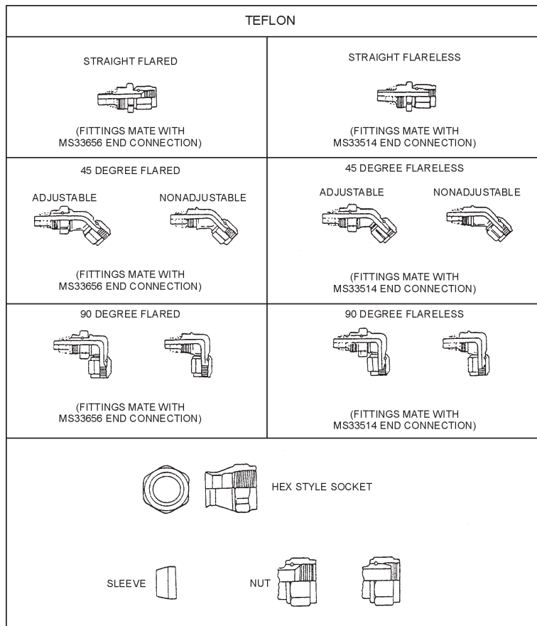
Figure 10-4.—Teflon® hose fittings.
