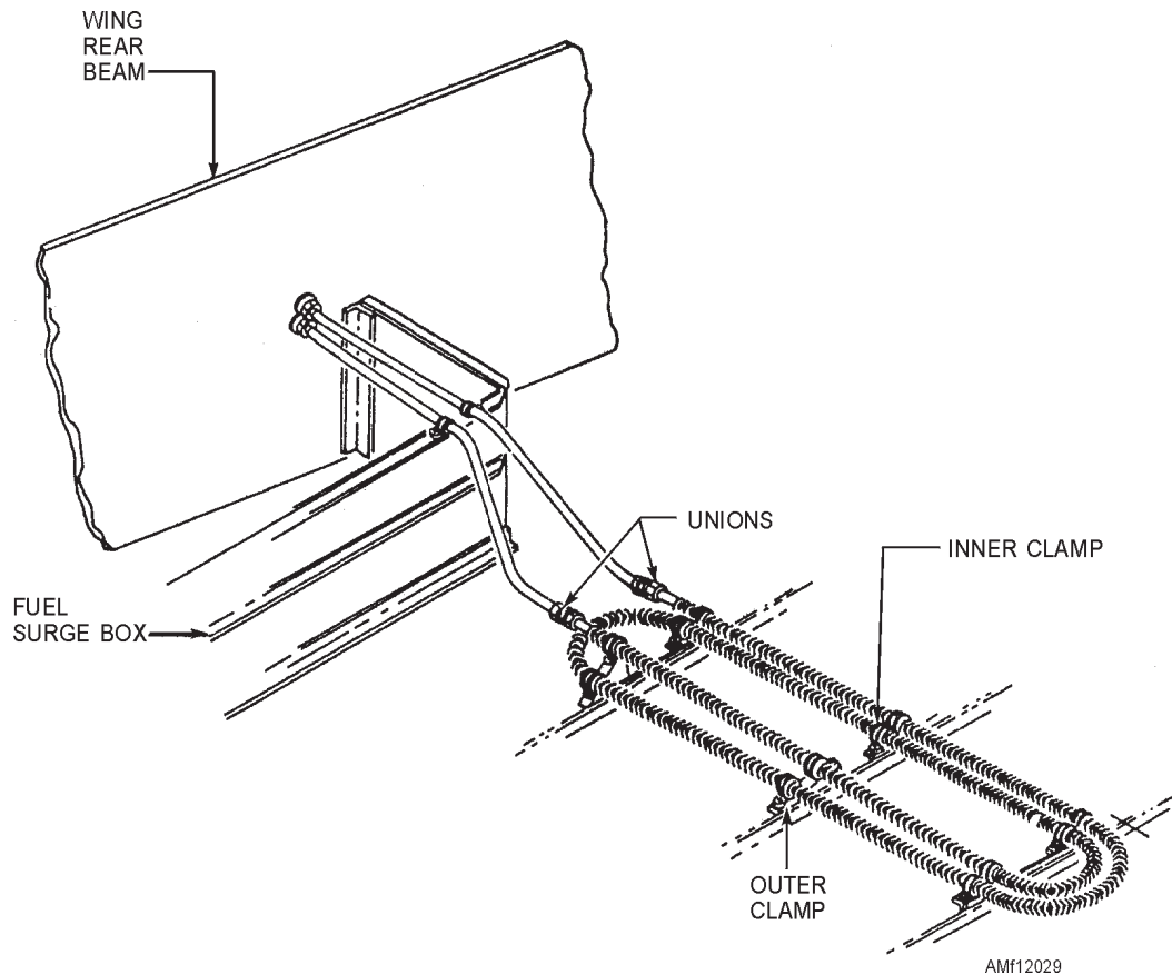
Figure 12-29.—Fin tubing assembly installation.
