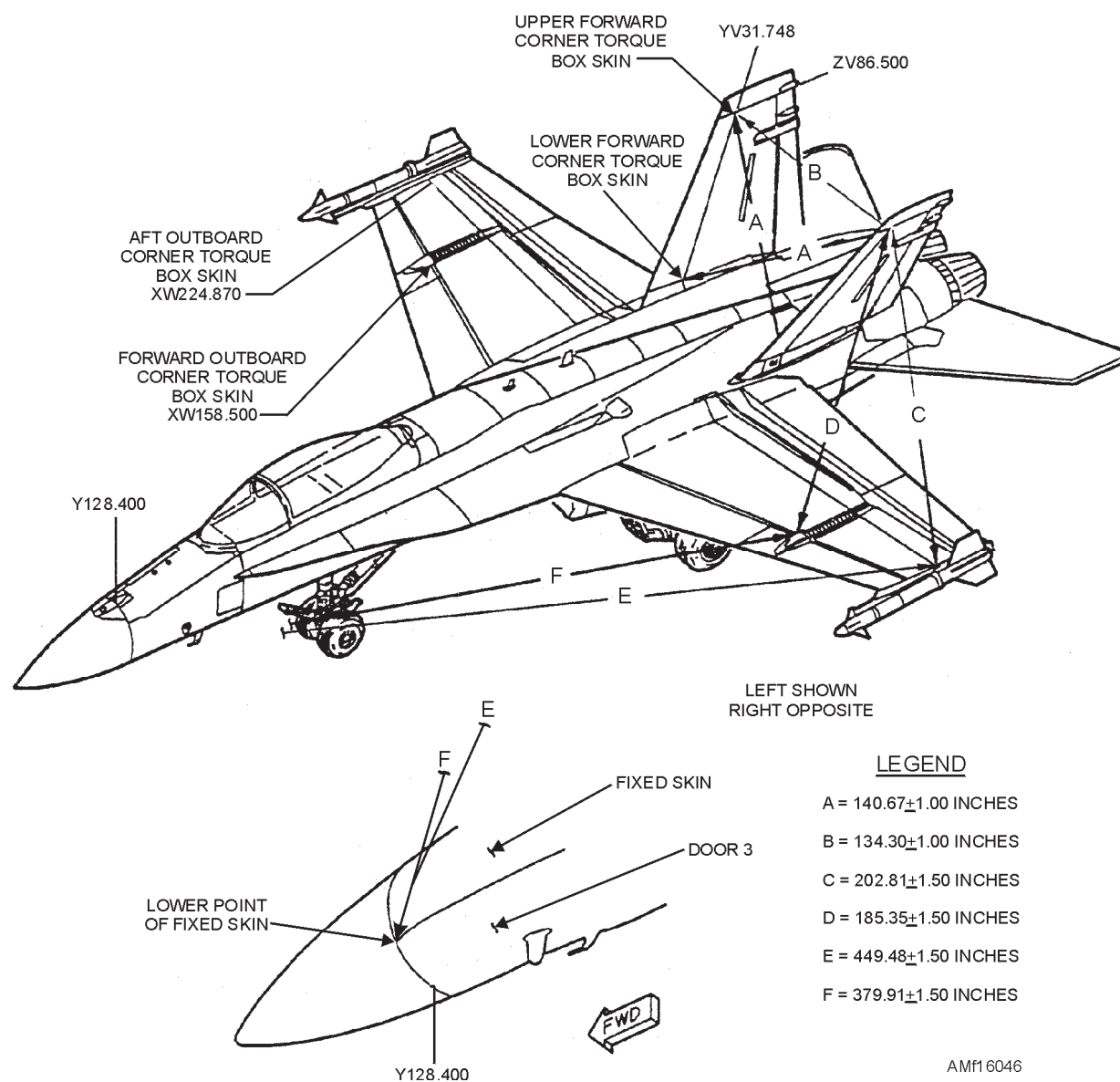
Figure 16-46.—Structure alignment dimensions.
