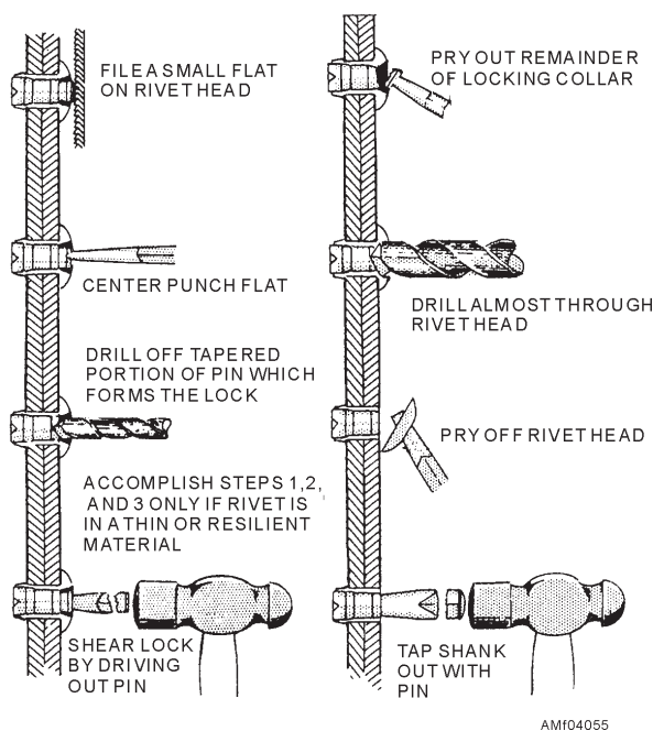
Figure 4-55.—Removing self-plugging rivets (mechanical lock).
