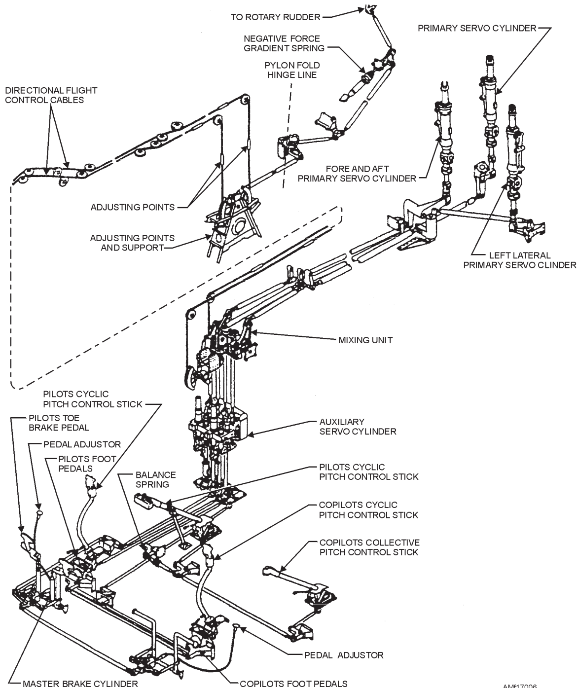
Figure 17-6.—Flight control systems.
