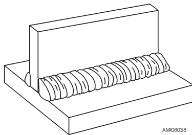
Figure 6-38.—Tee joint—single pass fillet weld.
