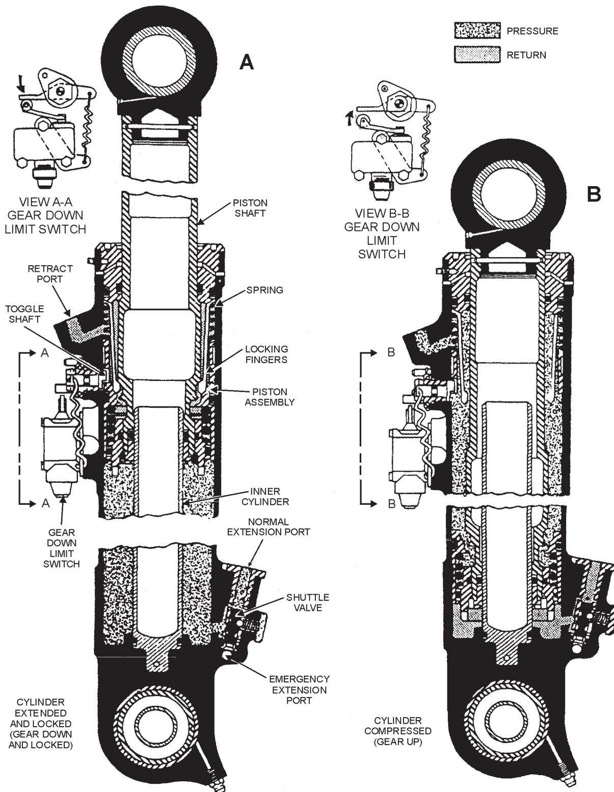
Figure 11-4.—Typical finger-lock actuating cylinder.
