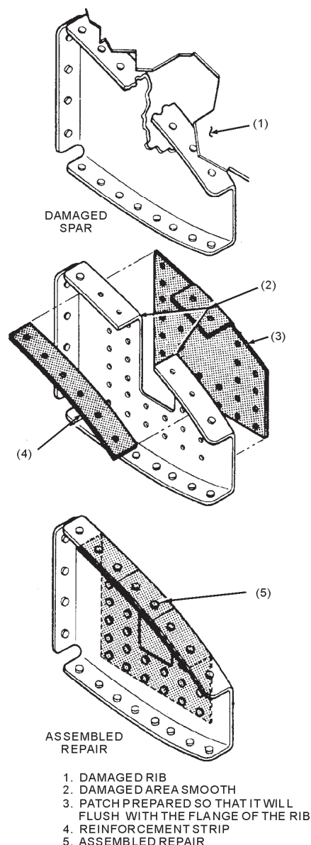
Figure 4-71.—Rib repair by patching.
