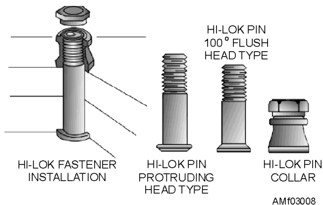
Figure 3-8.—Hi-lok fastener.
