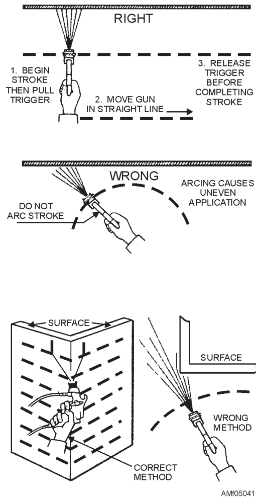
Figure 5-41.—Correct and incorrect methods of spraying.
