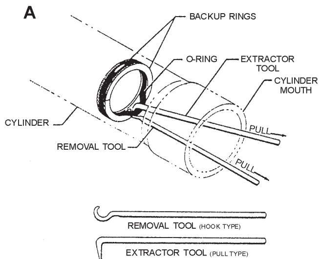
INTERNAL O-RING REMOVAL (USING PULL TYPE EXTRACTOR AND HOOK TYPE REMOVAL TOOLS)
