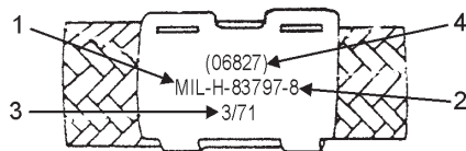
WIRE BRAID COVERED SYNTHETIC RUBBER HOSE
