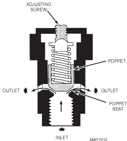
Figure 12-10.—Air relief valve.
