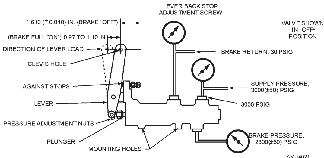
Figure 14-21.—Operational test setup—power brake valve.
