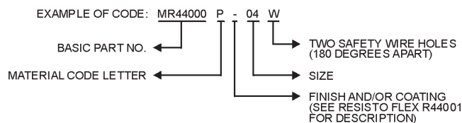
Figure 10-28.—Typical style of Dynatube fittings.
