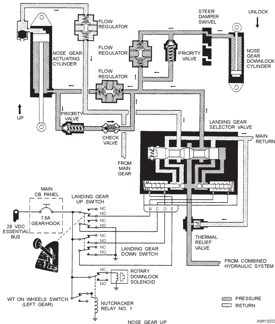
Figure 13-2.—Nose gear up cycle schematic.
