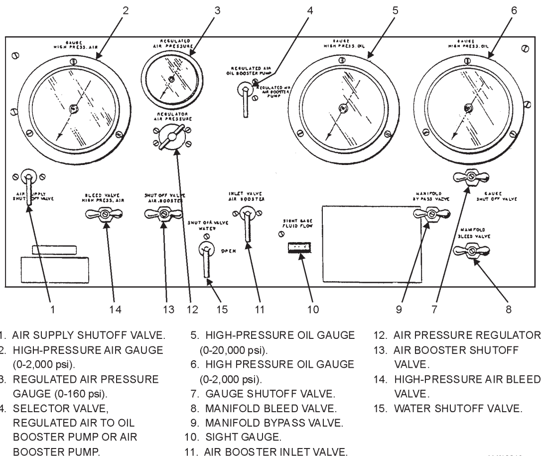
Figure 10-19.—Controls and instruments.
