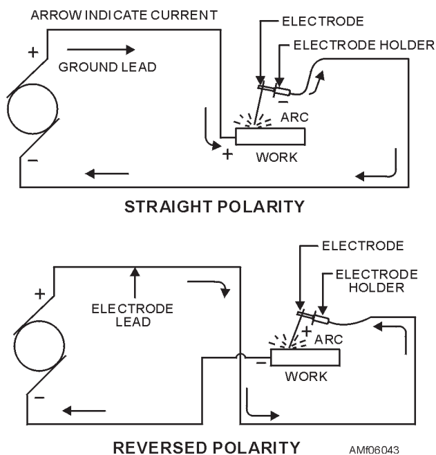
Figure 6-43.—Straight and reverse polarity in electric welding.
