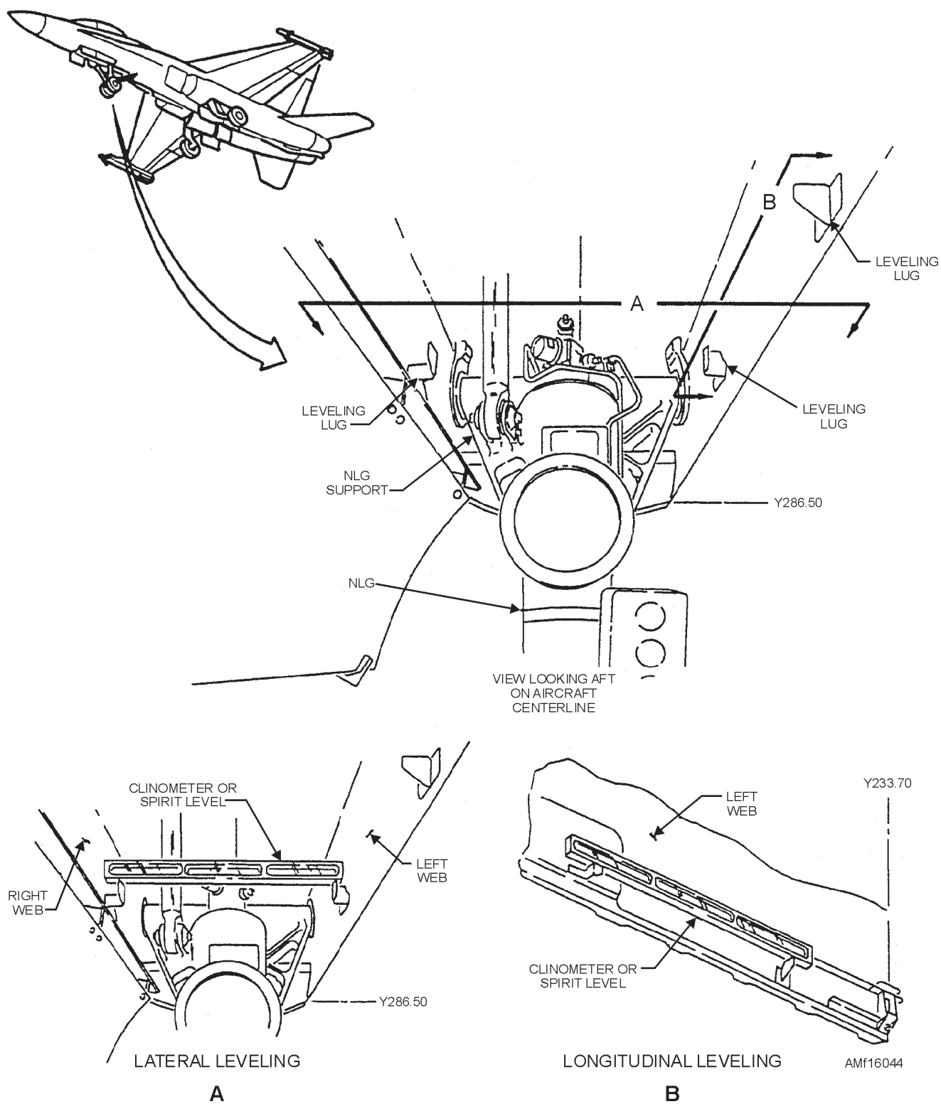
Figure 16-44.—Spirit leveling lugs.
