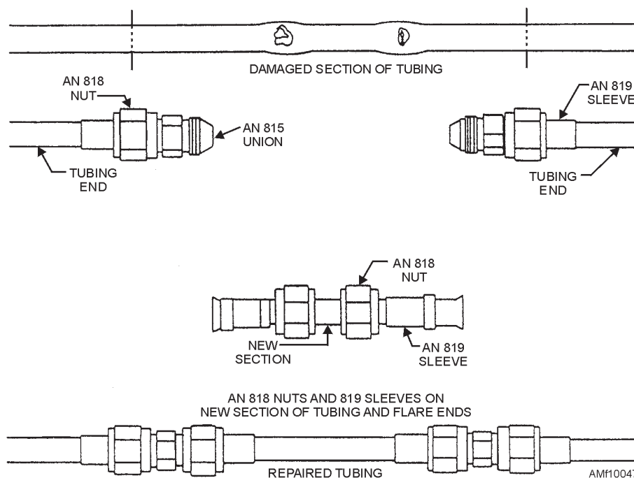
Figure 10-47.—Temporary tubing repair.
