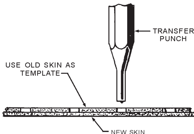
Figure 4-65.—Transferring rivet holes.
