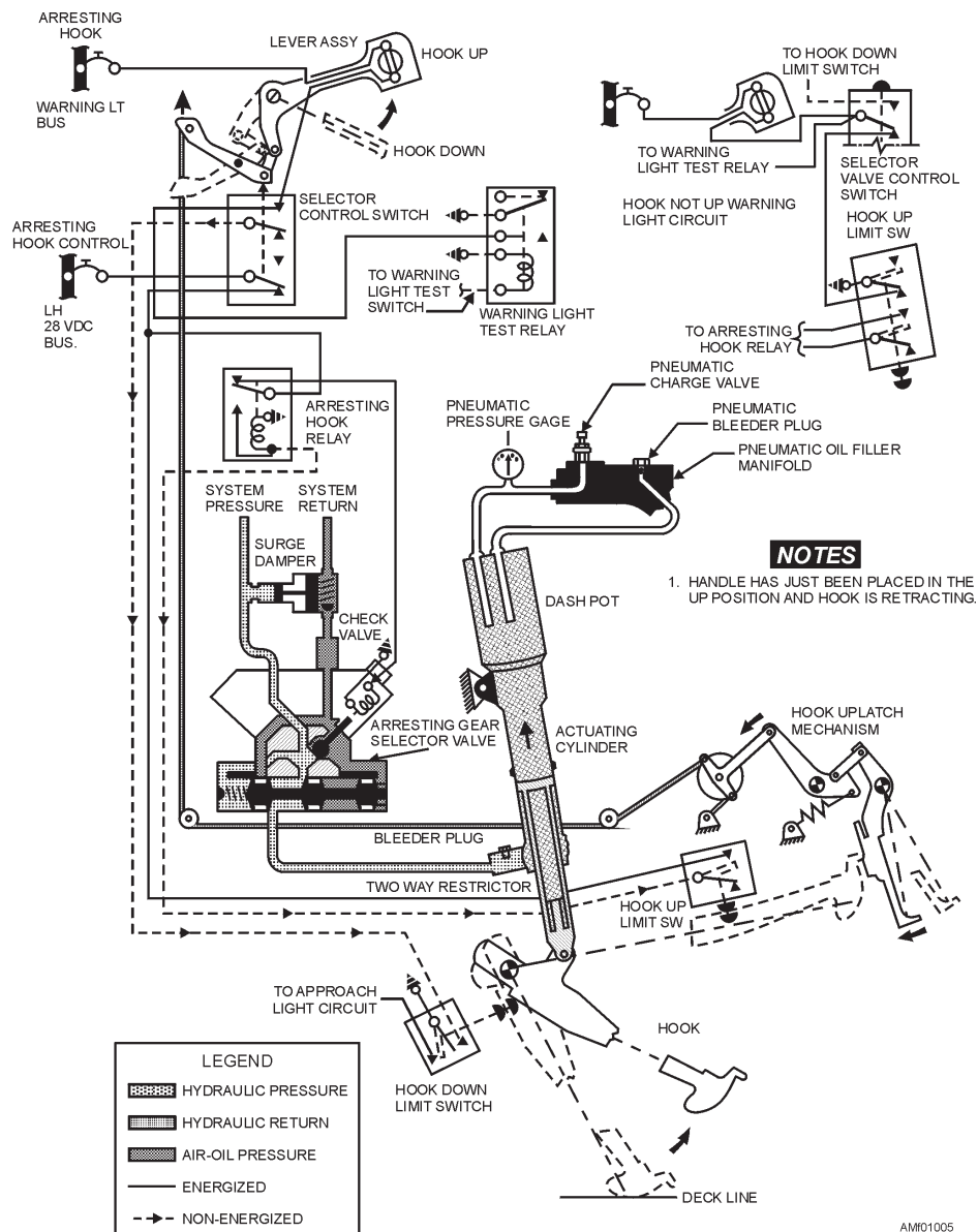
Figure 1-5.—Arresting gear system schematic.
