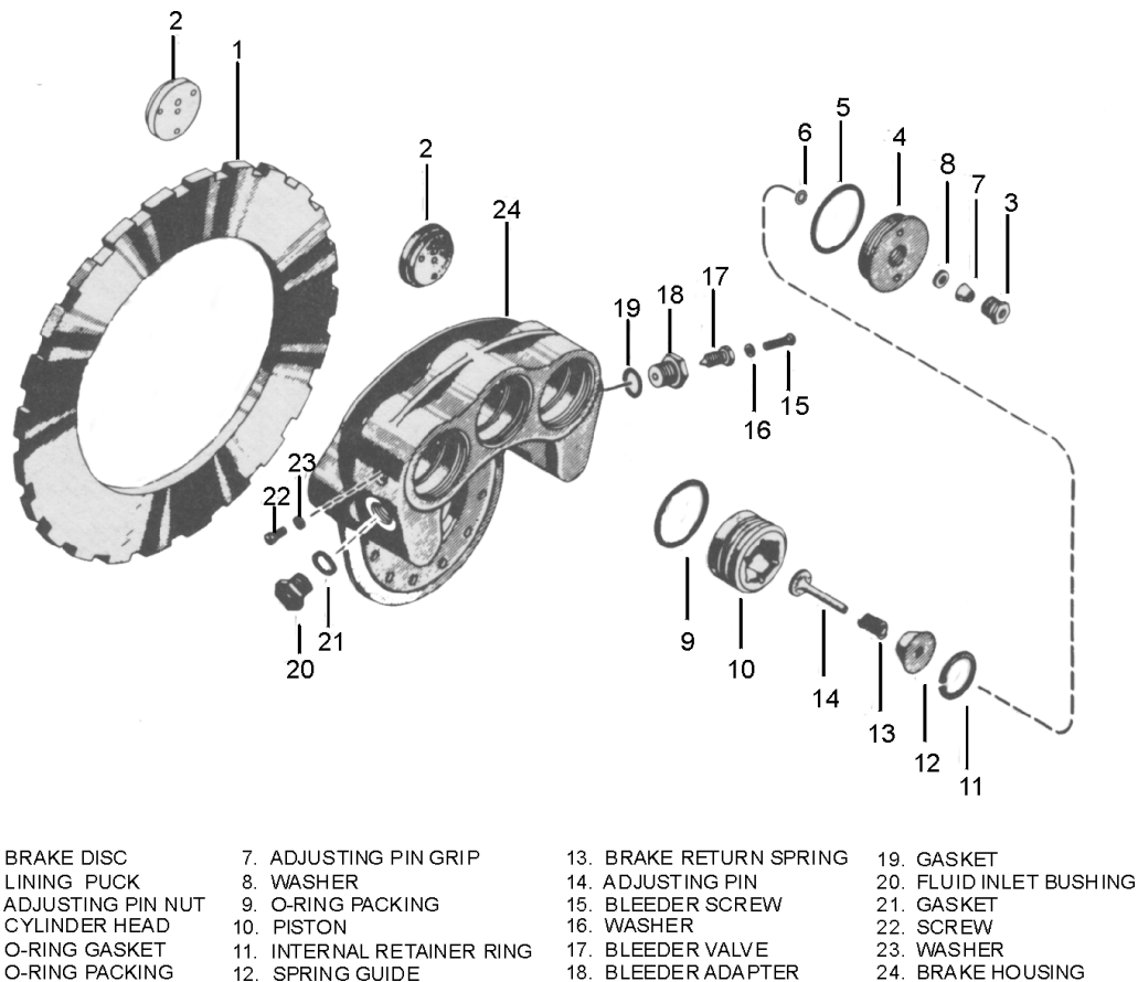
Figure 14-10.—Exploded view of single disc brake assembly.
