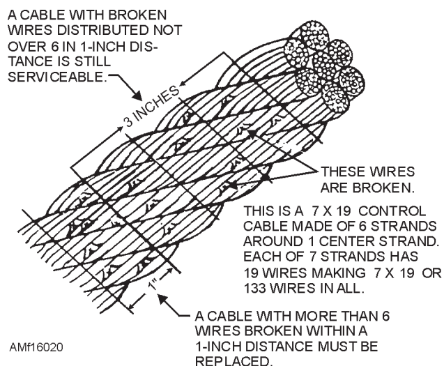
Figure 16-20.—Determining serviceable cable.
