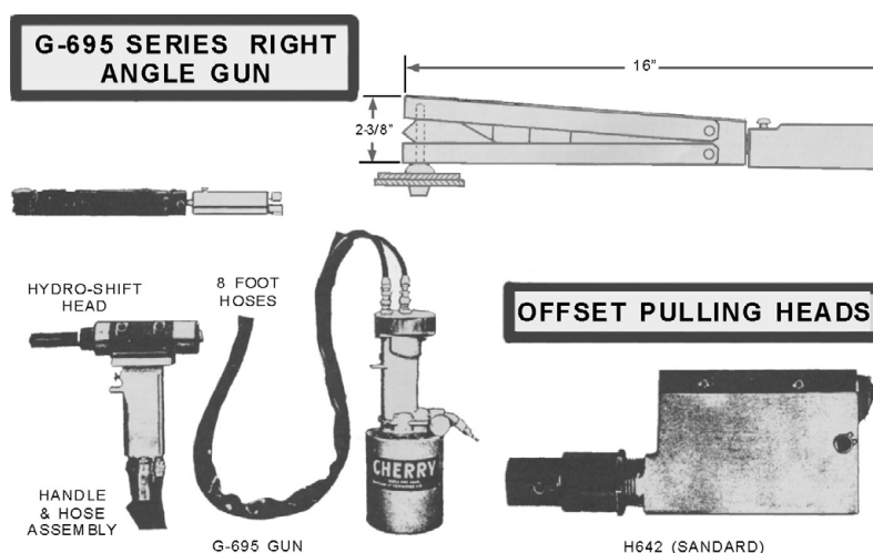
Figure 4-52.—Special use heads.
