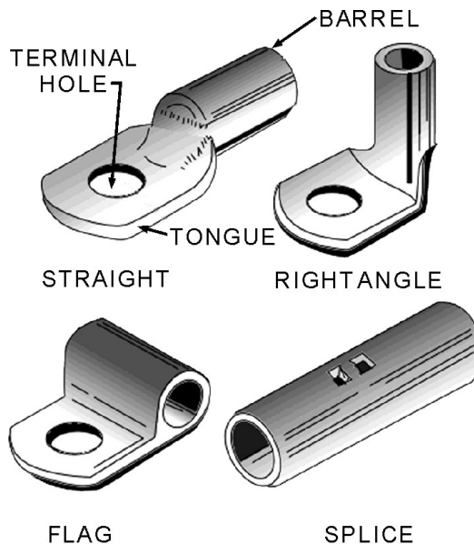
Figure 3-40.—Basic types of solderless terminals.
