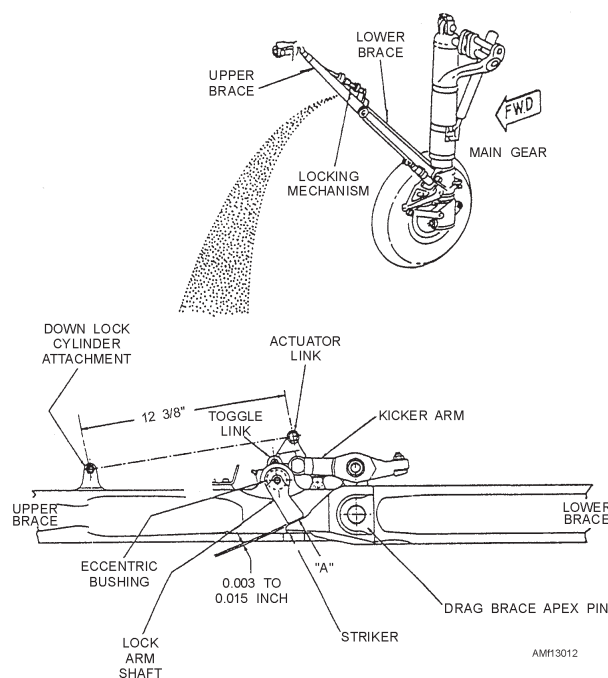
Figure 13-12.—Landing gear drag brace adjustment.
