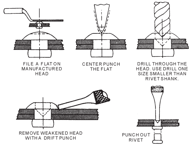
Figure 4-48.—Removal of rivets.
