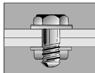
BOLT GRIP LENGTH CORRECT
