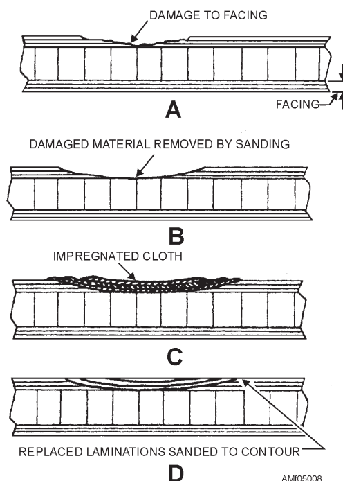
Figure 5-8.—Ply repair (scarfed method).
