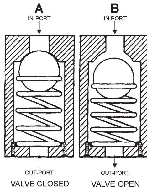
Figure 11-12.—Typical check valve.
