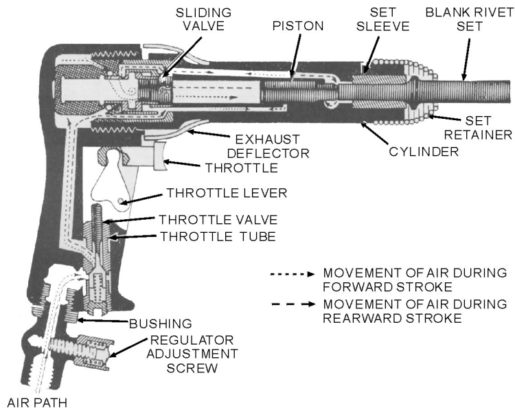
Figure 4-10.—Rivet gun internal airflow.
