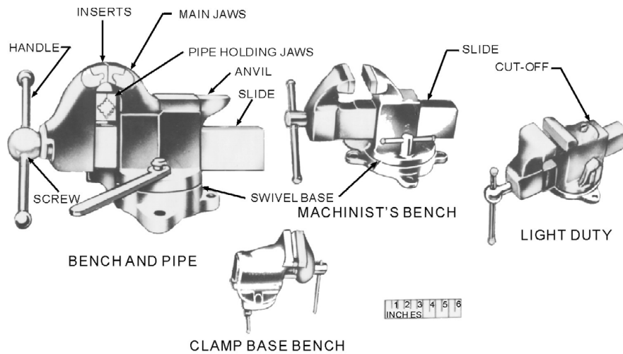
Figure 4-21.—Common types of bench vices.
