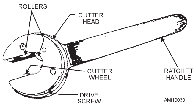
Figure 10-30.—Permaswage chipless cutter.
