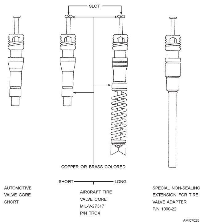
Figure 7-25.—Valve core identification.
