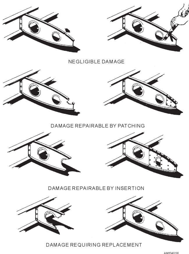
Figure 4-56.—Classifications of damage.
