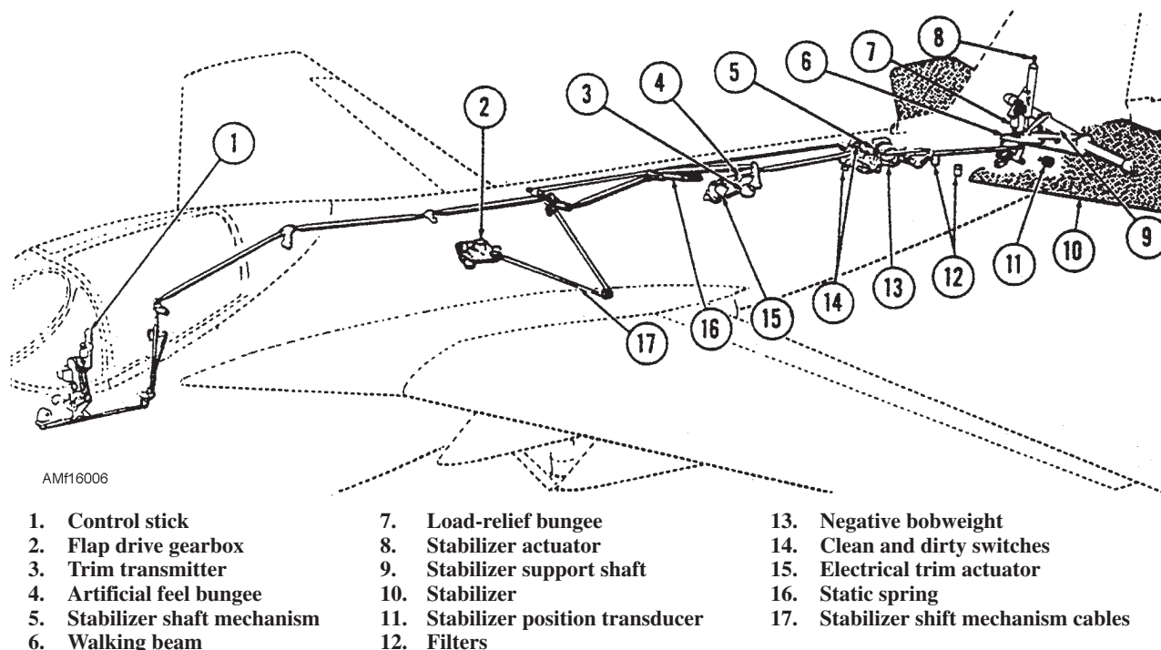
Figure 16-6.—Stabilizer control system.
