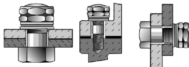
Figure 3-20.—Typical installations of the Klincher locknut.
