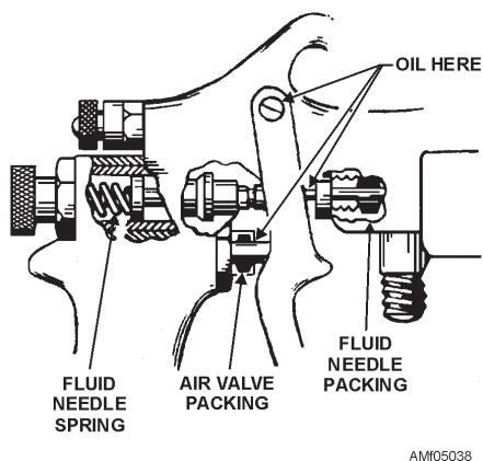
Figure 5-38.—Spray gun lubrication points.
