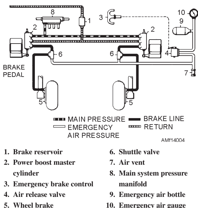
Figure 14-4.—Power boost brake system.
