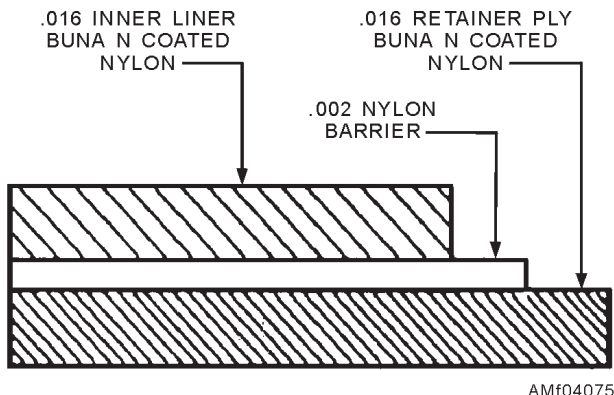
Figure 4-75.—Bladder cell construction.
