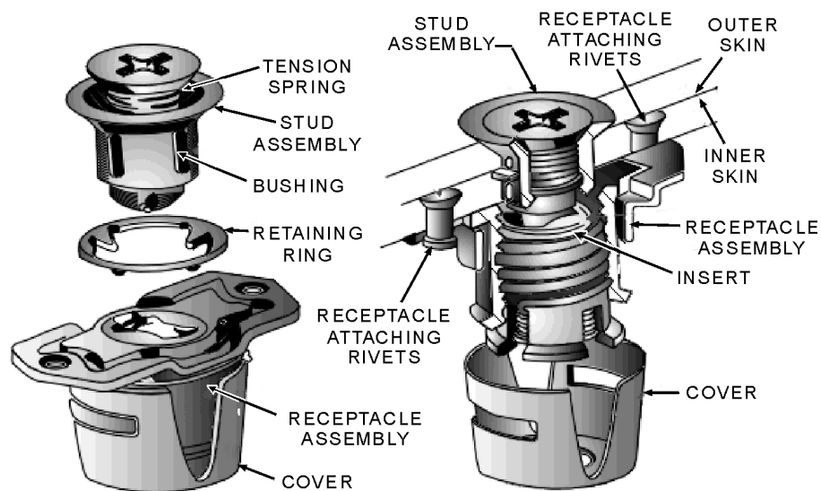
Figure 3-24.—Camloc high-stress panel fastener.
