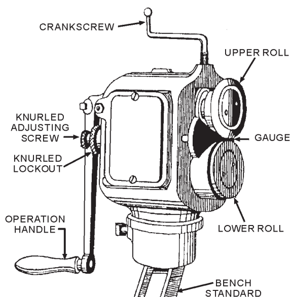
Figure 4-28.—Rotary machine.
