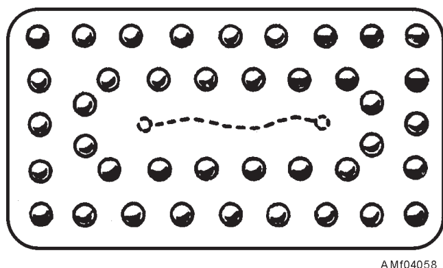
Figure 4-58.—Lap patch for repairing a crack in stressed skin.
