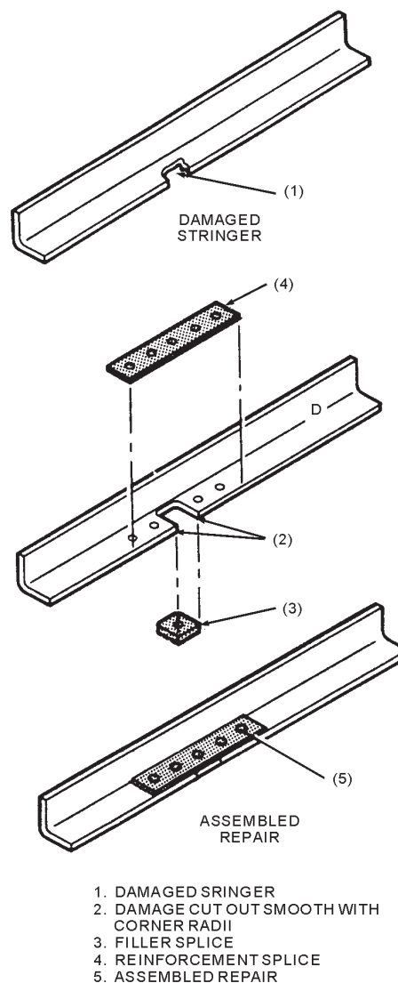
Figure 4-67.—Stringer repair by patching.
