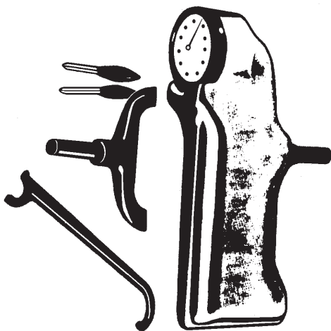
Figure 2-32.—Barcol portable hardness tester.
