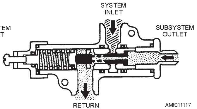
Figure 11-17.—Pressure-reducing valve operational schematic.
