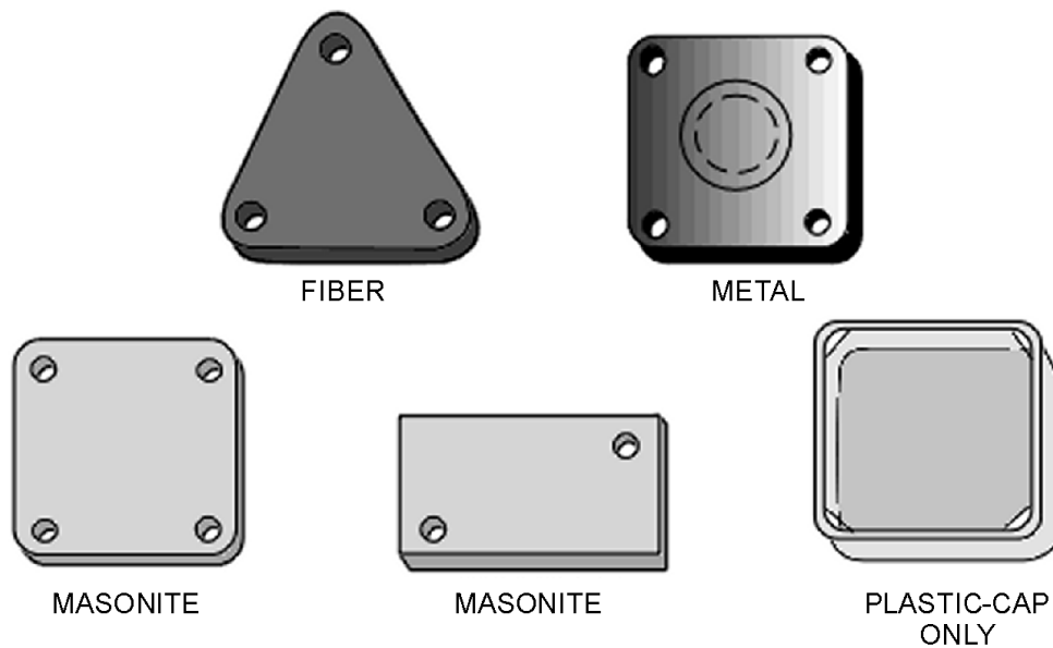
Figure 8-21.—Typical blank-off plates.
