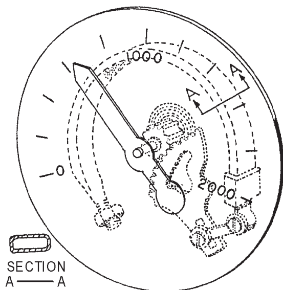
Figure 12-36.—Bourdon tube.
