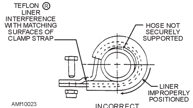
Figure 10-23.—Clamp installation.
