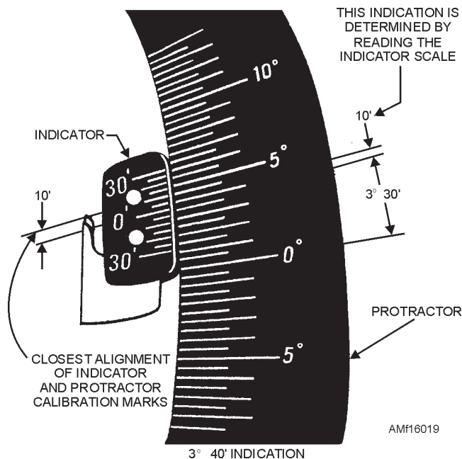
Figure 16-19.—Aileron throw protractor indications.
