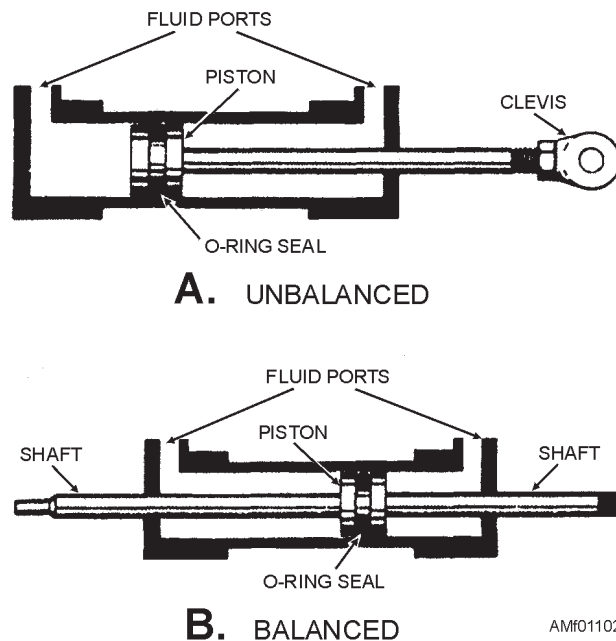
Figure 11-2.—Double-acting, piston-type, actuating cylinders.
