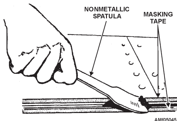
Figure 5-44.—Applying sealant.
