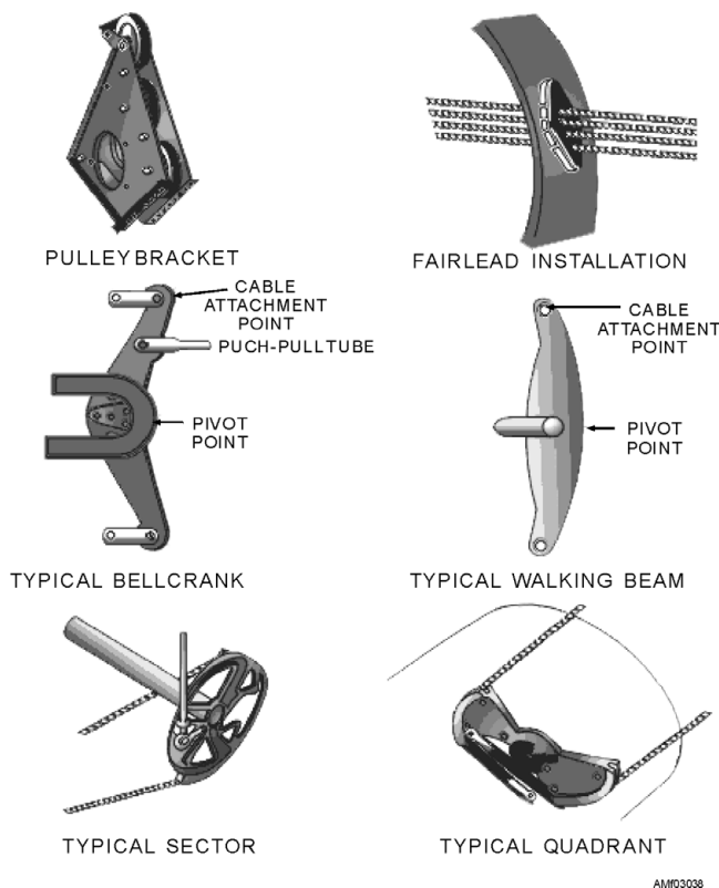
Figure 3-38.—Control system components.
