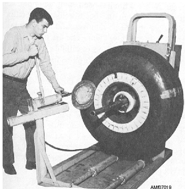
Figure 7-19.—Using bead-breaking pump.
