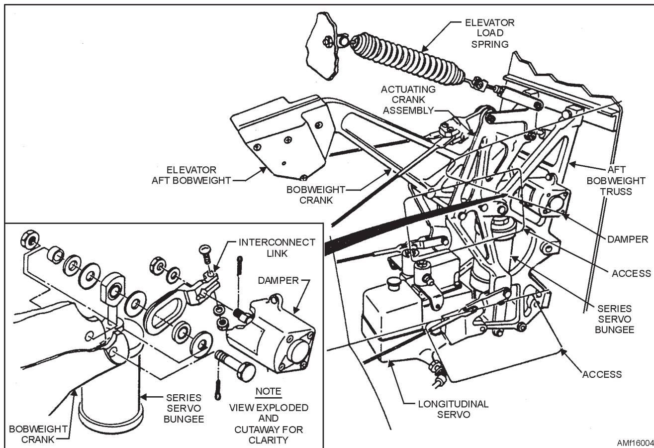
Figure 16-4.—Elevator aft bobweight and damper assembly.
