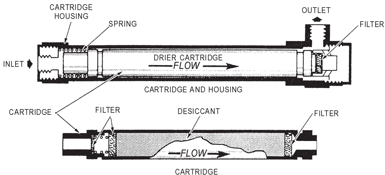
Figure 12-8.—Chemical air drier.
