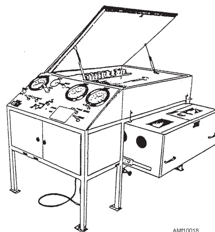
Figure 10-18.—Aircraft hose burst test stand (CGS Scientific).
