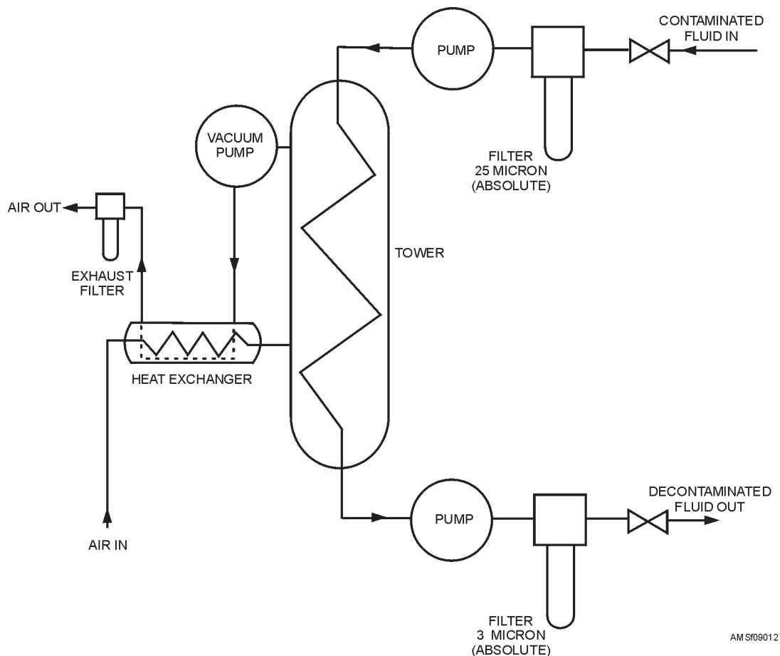
Figure 9-12.—Fluid purification system.
