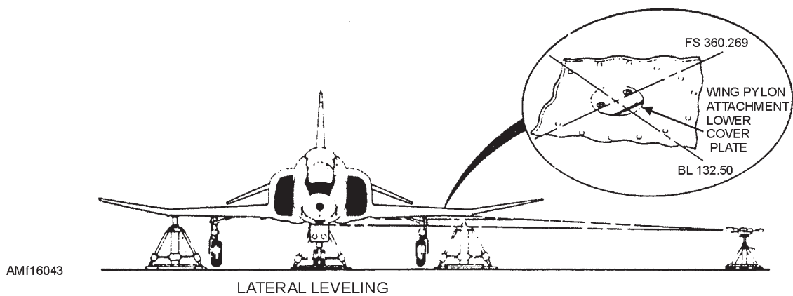
Figure 16-43.—Transit leveling.
