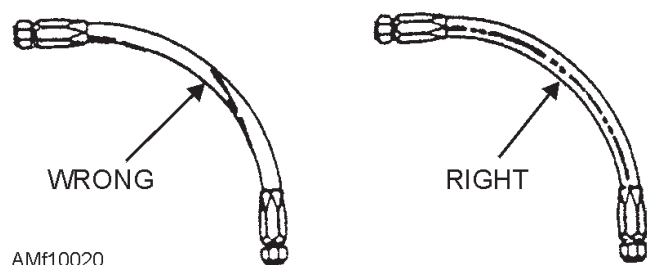
Figure 10-20.—Hose twist.
