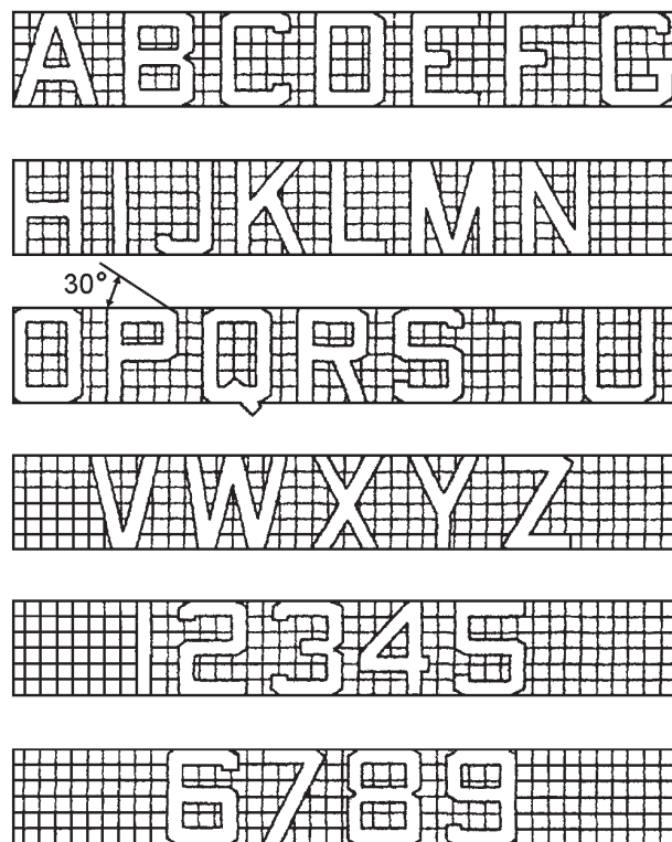
Figure 5-31.—Forms of letters and numerals.
