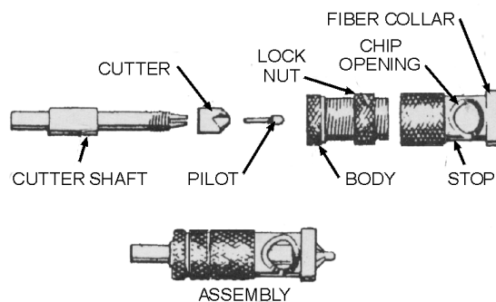
Figure 4-7.—Adjustable stop countersink.
