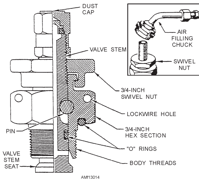
Figure 13-14.—High-pressure air valve, type MS 28889.
