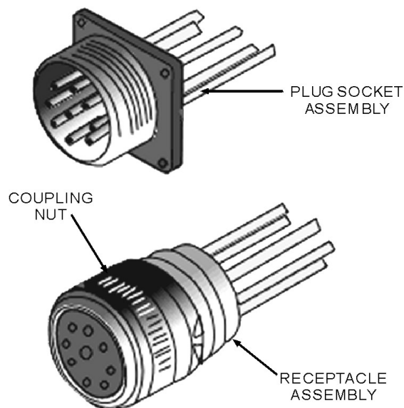
Figure 3-39.—Connector assembly.
