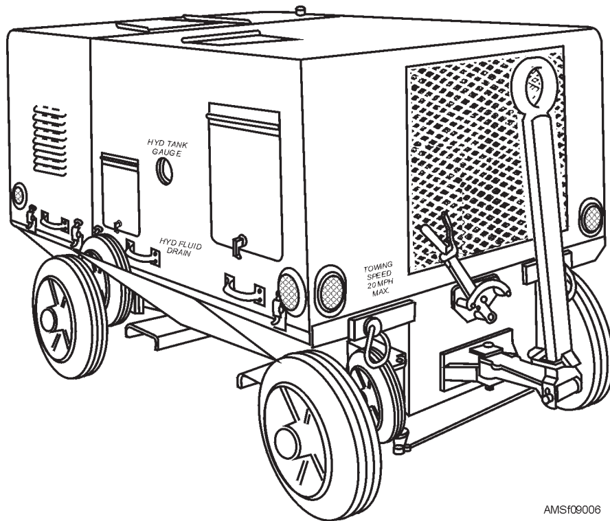
Figure 9-6.—Portable electric motor-driven hydraulic power supply (A/M27T-7).
