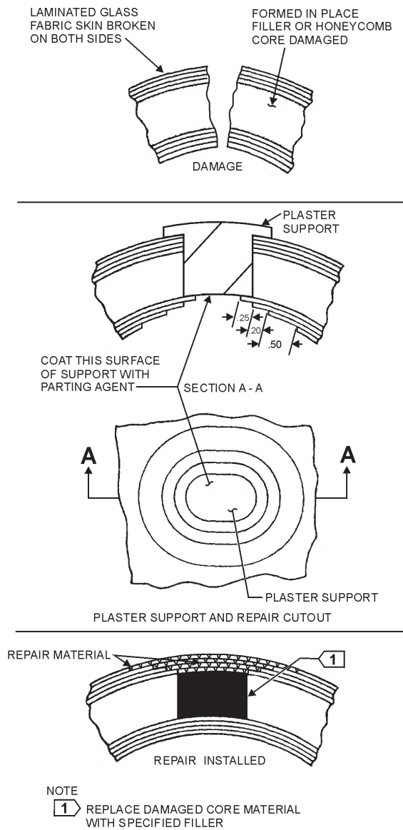
Figure 5-15.—Foam-type puncture repair.
