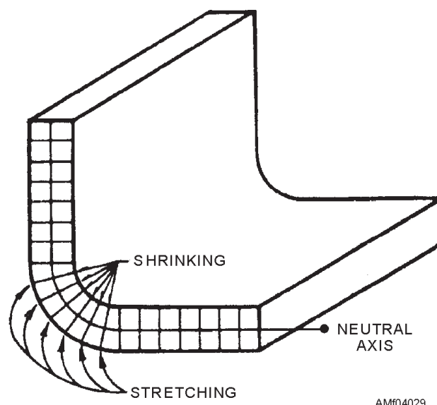
Figure 4-29.—Neutral axis.
