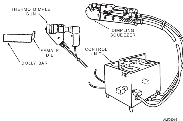
Figure 4-15.—Hot dimpling kit.
