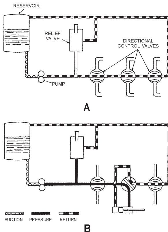
Figure 12-1.—Basic open-center hydraulic system.
