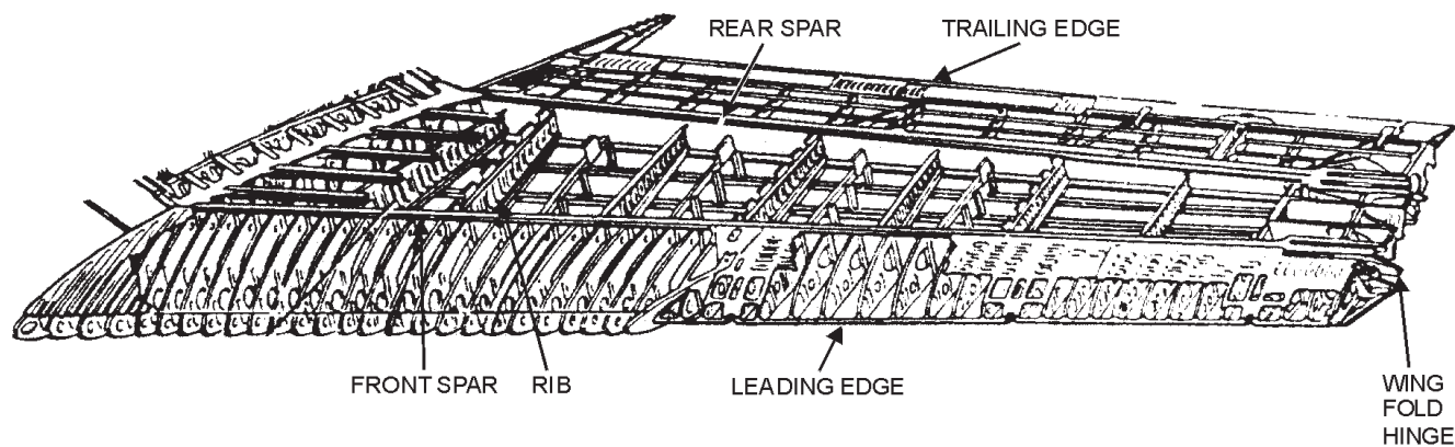
Figure 2-4.—Typical wing construction.
