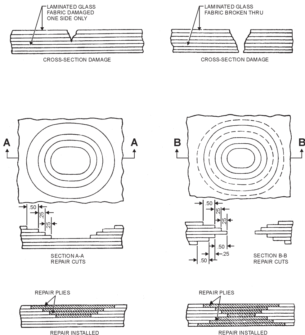
Figure 5-9.—Repair of solid laminates (stepped method).
