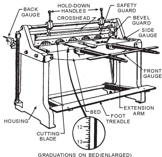
Figure 4-17.—Squaring shears.
