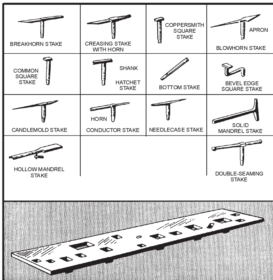
Figure 4-33.—Stakes and stake plates.
