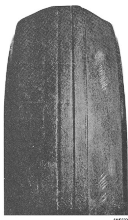
Figure 7-26.—Rapid tread wear caused by underinflation.
