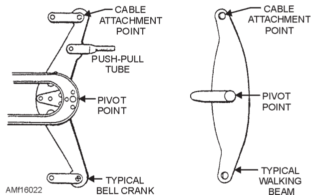
Figure 16-22.—Bell crank and walking beam.
