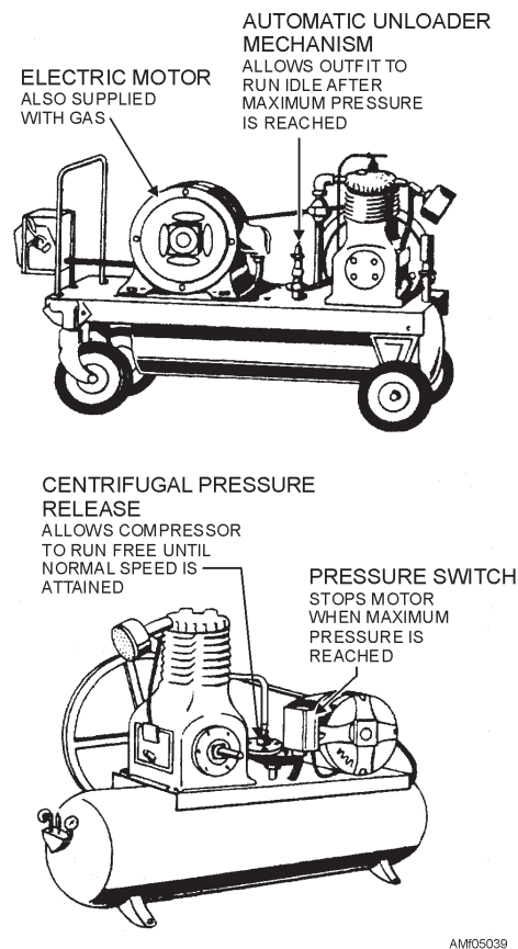
Figure 5-39.—Air compressors.
