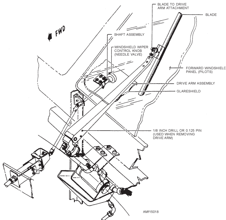
Figure 15-18.—Windshield wiper unit.
