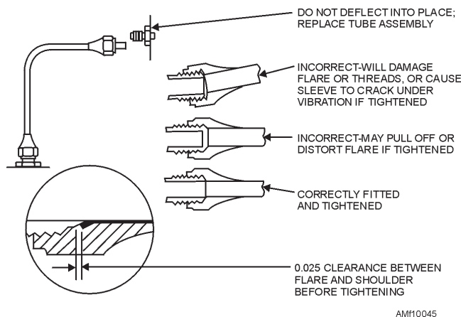
Figure 10-45.—Correct and incorrect methods of installing flared fittings.
