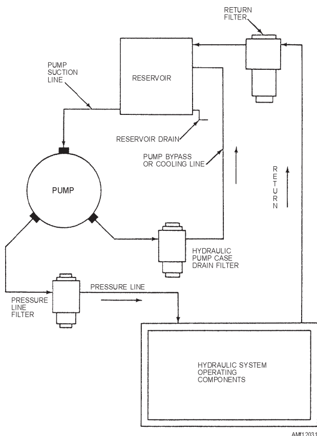
Figure 12-31.—Typical filter arrangement in hydraulic system.
