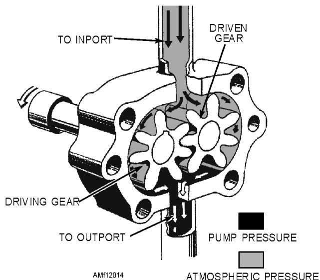
Figure 12-14.—Gear-type power pump.
