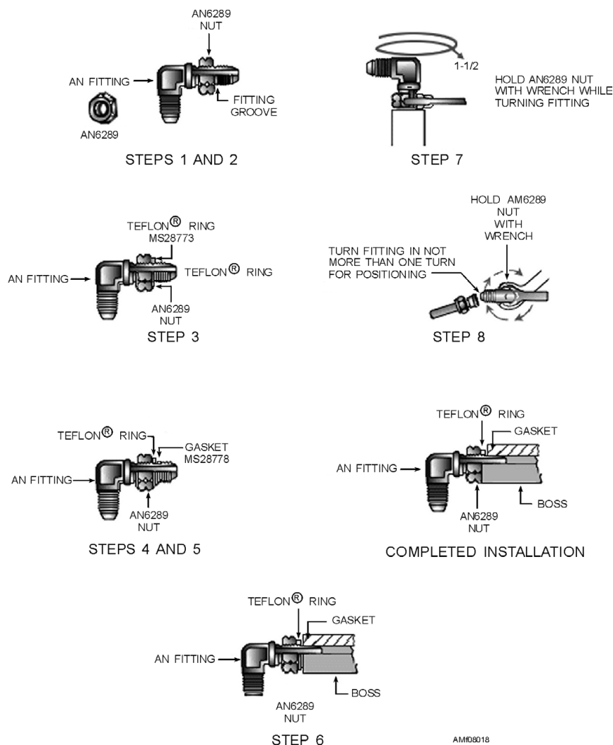
Figure 8-18.—Properly installed gasket and backup ring.
