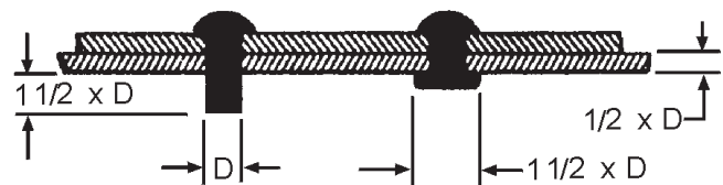
Figure 4-46.—Rivet dimensions before and after bucking.
