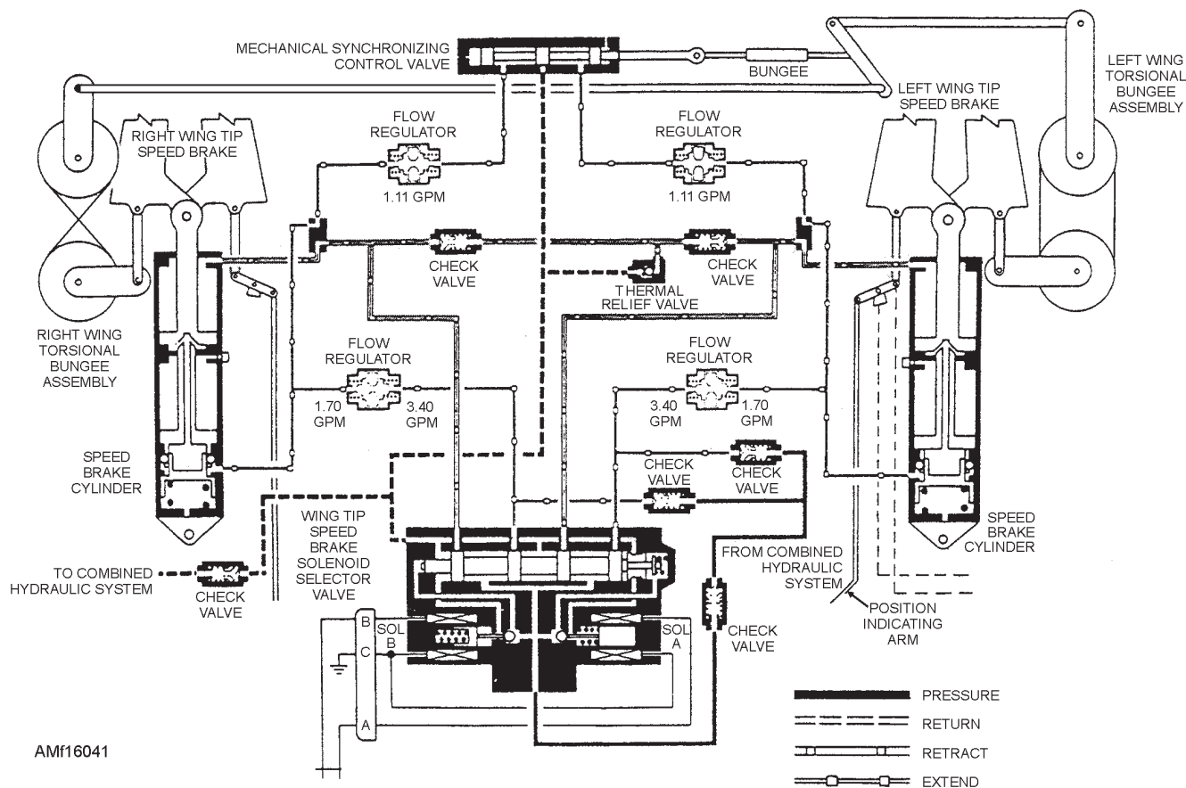
Figure 16-41.—Wingtip speed brake control system.
