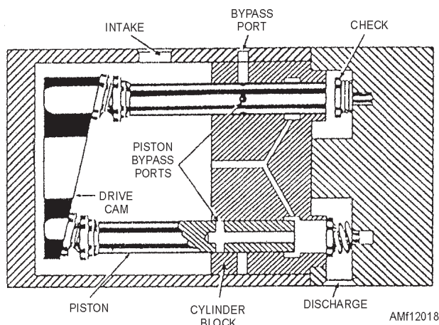
Figure 12-18.—Fluid displacement.
