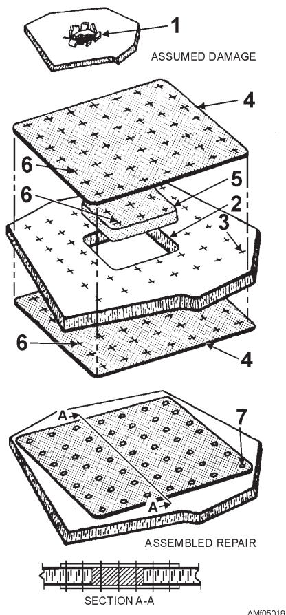
Figure 5-19.—Balsa wood repair with nonflush patch.
