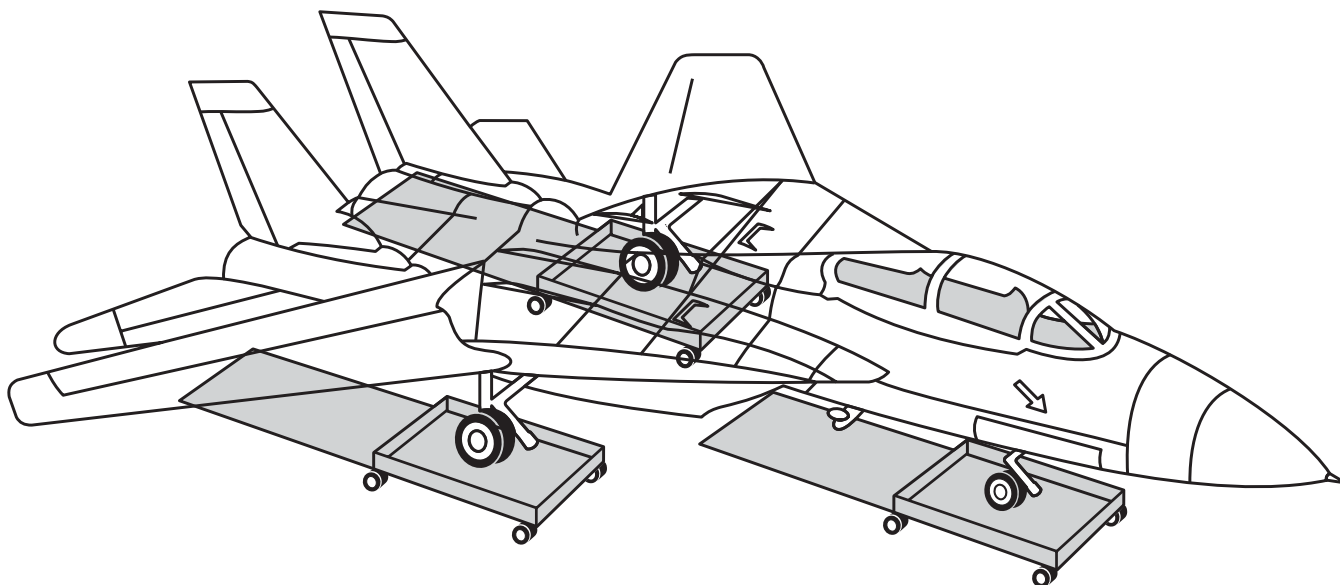
Figure 1-17.—Mobile Electronic Weighing System (MEWS).
