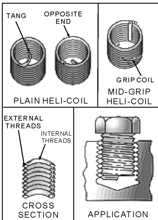
Figure 3-31.—Heli-coil insert.
