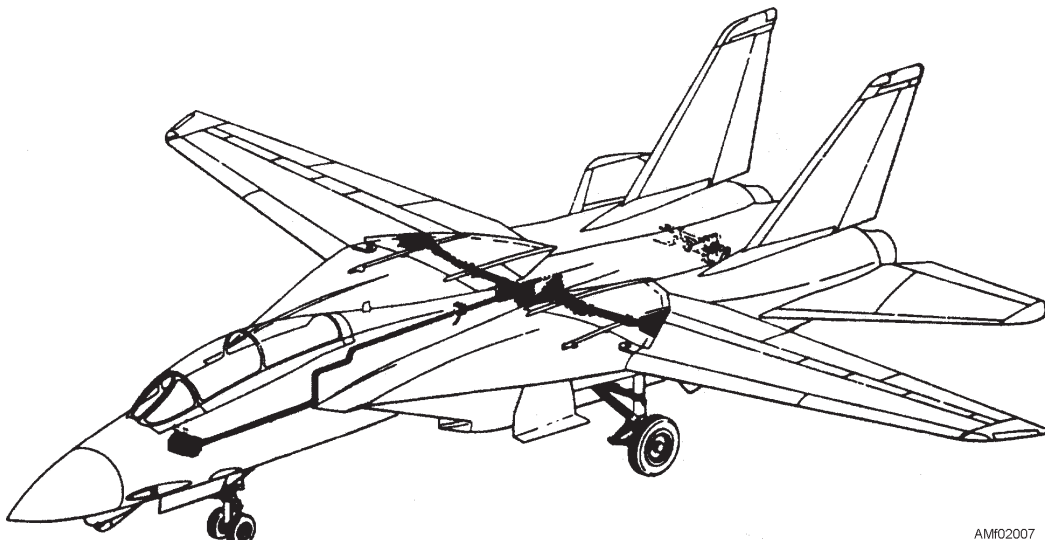
Figure 2-7.—Wing sweep control system (F-14).
