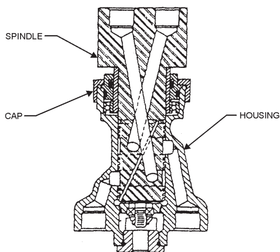
Figure 17-14.—Rotor coupling.
