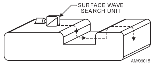
Figure 6-15.—Surface-wave inspection.
