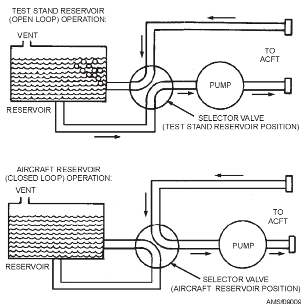
Figure 9-9.—Test stand operating modes.
