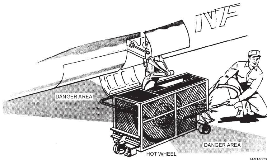
Figure 14-20.—Use of blowout screen on overheated brakes.
