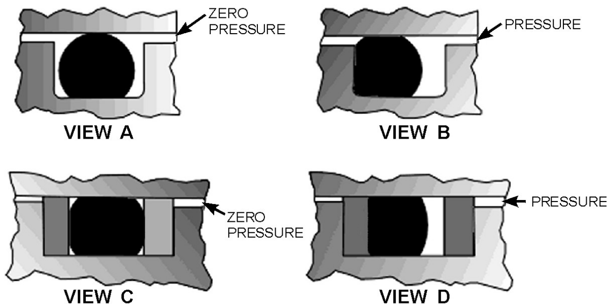
Figure 8-12.—Action of O-rings.
