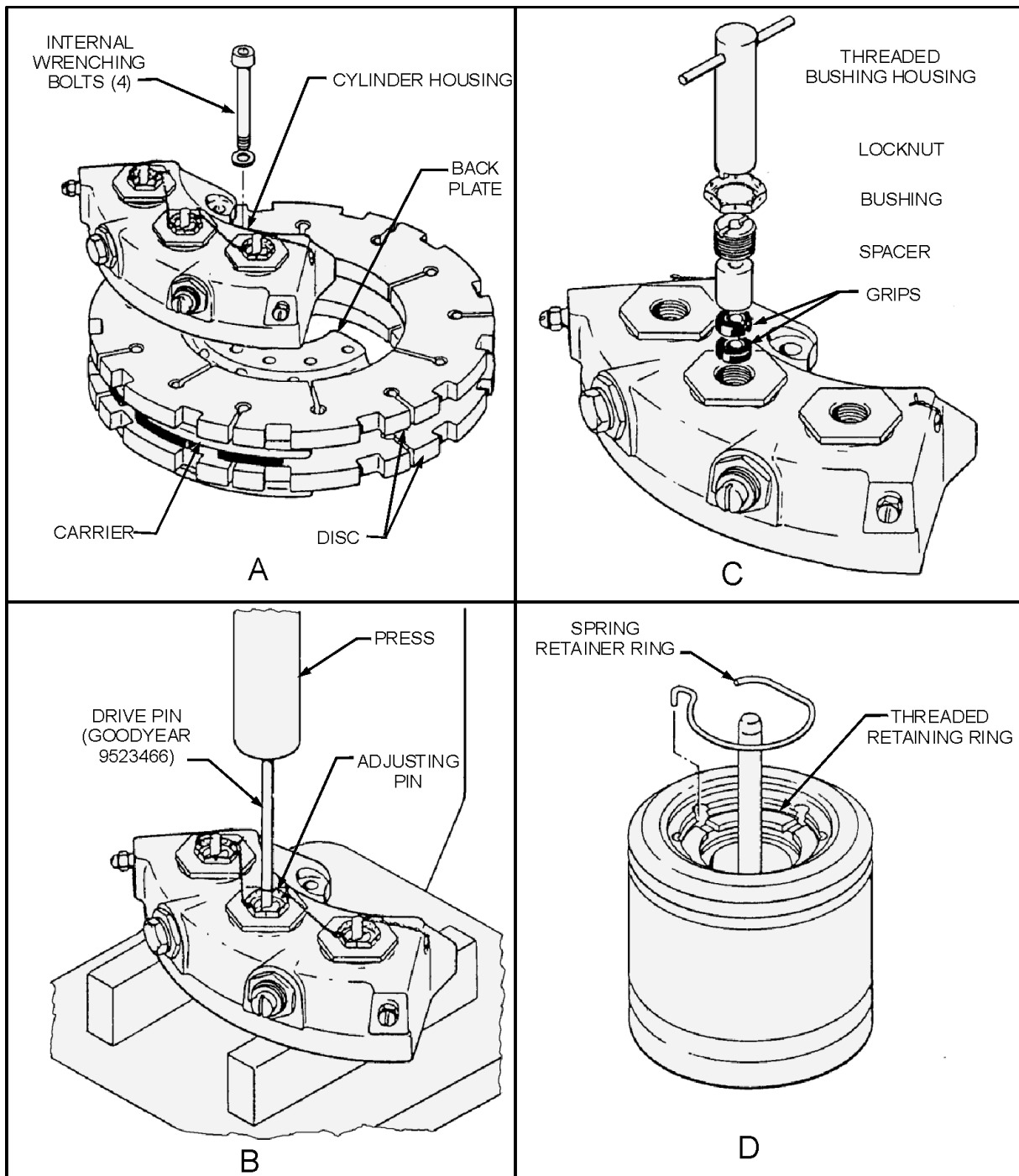
Figure 14-31.—Seal replacement and piston return adjustment.
