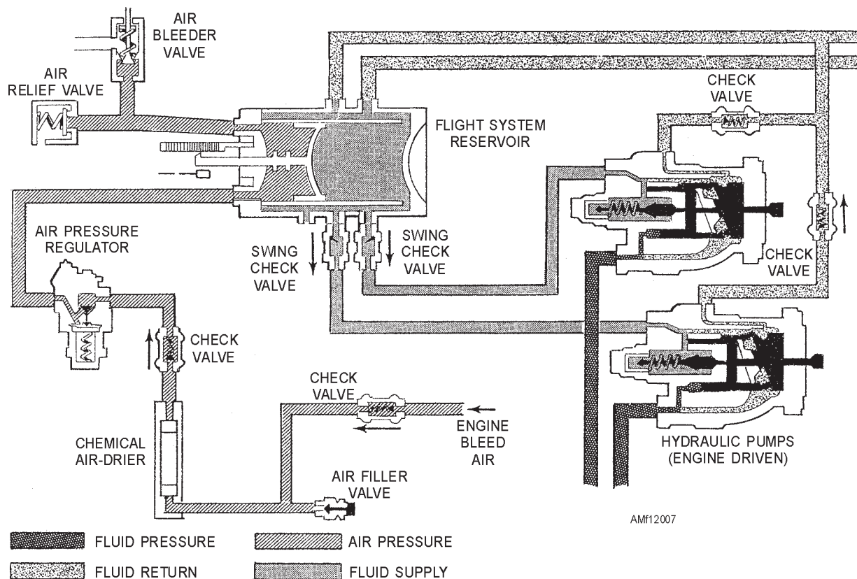
Figure 12-7.—Air-pressurized reservoir and components.
