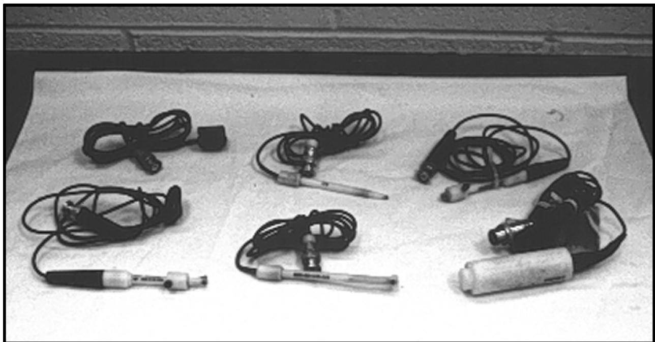
Figure 6-18.—Typical eddy current test probes.
