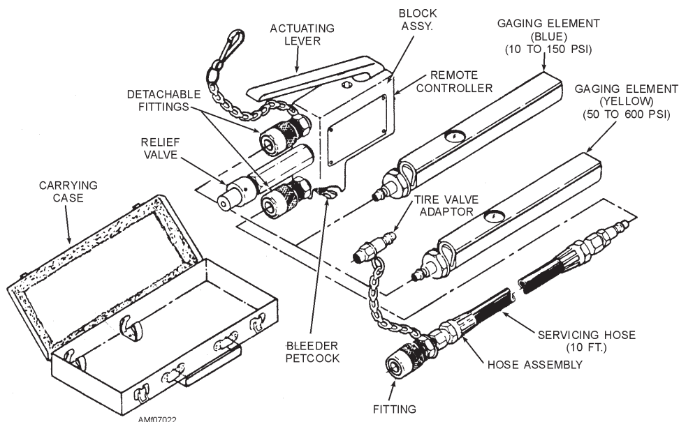
Figure 7-22.—Tire inflator assembly kit.
