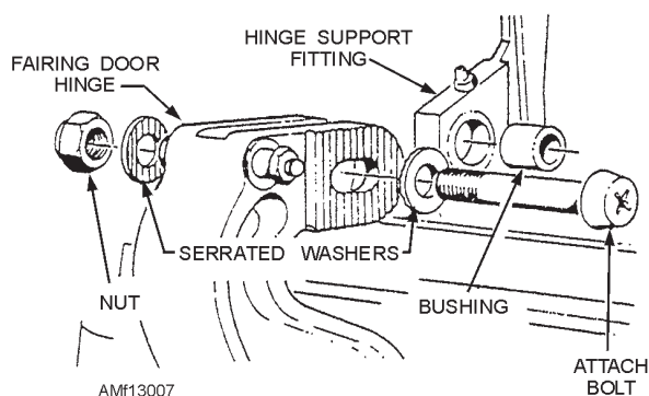
Figure 13-7.—Adjustable door hinge installation.
