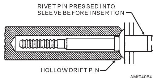
Figure 4-54.—Inserting self-plugging rivet (mechanical lock).
