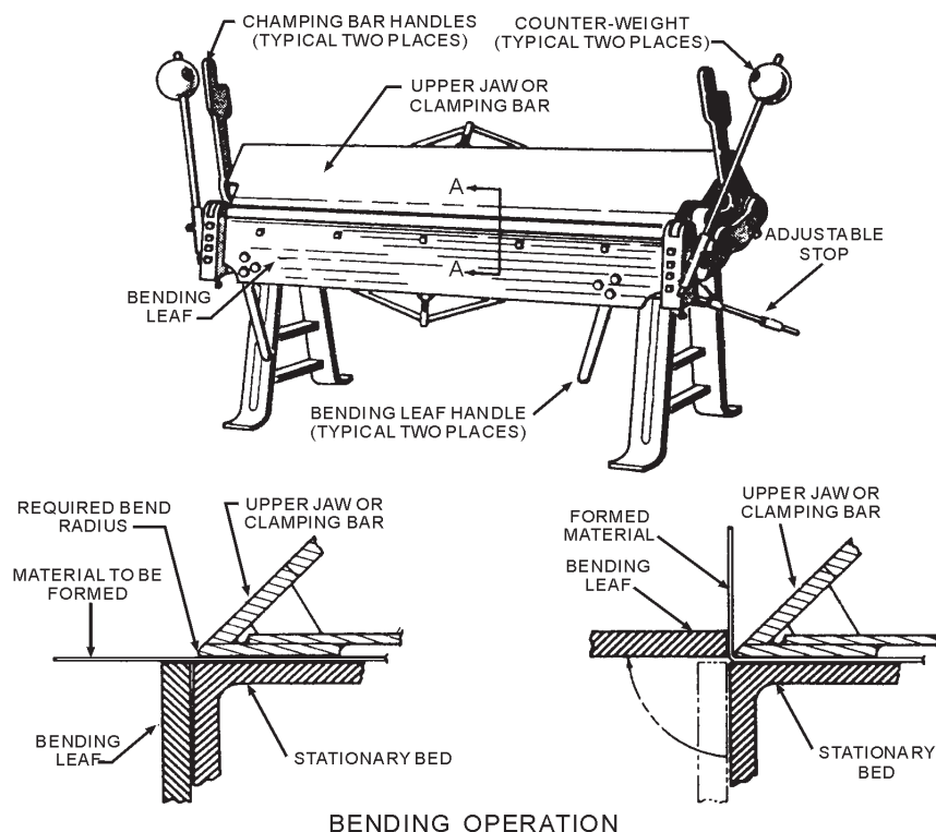
Figure 4-22.—Cornice brake and operation.
