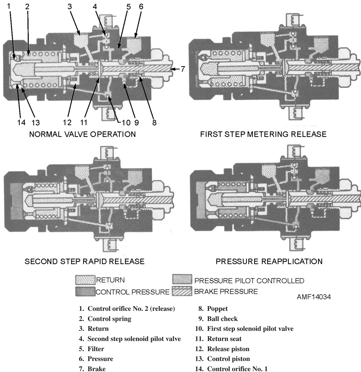
Figure 14-34.—Antiskid control valve schematic.
