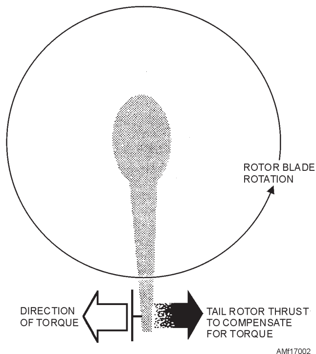
Figure 17-2.—Torque reaction.
