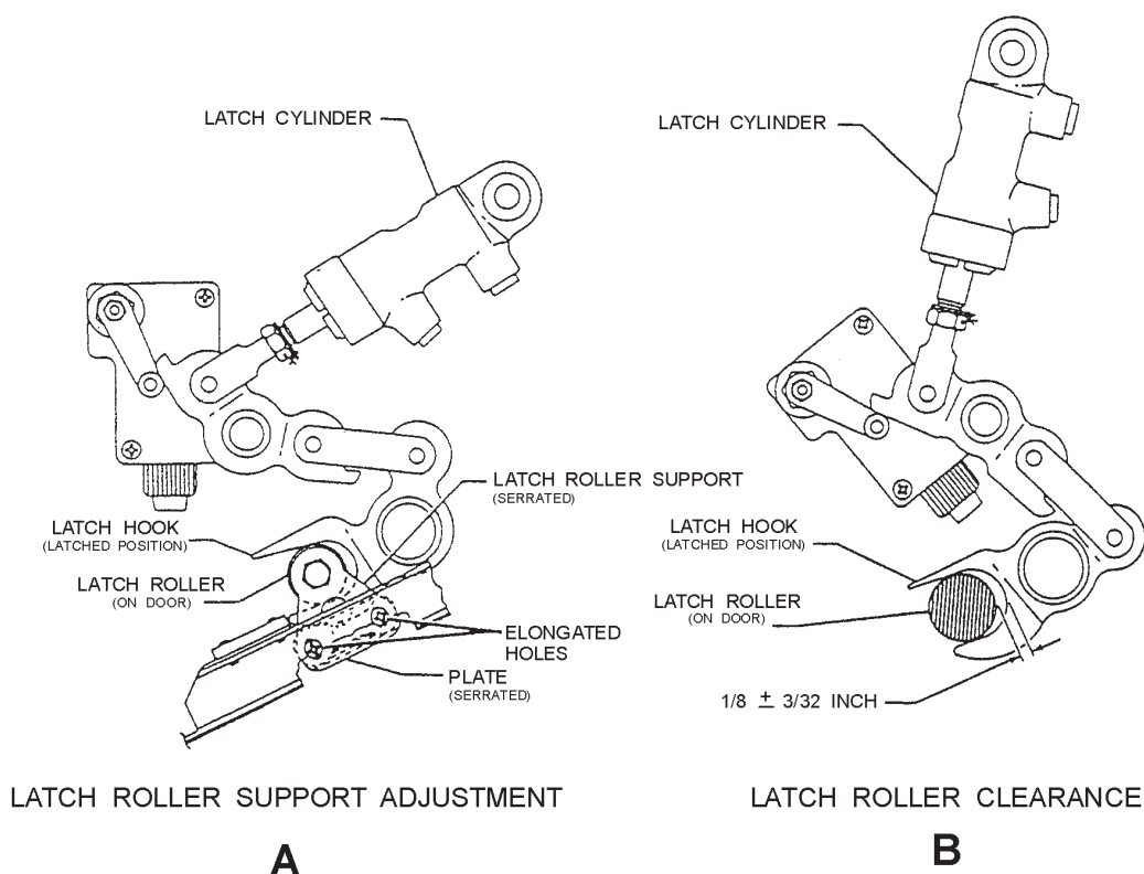
Figure 13-6.—Landing gear door latch installation.
