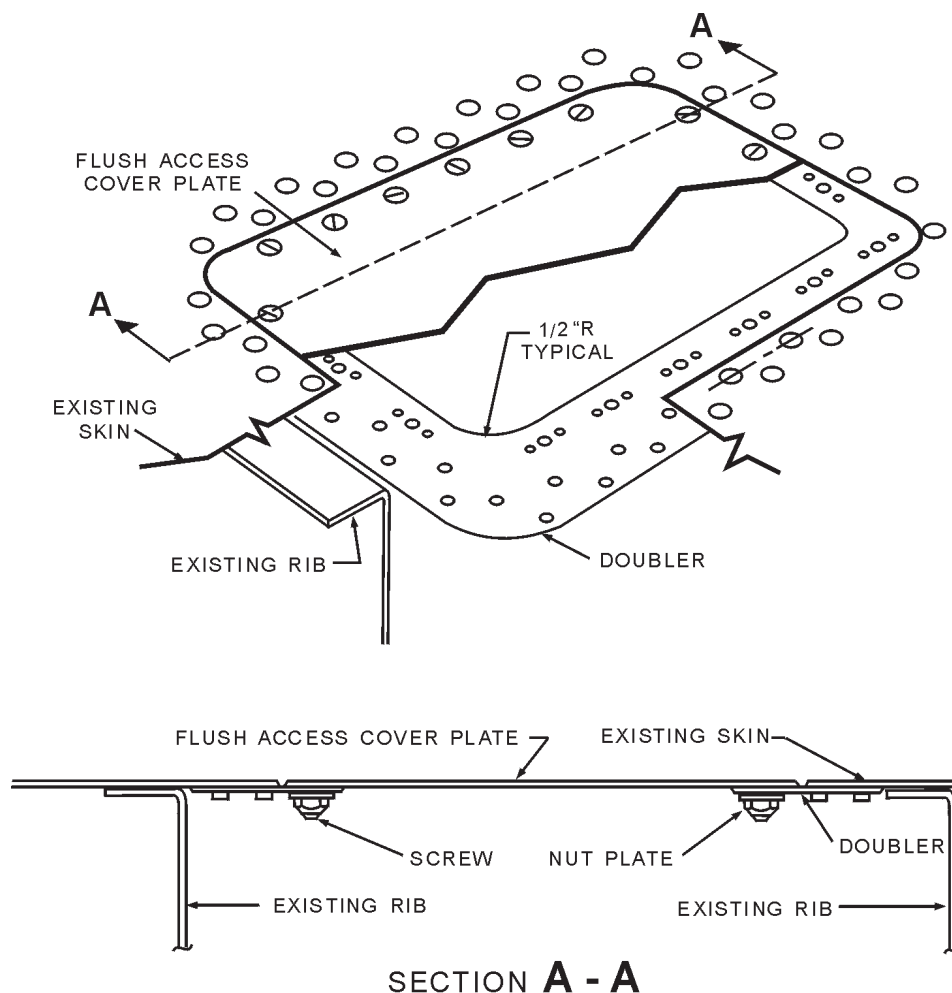
Figure 4-64.—Flush access door installation.
