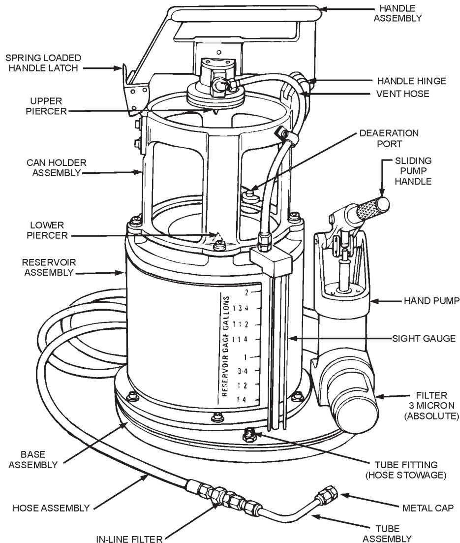
Figure 9-2.—Model HSU-1 fluid service unit.
