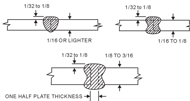
Figure 6-36.—Butt joints in light sections.
