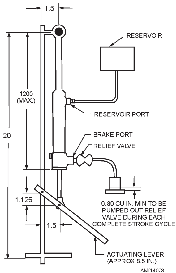
Figure 14-23.—Rod packing, cylinder leakage, and pumping function test.
