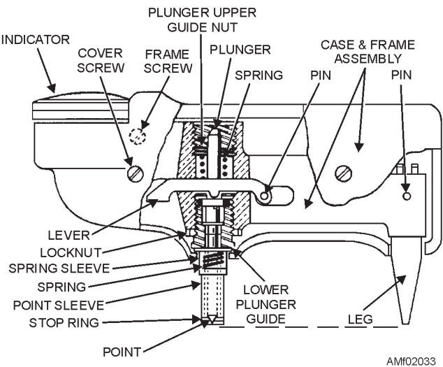
Figure 2-33.—Cutaway of Barcol tester.
