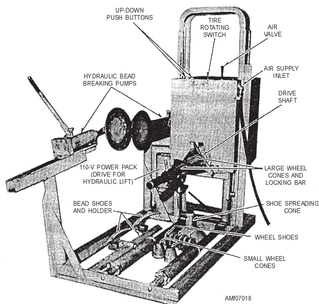
Figure 7-18.—Aircraft wheel holder and tire bead-breaking machine.
