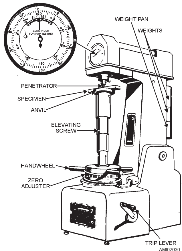
Figure 2-30.—Rockwell hardness tester.
