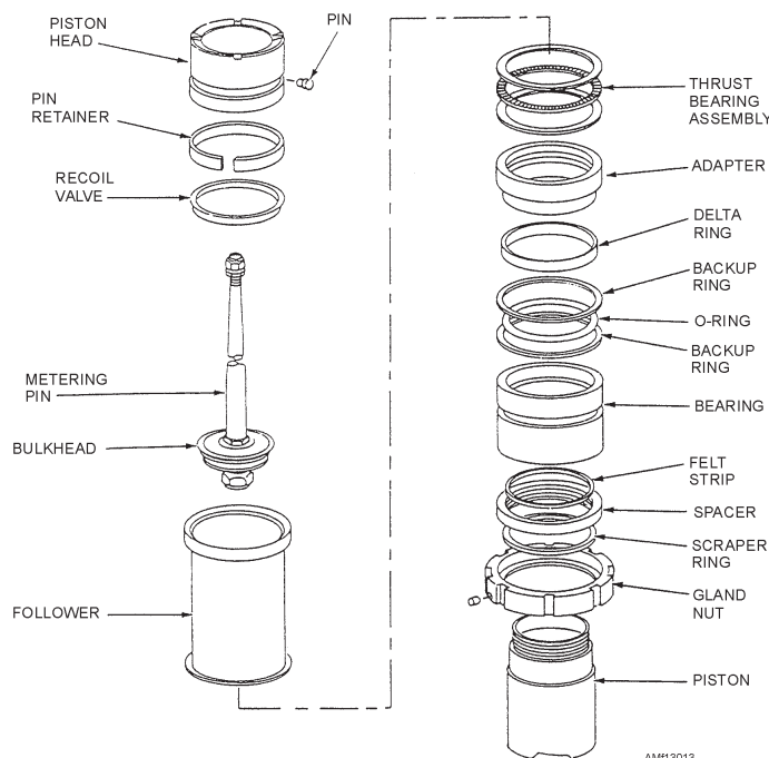
Figure 13-13.—Main gear recoil strut piston.
