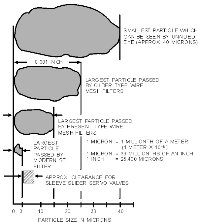
Figure 8-2.—Graphic comparison of particle sizes.
