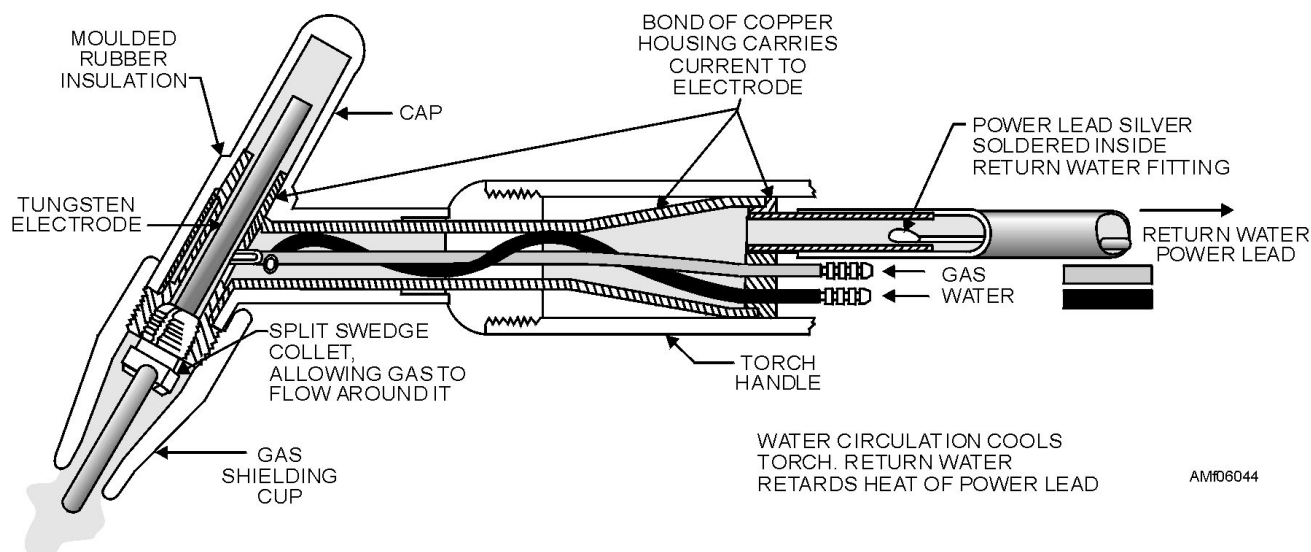
Figure 6-44.—Typical water-cooled GTA welding torch.
