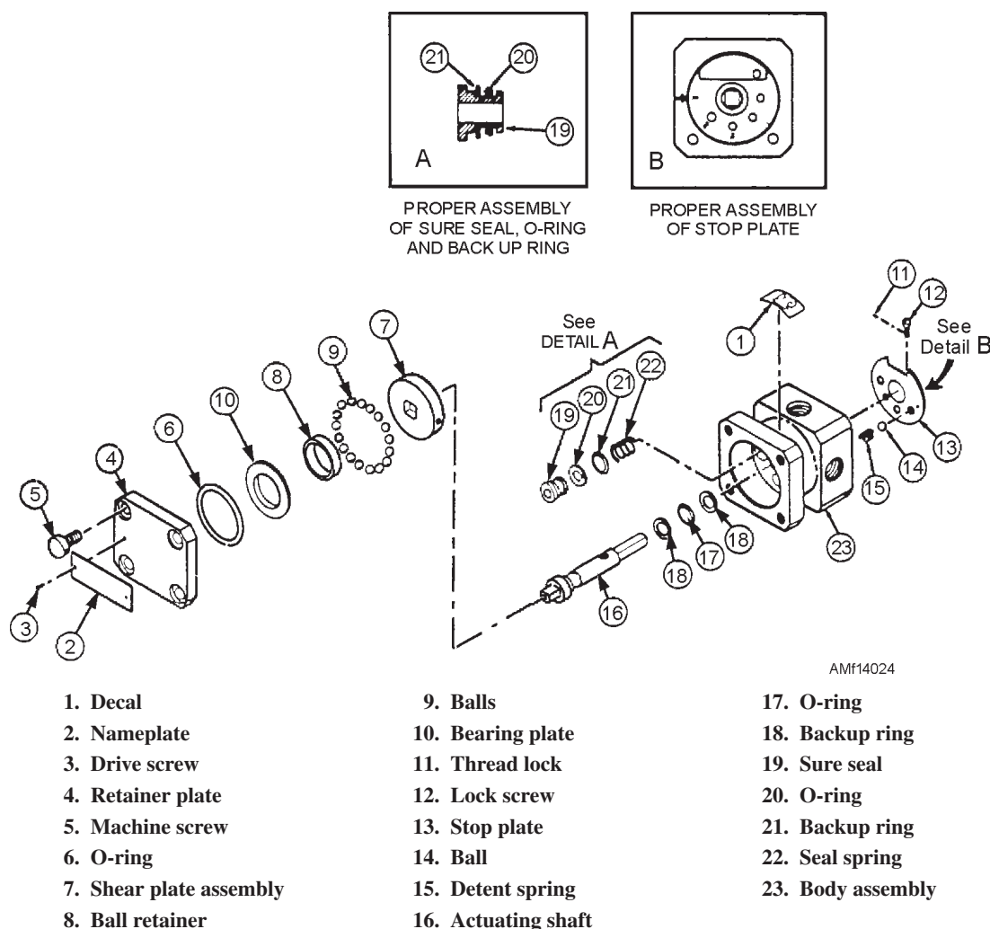
Figure 14-24.—Brake selector valve—exploded view.
