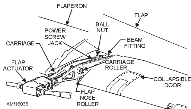
Figure 16-36.—Flap actuator.
