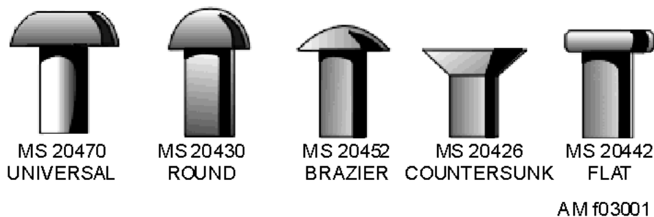
Figure 3-1.—Rivet head shapes and code numbers.
