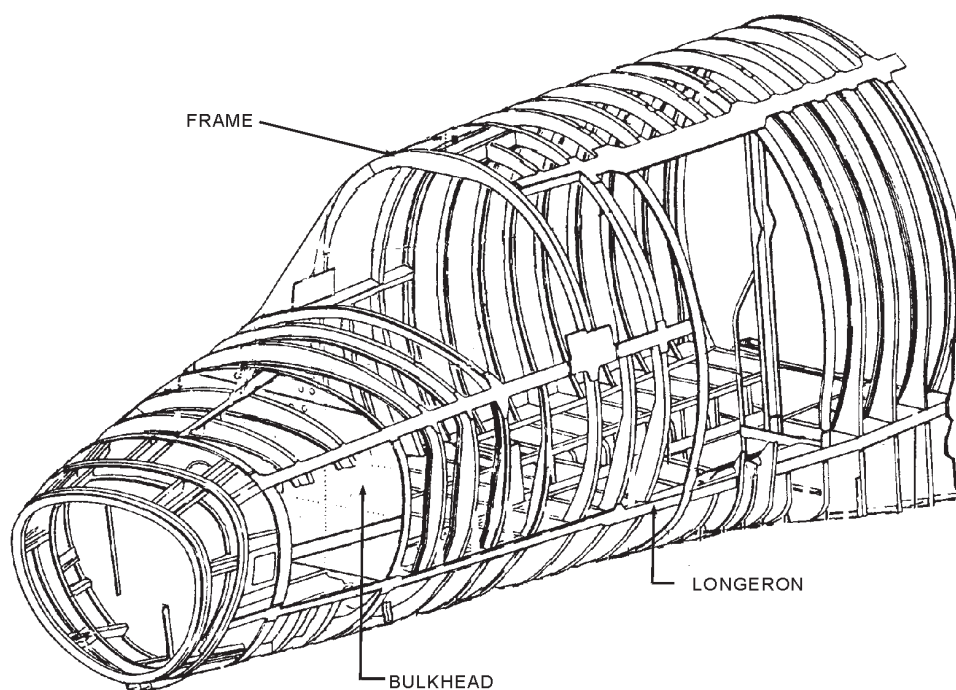
Figure 4-72.—Forward fuselage (semimonocoque).
