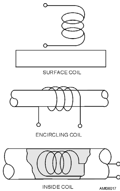
Figure 6-17.—Basic coil configurations.
