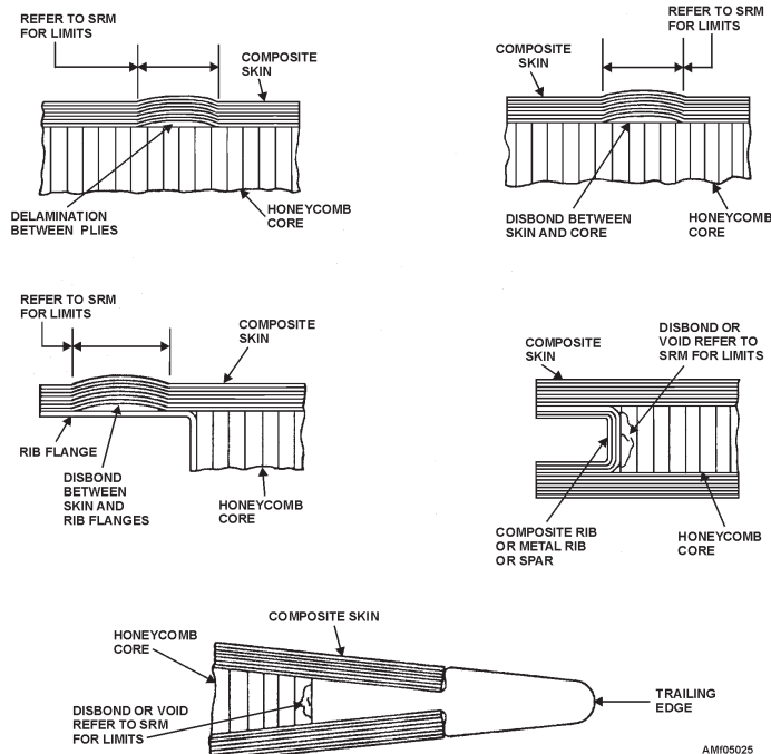
Figure 5-25.—Example of negligible damage on composite material.
