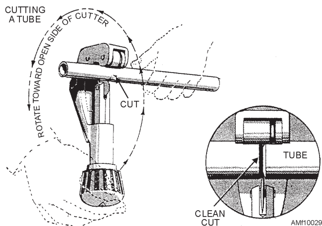
Figure 10-29.—Standard tube cutter.
