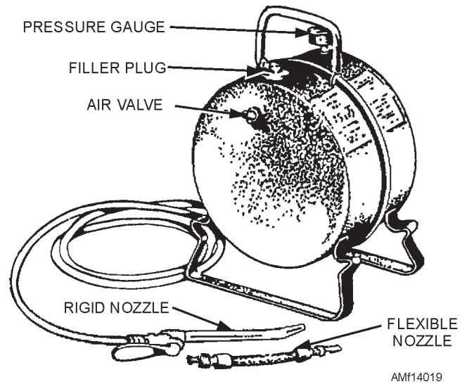
Figure 14-19.—Bleeder bomb.
