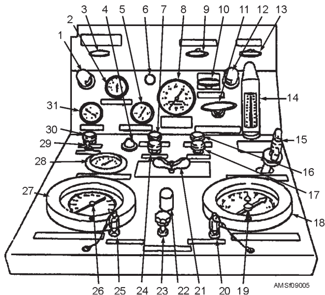
Figure 9-5.—A/M27T-5 main control panel controls and indicators.
