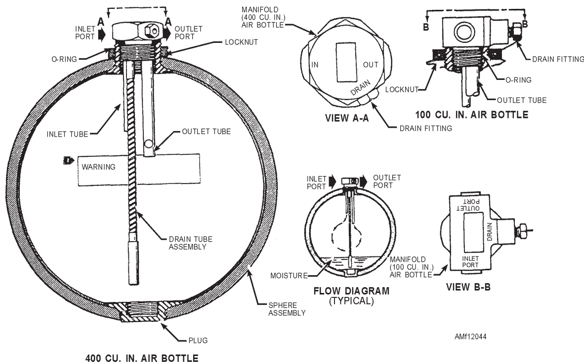
Figure 12-44.—Air cylinder.
