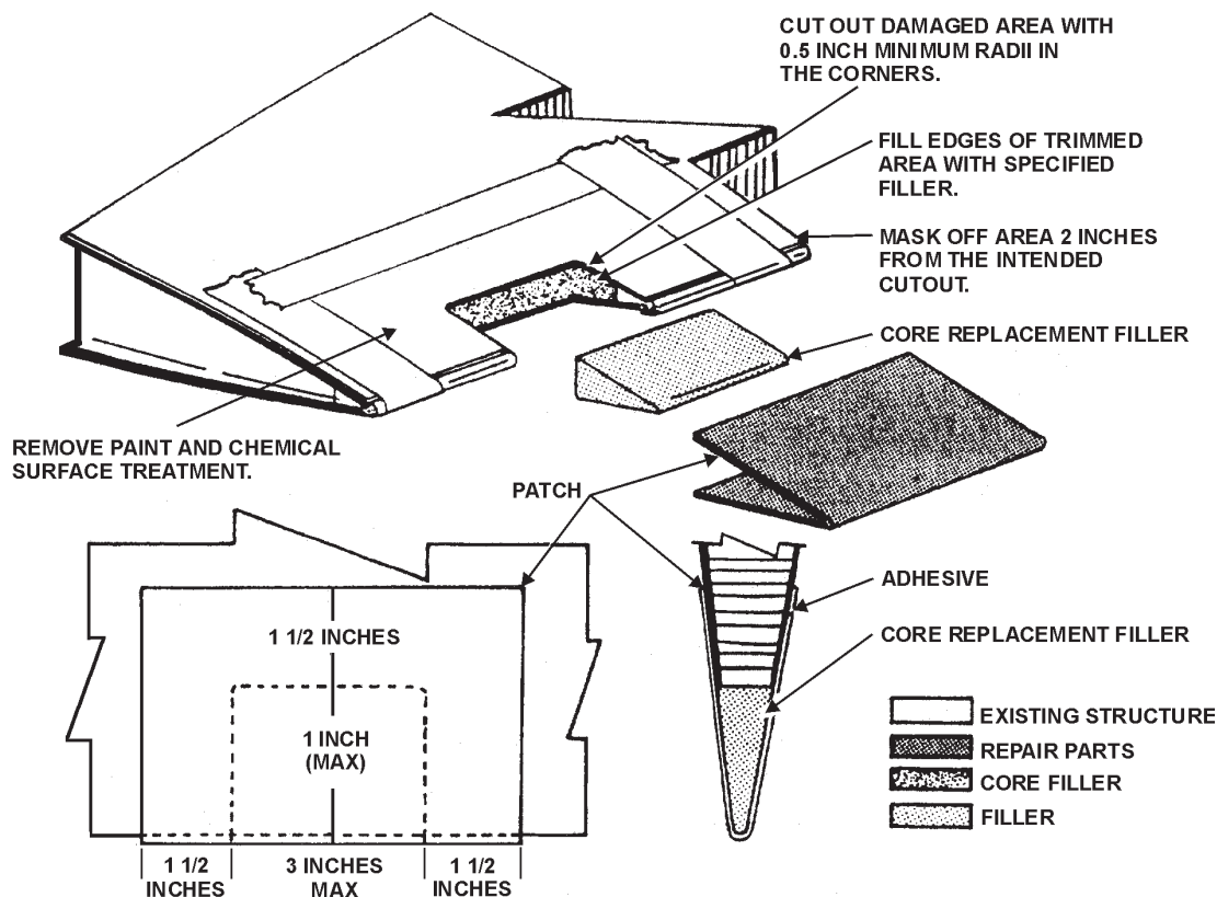
Figure 5-20.—Trailing edge repair (sandwich construction).
