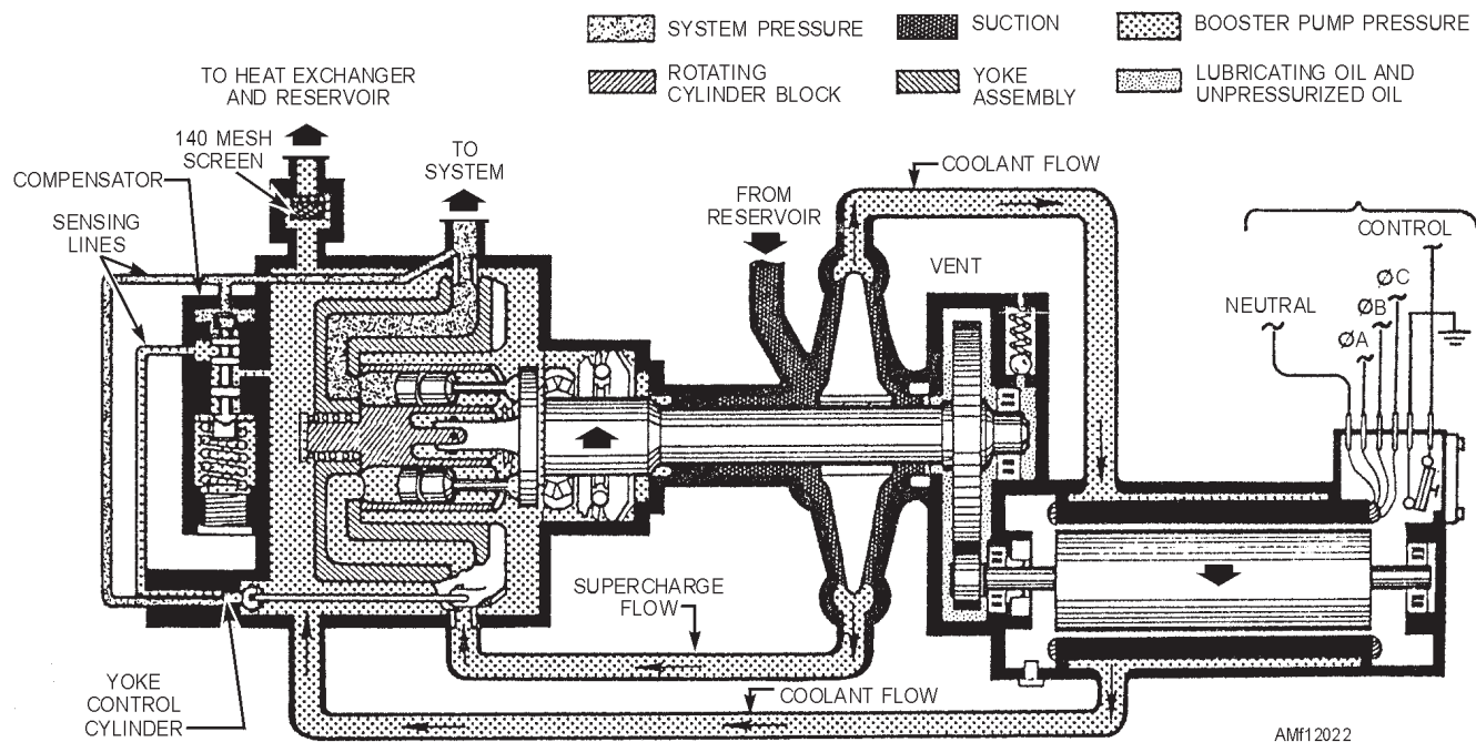
Figure 12-22.—Motor-driven variable displacement piston pump schematic.
