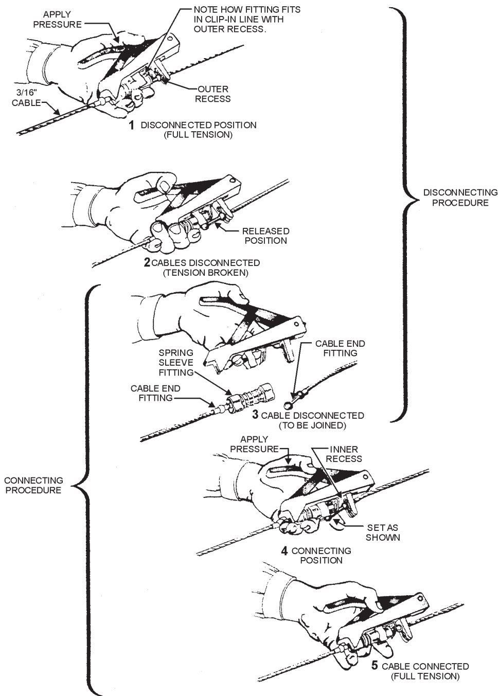
Figure 16-21.—Quick-disconnect procedures.
