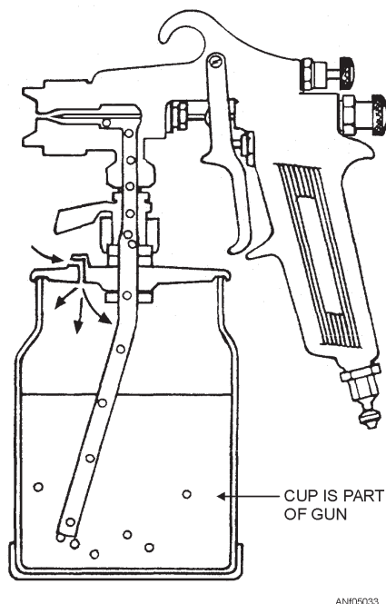
Figure 5-33.—Suction-feed spray gun.
