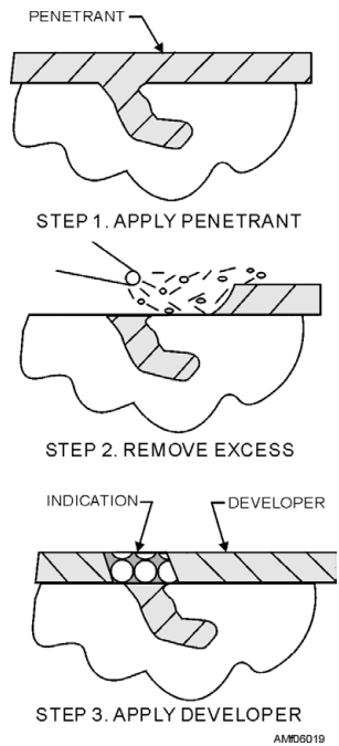
Figure 6-19.—Basic penetrant process.
