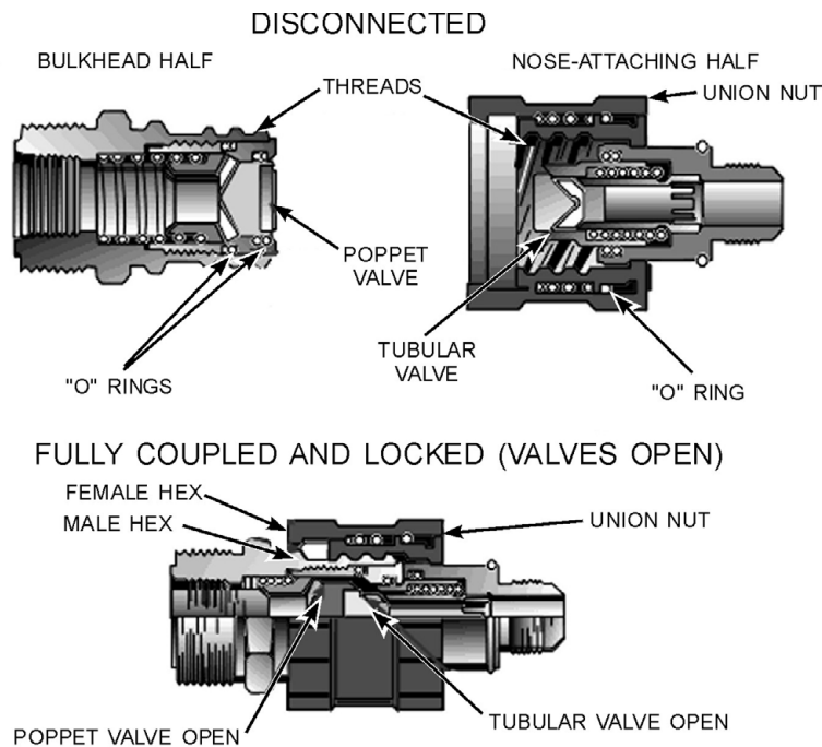
Figure 8-10.—Series 320 (Aeroquip) quick disconnect.
