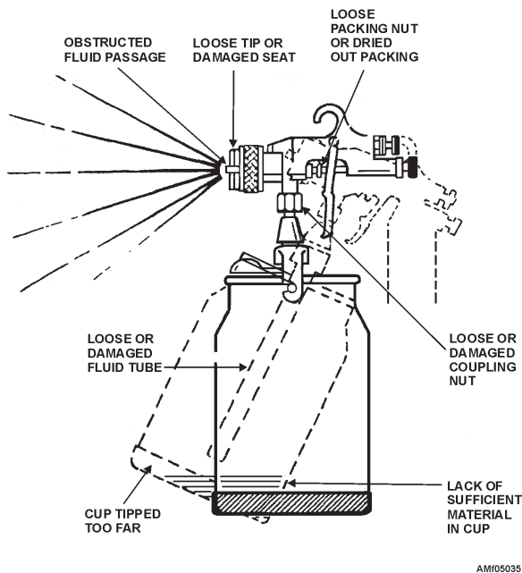
Figure 5-35.—Causes of jerky or fluttering spray.
