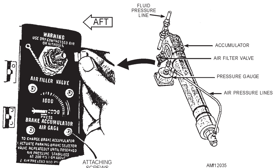
Figure 12-35.—Accumulator air charge valve and gauge installation.
