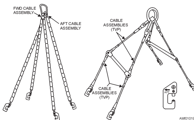
Figure 1-19.—Wire rope slings.
