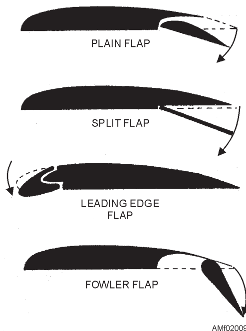
Figure 2-9.—Types of flaps.
