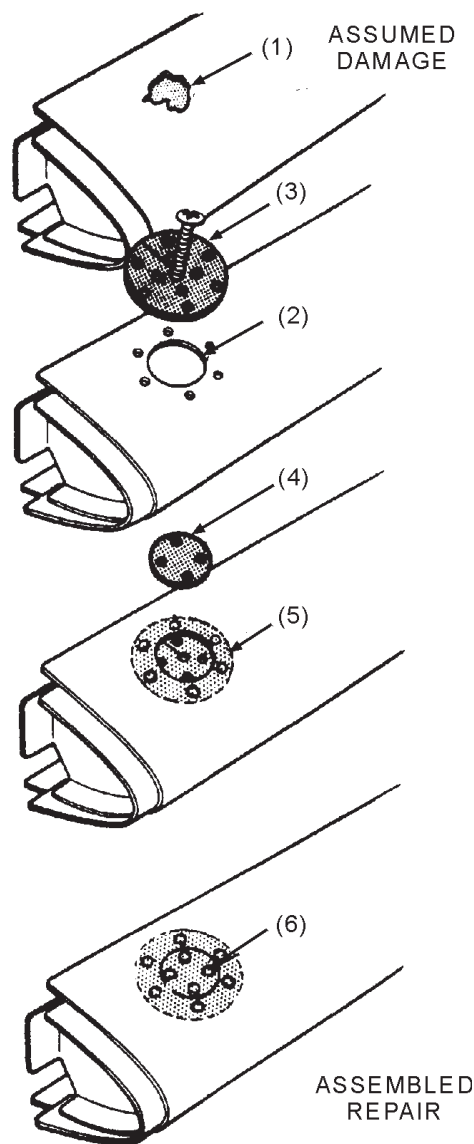
Figure 4-60.—Repair of small holes in skin with flush patch.
