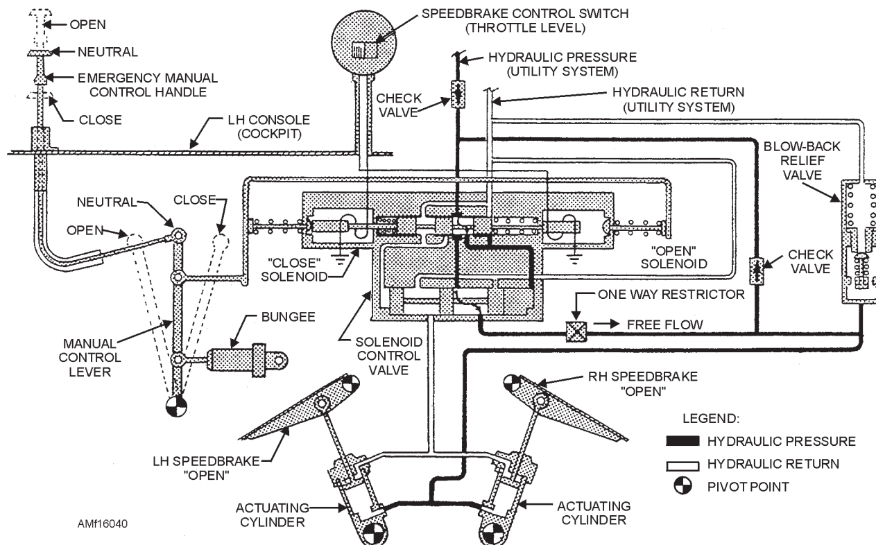
Figure 16-40.—Speed brake control system.
