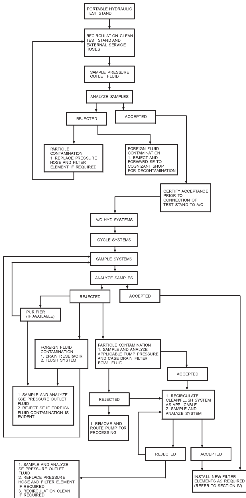
Figure 8-7.—Sequence control chart for aircraft system decontamination.
