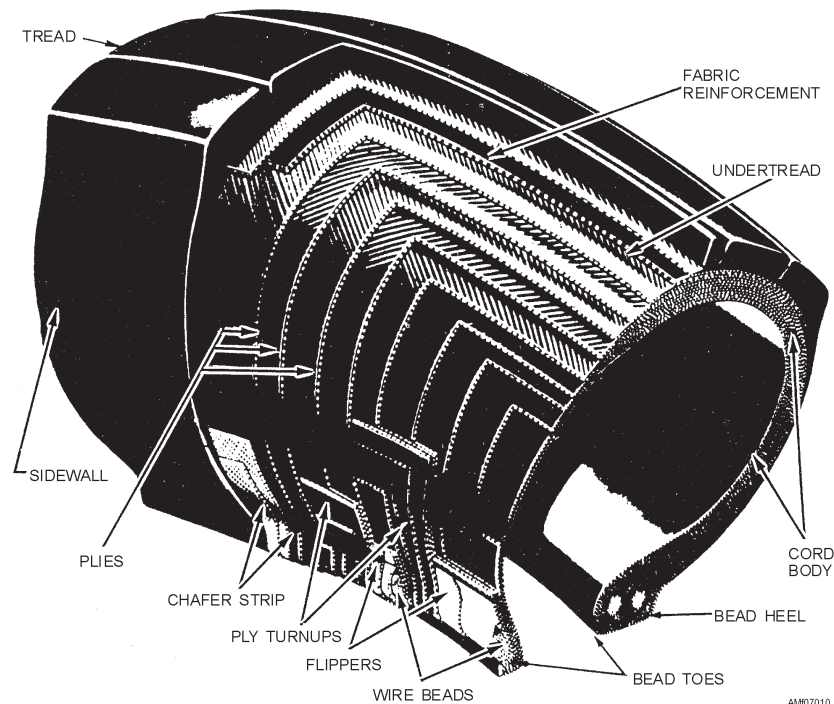
Figure 7-10.—Sectional view of aircraft tire showing construction details.
