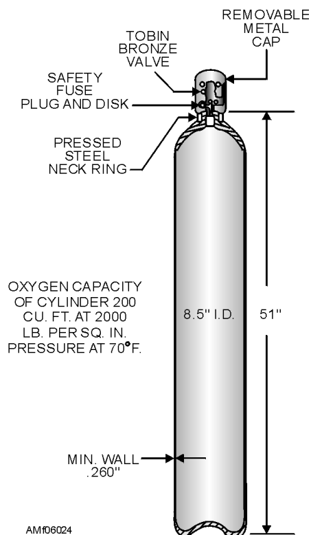
Figure 6-24.—Typical oxygen cylinder.
