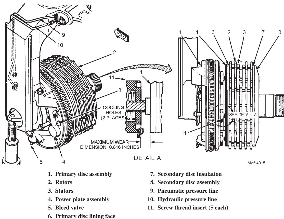
Figure 14-15.—Wheel brake.
