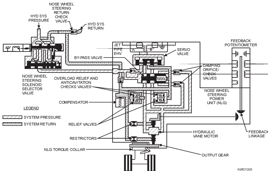
Figure 1-6.—Nosewheel steering system schematic.
