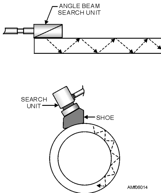
Figure 6-14.—Angle-beam inspection.
