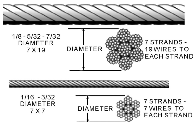
Figure 3-32.—Cable cross section.
