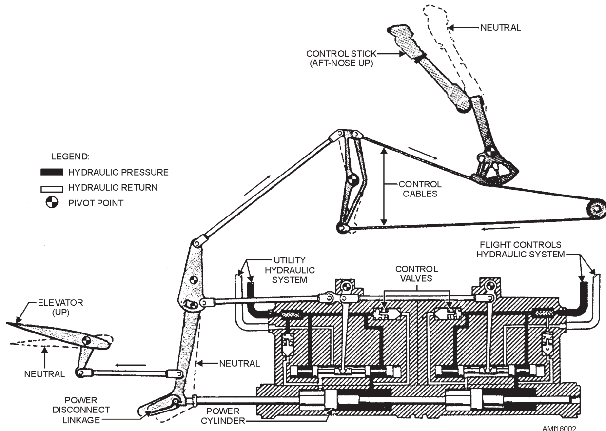
Figure 16-2.—Hydraulically powered elevator control system.
