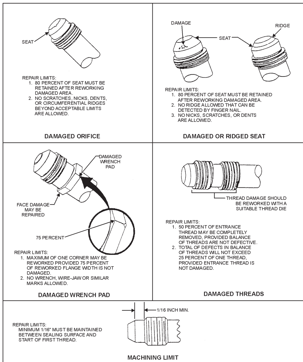
Figure 10-48.—Reworking damaged fittings.
