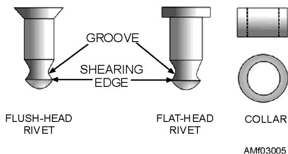
Figure 3-5.—Hi-shear rivet.
