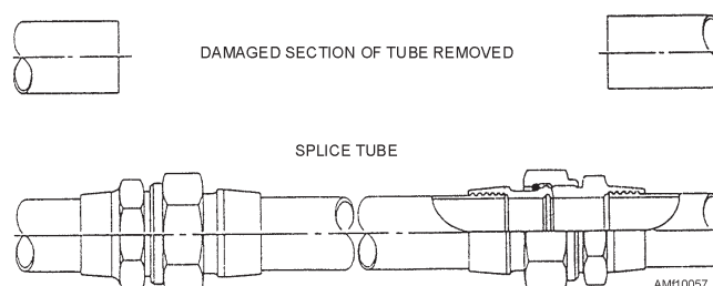
Figure 10-57.—Splice assembly repair.
