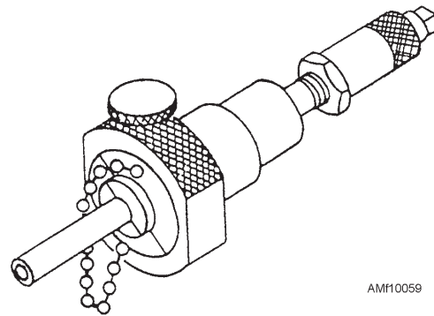
Figure 10-59.—Dynatube swaging process.
