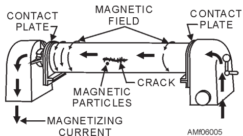
Figure 6-5.—Creating a circular magnetic field in a part.
