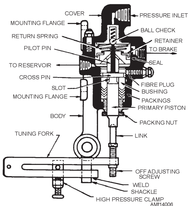
Figure 14-6.—Power brake control valve (pressure ball check type).
