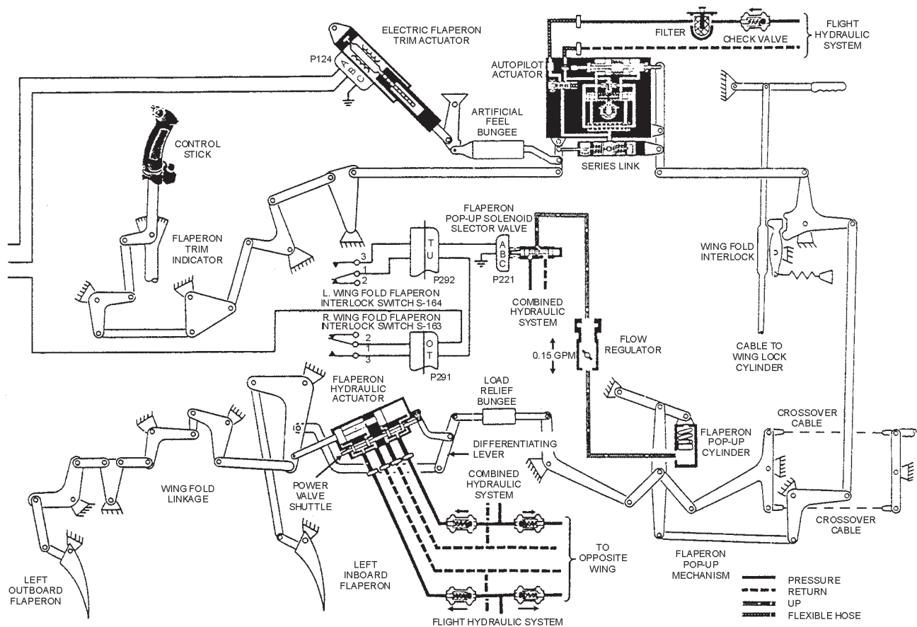
Figure 16-12.—Flaperon control system.
