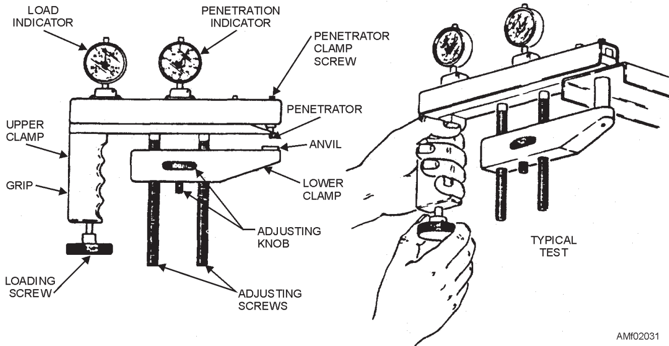
Figure 2-31.—Riehle portable hardness tester.
