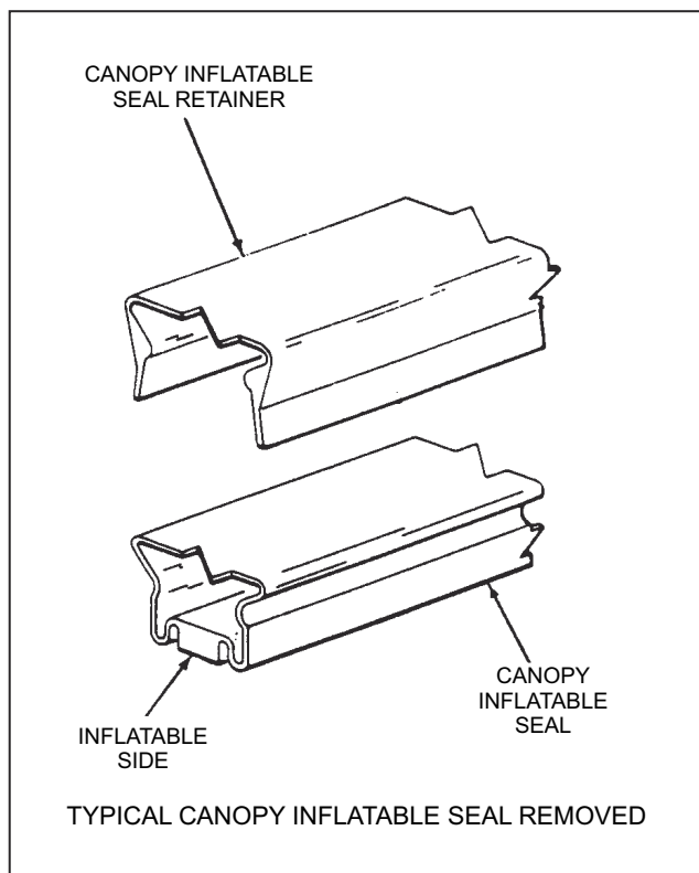
Figure 3-3.—Canopy inflatable seal (removed).
