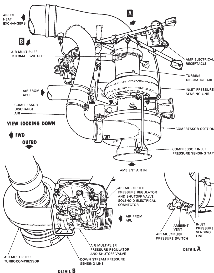
Figure 6-2.—AMP installation.
