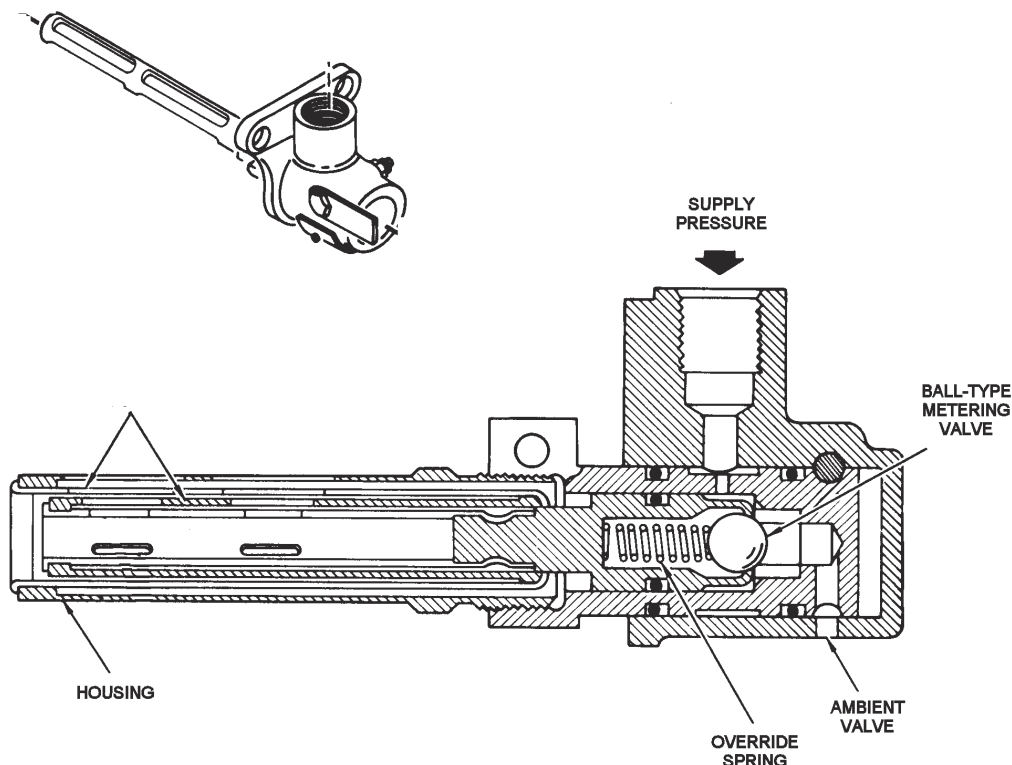
Figure 5-4.—Wing leading edge thermostat.
