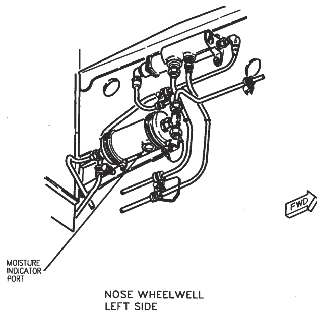
Figure 5-27.—Radar air desiccator.
