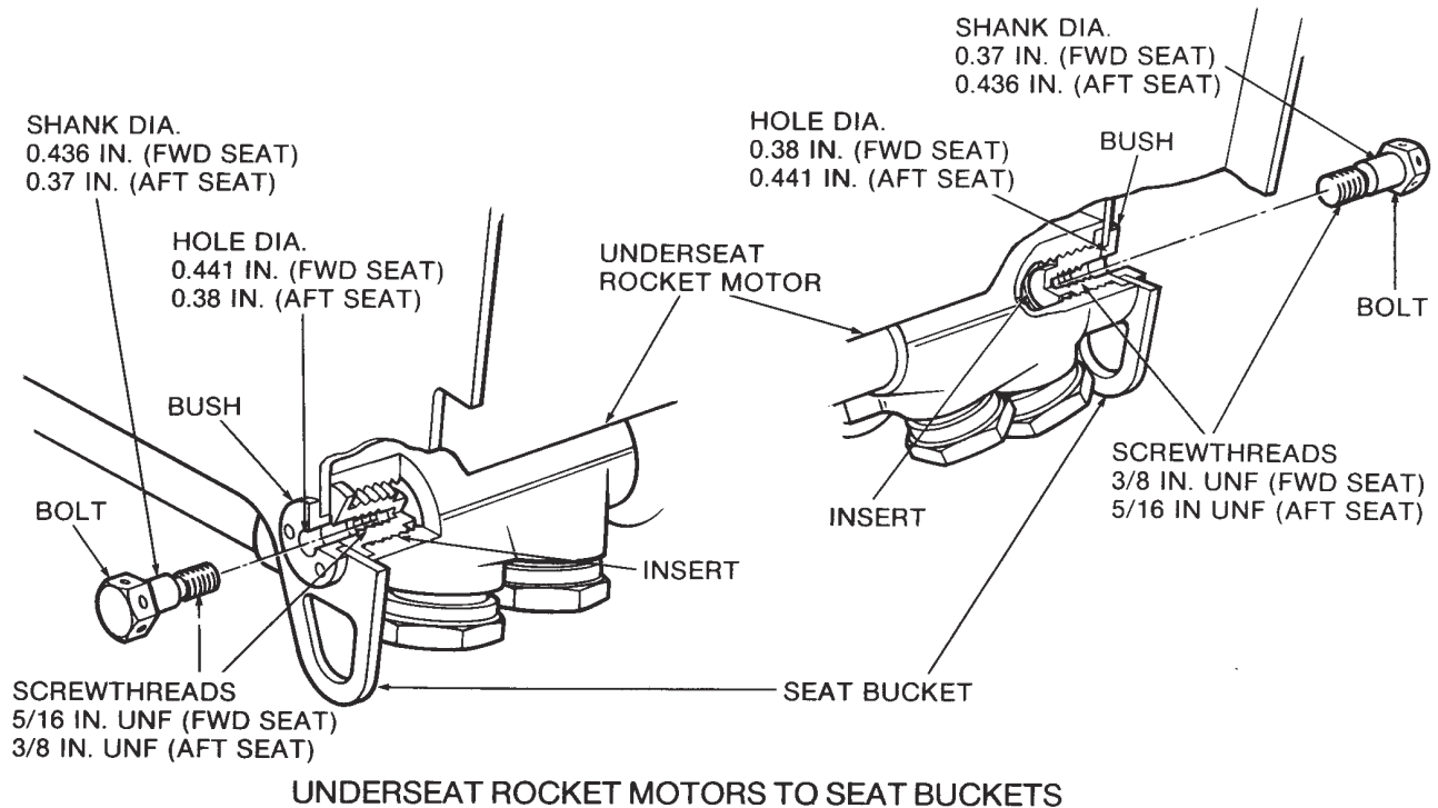
Figure 2-19.—Underseat rocket motor mounting bolt sizes (SJU-17(V)2/A).
