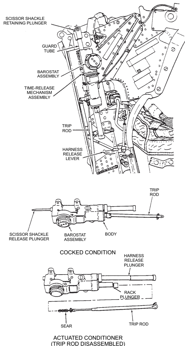
Figure 1-8.—Time-release mechanism.
