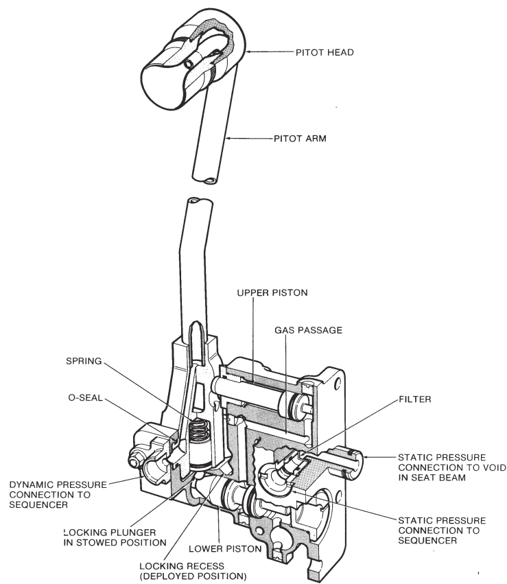
Figure 2-12.—Pitot assembly, right hand.
