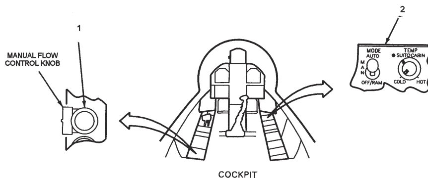
Figure 5-17.—ECS panel assembly, ECS MODE switch suit/cabin temp control.
