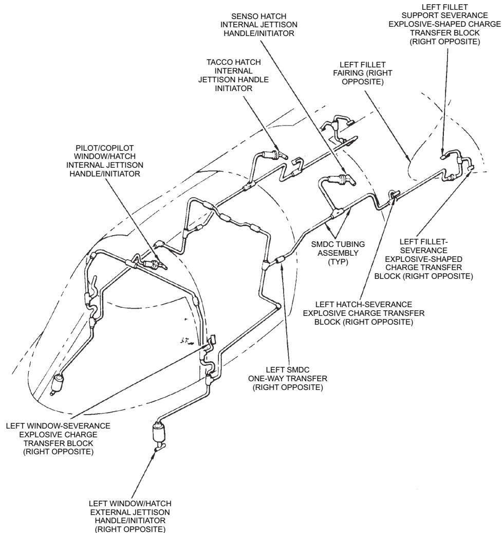
Figure 3-8.—Emergency egress system components and plumbing.
