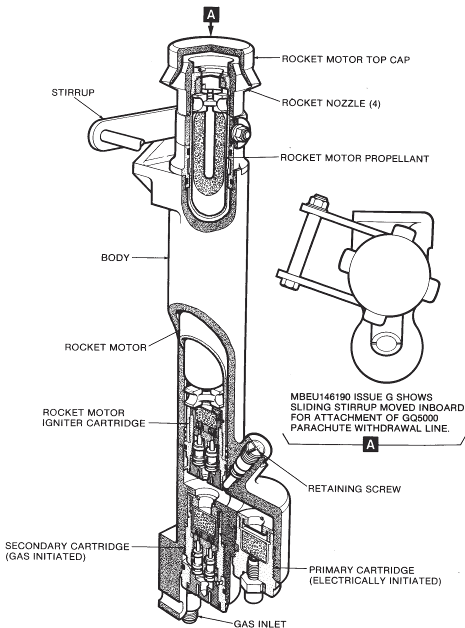
Figure 2-10.—Parachute deployment rocket motor MK 122 MOD 0.
