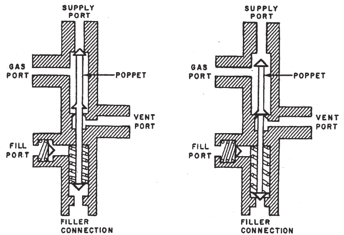
Figure 7-9.—Filler valve.
