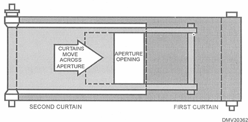
Figure 7-12. —Focal-plane shutters.
