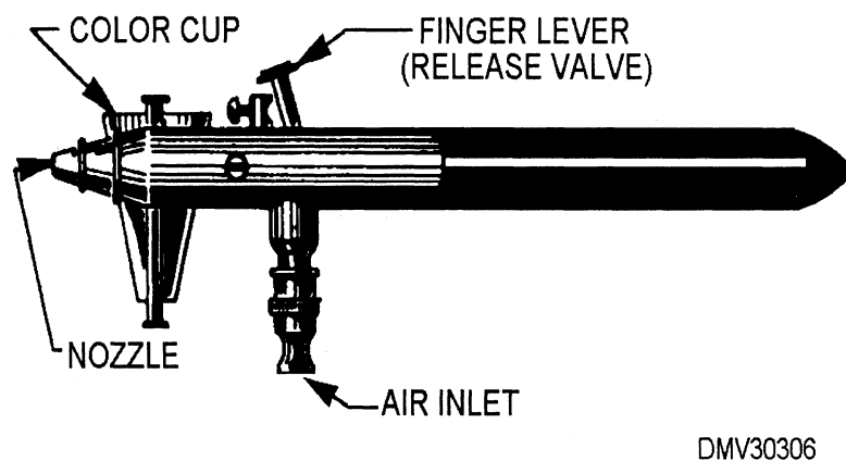
Figure 6-1. —Airbrush nomenclature.
