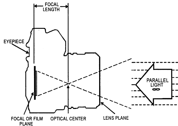
Figure 7-17. —The focal length of a standard lens.
