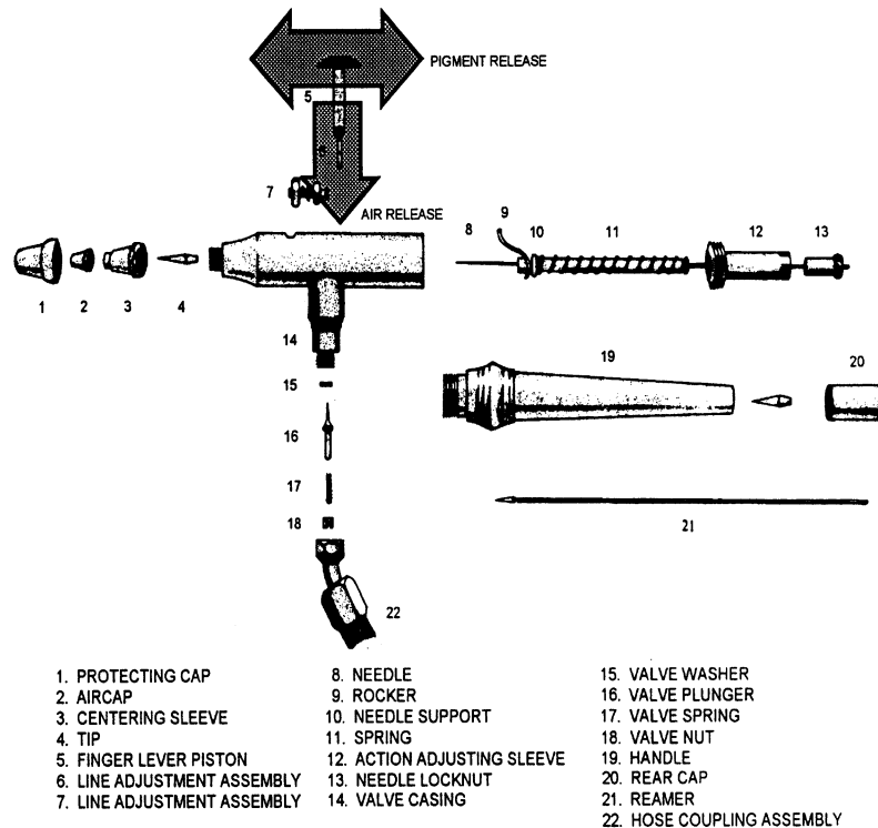
Figure 6-3.—Parts of a double-action airbrush.
