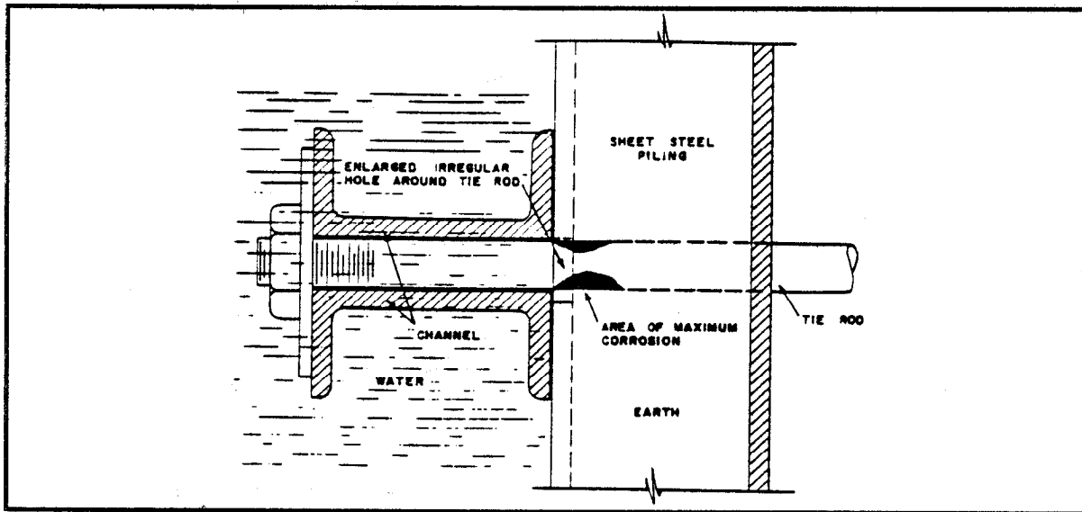
Figure 6-4 Tie-Rod Corrosion
