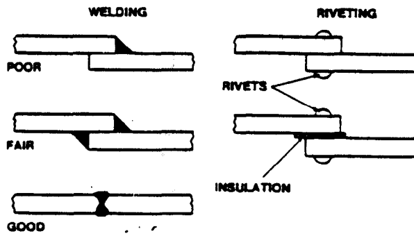
FIGURE 11—Joining Practices
