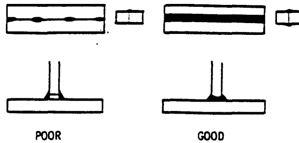
FIGURE 11—Joining Practices
