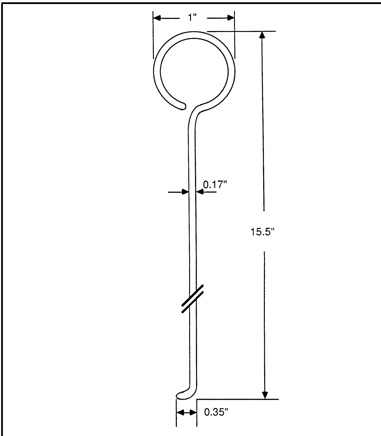
FIGURE 7-6 A Shell Thickness Indicator is used to Determine the Thickness of the Remaining Shell
