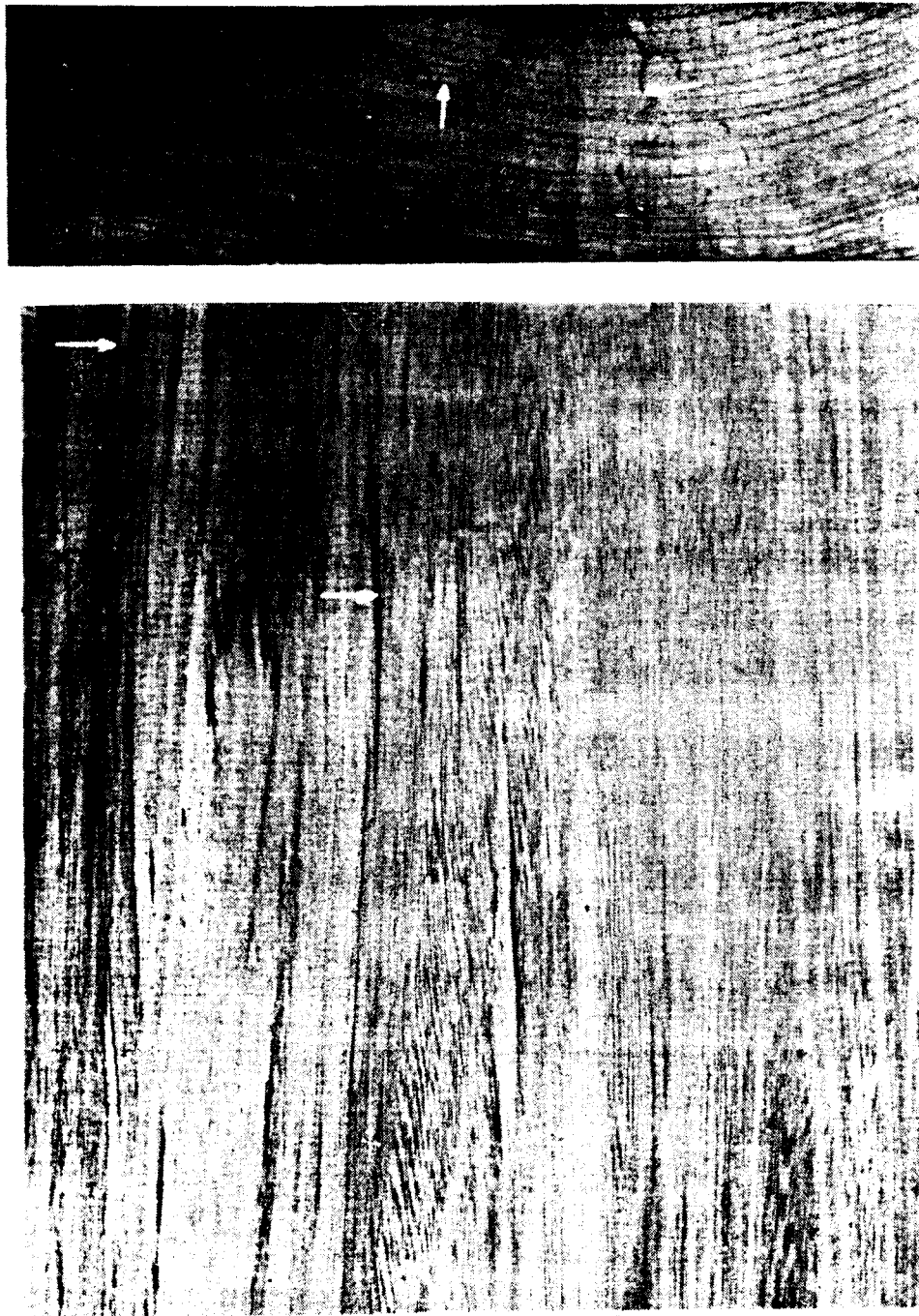
FIGURE 4-7 Discoloration from White Rot on End Grain, Characterized by Mottling and Dark Zone Lines (arrows) Bordering the Abnormally Light-Colored Areas (top) and Side Grain of the Same Board (bottom)
