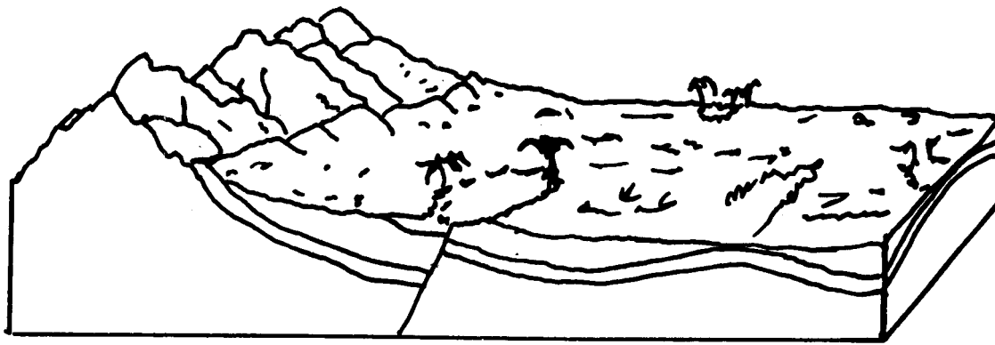
Figure 2-37. Oasis
