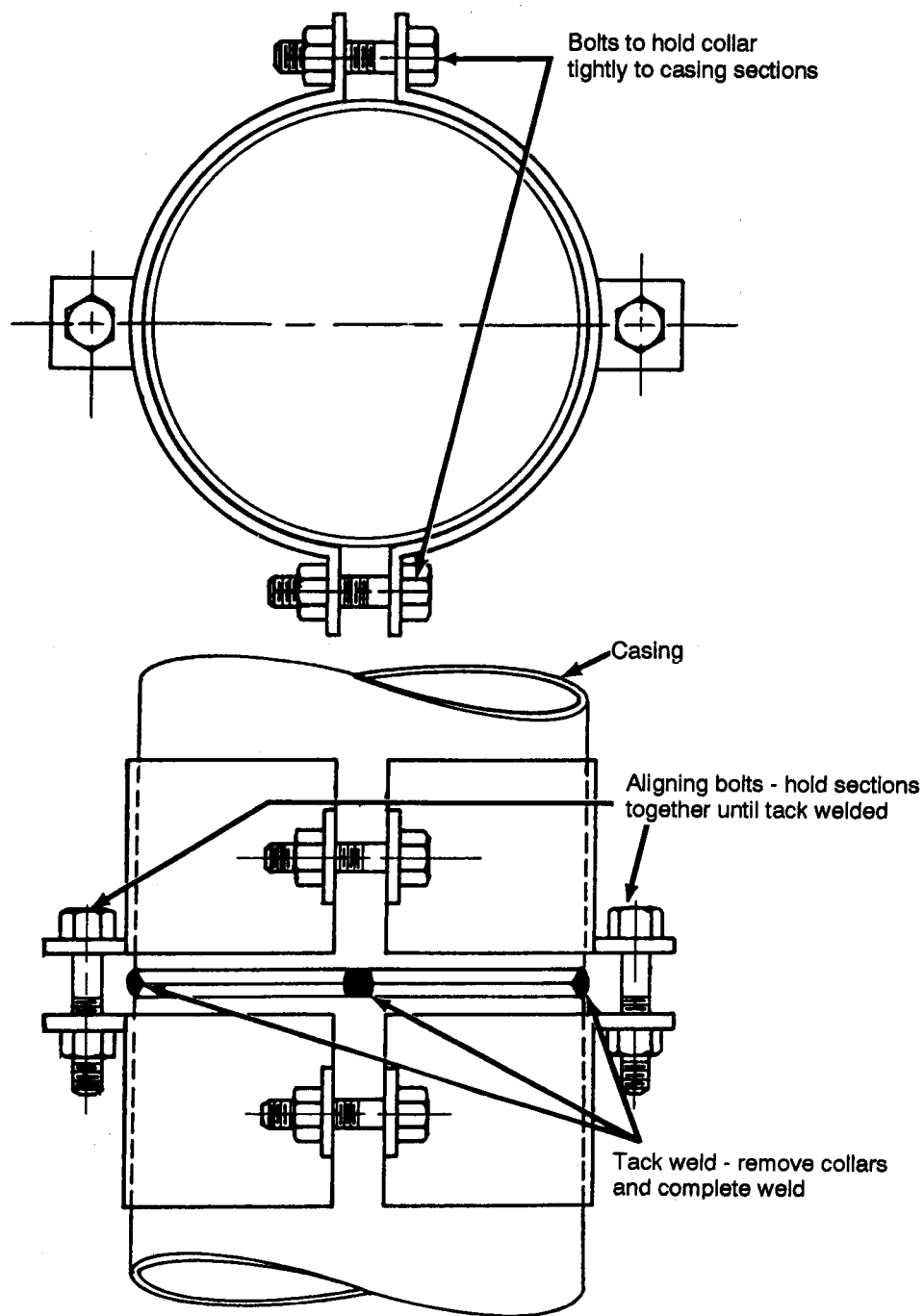
Figure 9-15. Alignment collar
