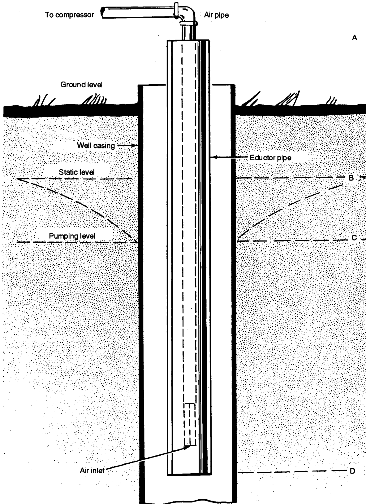
Figure 4-11. Submergence percentage
