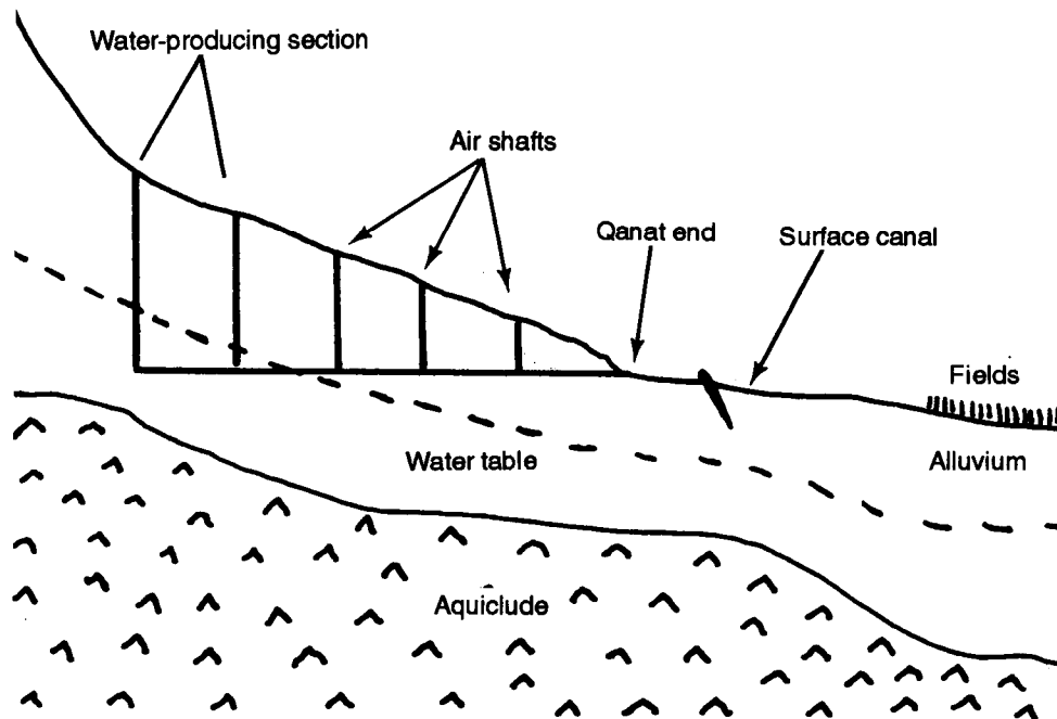
Figure 2-38. Qanat system
