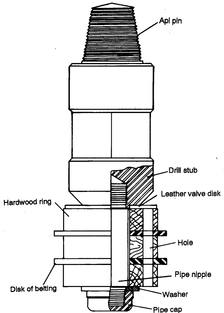
Figure 7-2. Surge block
