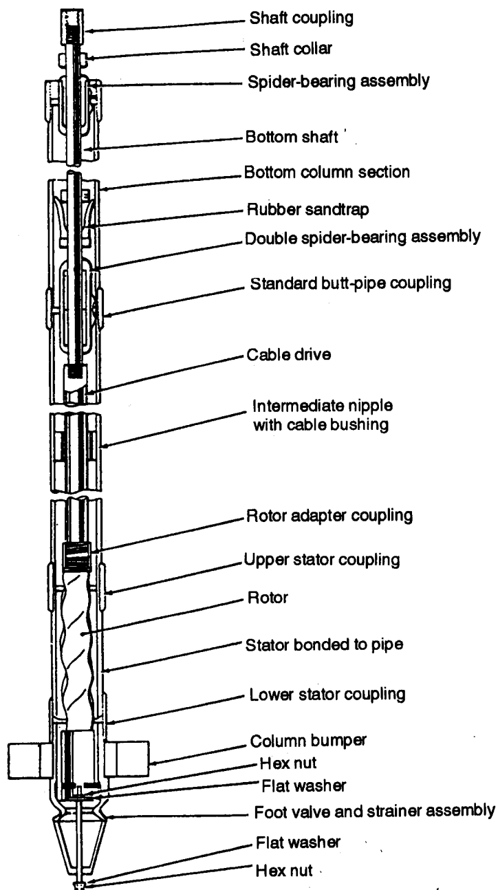
Figure 4-7. Helical-rotor pump
