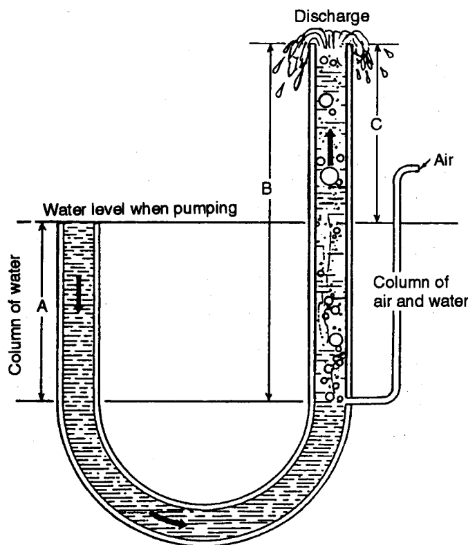
Figure 4-9. Air-lift principle
