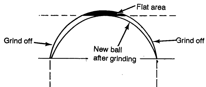
Figure E-14. Reconditioned button
