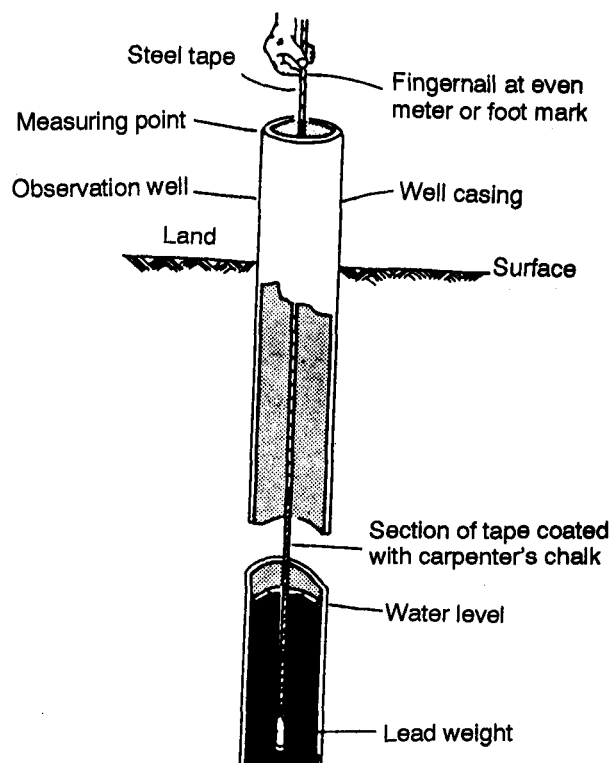
Figure 8-3. Steel-tape measurement method
