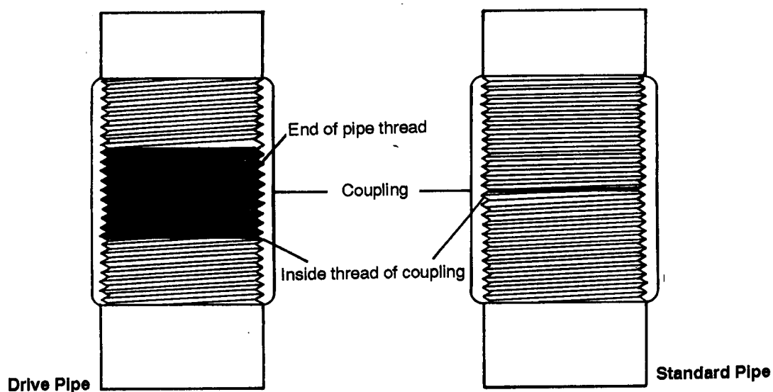
Figure 9-8. Butt joint
