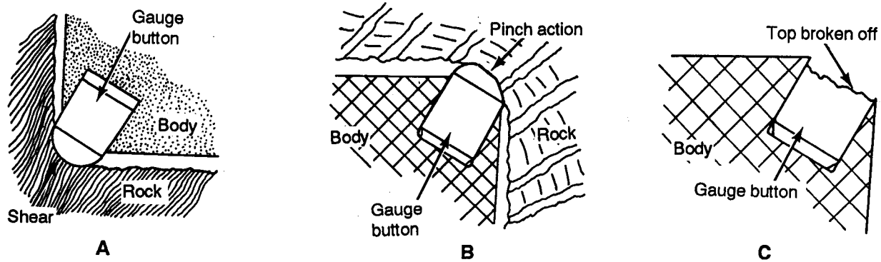
Figure E-4. Carbide shear
