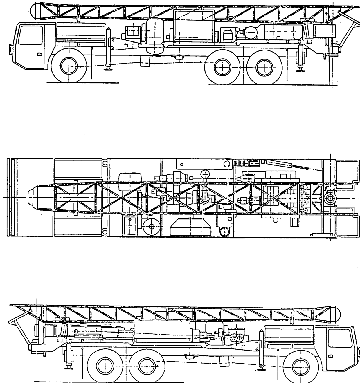
Figure 3-1. 600-foot well-drilling machine
