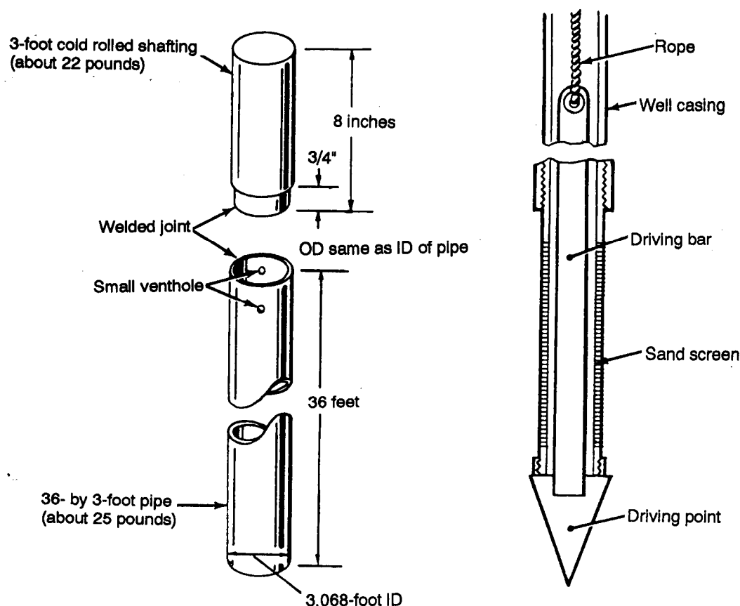
Figure 9-16. Drive point
