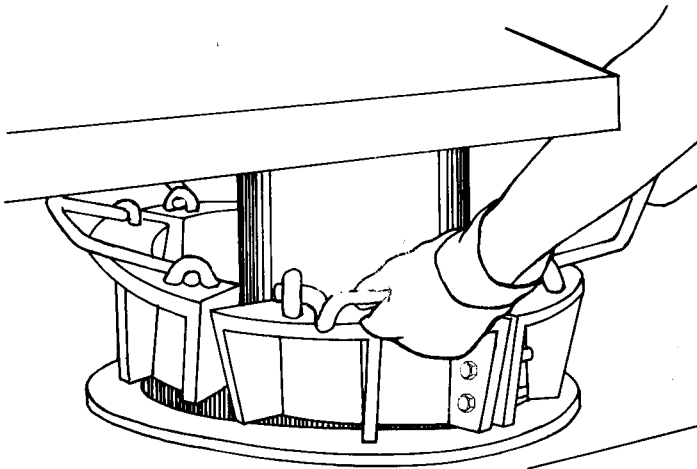
Figure 3-19. Setting slips
