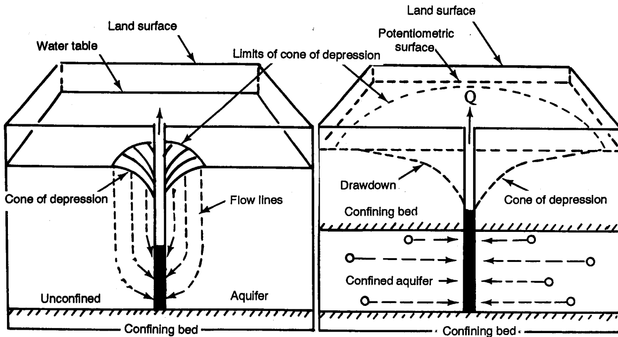
Figure 2-10. Drawdown
