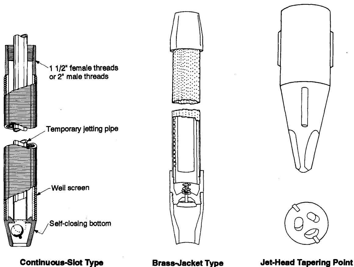
Figure 9-5. Well points
