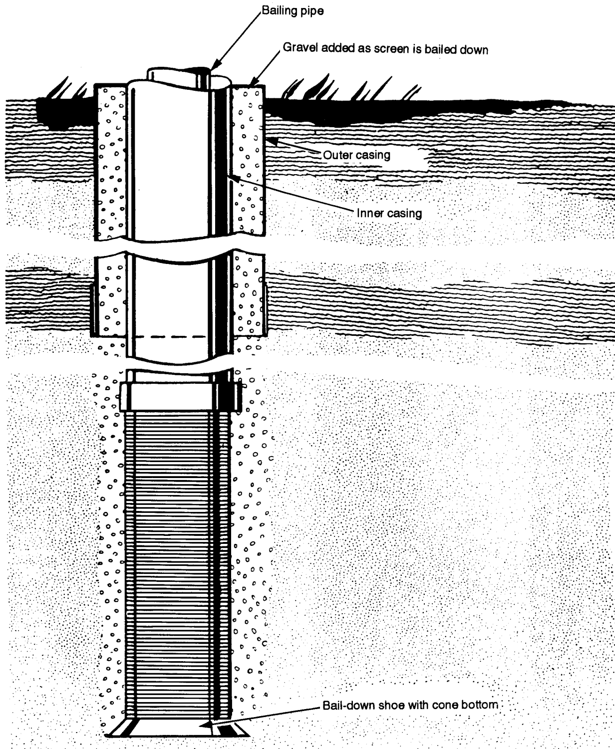
Figure 6-12. Bail-down placement
