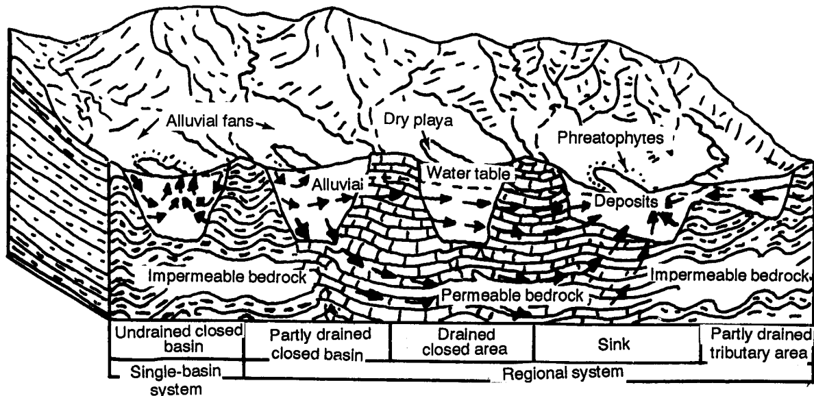
Figure 2-21. Alluvial basin
