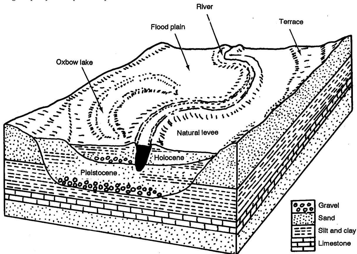
Figure 2-18. Alluvial valley
