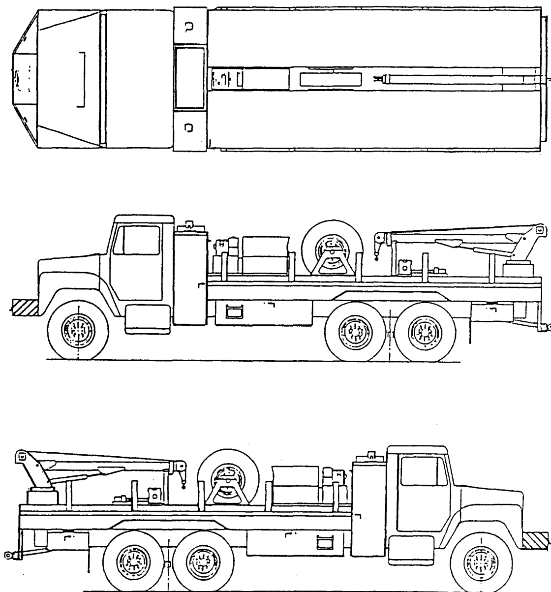
Figure 3-2. Support vehicle
