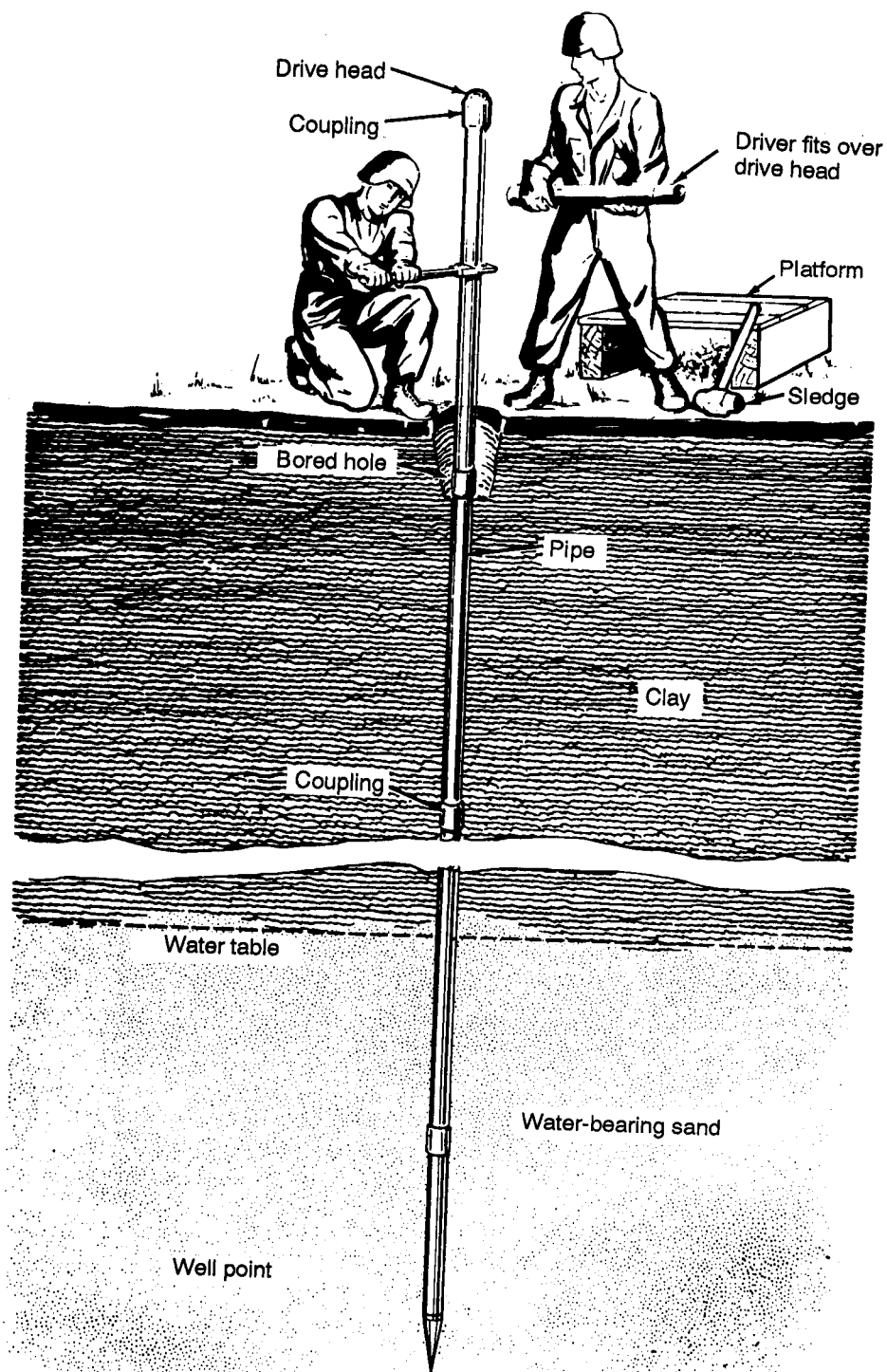
Figure 9-6. Drive-point well
