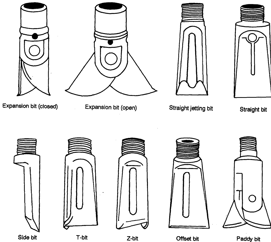
Figure 9-3. Bits
