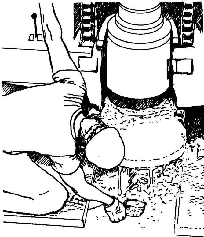
Figure 3-17. Taking samples
