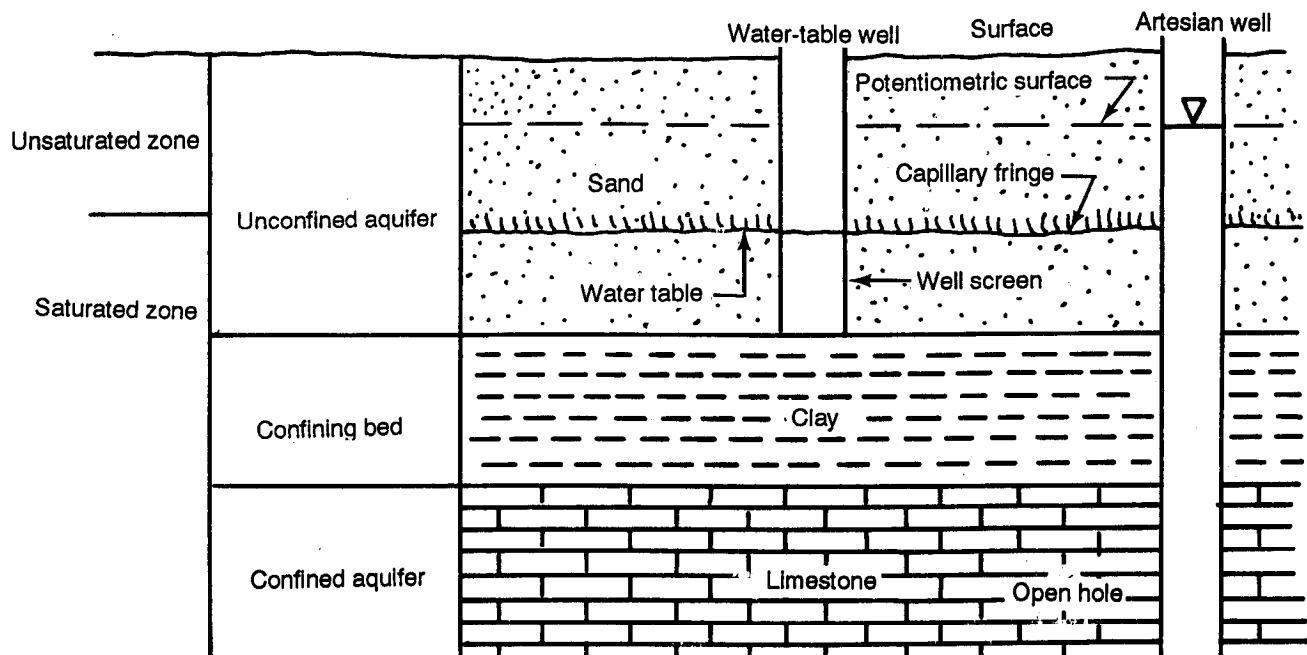
Figure 2-12. Unconfined aquifer
