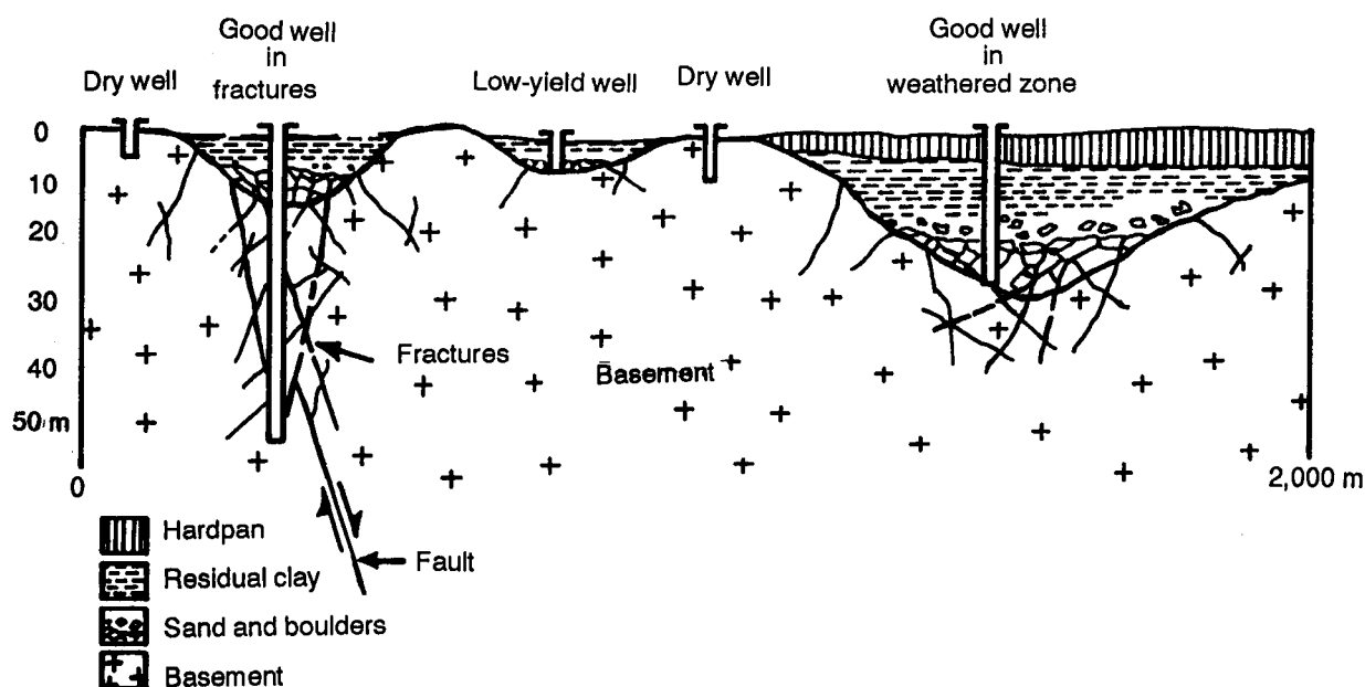
Figure 2-15. Catchment
