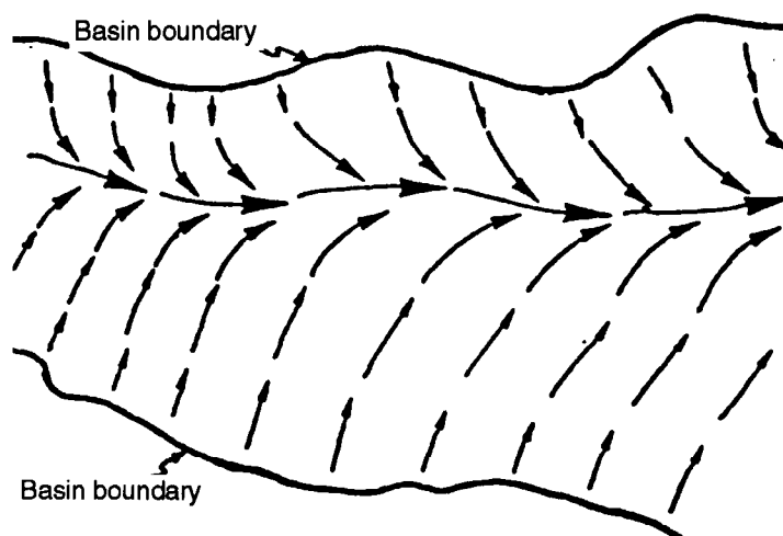
Figure 2-31. Groundwater flow from recharge to discharge areas
