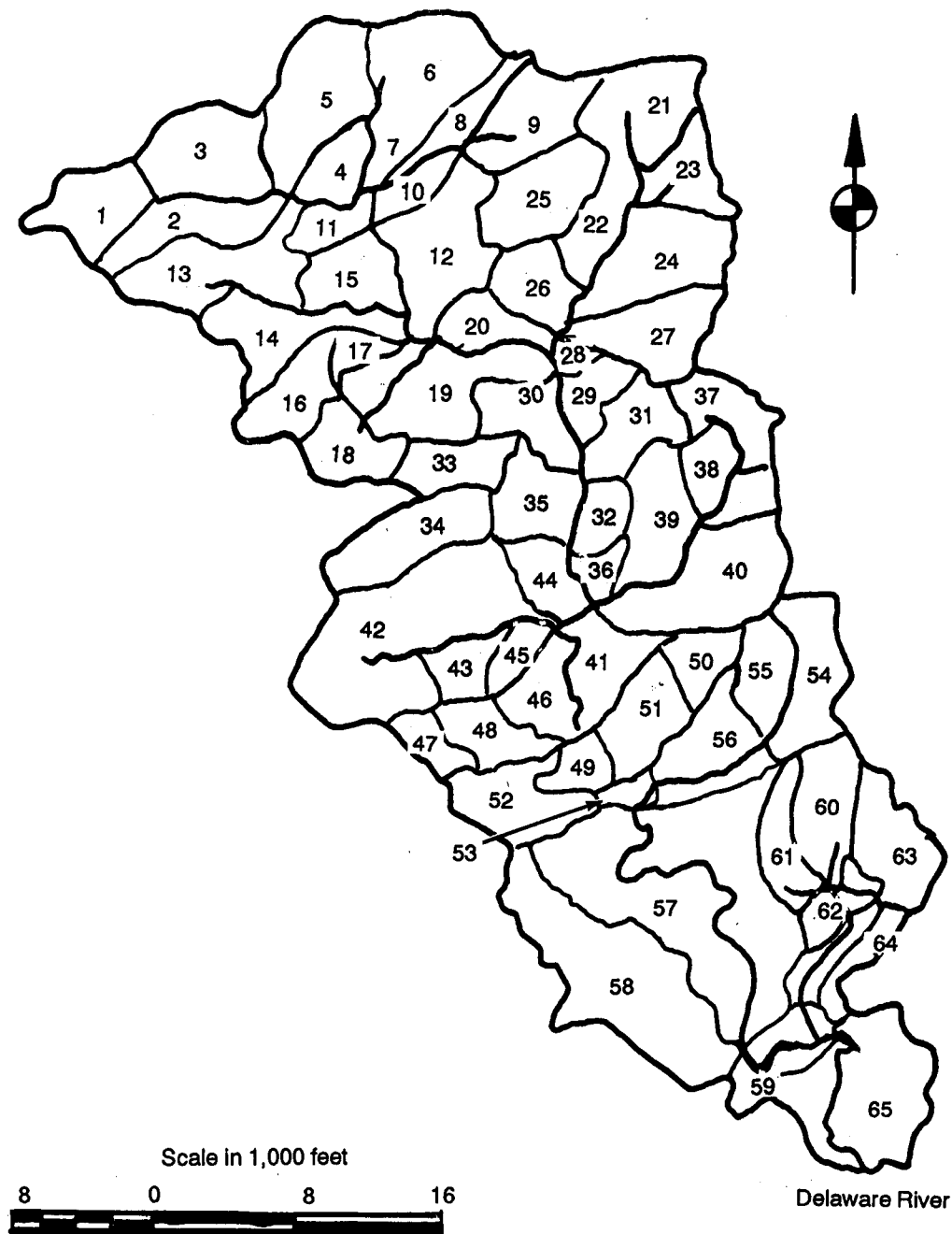
Figure 2-4. Hydrographic basin
