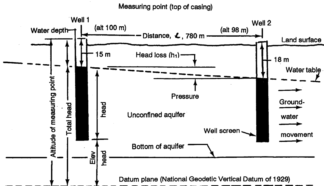
Figure 2-11. Hydraulic gradient
