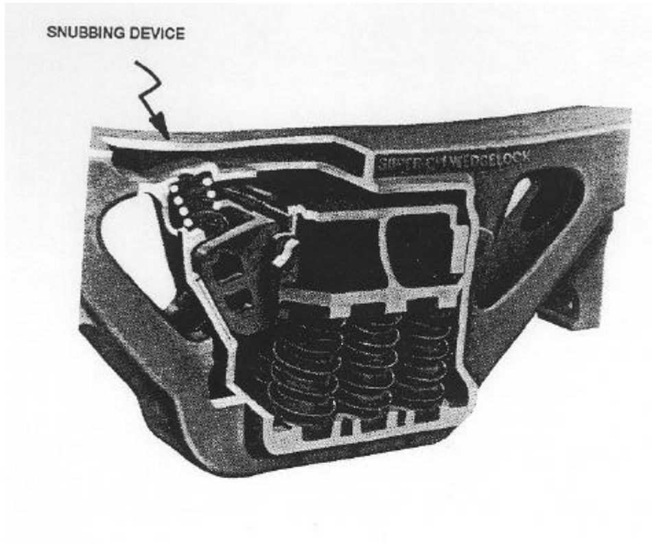
Figure A-19. Example of a snubbing device.
