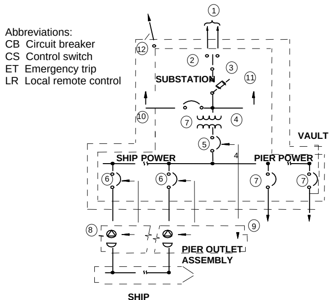
Figure 12-12 Preferred ship-to-shore circuit arrangement
