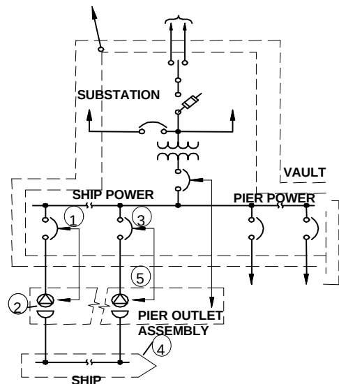
Figure 12-13 Procedures in safely energizing a ship from a shore electrical circuit
