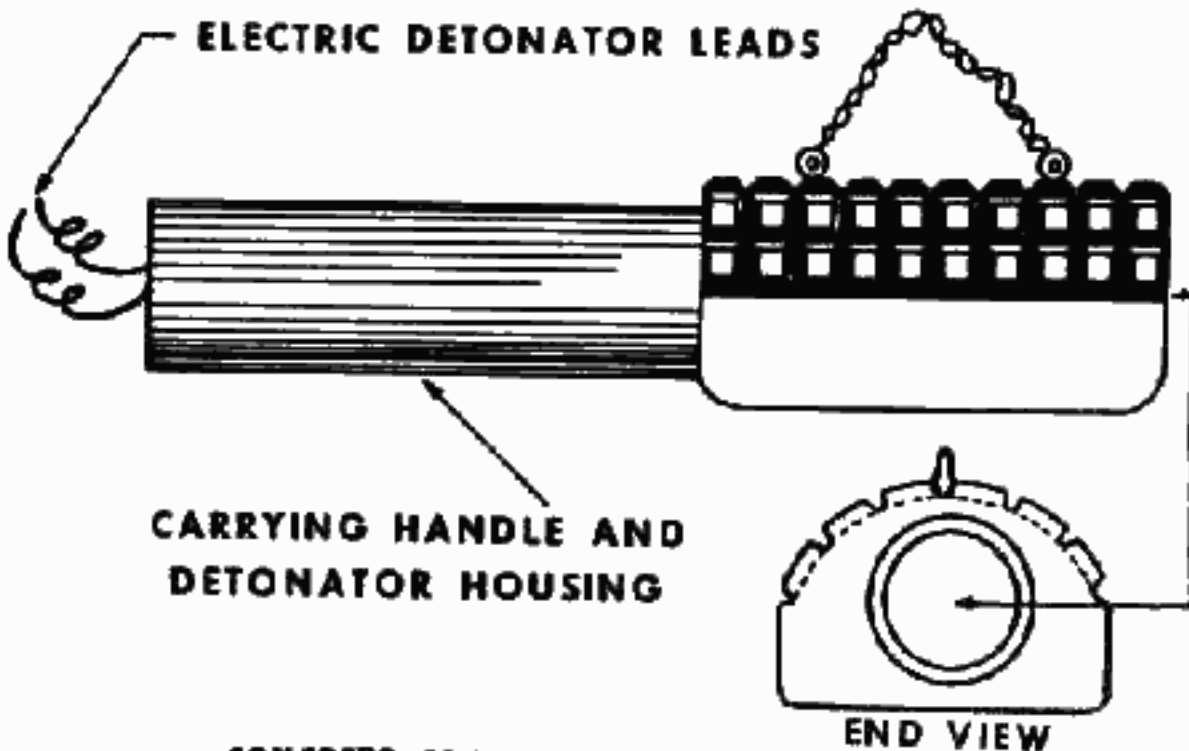
CONCRETE FRAGMENTATION MINE 25 Concrete Mound Mine
