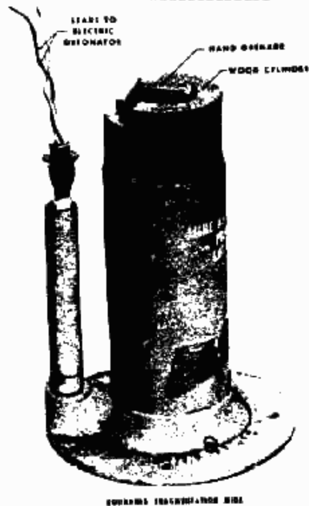
BOUNDING FRAGMENTATION MINE
