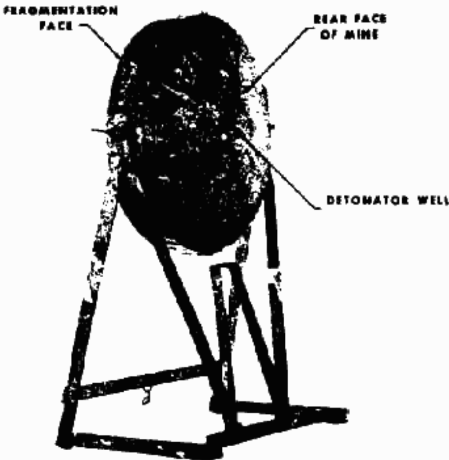
DH-10 DIRECTIONAL MINE
