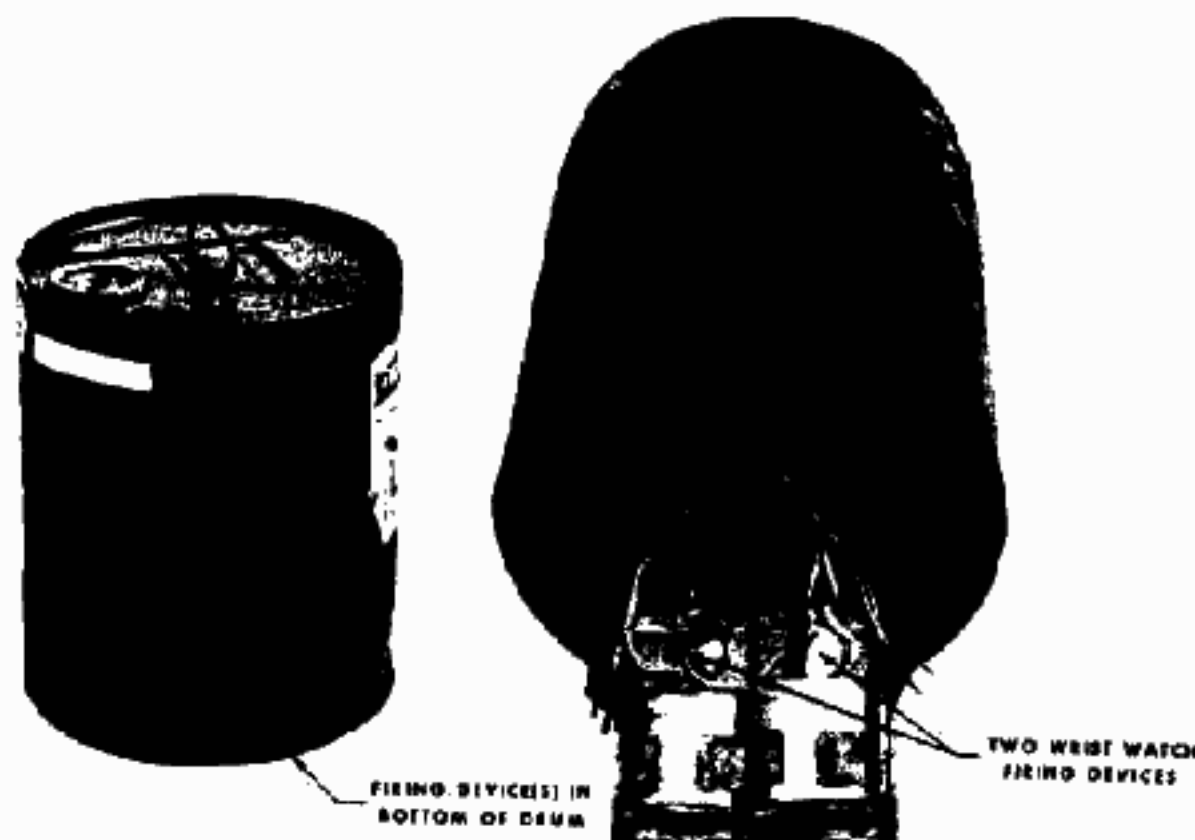
OIL DRUM CHARGE
