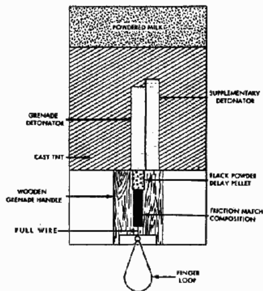
MILK CAN HAND GRENADE
