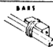
EXPLOSIVE CHARGE DIVIDED IN HALF, OFF SET MINIMUM THICKNESS OF WEB
