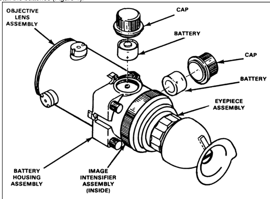
Figure 1. Battery emplacement.
