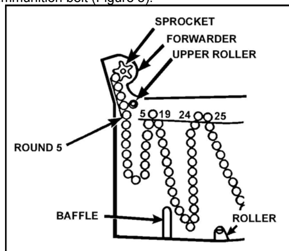
Figure 5. Rounds in forwarder.
