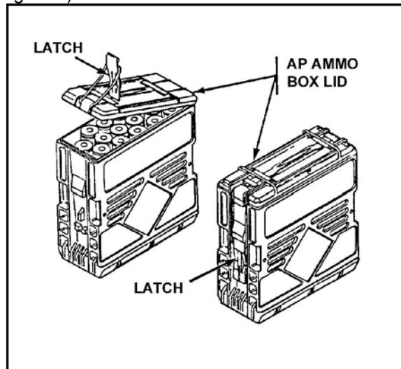
Figure 3. Ammunition box.
