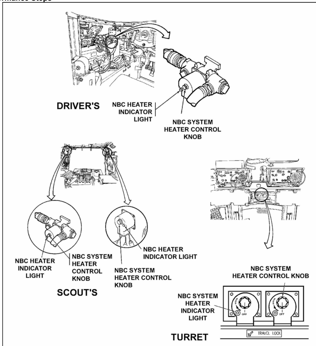
Figure 4. NBC heater.
