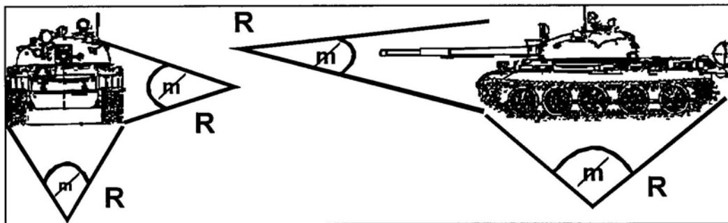
Figure 8. Use of the mil-relation formula.
