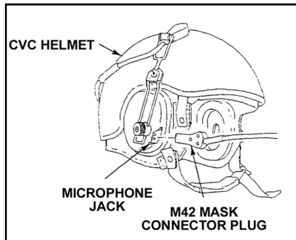
Figure 2. M42 connector.
