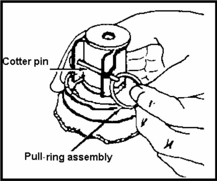
Figure 052-192-1118-2 Inserting the Cotter Pin
