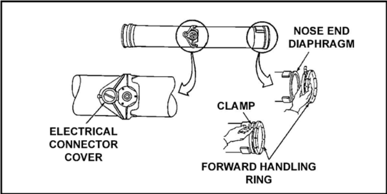
Figure 2. TOW missile.
