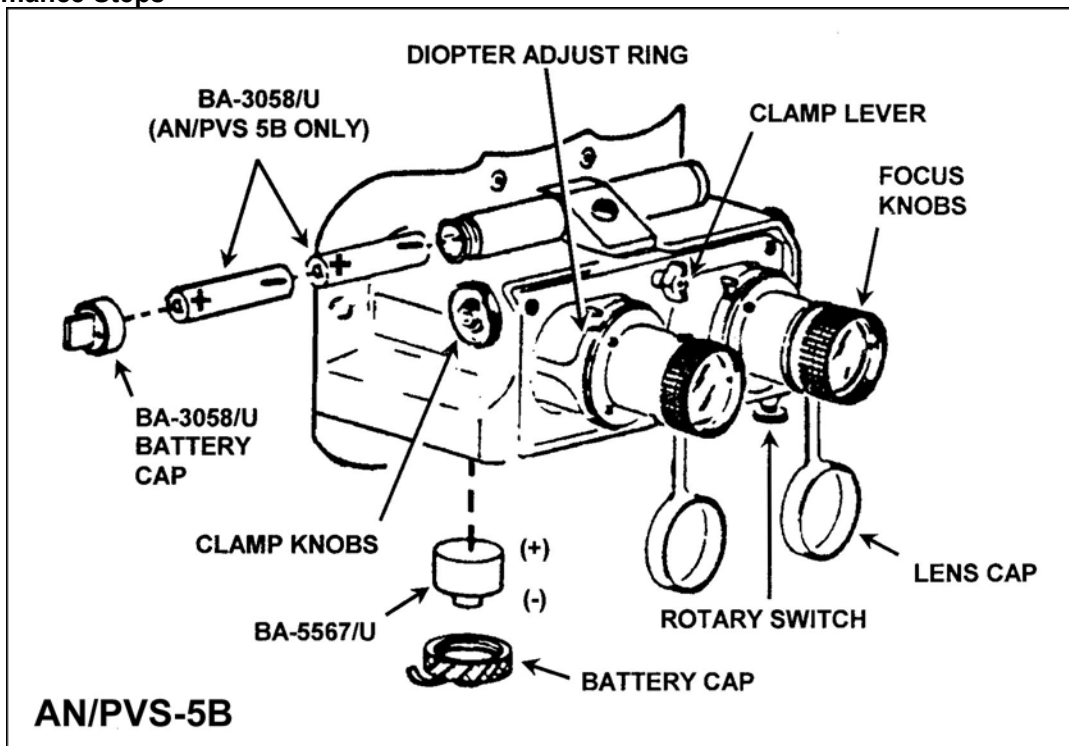
Figure 3. AN/PVS-5B goggles.
