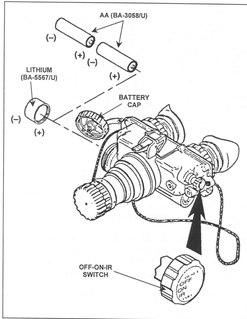
Figure 4. Battery installation.
