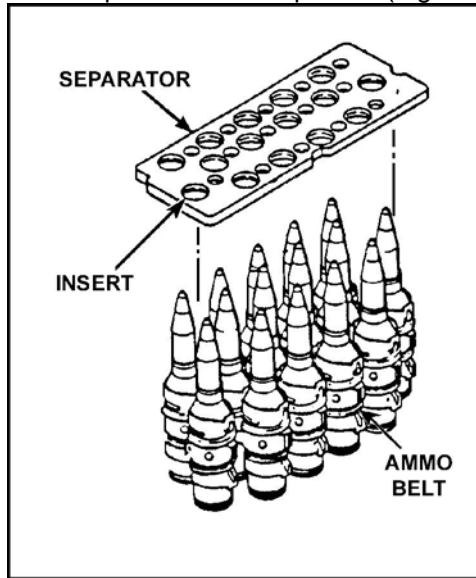
Figure 2. Separator.
