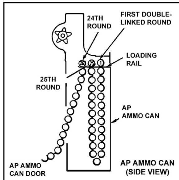
Figure 4. Loading rail.
