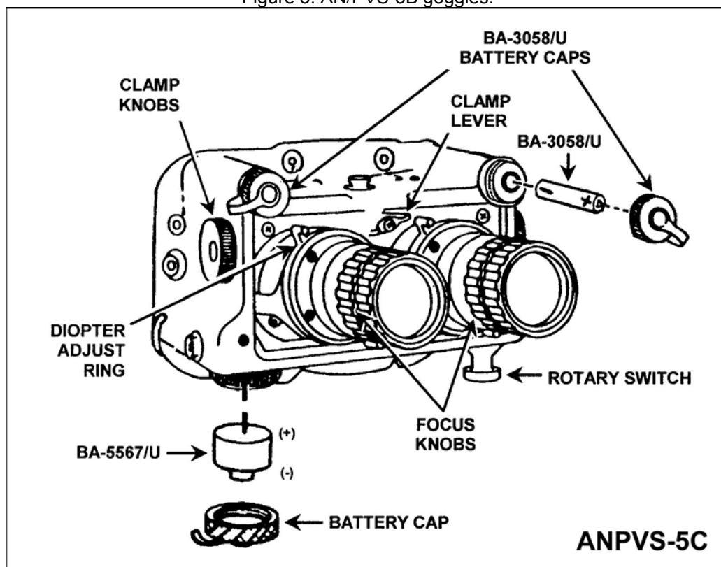
Figure 4. AN/PVS-5C goggles.
