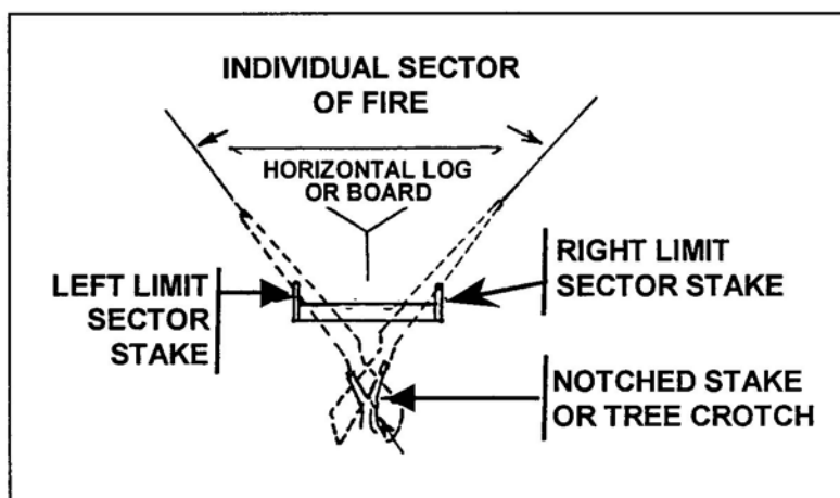
Figure 1. Sector stakes.
