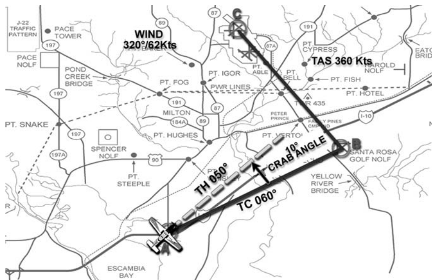
Figure 4.5-8 Crab Angle
