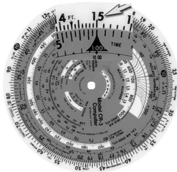
Figure 4.3-16 Time 1
