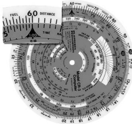
Figure 4.3-7 Rate Index
