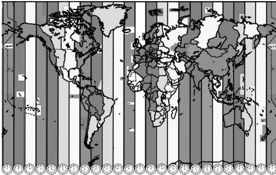
Figure 4.2-11 Time Zones
