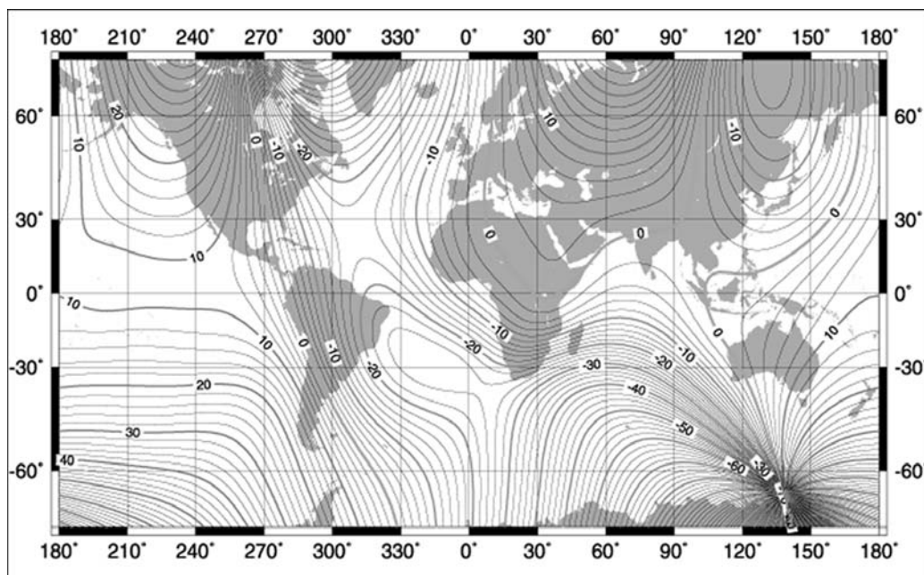
Figure 4.2-10 Isogonic Lines
