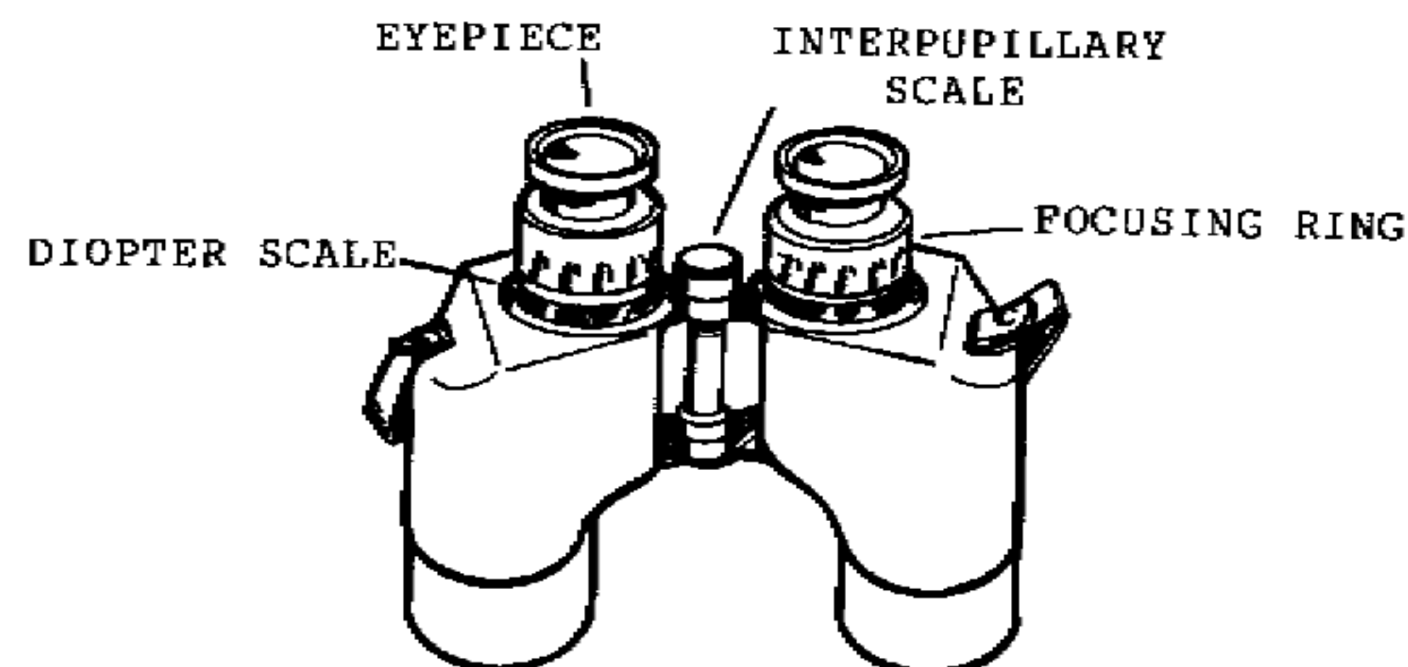
Figure 2-26. M19 binoculars.
