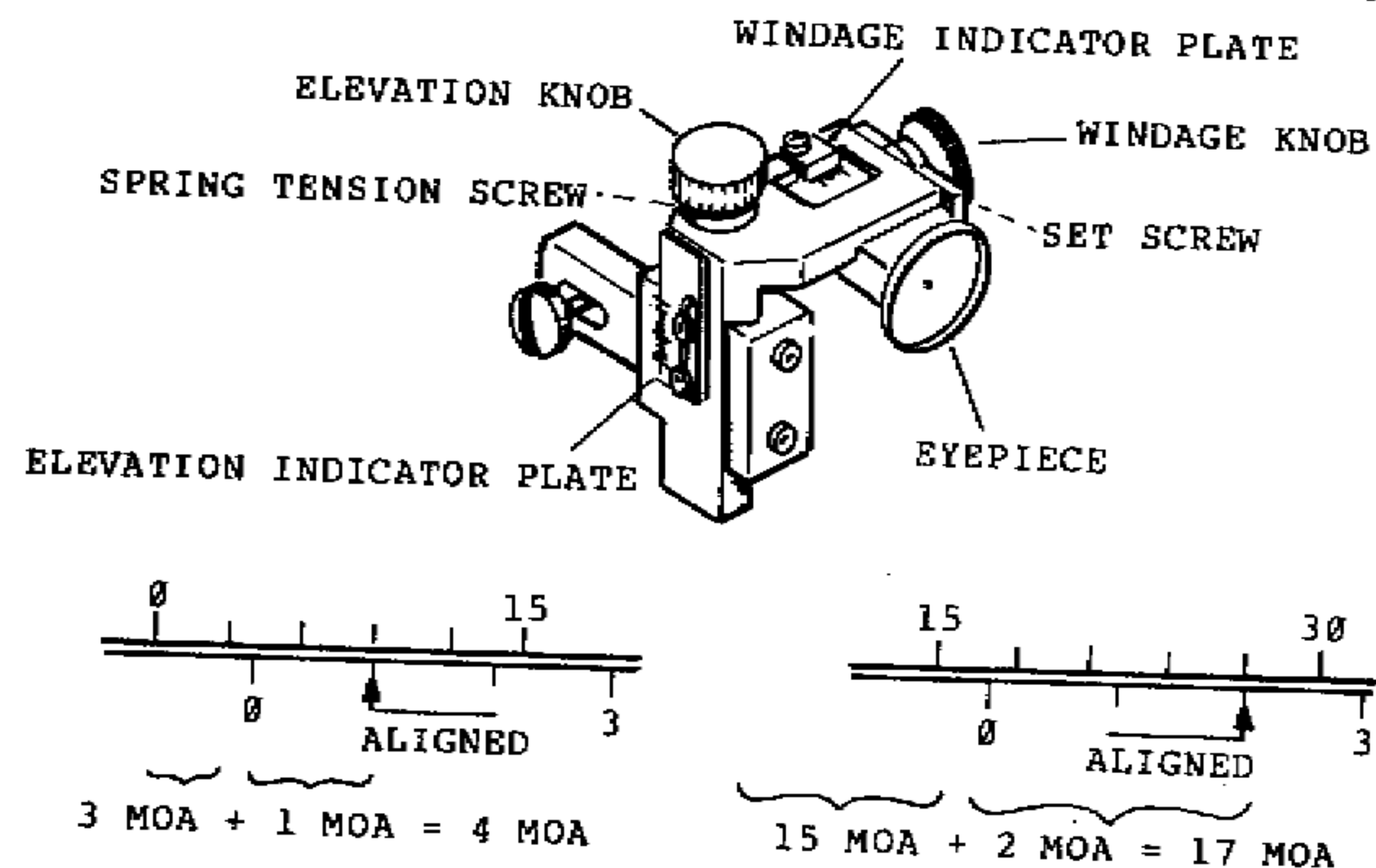
Figure 2-13. Rear sight adjustment.
