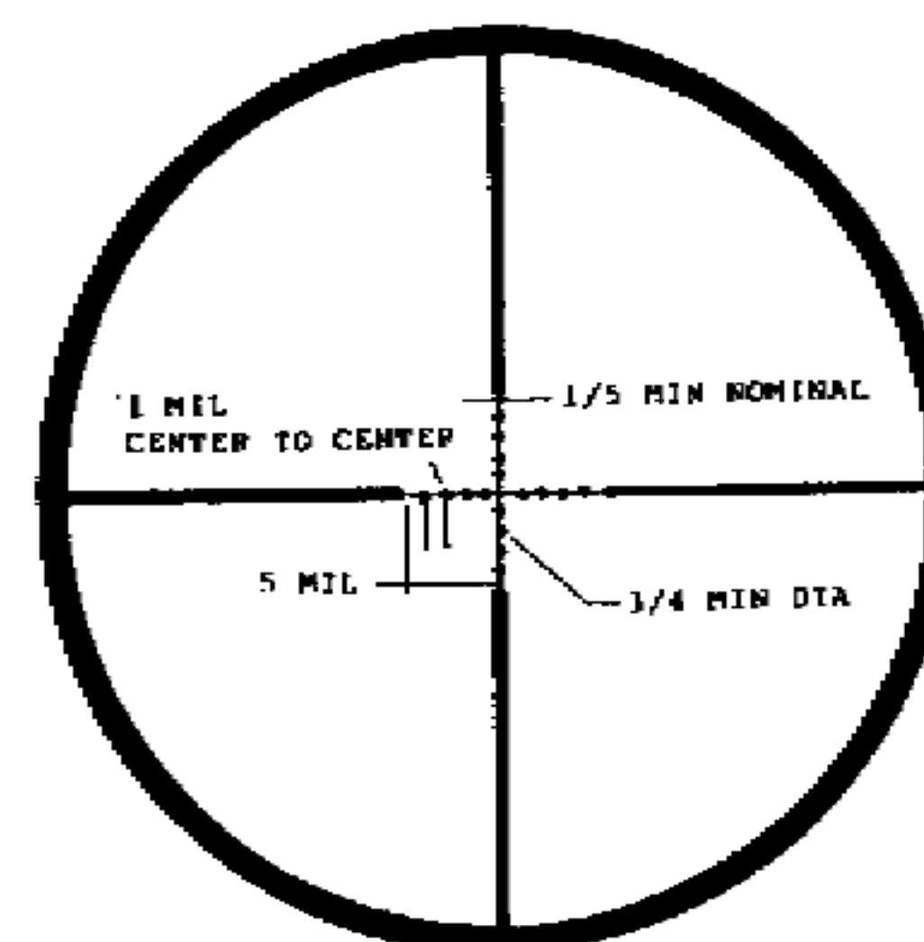
Figure 4-24. M3A sniperscope reticle.
